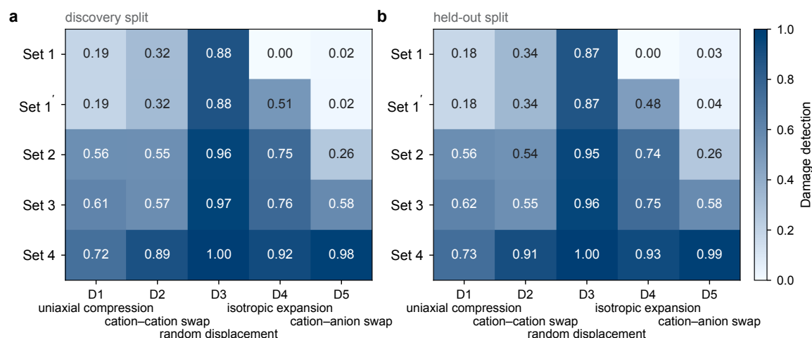
Fig. S4 Damage detection by perturbation class on the discovery and held-out splits. a , Discovery split used for law selection. b , Held-out split evaluated with the law sets fixed. Rows are PRIS law sets and columns are the D1–D5 composition-preserving perturbations. Cell colour and printed text encode the within-class damage-detection fraction on a shared scale, and the column labels define the perturbation operations.
