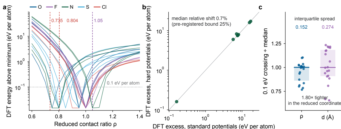
Fig. S12 The contact thresholds measured from first principles. a , Each line is one of twenty experimental compounds rigidly scaled along the reduced-contact coordinate and evaluated with plane-wave DFT. The vertical axis is the DFT energy above each compound's own minimum, and colour gives the dominant anion. The dotted horizontal line marks 0.1 eV per atom, the pre-registered cost of a chemical rather than geometric short contact. Dashed vertical lines mark the Law 1 floors of 0.735 and 0.804 and the Law 2 ceiling of 1.05. Every chemistry rises steeply below the floors, so the thresholds do not average soft and stiff cases. b , Eight compounds were recomputed with hard potentials, which freeze smaller cores, and compared with the standard set. Both axes report DFT energy excess at the floor, and the diagonal marks equality. The annotation gives the median relative shift against the threshold fixed before calculation. c , Each point is the contact at which a compound first pays the pre-registered cost. Reduced-contact and Å crossings are each normalised by their own median. Boxes span the interquartile range, and the number above each box gives its width. The crossing is 1.80 times more tightly localised in the reduced coordinate, enabling comparison across chemistries.
