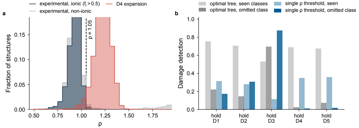
Fig. S14 Conditional contact thresholds and leave-one-damage-class-out evaluation. a , Normalised reduced-contact distributions for experimental structures separated by ionicity and for isotropically expanded structures. Filled step curves identify the cohorts, and the vertical dashed line marks the conditional upper bound. b , Damage detection for a depth-limited tree and a single \rho threshold when each perturbation class is omitted in turn. Grey and blue identify the two model classes, while pale and solid bars distinguish retained and omitted perturbation classes.
