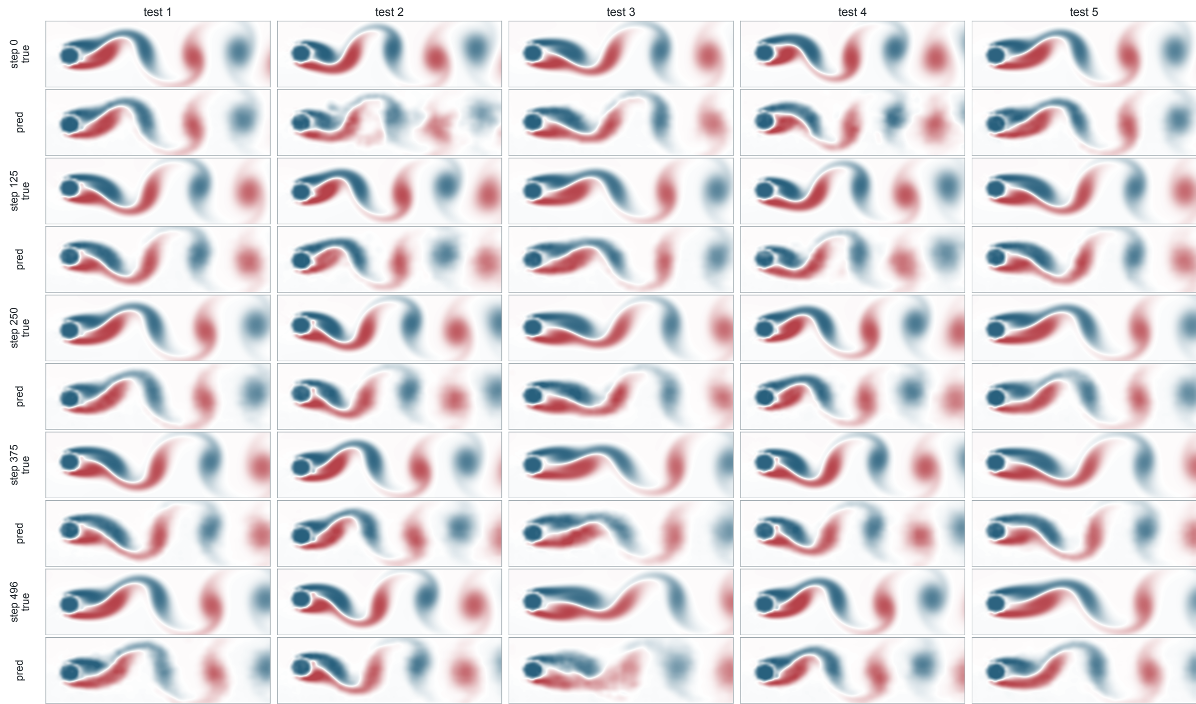
Forced cylinder wake test-set slices: true / pred (tests 1-5)
