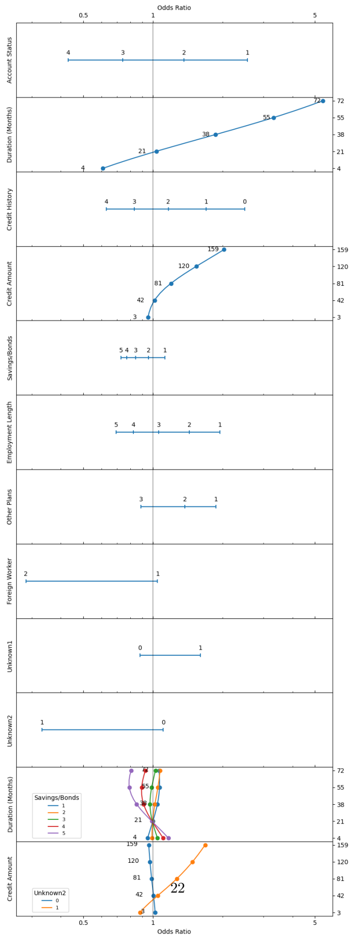
Nomogram of univariate and mixed bivariate partial responses (Lebesgue)
