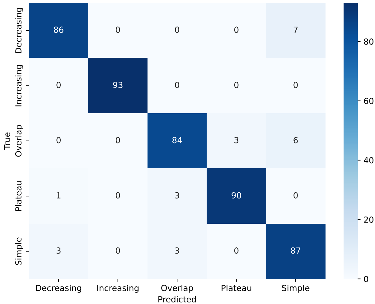
Confusion Matrix
