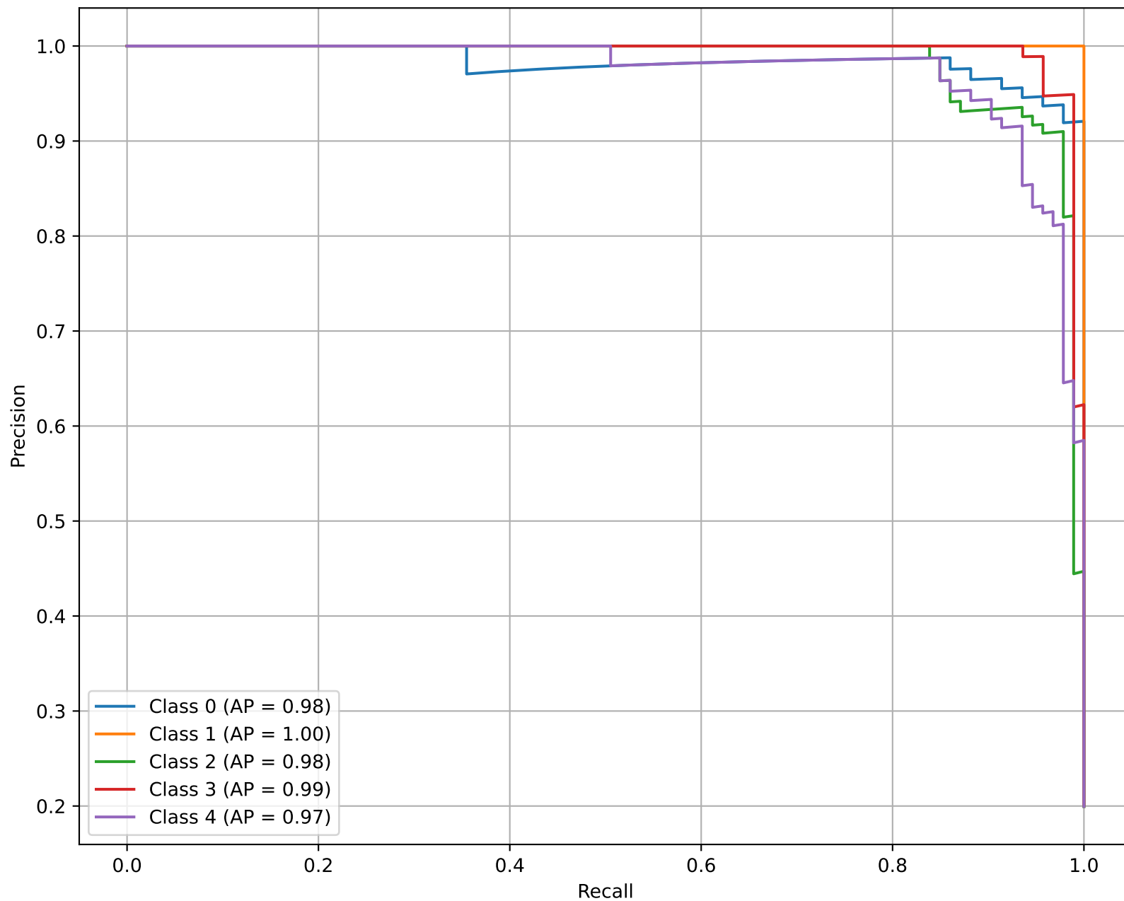
Precision-Recall Curve
