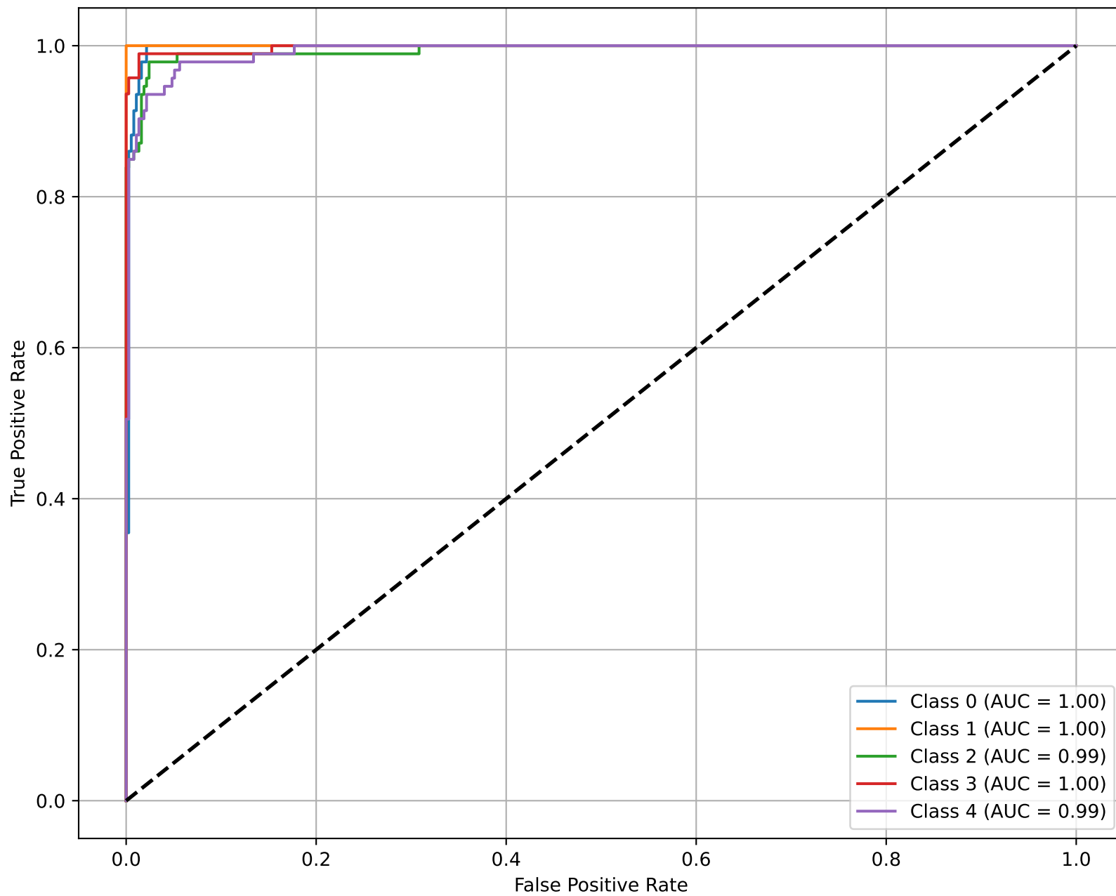
ROC Curve
