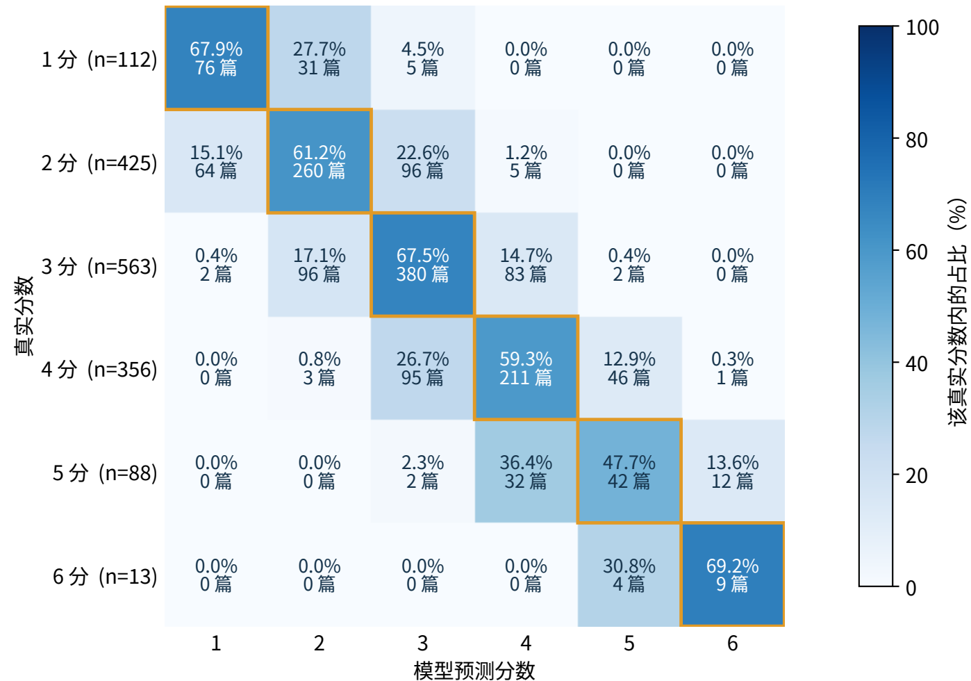
B1 · calibration 集拟合阈值 QWK = 0.82011
