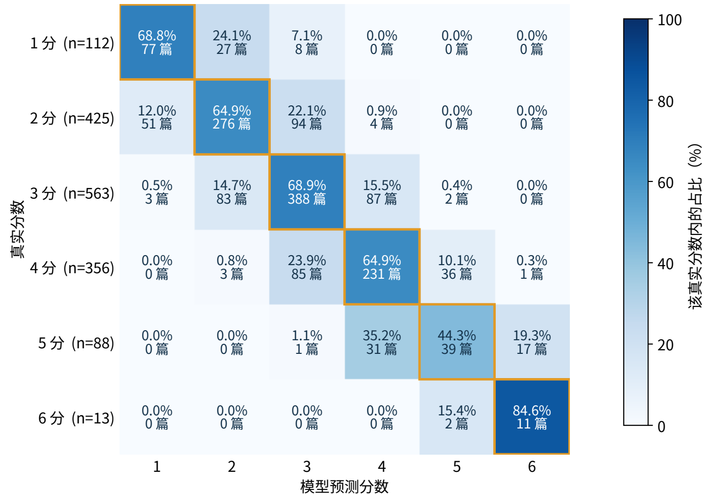
B1 · calibration 集拟合阈值 QWK = 0.83002
