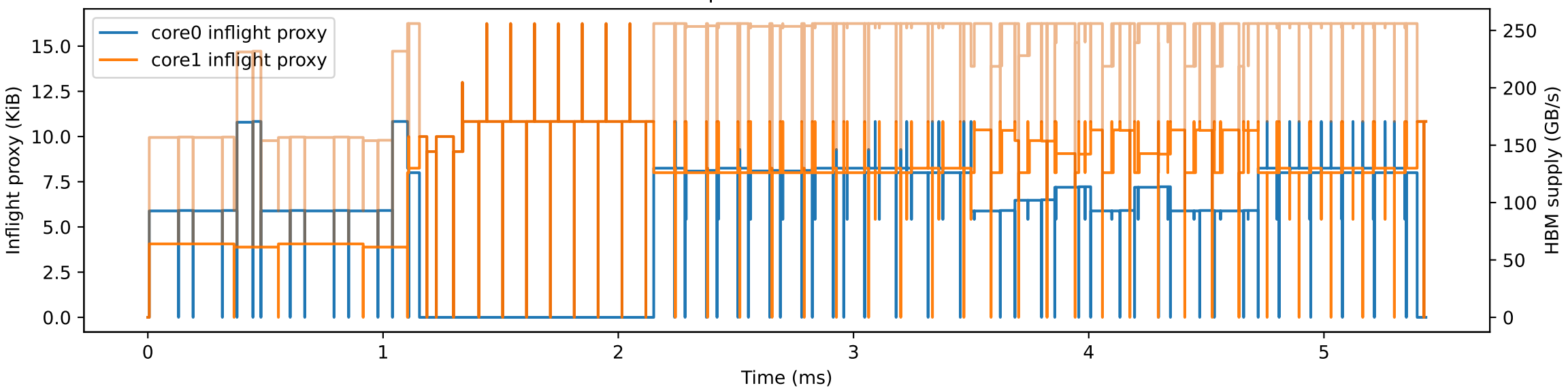
H2 — phase-fluid estimate
