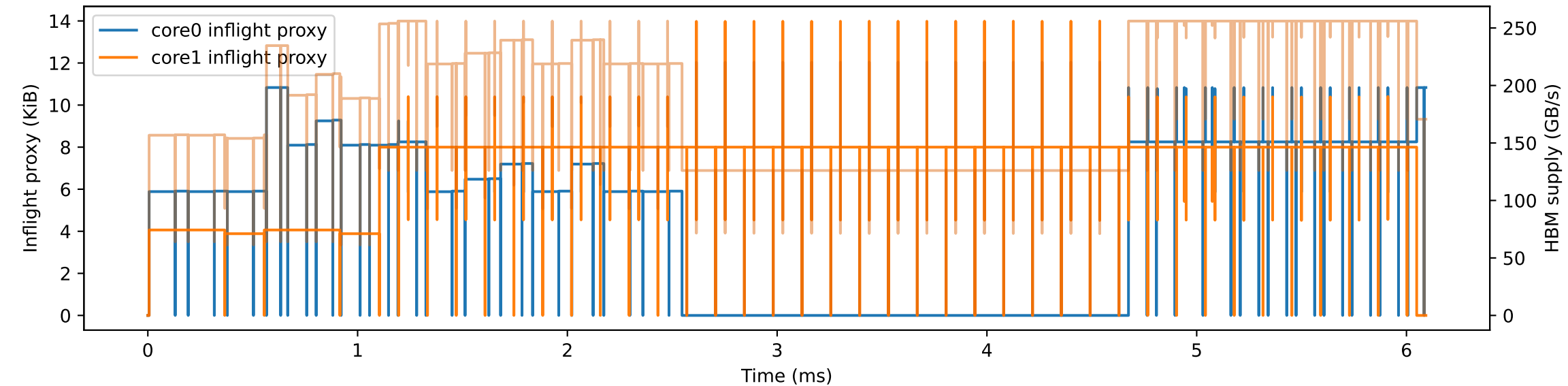
H3 — phase-fluid estimate
