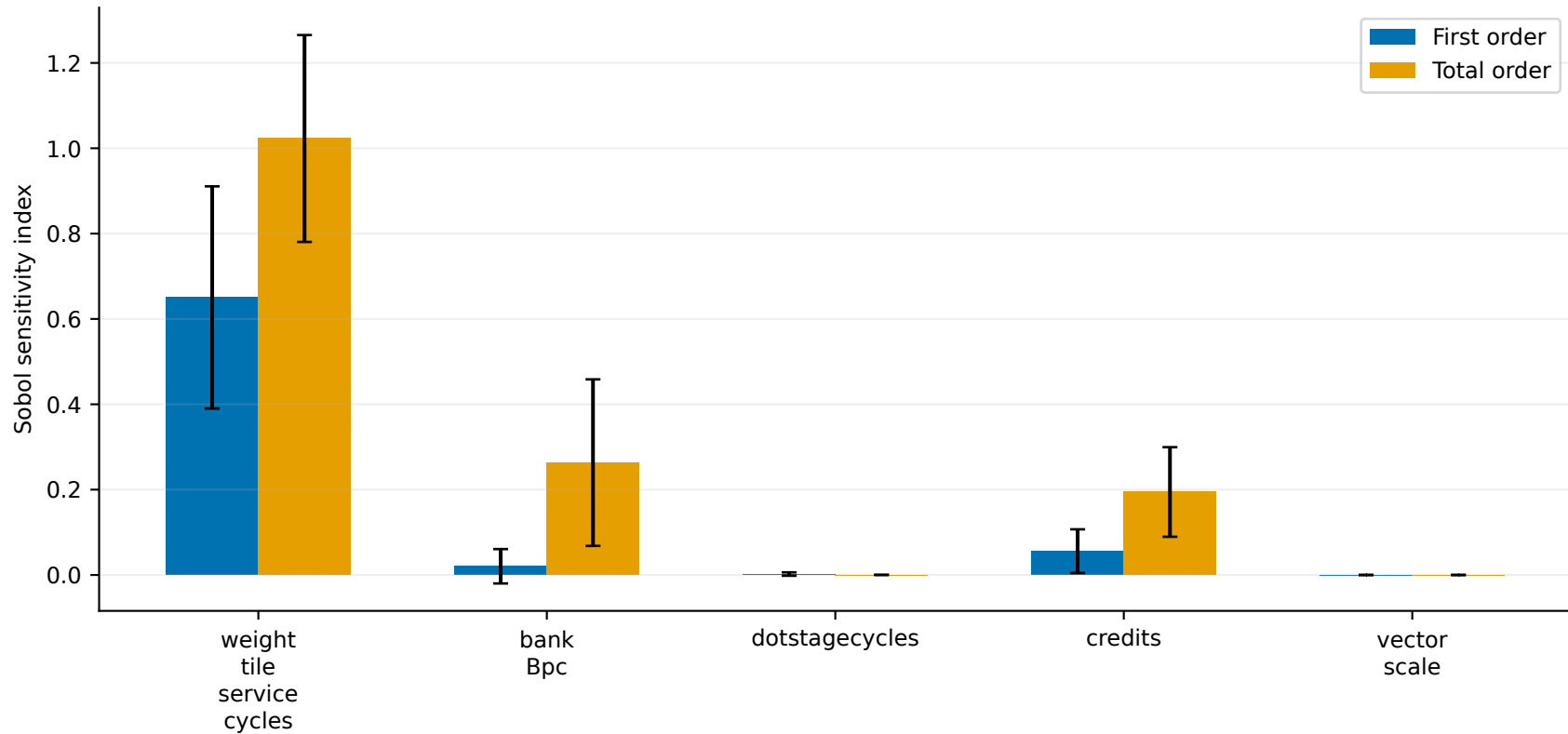
Hardware is reoptimized per parameter sample. Indices describe best-evaluated candidates from time-limited searches; they do not certify global-optimum sensitivity. Error bars are estimator confidence intervals.
