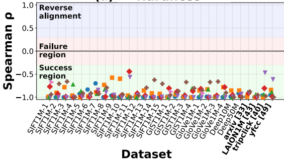
(a) \alpha -Hardness
