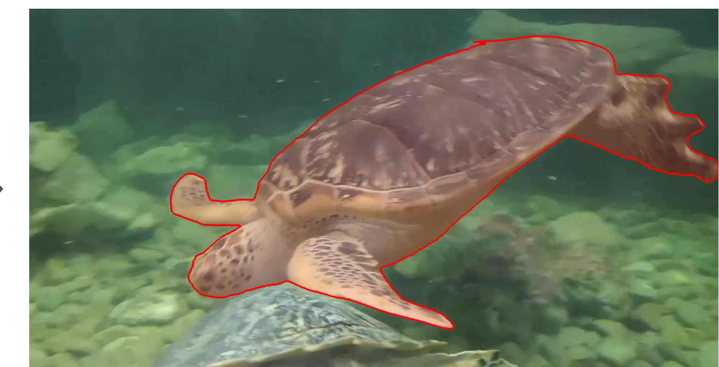
Predicted Mask
