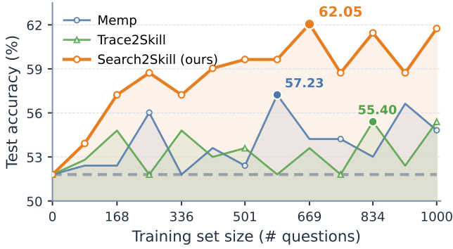
Figure 5: Skill acquisition efficiency on MMLU-Pro Philosophy. Search2Skill reaches higher accuracy with fewer training questions than baselines.
