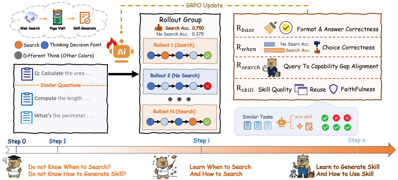
Figure 3: Overview of Search2Skill and its reward design. The agent searches when needed, distills retrieved evidence into reusable skills, and is trained with rewards for when to search , how to search , and how to generate skills .
