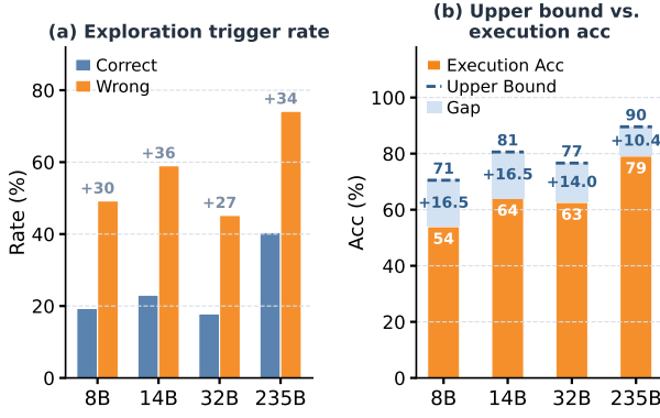
Figure 2: Knowledge-boundary awareness across Qwen3 model scales on SuperGPQA-Science: (a) Exploration trigger rate on eventually correct and incorrect questions; (b) Execution accuracy and upper bound of self-evolving.
