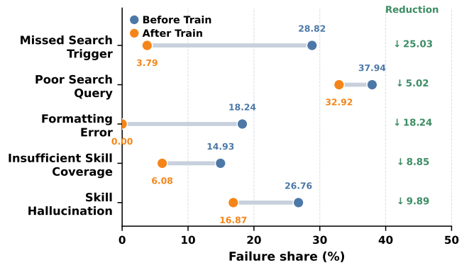
Figure 4: Failure patterns before and after RL training. RL reduces the failure share of all five patterns.
