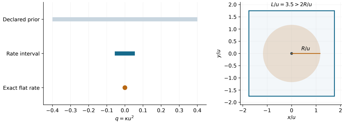
Figure 2: Left: synthetic curvature-prior interval, refinement by a rate interval, and the exact flat rate. Right: a two-dimensional cross-section illustrating the injective ball inside a cubic torus domain; the full construction is three-dimensional. No cosmological data fit is shown.
