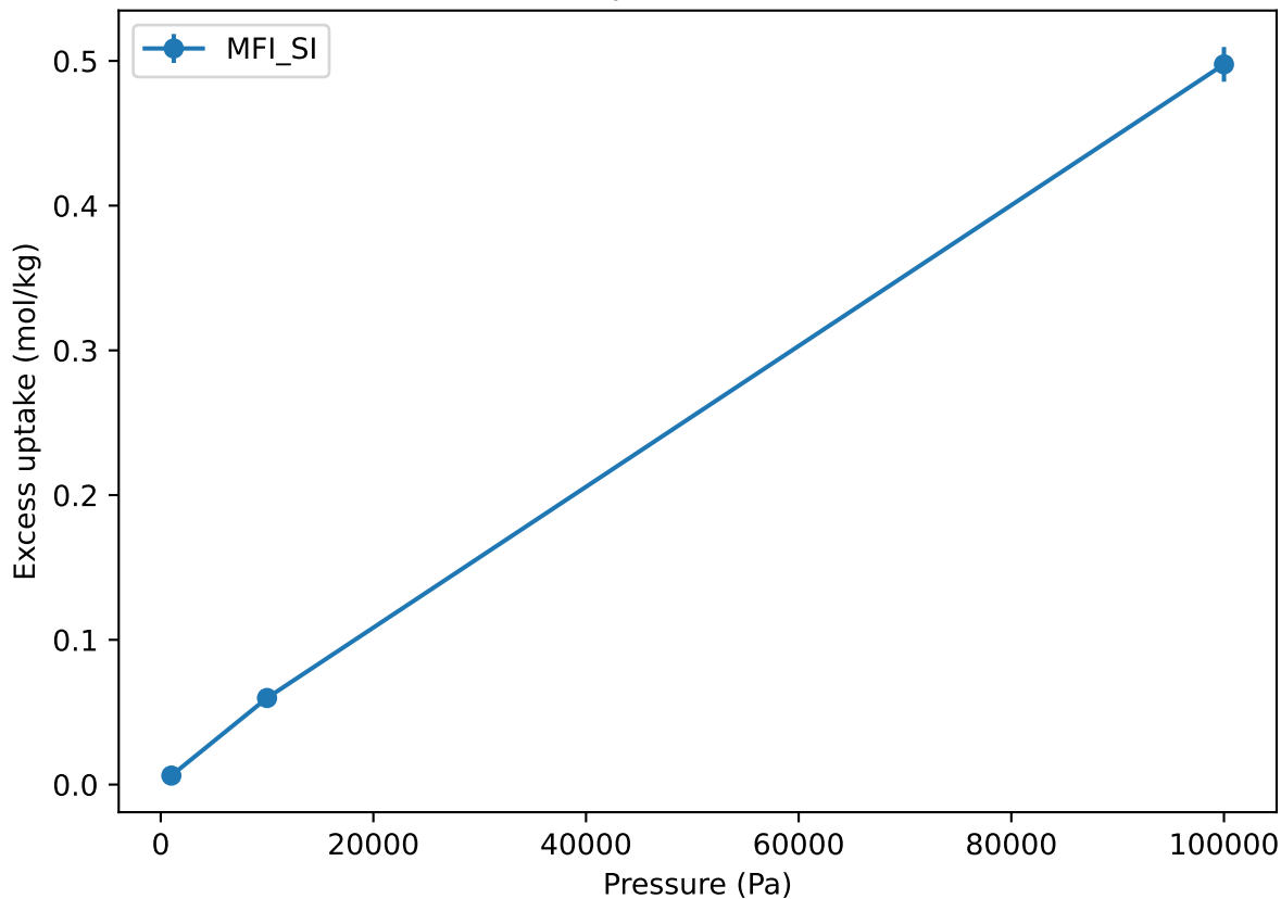
Adsorption Isotherms
