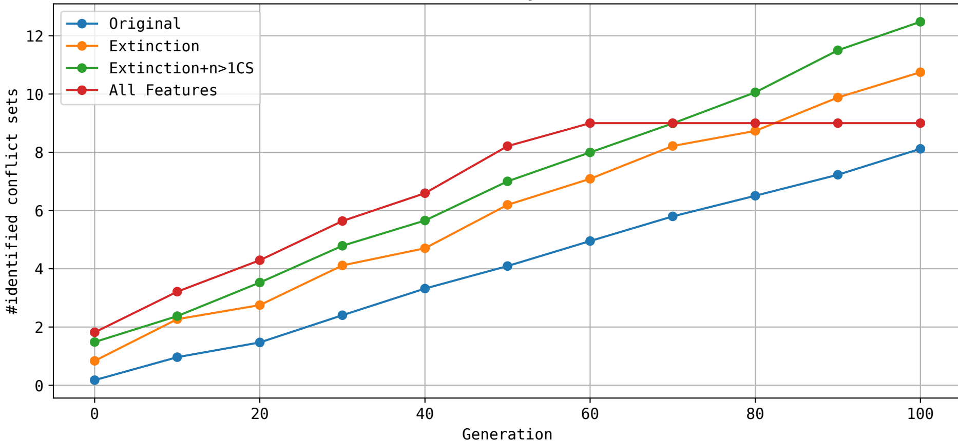
Conflict Set Discovery Over Generations
