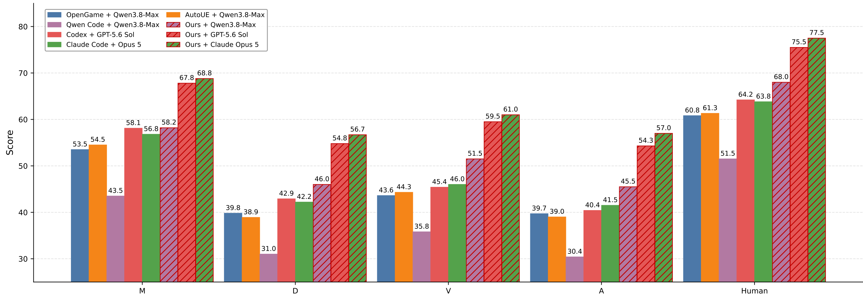
Playable-Game Quality on GameCode4D
