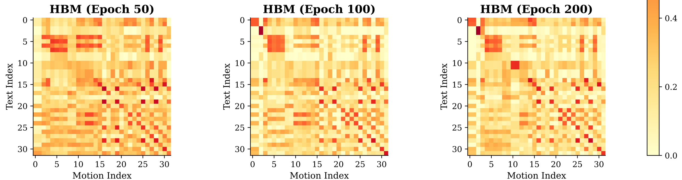
(b) Heatmap of HBM training process
