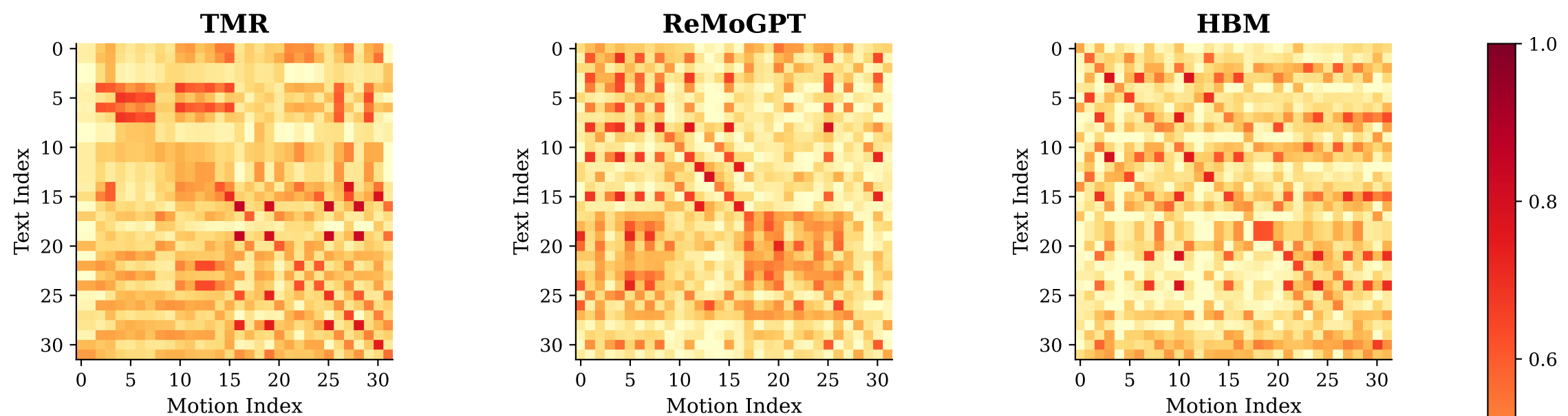
(a) Heatmap between different retrieval models
