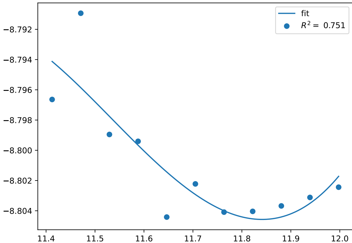
Cr_pv20Co_pv4.C36-BAAAA.FM
