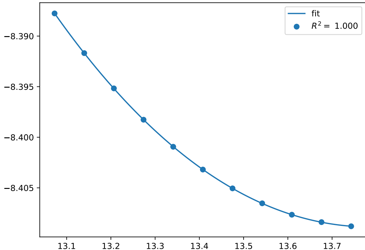
Cr_pv4Co_pv14W_sv6.C36-ABBBC.FM
