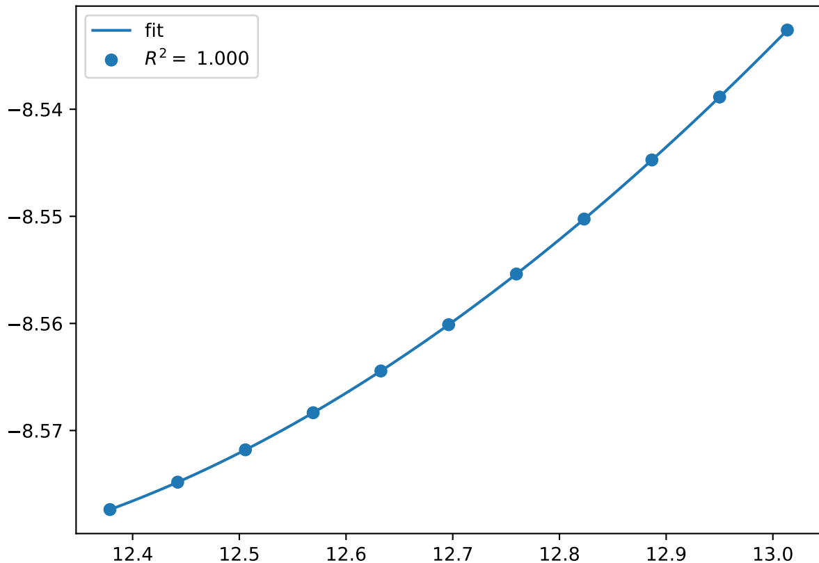
Cr_pv2Co_pv8W_sv3.mu-CBBCA.FM
