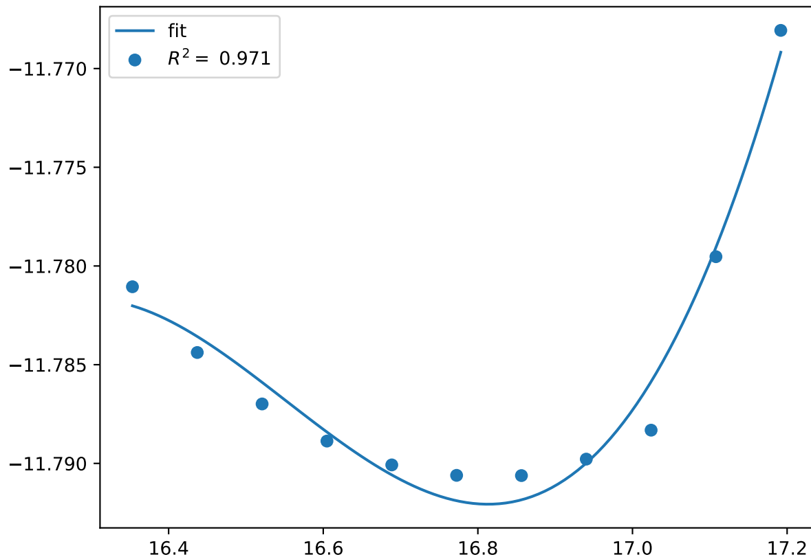
Cr_pv4W_sv20.C36-BABBB.FM
