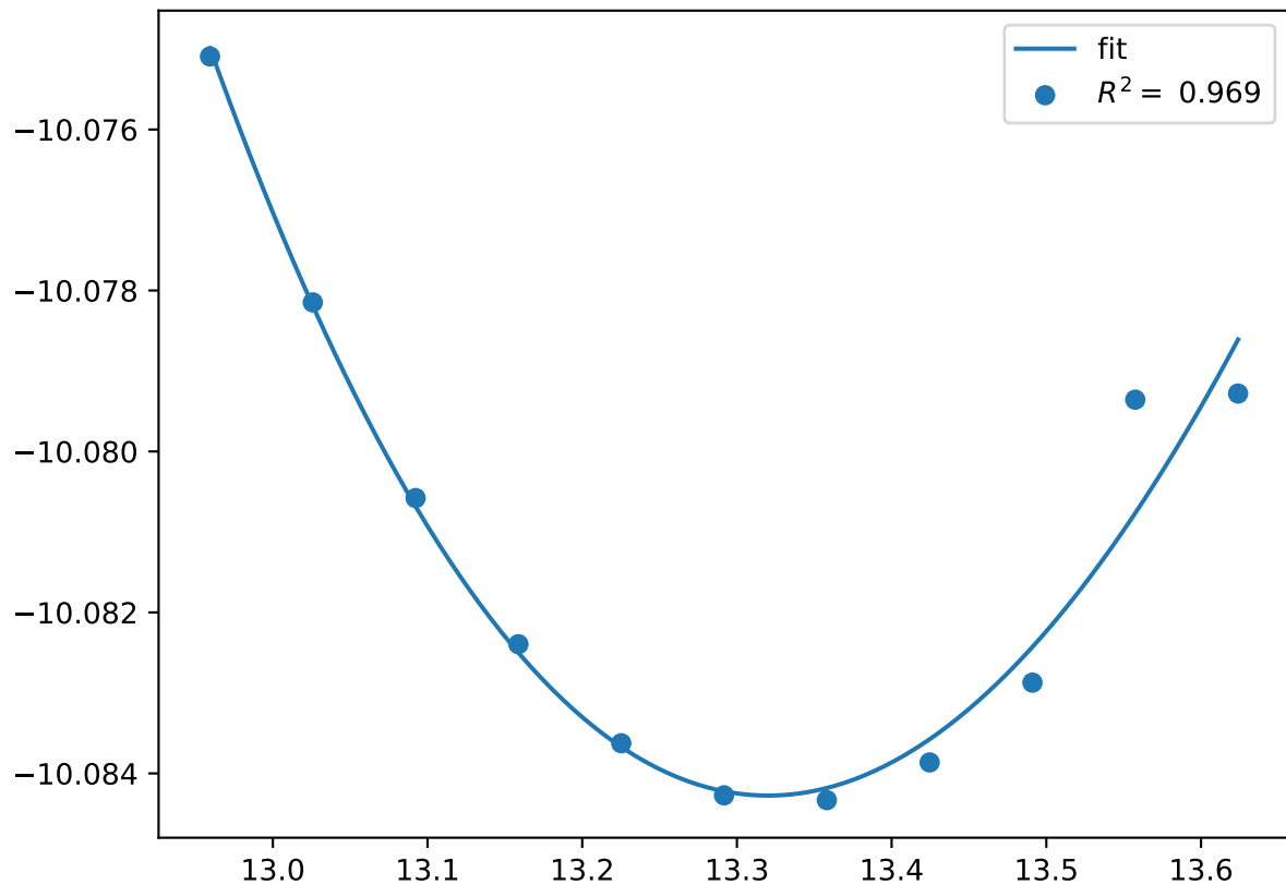
Cr_pv10Co_pv8W_sv12.sigma-ACBCA.FM
