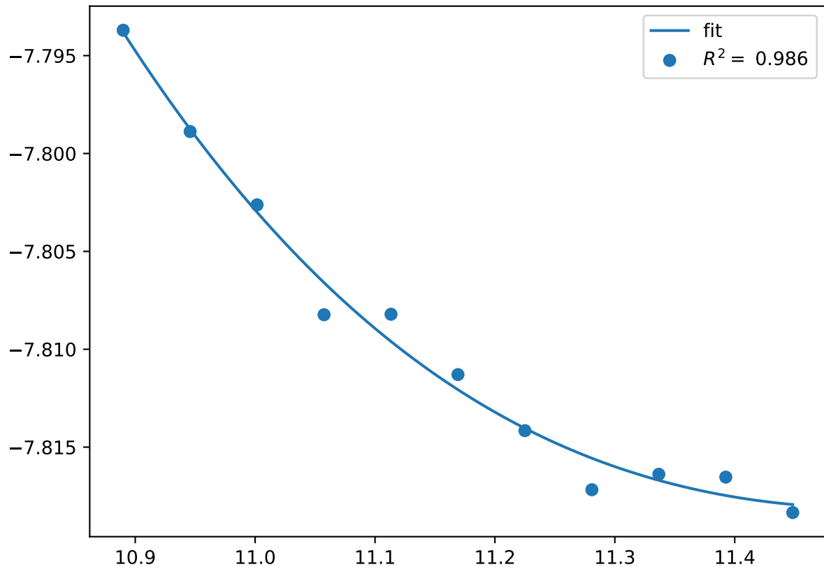
Cr_pv10Co_pv14.C36-BABBA.FM
