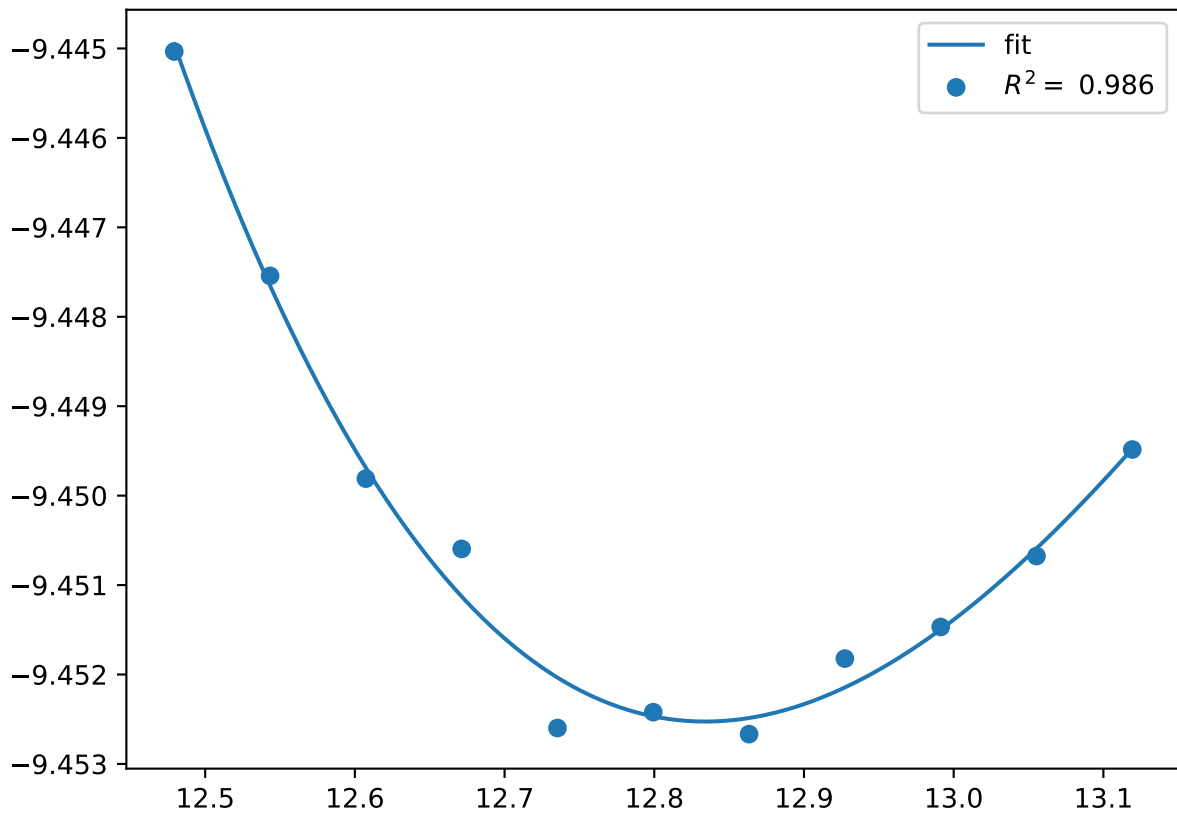
Cr_pv8Co_pv12W_sv10.sigma-CBCAB.FM
