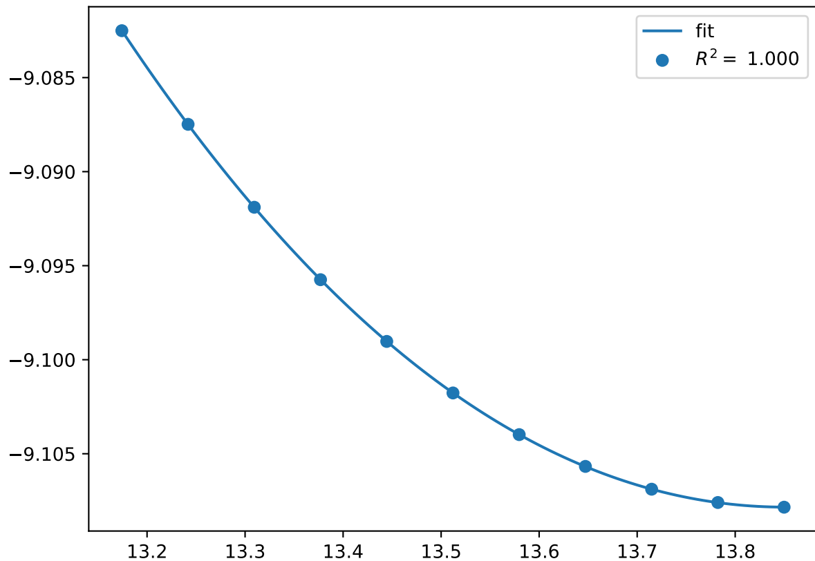
Co_pv14W_sv10.C36-BAABA.FM
