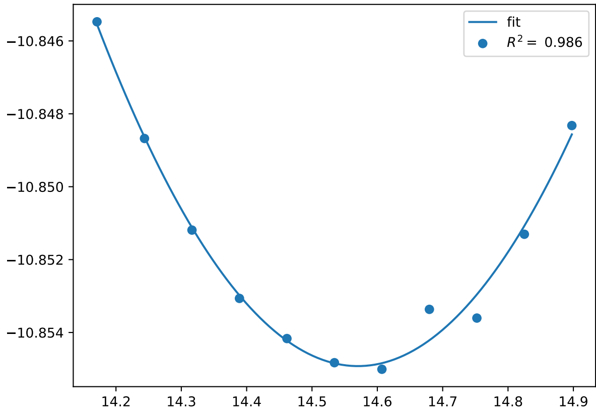
Cr_pv12Co_pv2W_sv16.sigma-BAACC.FM
