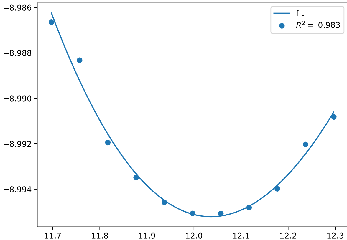
Co_pv16W_sv8.C36-BBAAA.FM
