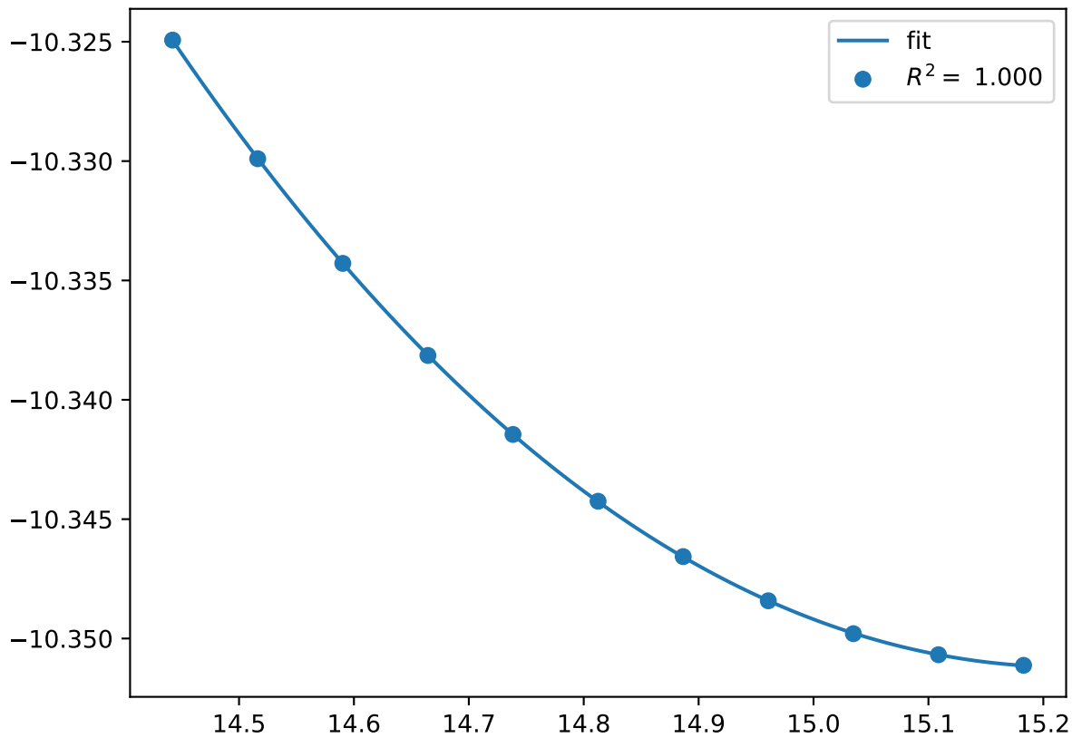
Cr_pv14W_sv10.C36-AABAB.FM
