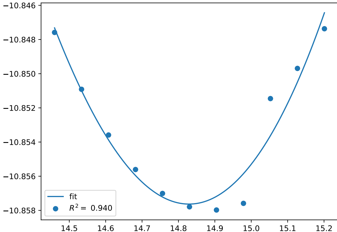
Cr_pv8Co_pv4W_sv18.sigma-CBCCA.FM
