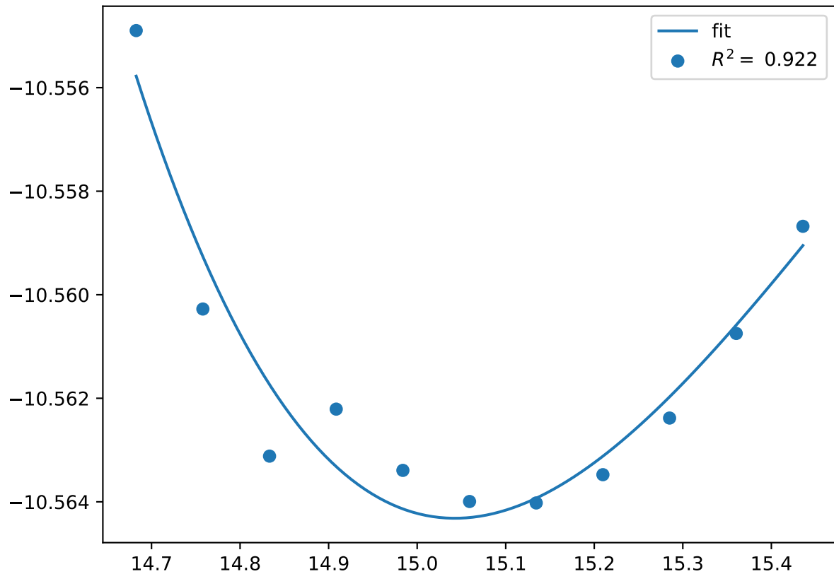
Cr_pv6Co_pv4W_sv14.C36-BCCAC.FM
