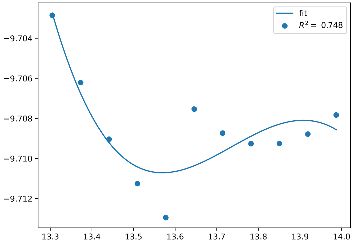
Cr_pv4Co_pv12W_sv13.chi-CABC.FM
