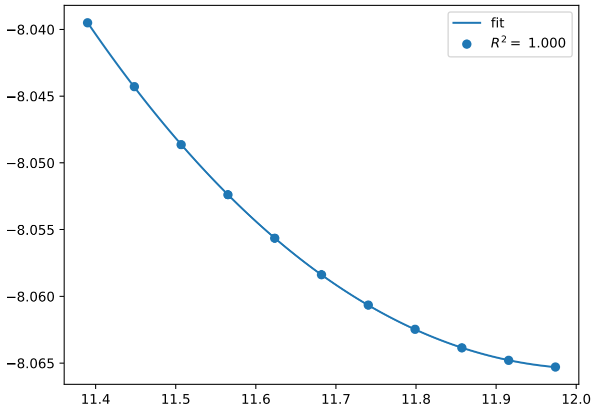
Co_pv24W_sv6.sigma-BBAAA.FM
