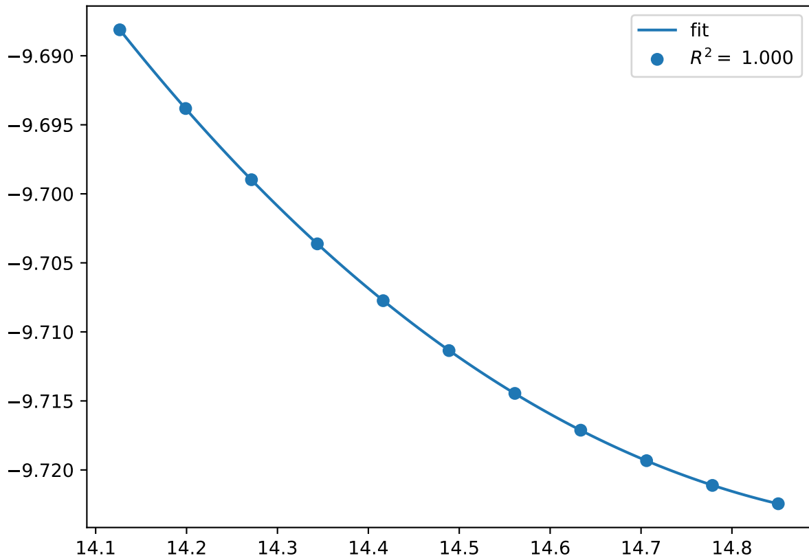
Cr_pv8Co_pv6W_sv10.C36-AACBC.FM
