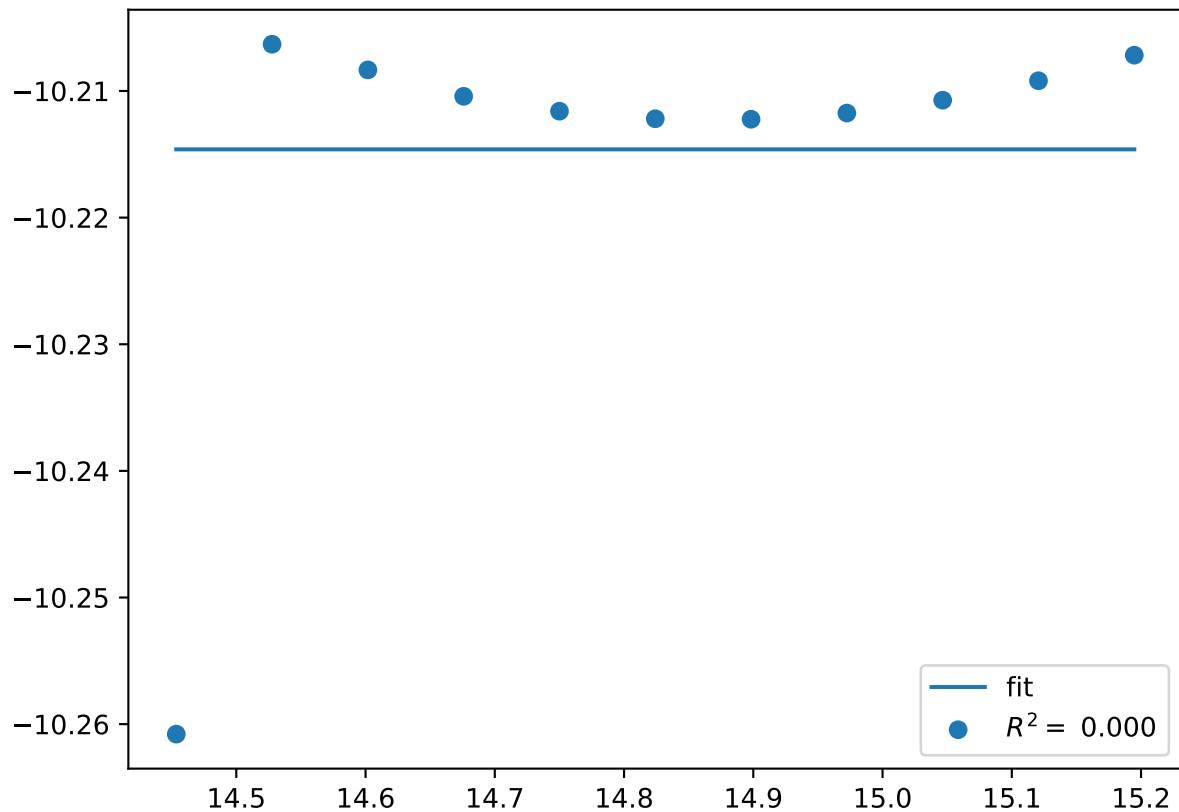
Cr_pv4Co_pv2W_sv6.C14-BCA.FM
