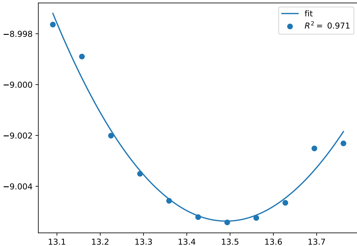
Cr_pv10Co_pv8W_sv6.C36-BABAC.FM
