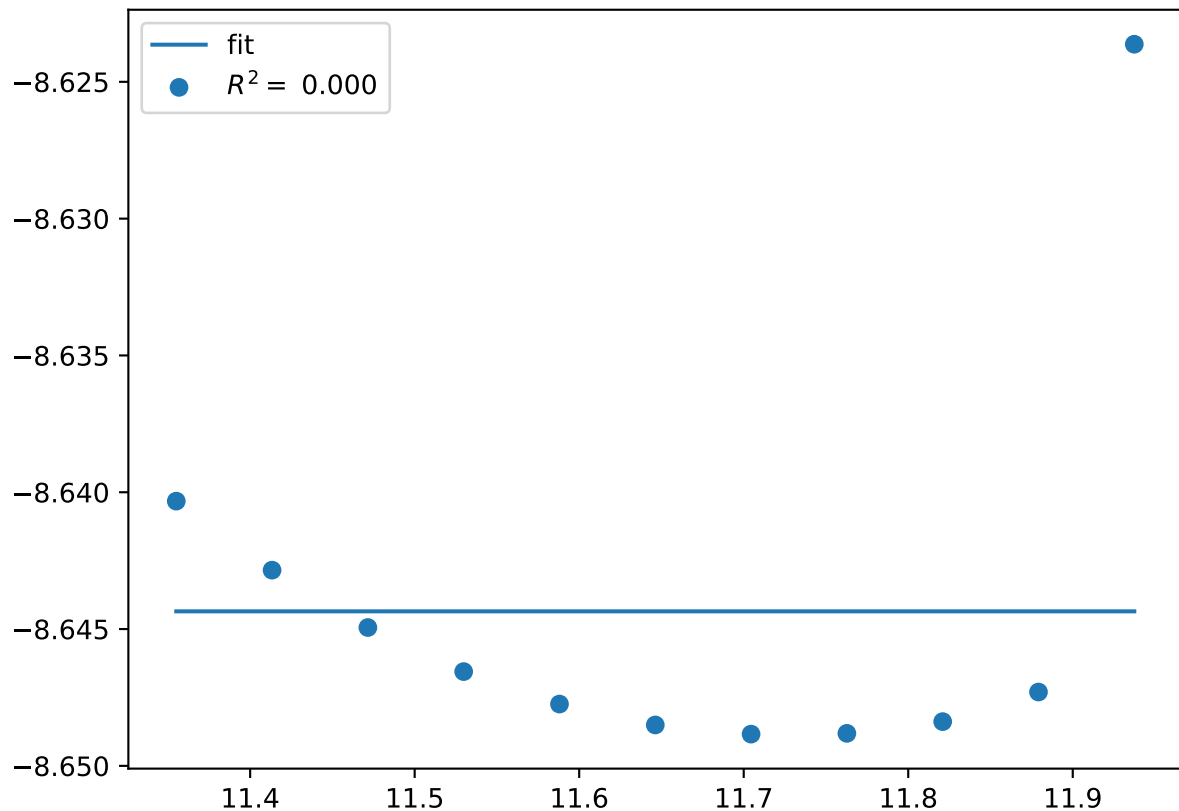
Cr_pv18Co_pv6.C36-AAABA.FM
