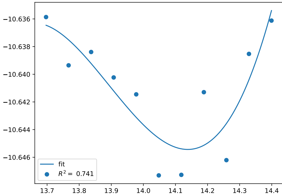
Cr_pv8Co_pv6W_sv16.sigma-BBCAC.FM
