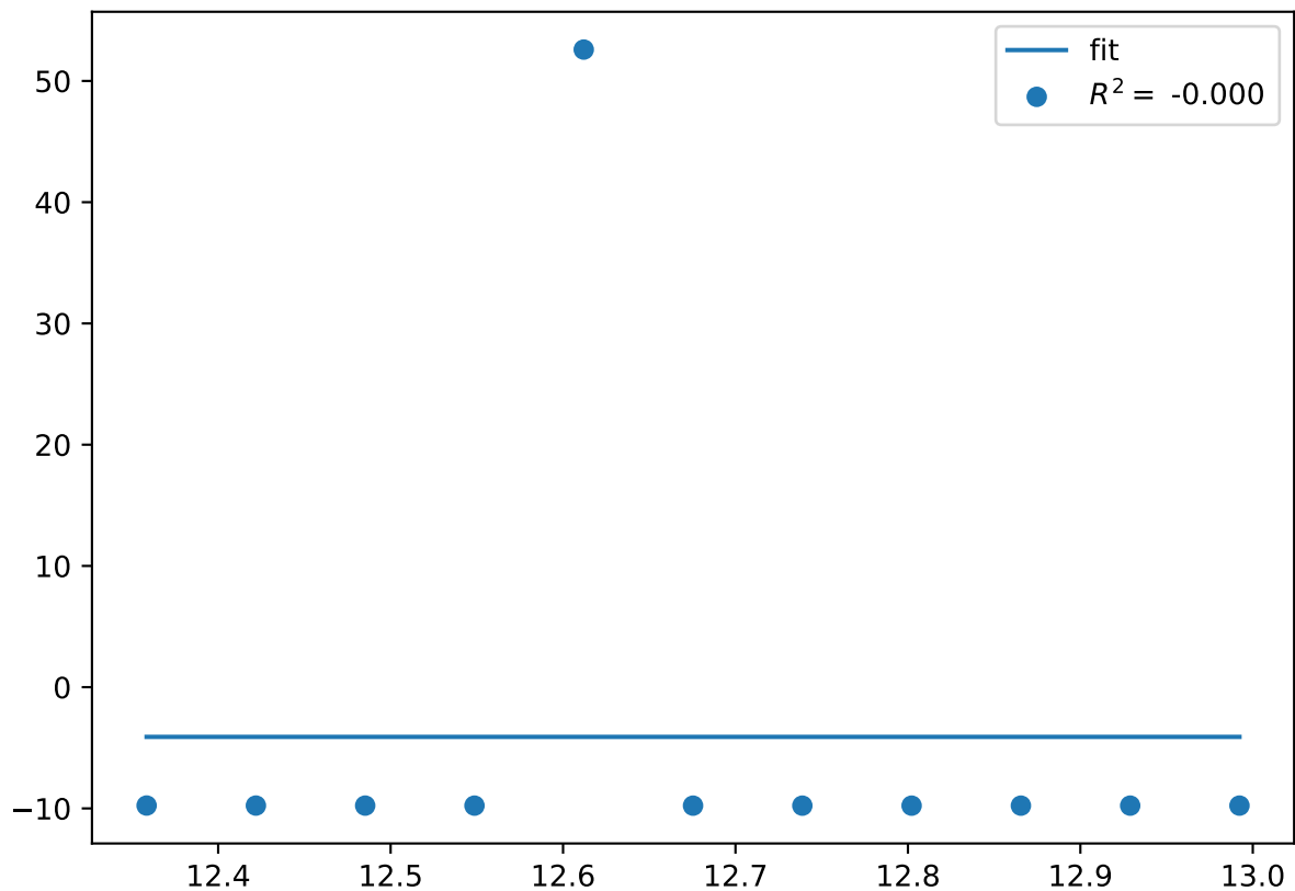
Cr_pv11W_sv2.mu-AAAAB.NM
