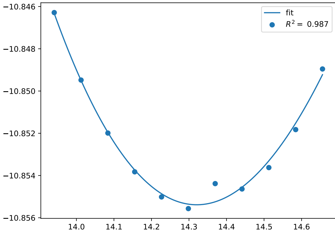
Cr_pv6Co_pv4W_sv14.C36-CCBAC.FM
