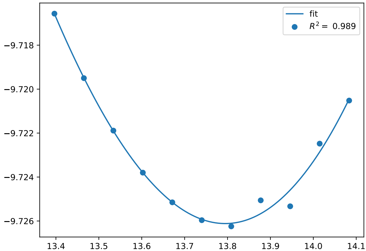
Cr_pv6Co_pv8W_sv10.C36-CBBCA.FM
