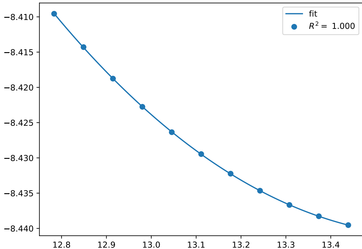
Cr_pv4Co_pv14W_sv6.C36-ABBCB.FM
