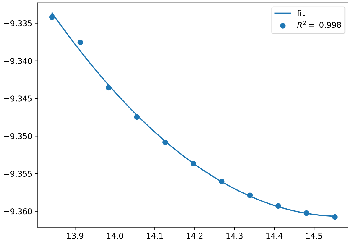
Cr_pv4Co_pv10W_sv10.C36-BACCB.FM
