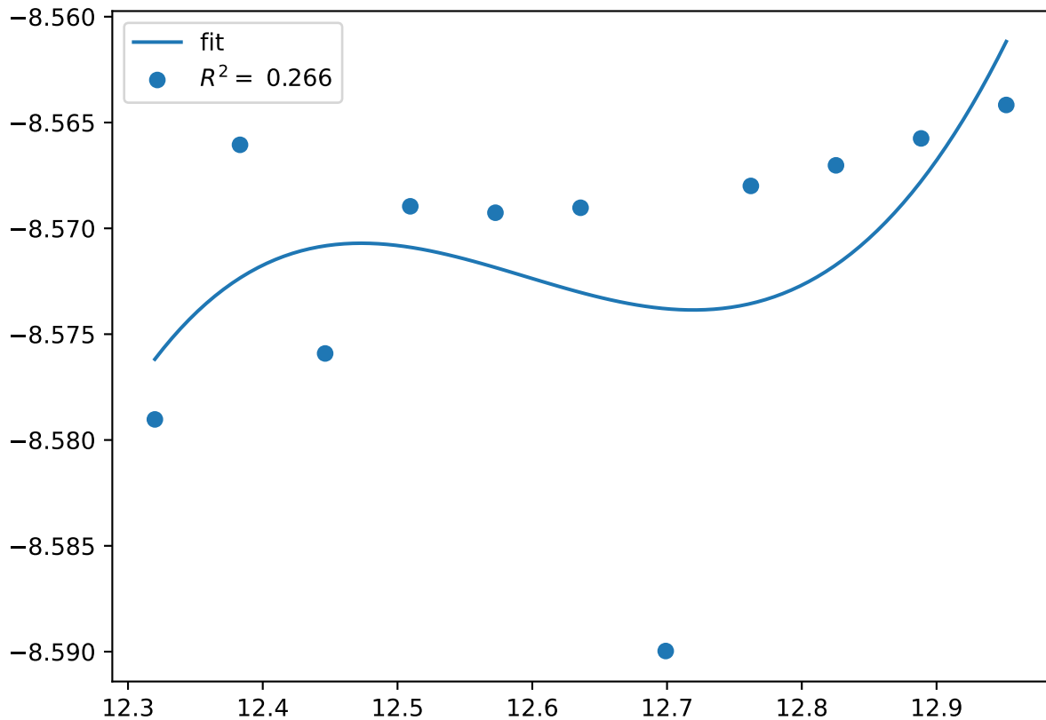
Cr_pv8Co_pv12W_sv4.C36-AACBB.FM
