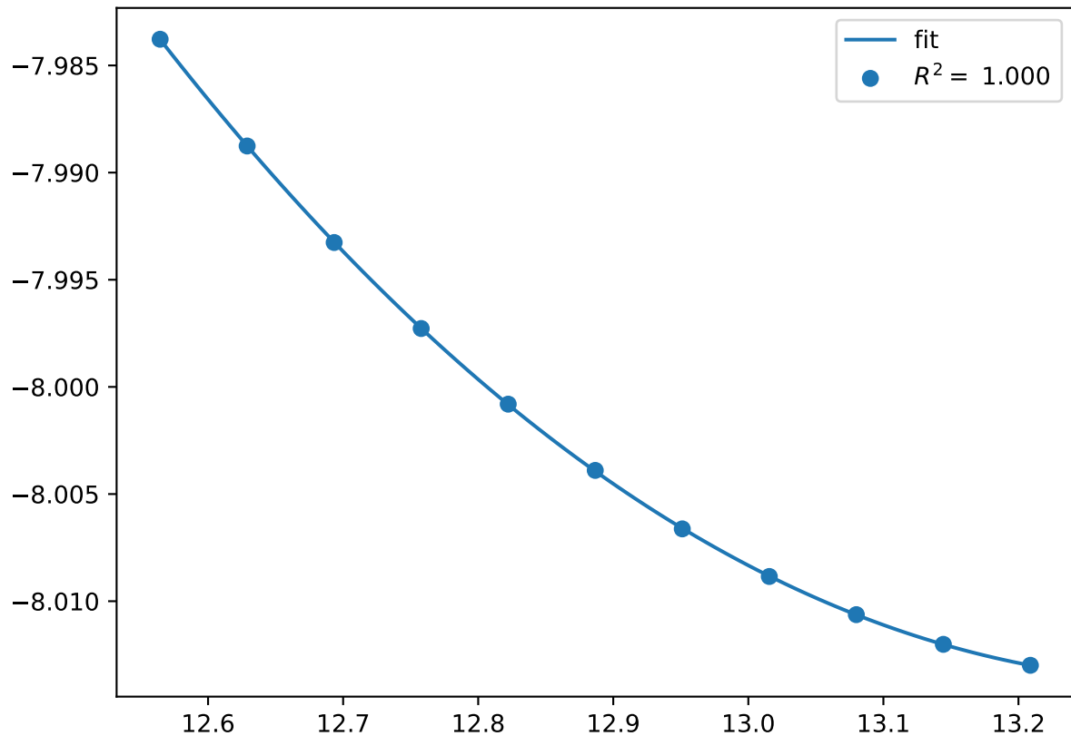
Co_pv18W_sv6.C36-AAABA.FM
