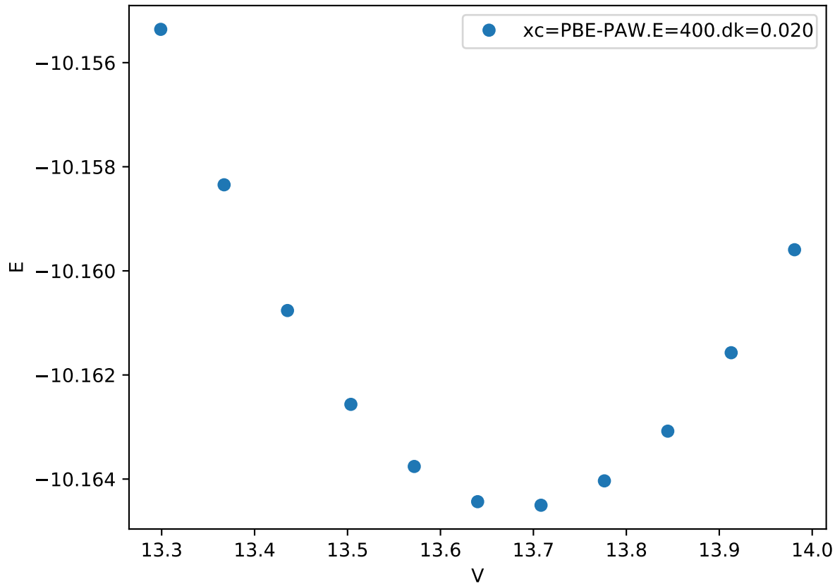
Cr_pv-Co_pv-W_sv/Cr_pv-Co_pv-W_sv_chi-BBCA_
