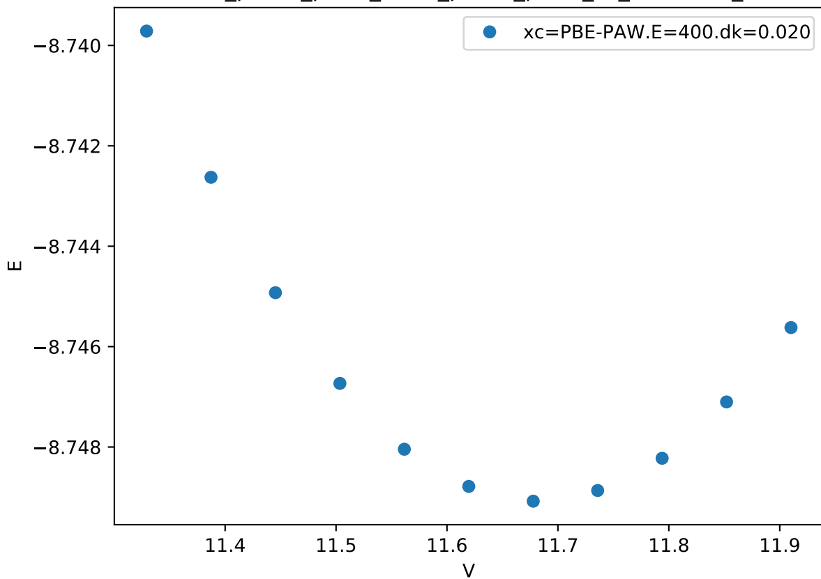
Cr_pv-Co_pv-W_sv/Cr_pv-Co_pv-W_sv_chi-BCAB_
