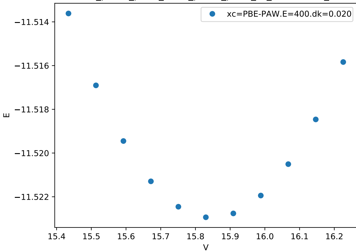
Cr_pv-Co_pv-W_sv/Cr_pv-Co_pv-W_sv_mu-BCACC_
