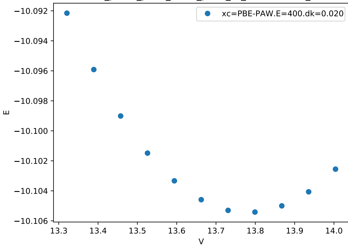
Cr_pv-Co_pv-W_sv/Co_pv-W_sv_chi-ABBA.FM_
