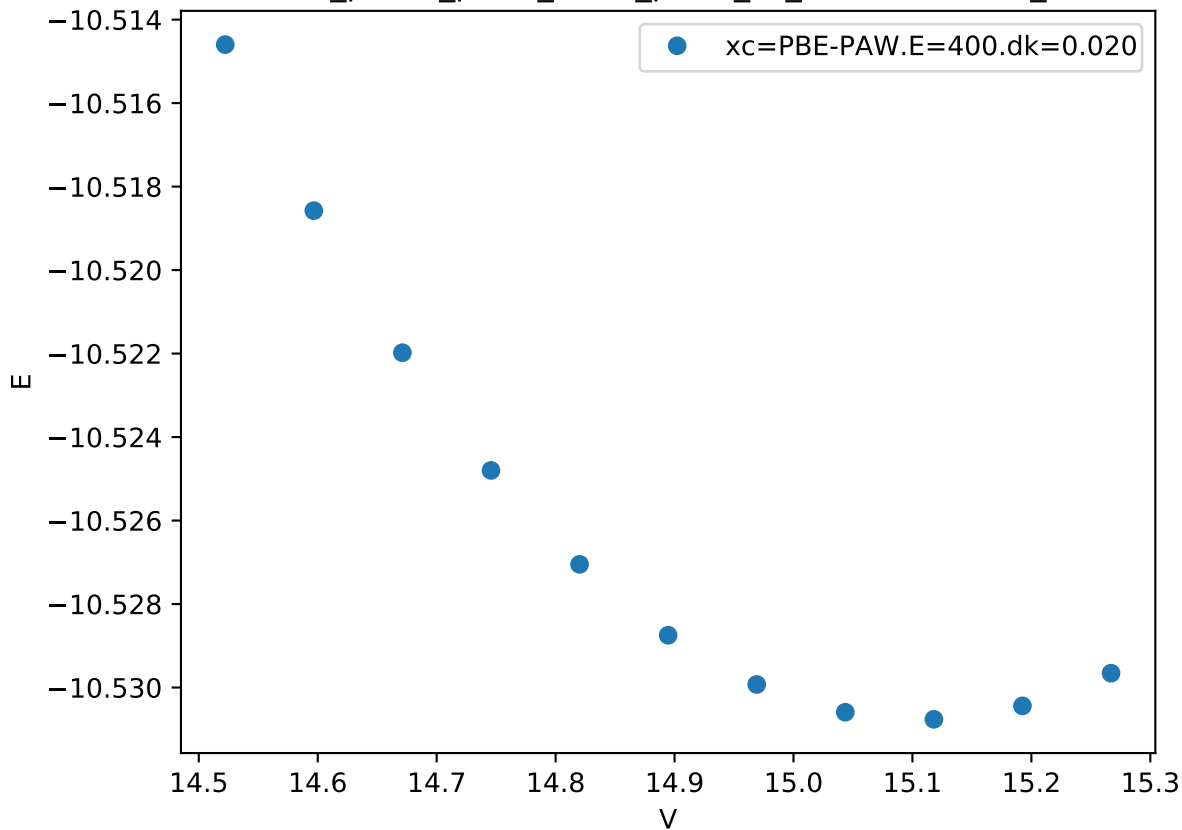
Cr_pv-Co_pv-W_sv/Cr_pv-W_sv_mu-ABAAA.FM_
