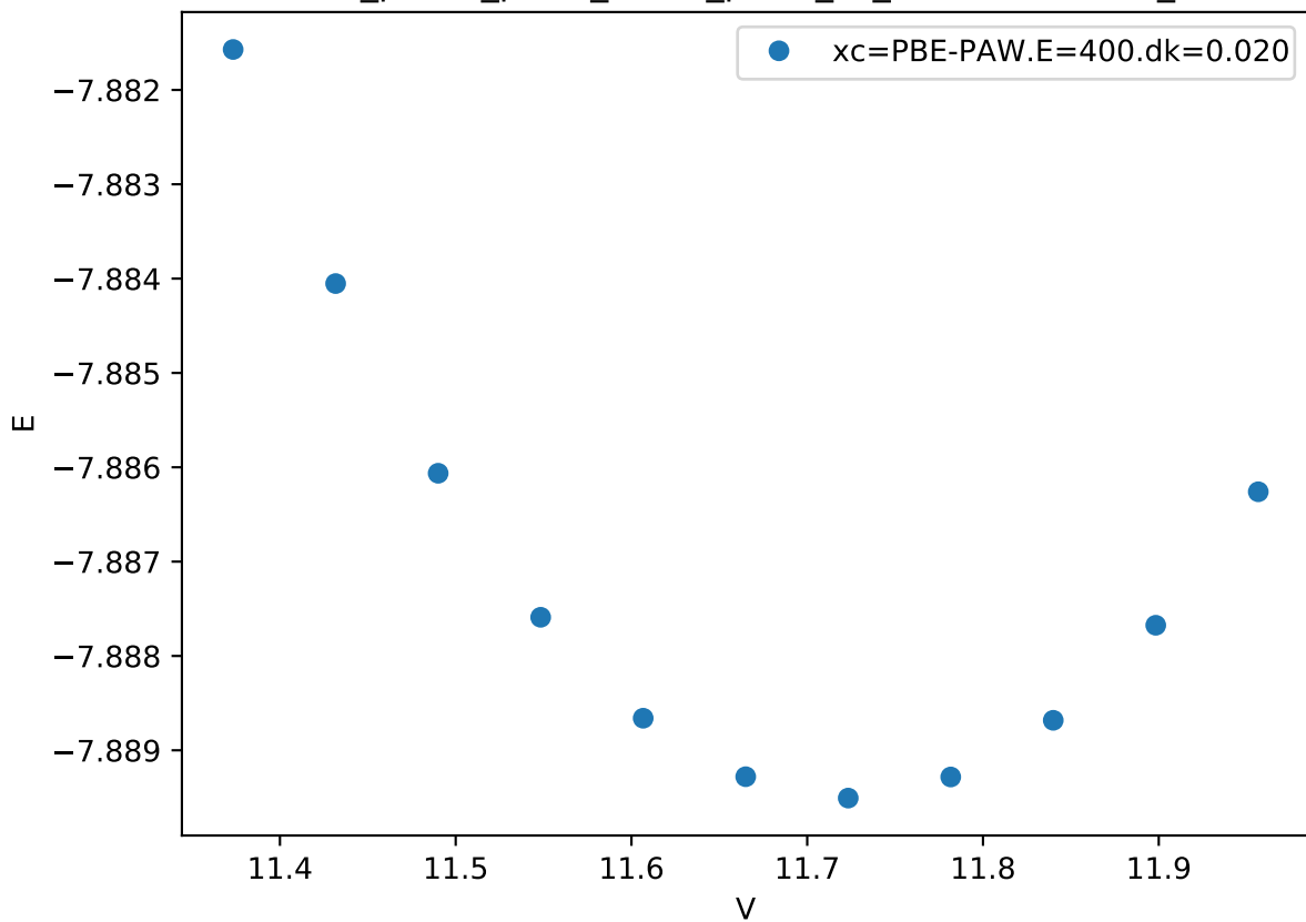
Cr_pv-Co_pv-W_sv/Co_pv-W_sv_C36-BAAAA.FM_
