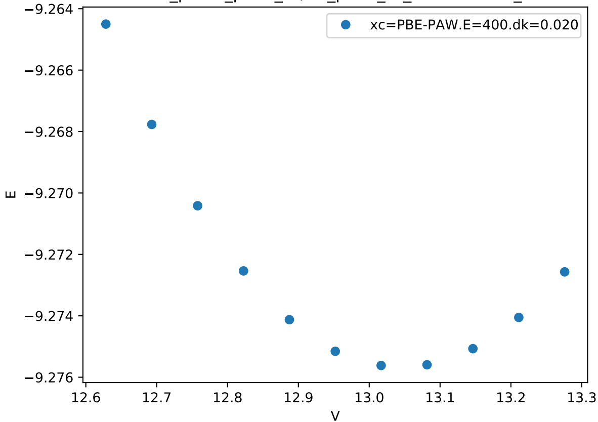
Cr_pv-Co_pv-W_sv/Co_pv-W_sv_chi-AABA.FM_
