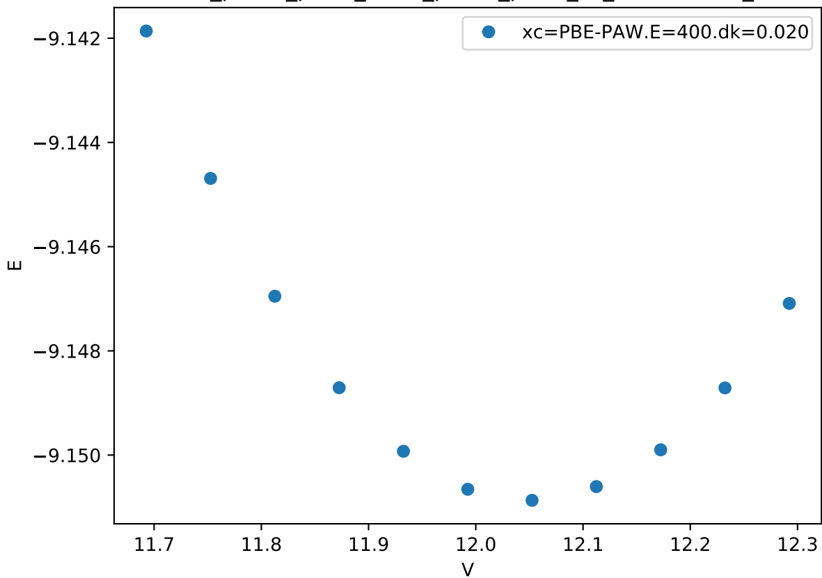
Cr_pv-Co_pv-W_sv/Cr_pv-Co_pv-W_sv_C36-CBBAA_
