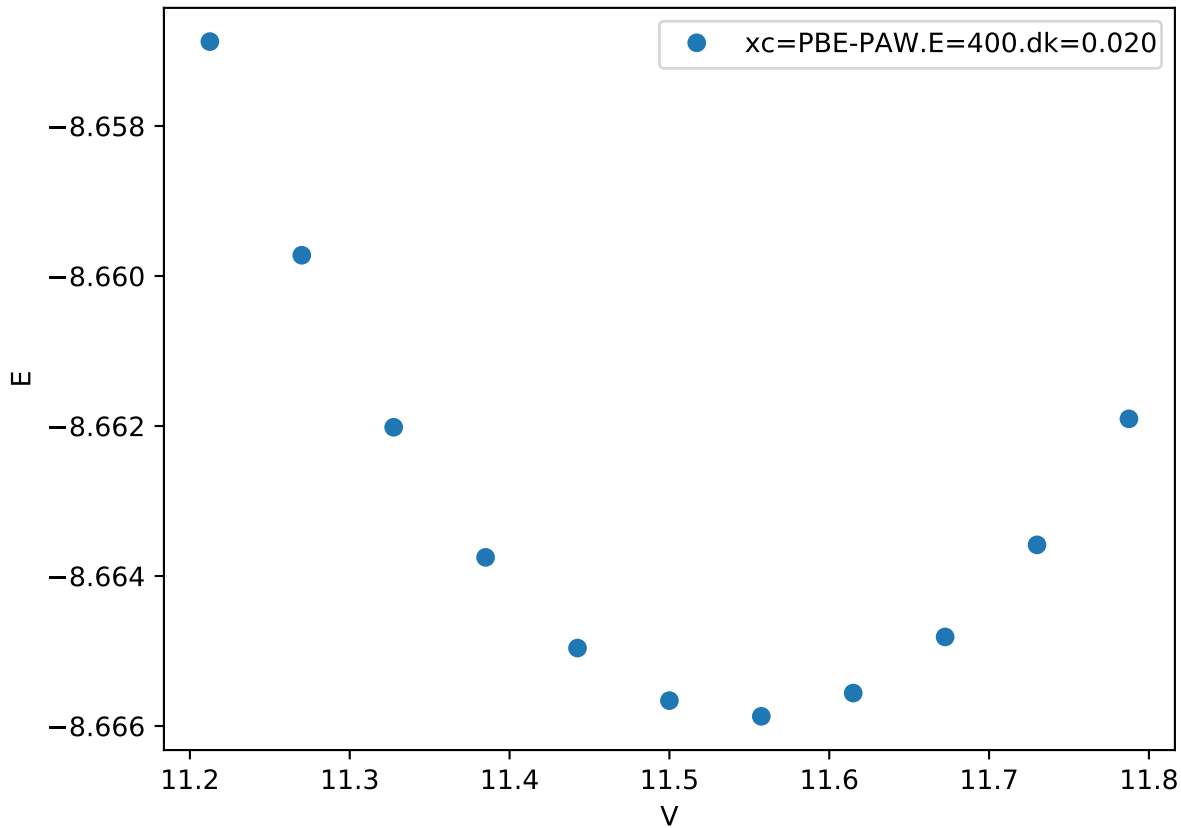
Cr_pv-Co_pv-W_sv/Cr_pv-Co_pv-W_sv_mu-BBACA.FM_
