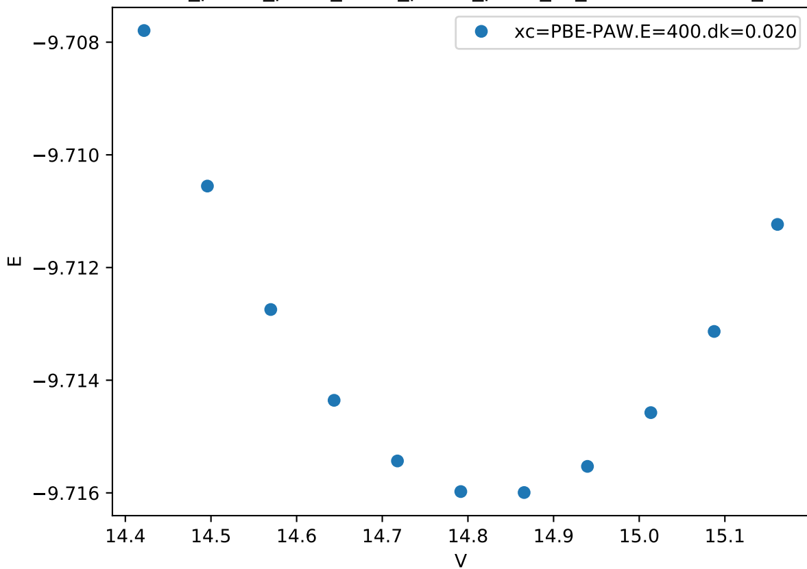
Cr_pv-Co_pv-W_sv/Cr_pv-Co_pv-W_sv_C36-BBACC.FM_
