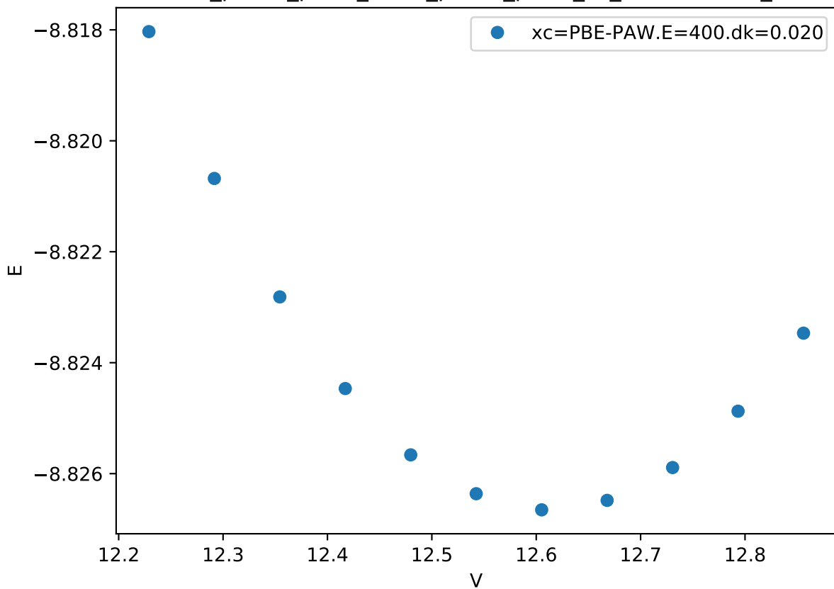
Cr_pv-Co_pv-W_sv/Cr_pv-Co_pv-W_sv_C14-CAB.FM_
