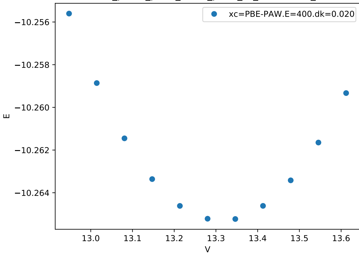
Cr_pv-Co_pv-W_sv/Co_pv-W_sv_mu-BABBB_
