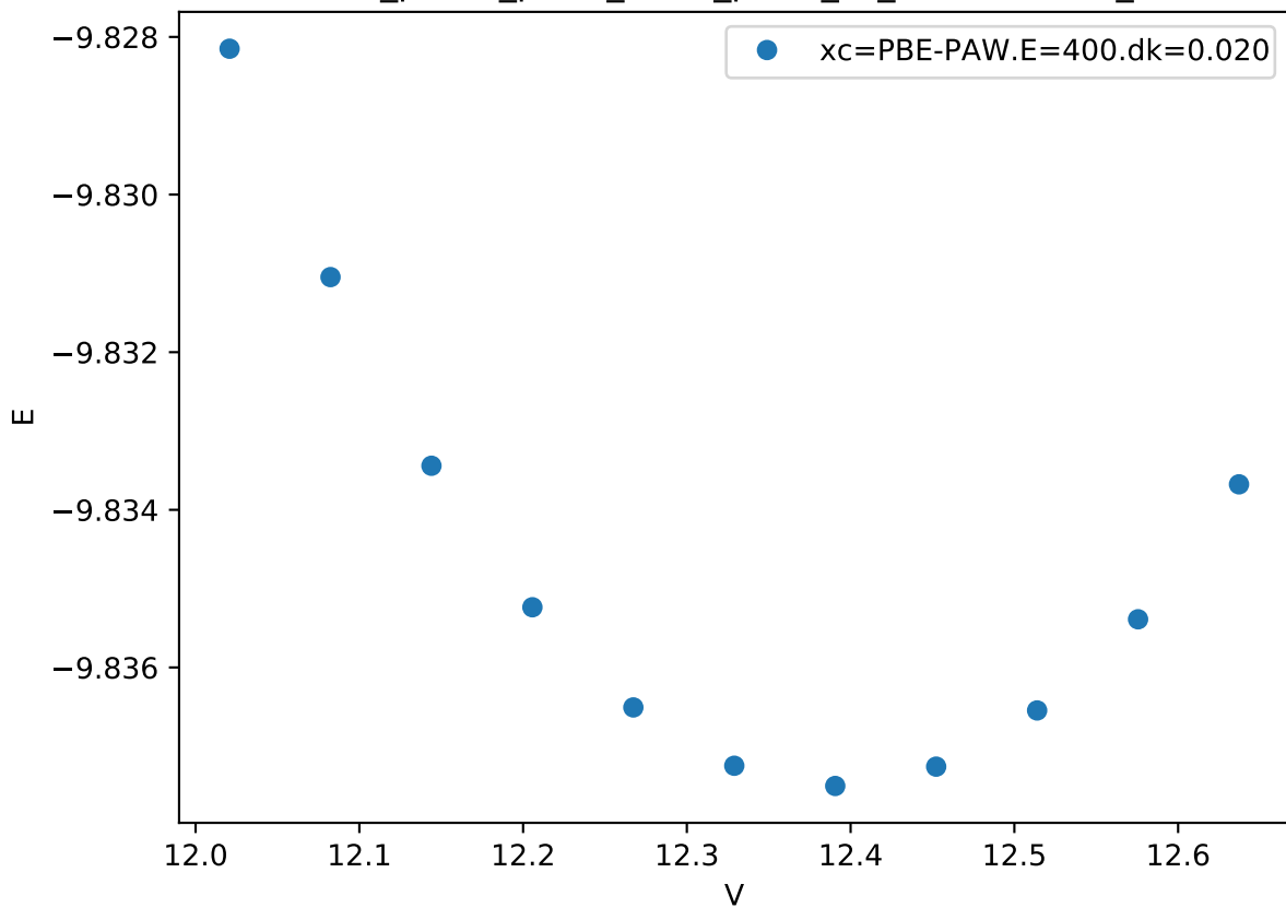
Cr_pv-Co_pv-W_sv/Cr_pv-W_sv_chi-ABAA.FM_
