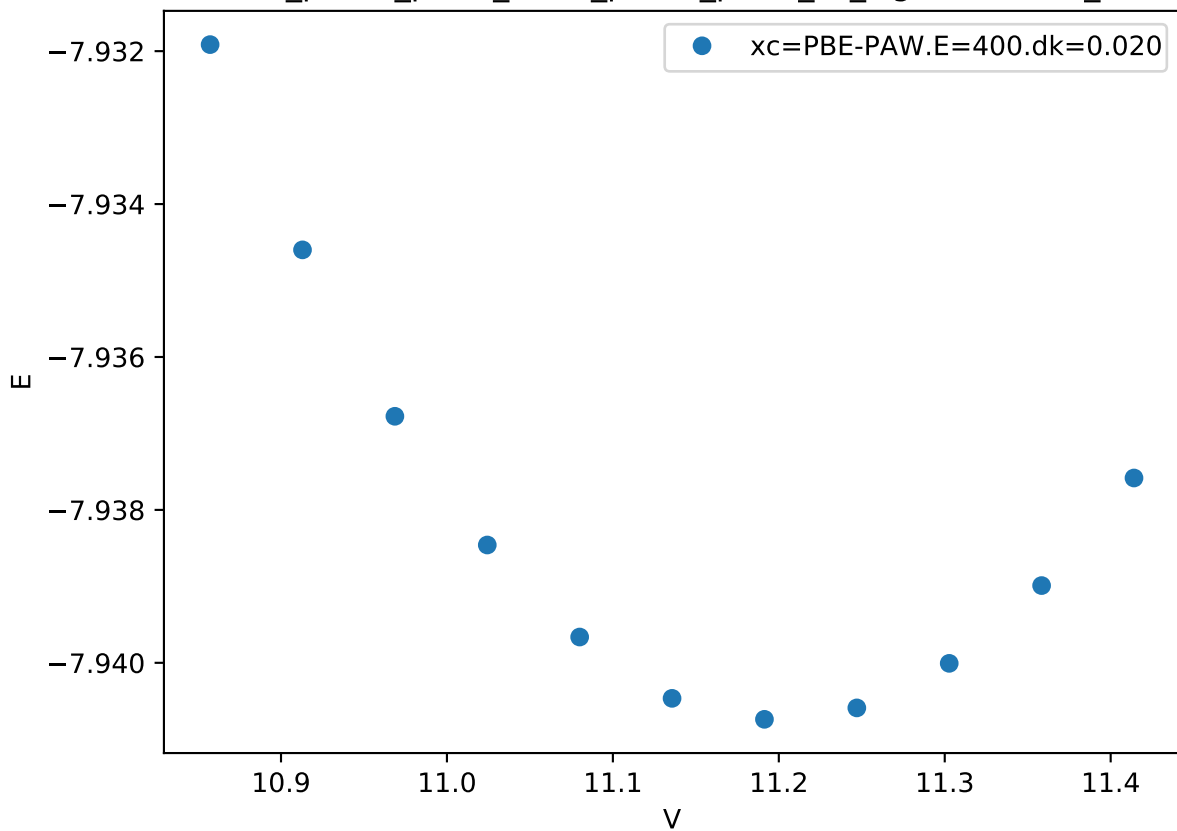
Cr_pv-Co_pv-W_sv/Cr_pv-Co_pv-W_sv_sigma-CBABB_
