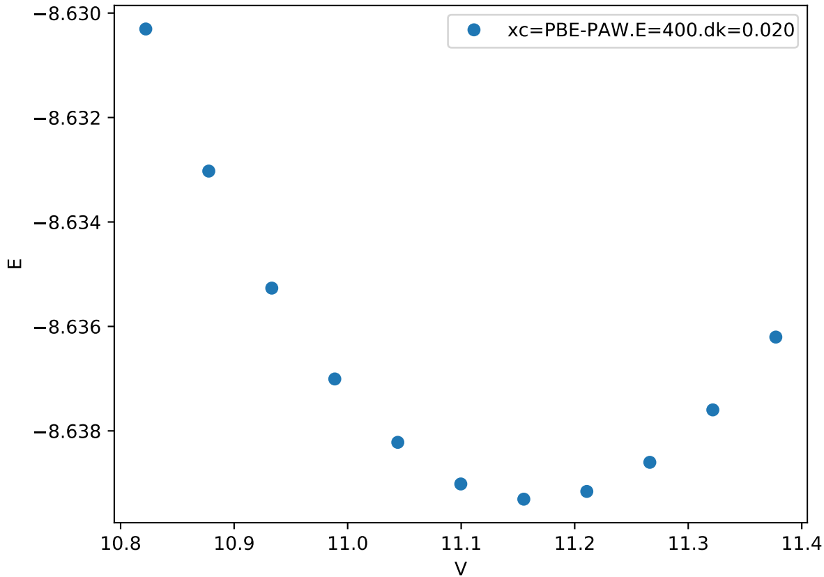
Cr_pv-Co_pv-W_sv/Cr_pv-Co_pv_sigma-BAABA_
