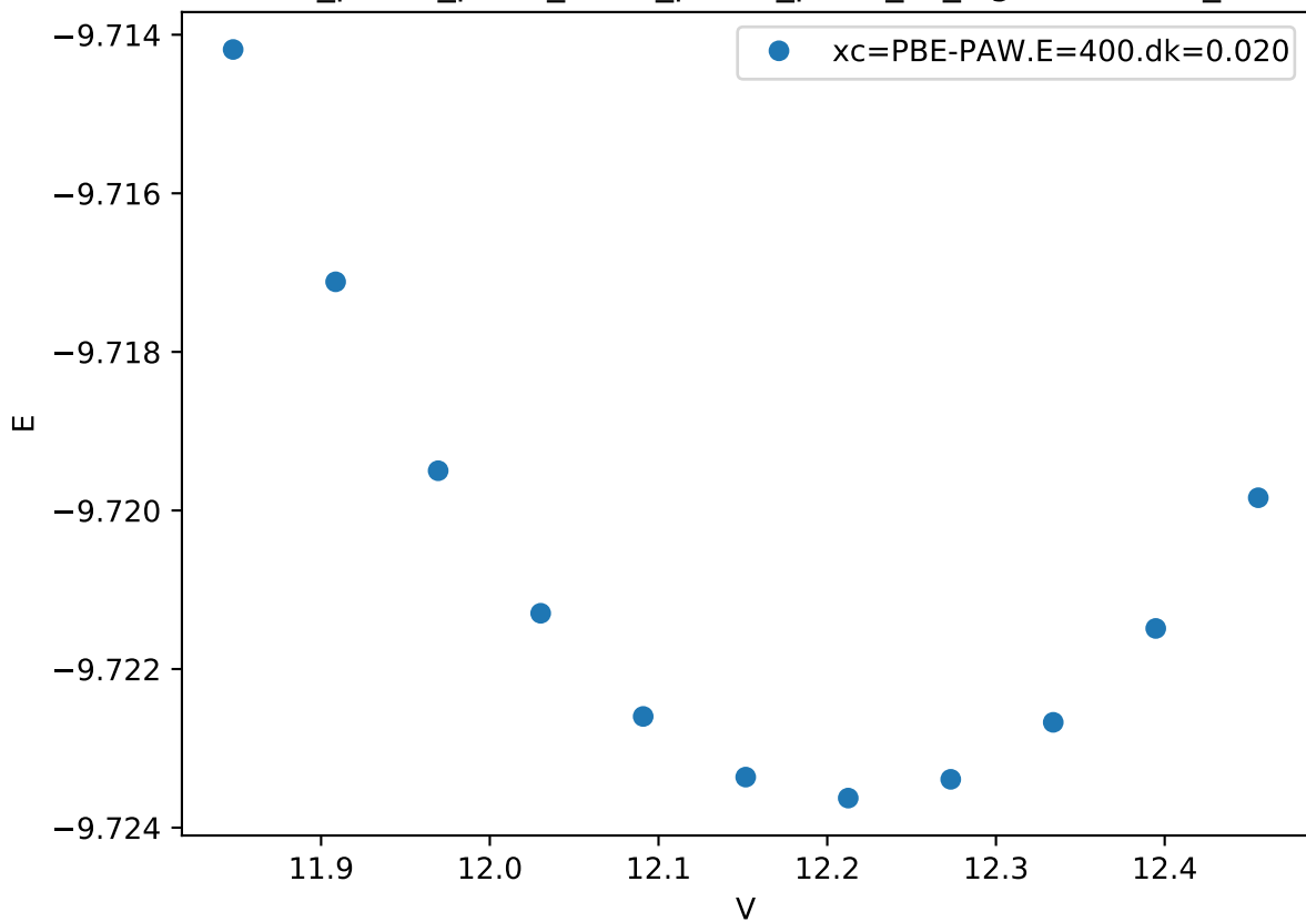
Cr_pv-Co_pv-W_sv/Cr_pv-Co_pv-W_sv_sigma-BCAAA_
