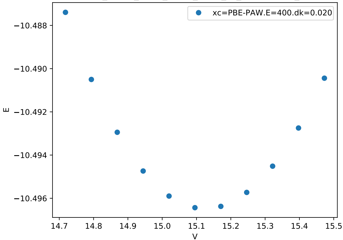
Cr_pv-Co_pv-W_sv/Co_pv-W_sv_C36-BAABB_
