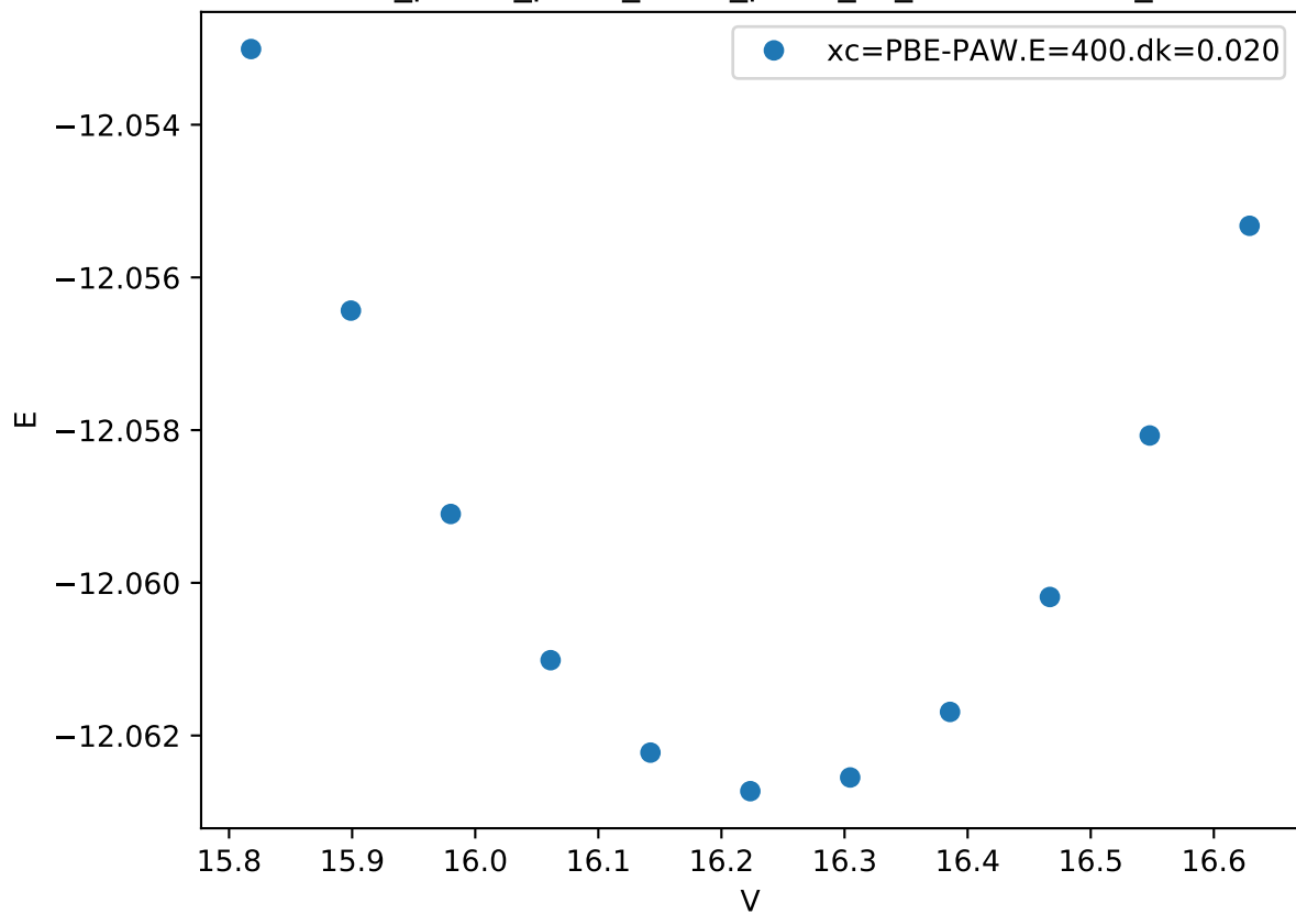
Cr_pv-Co_pv-W_sv/Cr_pv-W_sv_chi-BABB.FM_
