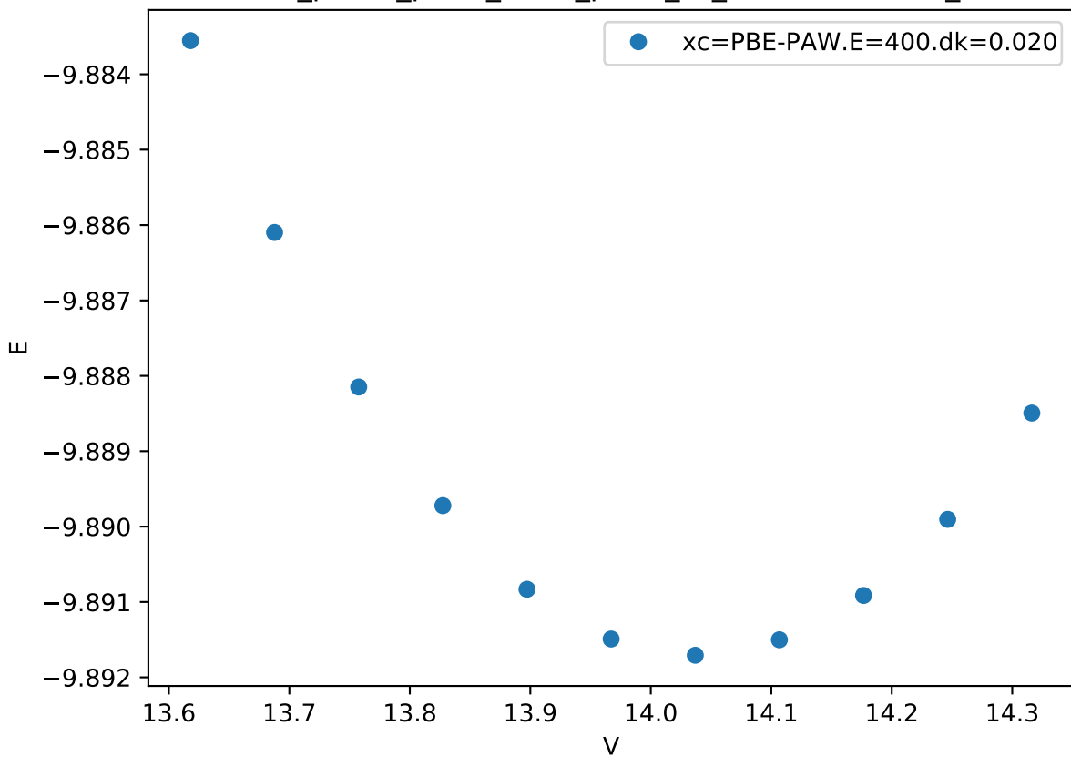
Cr_pv-Co_pv-W_sv/Cr_pv-W_sv_C36-AAAAB.FM_
