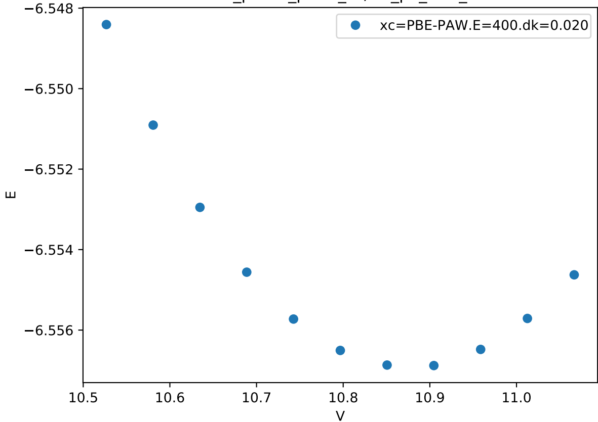
Cr_pv-Co_pv-W_sv/Co_pv_C14_
