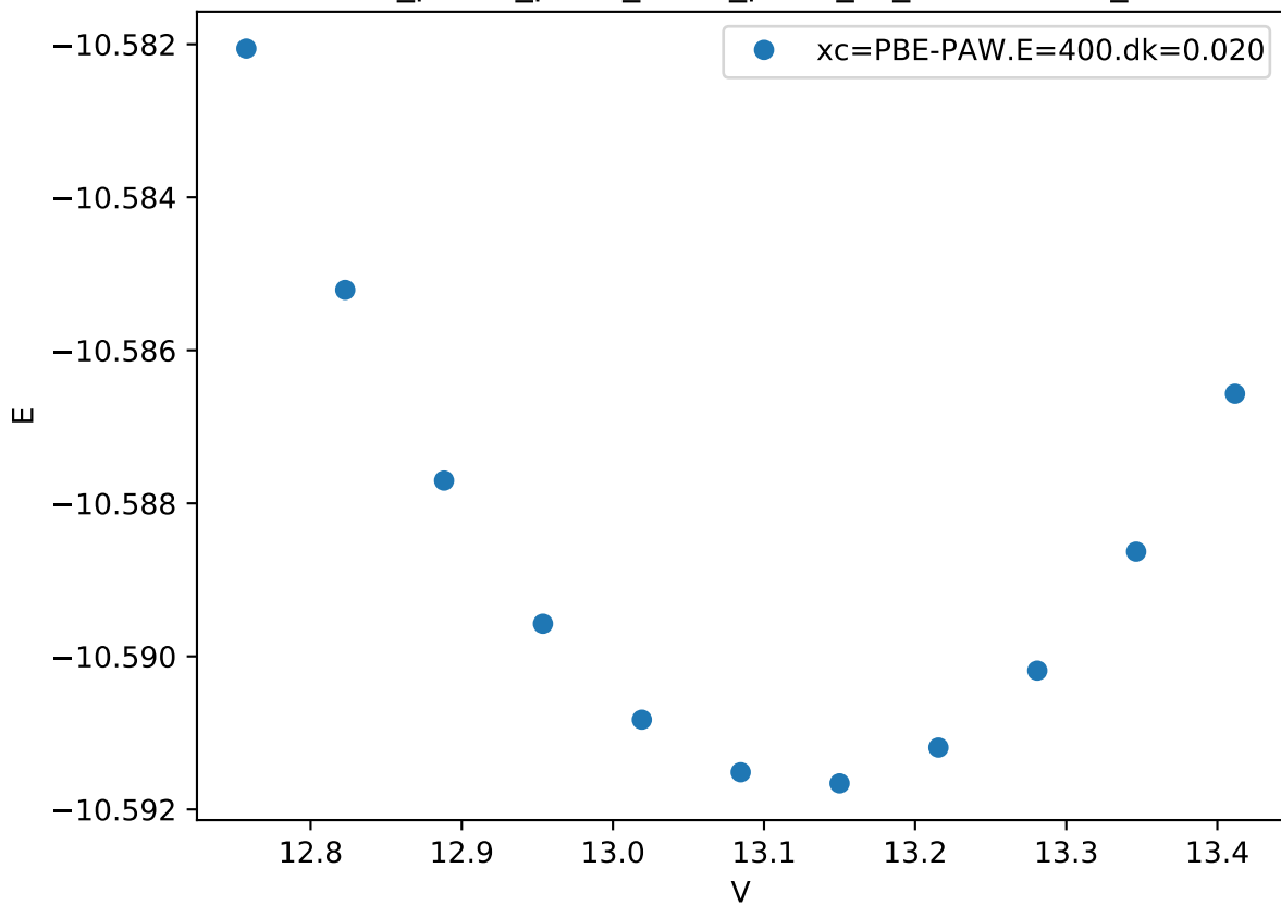
Cr_pv-Co_pv-W_sv/Cr_pv-W_sv_C36-BBAAA_
