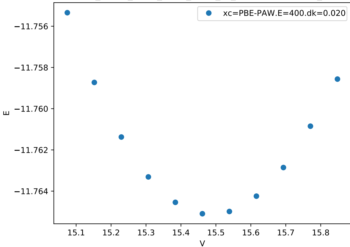
Cr_pv-Co_pv-W_sv/Cr_pv-W_sv_sigma-BBBBA.FM_
