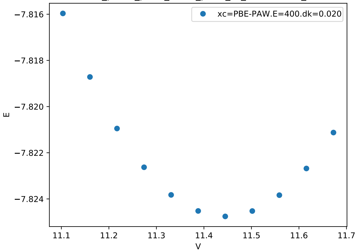
Cr_pv-Co_pv-W_sv/Co_pv-W_sv_C36-BAAAA_
