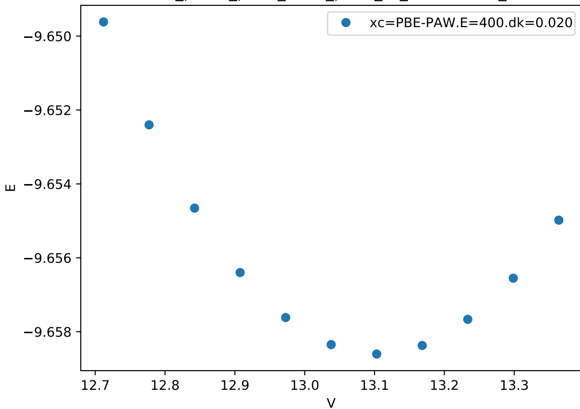
Cr_pv-Co_pv-W_sv/Cr_pv-W_sv_C36-AABAA_
