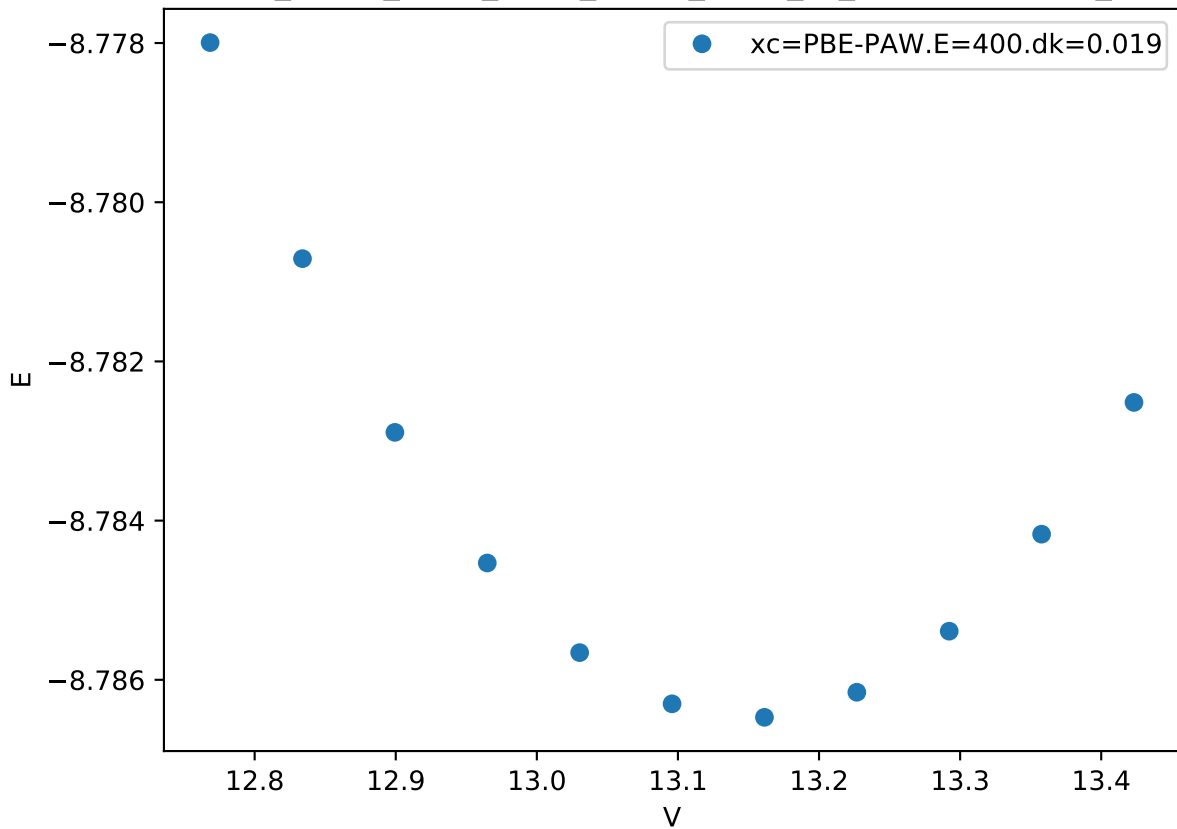
Cr_pv-Co_pv-W_sv/Cr_pv-Co_pv-W_sv_C36-AABCB.FM_
