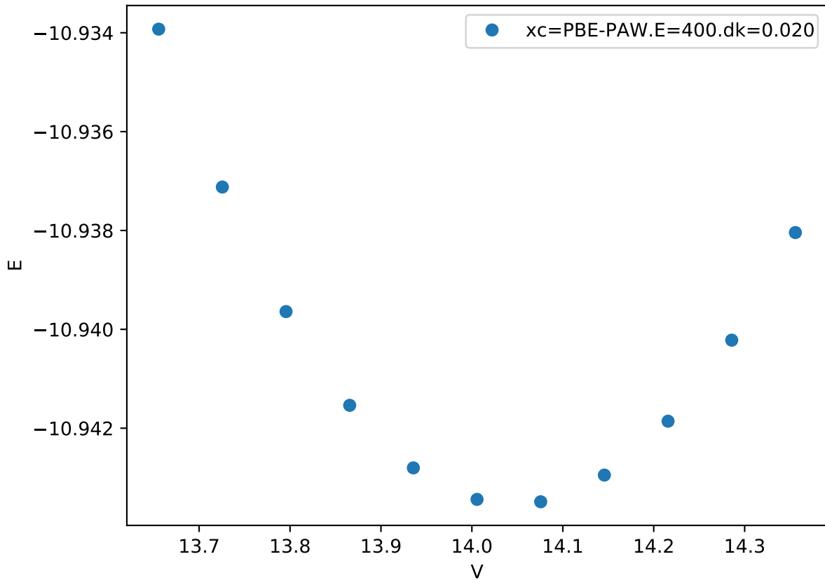
Cr_pv-Co_pv-W_sv/Cr_pv-W_sv_sigma-BBAA_
