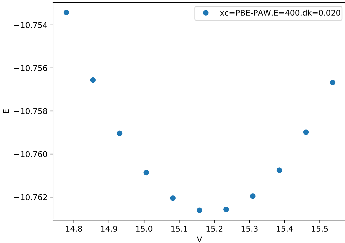
Cr_pv-Co_pv-W_sv/Cr_pv-Co_pv-W_sv_mu-ACBCA.FM_
