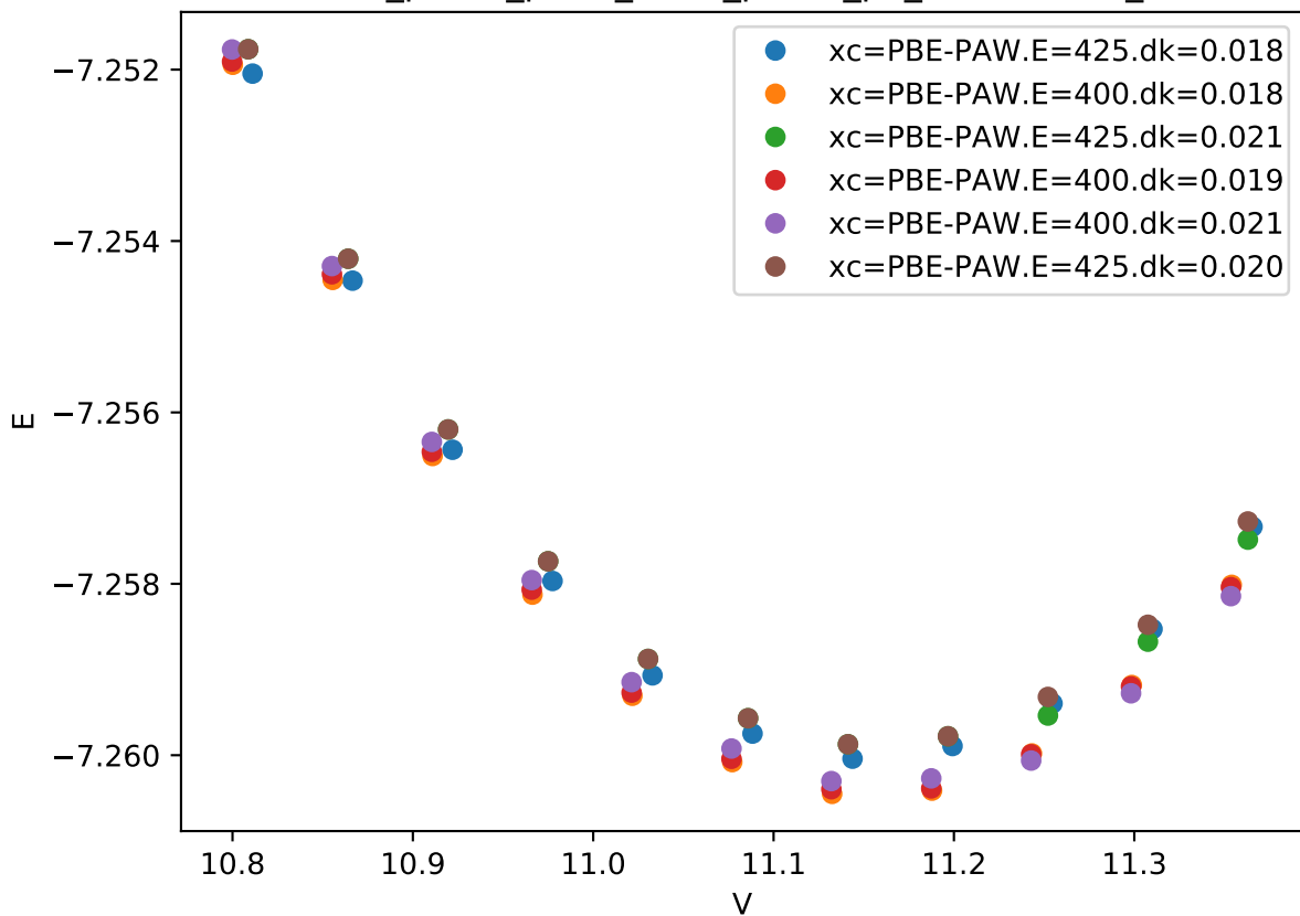
Cr_pv-Co_pv-W_sv/Cr_pv-Co_pv_C36-BBBBA_
