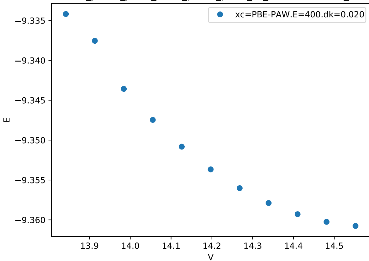
Cr_pv-Co_pv-W_sv/Cr_pv-Co_pv-W_sv_C36-BACCB.FM_
