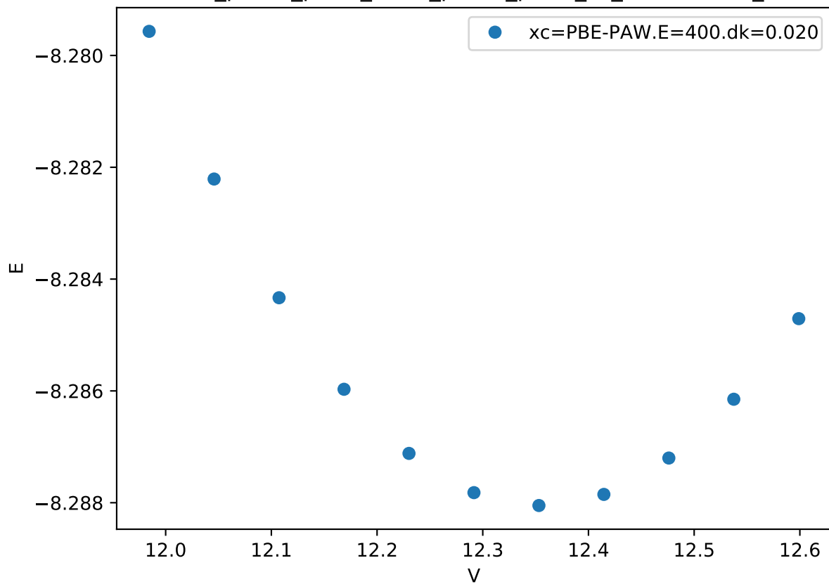
Cr_pv-Co_pv-W_sv/Cr_pv-Co_pv-W_sv_C36-BBCAB_
