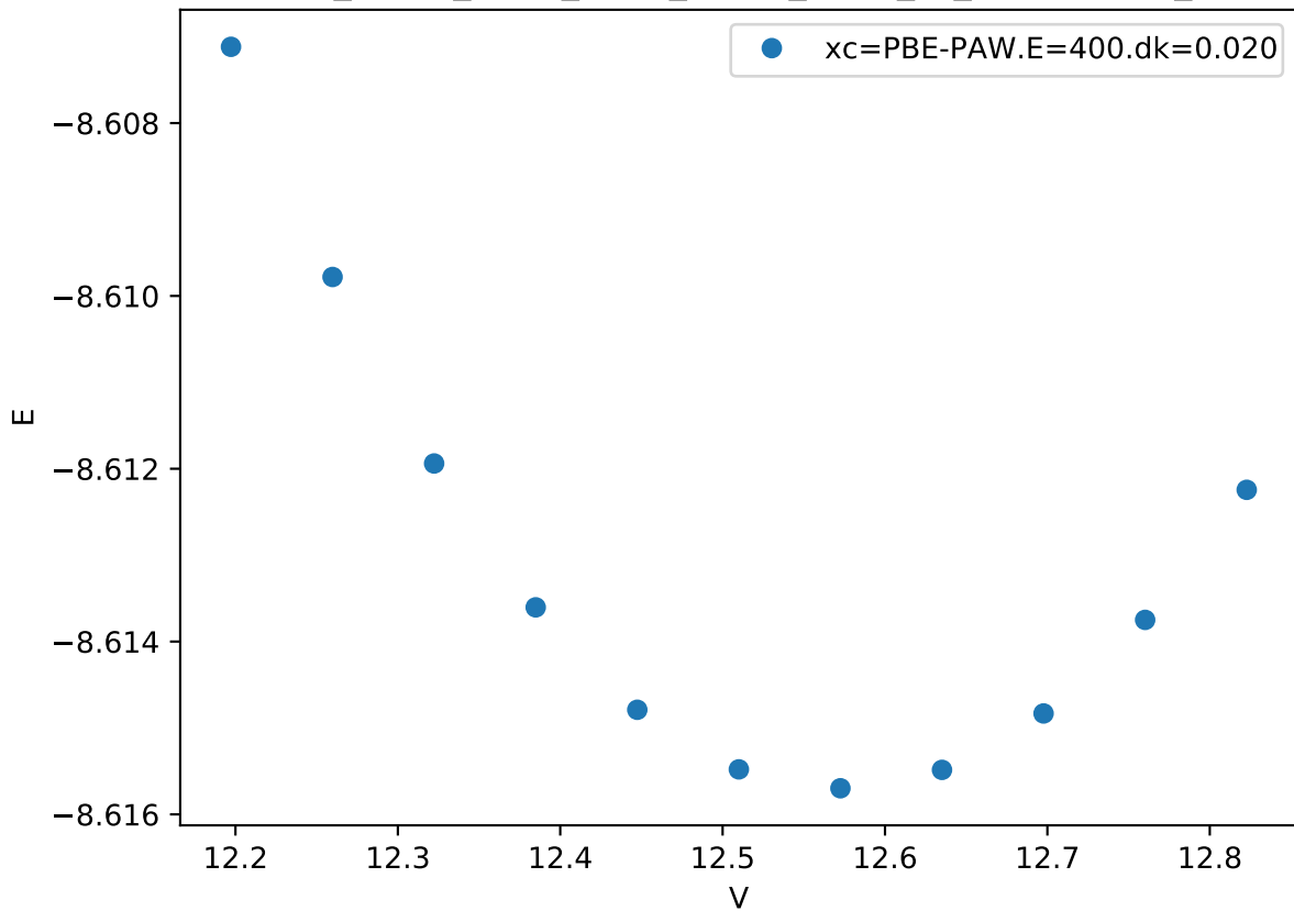
Cr_pv-Co_pv-W_sv/Cr_pv-Co_pv-W_sv_C36-BACBA_
