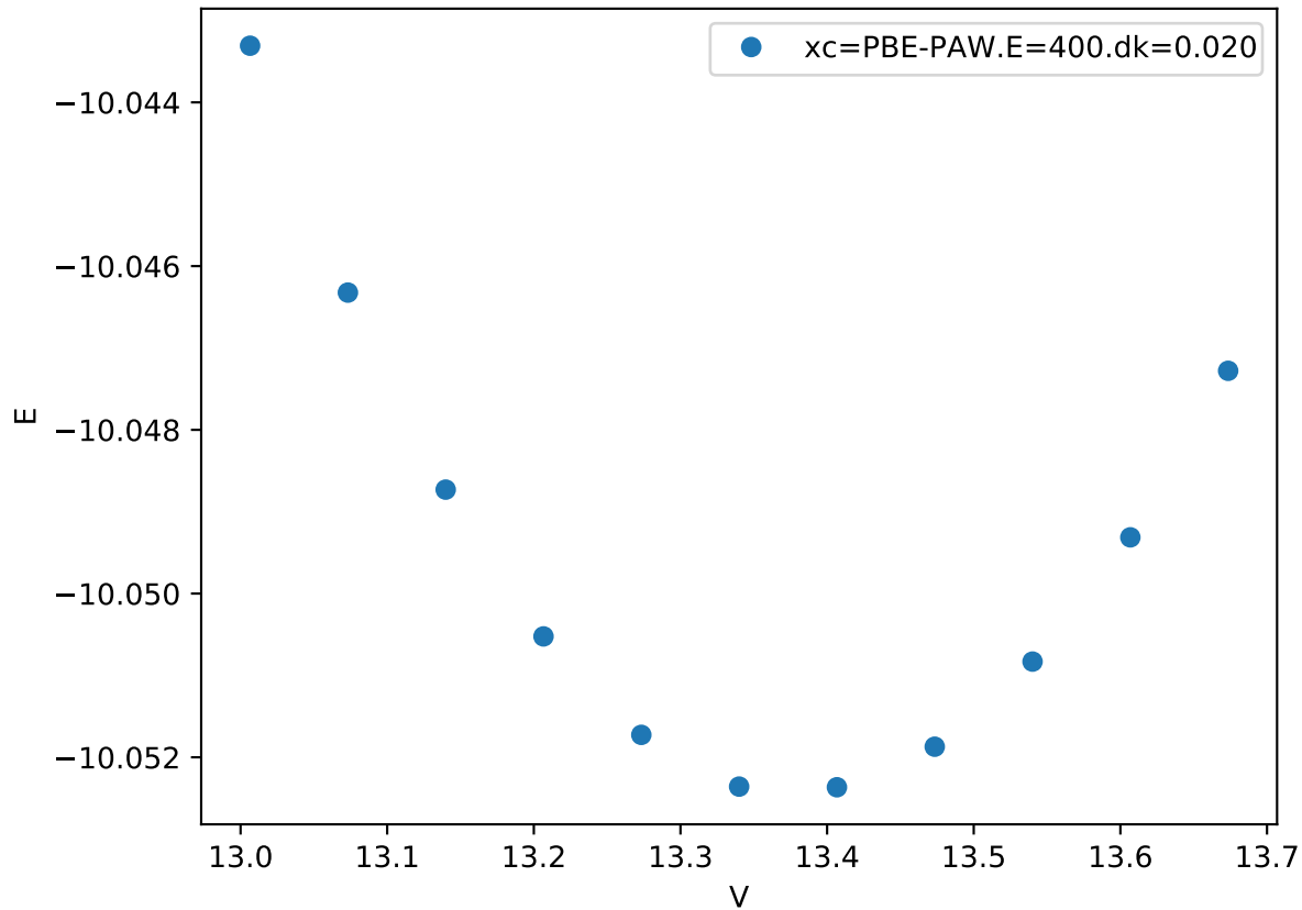
Cr_pv-Co_pv-W_sv/Cr_pv-Co_pv-W_sv_sigma-ACBAC_
