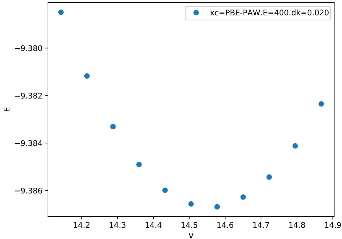
Cr_pv-Co_pv-W_sv/Cr_pv-Co_pv-W_sv_C36-BBCAC_
