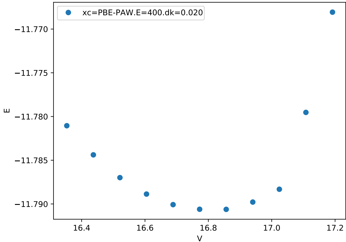
Cr_pv-Co_pv-W_sv/Cr_pv-W_sv_C36-BABBB.FM_
