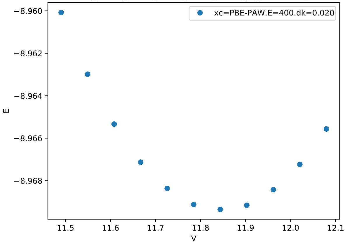
Cr_pv-Co_pv-W_sv/Cr_pv-Co_pv-W_sv_chi-CCAB_
