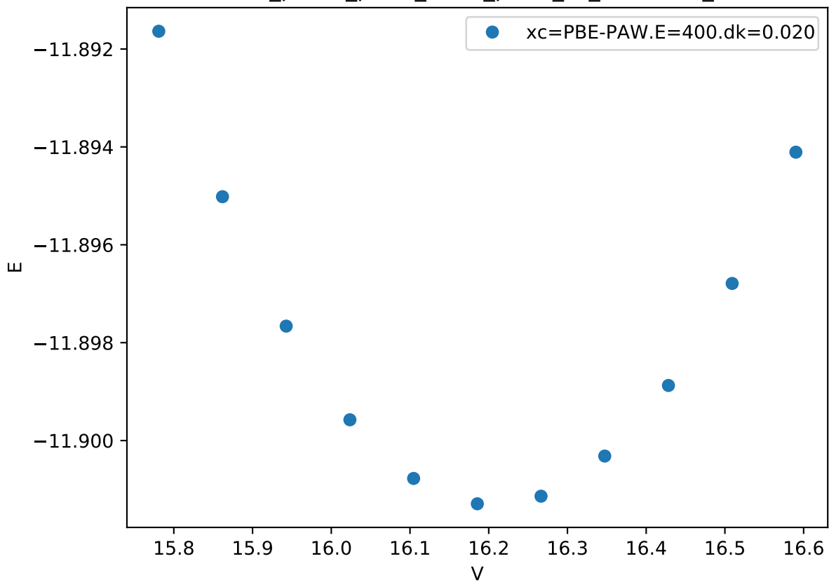
Cr_pv-Co_pv-W_sv/Cr_pv-W_sv_chi-AABB_
