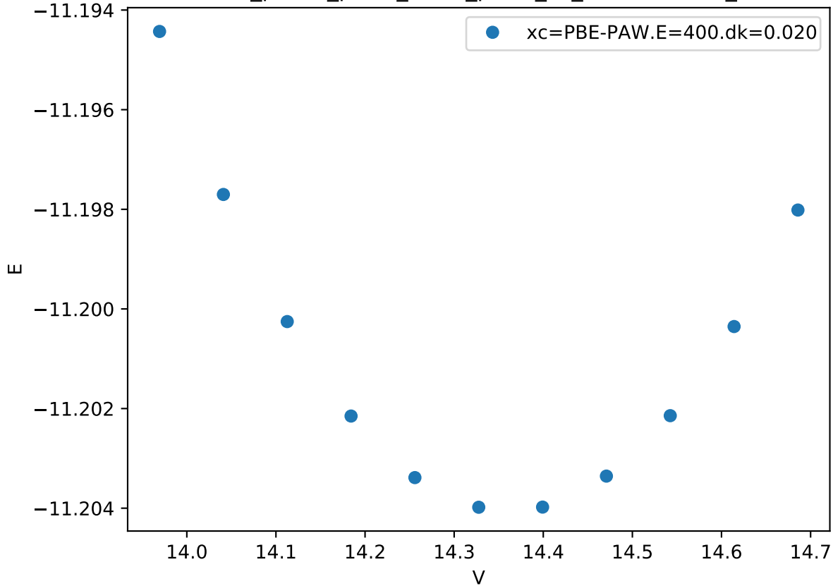
Cr_pv-Co_pv-W_sv/Cr_pv-W_sv_chi-ABBA.FM_
