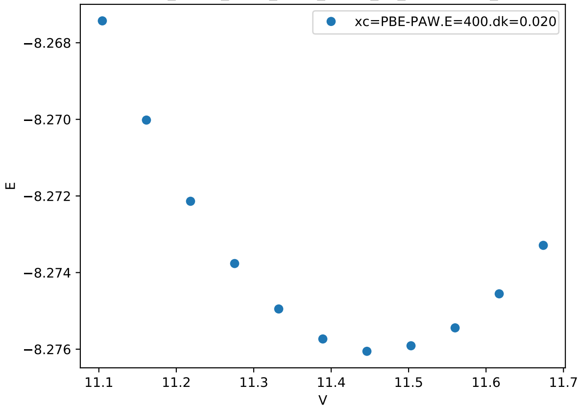
Cr_pv-Co_pv-W_sv/Cr_pv-Co_pv_mu-BABBA_
