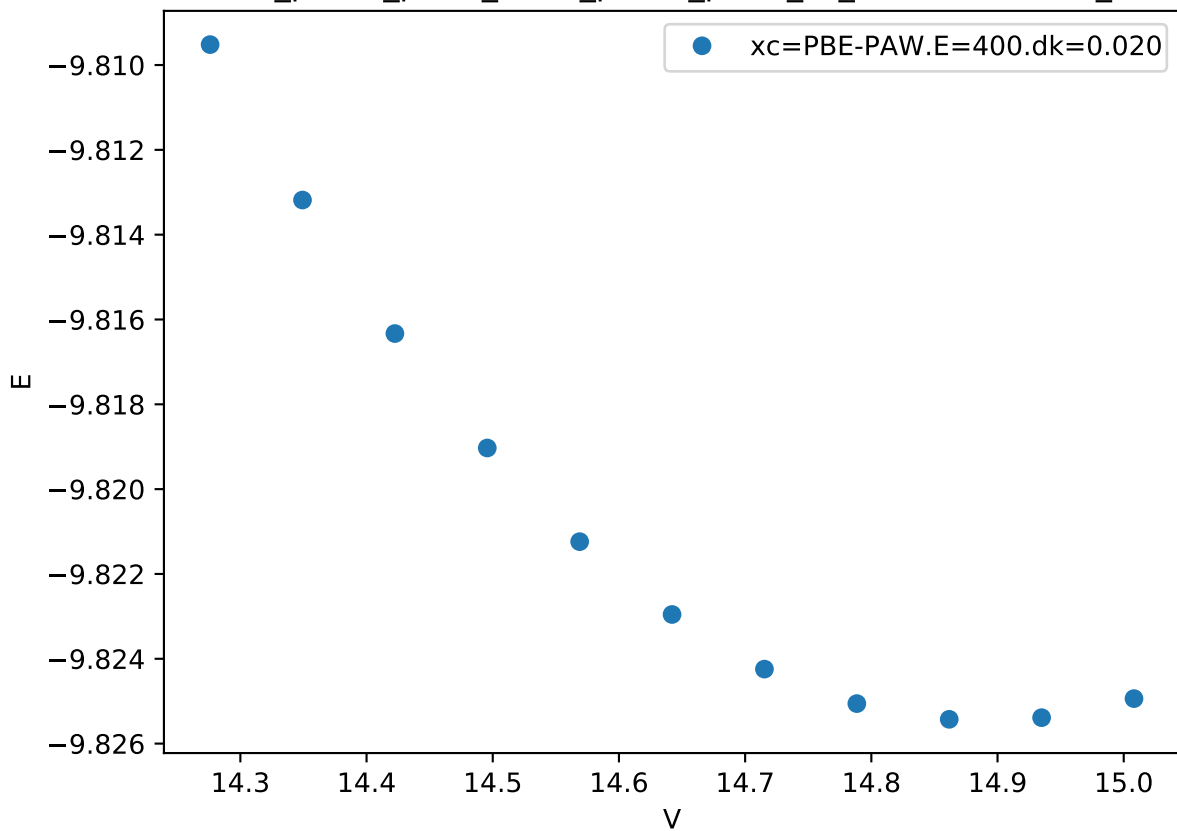
Cr_pv-Co_pv-W_sv/Cr_pv-Co_pv-W_sv_C36-AACCB.FM_
