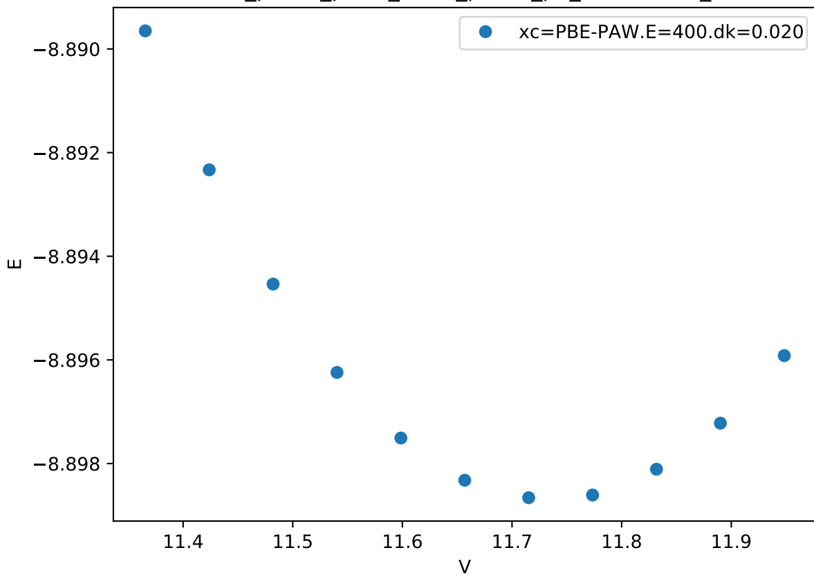
Cr_pv-Co_pv-W_sv/Cr_pv-Co_pv_mu-AAABA_
