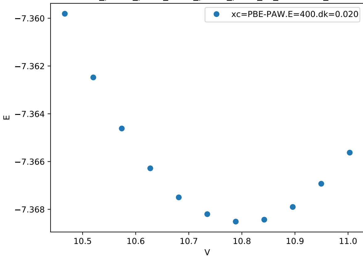
Cr_pv-Co_pv-W_sv/Cr_pv-Co_pv-W_sv_chi-CABB_
