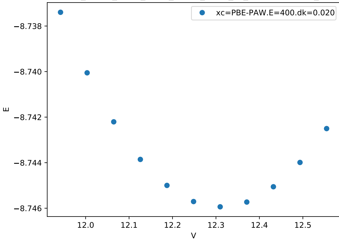
Cr_pv-Co_pv-W_sv/Cr_pv-Co_pv-W_sv_mu-BABBC.FM_
