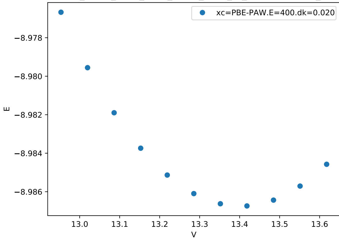
Cr_pv-Co_pv-W_sv/Cr_pv-Co_pv-W_sv_C36-BBACA.FM_
