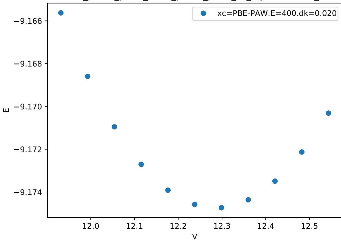
Cr_pv-Co_pv-W_sv/Cr_pv-Co_pv-W_sv_sigma-BBCBA_
