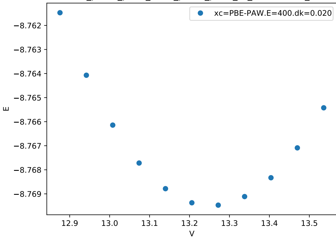
Cr_pv-Co_pv-W_sv/Cr_pv-Co_pv-W_sv_C36-ABACB_
