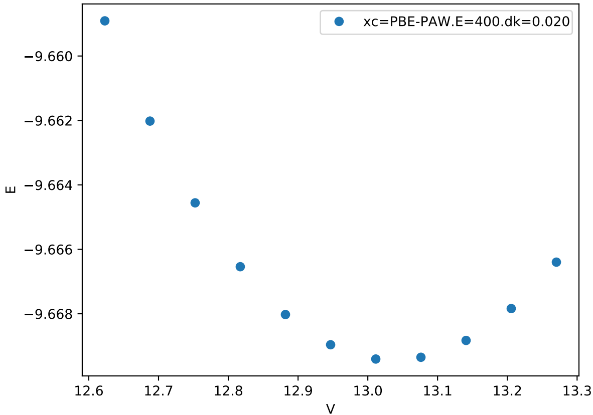
Cr_pv-Co_pv-W_sv/Cr_pv-Co_pv-W_sv_sigma-BBAAC.FM_
