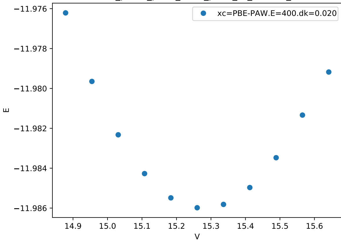
Cr_pv-Co_pv-W_sv/Cr_pv-W_sv_A15-BA_
