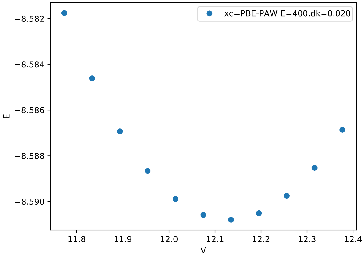
Cr_pv-Co_pv-W_sv/Cr_pv-Co_pv-W_sv_mu-CBCAB.FM_
