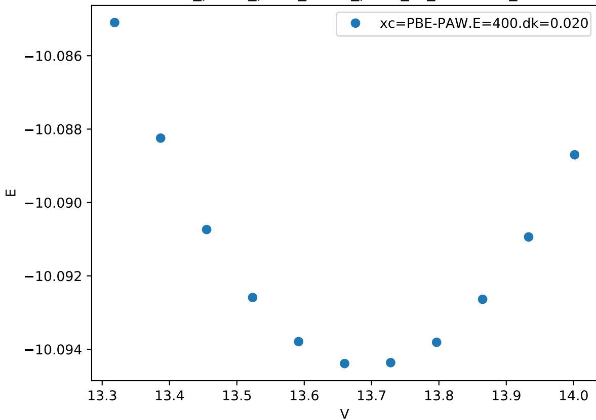
Cr_pv-Co_pv-W_sv/Co_pv-W_sv_chi-ABBA_
