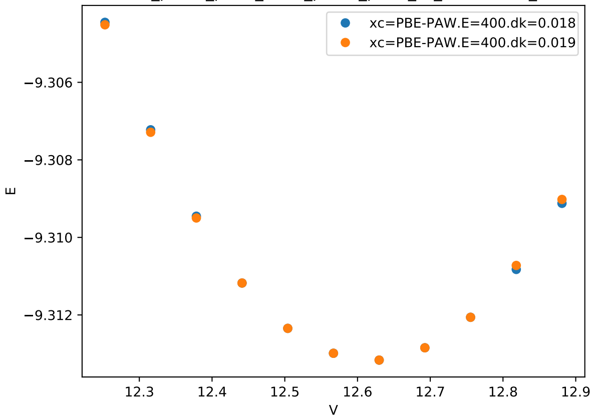
Cr_pv-Co_pv-W_sv/Cr_pv-Co_pv-W_sv_mu-CACBB_
