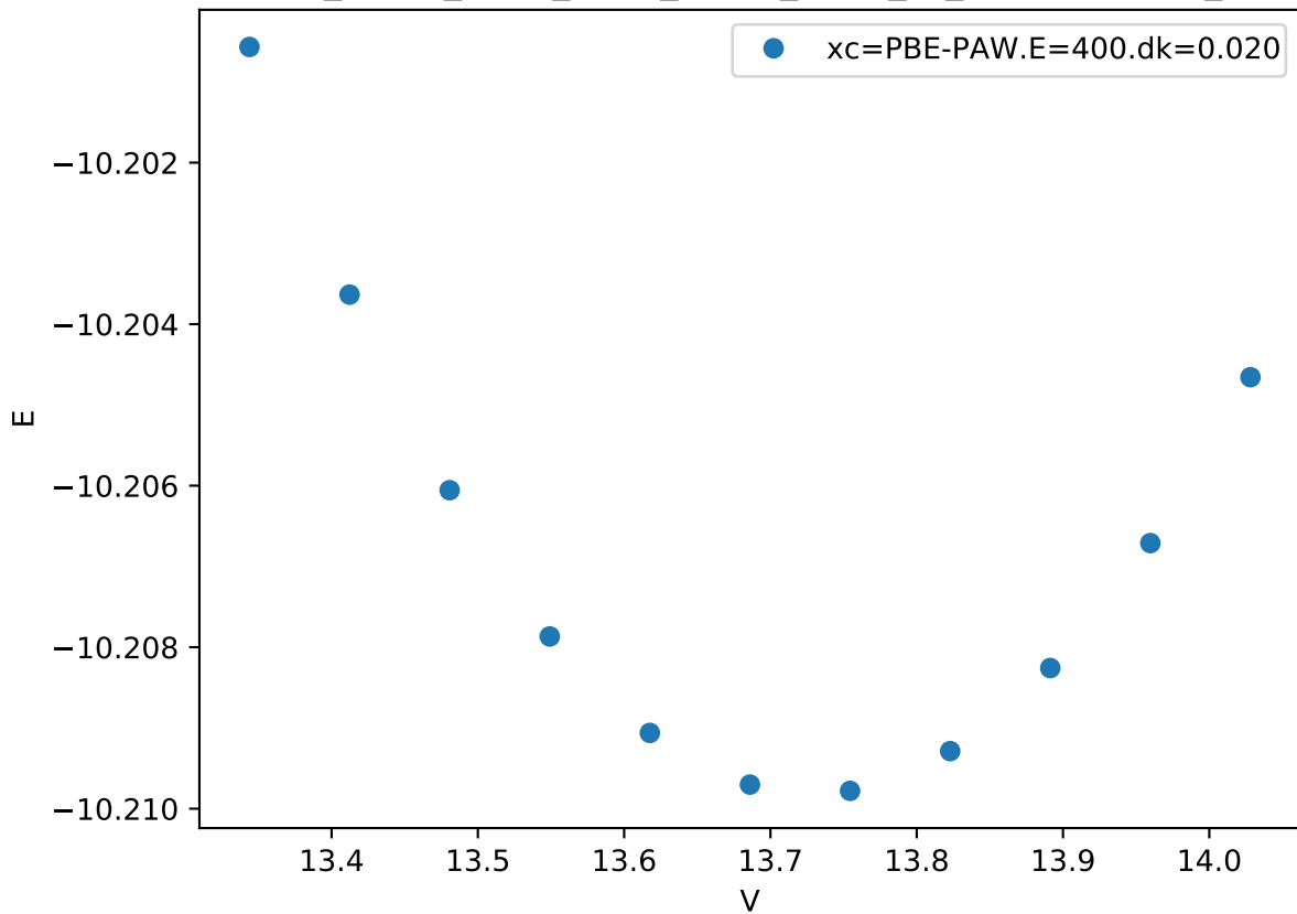
Cr_pv-Co_pv-W_sv/Cr_pv-Co_pv-W_sv_sigma-CCCAB_
