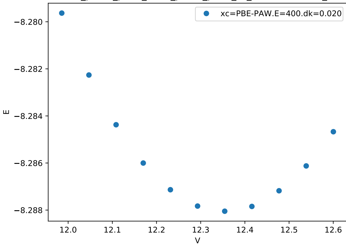
Cr_pv-Co_pv-W_sv/Cr_pv-Co_pv-W_sv_C36-BBCAB.FM_
