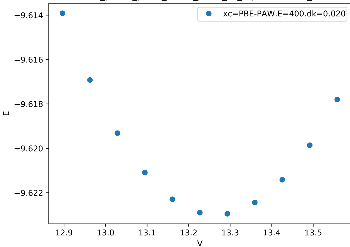
Cr_pv-Co_pv-W_sv/Co_pv-W_sv_sigma-BBAA_
