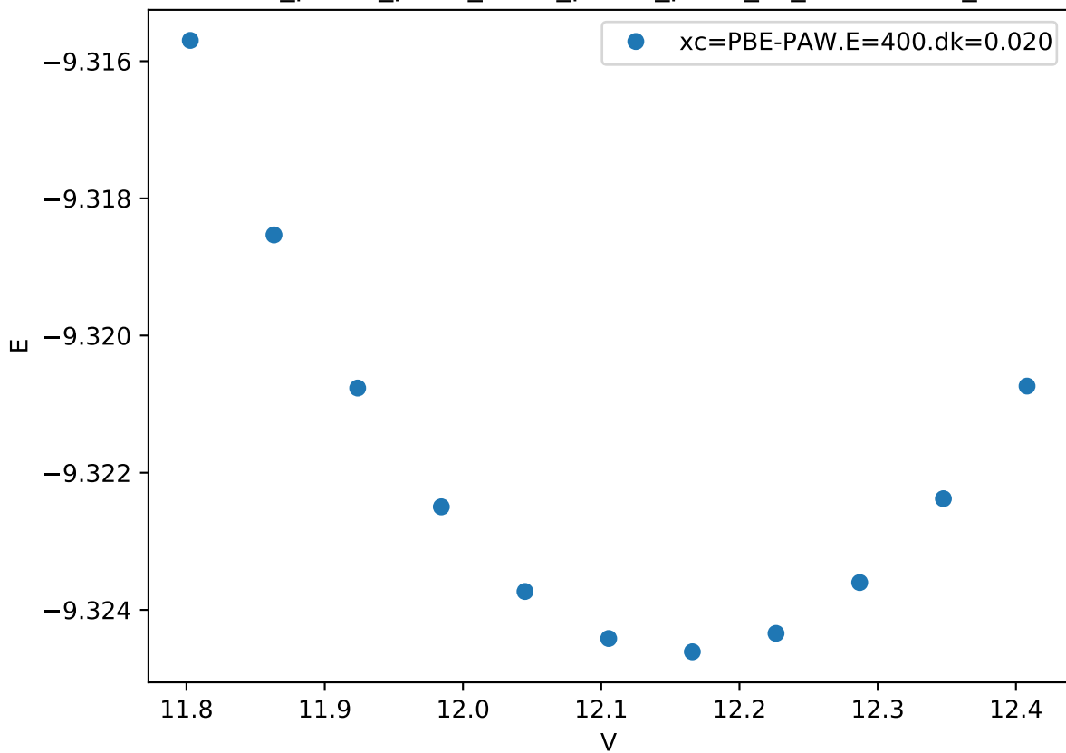
Cr_pv-Co_pv-W_sv/Cr_pv-Co_pv-W_sv_mu-BABCA_
