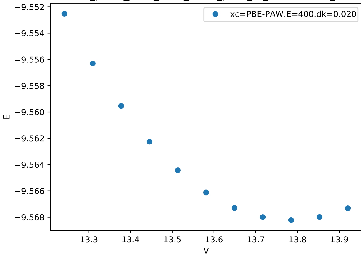
Cr_pv-Co_pv-W_sv/Cr_pv-Co_pv-W_sv_chi-AABC.FM_
