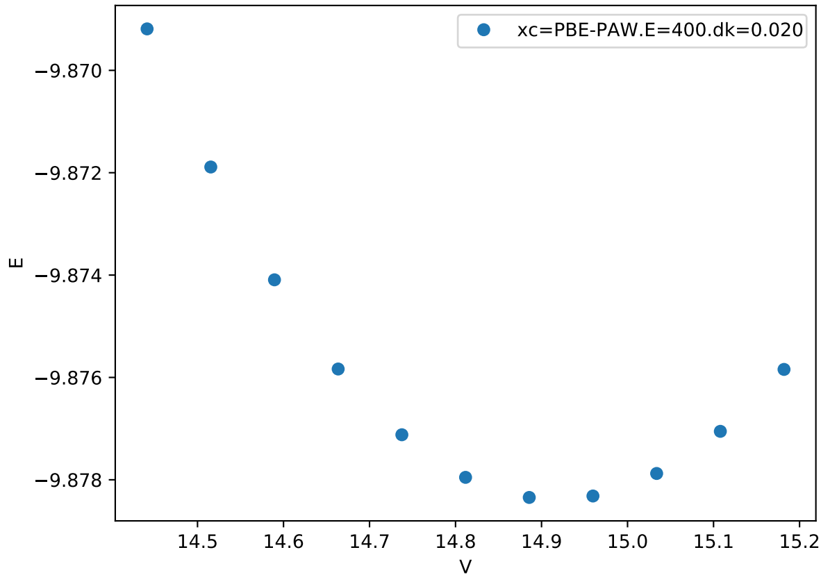
Cr_pv-Co_pv-W_sv/Cr_pv-Co_pv-W_sv_C36-ABCAC.FM_
