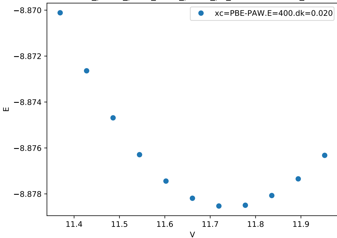
Cr_pv-Co_pv-W_sv/Cr_pv-Co_pv_C36-AABAA.FM_
