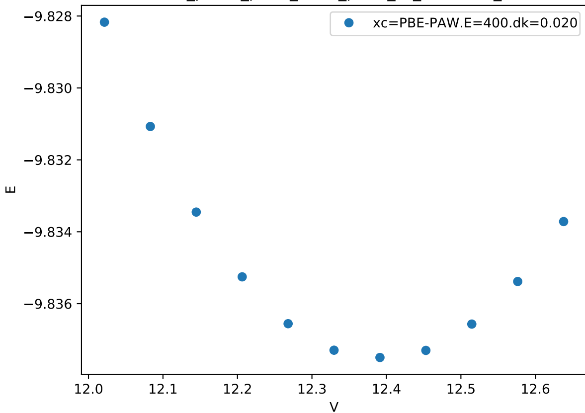
Cr_pv-Co_pv-W_sv/Cr_pv-W_sv_chi-ABAA_
