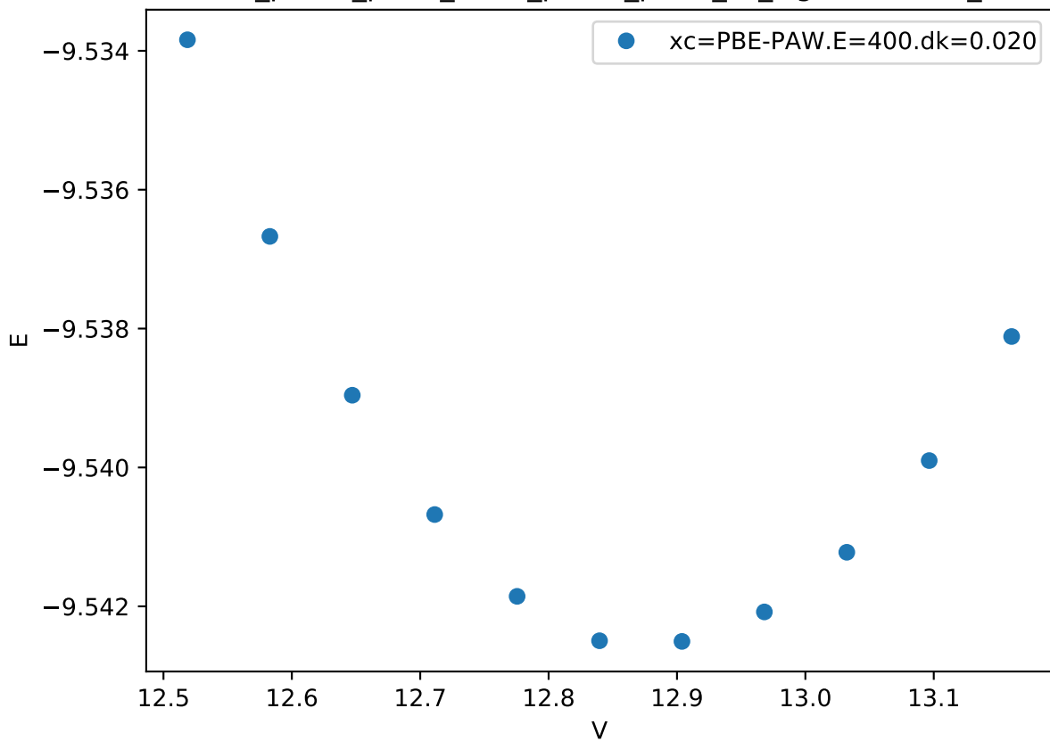
Cr_pv-Co_pv-W_sv/Cr_pv-Co_pv-W_sv_sigma-AABAC_
