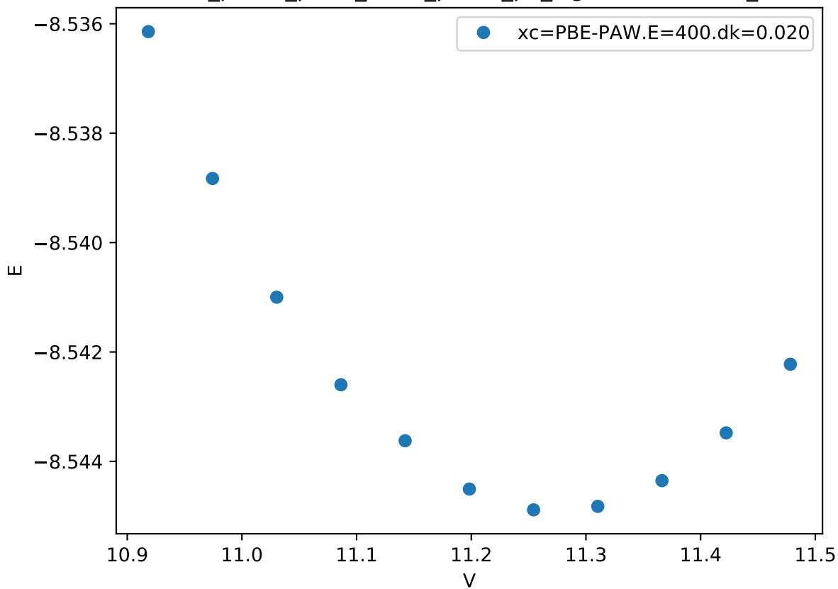
Cr_pv-Co_pv-W_sv/Cr_pv-Co_pv_sigma-BAAAB.FM_
