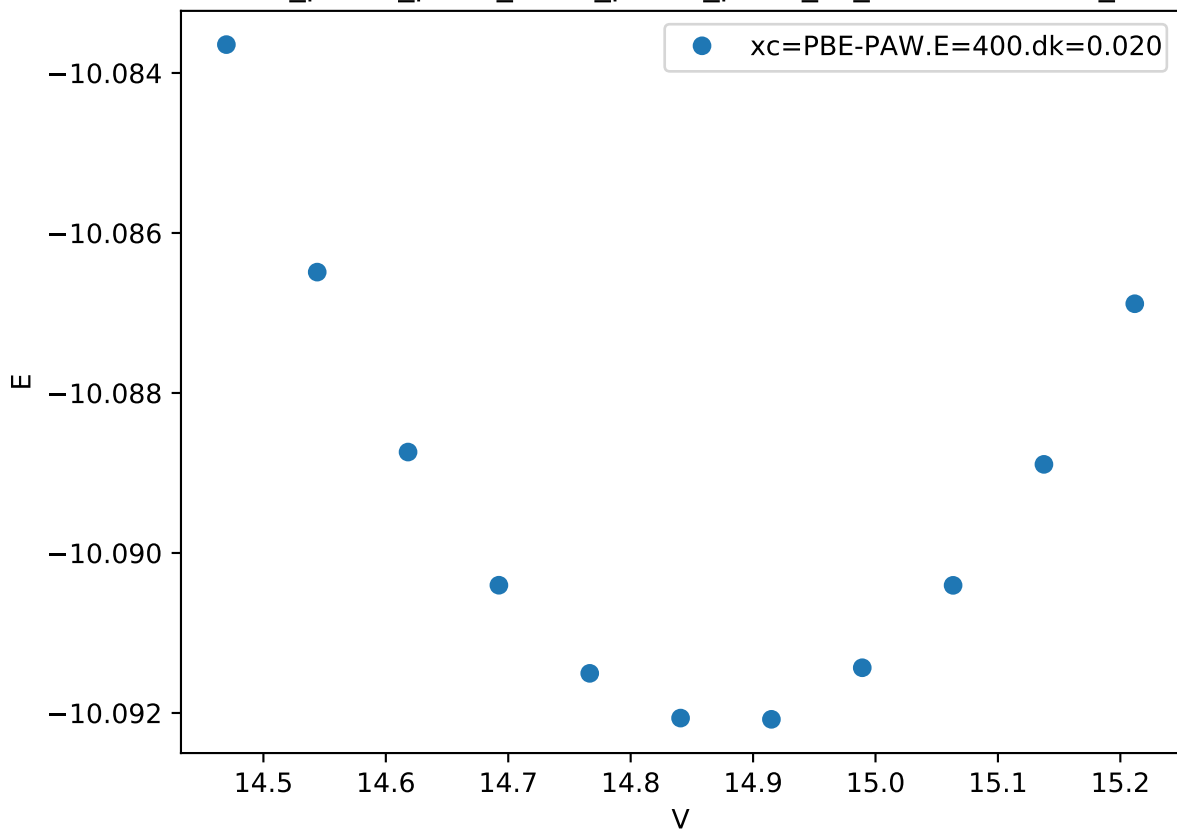
Cr_pv-Co_pv-W_sv/Cr_pv-Co_pv-W_sv_mu-ACBAA.FM_
