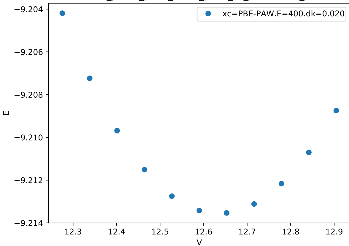
Cr_pv-Co_pv-W_sv/Co_pv-W_sv_mu-BABBA_
