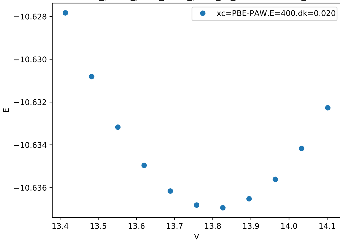
Cr_pv-Co_pv-W_sv/Cr_pv-W_sv_mu-BABAB.FM_
