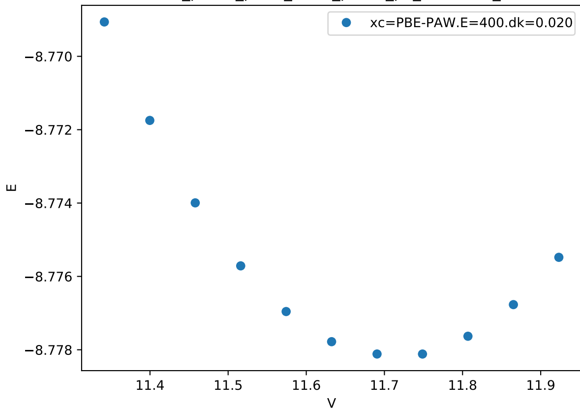
Cr_pv-Co_pv-W_sv/Cr_pv-Co_pv_chi-BBAA_
