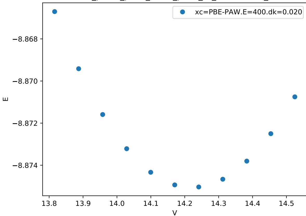
Cr_pv-Co_pv-W_sv/Co_pv-W_sv_C36-AABBA_
