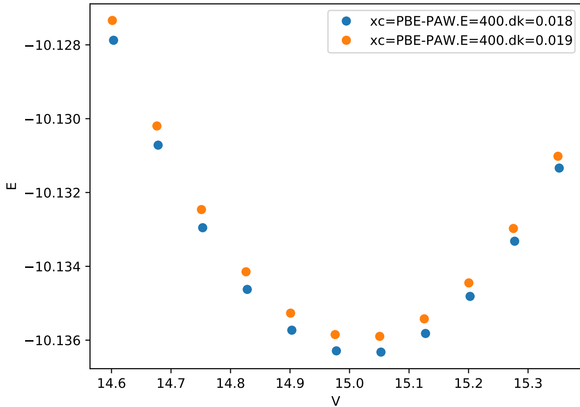
Cr_pv-Co_pv-W_sv/Cr_pv-Co_pv-W_sv_C36-BAACC_
