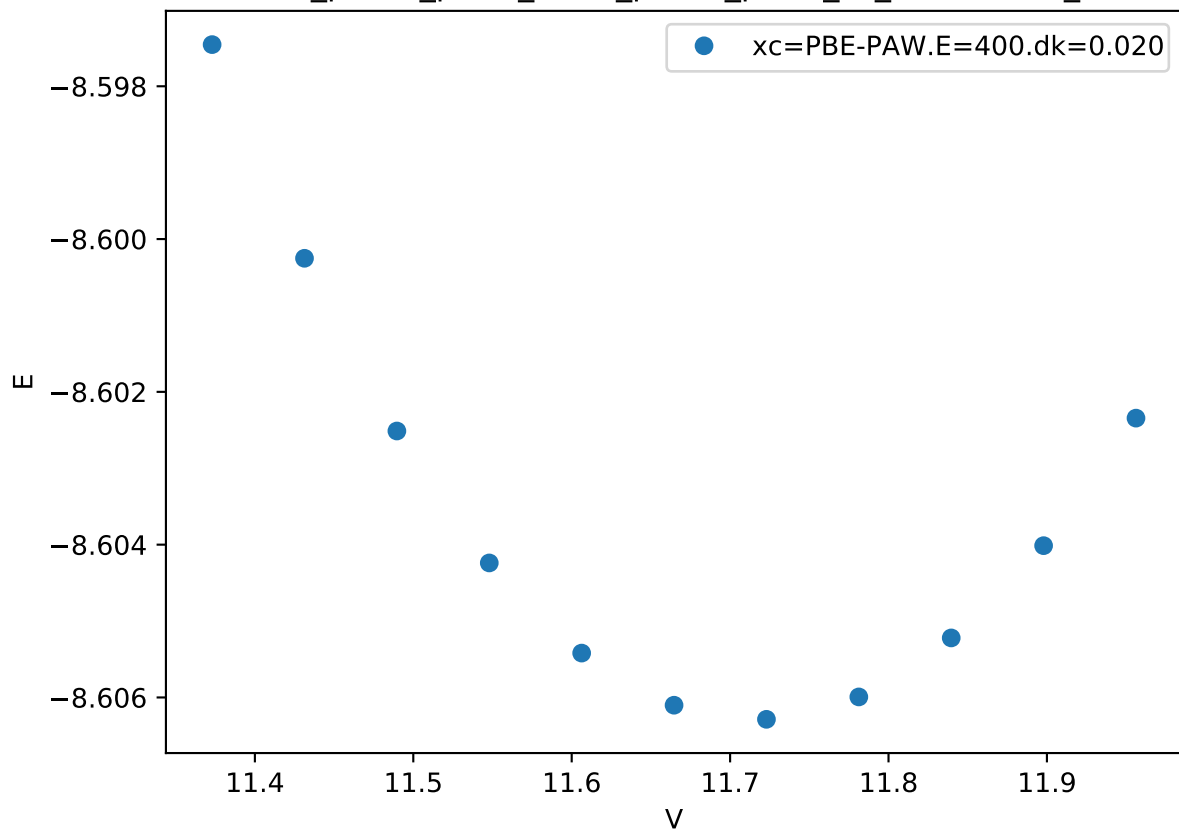
Cr_pv-Co_pv-W_sv/Cr_pv-Co_pv-W_sv_mu-BBCAA_
