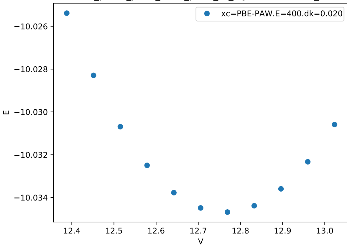
Cr_pv-Co_pv-W_sv/Cr_pv-W_sv_sigma-BBAAA.FM_
