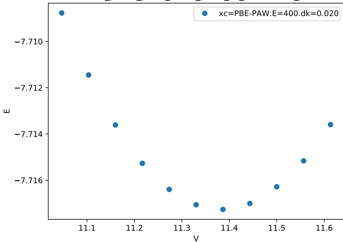
Cr_pv-Co_pv-W_sv/Co_pv-W_sv_mu-AAABA_
