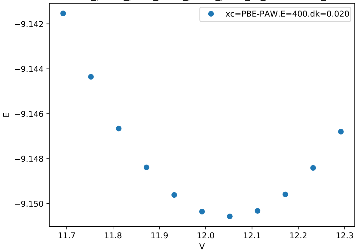
Cr_pv-Co_pv-W_sv/Cr_pv-Co_pv-W_sv_C36-BCBAA_
