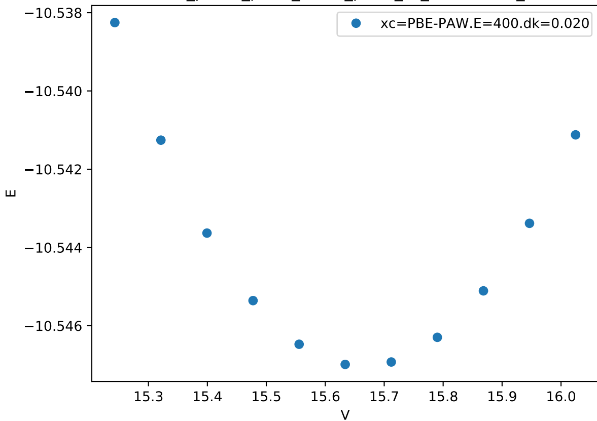
Cr_pv-Co_pv-W_sv/Co_pv-W_sv_mu-BBAA_
