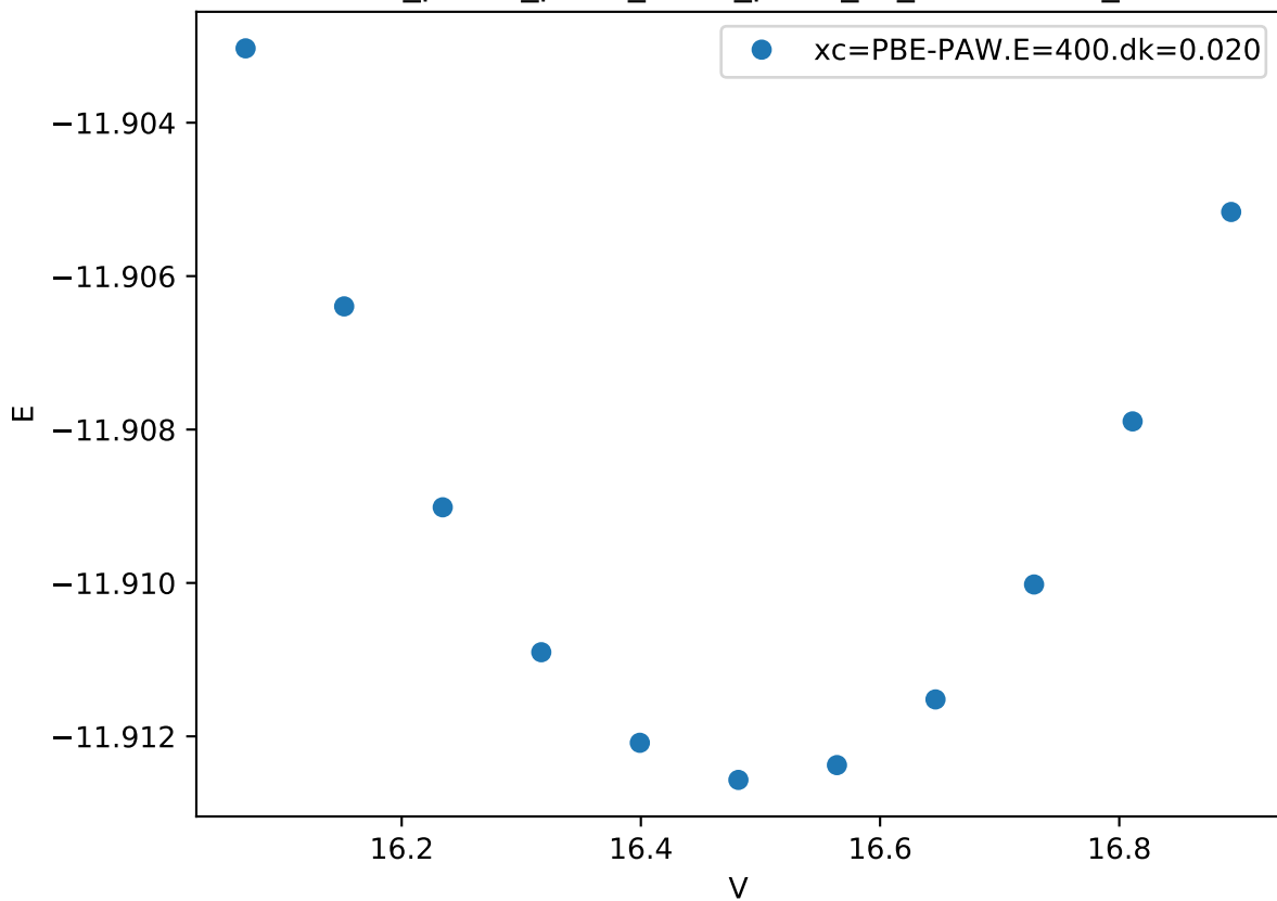
Cr_pv-Co_pv-W_sv/Cr_pv-W_sv_mu-BBBAB_
