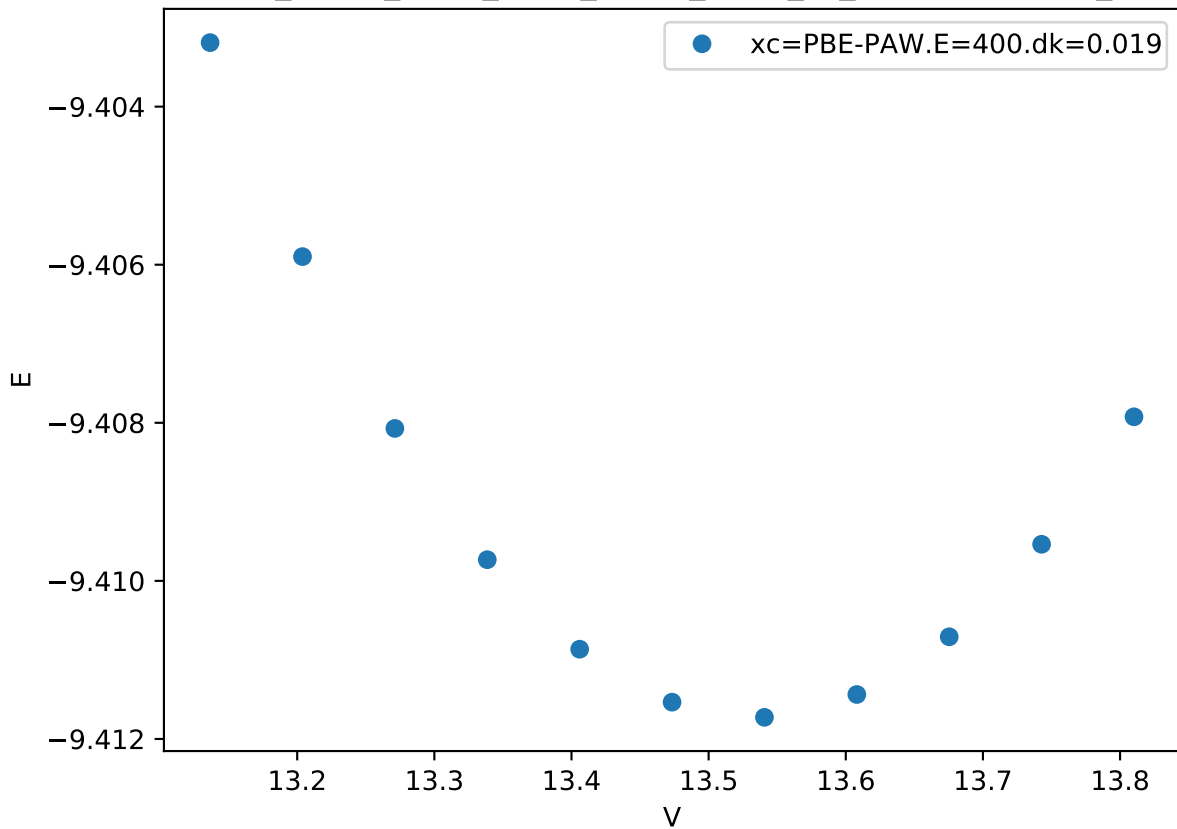
Cr_pv-Co_pv-W_sv/Cr_pv-Co_pv-W_sv_C36-BAACA.FM_
