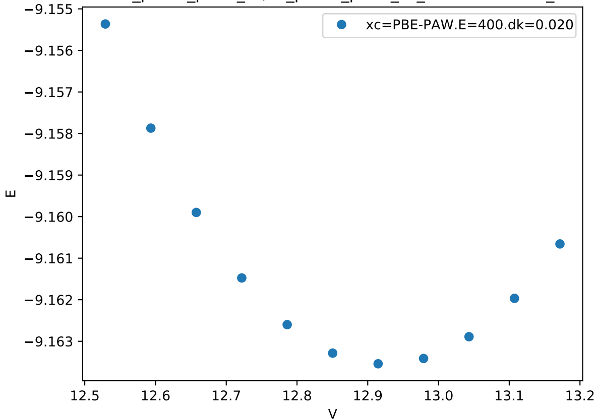
Cr_pv-Co_pv-W_sv/Cr_pv-Co_pv-W_sv_C36-AACAB.FM_
