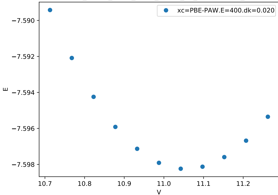
Cr_pv-Co_pv-W_sv/Cr_pv-Co_pv_C36-AABBB_
