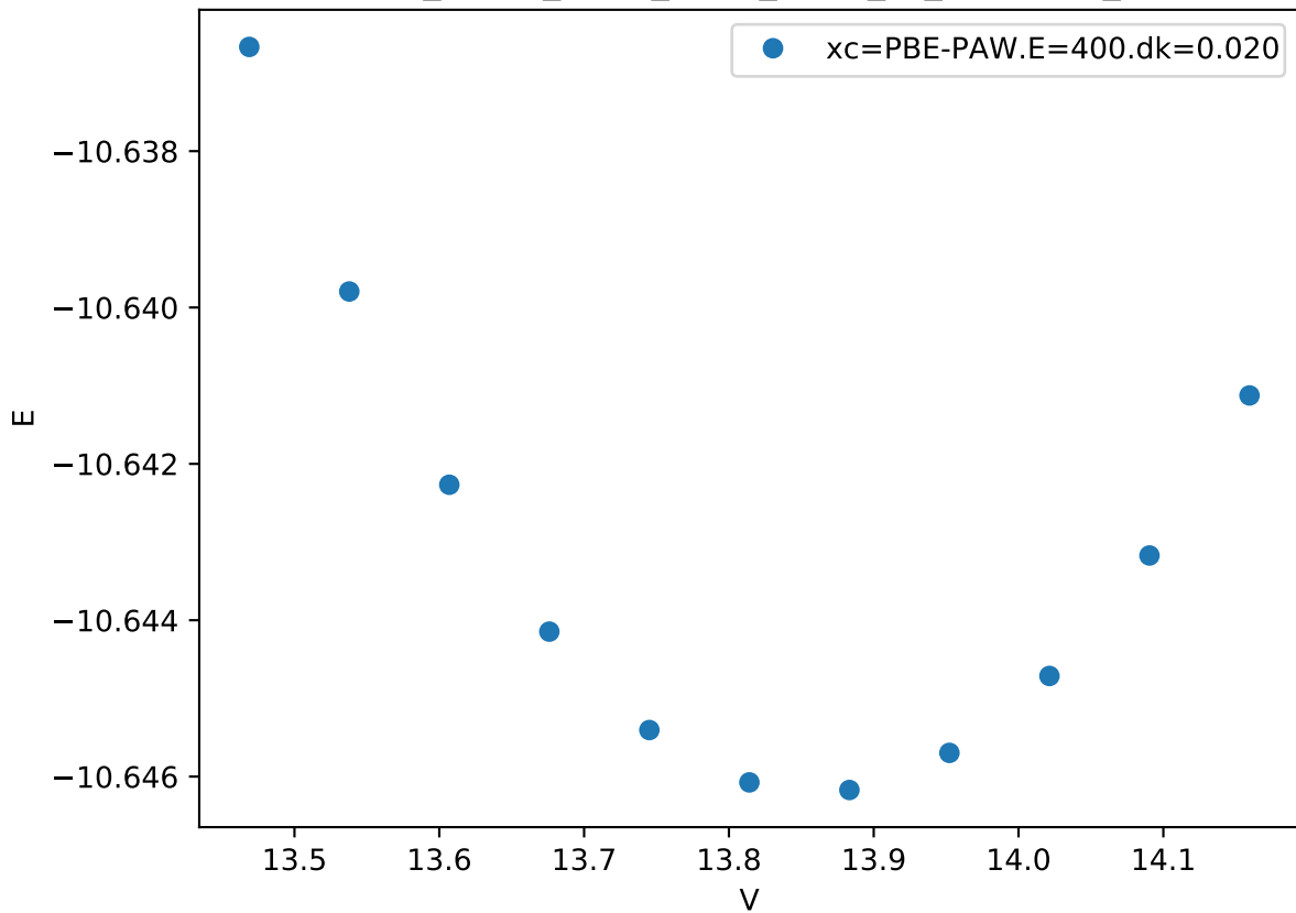
Cr_pv-Co_pv-W_sv/Cr_pv-W_sv_chi-AABA_
