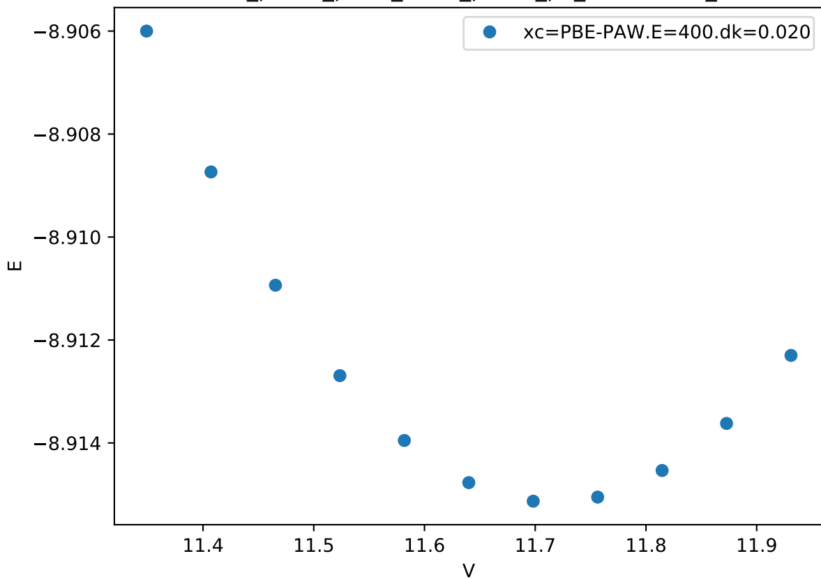
Cr_pv-Co_pv-W_sv/Cr_pv-Co_pv_mu-AAAAB_
