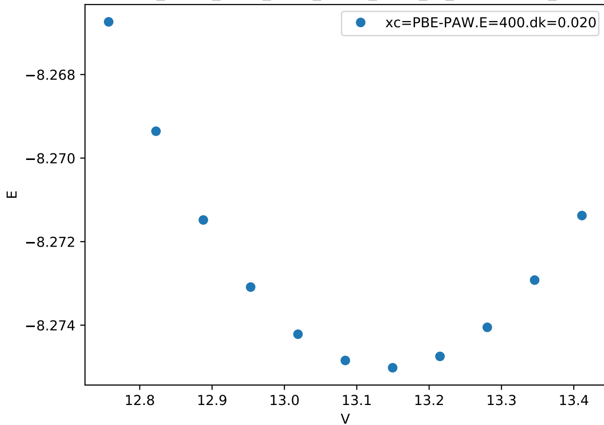
Cr_pv-Co_pv-W_sv/Cr_pv-Co_pv-W_sv_C36-BABBC_
