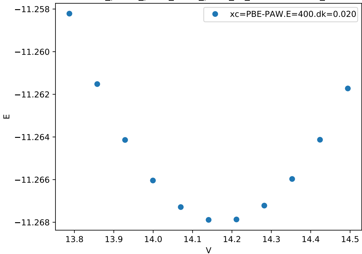
Cr_pv-Co_pv-W_sv/Cr_pv-W_sv_mu-BABBB.FM_
