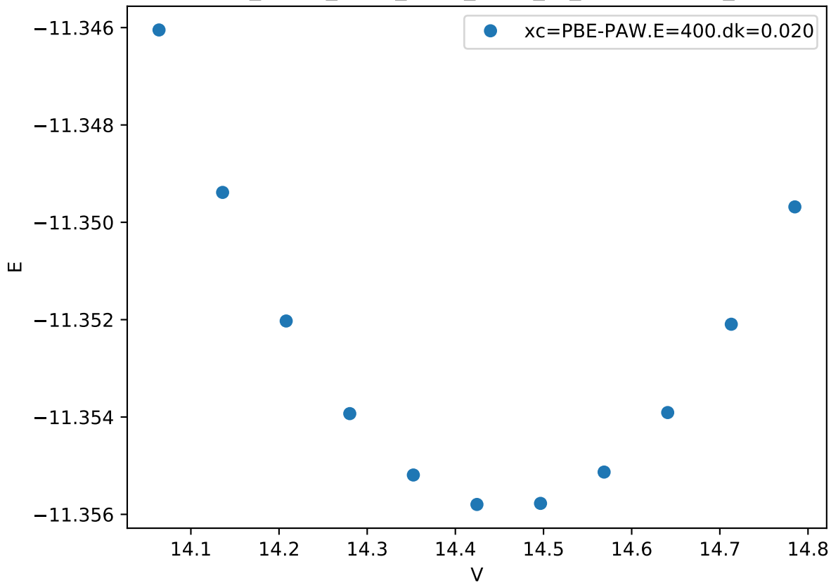
Cr_pv-Co_pv-W_sv/Cr_pv-W_sv_chi-BBBA.FM_
