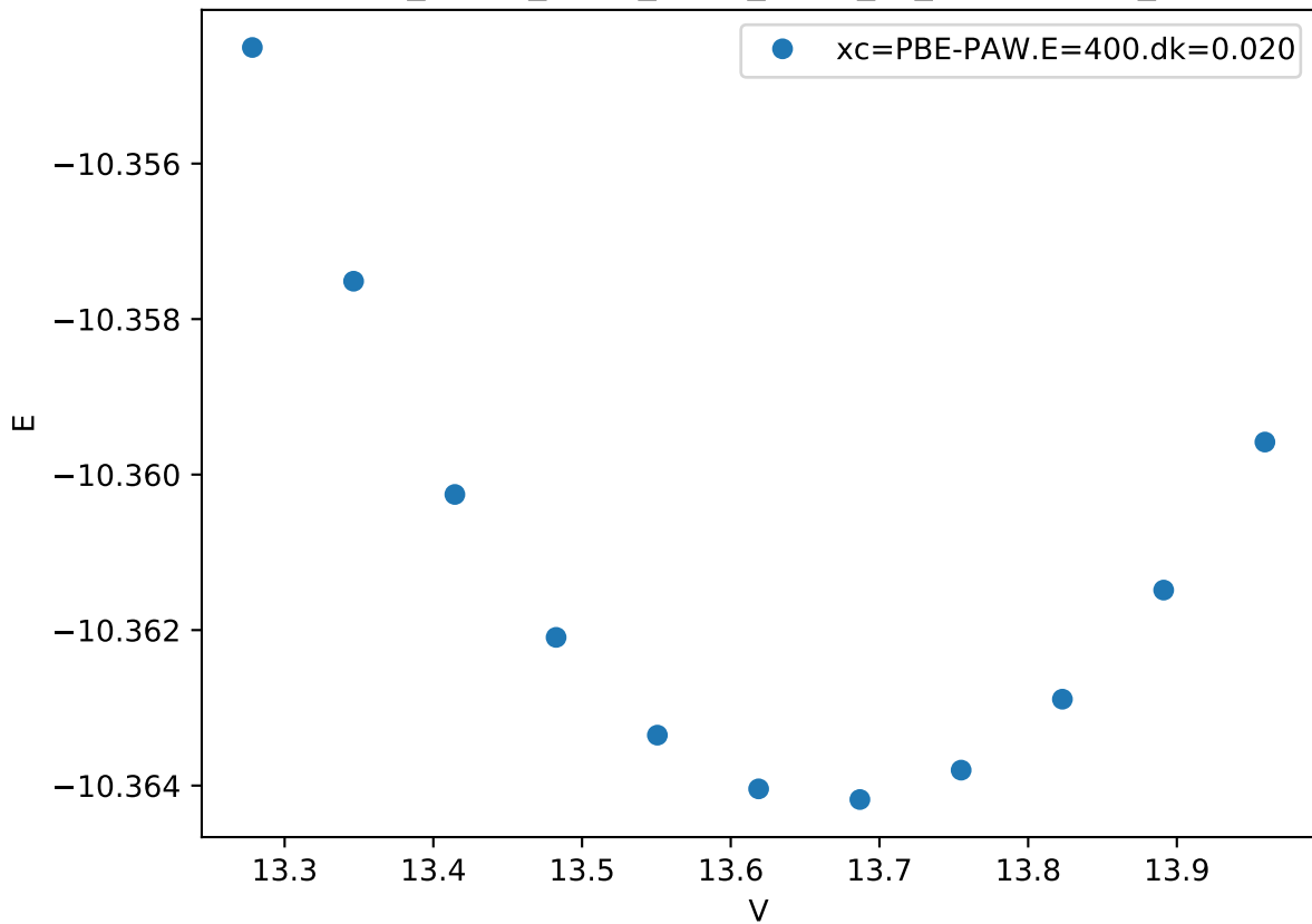
Cr_pv-Co_pv-W_sv/Cr_pv-W_sv_C36-BABAA_
