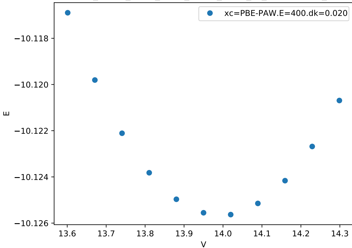
Cr_pv-Co_pv-W_sv/Cr_pv-Co_pv-W_sv_C36-CBACA_
