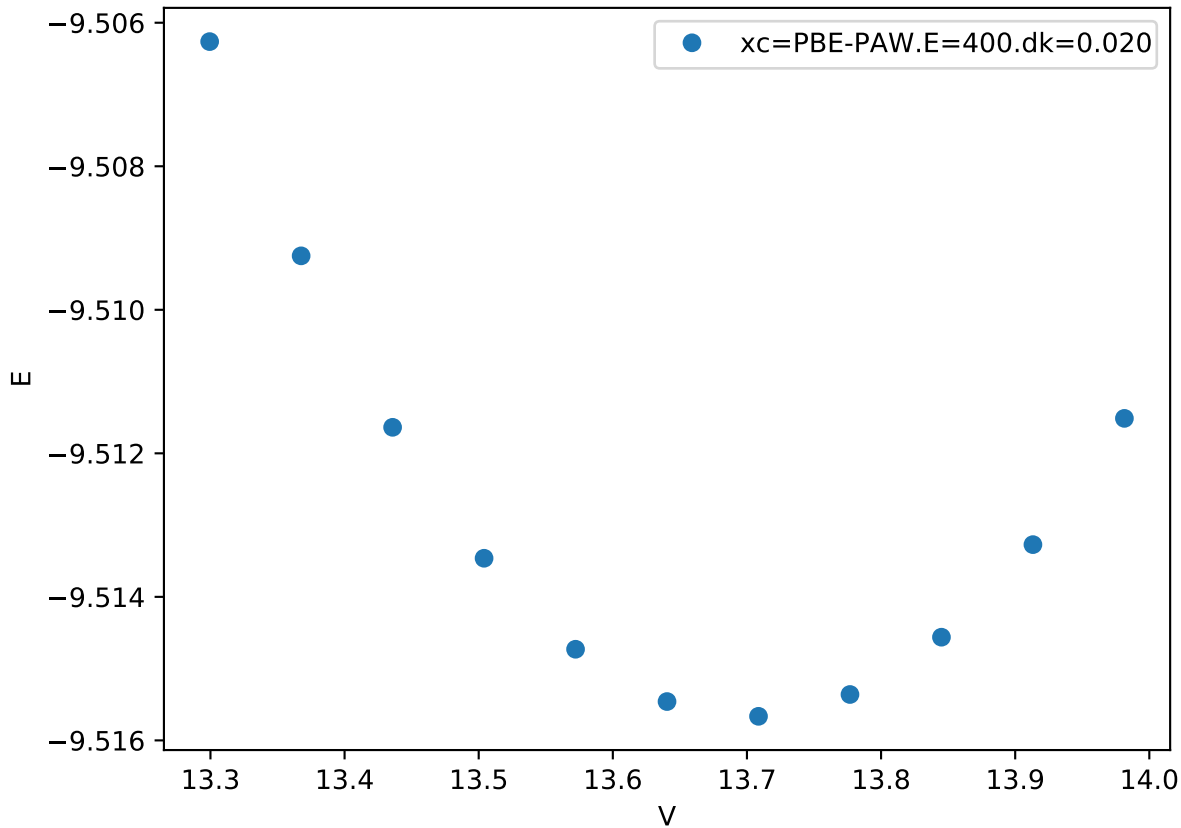
Cr_pv-Co_pv-W_sv/Cr_pv-Co_pv-W_sv_C36-BCACB.FM_
