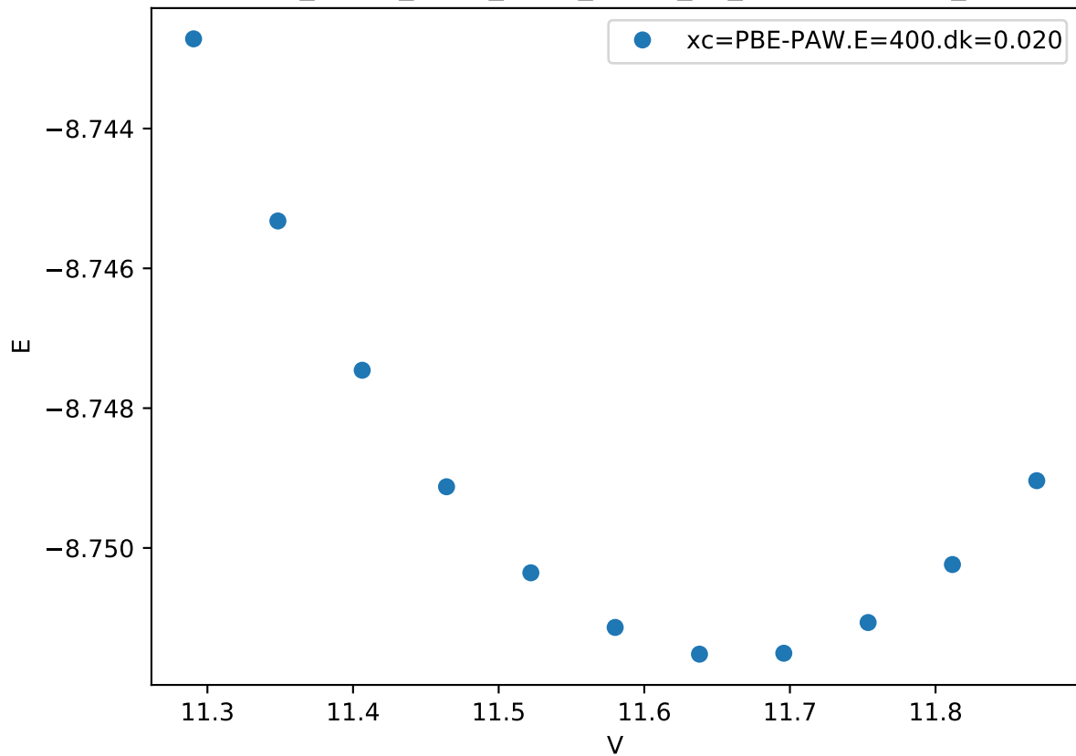
Cr_pv-Co_pv-W_sv/Cr_pv-Co_pv_mu-BAAAB.FM_
