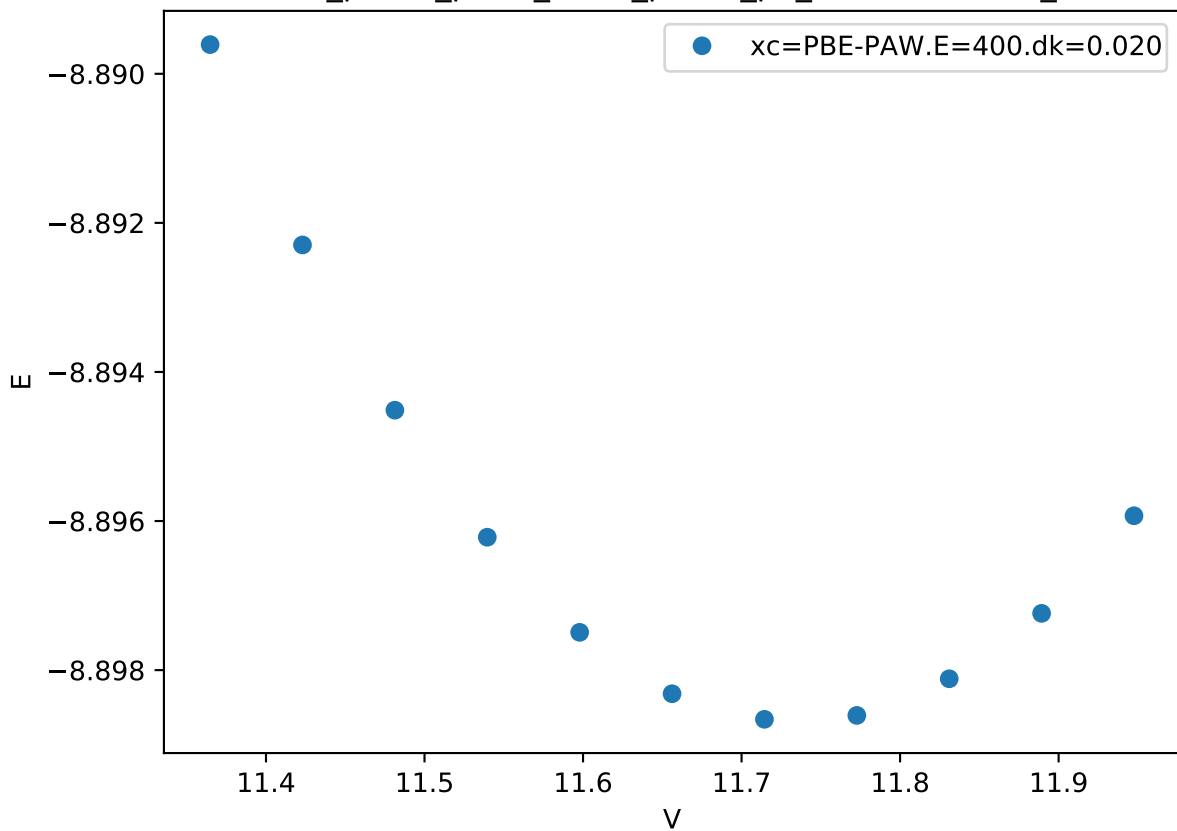
Cr_pv-Co_pv-W_sv/Cr_pv-Co_pv_mu-AAABA.FM_
