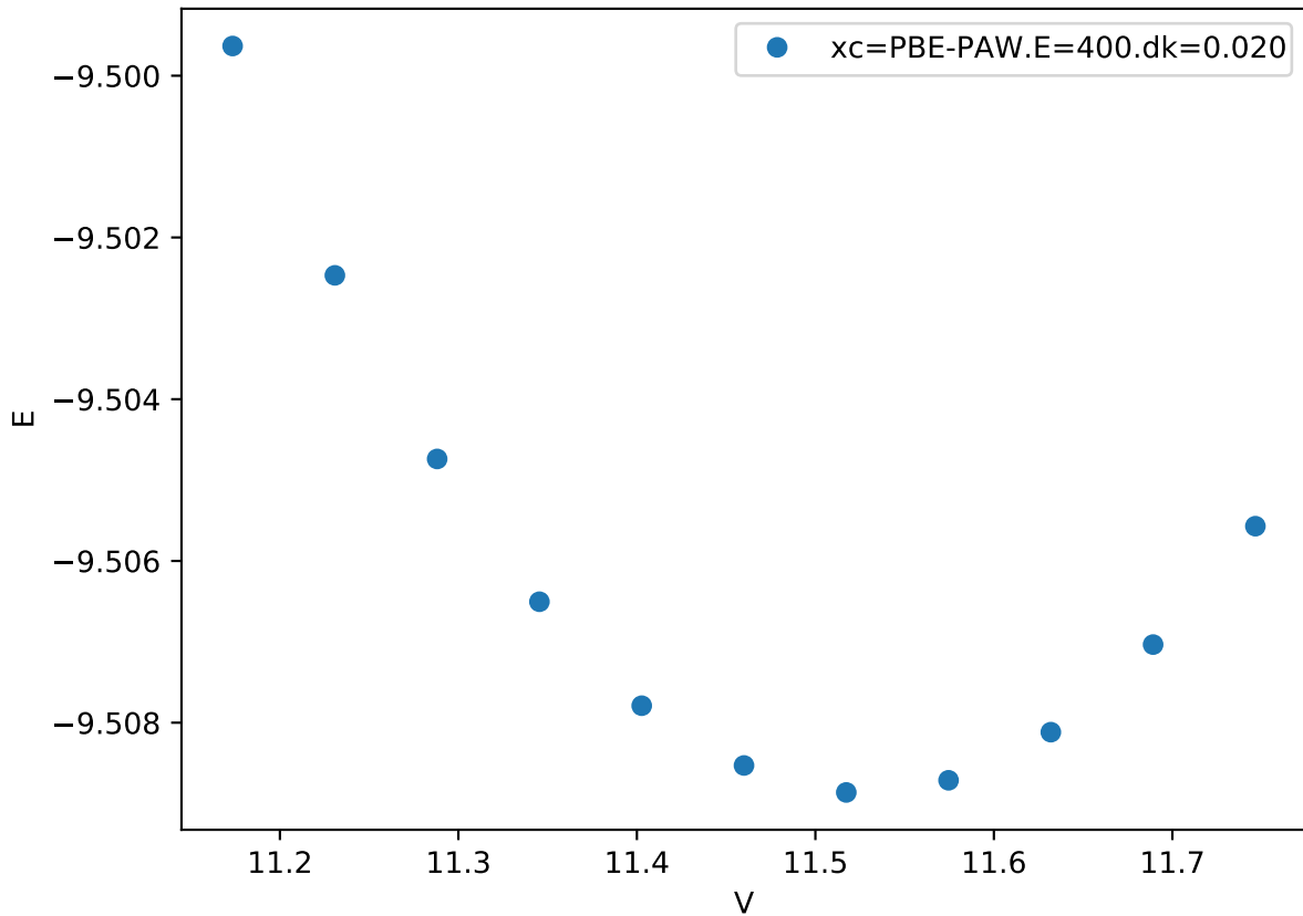
Cr_pv-Co_pv-W_sv/Cr_pv_bcc.FM_
