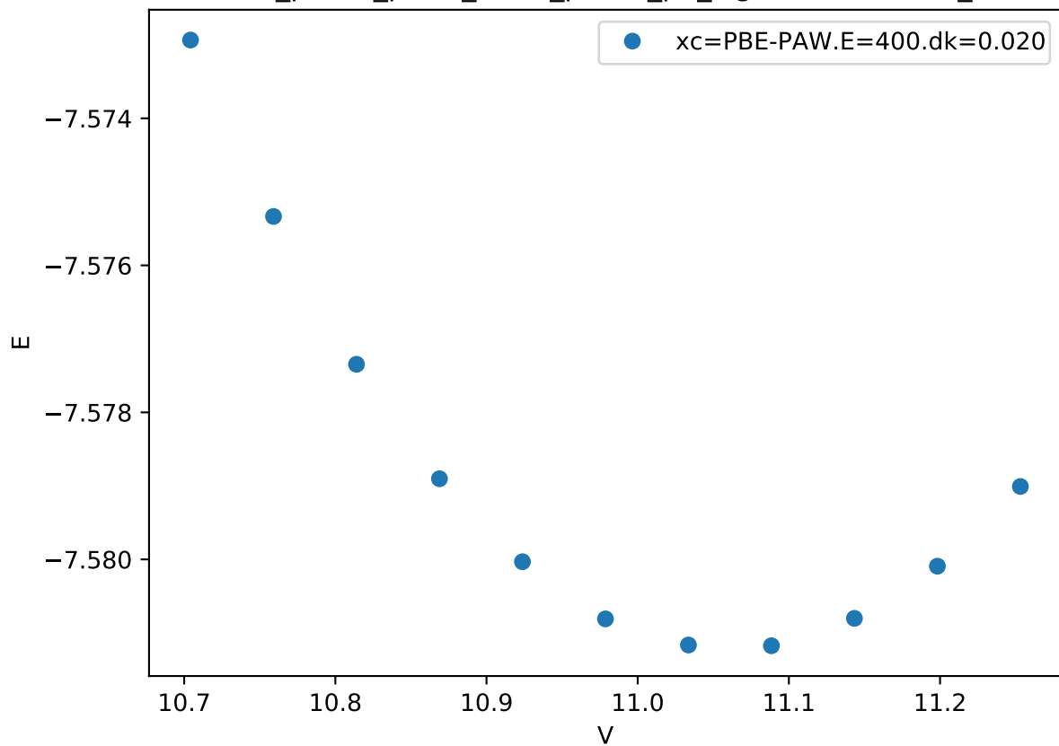
Cr_pv-Co_pv-W_sv/Cr_pv-Co_pv_sigma-BBBBA.FM_
