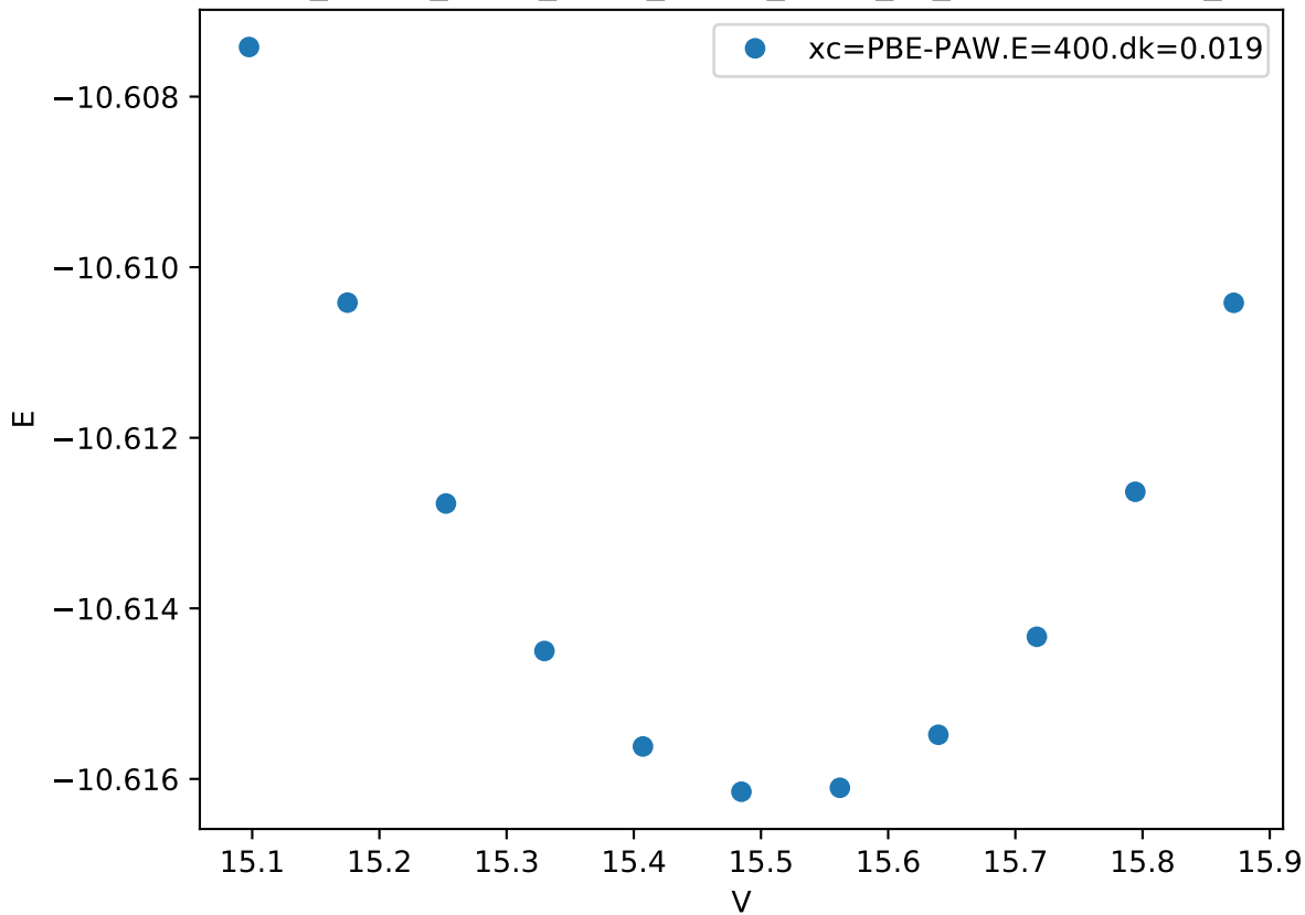
Cr_pv-Co_pv-W_sv/Cr_pv-Co_pv-W_sv_mu-ACBAC.FM_
