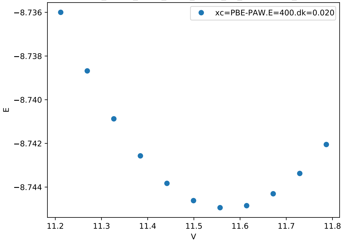
Cr_pv-Co_pv-W_sv/Cr_pv-Co_pv_mu-BAAAB_
