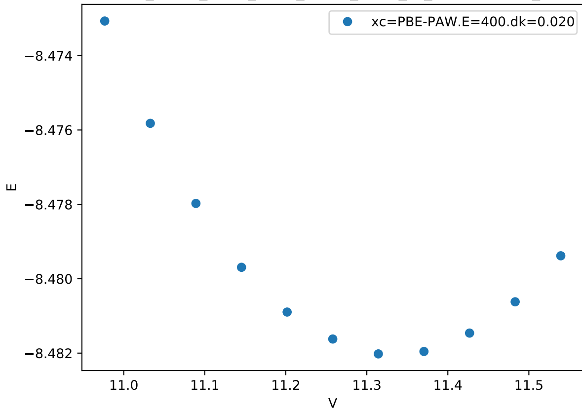
Cr_pv-Co_pv-W_sv/Cr_pv-Co_pv-W_sv_chi-CAAB.FM_
