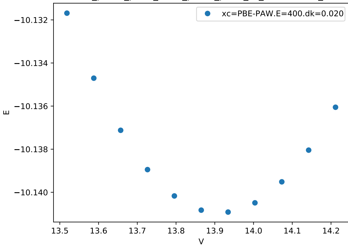
Cr_pv-Co_pv-W_sv/Cr_pv-Co_pv-W_sv_C36-CABAC_
