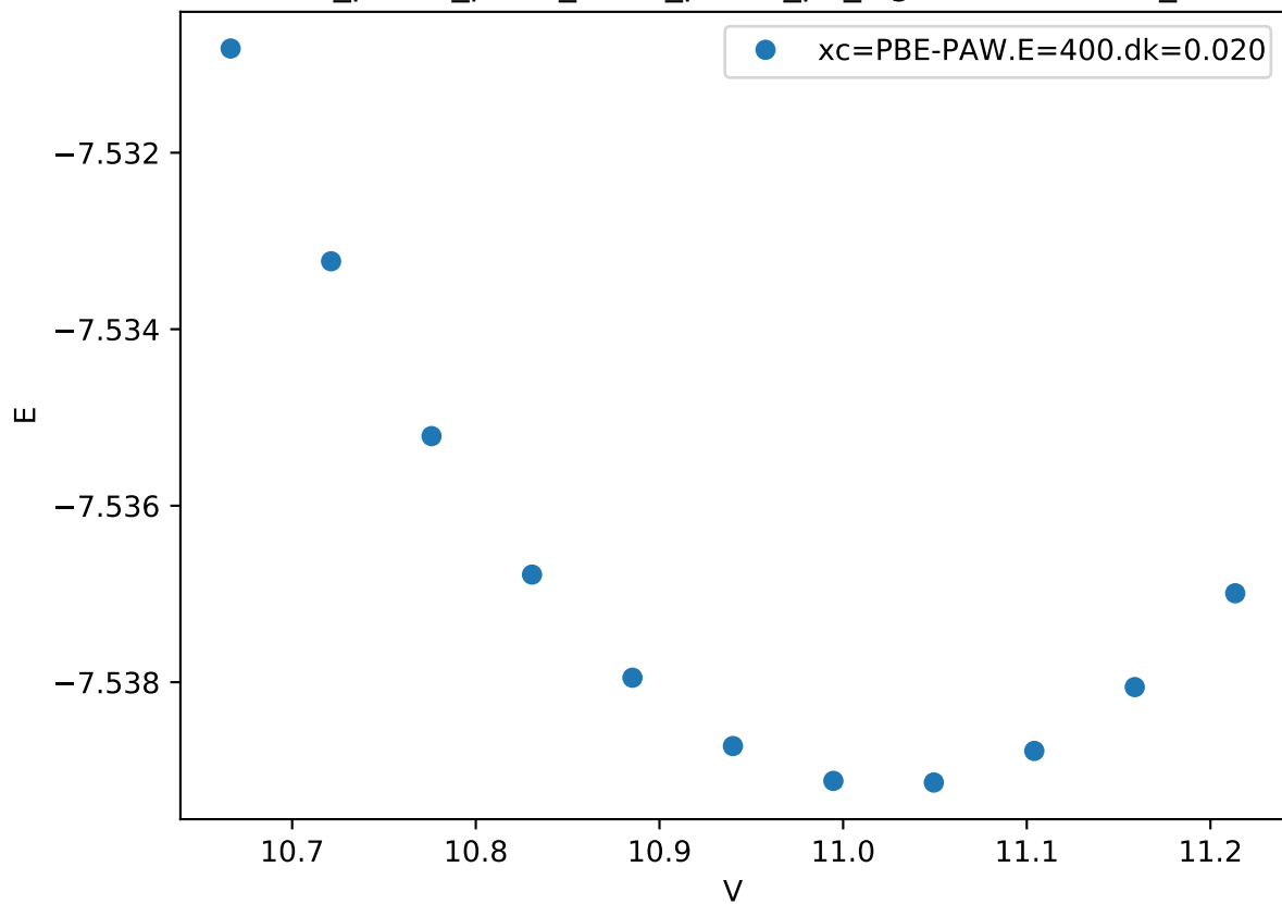
Cr_pv-Co_pv-W_sv/Cr_pv-Co_pv_sigma-BBBAB.FM_
