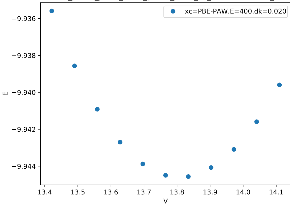
Cr_pv-Co_pv-W_sv/Cr_pv-Co_pv-W_sv_C36-ACACB.FM_
