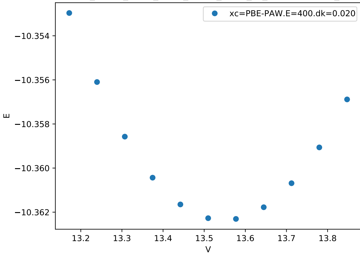
Cr_pv-Co_pv-W_sv/Cr_pv-Co_pv-W_sv_sigma-CCCBA_
