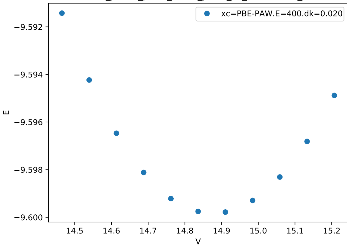
Cr_pv-Co_pv-W_sv/Co_pv-W_sv_mu-BBAAA_
