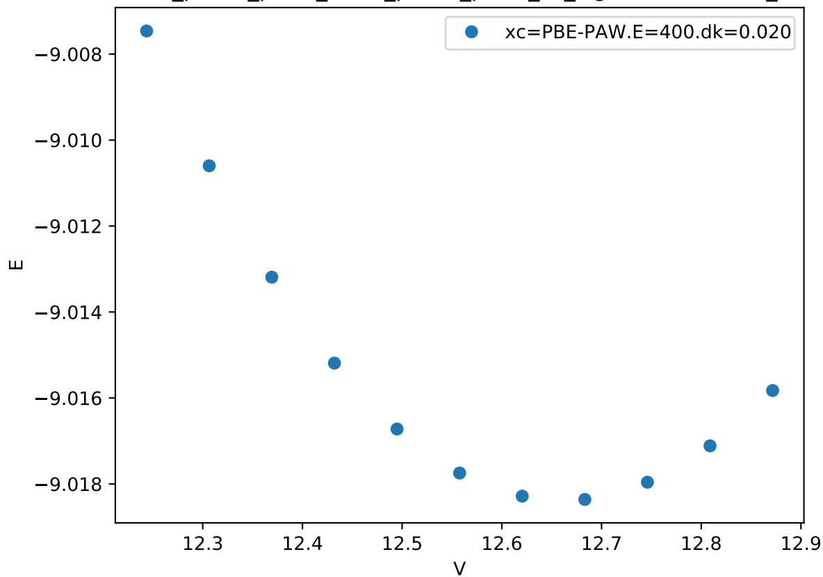
Cr_pv-Co_pv-W_sv/Cr_pv-Co_pv-W_sv_sigma-BBBAC.FM_
