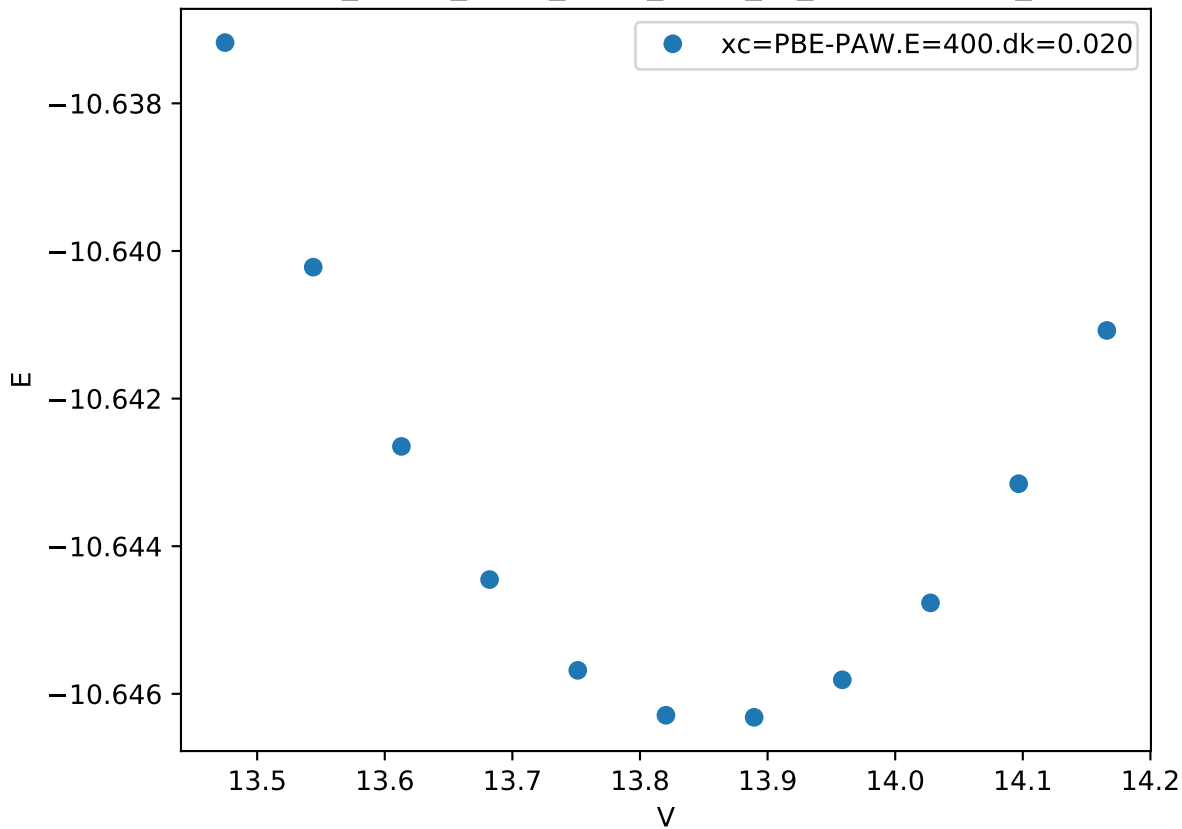
Cr_pv-Co_pv-W_sv/Cr_pv-W_sv_chi-AABA.FM_
