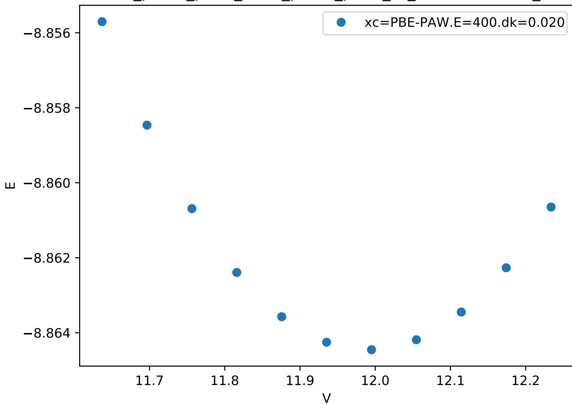
Cr_pv-Co_pv-W_sv/Cr_pv-Co_pv-W_sv_C36-CBABA.FM_
