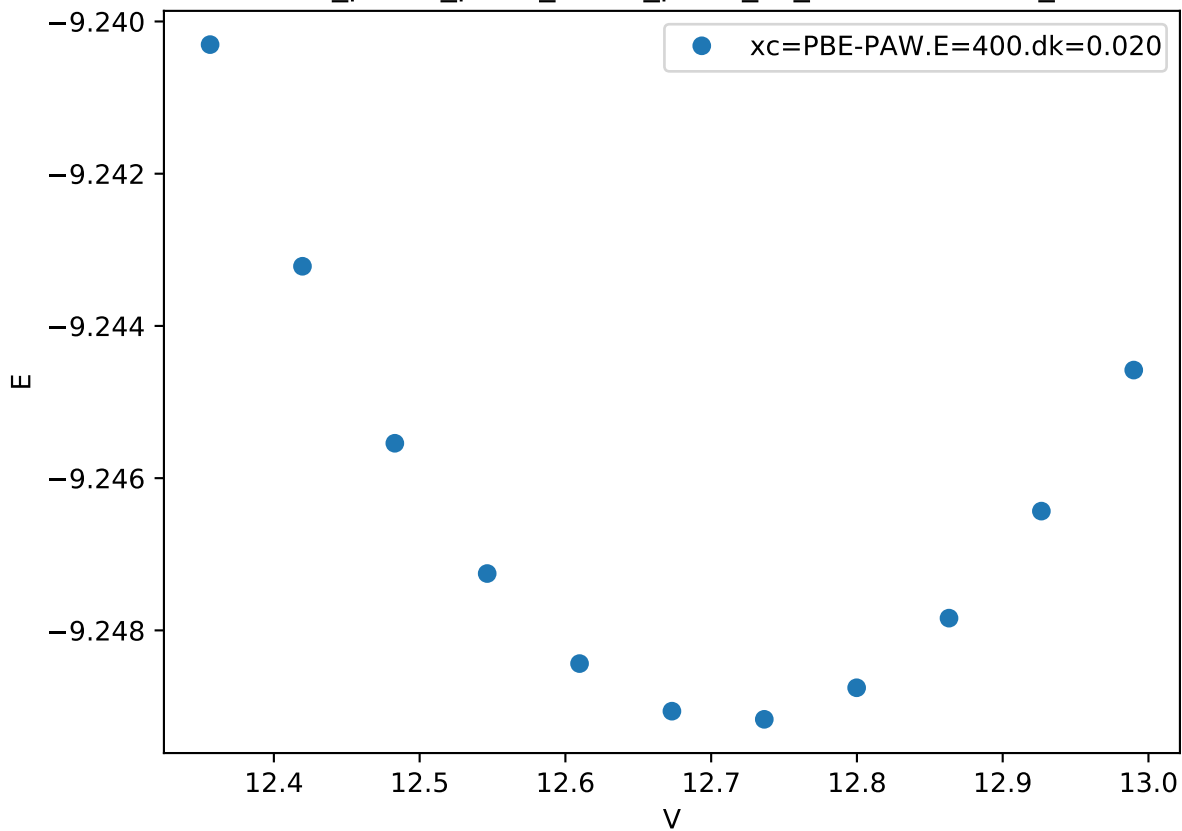
Cr_pv-Co_pv-W_sv/Co_pv-W_sv_mu-BABBA.FM_
