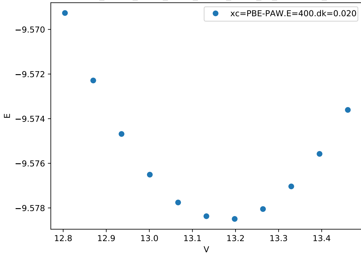
Cr_pv-Co_pv-W_sv/Cr_pv-Co_pv-W_sv_chi-BACB_
