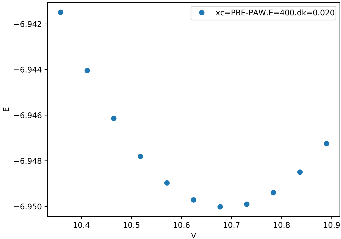
Cr_pv-Co_pv-W_sv/Co_pv-W_sv_chi-BAAA_
