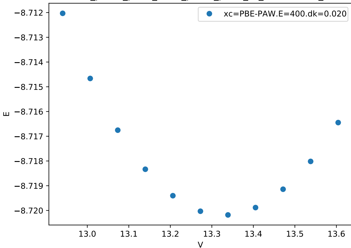
Cr_pv-Co_pv-W_sv/Cr_pv-Co_pv-W_sv_C36-ABABC_
