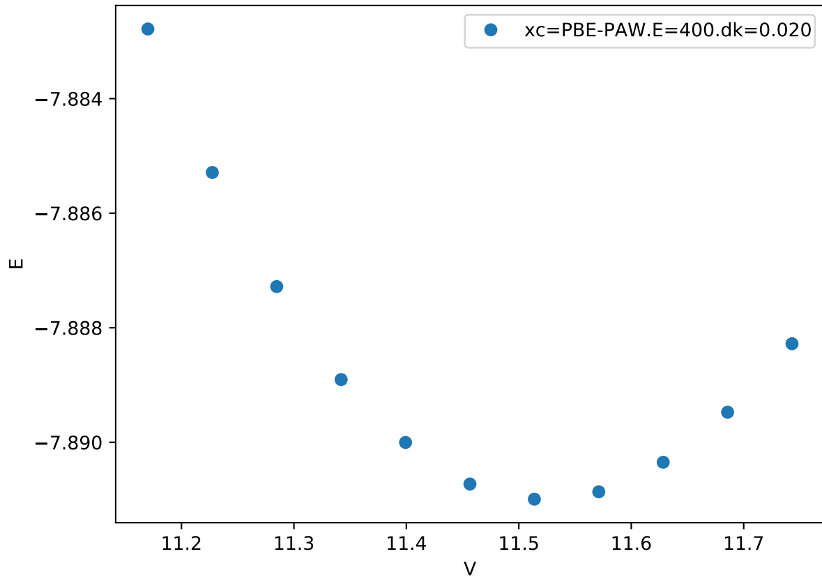
Cr_pv-Co_pv-W_sv/Cr_pv-Co_pv-W_sv_chi-ACBB.FM_
