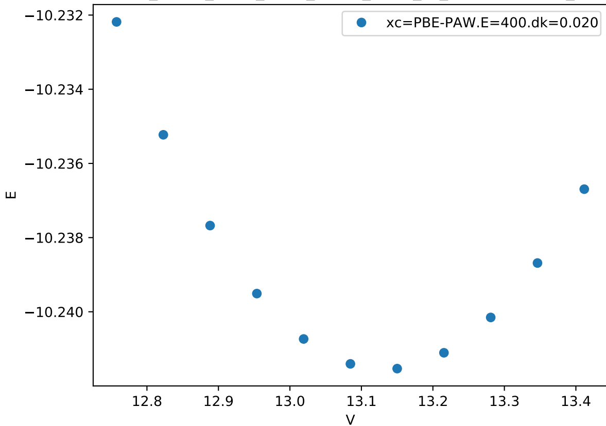
Cr_pv-Co_pv-W_sv/Cr_pv-Co_pv-W_sv_mu-BACAC.FM_
