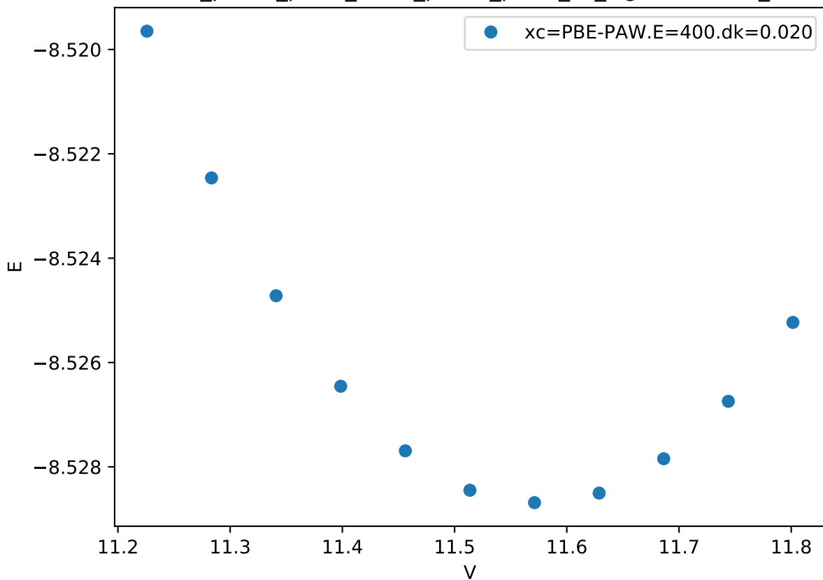
Cr_pv-Co_pv-W_sv/Cr_pv-Co_pv-W_sv_sigma-ACABB_
