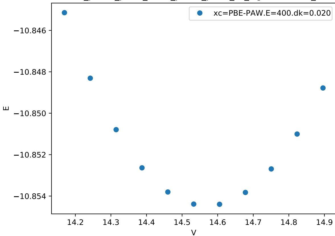
Cr_pv-Co_pv-W_sv/Cr_pv-Co_pv-W_sv_sigma-BAACC_
