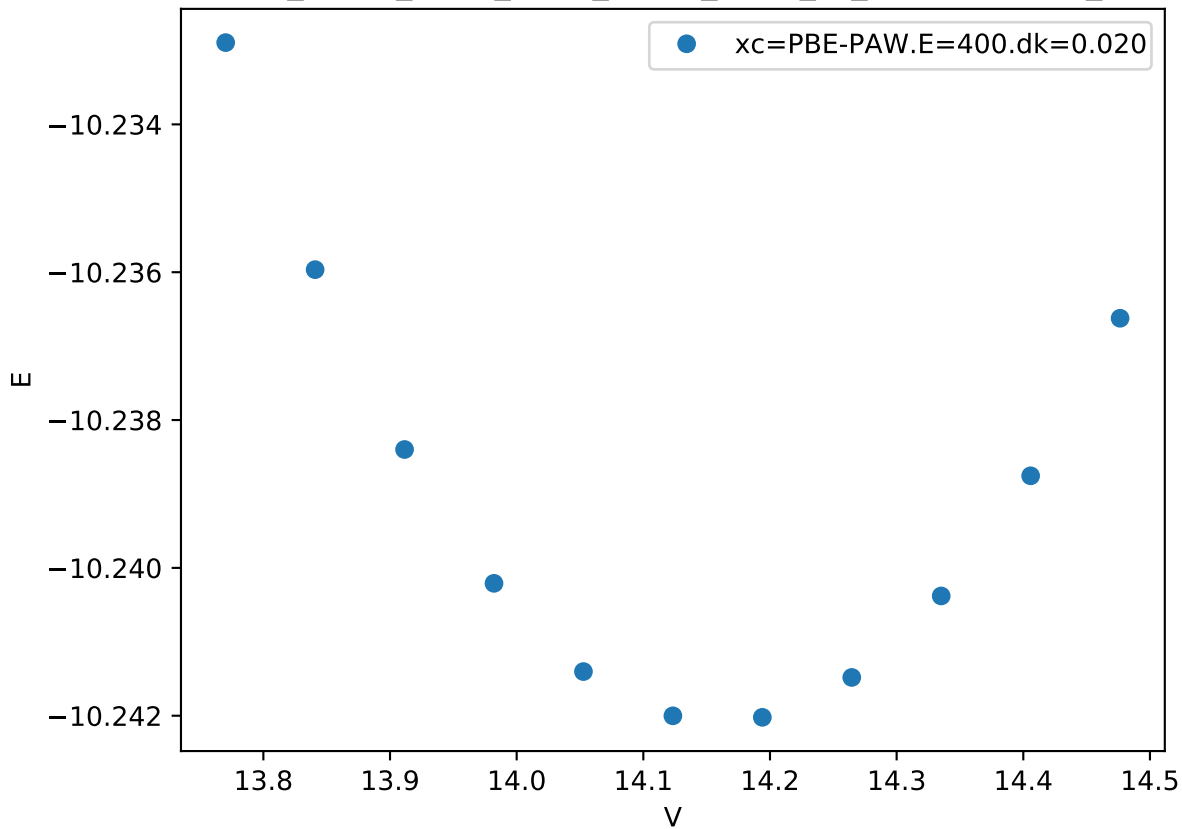
Cr_pv-Co_pv-W_sv/Cr_pv-Co_pv-W_sv_sigma-BABCC_
