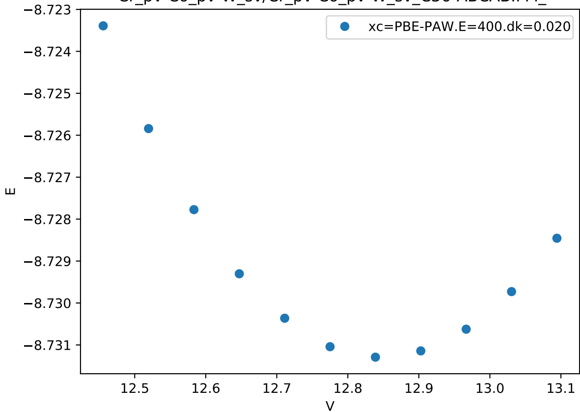
Cr_pv-Co_pv-W_sv/Cr_pv-Co_pv-W_sv_C36-ABCAB.FM_
