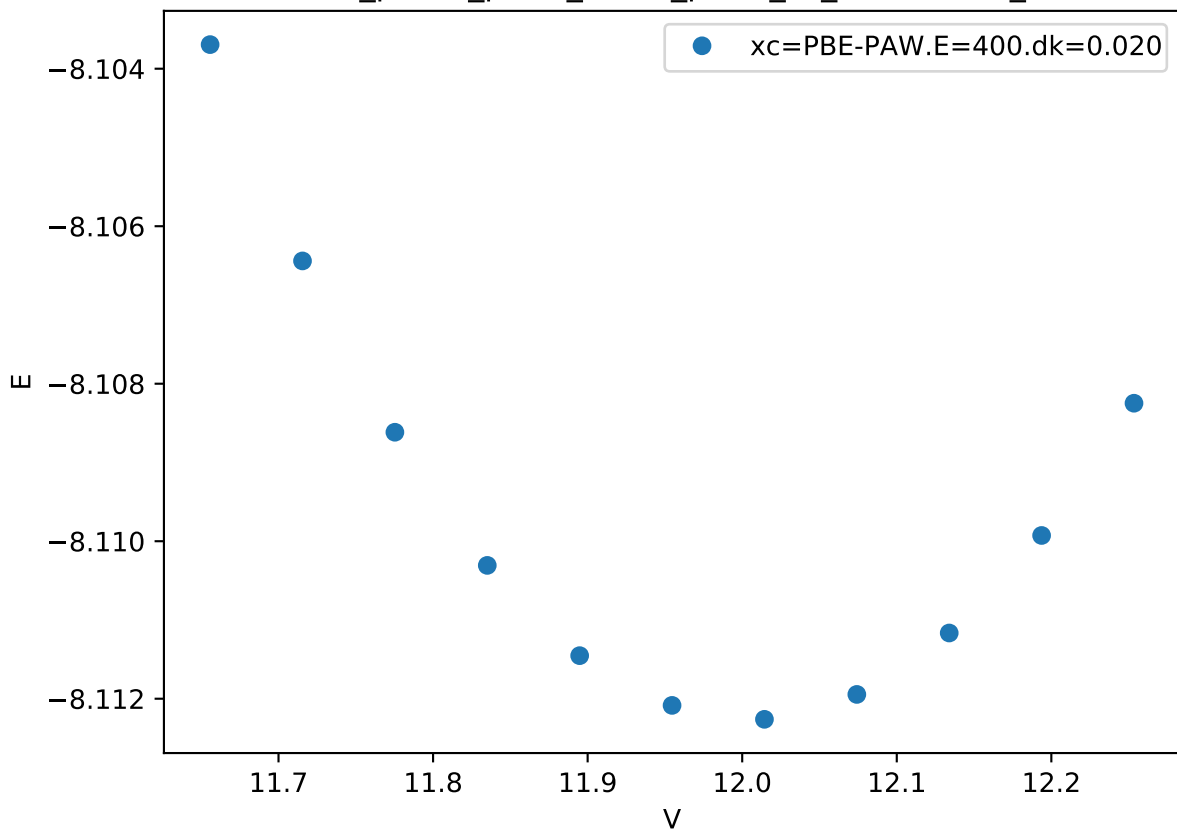
Cr_pv-Co_pv-W_sv/Co_pv-W_sv_mu-BAABA_
