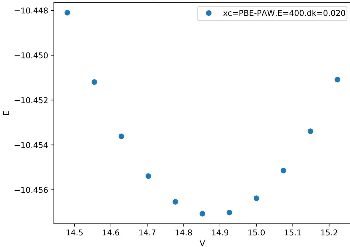
Cr_pv-Co_pv-W_sv/Cr_pv-Co_pv-W_sv_mu-ACBCB.FM_
