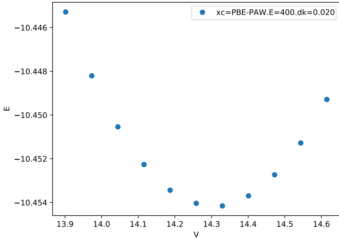
Cr_pv-Co_pv-W_sv/Cr_pv-W_sv_chi-AAAB.FM_
