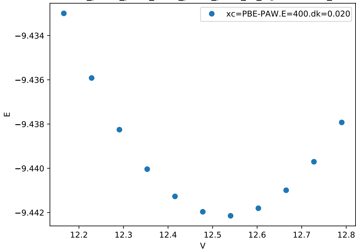
Cr_pv-Co_pv-W_sv/Cr_pv-Co_pv-W_sv_sigma-BACAB_
