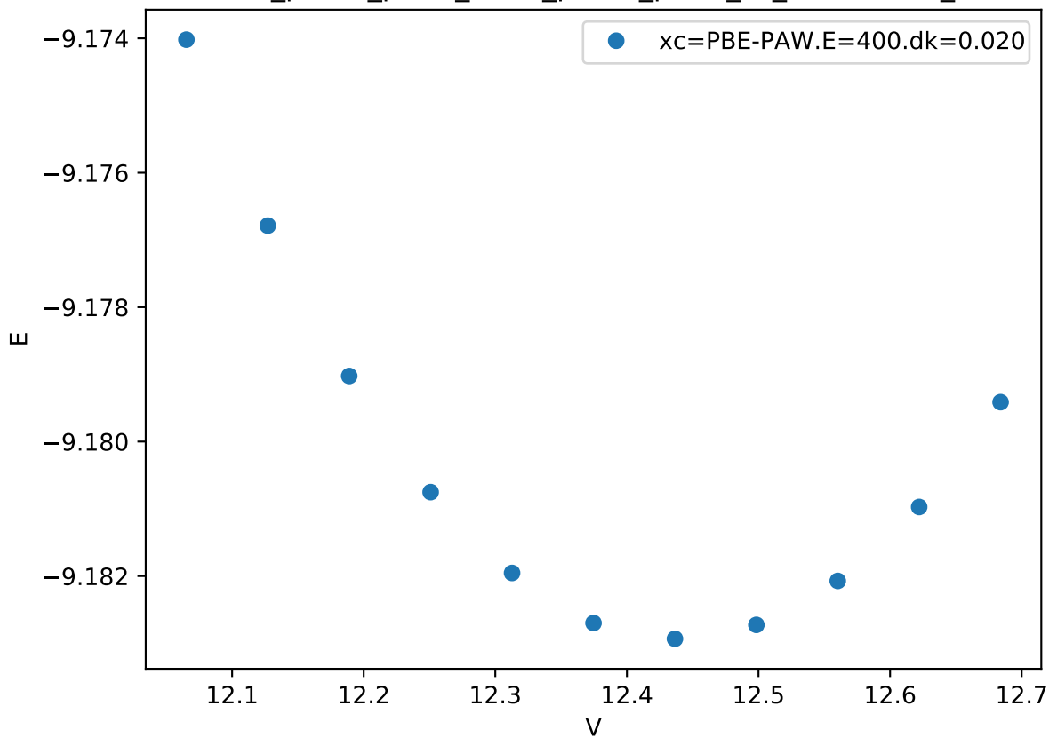
Cr_pv-Co_pv-W_sv/Cr_pv-Co_pv-W_sv_mu-BABAC_
