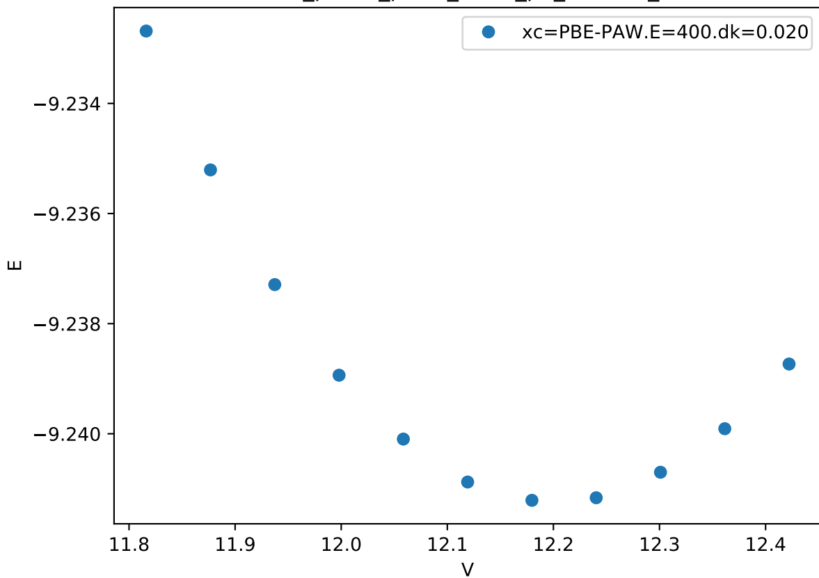
Cr_pv-Co_pv-W_sv/Cr_pv_C14.FM_
