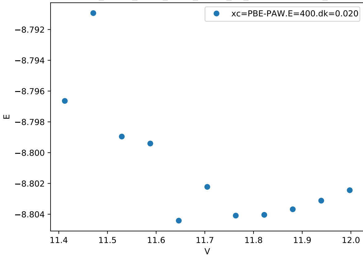
Cr_pv-Co_pv-W_sv/Cr_pv-Co_pv_C36-BAAAA.FM_
