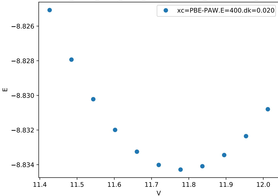
Cr_pv-Co_pv-W_sv/Cr_pv-Co_pv-W_sv_chi-ACBA.FM_
