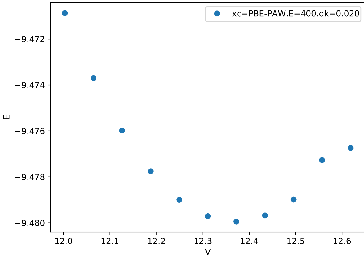
Cr_pv-Co_pv-W_sv/Cr_pv-Co_pv-W_sv_C36-BCAAA.FM_
