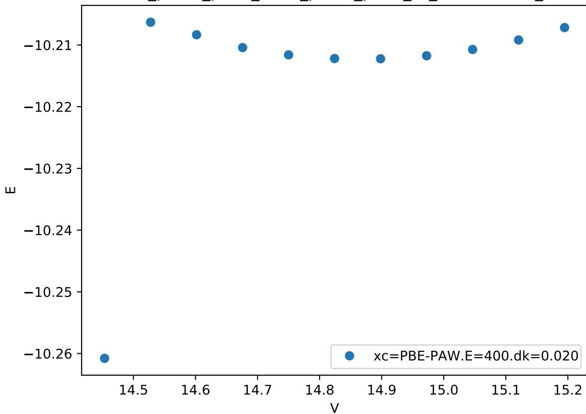
Cr_pv-Co_pv-W_sv/Cr_pv-Co_pv-W_sv_C14-BCA.FM_
