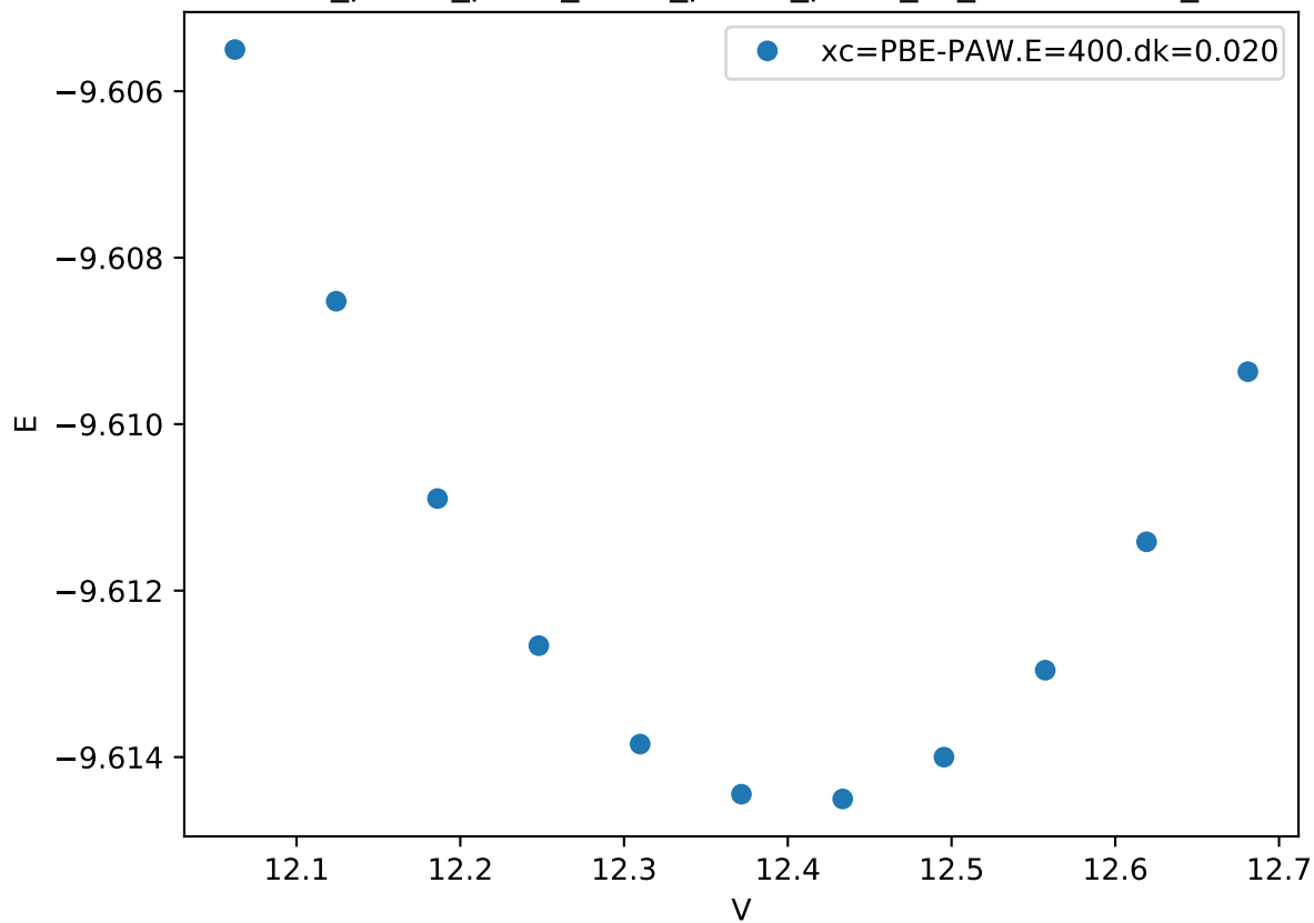
Cr_pv-Co_pv-W_sv/Cr_pv-Co_pv-W_sv_C36-CCBAB_
