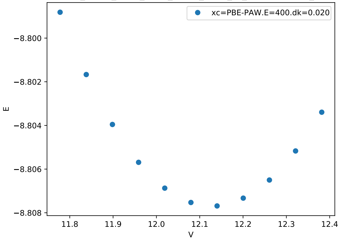
Cr_pv-Co_pv-W_sv/Cr_pv-Co_pv-W_sv_sigma-BACBB_
