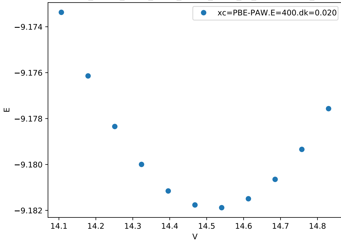
Cr_pv-Co_pv-W_sv/Cr_pv-Co_pv-W_sv_C36-BACBC_
