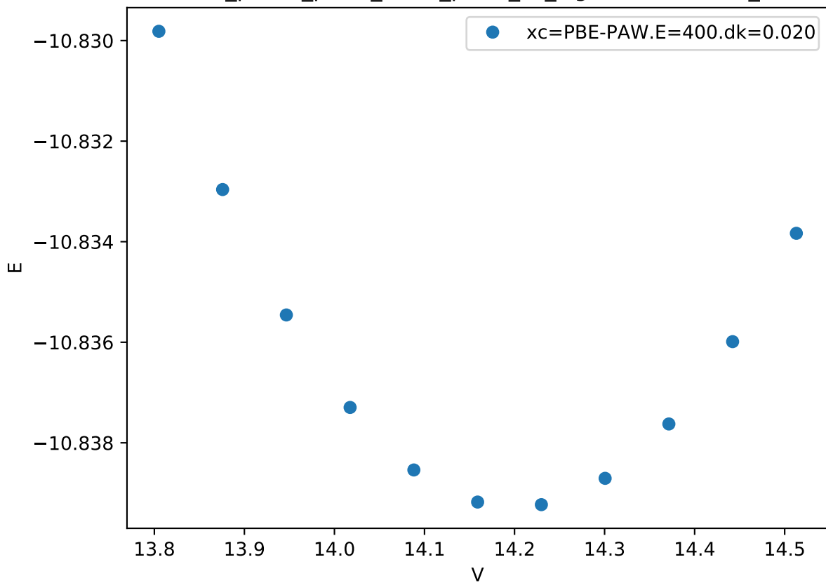
Cr_pv-Co_pv-W_sv/Cr_pv-W_sv_sigma-BBABA.FM_
