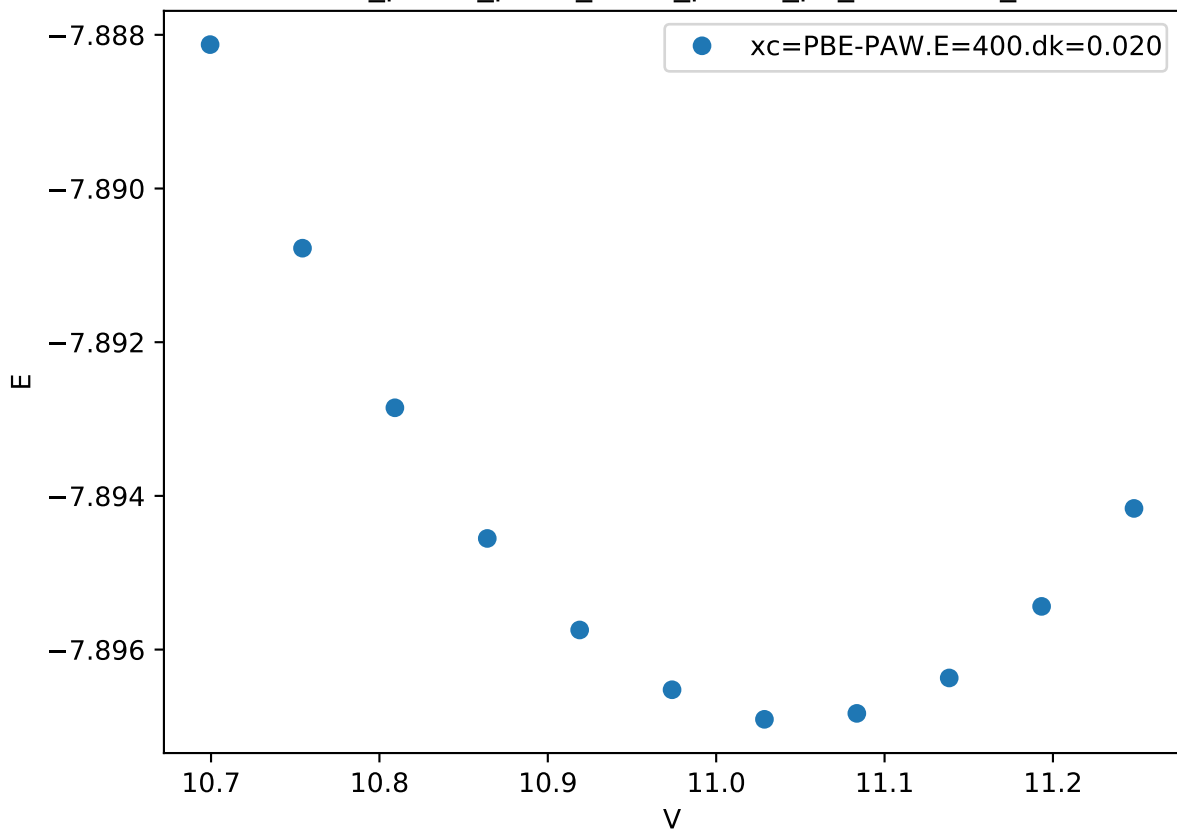
Cr_pv-Co_pv-W_sv/Cr_pv-Co_pv_chi-BBBA_
