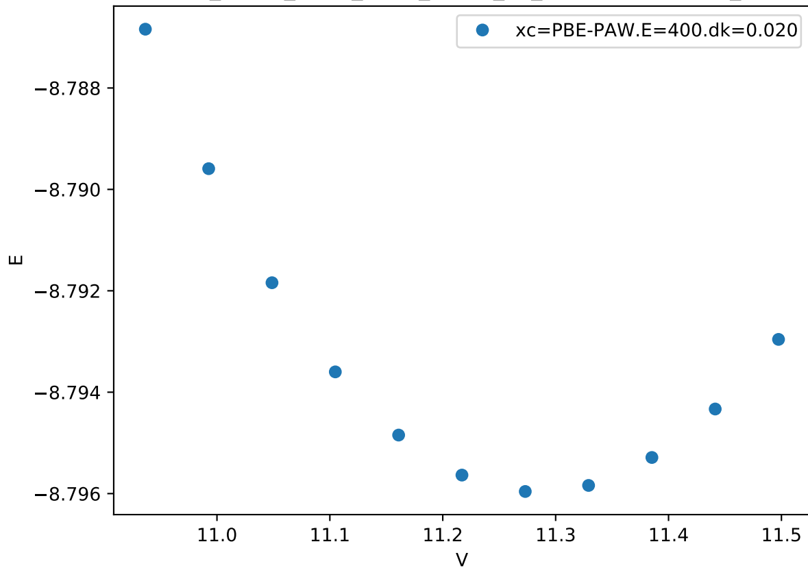
Cr_pv-Co_pv-W_sv/Cr_pv-Co_pv_sigma-AAABA.FM_
