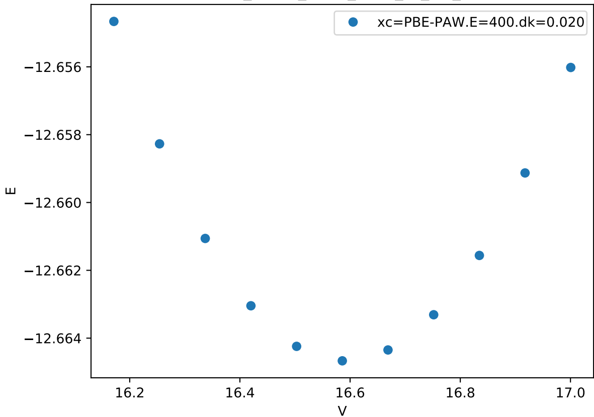
Cr_pv-Co_pv-W_sv/W_sv_chi_
