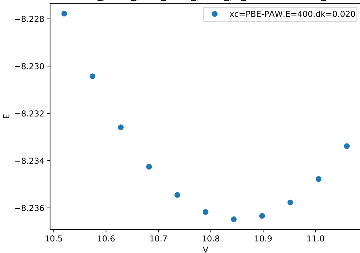
Cr_pv-Co_pv-W_sv/Cr_pv-Co_pv_L10-NiAl-AB.FM_
