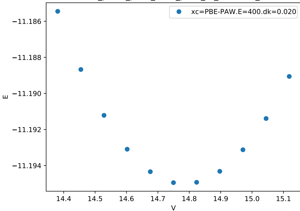
Cr_pv-Co_pv-W_sv/Cr_pv-W_sv_chi-BBAB_
