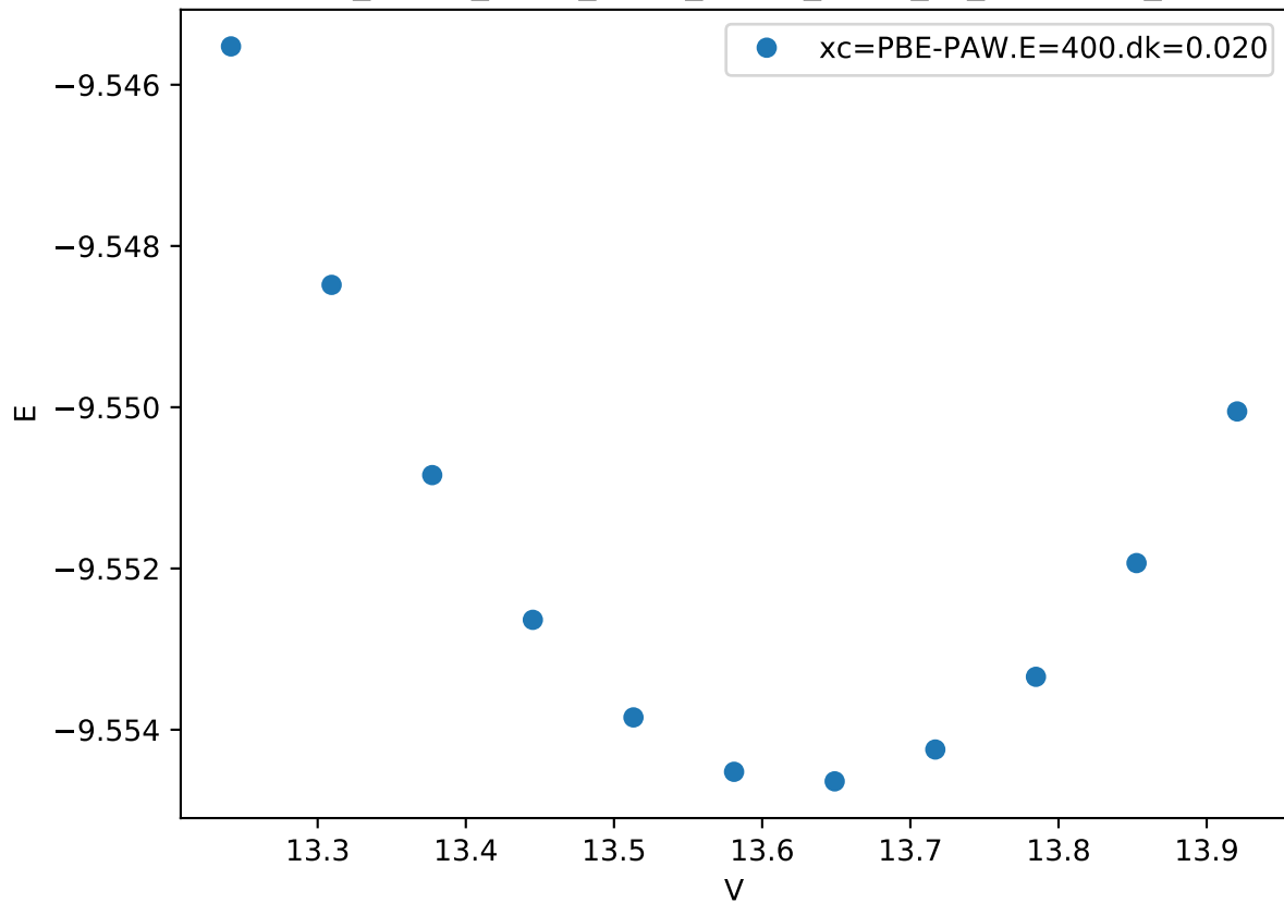
Cr_pv-Co_pv-W_sv/Cr_pv-Co_pv-W_sv_chi-AABC_
