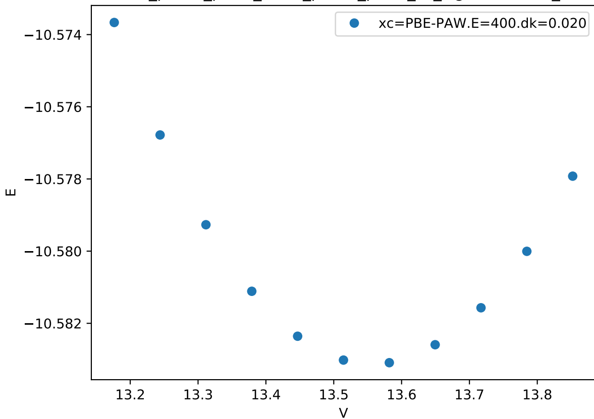
Cr_pv-Co_pv-W_sv/Cr_pv-Co_pv-W_sv_sigma-BCAAC_
