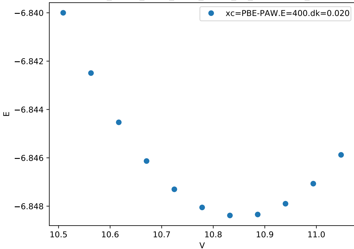
Cr_pv-Co_pv-W_sv/Cr_pv-Co_pv_mu-ABBBB_
