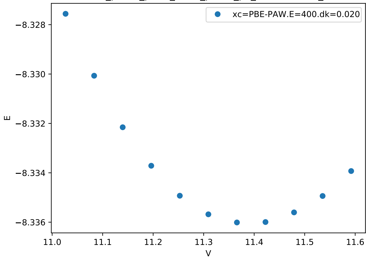
Cr_pv-Co_pv-W_sv/Cr_pv-Co_pv_chi-AABA.FM_
