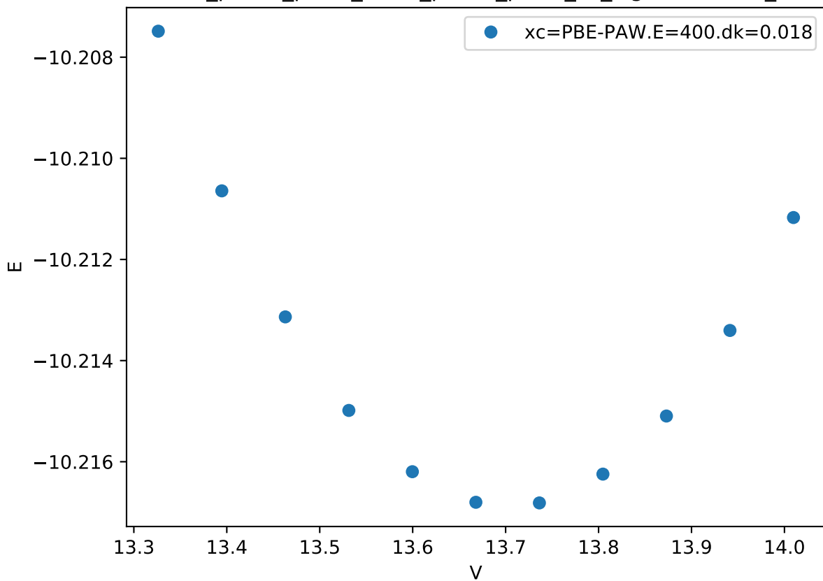
Cr_pv-Co_pv-W_sv/Cr_pv-Co_pv-W_sv_sigma-ABCBC_
