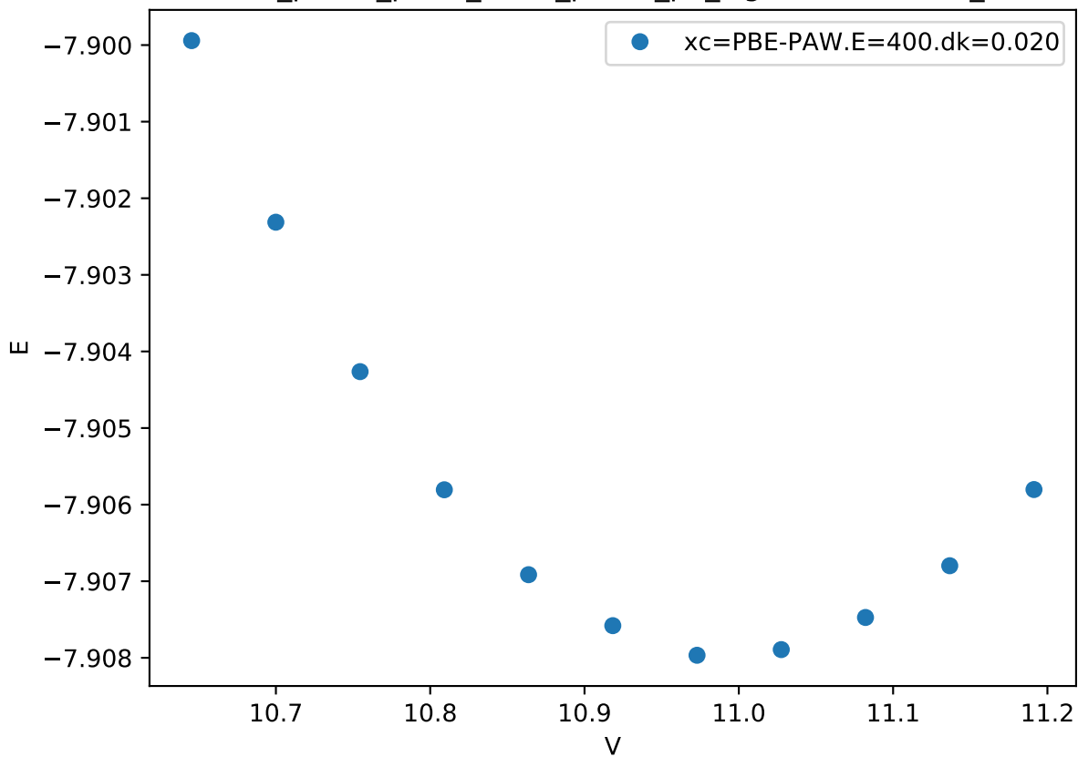
Cr_pv-Co_pv-W_sv/Cr_pv-Co_pv_sigma-BAABB.FM_
