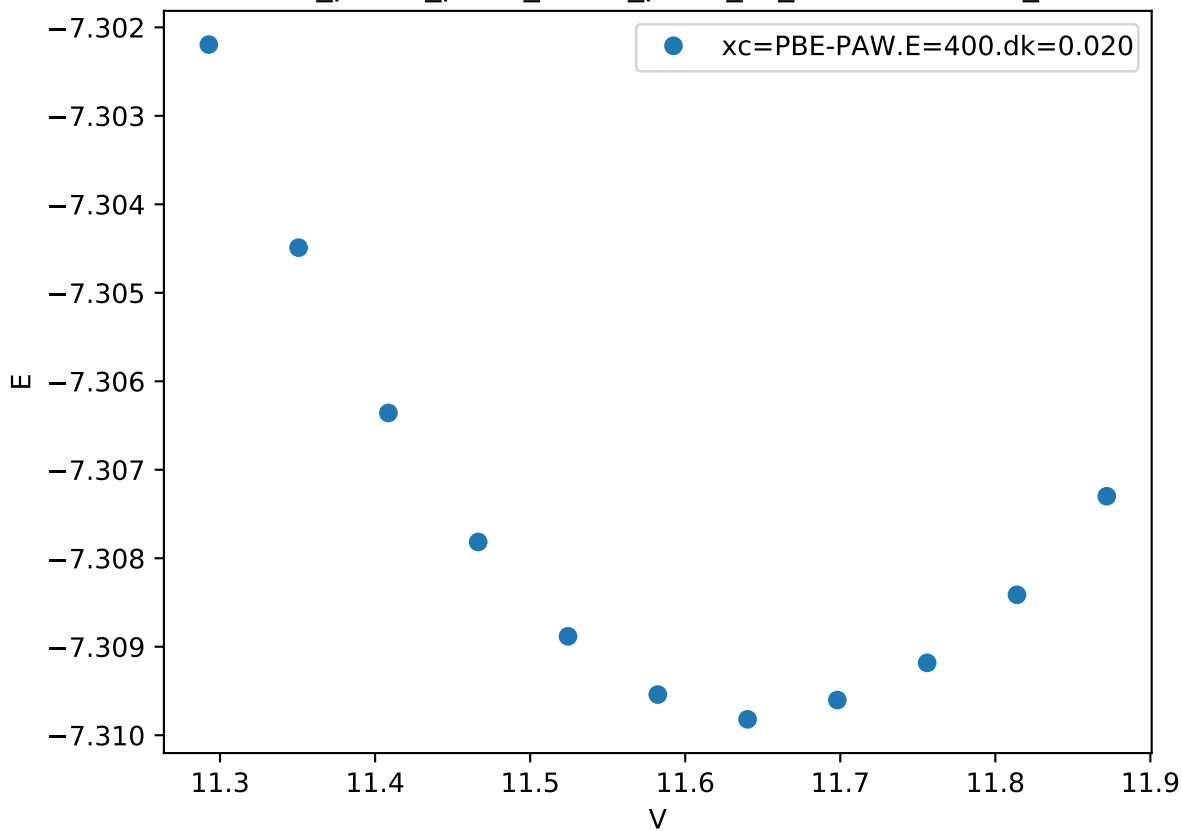
Cr_pv-Co_pv-W_sv/Co_pv-W_sv_mu-BAAAA.FM_
