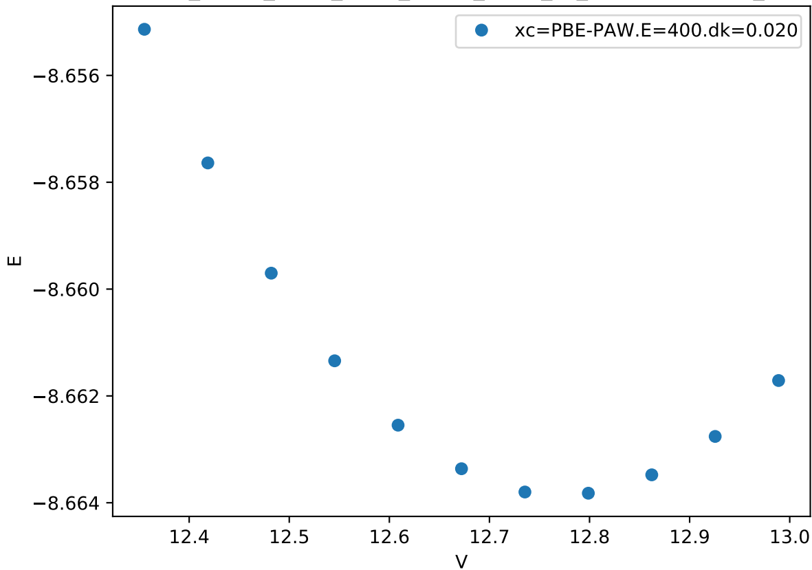
Cr_pv-Co_pv-W_sv/Cr_pv-Co_pv-W_sv_C36-ABCBA.FM_
