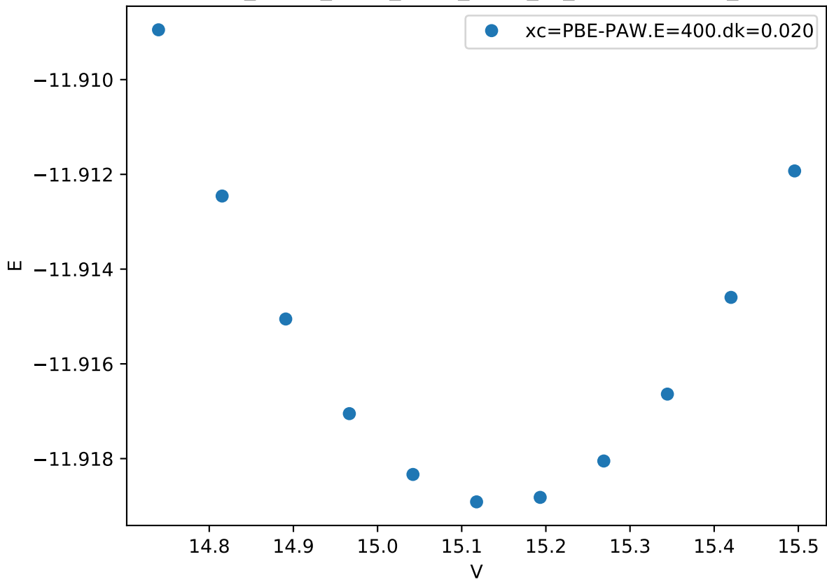
Cr_pv-Co_pv-W_sv/Cr_pv-W_sv_sigma-BBBAB_
