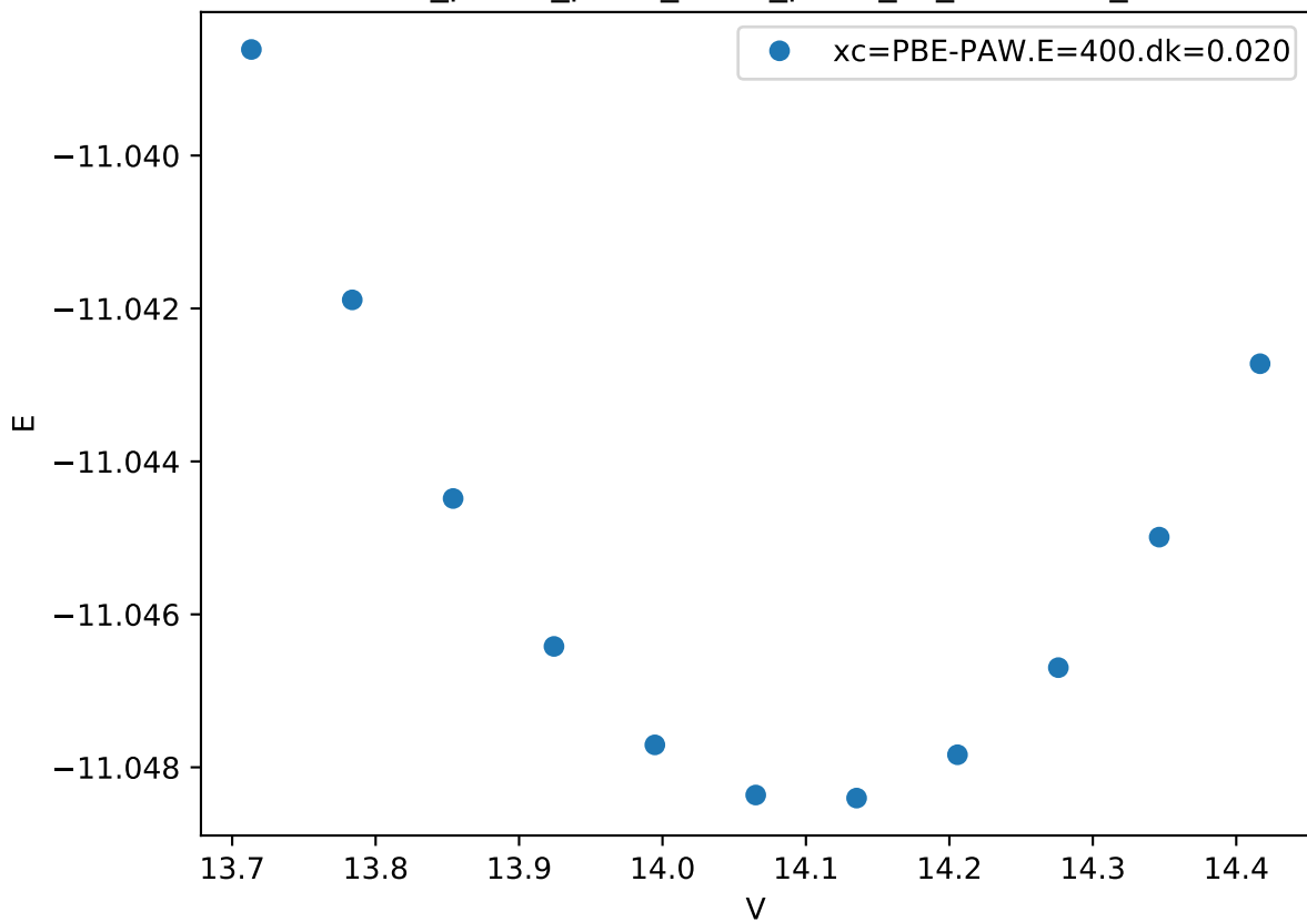
Cr_pv-Co_pv-W_sv/Cr_pv-W_sv_C14-BBA_
