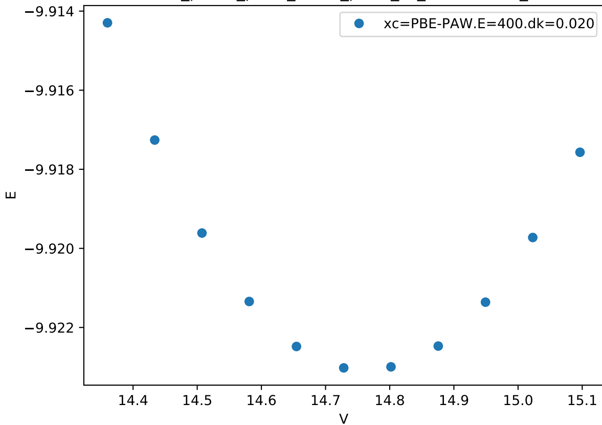
Cr_pv-Co_pv-W_sv/Co_pv-W_sv_C36-BABAB_
