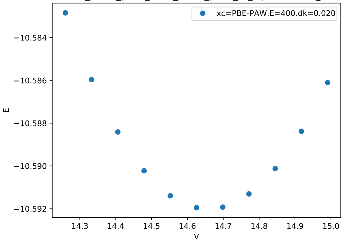
Cr_pv-Co_pv-W_sv/Cr_pv-Co_pv-W_sv_sigma-CABCC_
