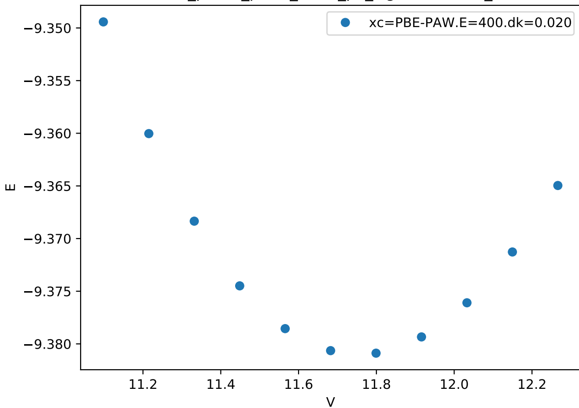
Cr_pv-Co_pv-W_sv/Cr_pv_sigma.DUDUU_
