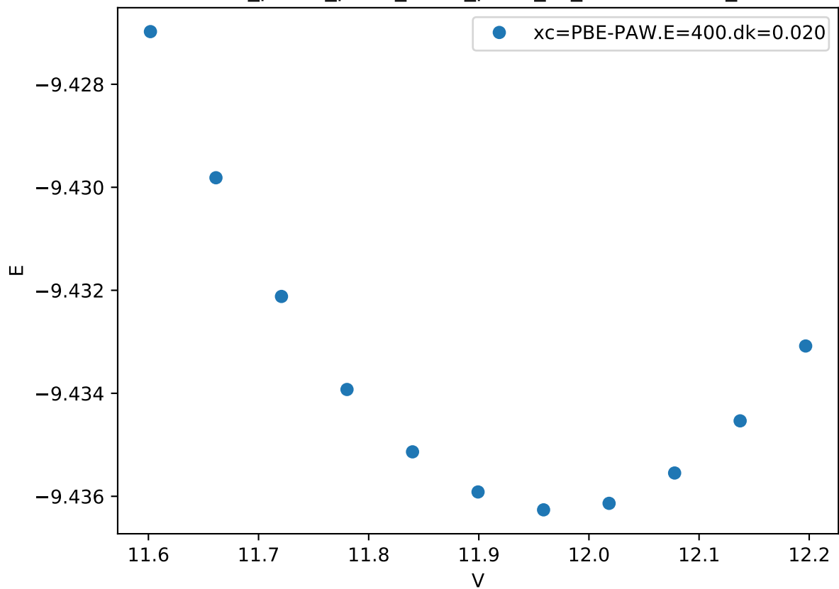
Cr_pv-Co_pv-W_sv/Cr_pv-W_sv_chi-BAAA.FM_
