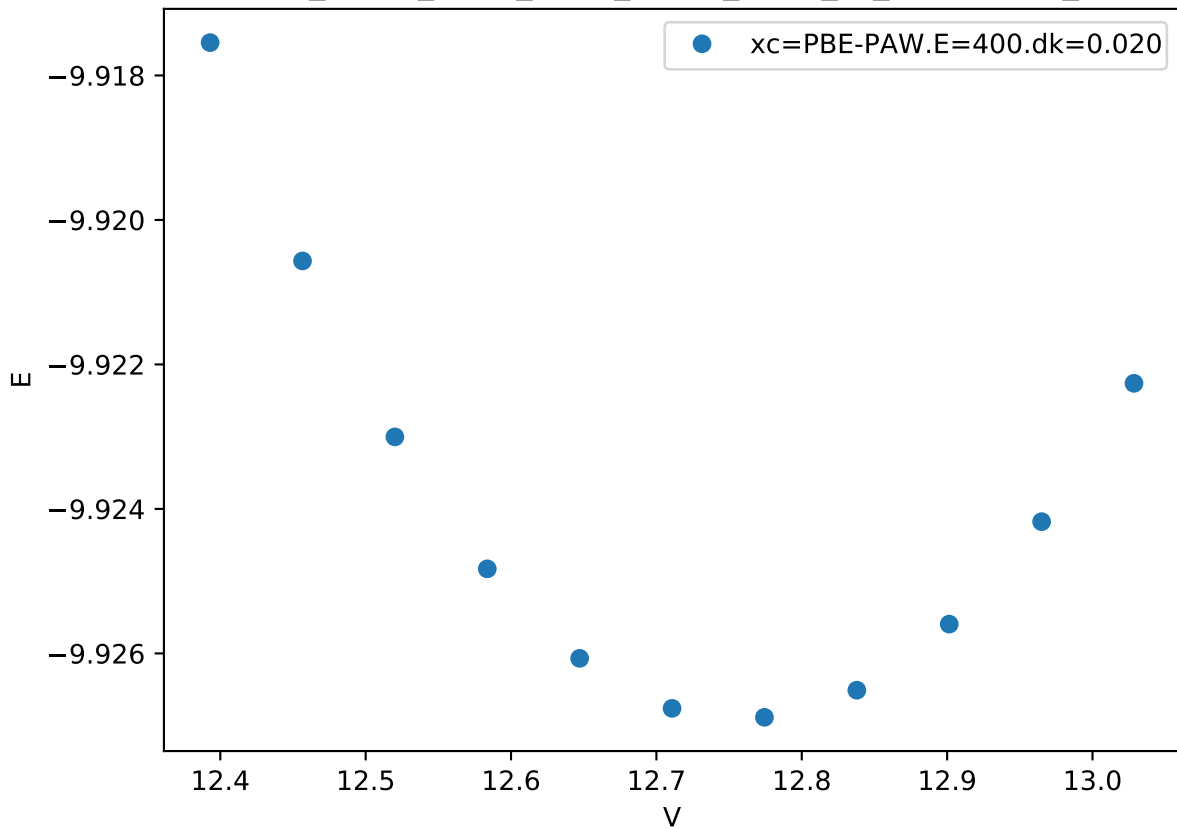
Cr_pv-Co_pv-W_sv/Cr_pv-Co_pv-W_sv_mu-BACCB_
