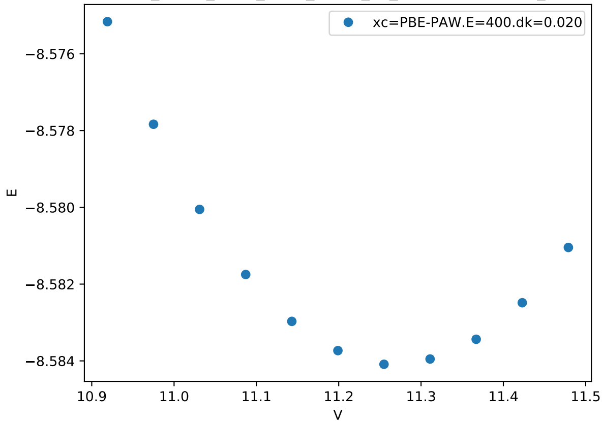
Cr_pv-Co_pv-W_sv/Cr_pv-Co_pv_sigma-BABAA.FM_
