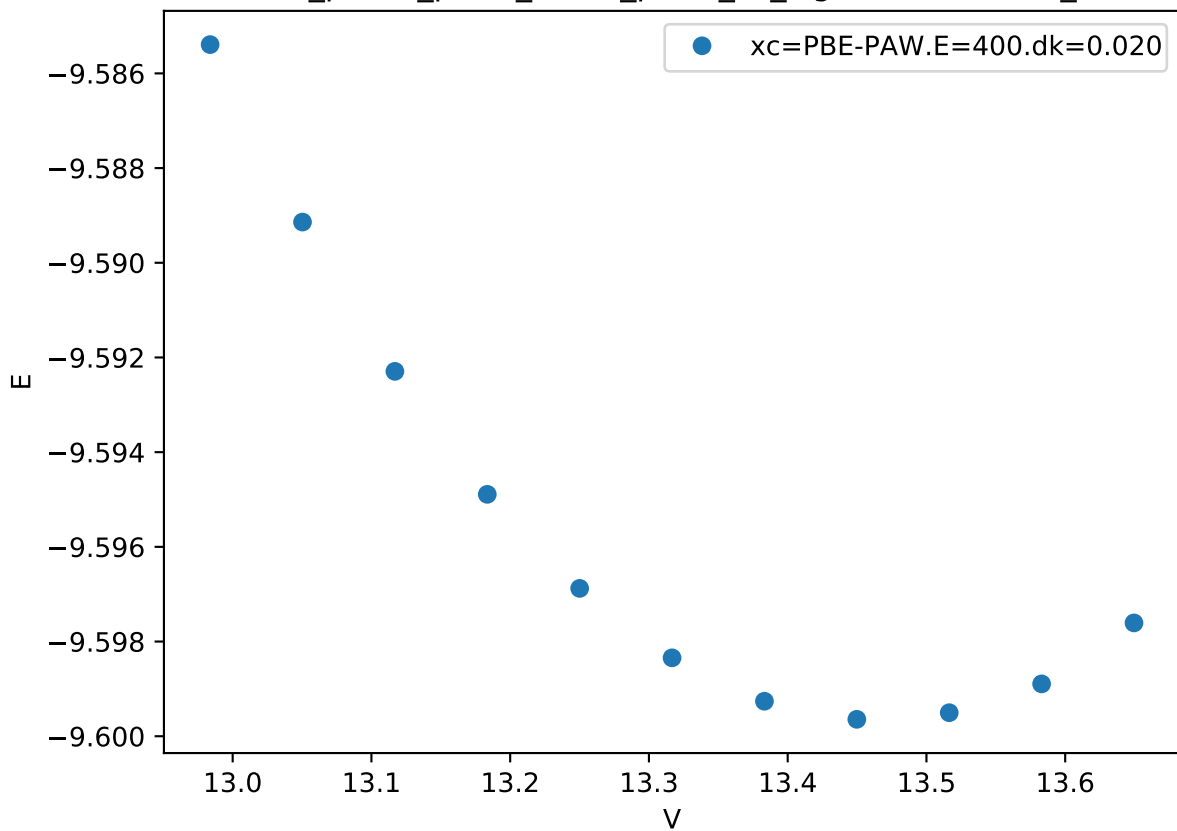
Cr_pv-Co_pv-W_sv/Co_pv-W_sv_sigma-BBAAB.FM_
