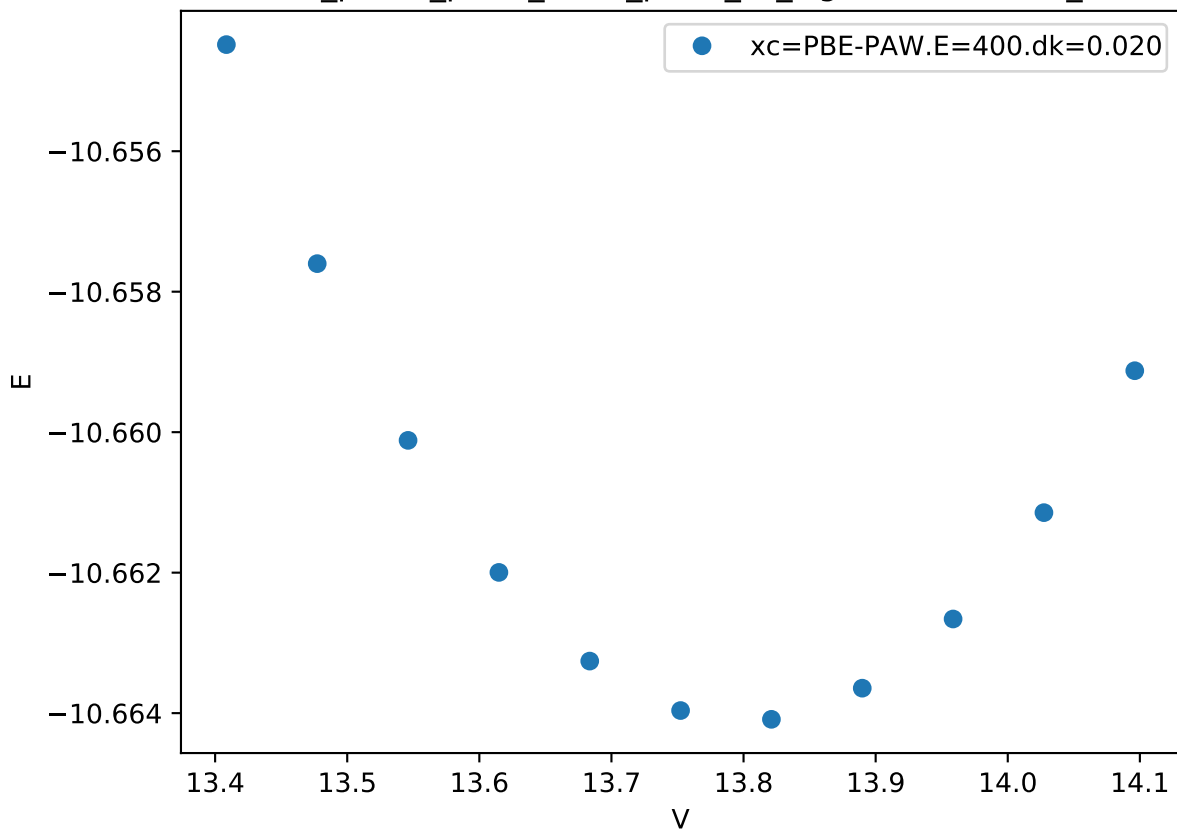
Cr_pv-Co_pv-W_sv/Cr_pv-W_sv_sigma-ABABA.FM_
