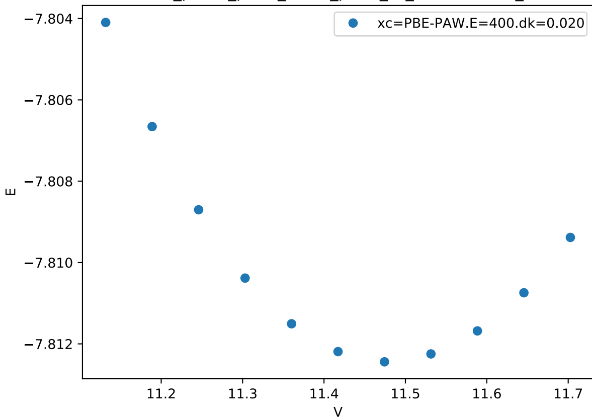
Cr_pv-Co_pv-W_sv/Co_pv-W_sv_chi-ABAA.FM_
