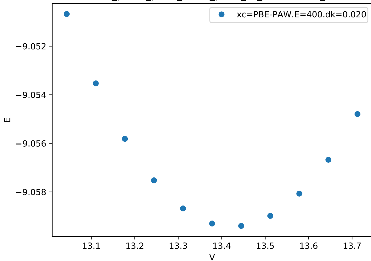
Cr_pv-Co_pv-W_sv/Co_pv-W_sv_C36-BAAAB_
