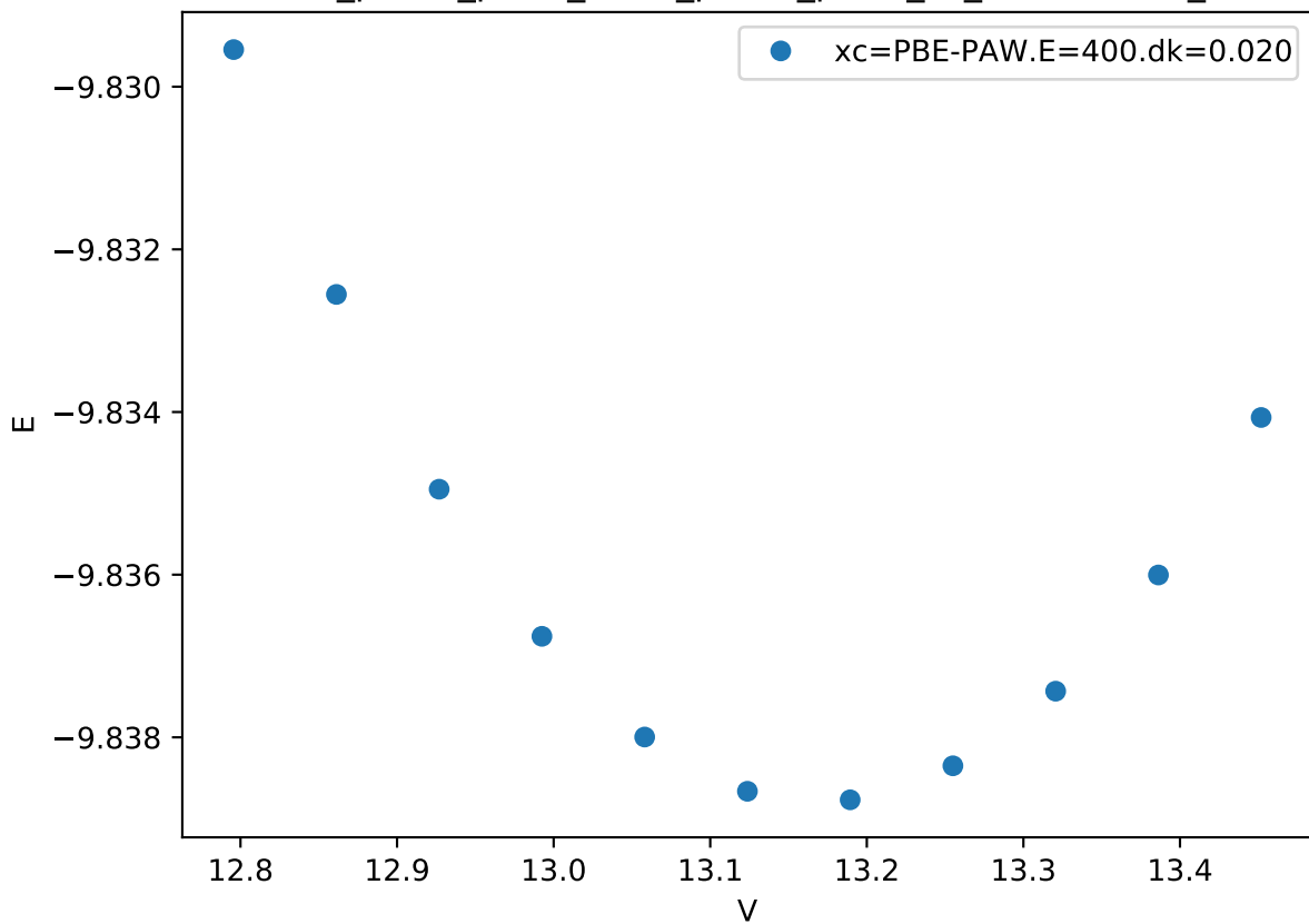
Cr_pv-Co_pv-W_sv/Cr_pv-Co_pv-W_sv_C36-CACAB_
