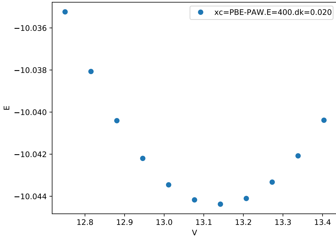
Cr_pv-Co_pv-W_sv/Cr_pv-Co_pv-W_sv_sigma-BAAAC.FM_
