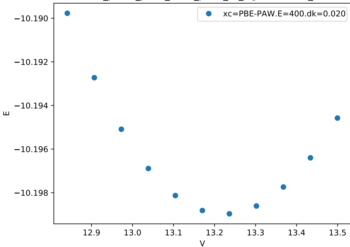
Cr_pv-Co_pv-W_sv/Cr_pv-W_sv_sigma-AAAAB_
