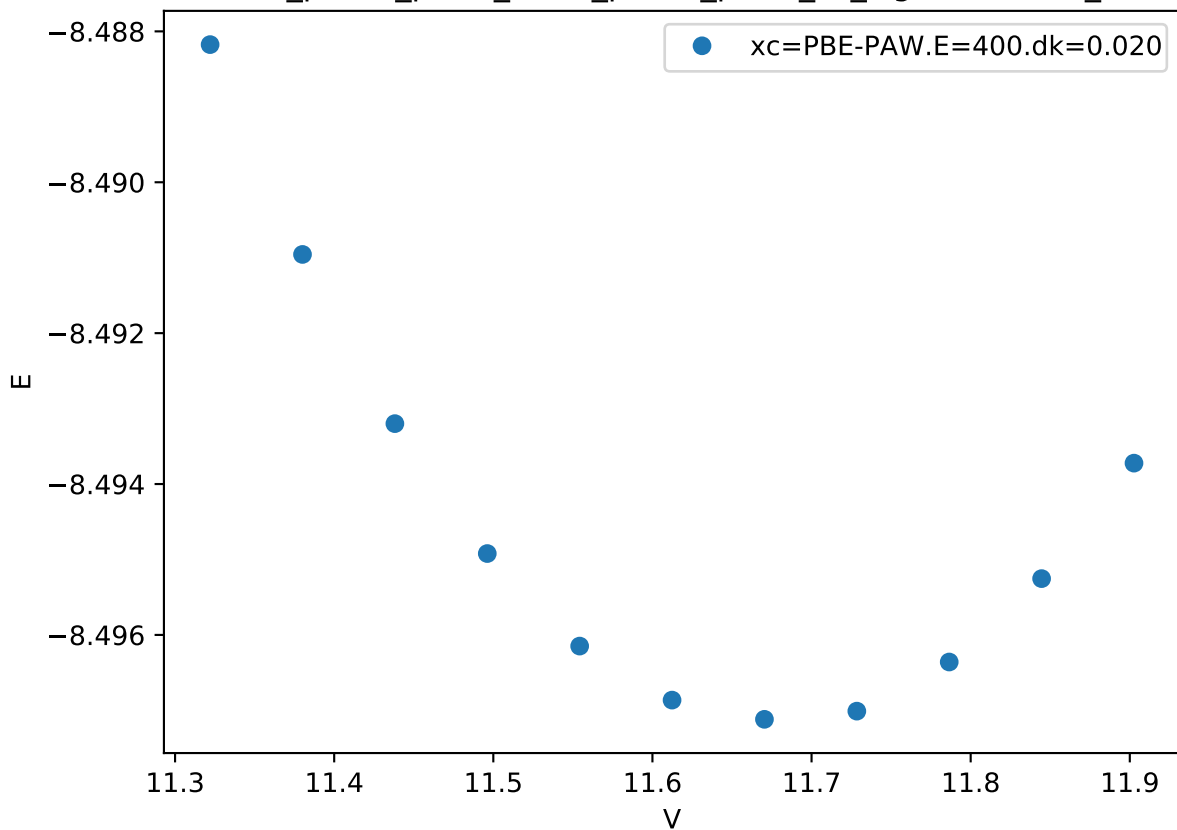
Cr_pv-Co_pv-W_sv/Cr_pv-Co_pv-W_sv_sigma-ACBAB_
