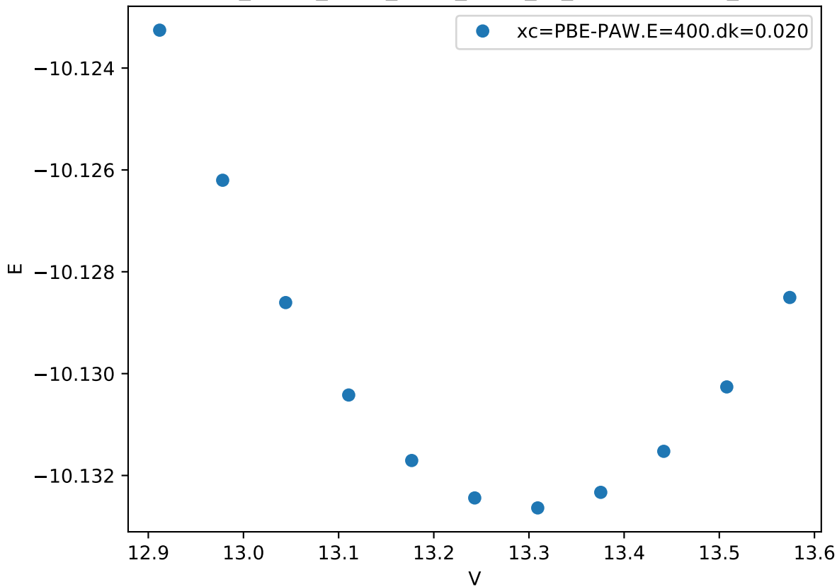
Cr_pv-Co_pv-W_sv/Cr_pv-W_sv_sigma-AAABA_
