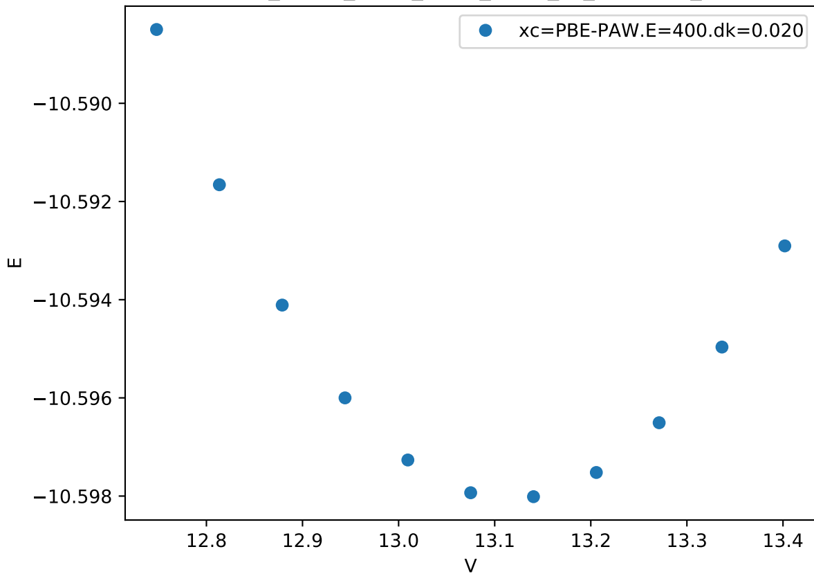
Cr_pv-Co_pv-W_sv/Cr_pv-W_sv_C15-A2B_
