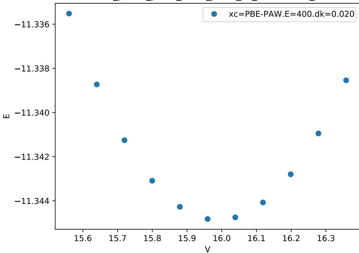
Cr_pv-Co_pv-W_sv/Cr_pv-W_sv_mu-BBAA_
