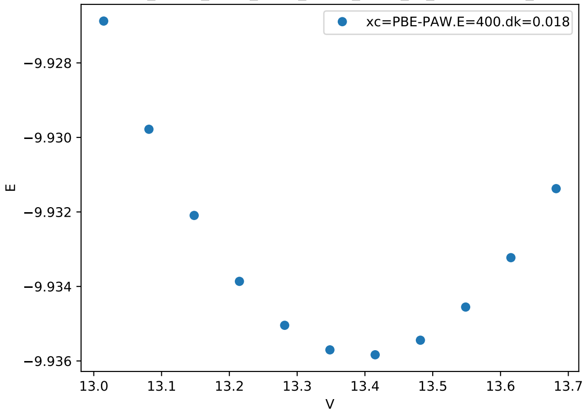
Cr_pv-Co_pv-W_sv/Cr_pv-Co_pv-W_sv_C36-BCCAA_
