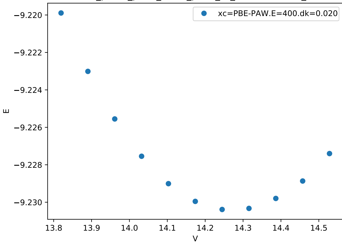
Cr_pv-Co_pv-W_sv/Co_pv-W_sv_mu-ABAAA.FM_
