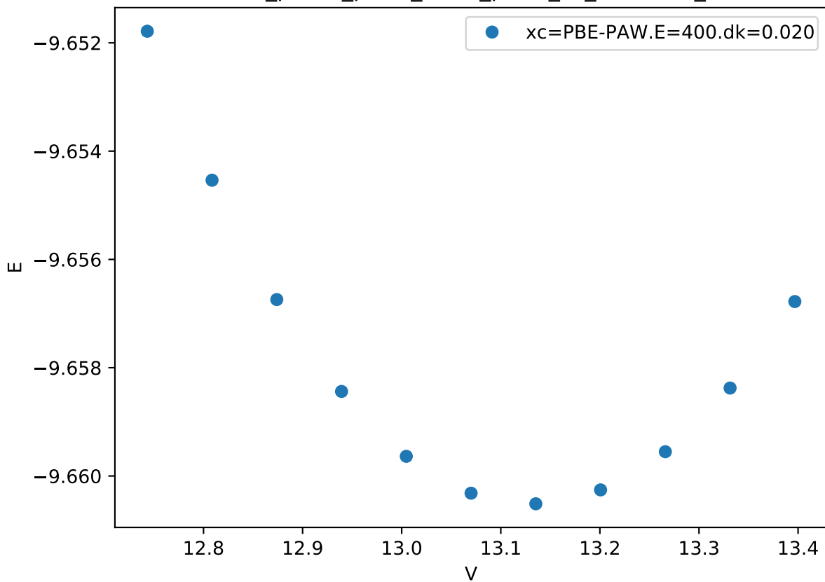
Cr_pv-Co_pv-W_sv/Cr_pv-W_sv_C14-ABA_
