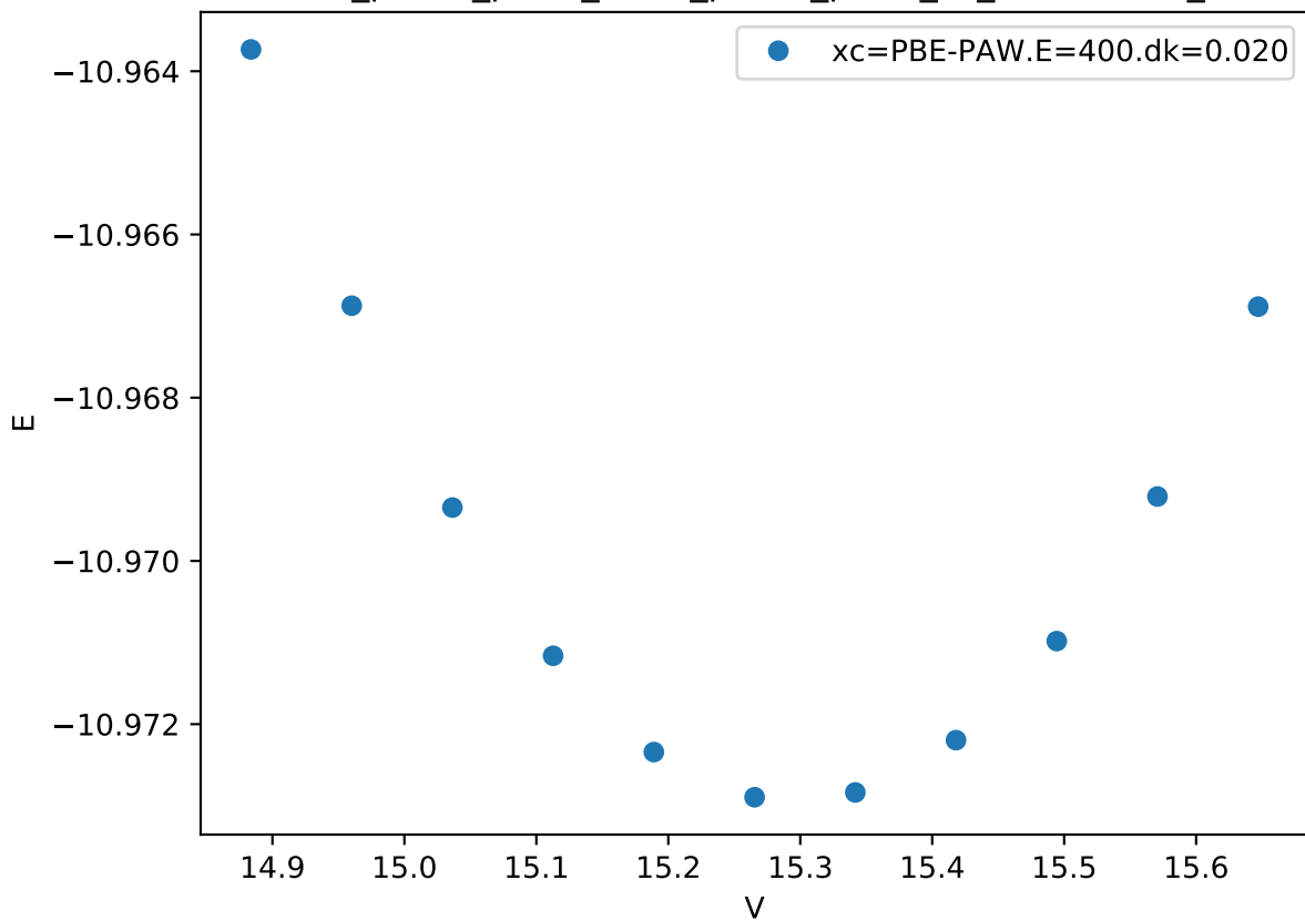
Cr_pv-Co_pv-W_sv/Cr_pv-Co_pv-W_sv_mu-BCCAA_
