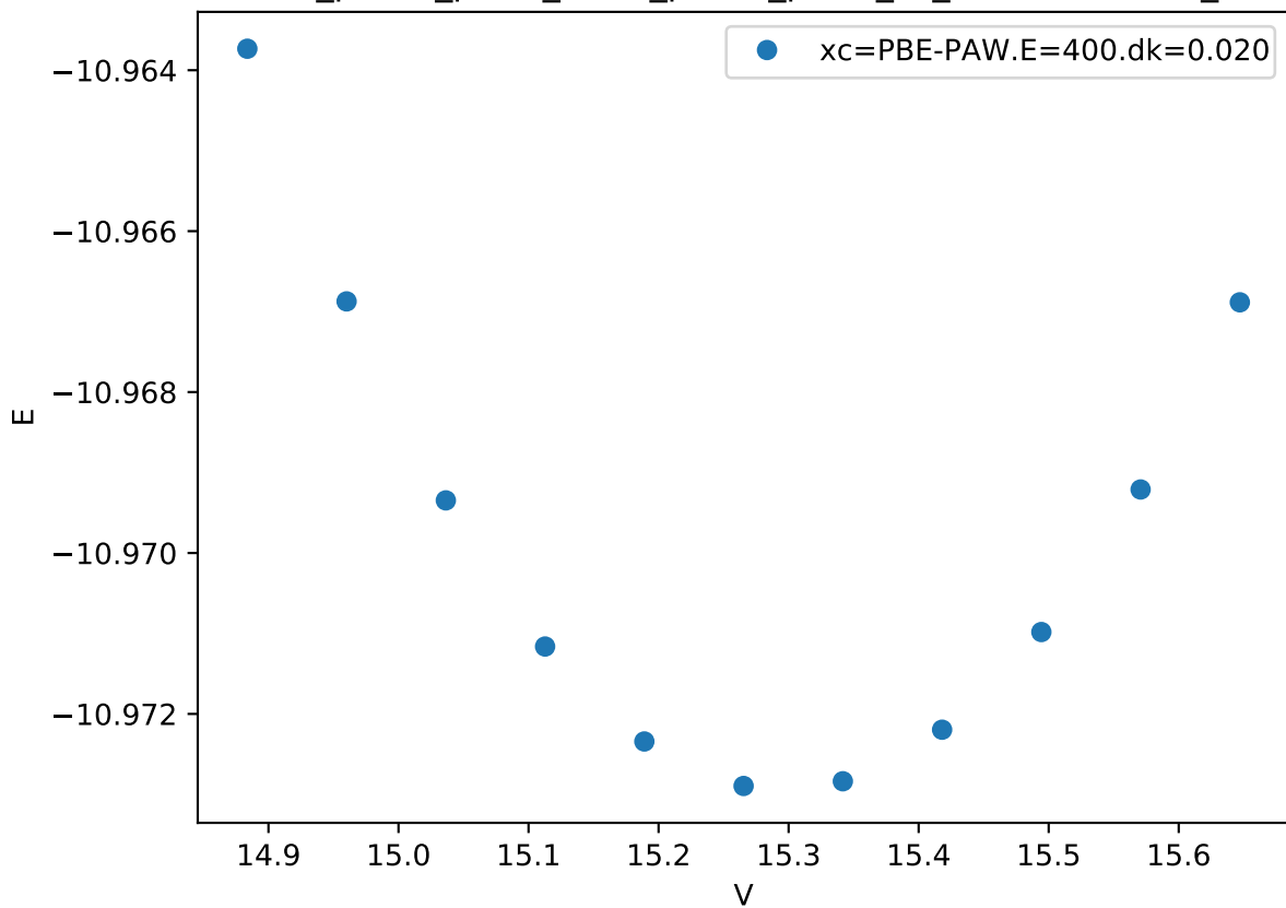
Cr_pv-Co_pv-W_sv/Cr_pv-Co_pv-W_sv_mu-BCCAA.FM_
