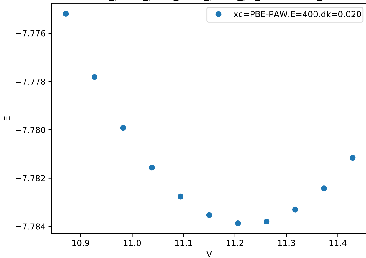
Cr_pv-Co_pv-W_sv/Cr_pv-Co_pv_C36-BABAB_
