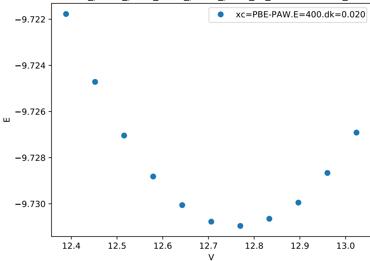
Cr_pv-Co_pv-W_sv/Cr_pv-Co_pv-W_sv_mu-CAACB.FM_
