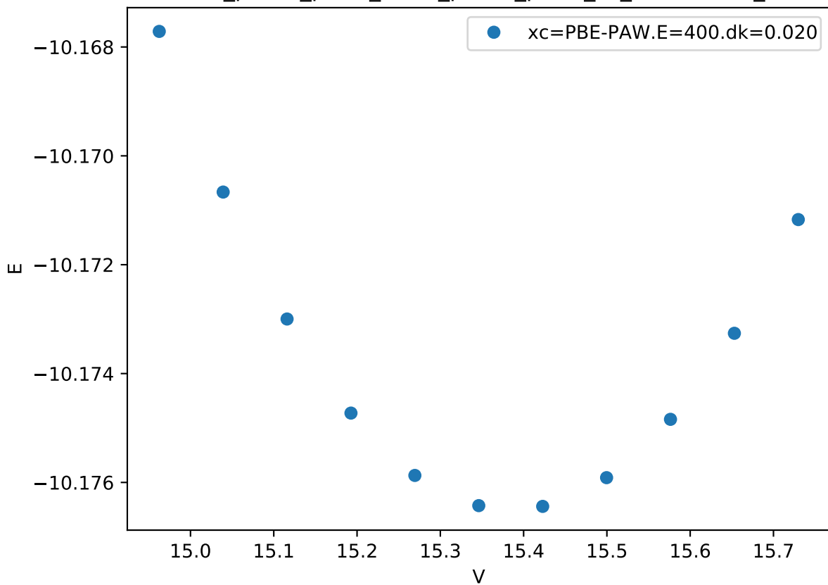
Cr_pv-Co_pv-W_sv/Cr_pv-Co_pv-W_sv_mu-ACBBC_
