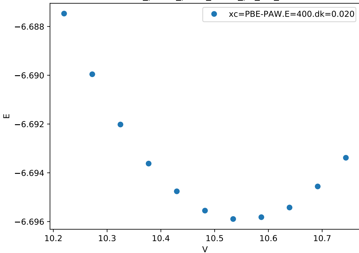
Cr_pv-Co_pv-W_sv/Co_pv_chi_
