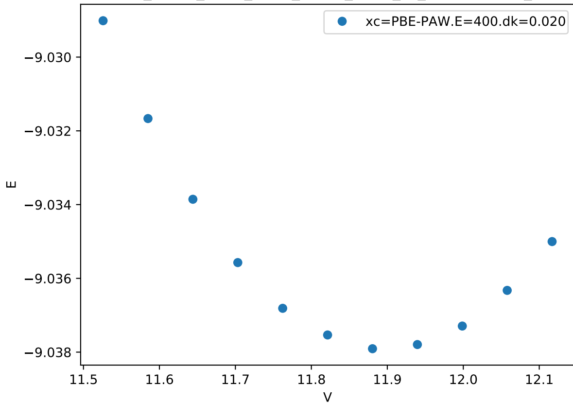
Cr_pv-Co_pv-W_sv/Cr_pv-Co_pv-W_sv_chi-CBAA.FM_
