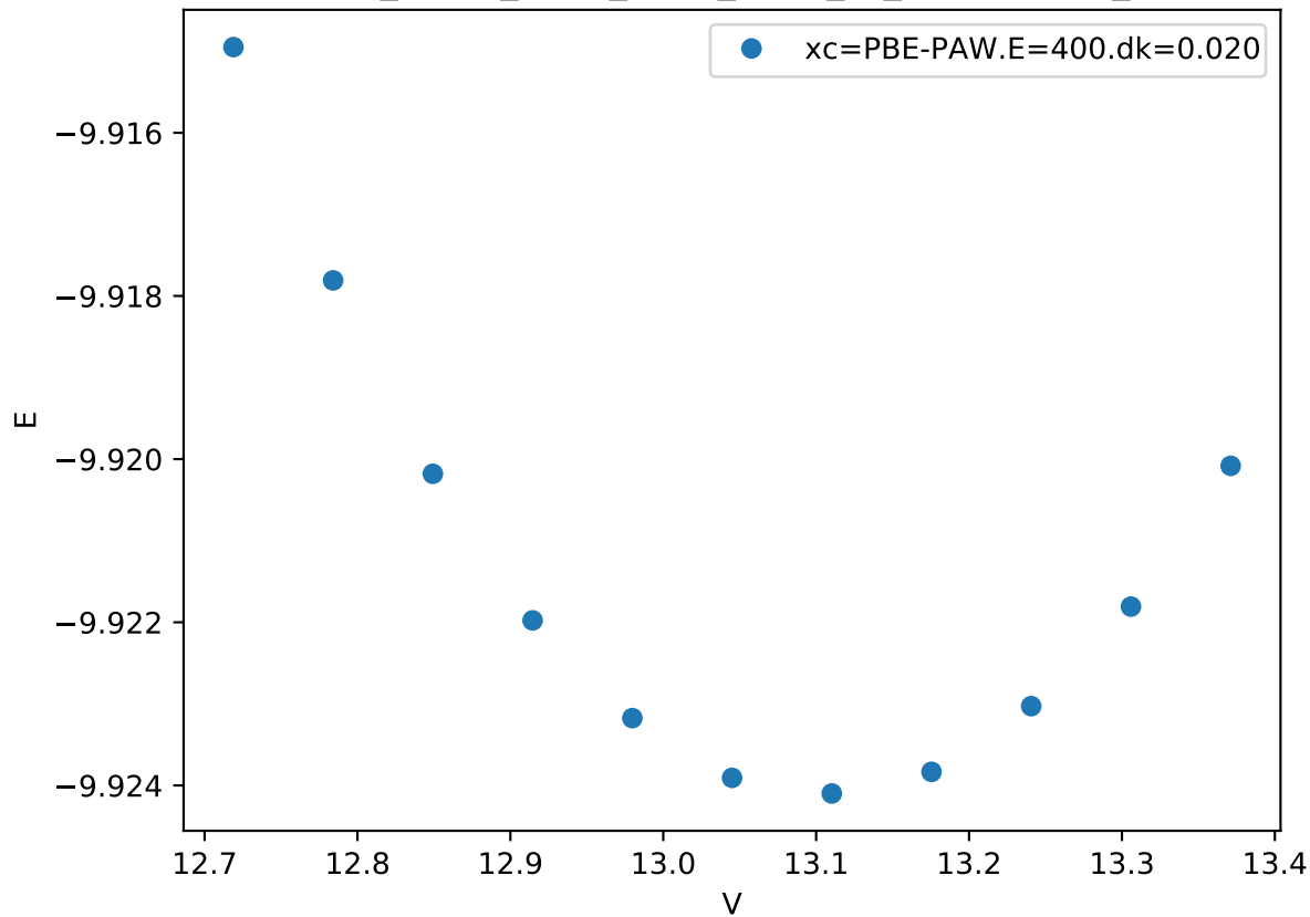
Cr_pv-Co_pv-W_sv/Cr_pv-W_sv_L12-A3B.FM_
