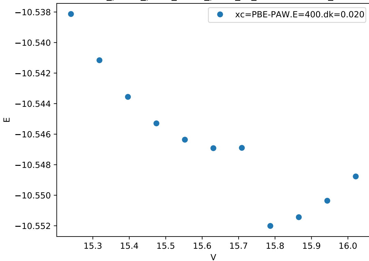
Cr_pv-Co_pv-W_sv/Co_pv-W_sv_mu-BBBAA.FM_
