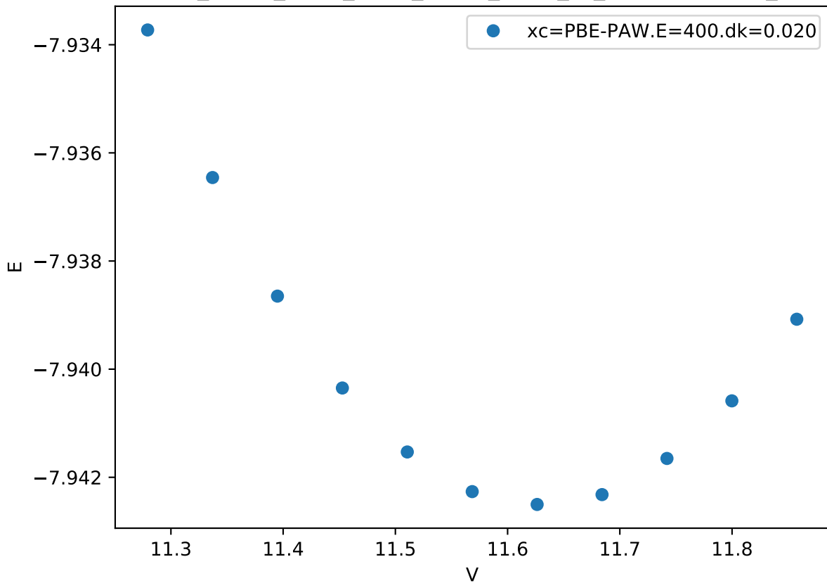
Cr_pv-Co_pv-W_sv/Cr_pv-Co_pv-W_sv_mu-ABBBC.FM_
