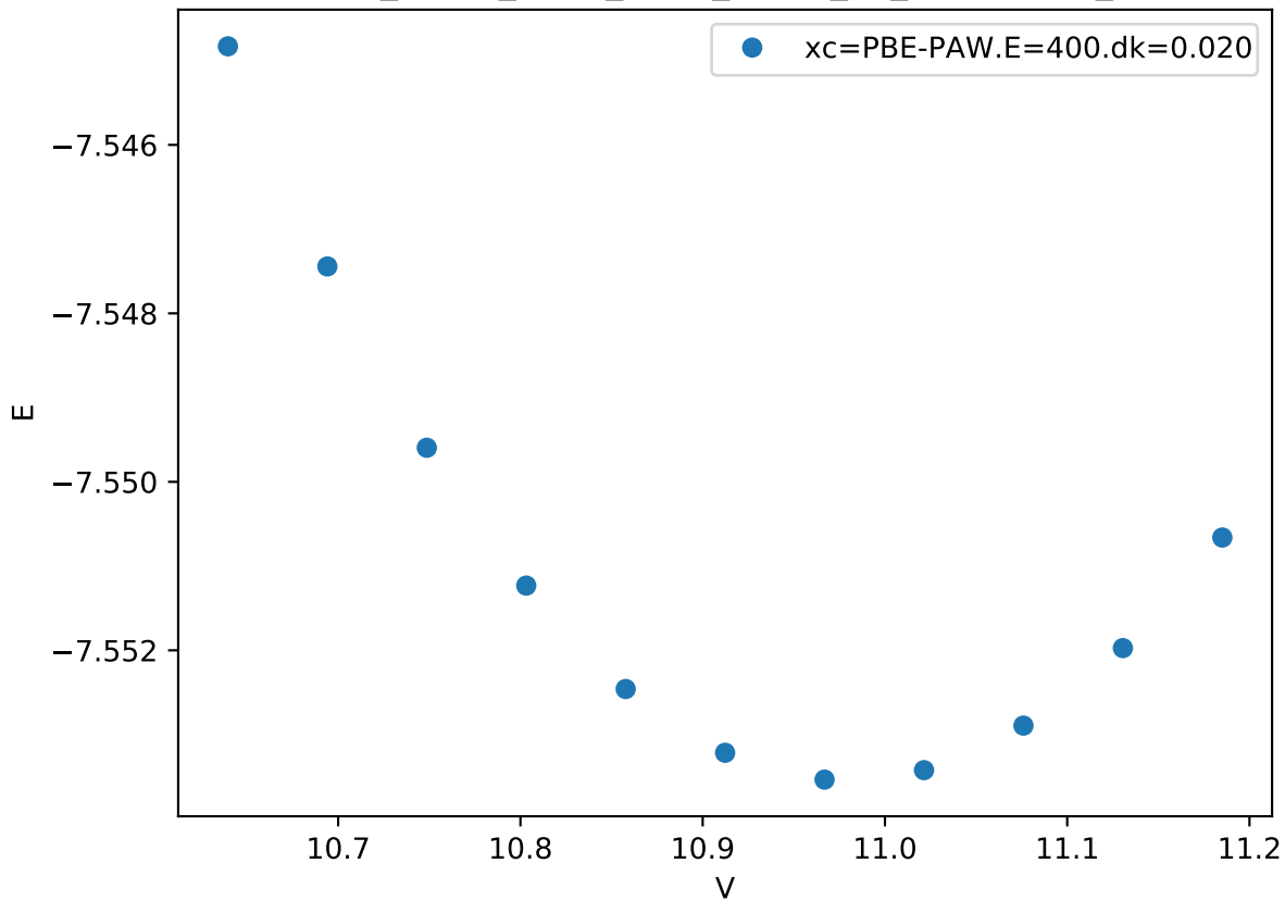
Cr_pv-Co_pv-W_sv/Cr_pv-Co_pv_mu-BBAAB_
