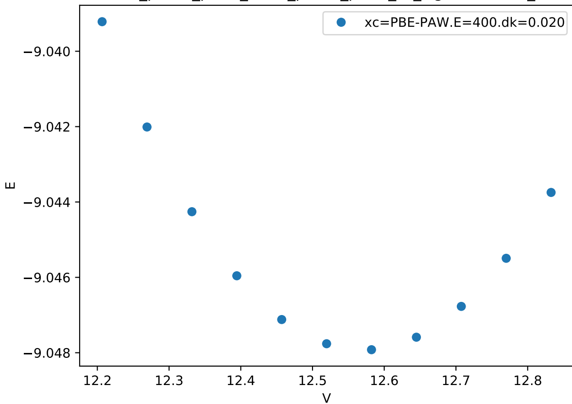
Cr_pv-Co_pv-W_sv/Cr_pv-Co_pv-W_sv_sigma-BBBCA_
