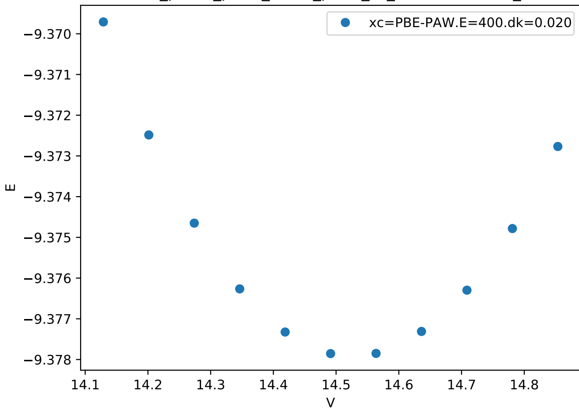
Cr_pv-Co_pv-W_sv/Co_pv-W_sv_C36-AAABB.FM_
