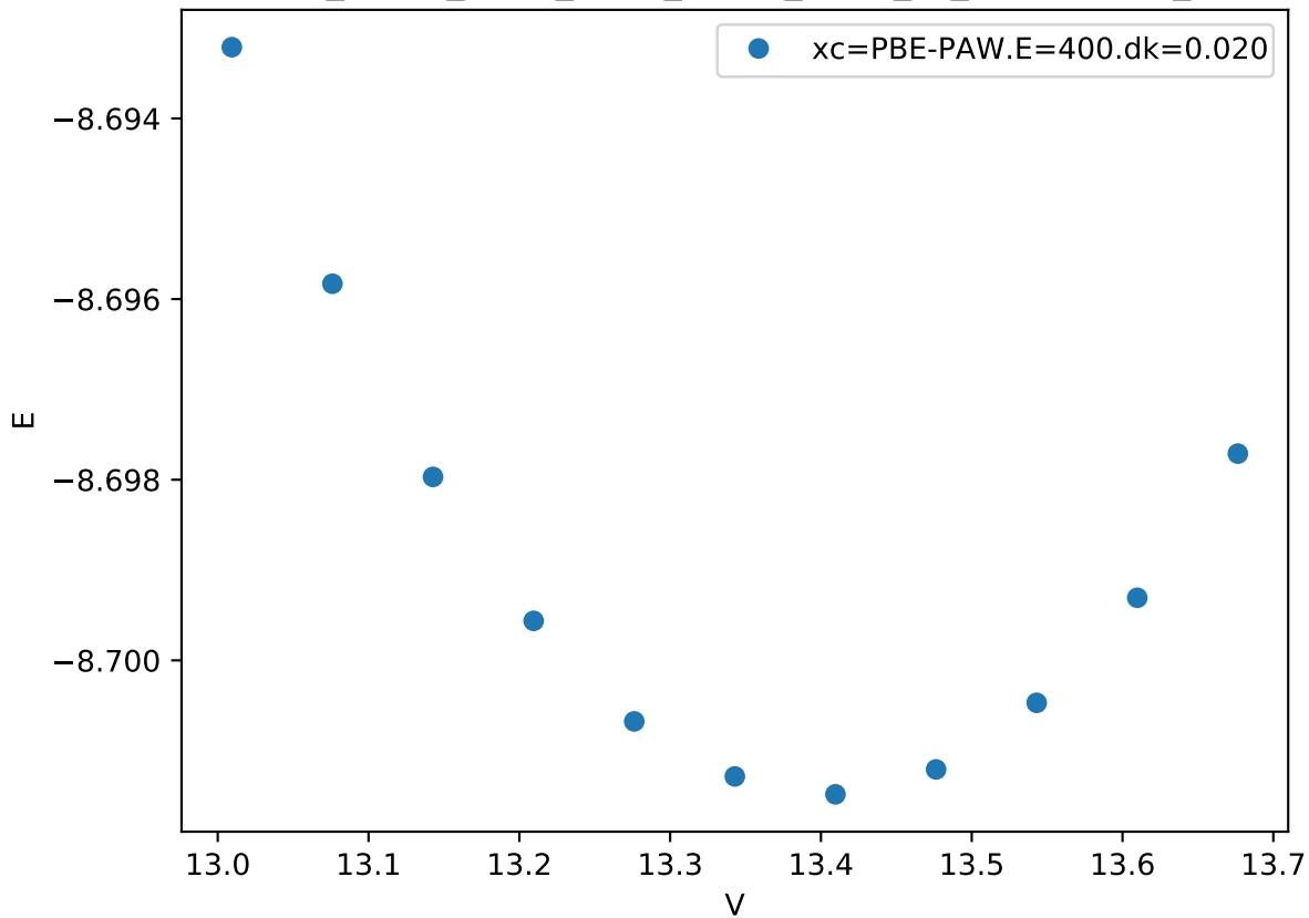
Cr_pv-Co_pv-W_sv/Cr_pv-Co_pv-W_sv_C36-BAABC_
