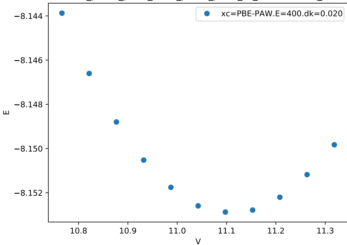
Cr_pv-Co_pv-W_sv/Cr_pv-Co_pv-W_sv_chi-CBAB.FM_
