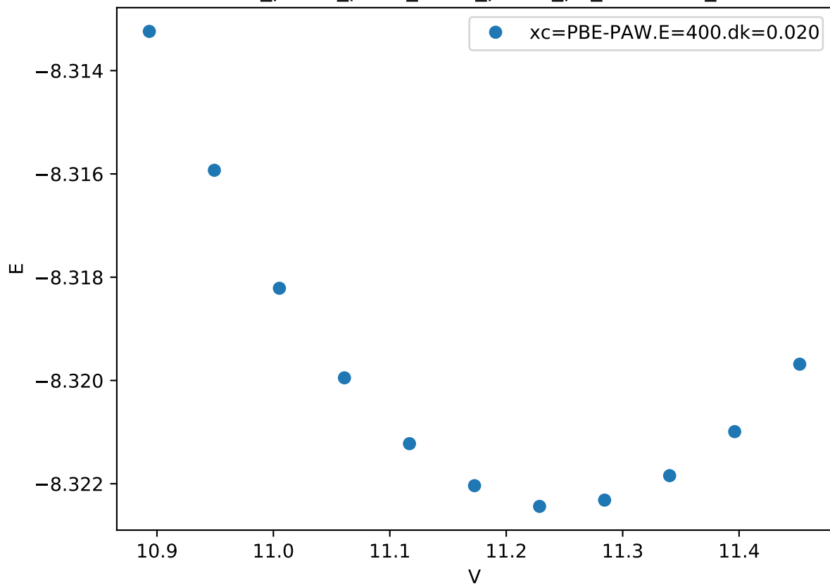
Cr_pv-Co_pv-W_sv/Cr_pv-Co_pv_chi-AABA_
