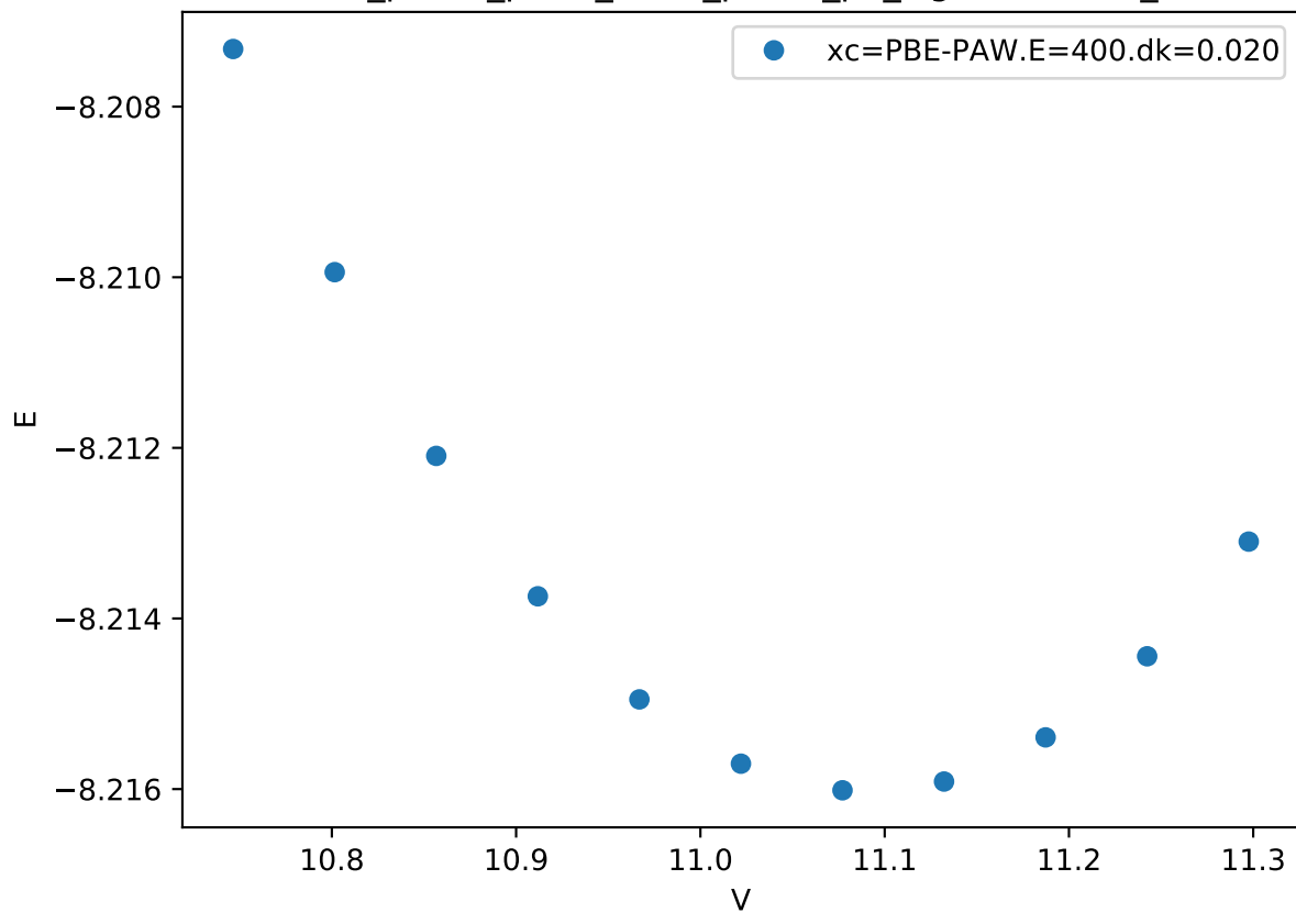
Cr_pv-Co_pv-W_sv/Cr_pv-Co_pv_sigma-BBBAA_
