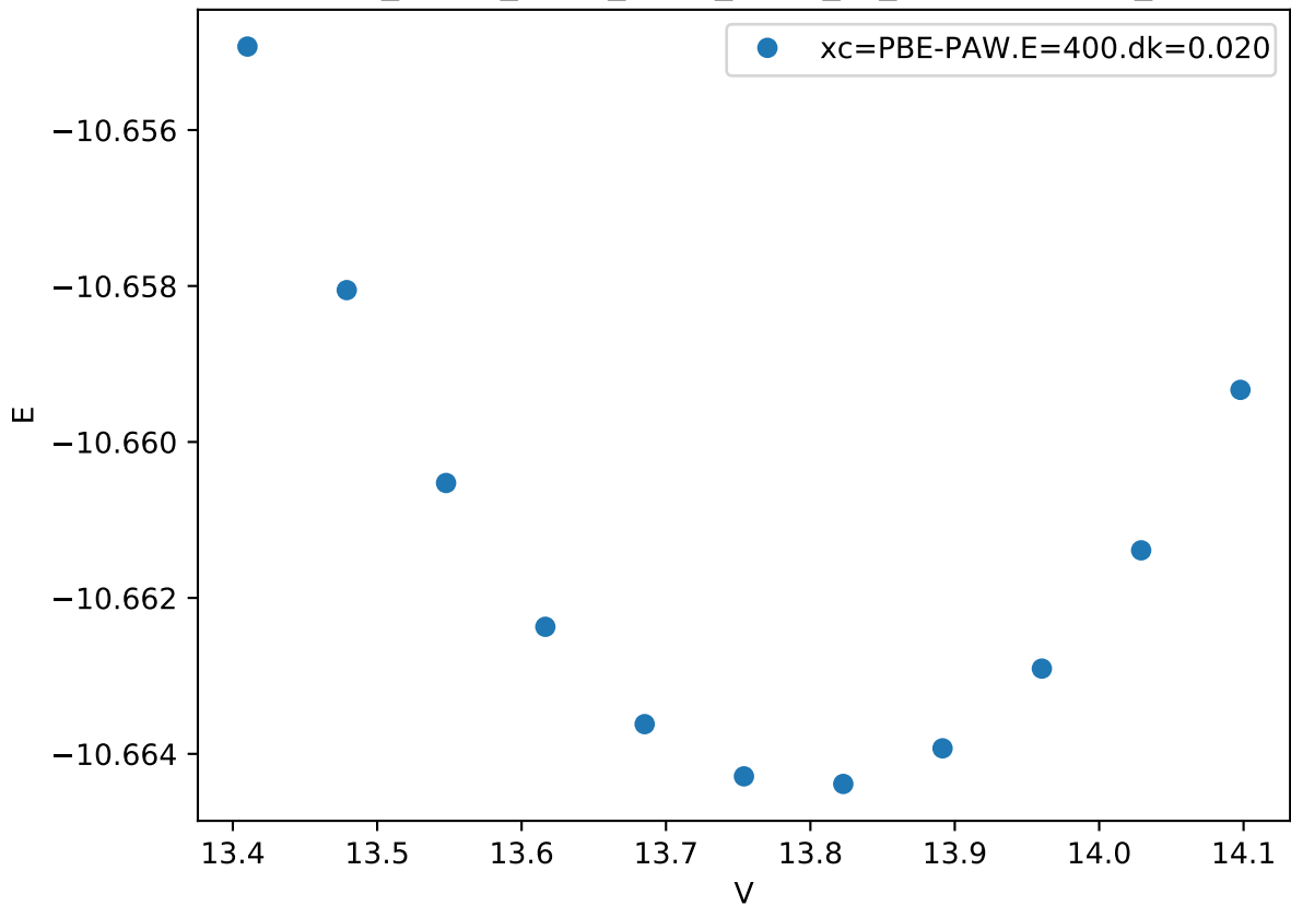
Cr_pv-Co_pv-W_sv/Cr_pv-W_sv_sigma-ABABA_
