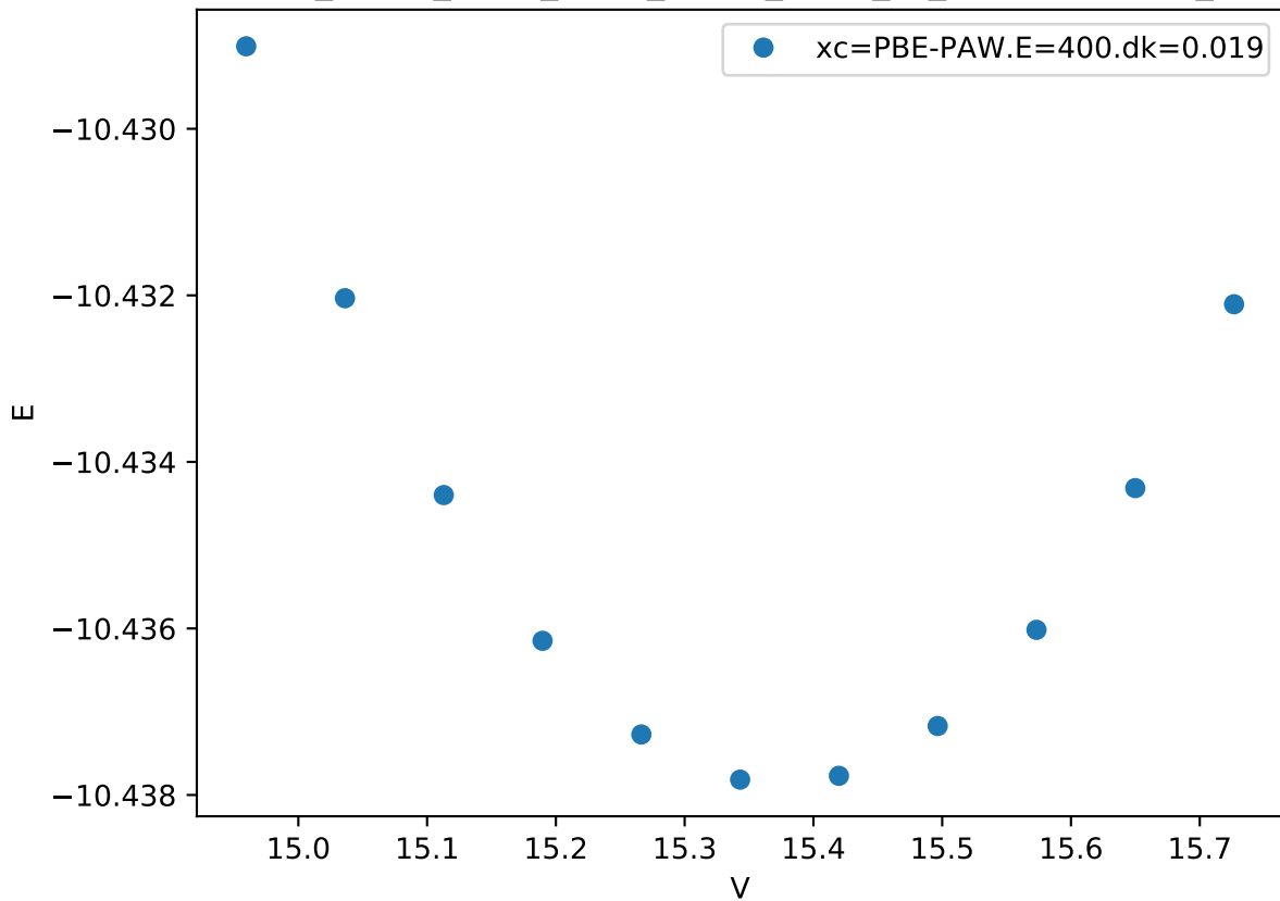
Cr_pv-Co_pv-W_sv/Cr_pv-Co_pv-W_sv_mu-BCBAC.FM_
