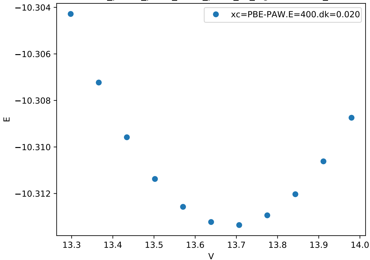
Cr_pv-Co_pv-W_sv/Cr_pv-W_sv_sigma-BAABA_
