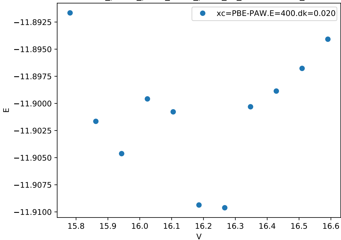
Cr_pv-Co_pv-W_sv/Cr_pv-W_sv_chi-AABB.FM_
