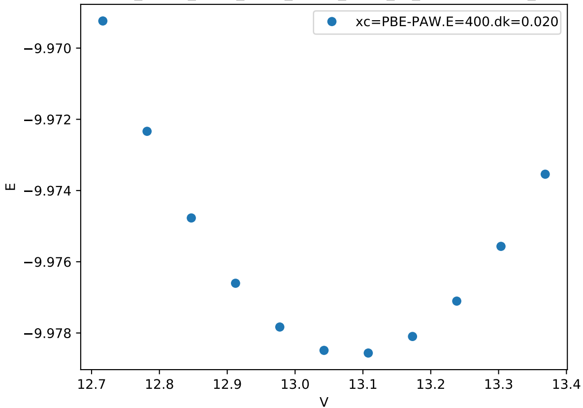
Cr_pv-Co_pv-W_sv/Cr_pv-Co_pv-W_sv_sigma-BCABC_
