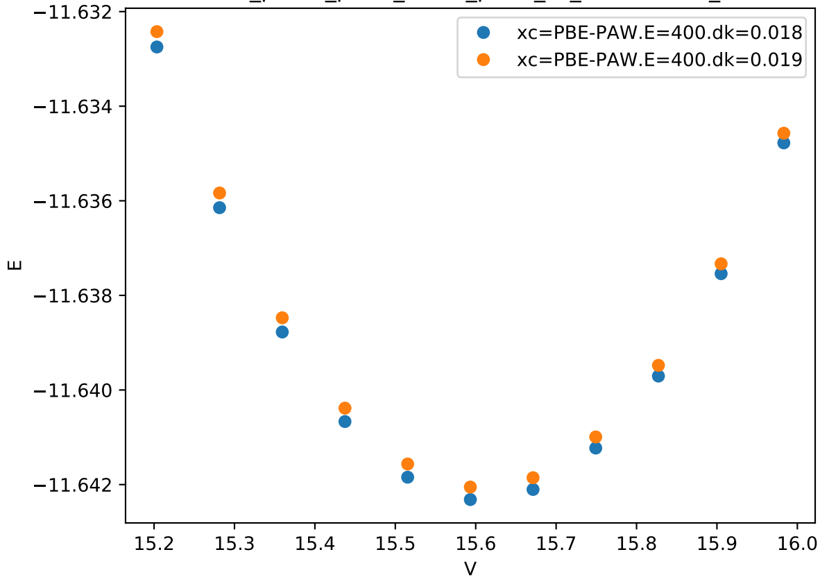
Cr_pv-Co_pv-W_sv/Co_pv-W_sv_C36-BBABB_
