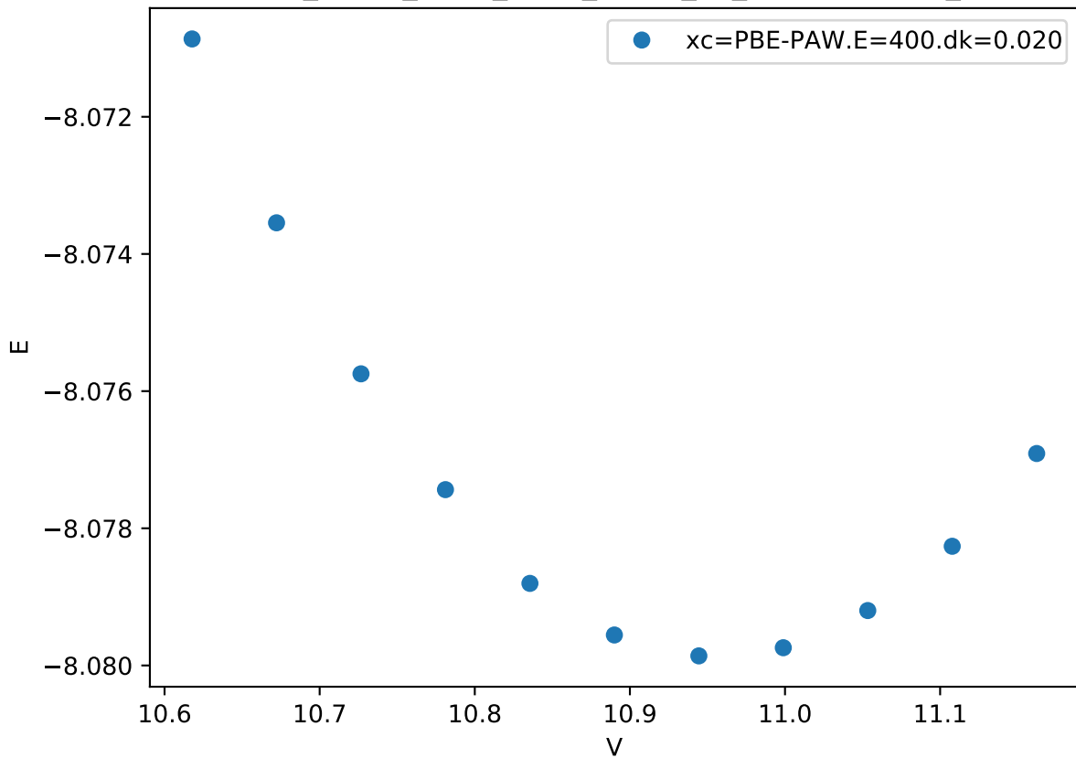
Cr_pv-Co_pv-W_sv/Cr_pv-Co_pv_sigma-AAABB_
