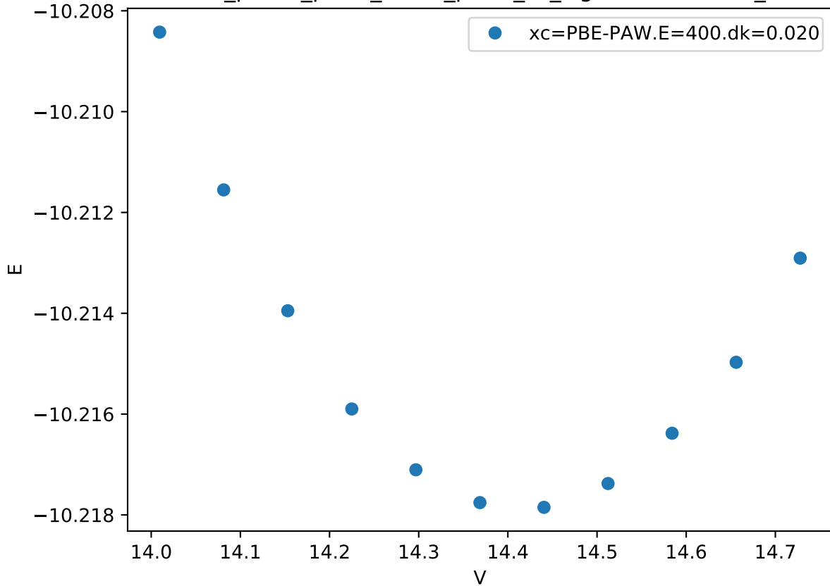
Cr_pv-Co_pv-W_sv/Co_pv-W_sv_sigma-BABBA.FM_
