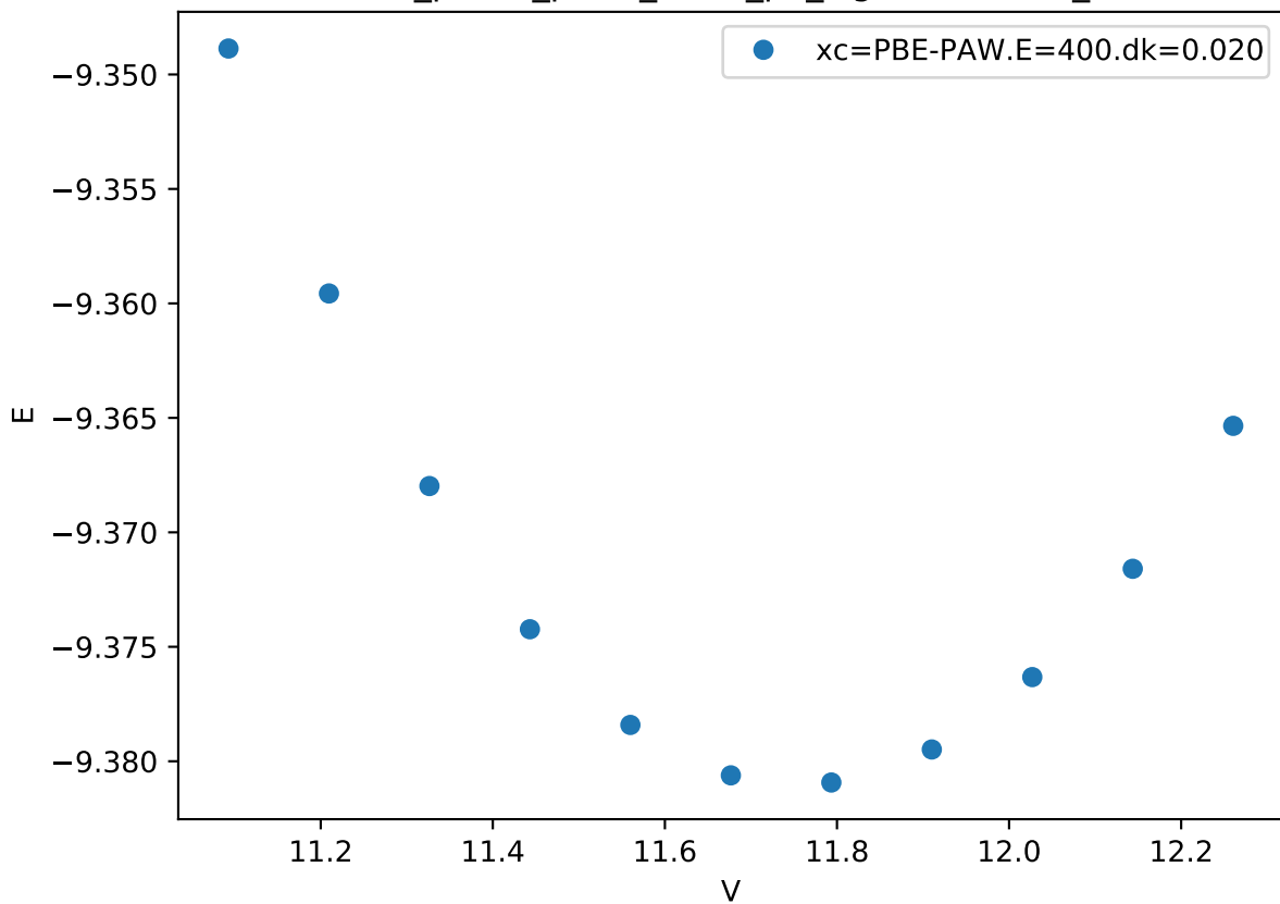
Cr_pv-Co_pv-W_sv/Cr_pv_sigma.UDDDD_
