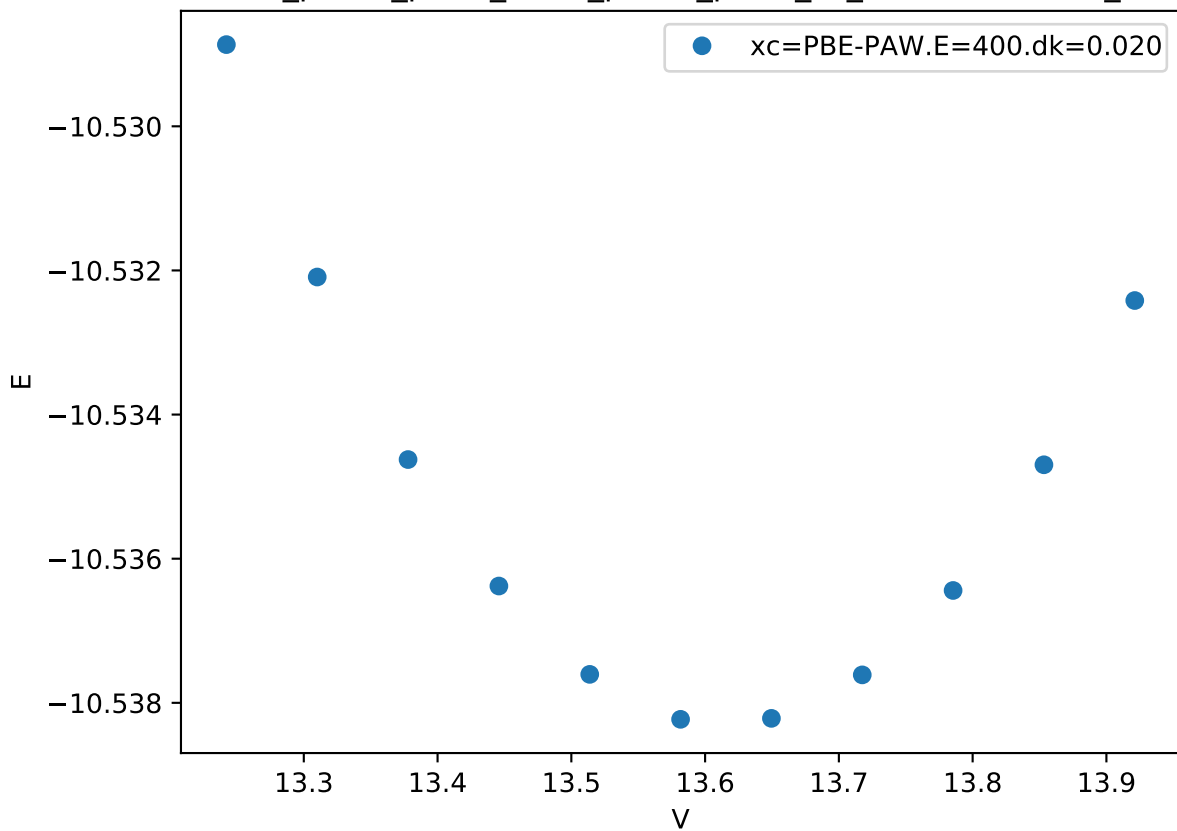
Cr_pv-Co_pv-W_sv/Cr_pv-Co_pv-W_sv_C36-CCCAB.FM_
