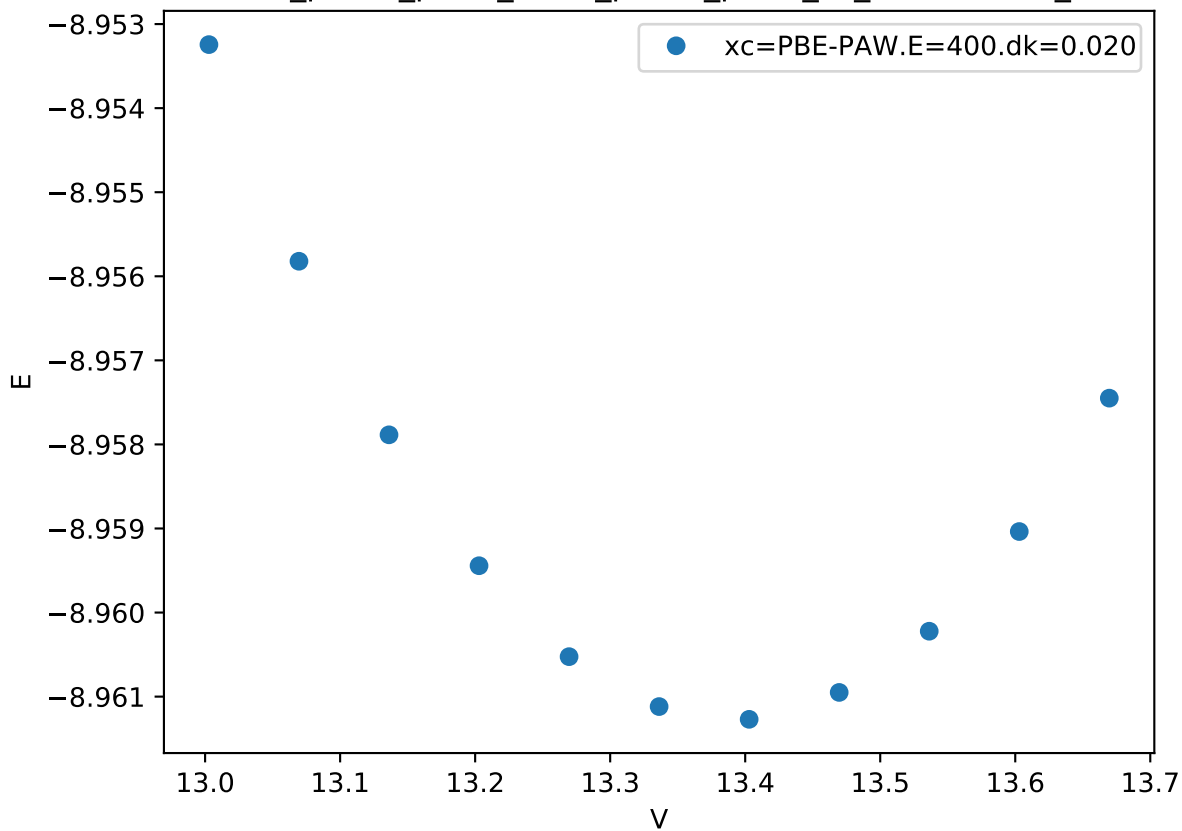
Cr_pv-Co_pv-W_sv/Cr_pv-Co_pv-W_sv_C36-BBAAC_
