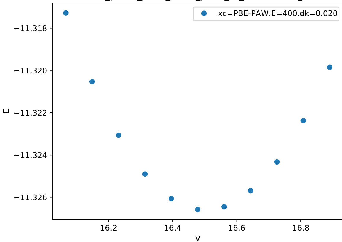
Cr_pv-Co_pv-W_sv/Co_pv-W_sv_C36-ABBBB_
