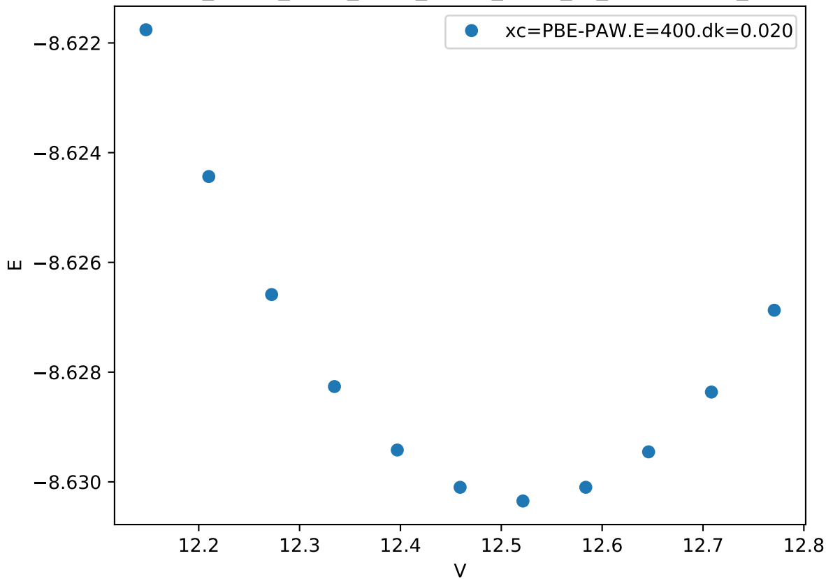
Cr_pv-Co_pv-W_sv/Cr_pv-Co_pv-W_sv_C36-ABCBA_
