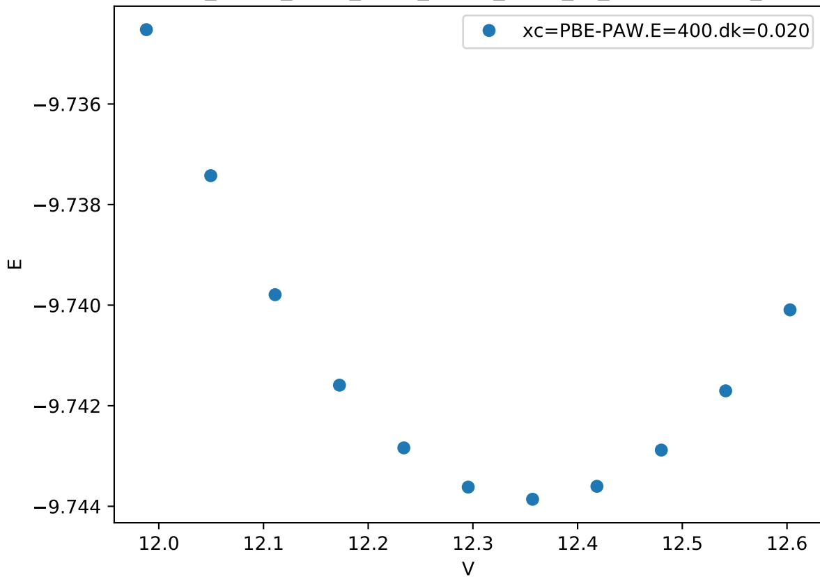
Cr_pv-Co_pv-W_sv/Cr_pv-Co_pv-W_sv_chi-BCAA.FM_
