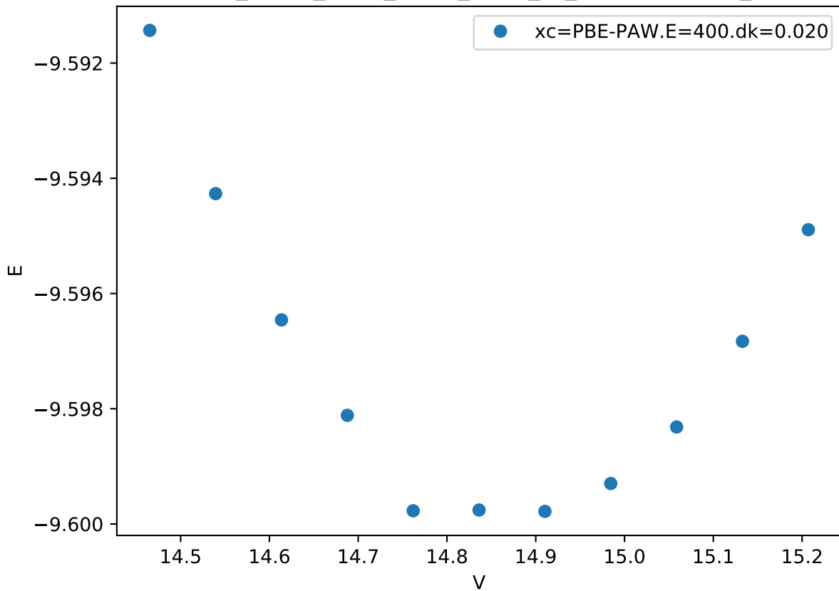
Cr_pv-Co_pv-W_sv/Co_pv-W_sv_mu-BBAAA.FM_
