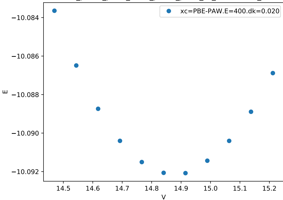
Cr_pv-Co_pv-W_sv/Cr_pv-Co_pv-W_sv_mu-ACBAA_
