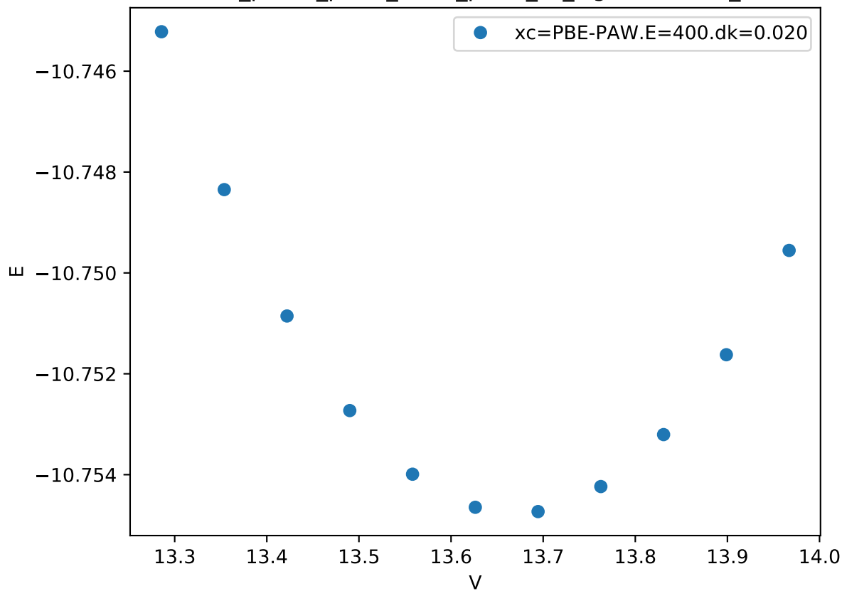
Cr_pv-Co_pv-W_sv/Cr_pv-W_sv_sigma-ABBAA_
