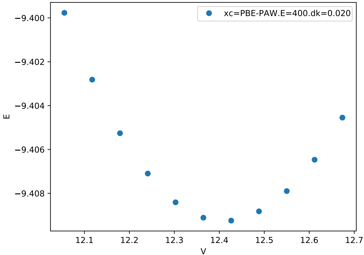
Cr_pv-Co_pv-W_sv/Cr_pv-Co_pv-W_sv_mu-ABCAC.FM_
