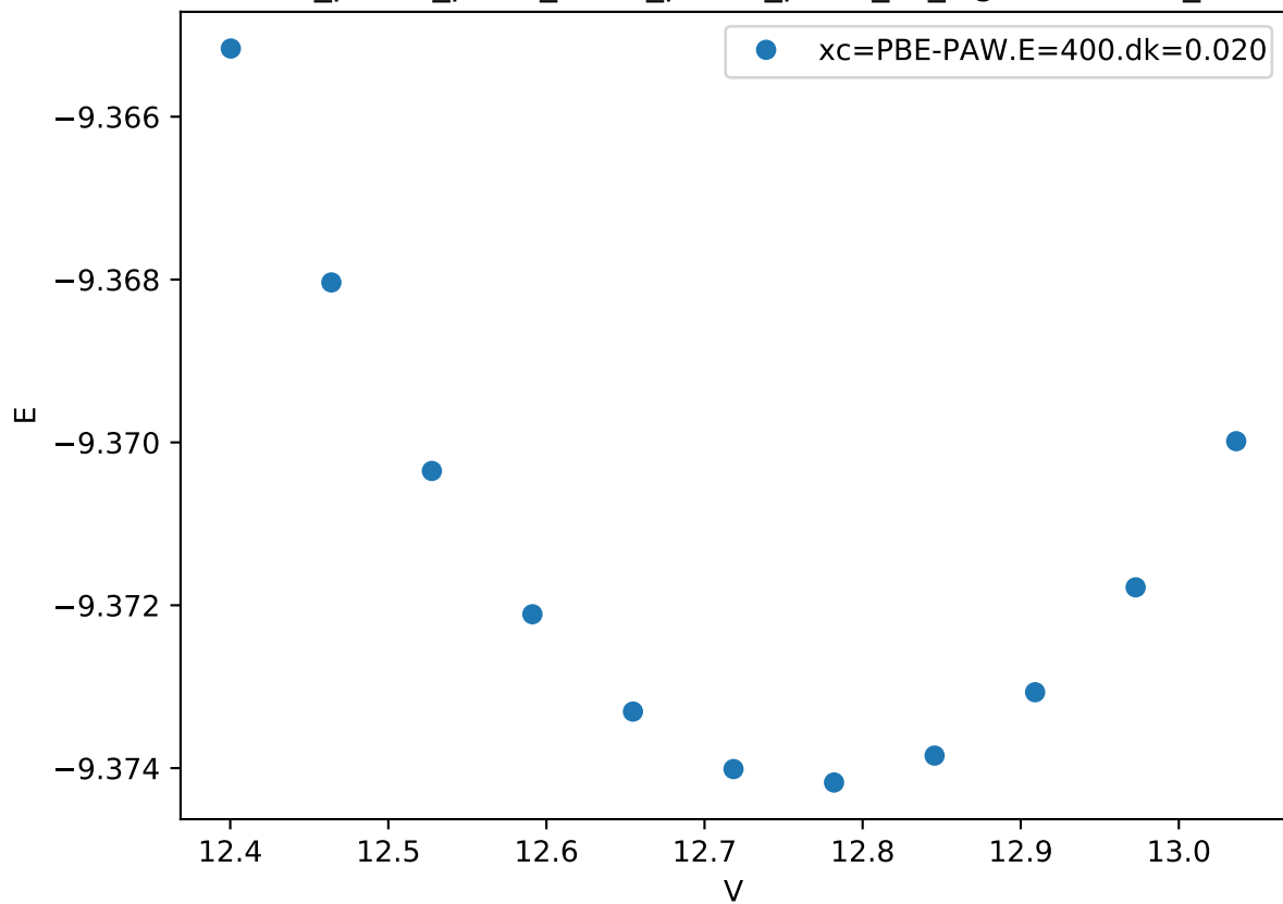
Cr_pv-Co_pv-W_sv/Cr_pv-Co_pv-W_sv_sigma-BABAC_
