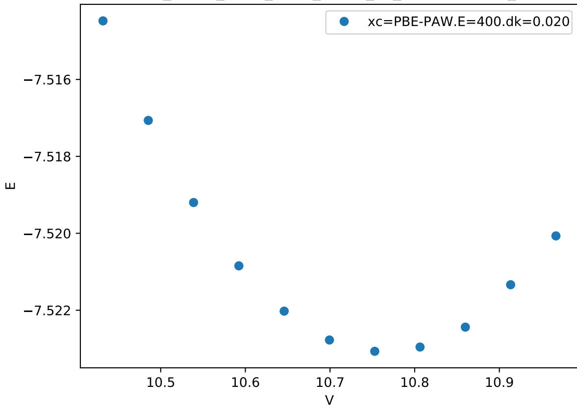
Cr_pv-Co_pv-W_sv/Cr_pv-Co_pv_sigma-BBABB_
