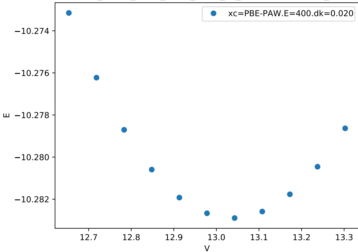
Cr_pv-Co_pv-W_sv/Cr_pv-W_sv_sigma-AABAA.FM_
