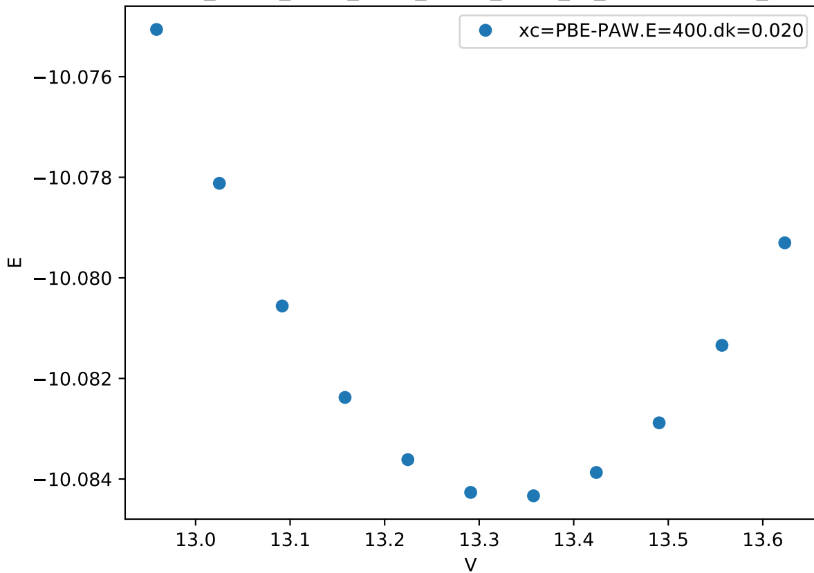
Cr_pv-Co_pv-W_sv/Cr_pv-Co_pv-W_sv_sigma-ACBCA_
