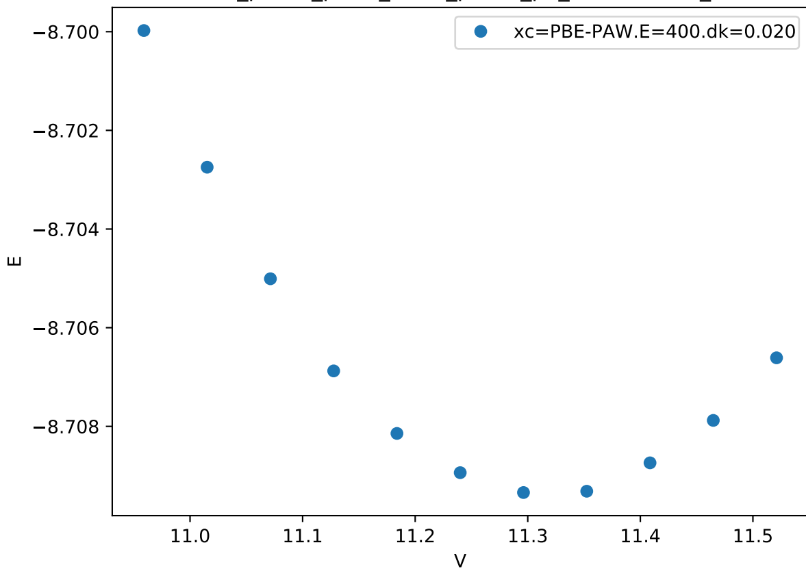
Cr_pv-Co_pv-W_sv/Cr_pv-Co_pv_L12-A3B.FM_
