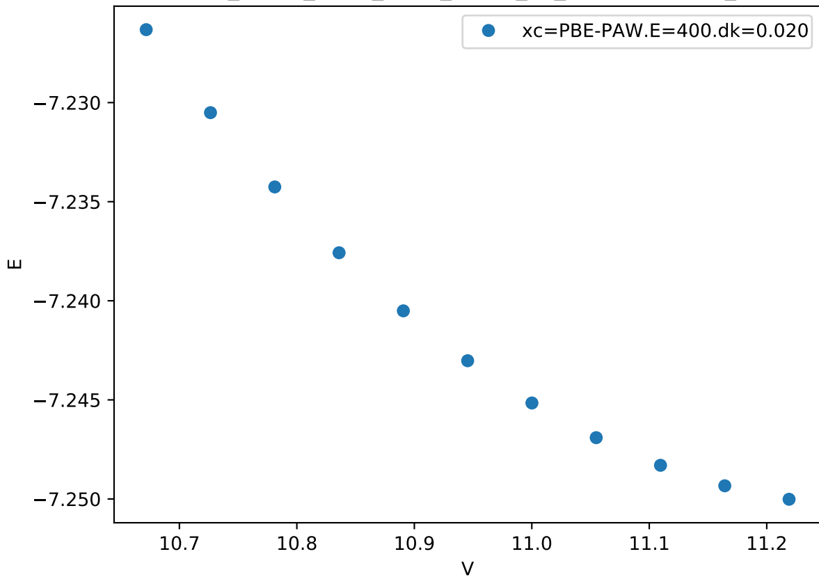
Cr_pv-Co_pv-W_sv/Cr_pv-Co_pv_mu-BBBBA.FM_
