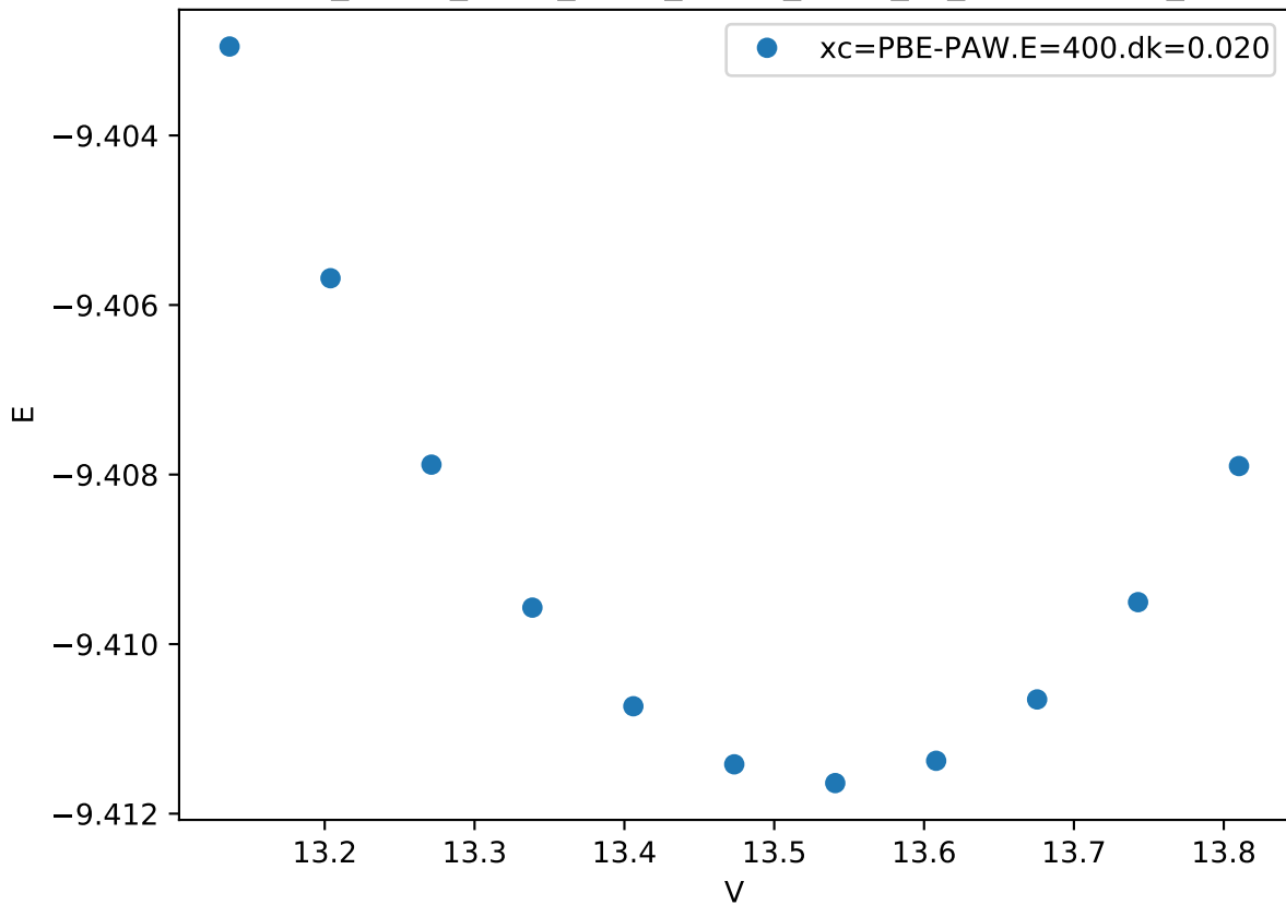
Cr_pv-Co_pv-W_sv/Cr_pv-Co_pv-W_sv_C36-BAACA_
