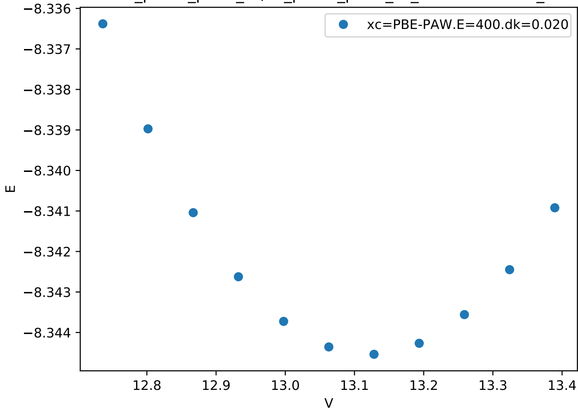
Cr_pv-Co_pv-W_sv/Cr_pv-Co_pv-W_sv_C36-BBACB.FM_
