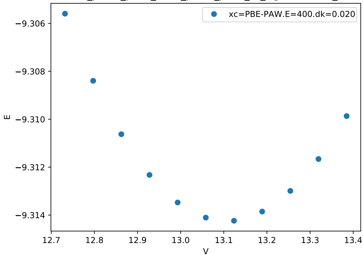
Cr_pv-Co_pv-W_sv/Cr_pv-Co_pv-W_sv_sigma-CBACB_
