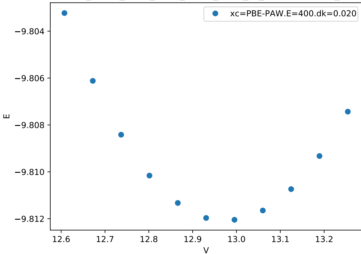
Cr_pv-Co_pv-W_sv/Cr_pv-Co_pv-W_sv_mu-BABCC.FM_
