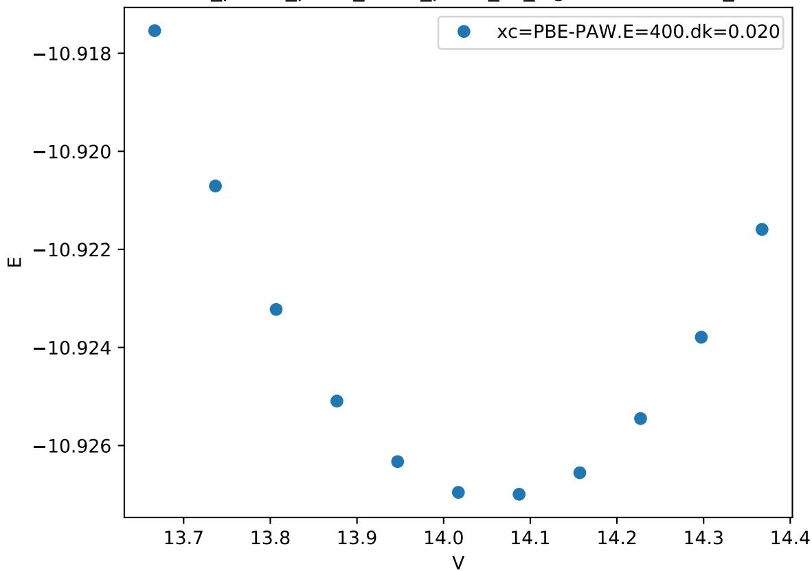
Cr_pv-Co_pv-W_sv/Cr_pv-W_sv_sigma-BBAAB.FM_
