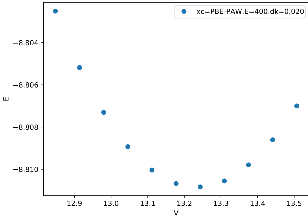
Cr_pv-Co_pv-W_sv/Cr_pv-Co_pv-W_sv_C36-BAACB_
