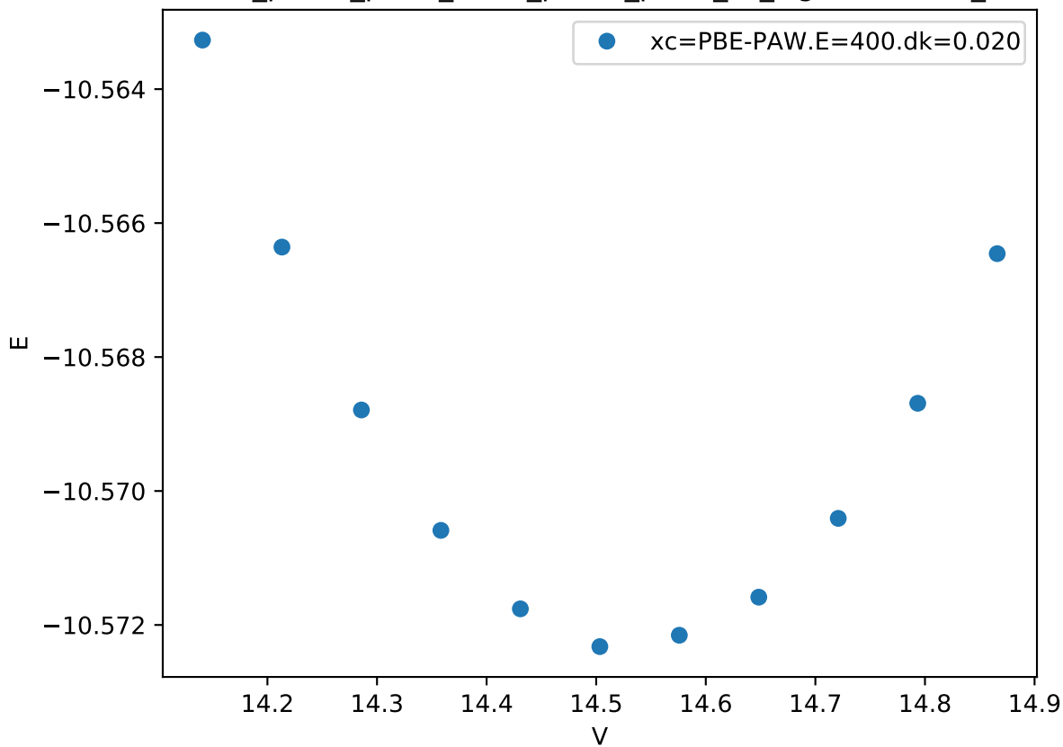
Cr_pv-Co_pv-W_sv/Cr_pv-Co_pv-W_sv_sigma-CACCB_
