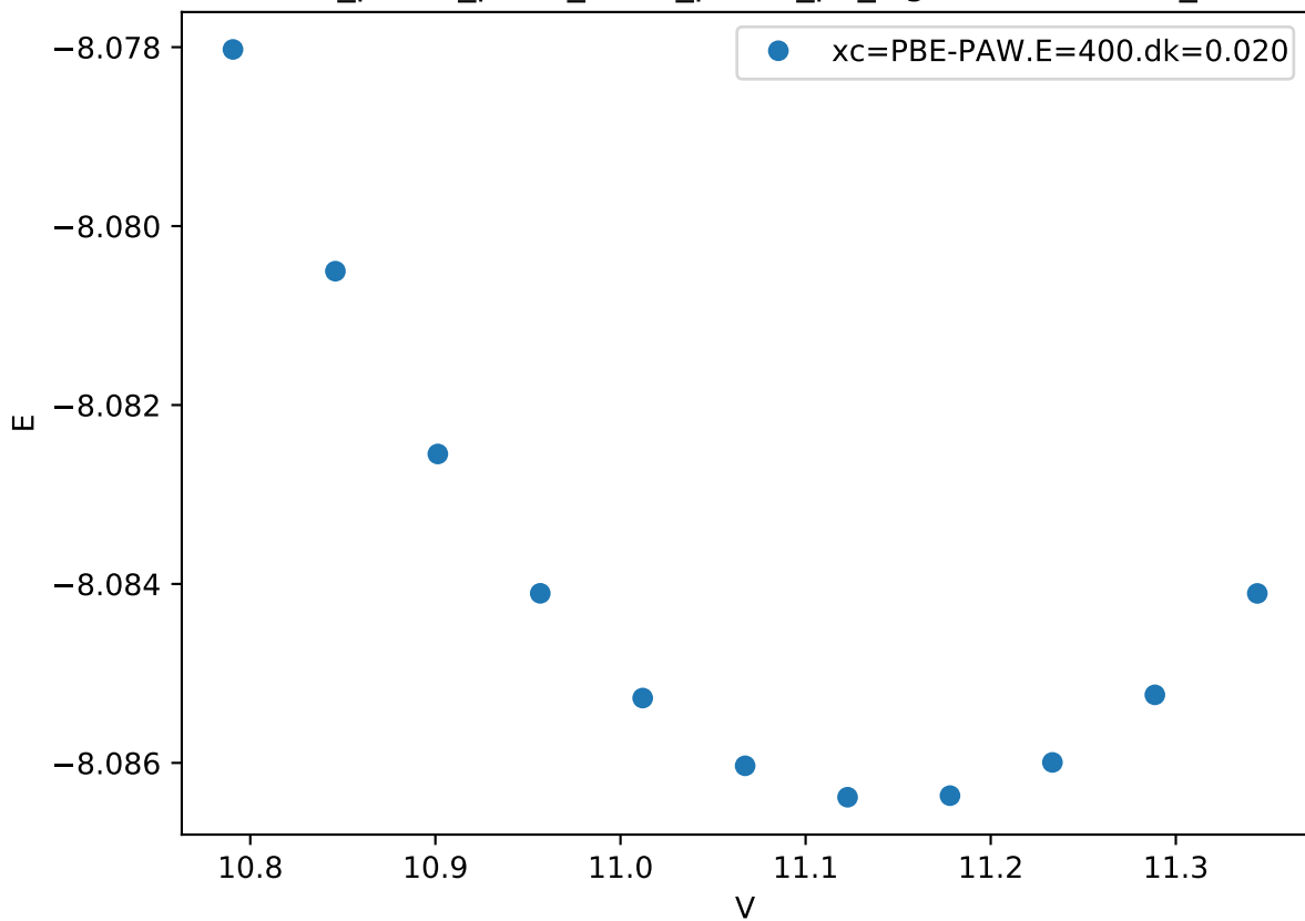
Cr_pv-Co_pv-W_sv/Cr_pv-Co_pv_sigma-AABBA.FM_
