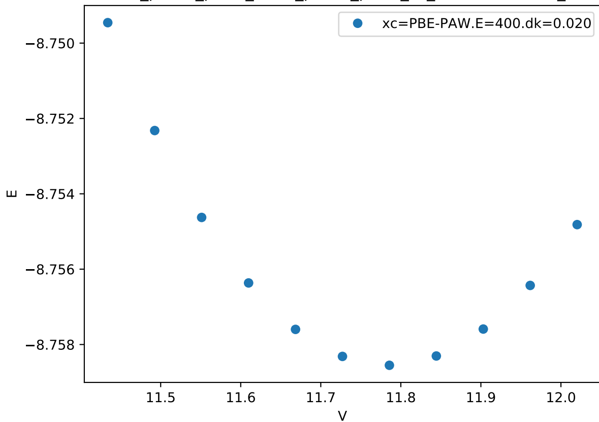
Cr_pv-Co_pv-W_sv/Cr_pv-Co_pv-W_sv_C36-CAABB.FM_
