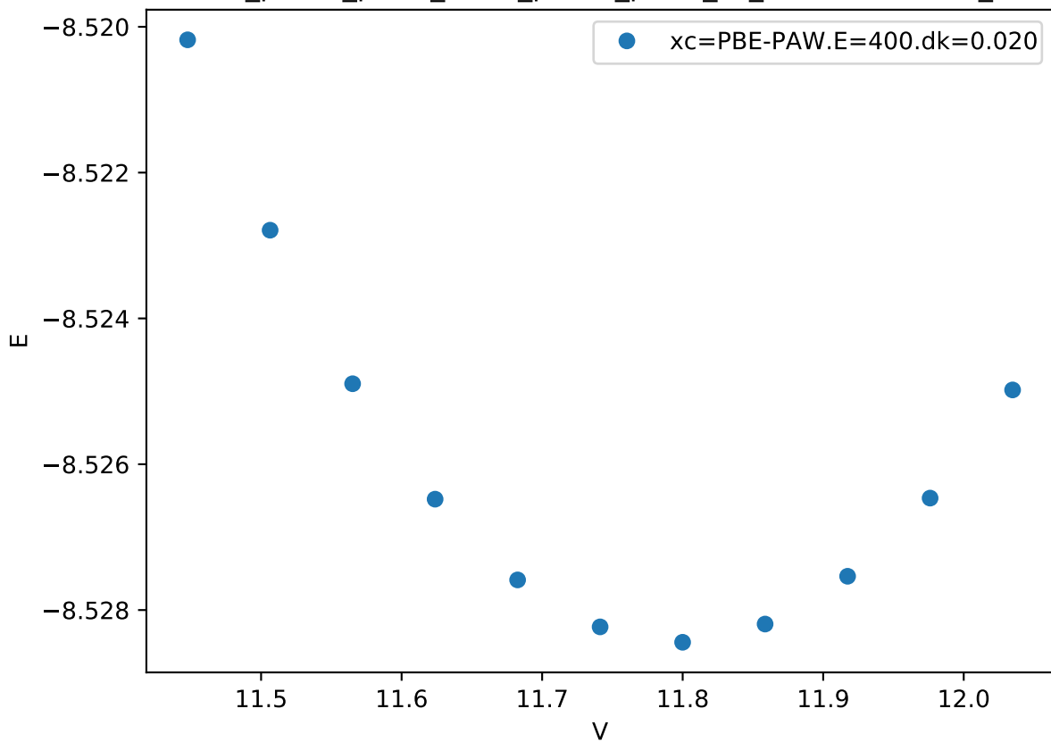
Cr_pv-Co_pv-W_sv/Cr_pv-Co_pv-W_sv_C36-CBBBA.FM_
