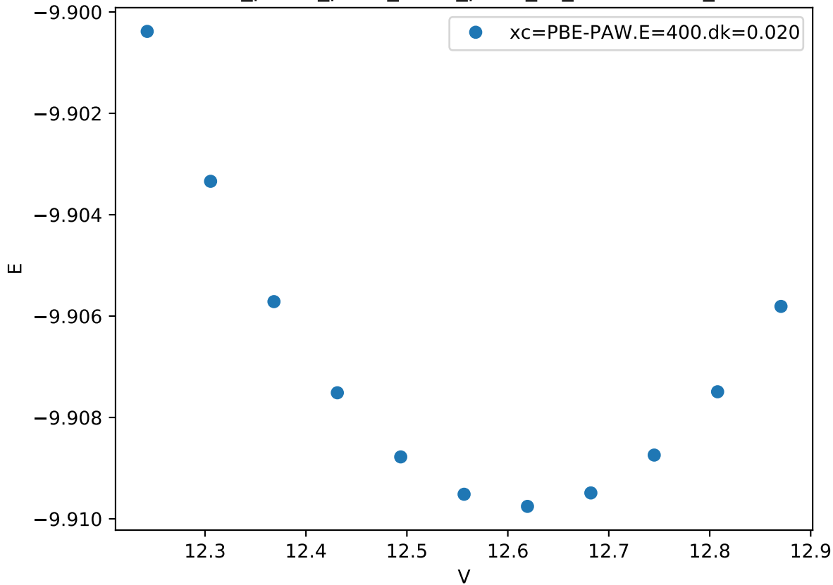
Cr_pv-Co_pv-W_sv/Cr_pv-W_sv_C36-BAAAA_
