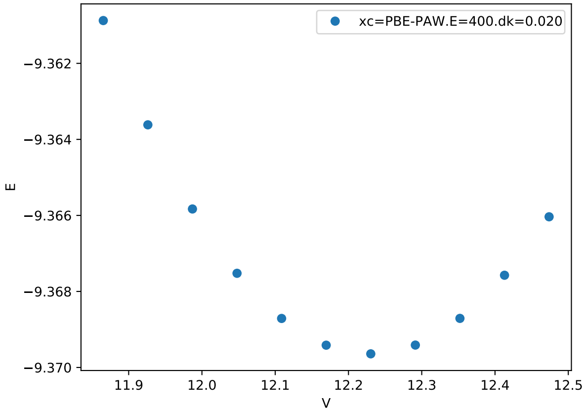
Cr_pv-Co_pv-W_sv/Cr_pv-Co_pv-W_sv_C36-ACAAB.FM_
