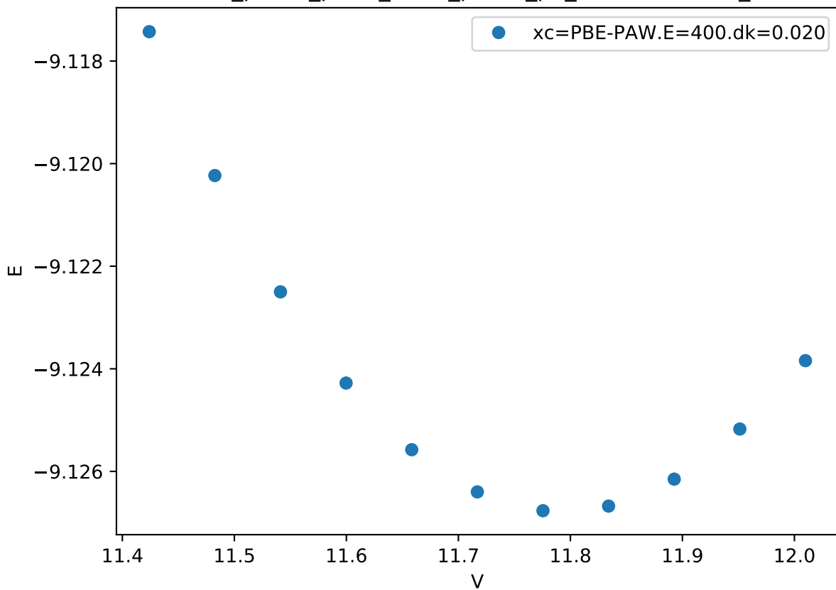
Cr_pv-Co_pv-W_sv/Cr_pv-Co_pv_mu-BAAAA.FM_
