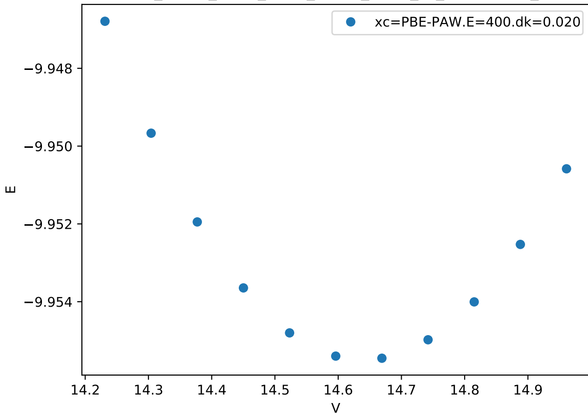
Cr_pv-Co_pv-W_sv/Cr_pv-Co_pv-W_sv_mu-BCAAB_
