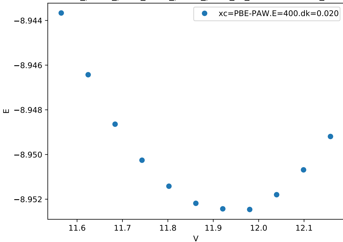
Cr_pv-Co_pv-W_sv/Cr_pv-Co_pv-W_sv_C36-ACBBA.FM_
