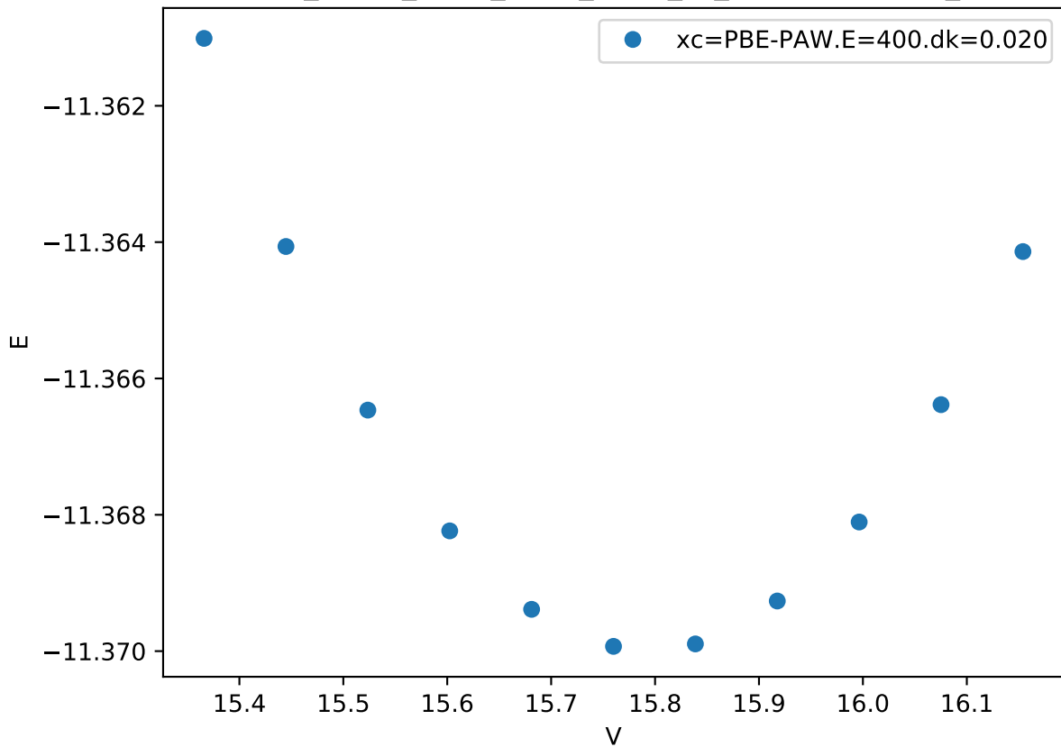
Cr_pv-Co_pv-W_sv/Cr_pv-W_sv_C36-BAABB.FM_
