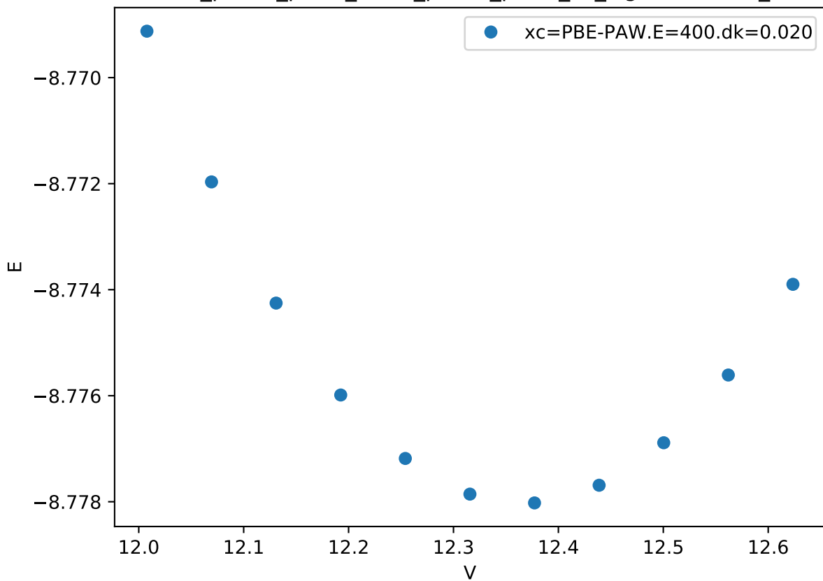
Cr_pv-Co_pv-W_sv/Cr_pv-Co_pv-W_sv_sigma-BABCB_
