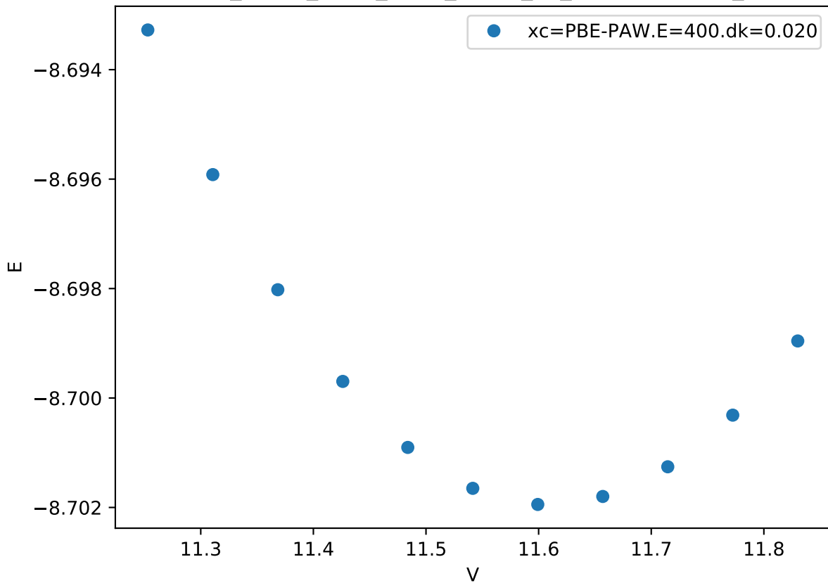
Cr_pv-Co_pv-W_sv/Cr_pv-Co_pv_mu-BABAA.FM_
