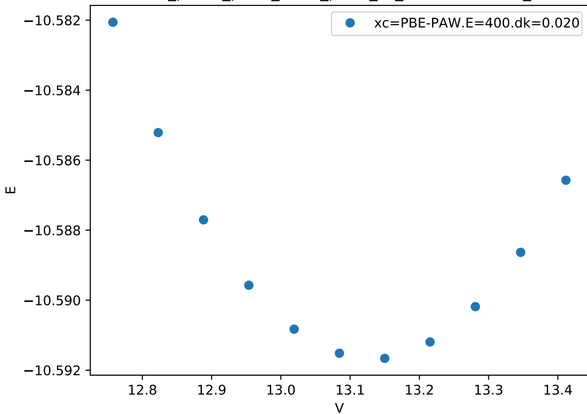
Cr_pv-Co_pv-W_sv/Cr_pv-W_sv_C36-BBAAA.FM_
