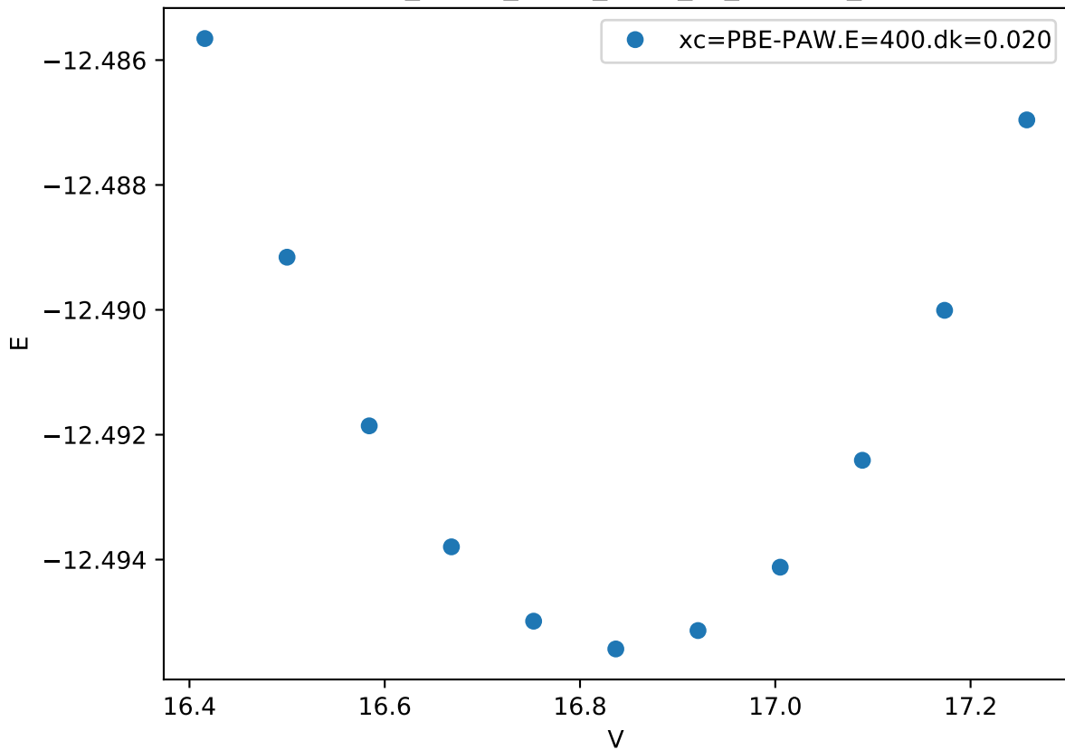
Cr_pv-Co_pv-W_sv/W_sv_C15.FM_
