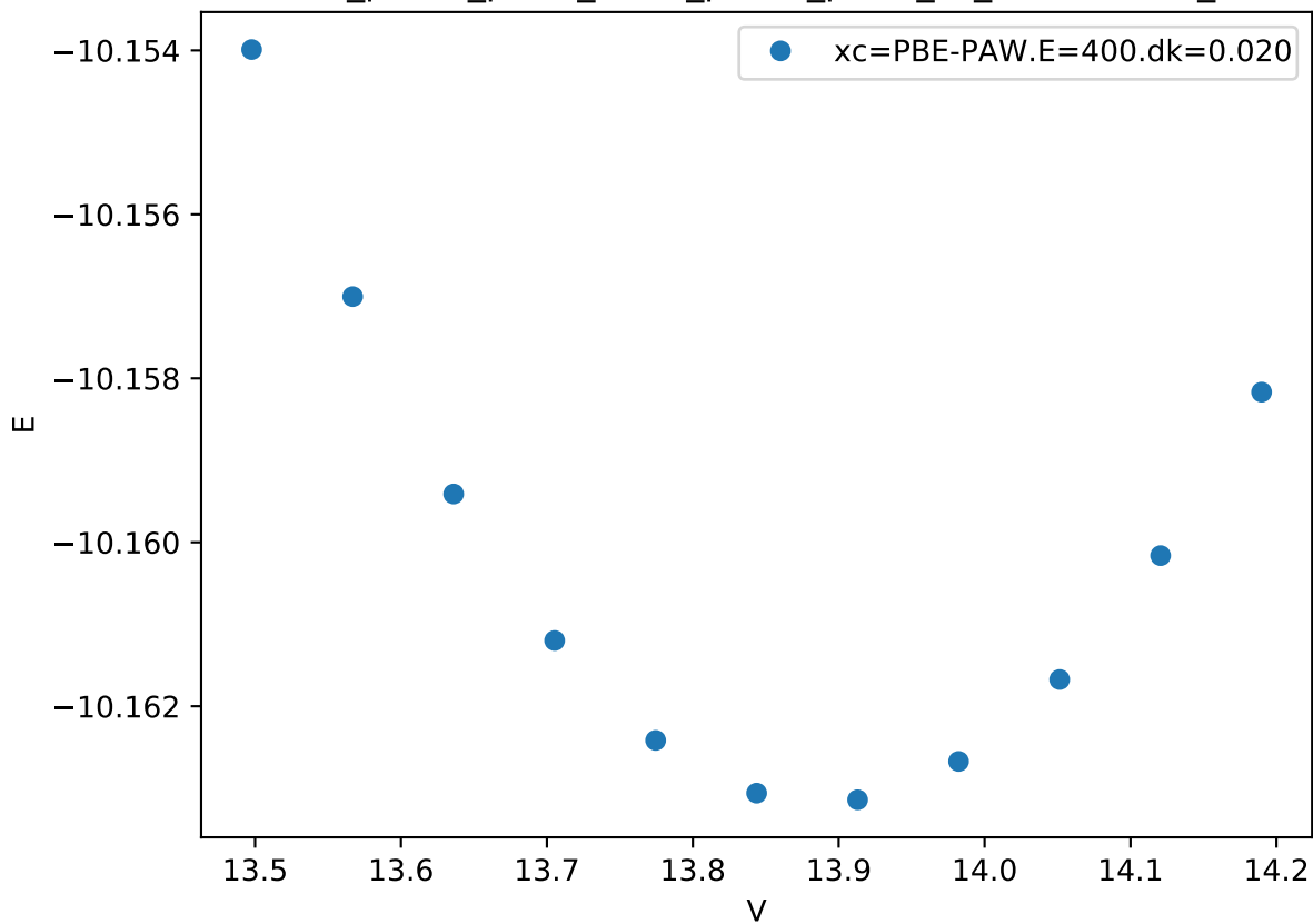
Cr_pv-Co_pv-W_sv/Cr_pv-Co_pv-W_sv_C36-ACBCA_
