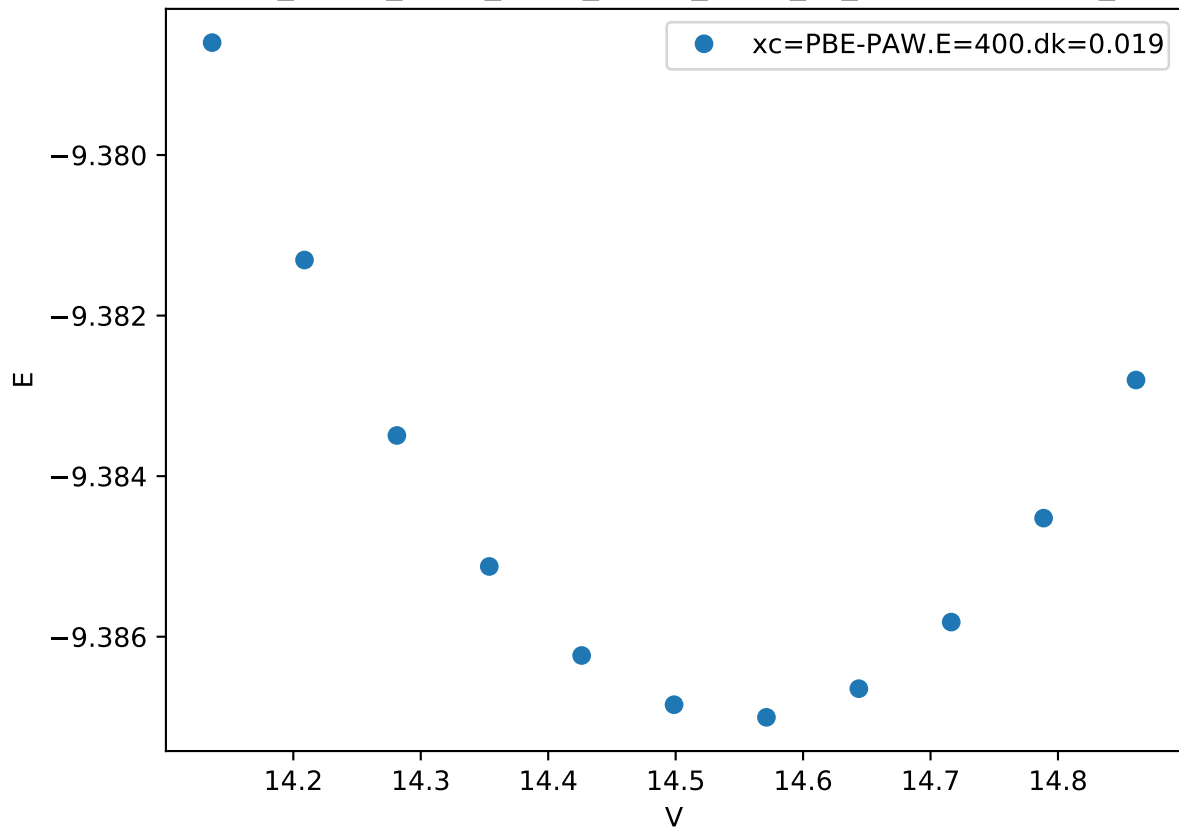
Cr_pv-Co_pv-W_sv/Cr_pv-Co_pv-W_sv_C36-BBCAC.FM_
