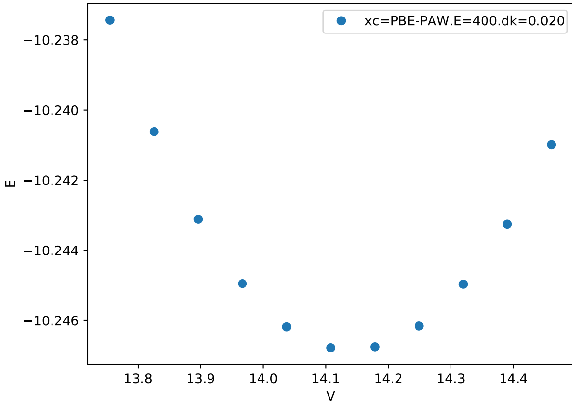
Cr_pv-Co_pv-W_sv/Co_pv-W_sv_chi-BBAB_
