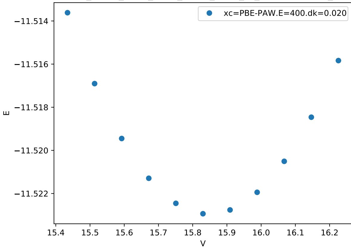
Cr_pv-Co_pv-W_sv/Cr_pv-Co_pv-W_sv_mu-BCACC.FM_
