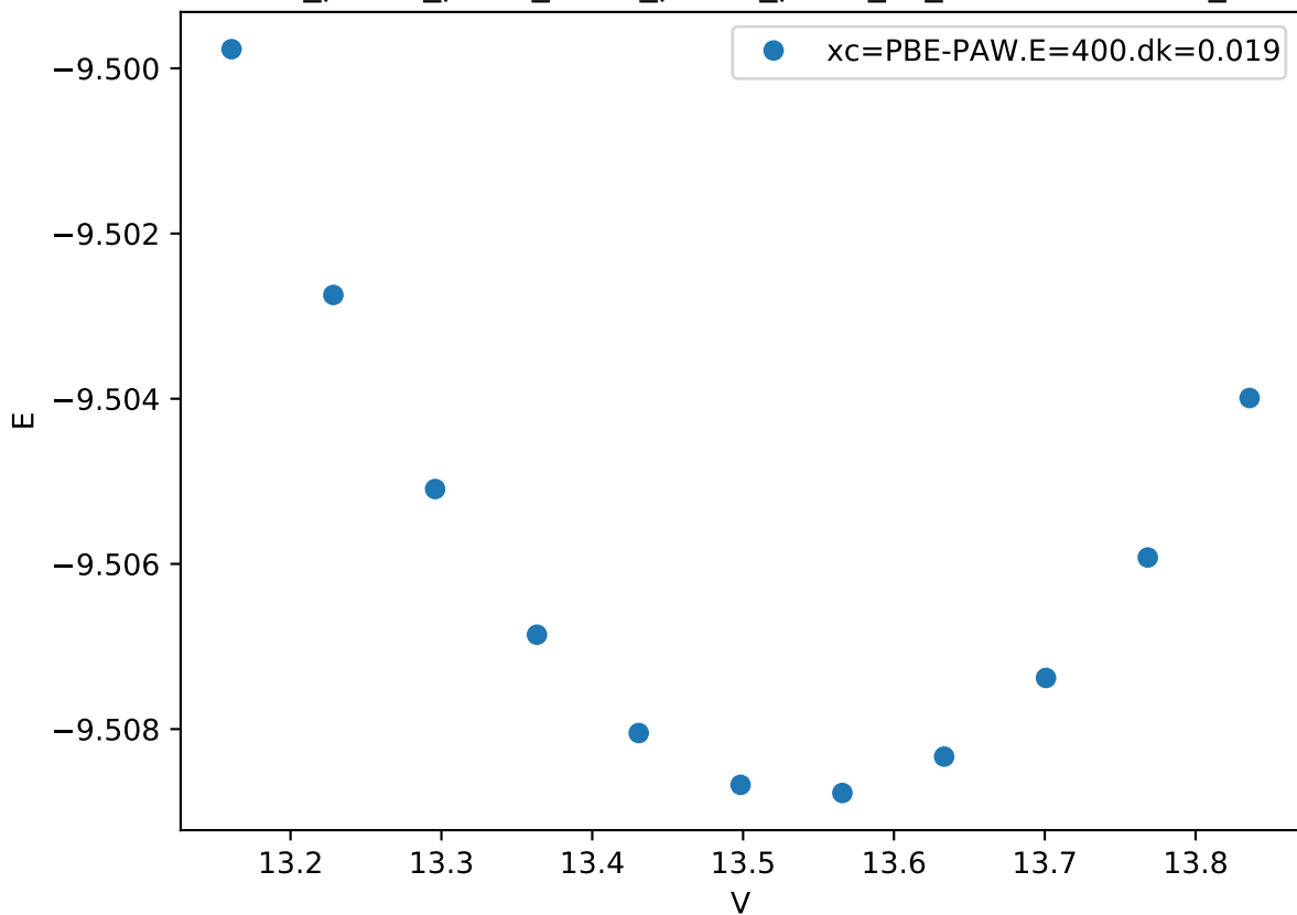
Cr_pv-Co_pv-W_sv/Cr_pv-Co_pv-W_sv_C36-ACBCB.FM_
