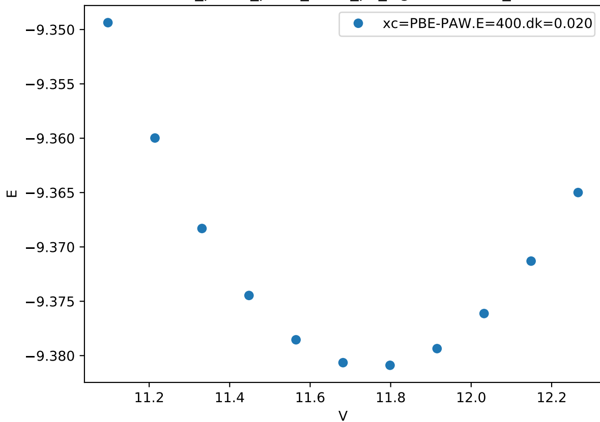
Cr_pv-Co_pv-W_sv/Cr_pv_sigma.UDUDD_
