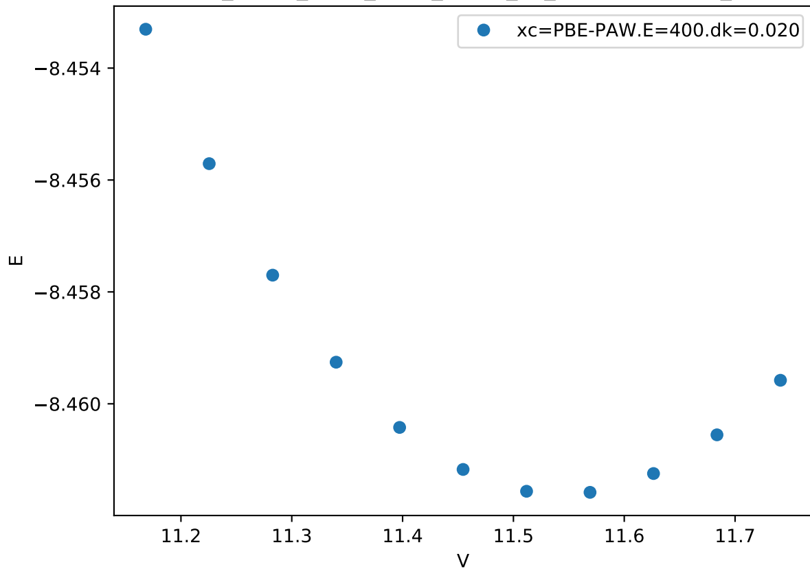
Cr_pv-Co_pv-W_sv/Cr_pv-Co_pv_C36-ABBAA.FM_
