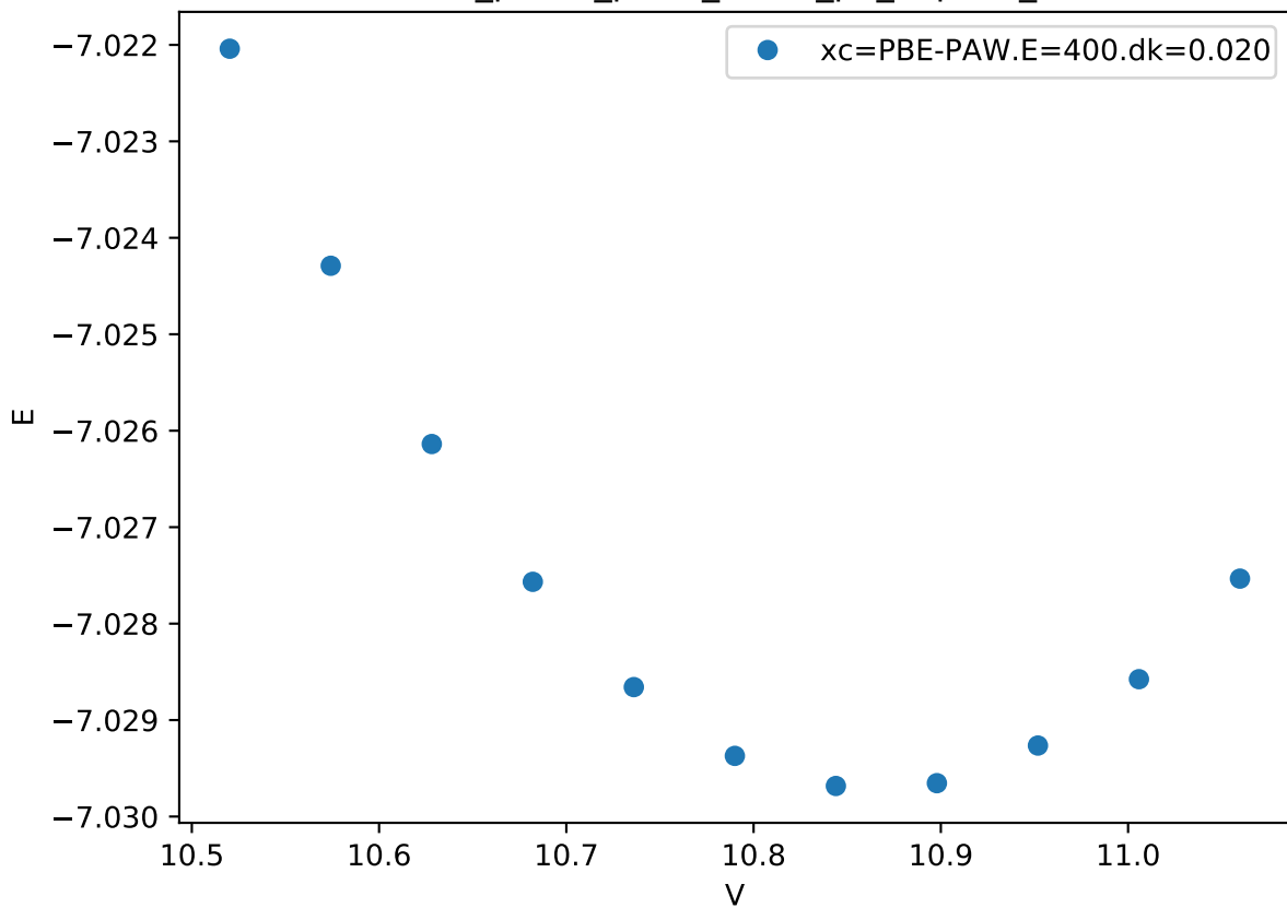
Cr_pv-Co_pv-W_sv/Co_pv_hcp.FM_
