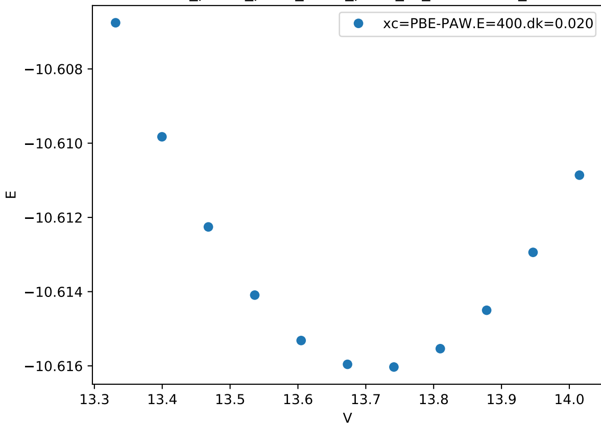
Cr_pv-Co_pv-W_sv/Cr_pv-W_sv_mu-BAABB_
