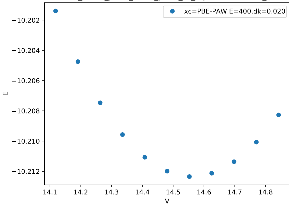
Cr_pv-Co_pv-W_sv/Co_pv-W_sv_sigma-BAABB.FM_
