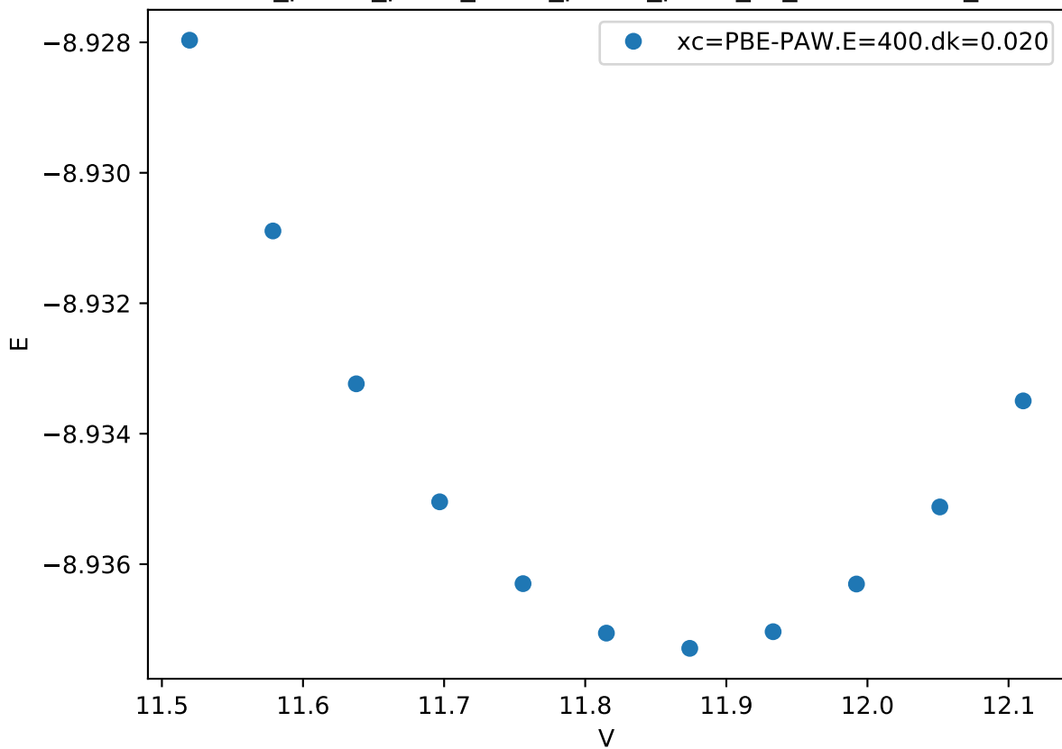
Cr_pv-Co_pv-W_sv/Cr_pv-Co_pv-W_sv_C36-ACBAB_
