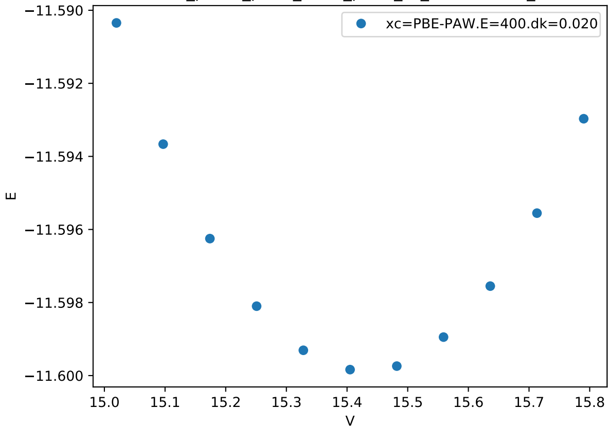
Cr_pv-Co_pv-W_sv/Cr_pv-W_sv_L12-AB3.FM_
