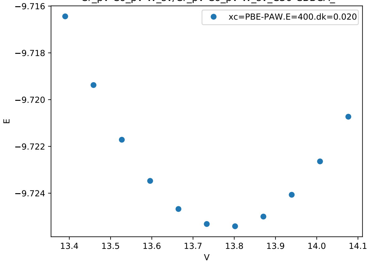
Cr_pv-Co_pv-W_sv/Cr_pv-Co_pv-W_sv_C36-CBBCA_
