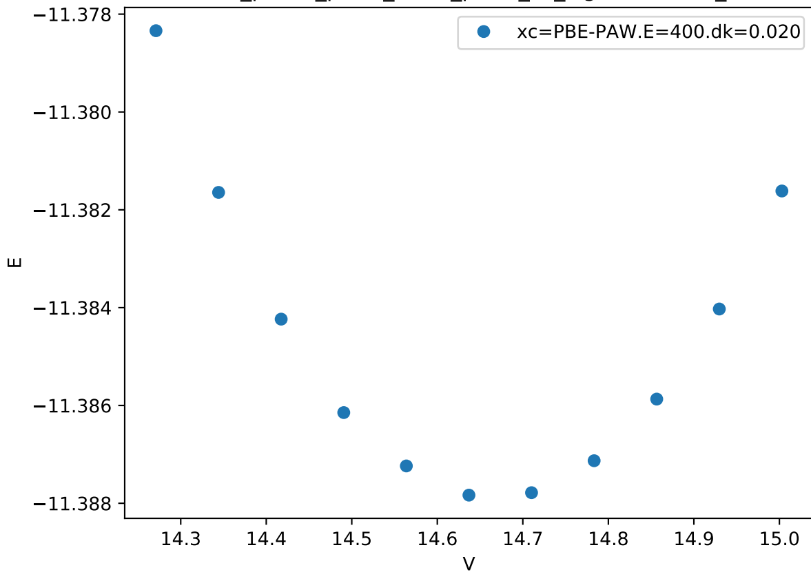
Cr_pv-Co_pv-W_sv/Cr_pv-W_sv_sigma-BABAB_
