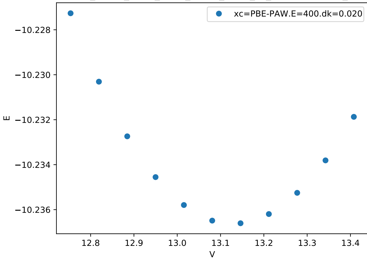
Cr_pv-Co_pv-W_sv/Cr_pv-Co_pv-W_sv_mu-BAACC.FM_
