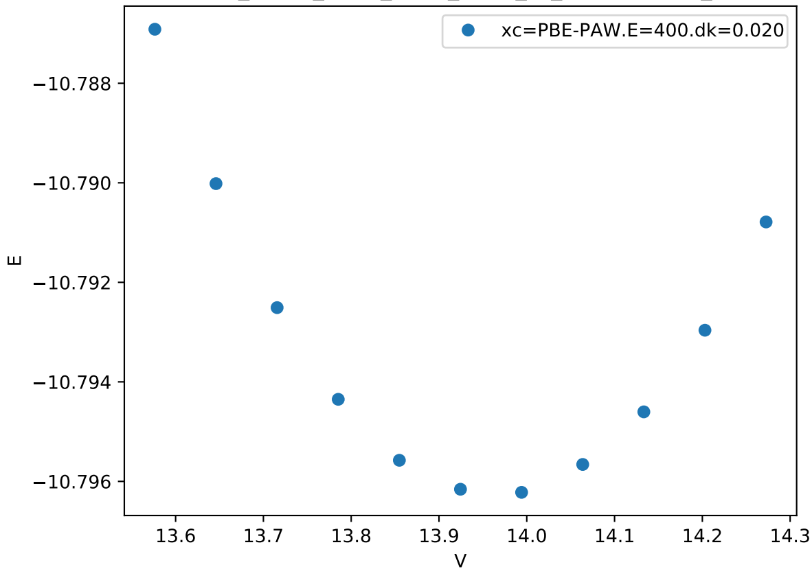
Cr_pv-Co_pv-W_sv/Cr_pv-W_sv_chi-BABA.FM_
