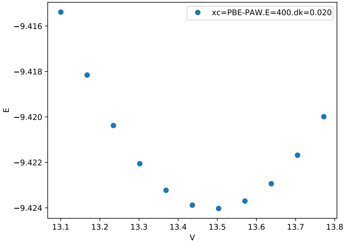
Cr_pv-Co_pv-W_sv/Cr_pv-Co_pv-W_sv_C36-AABAC_
