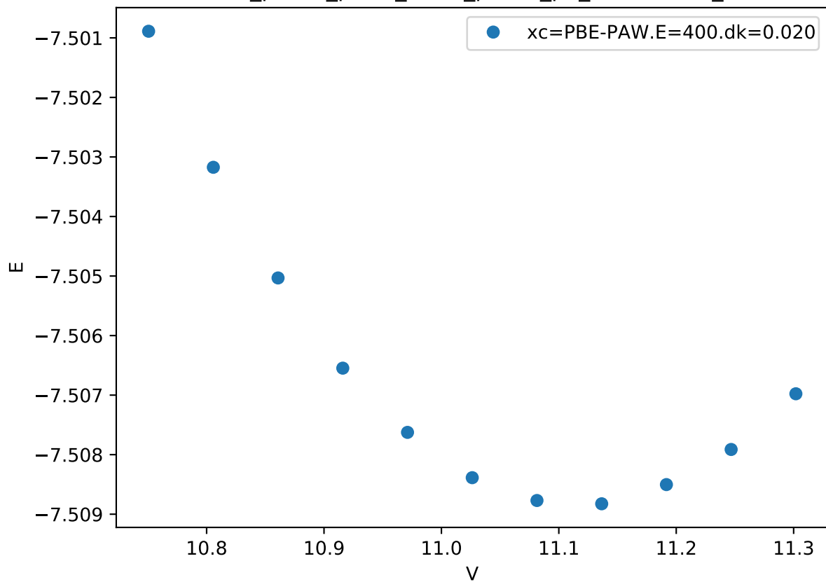
Cr_pv-Co_pv-W_sv/Cr_pv-Co_pv_A15-BA.FM_
