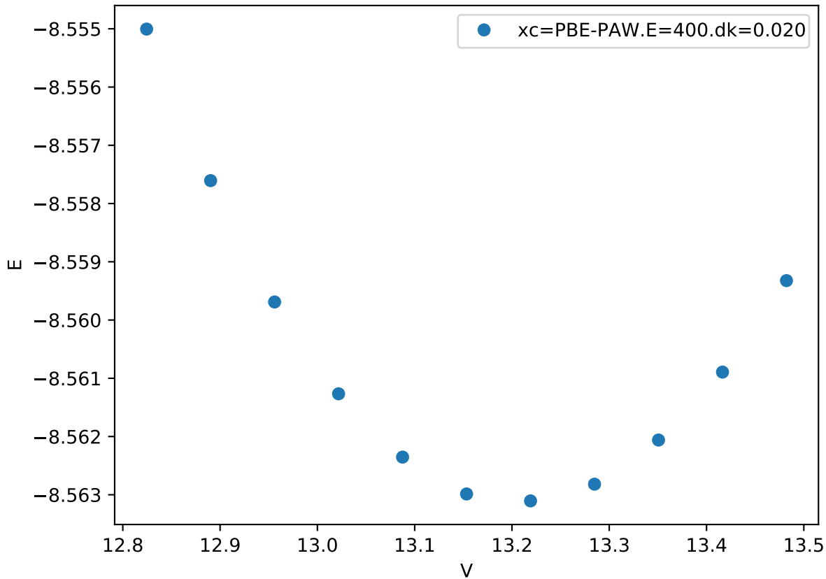
Cr_pv-Co_pv-W_sv/Cr_pv-Co_pv-W_sv_C36-BBBAC.FM_
