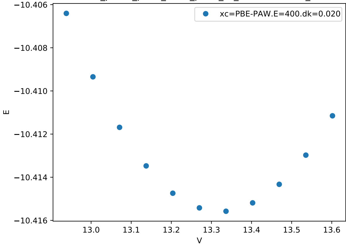
Cr_pv-Co_pv-W_sv/Cr_pv-W_sv_mu-AABAB.FM_
