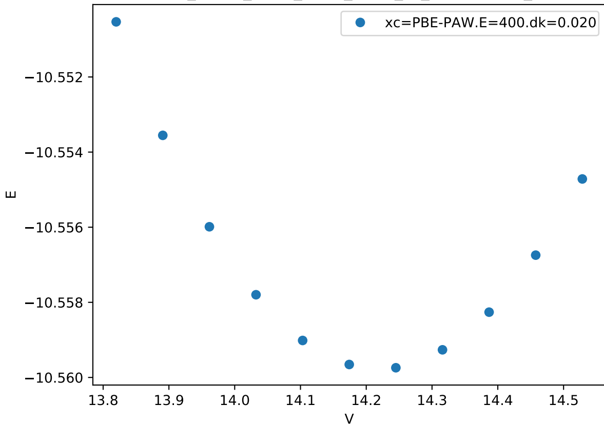
Cr_pv-Co_pv-W_sv/Cr_pv-W_sv_C36-BAABA_
