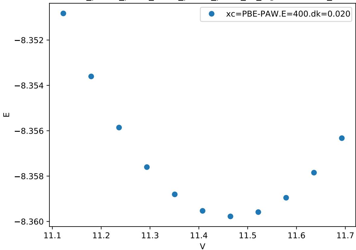
Cr_pv-Co_pv-W_sv/Cr_pv-Co_pv-W_sv_sigma-BCABB_
