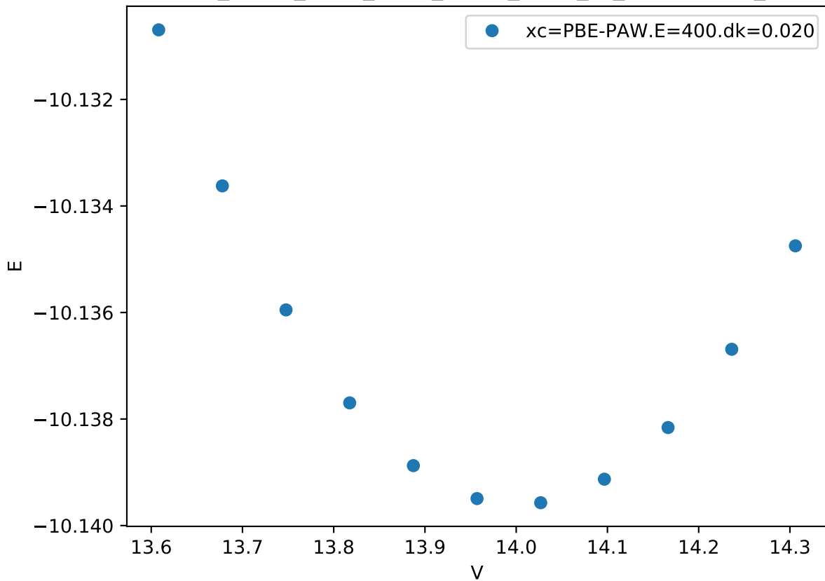
Cr_pv-Co_pv-W_sv/Cr_pv-Co_pv-W_sv_C36-CBAAC_
