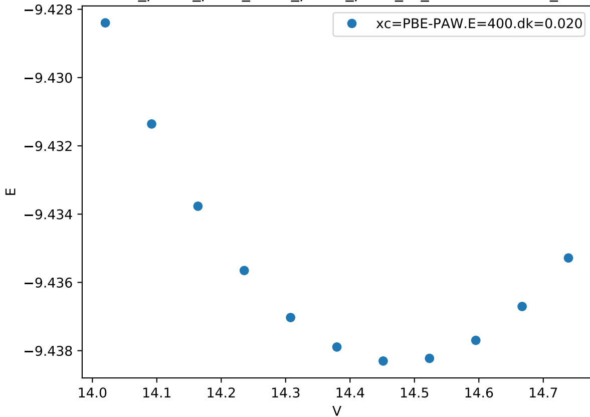
Cr_pv-Co_pv-W_sv/Cr_pv-Co_pv-W_sv_C36-BBCCA.FM_
