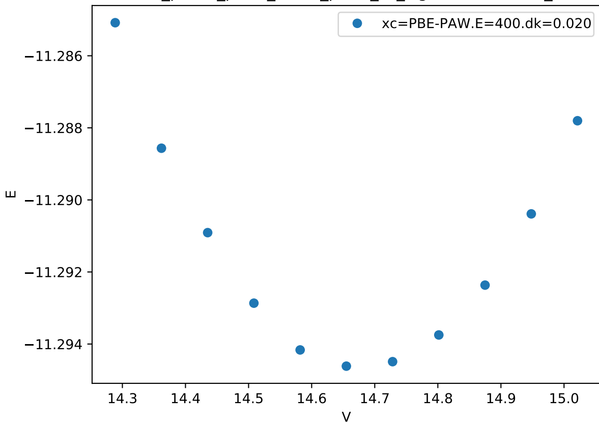
Cr_pv-Co_pv-W_sv/Co_pv-W_sv_sigma-BBBAB.FM_
