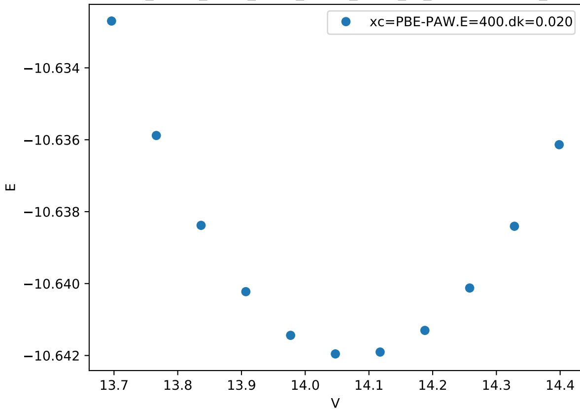
Cr_pv-Co_pv-W_sv/Cr_pv-Co_pv-W_sv_sigma-BBCAC_
