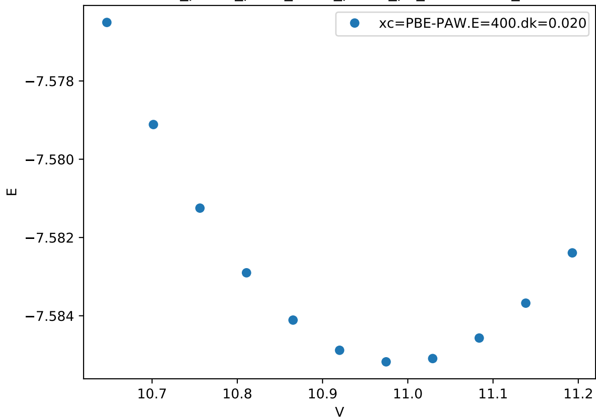
Cr_pv-Co_pv-W_sv/Cr_pv-Co_pv_mu-BBABA_
