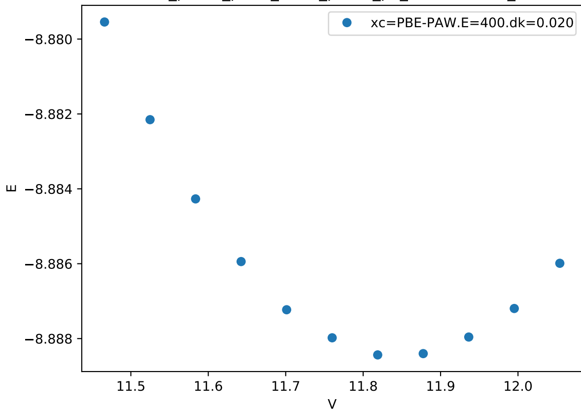
Cr_pv-Co_pv-W_sv/Cr_pv-Co_pv_chi-ABAA.FM_
