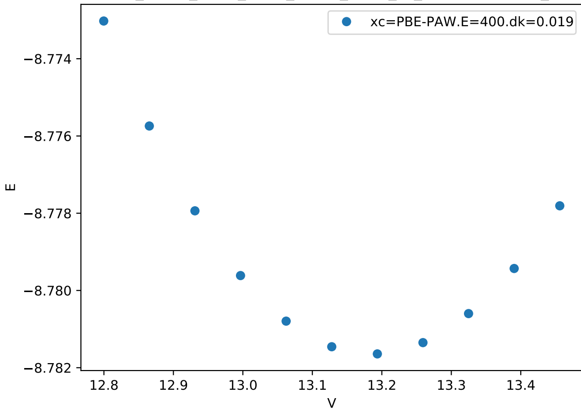
Cr_pv-Co_pv-W_sv/Cr_pv-Co_pv-W_sv_C36-AABBC.FM_
