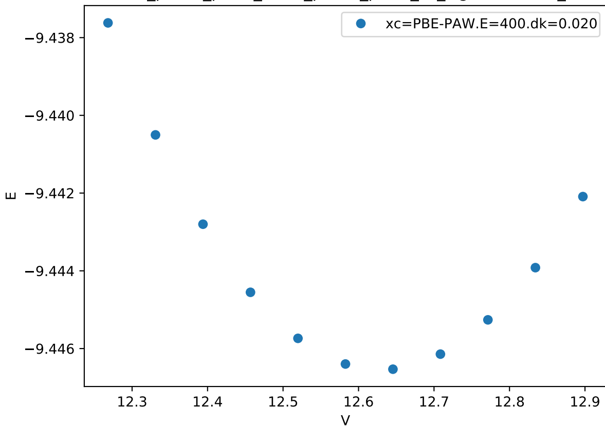
Cr_pv-Co_pv-W_sv/Cr_pv-Co_pv-W_sv_sigma-BAABC_
