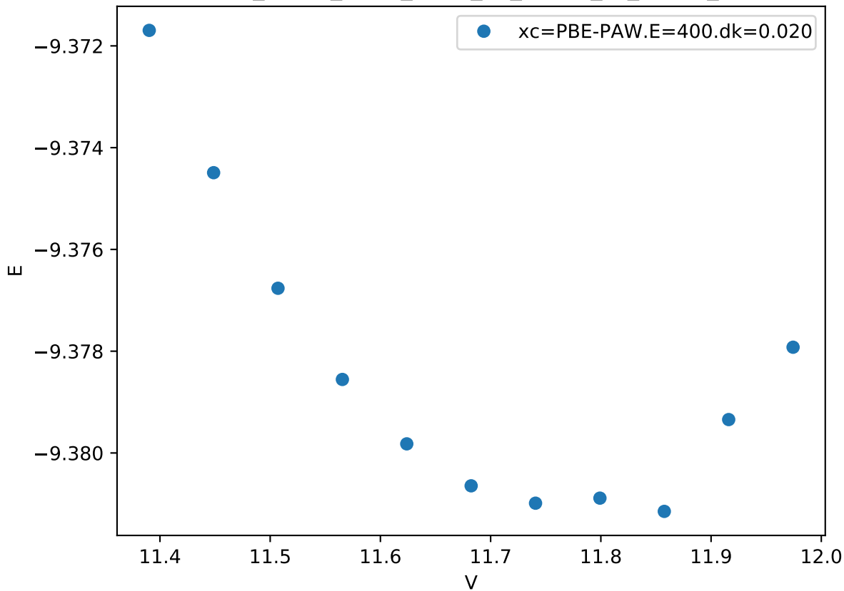
Cr_pv-Co_pv-W_sv/Cr_pv_sigma_Cr_pv.FM_
