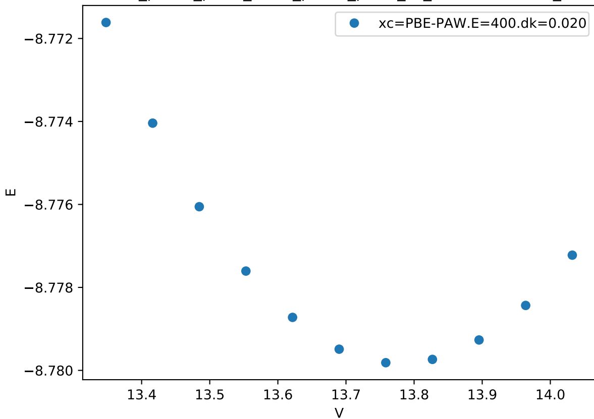
Cr_pv-Co_pv-W_sv/Cr_pv-Co_pv-W_sv_C36-BAABC.FM_
