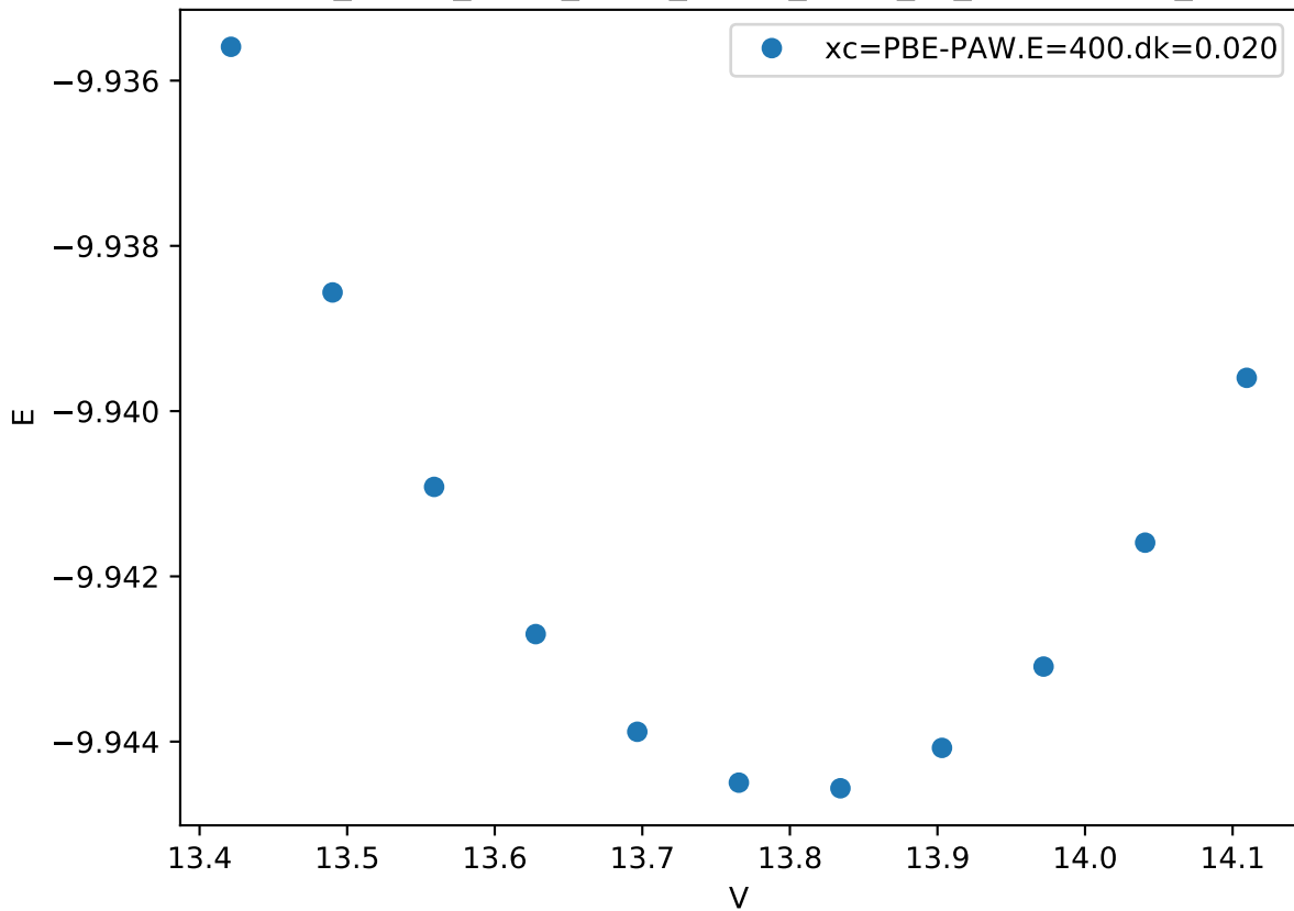
Cr_pv-Co_pv-W_sv/Cr_pv-Co_pv-W_sv_C36-ACACB_
