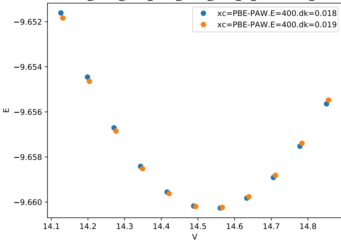
Cr_pv-Co_pv-W_sv/Cr_pv-Co_pv-W_sv_C36-AACBC_
