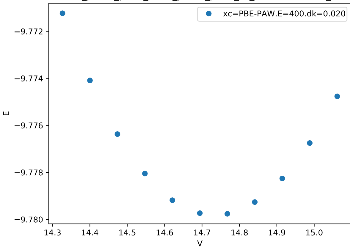
Cr_pv-Co_pv-W_sv/Cr_pv-Co_pv-W_sv_C36-BABCC.FM_
