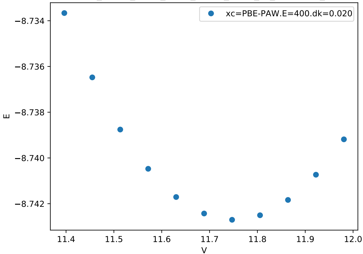
Cr_pv-Co_pv-W_sv/Cr_pv-Co_pv-W_sv_chi-BCBA_
