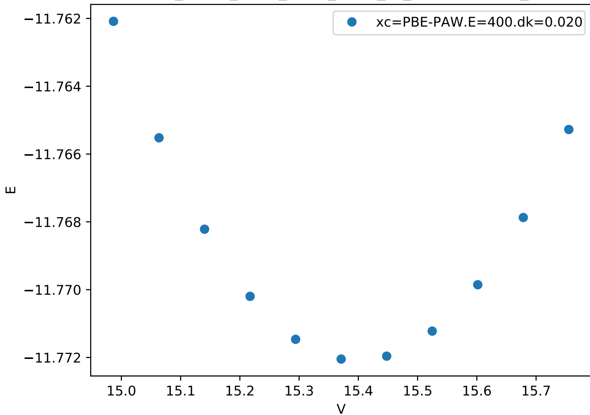
Cr_pv-Co_pv-W_sv/Cr_pv-W_sv_sigma-BBABB_
