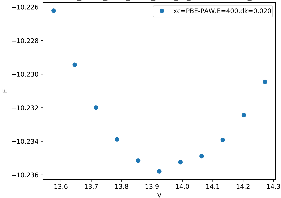
Cr_pv-Co_pv-W_sv/Co_pv-W_sv_C36-BBAAB.FM_
