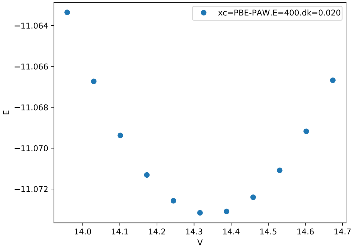
Cr_pv-Co_pv-W_sv/Cr_pv-Co_pv-W_sv_sigma-ACCBC_
