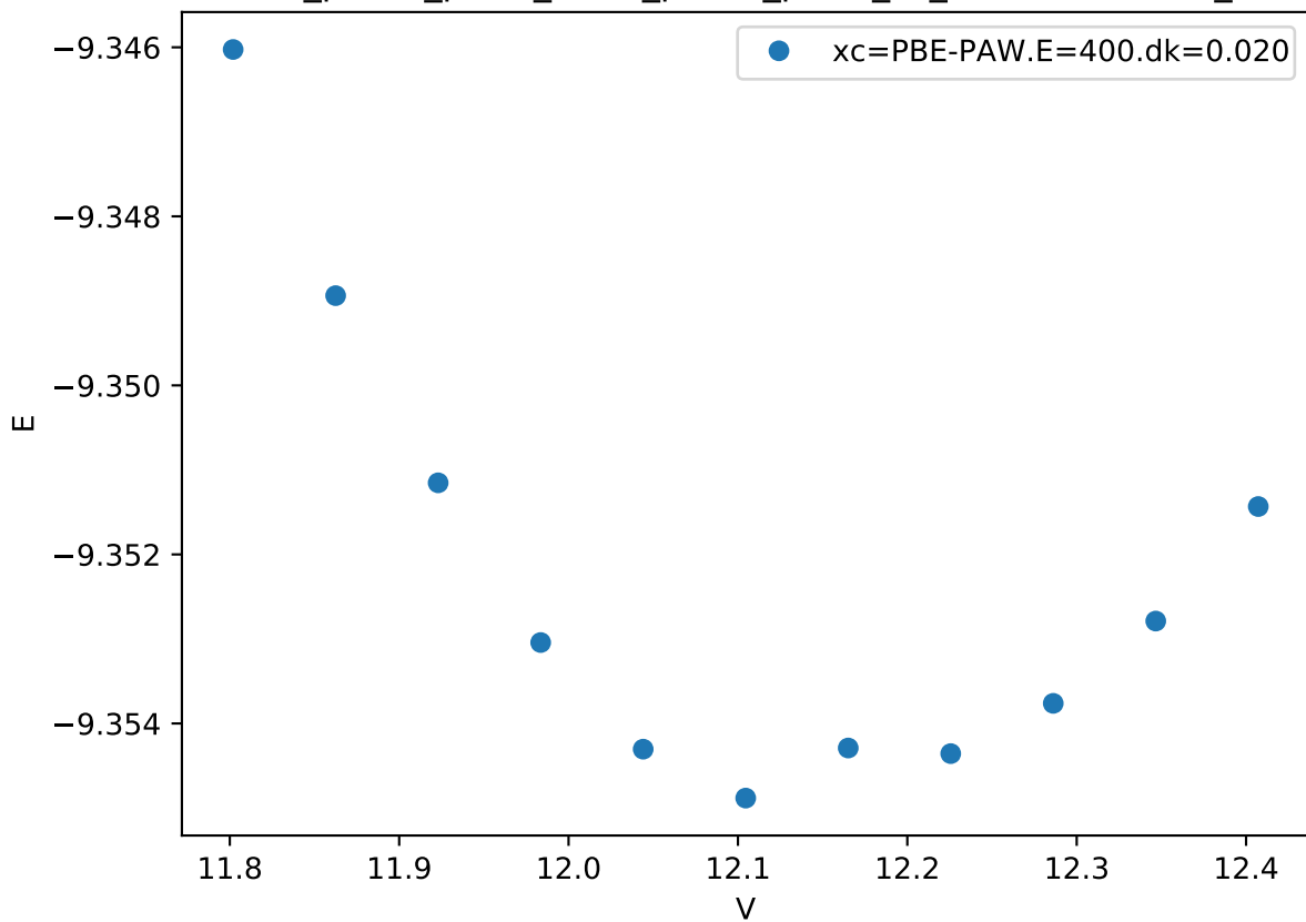
Cr_pv-Co_pv-W_sv/Cr_pv-Co_pv-W_sv_C36-CAAAB.FM_
