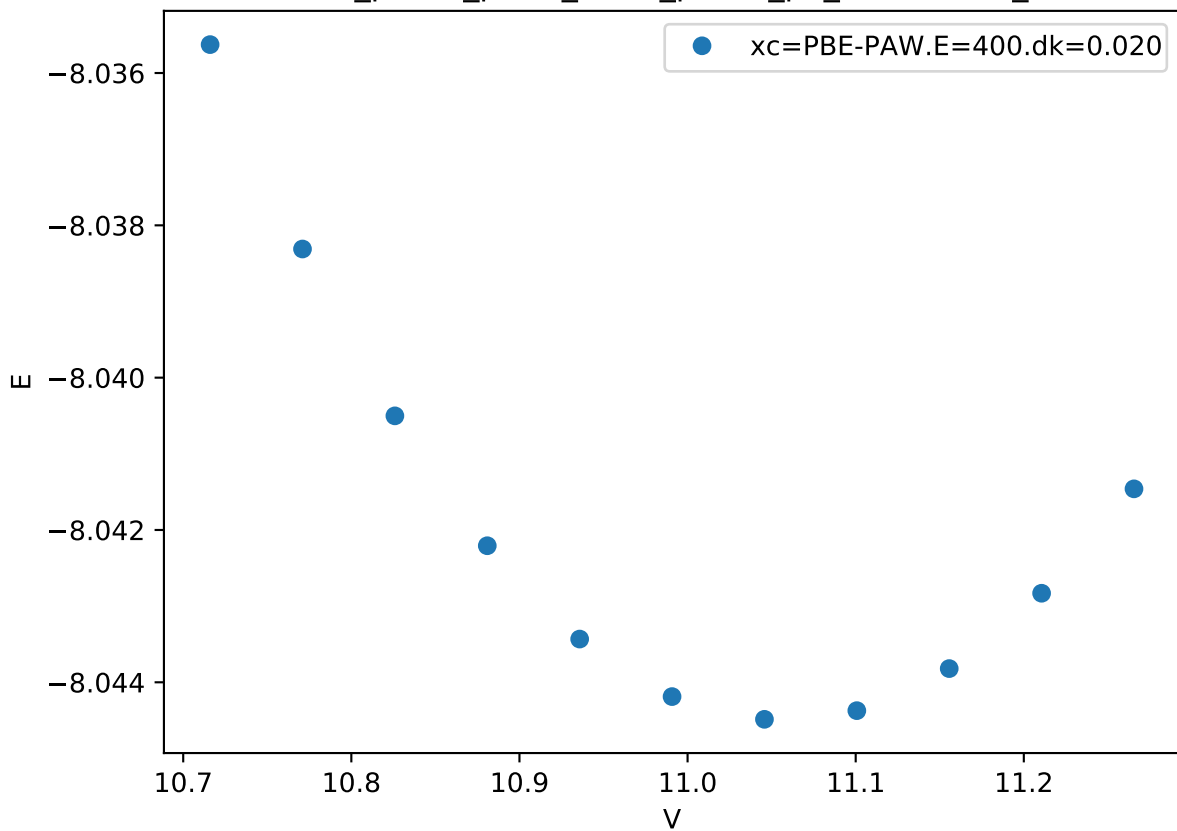
Cr_pv-Co_pv-W_sv/Cr_pv-Co_pv_mu-BBAAA_
