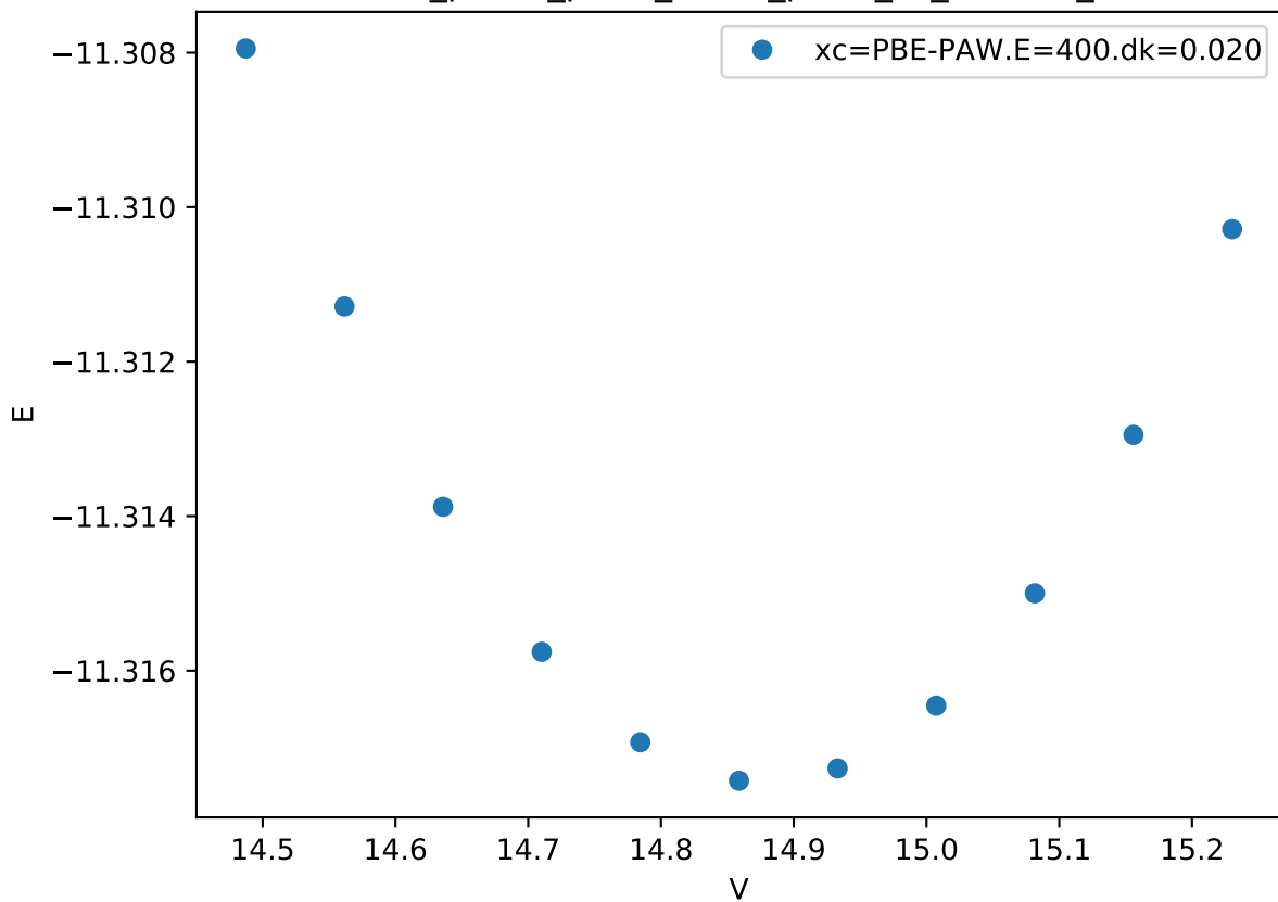
Cr_pv-Co_pv-W_sv/Co_pv-W_sv_A15-BA_
