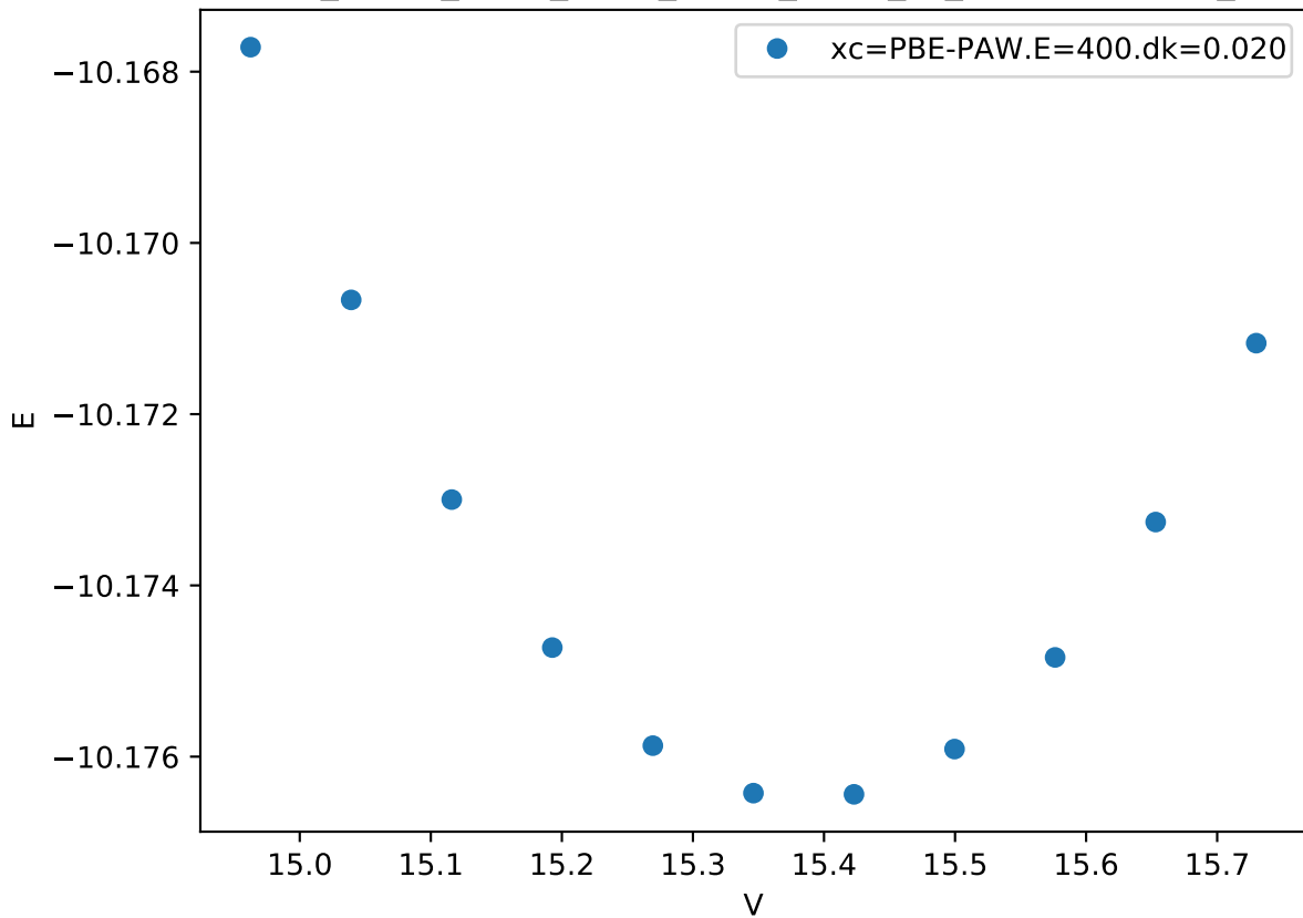
Cr_pv-Co_pv-W_sv/Cr_pv-Co_pv-W_sv_mu-ACBBC.FM_
