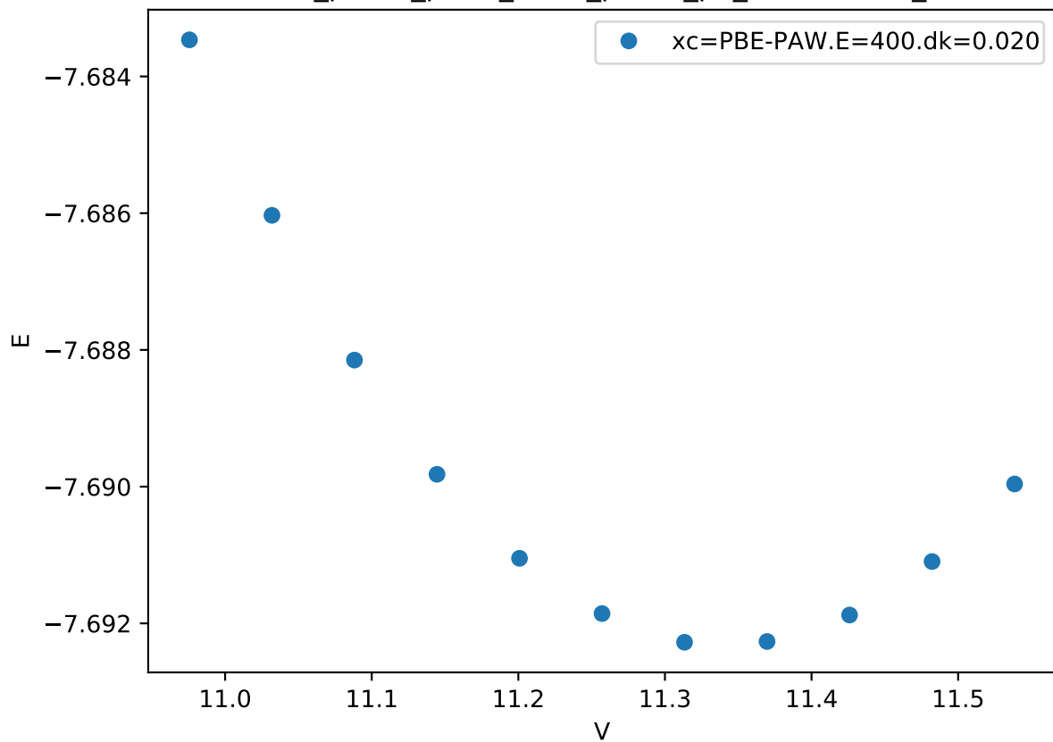
Cr_pv-Co_pv-W_sv/Cr_pv-Co_pv_C36-BBABA_
