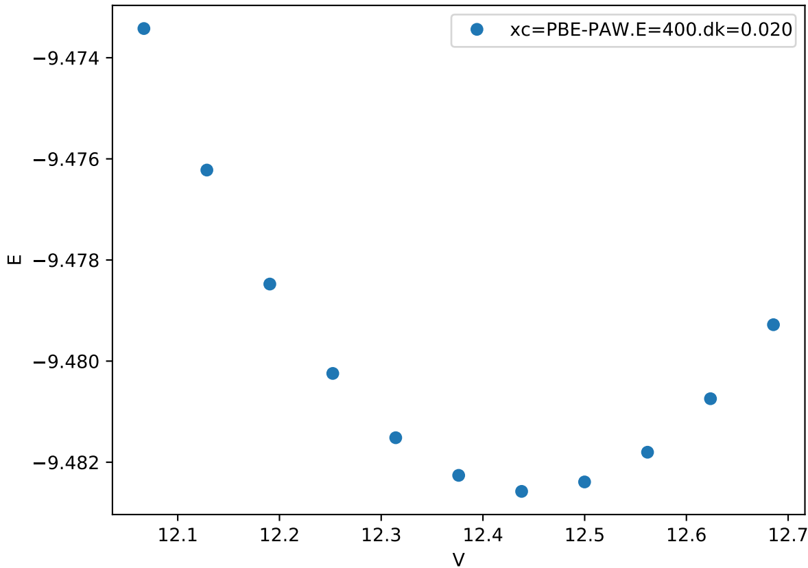
Cr_pv-Co_pv-W_sv/Cr_pv-W_sv_mu-BAAAA_
