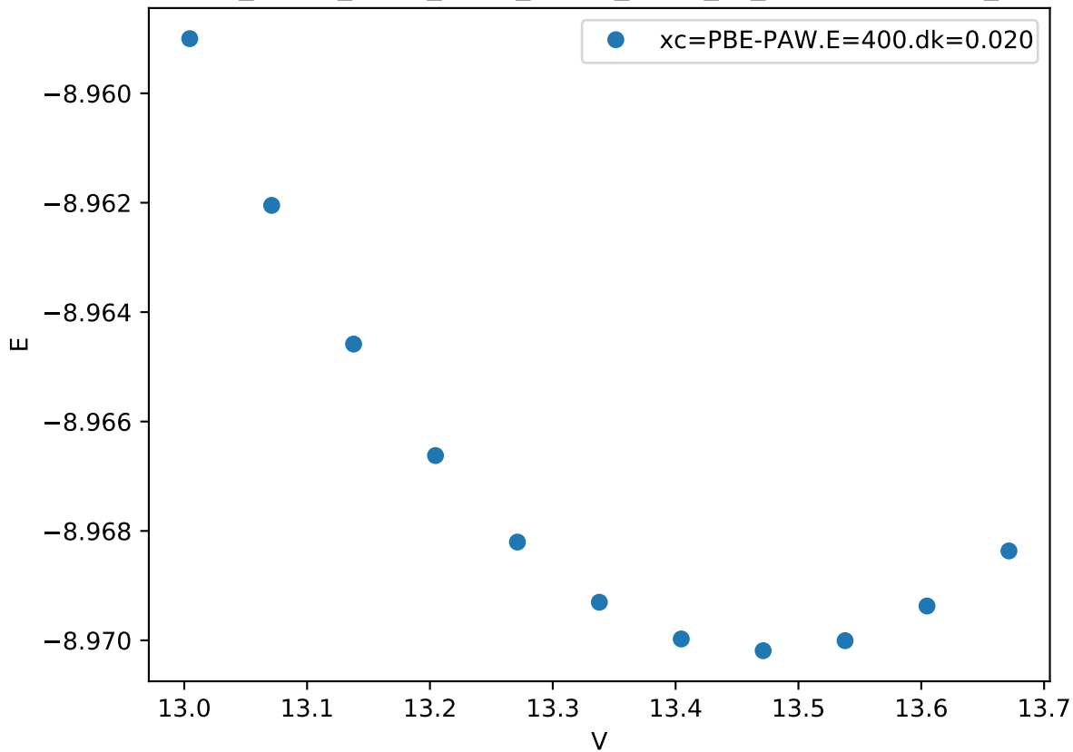
Cr_pv-Co_pv-W_sv/Cr_pv-Co_pv-W_sv_C36-BBAAC.FM_
