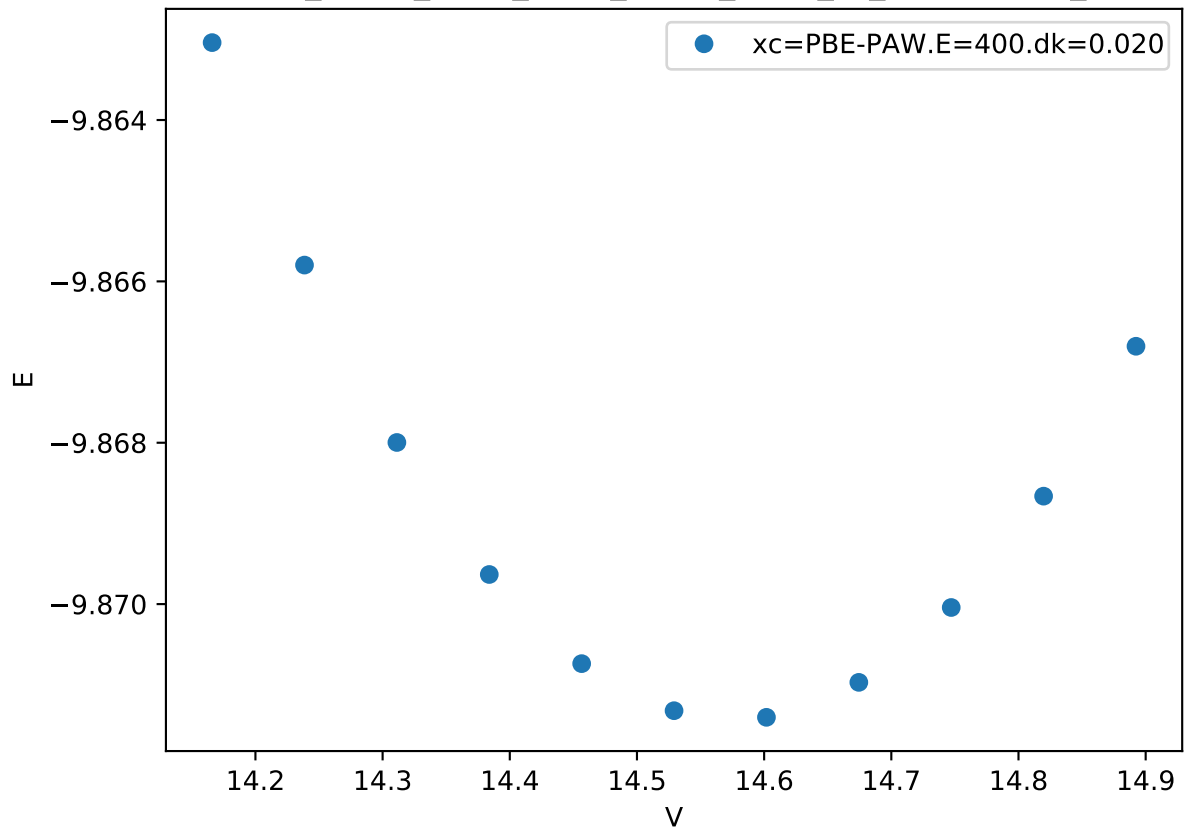
Cr_pv-Co_pv-W_sv/Cr_pv-Co_pv-W_sv_C36-ABCCA_
