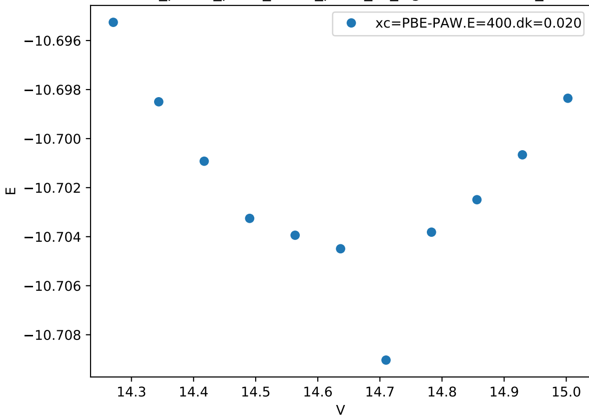
Cr_pv-Co_pv-W_sv/Co_pv-W_sv_sigma-ABBBA.FM_
