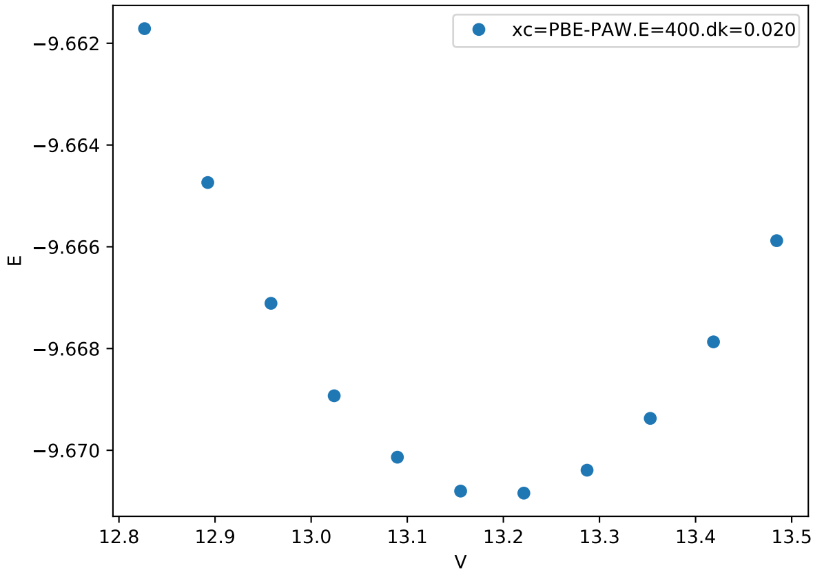
Cr_pv-Co_pv-W_sv/Cr_pv-Co_pv-W_sv_chi-AACB.FM_
