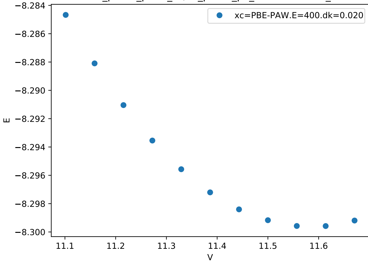
Cr_pv-Co_pv-W_sv/Cr_pv-Co_pv_mu-BABBA.FM_
