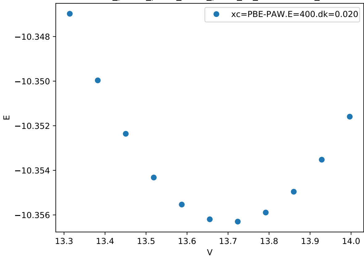
Cr_pv-Co_pv-W_sv/Cr_pv-W_sv_C36-ABBAA_
