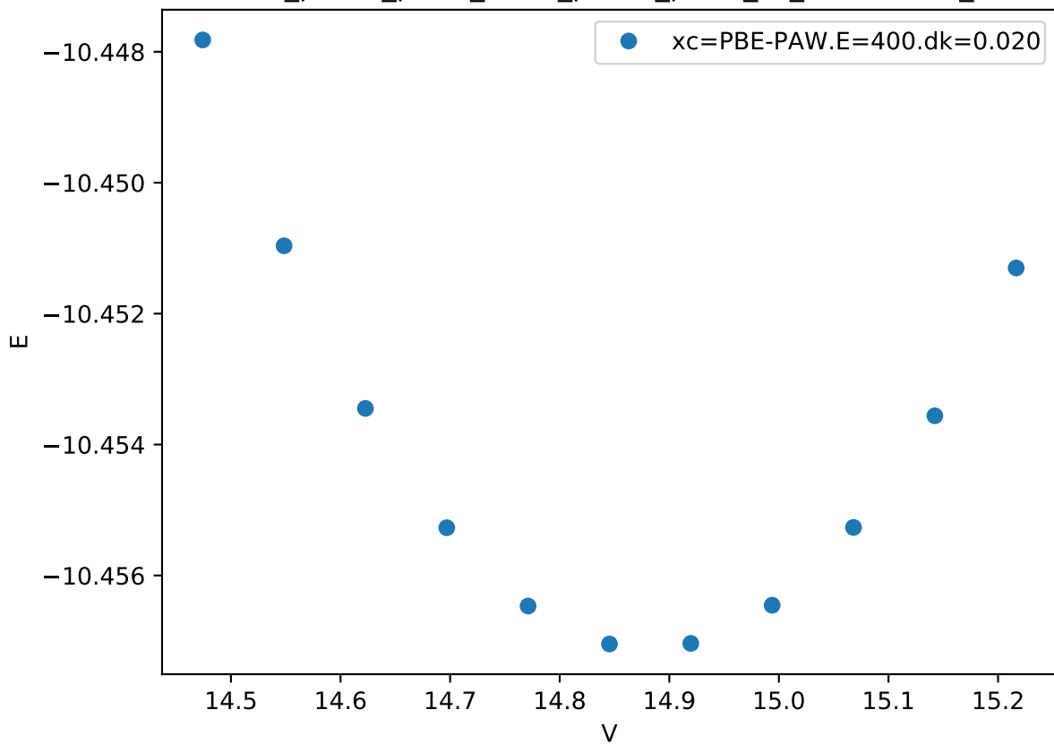
Cr_pv-Co_pv-W_sv/Cr_pv-Co_pv-W_sv_mu-ACBCB_
