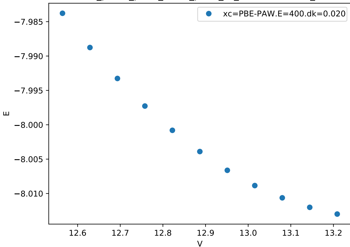
Cr_pv-Co_pv-W_sv/Co_pv-W_sv_C36-AAABA.FM_
