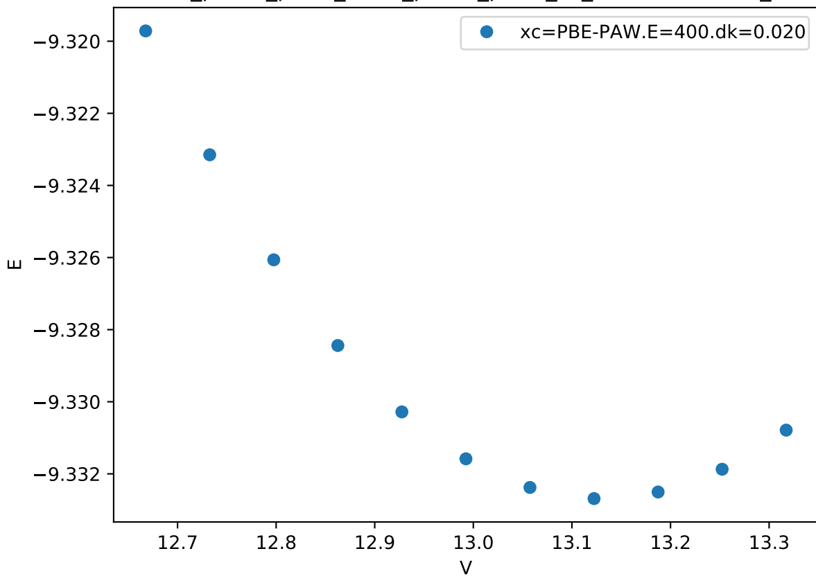
Cr_pv-Co_pv-W_sv/Cr_pv-Co_pv-W_sv_C36-CBCBA.FM_
