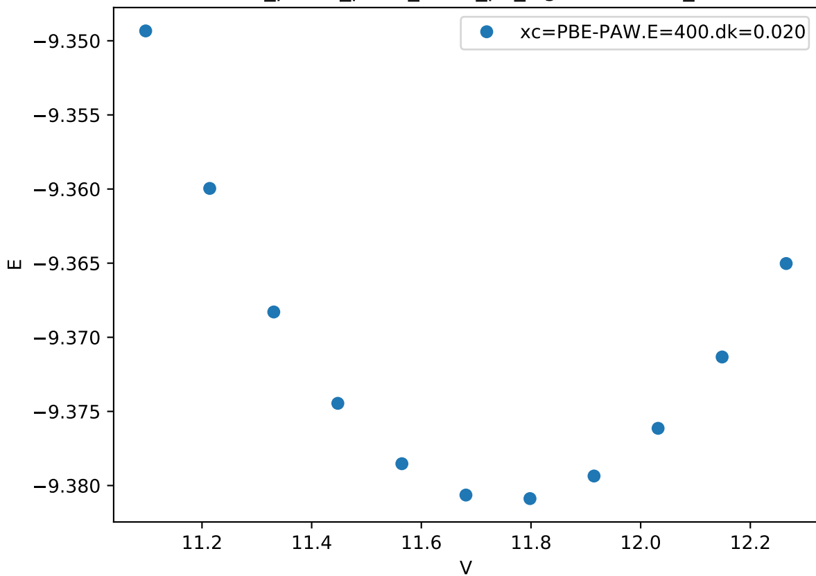
Cr_pv-Co_pv-W_sv/Cr_pv_sigma.DUUDD_
