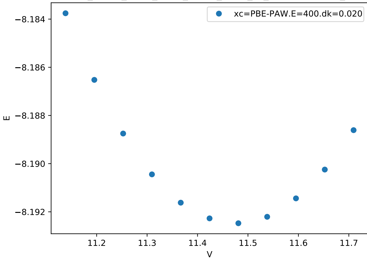
Cr_pv-Co_pv-W_sv/Cr_pv-Co_pv-W_sv_mu-BBACB.FM_
