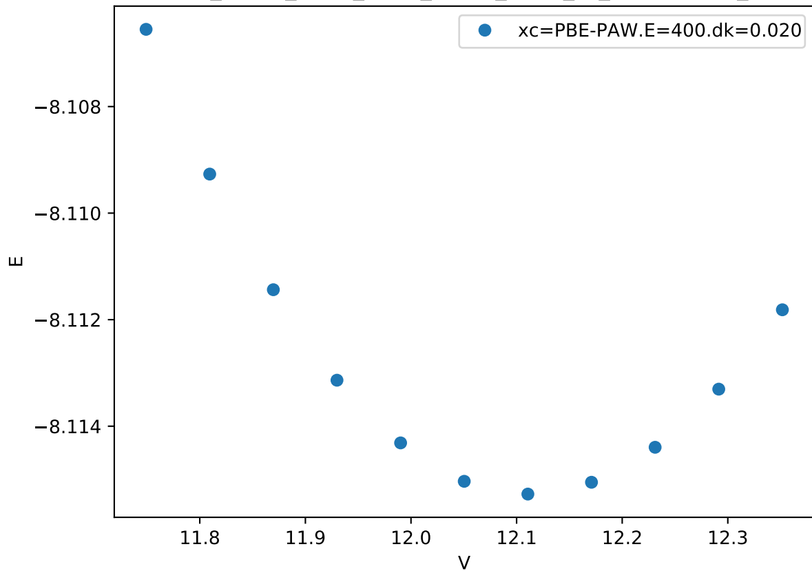
Cr_pv-Co_pv-W_sv/Cr_pv-Co_pv-W_sv_C36-BACBB_
