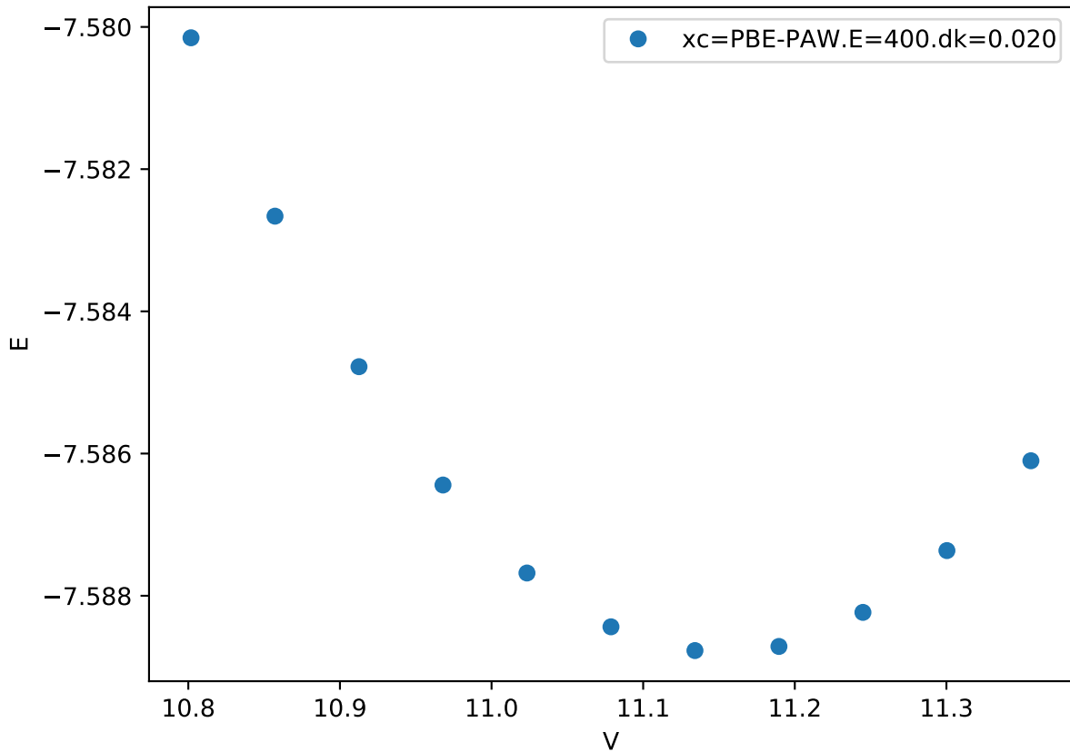
Cr_pv-Co_pv-W_sv/Cr_pv-Co_pv_C36-ABABB_
