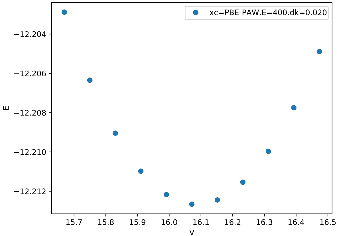
Cr_pv-Co_pv-W_sv/Cr_pv-W_sv_sigma-BABBB.FM_
