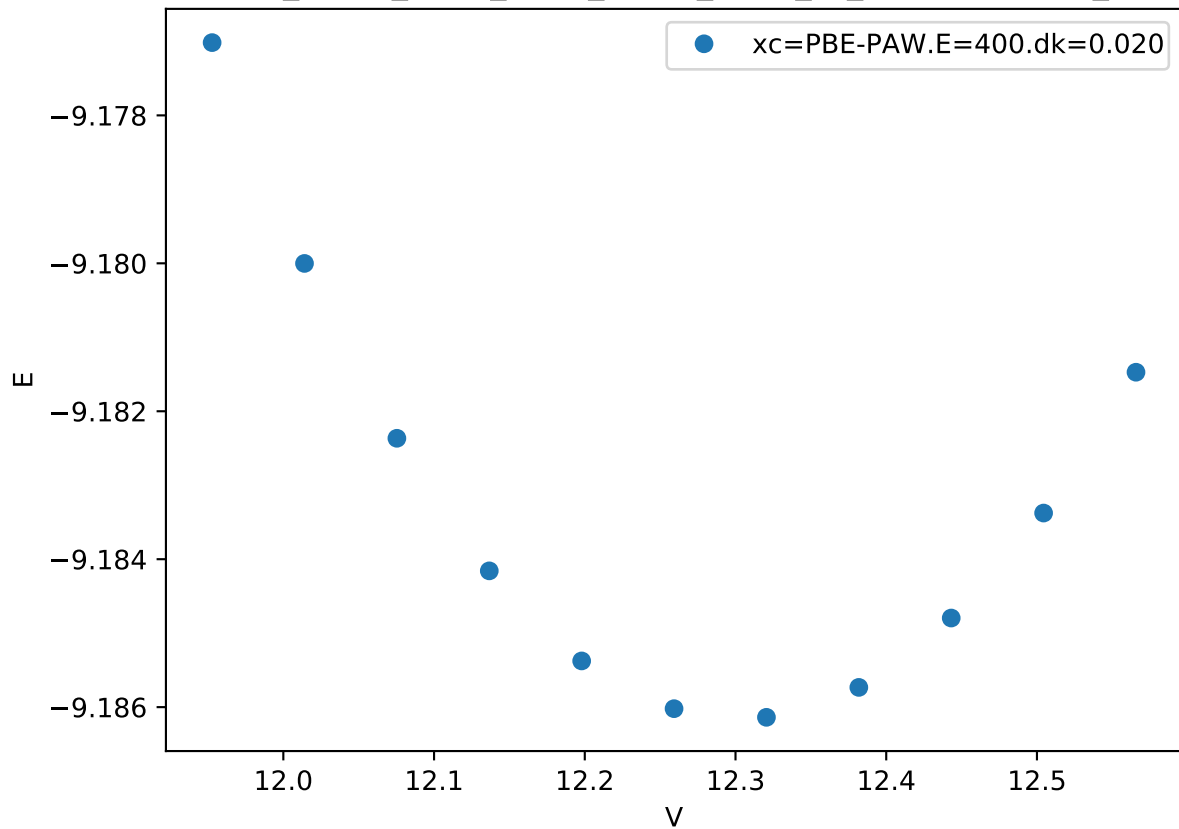
Cr_pv-Co_pv-W_sv/Cr_pv-Co_pv-W_sv_mu-BBACC.FM_
