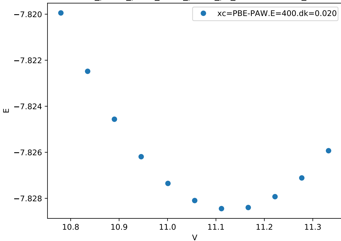
Cr_pv-Co_pv-W_sv/Cr_pv-Co_pv_mu-ABBAA.FM_
