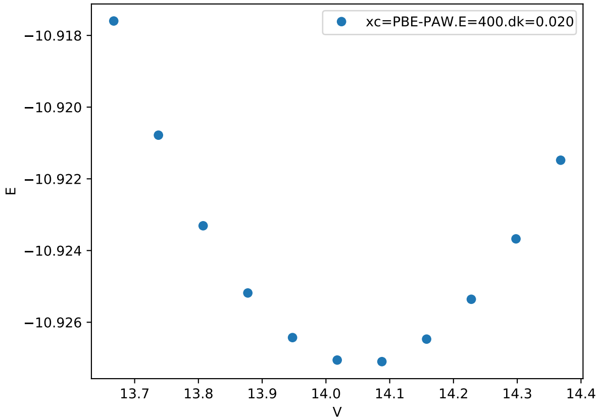
Cr_pv-Co_pv-W_sv/Cr_pv-W_sv_sigma-BBAAB_
