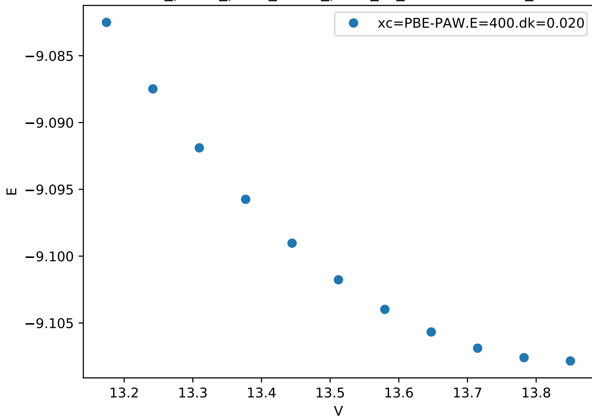
Cr_pv-Co_pv-W_sv/Co_pv-W_sv_C36-BAABA.FM_
