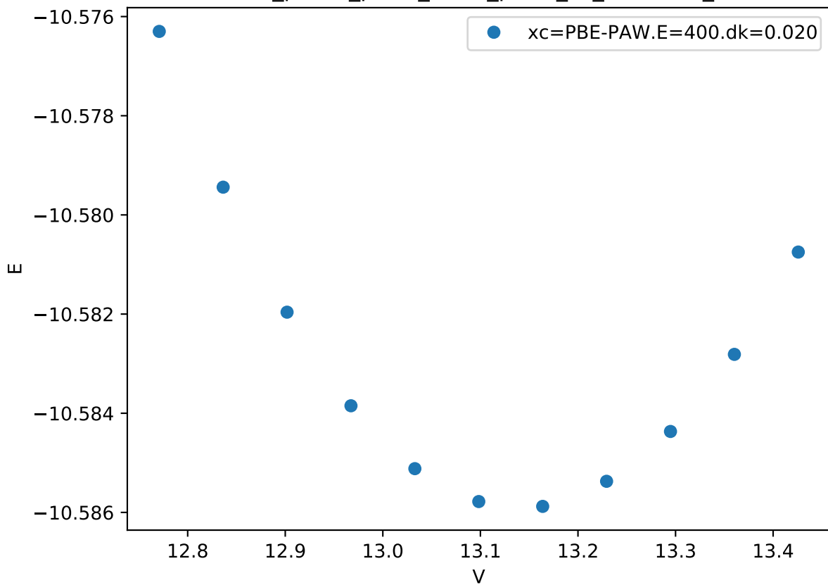
Cr_pv-Co_pv-W_sv/Cr_pv-W_sv_C14-BAA_
