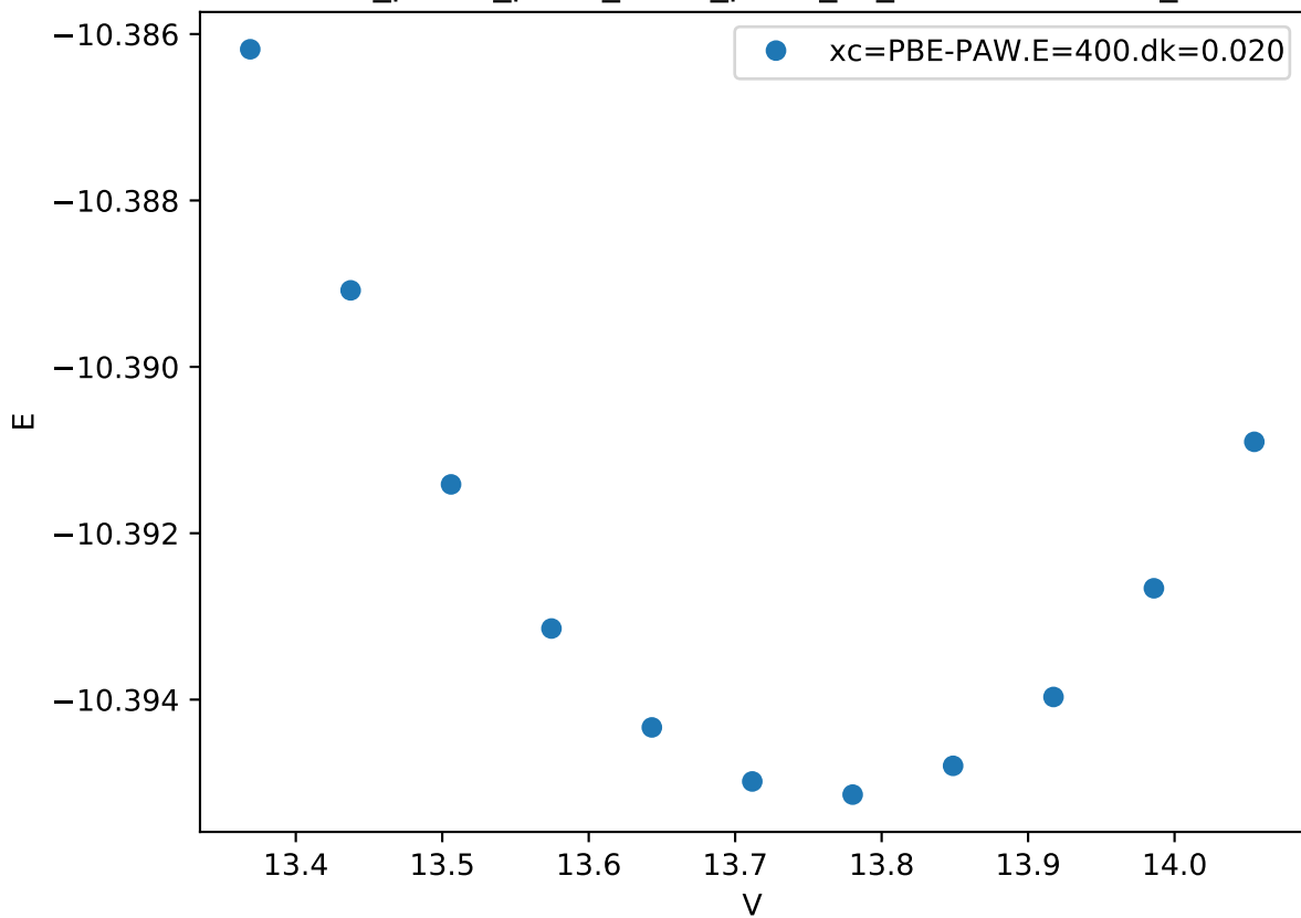
Cr_pv-Co_pv-W_sv/Cr_pv-W_sv_C36-BABAA.FM_
