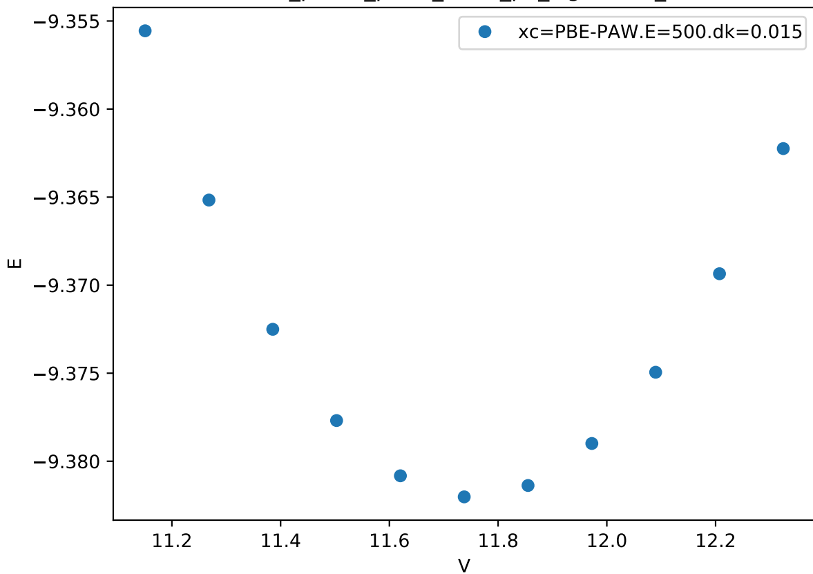
Cr_pv-Co_pv-W_sv/Cr_pv_sigma.FM_
