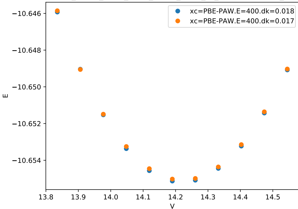
Cr_pv-Co_pv-W_sv/Cr_pv-Co_pv-W_sv_C36-CCACB.FM_
