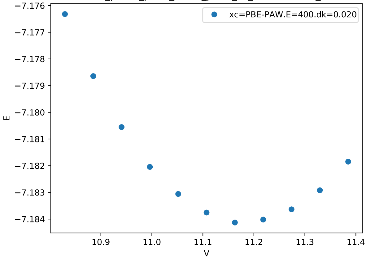
Cr_pv-Co_pv-W_sv/Co_pv-W_sv_chi-BAAA.FM_
