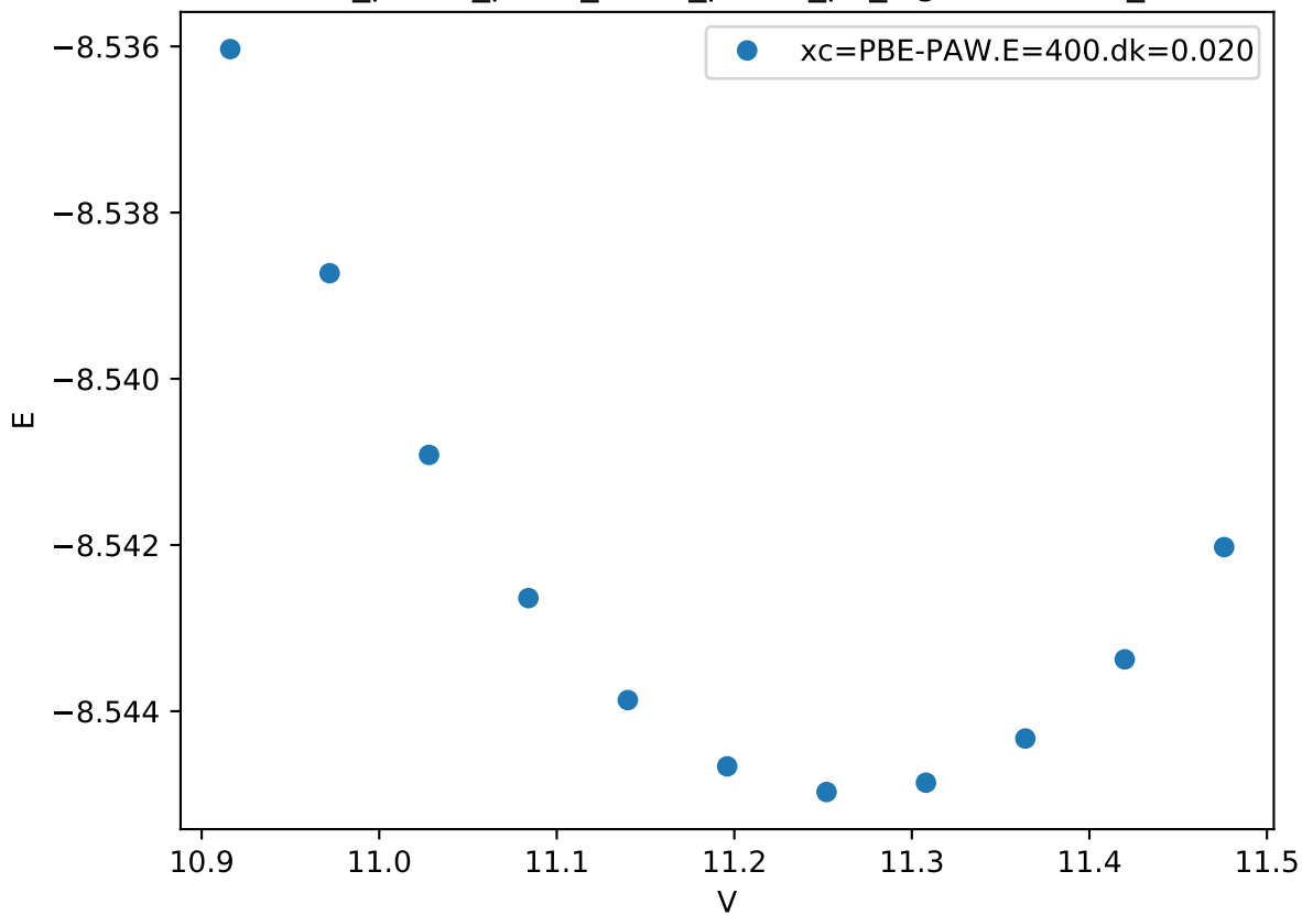
Cr_pv-Co_pv-W_sv/Cr_pv-Co_pv_sigma-BAAAB_
