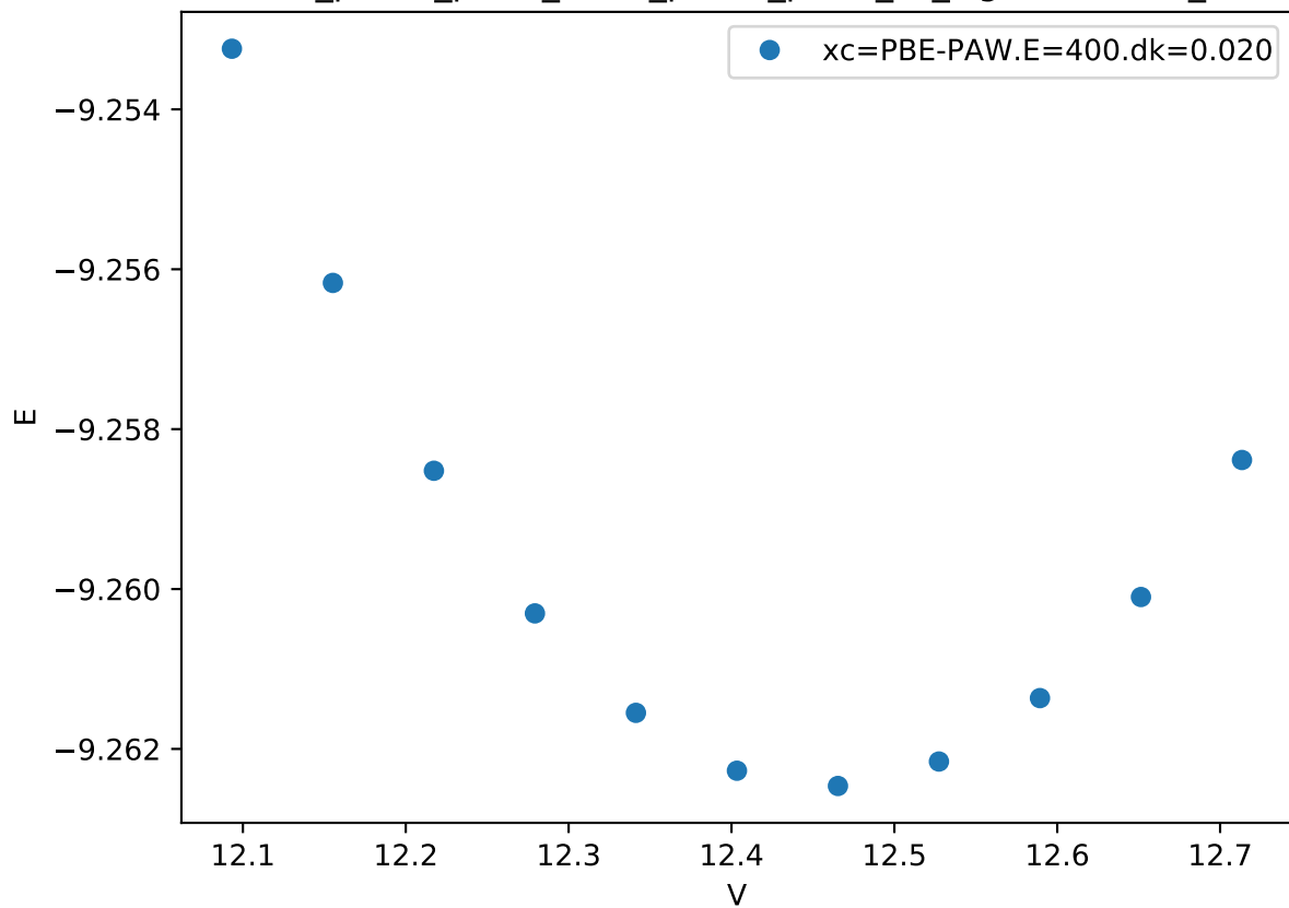
Cr_pv-Co_pv-W_sv/Cr_pv-Co_pv-W_sv_sigma-ABCAB_
