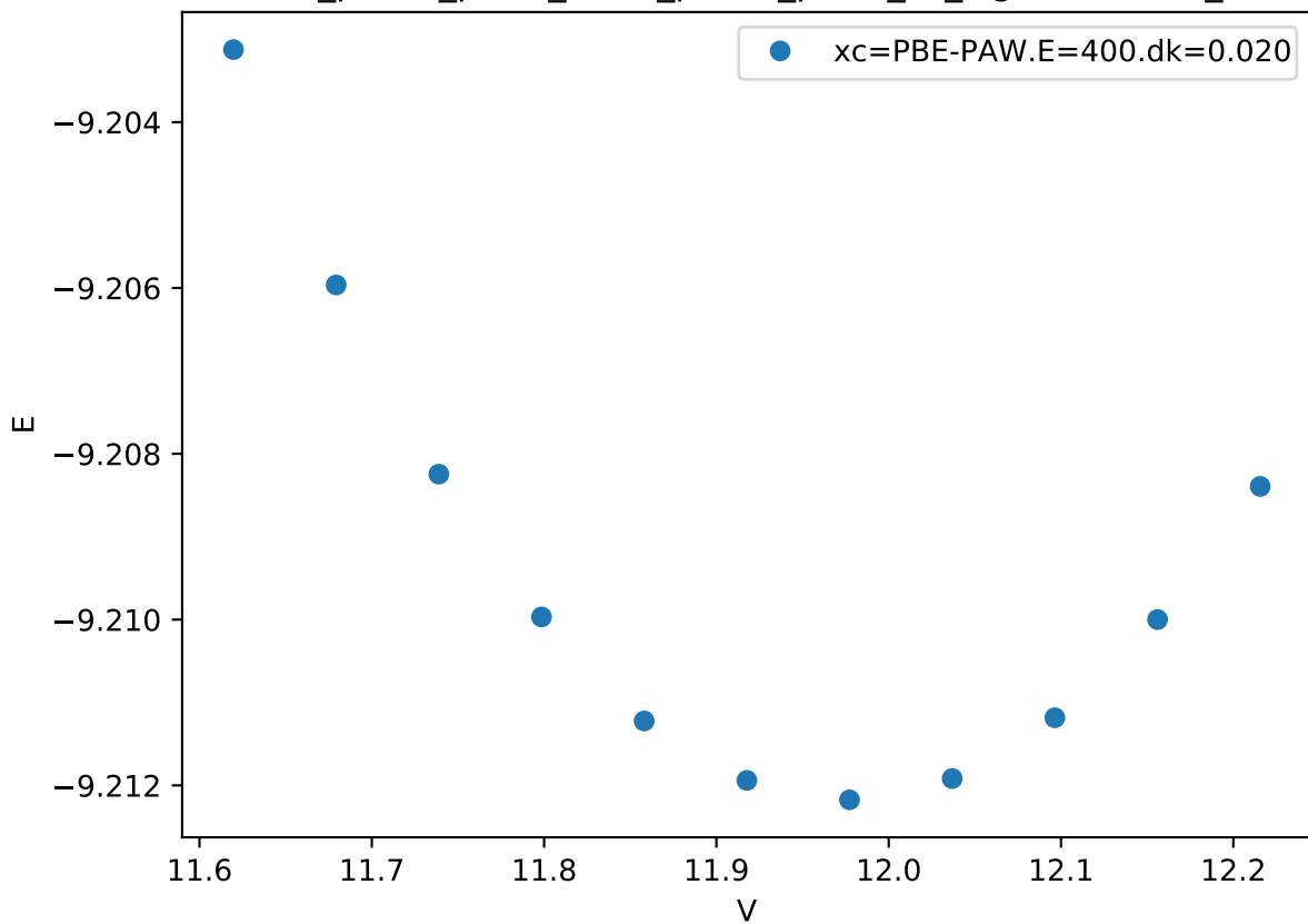
Cr_pv-Co_pv-W_sv/Cr_pv-Co_pv-W_sv_sigma-ACBAA_
