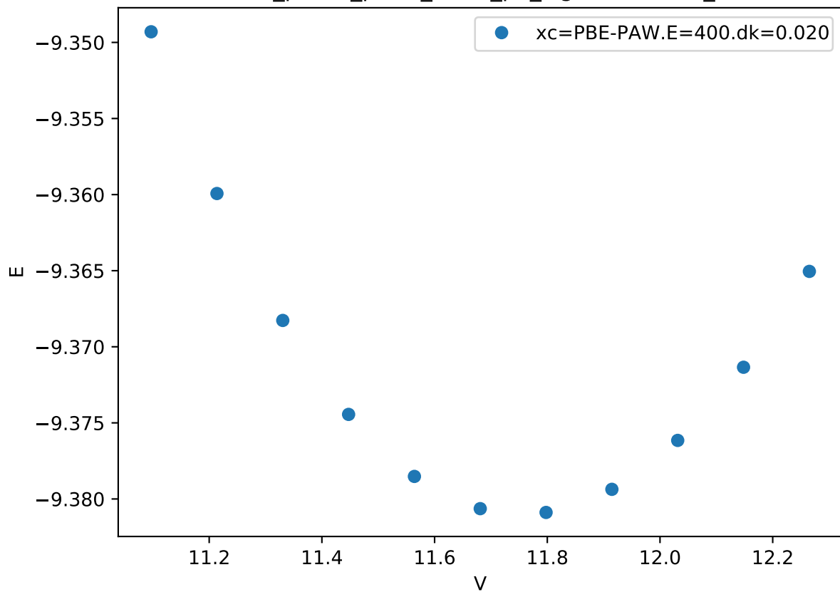
Cr_pv-Co_pv-W_sv/Cr_pv_sigma.UDDDU_
