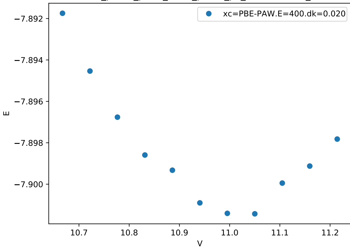
Cr_pv-Co_pv-W_sv/Cr_pv-Co_pv_chi-BBAB.FM_
