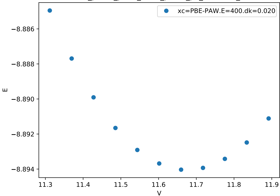
Cr_pv-Co_pv-W_sv/Cr_pv-Co_pv_C14-ABA_
