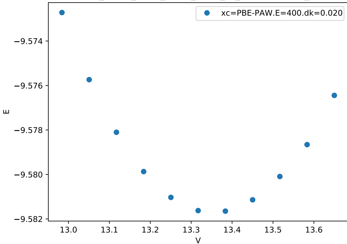
Cr_pv-Co_pv-W_sv/Co_pv-W_sv_sigma-BBAAB_
