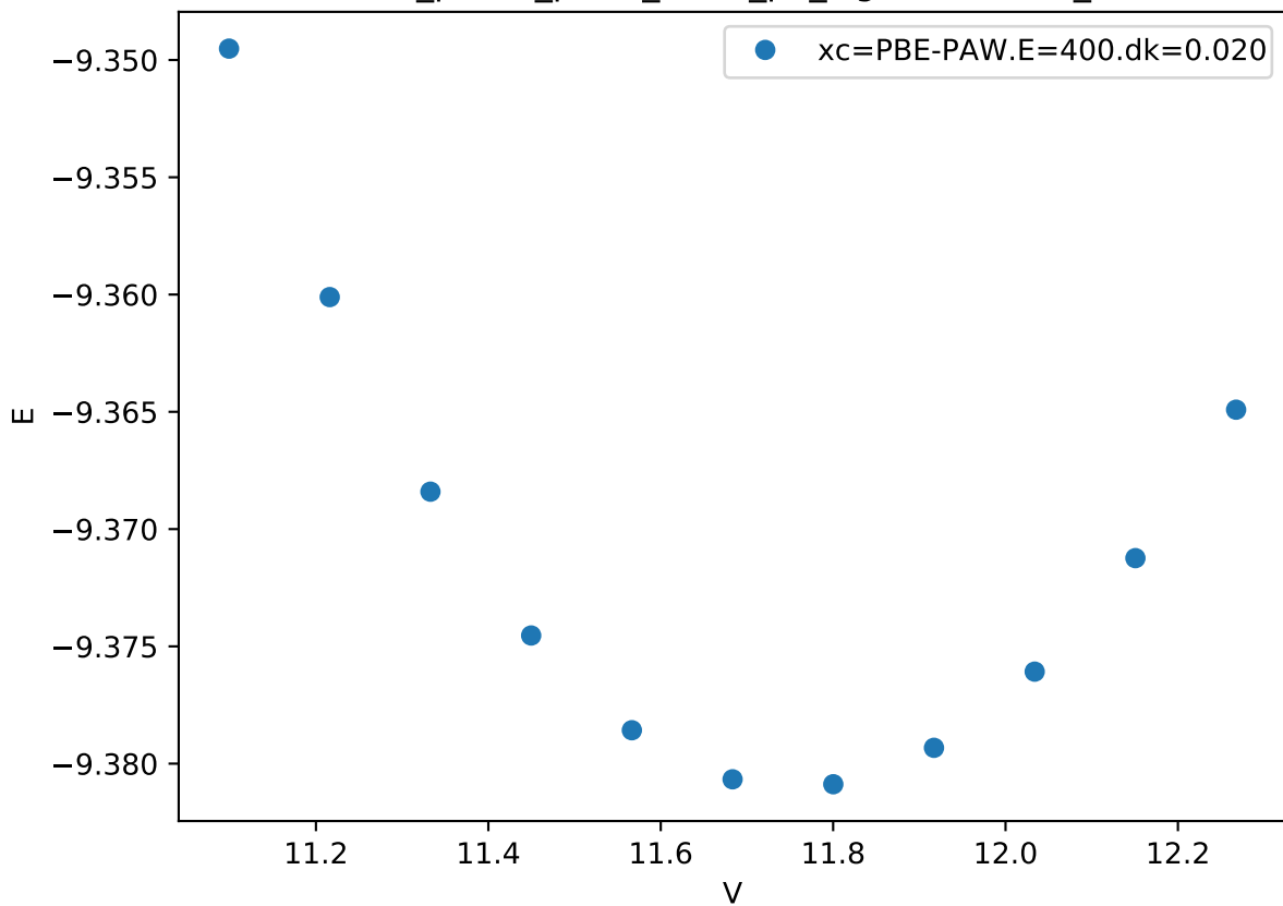
Cr_pv-Co_pv-W_sv/Cr_pv_sigma.DUUDU_
