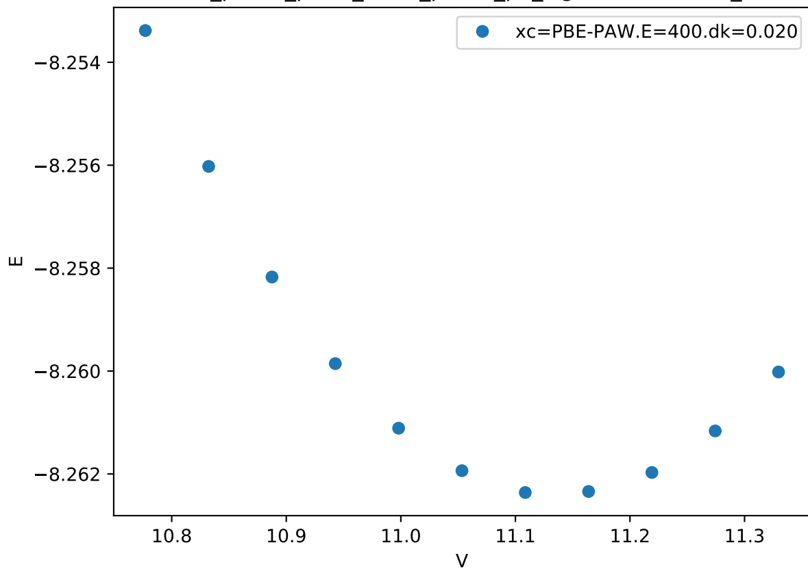
Cr_pv-Co_pv-W_sv/Cr_pv-Co_pv_sigma-BBABA.FM_
