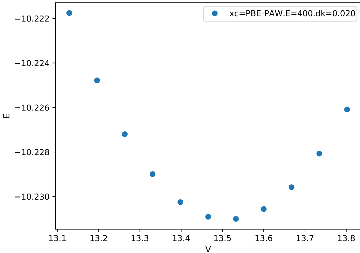
Cr_pv-Co_pv-W_sv/Cr_pv-Co_pv-W_sv_mu-CACBC.FM_
