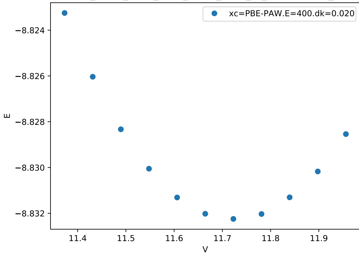
Cr_pv-Co_pv-W_sv/Cr_pv-Co_pv-W_sv_chi-ACAB.FM_
