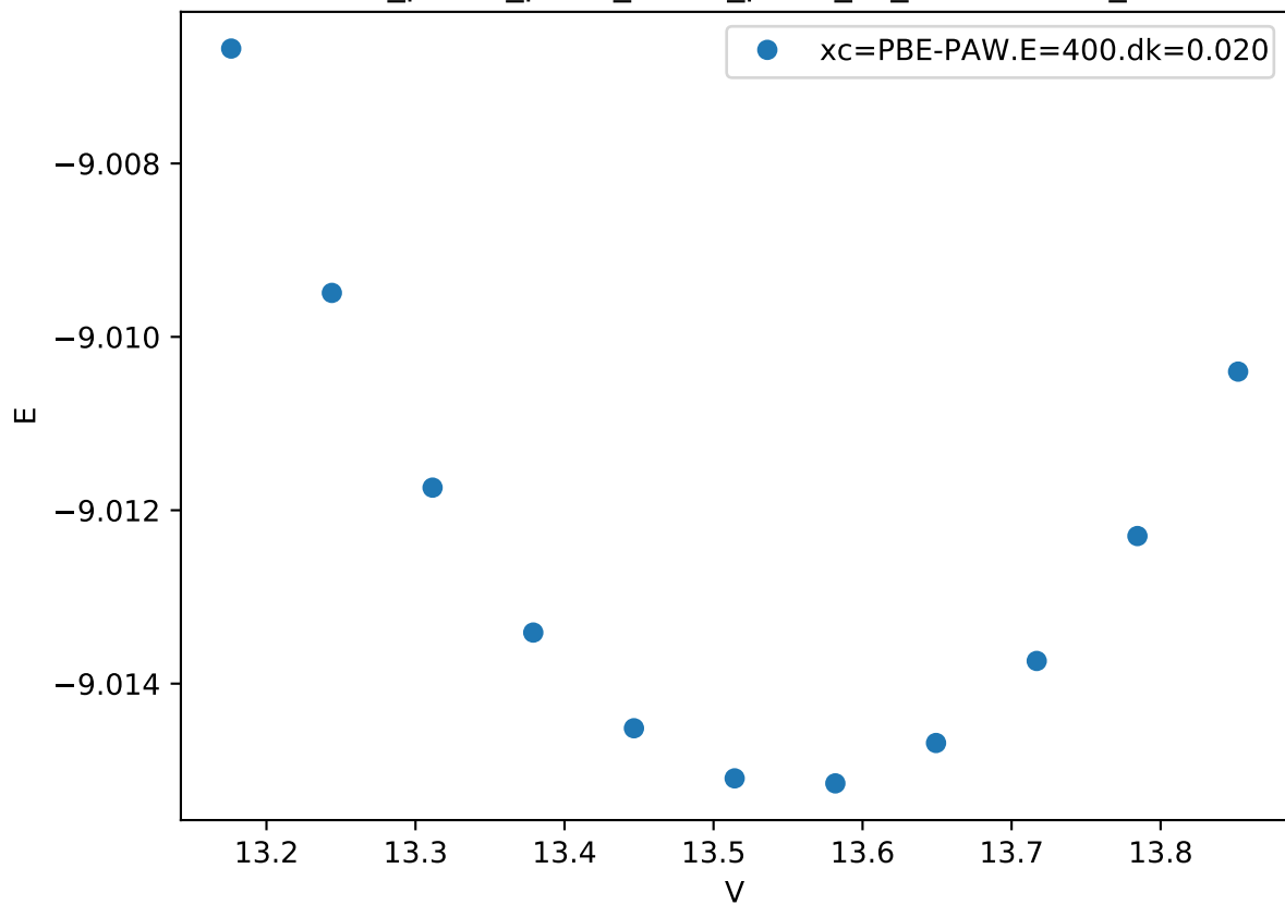
Cr_pv-Co_pv-W_sv/Co_pv-W_sv_C36-BAABA_
