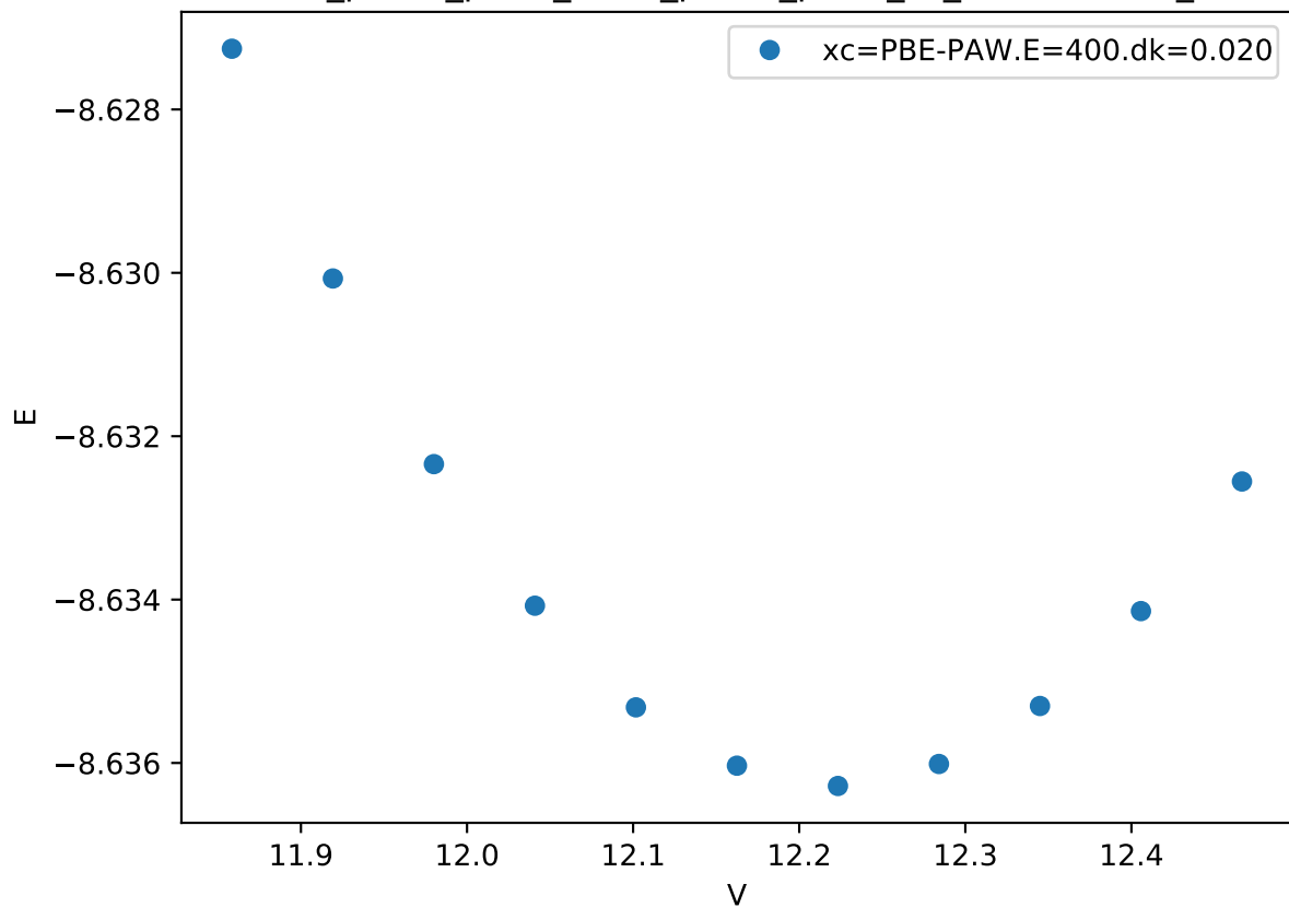
Cr_pv-Co_pv-W_sv/Cr_pv-Co_pv-W_sv_C14-CBA.FM_
