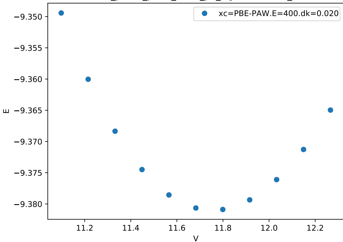
Cr_pv-Co_pv-W_sv/Cr_pv_sigma.DDUDD_
