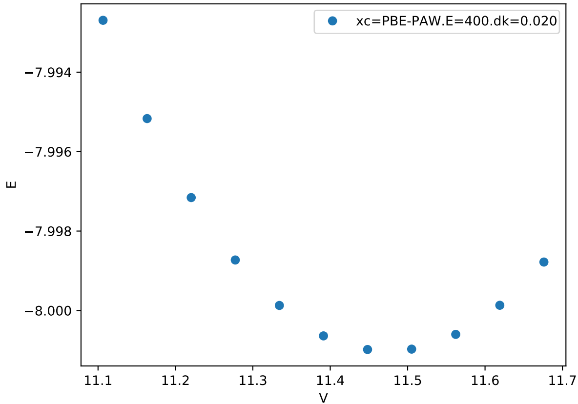
Cr_pv-Co_pv-W_sv/Cr_pv-Co_pv_C36-BBBAA.FM_
