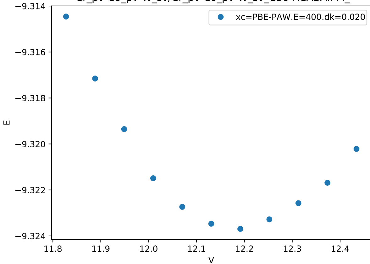
Cr_pv-Co_pv-W_sv/Cr_pv-Co_pv-W_sv_C36-ACABA.FM_
