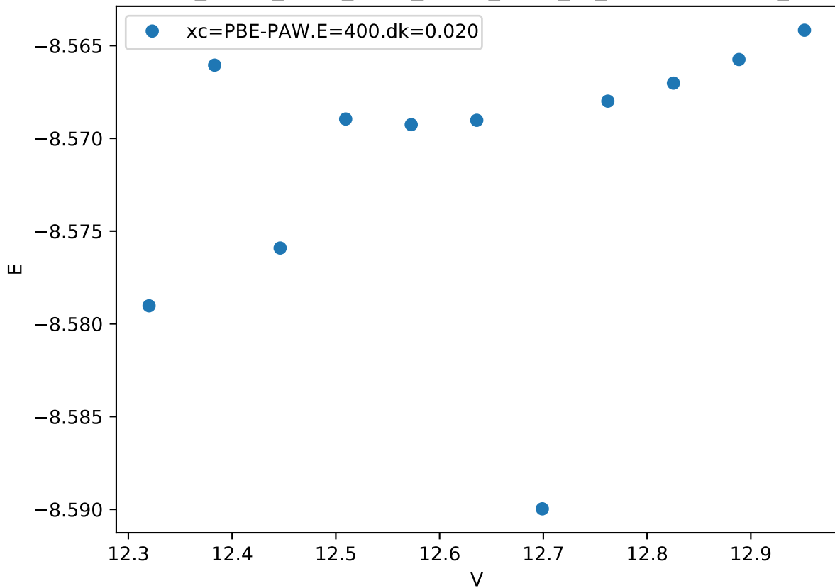
Cr_pv-Co_pv-W_sv/Cr_pv-Co_pv-W_sv_C36-AACBB.FM_
