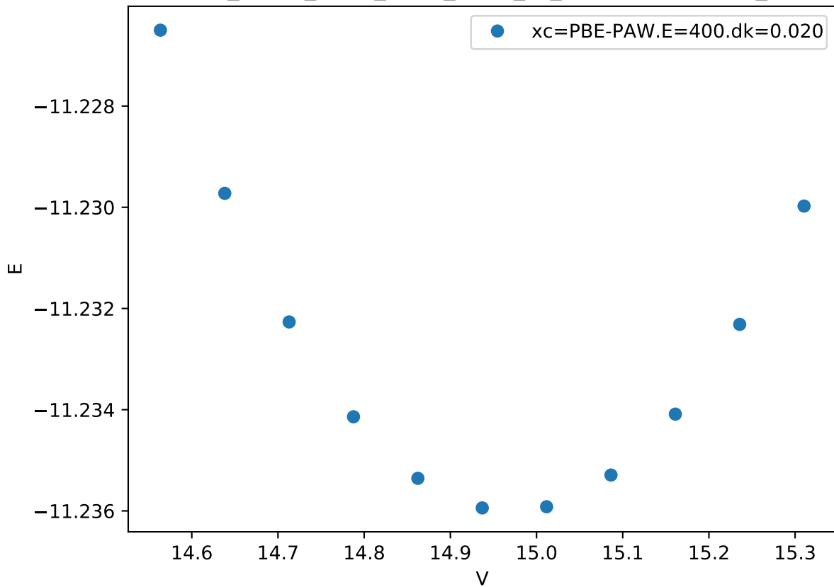
Cr_pv-Co_pv-W_sv/Cr_pv-W_sv_sigma-BABBA.FM_
