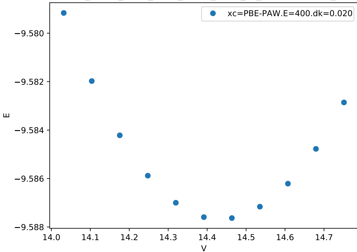
Cr_pv-Co_pv-W_sv/Cr_pv-Co_pv-W_sv_mu-BCABB.FM_
