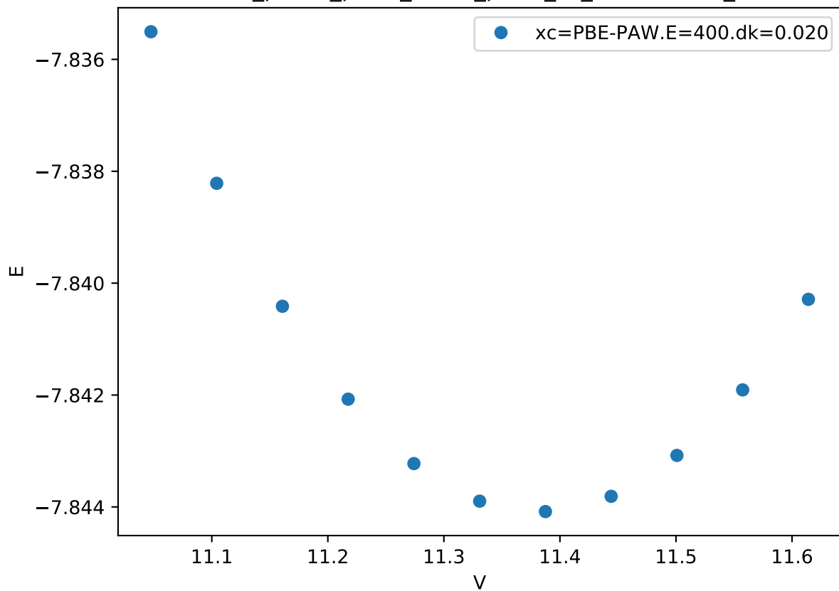
Cr_pv-Co_pv-W_sv/Co_pv-W_sv_C36-ABAAA_
