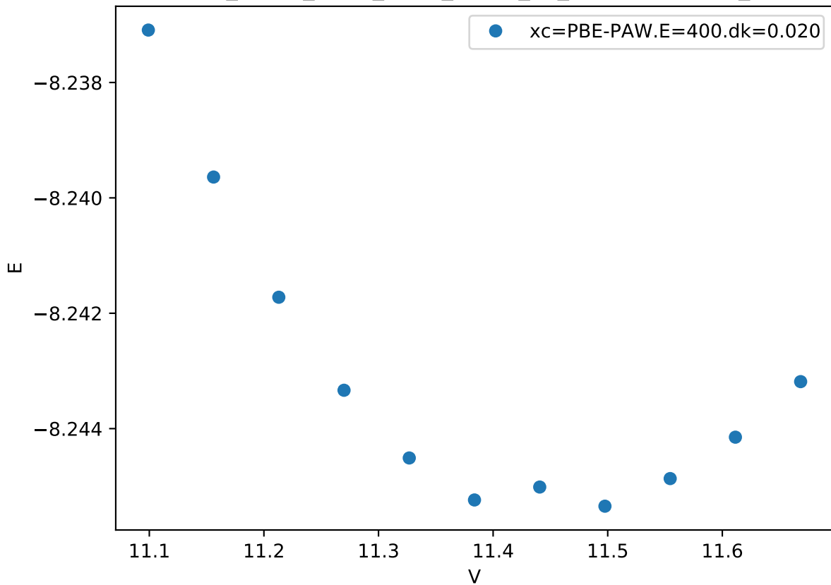
Cr_pv-Co_pv-W_sv/Cr_pv-Co_pv_C36-BAAAB.FM_
