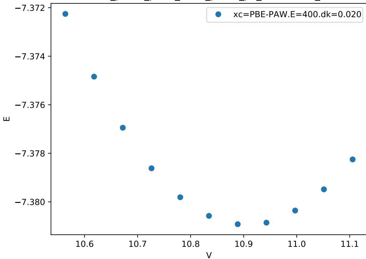
Cr_pv-Co_pv-W_sv/Cr_pv-Co_pv_mu-ABBBA_
