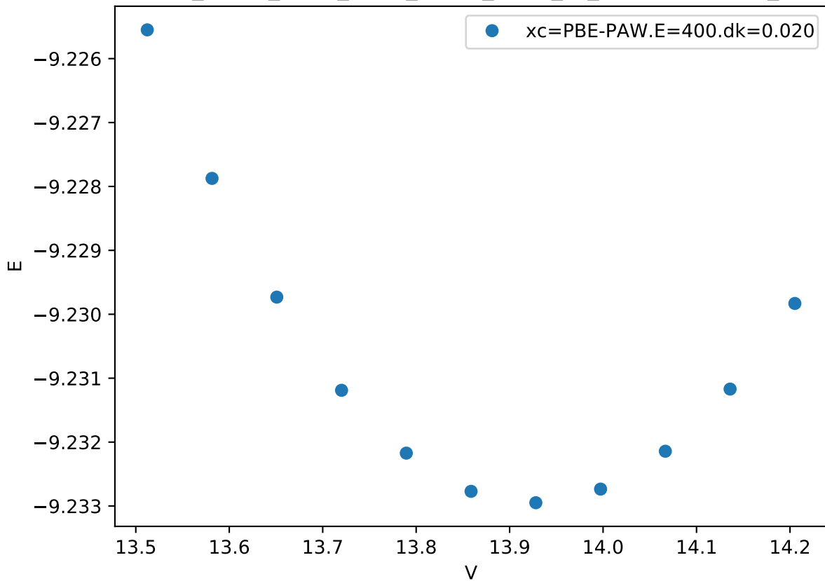
Cr_pv-Co_pv-W_sv/Cr_pv-Co_pv-W_sv_C36-AAABC.FM_
