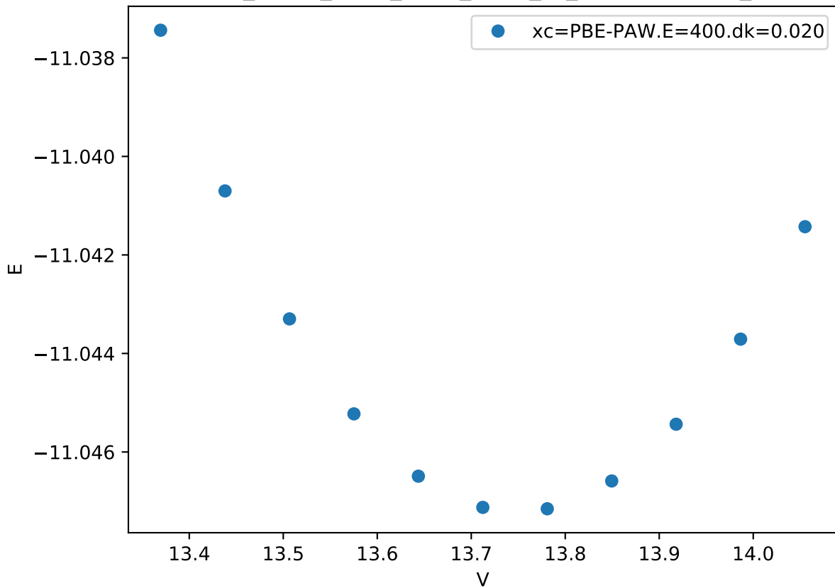
Cr_pv-Co_pv-W_sv/Cr_pv-W_sv_mu-AABBB.FM_
