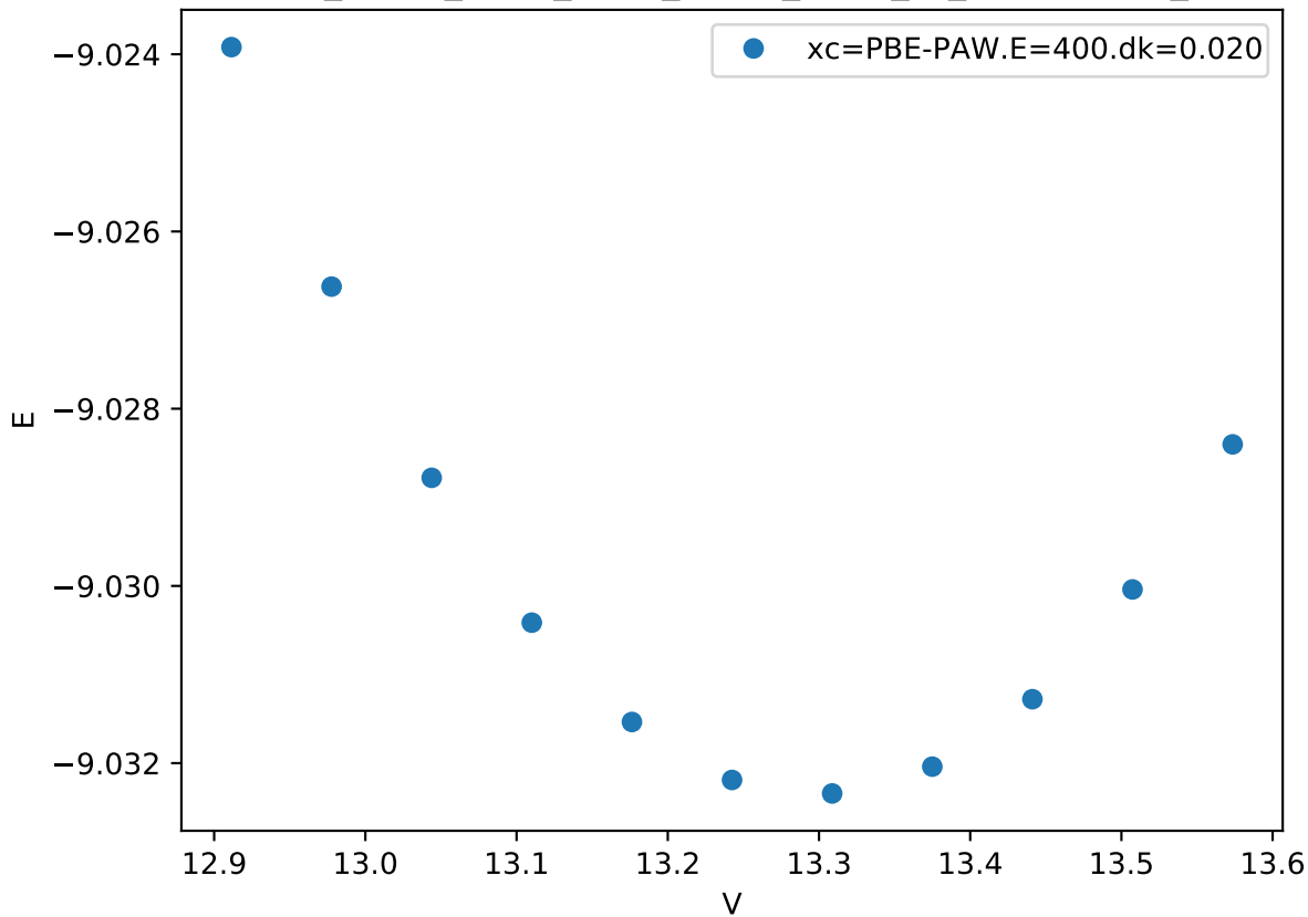
Cr_pv-Co_pv-W_sv/Cr_pv-Co_pv-W_sv_C36-BABCA_
