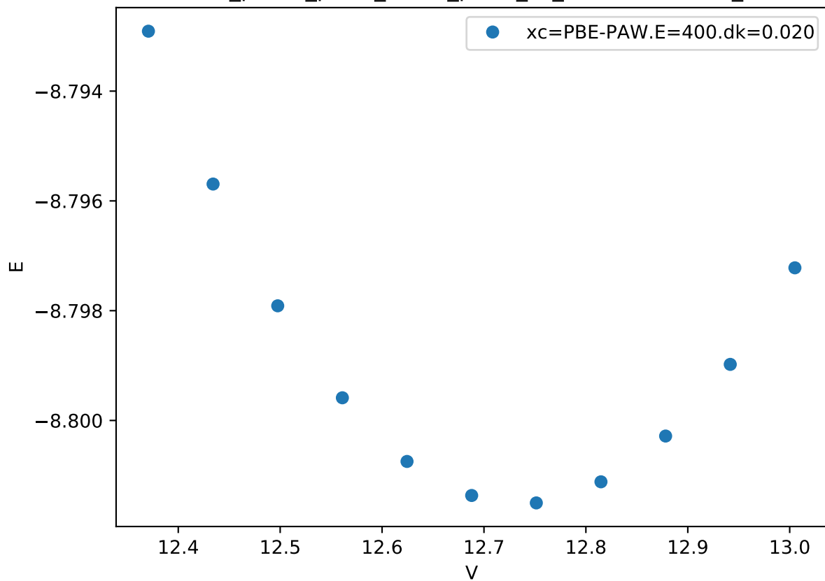
Cr_pv-Co_pv-W_sv/Co_pv-W_sv_C36-BABAA.FM_
