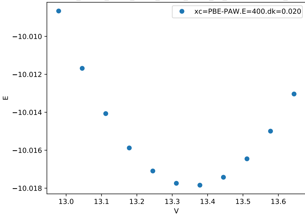
Cr_pv-Co_pv-W_sv/Cr_pv-Co_pv-W_sv_sigma-ACCAB_
