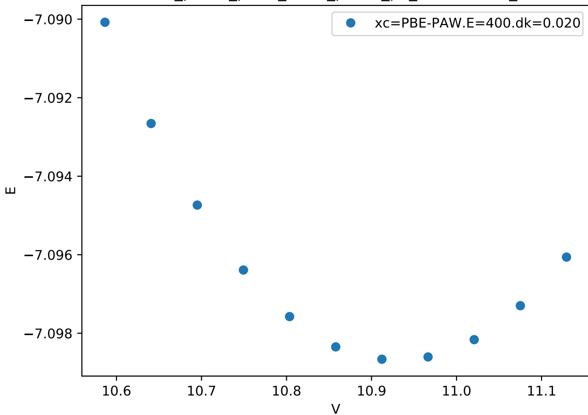
Cr_pv-Co_pv-W_sv/Cr_pv-Co_pv_C36-BABBB_
