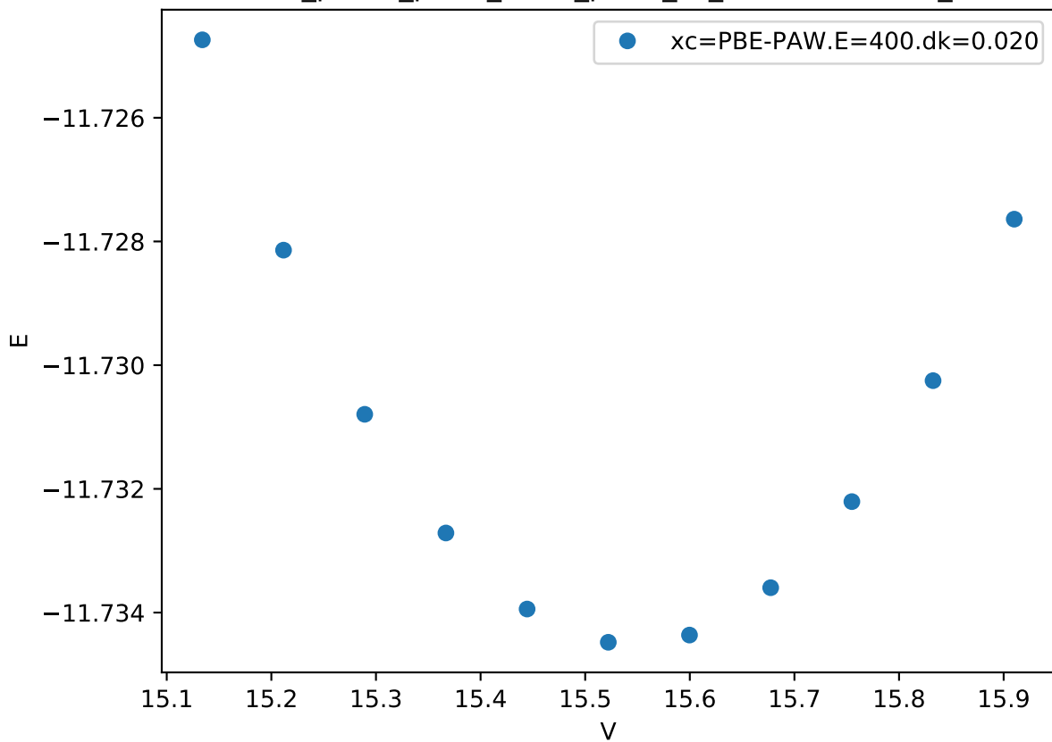
Cr_pv-Co_pv-W_sv/Cr_pv-W_sv_C36-BBBAB.FM_
