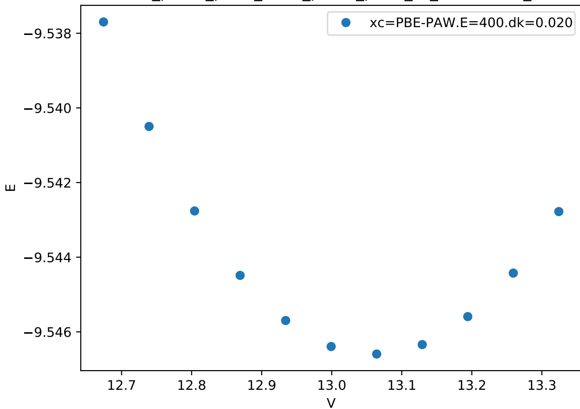
Cr_pv-Co_pv-W_sv/Cr_pv-Co_pv-W_sv_mu-CABAC_
