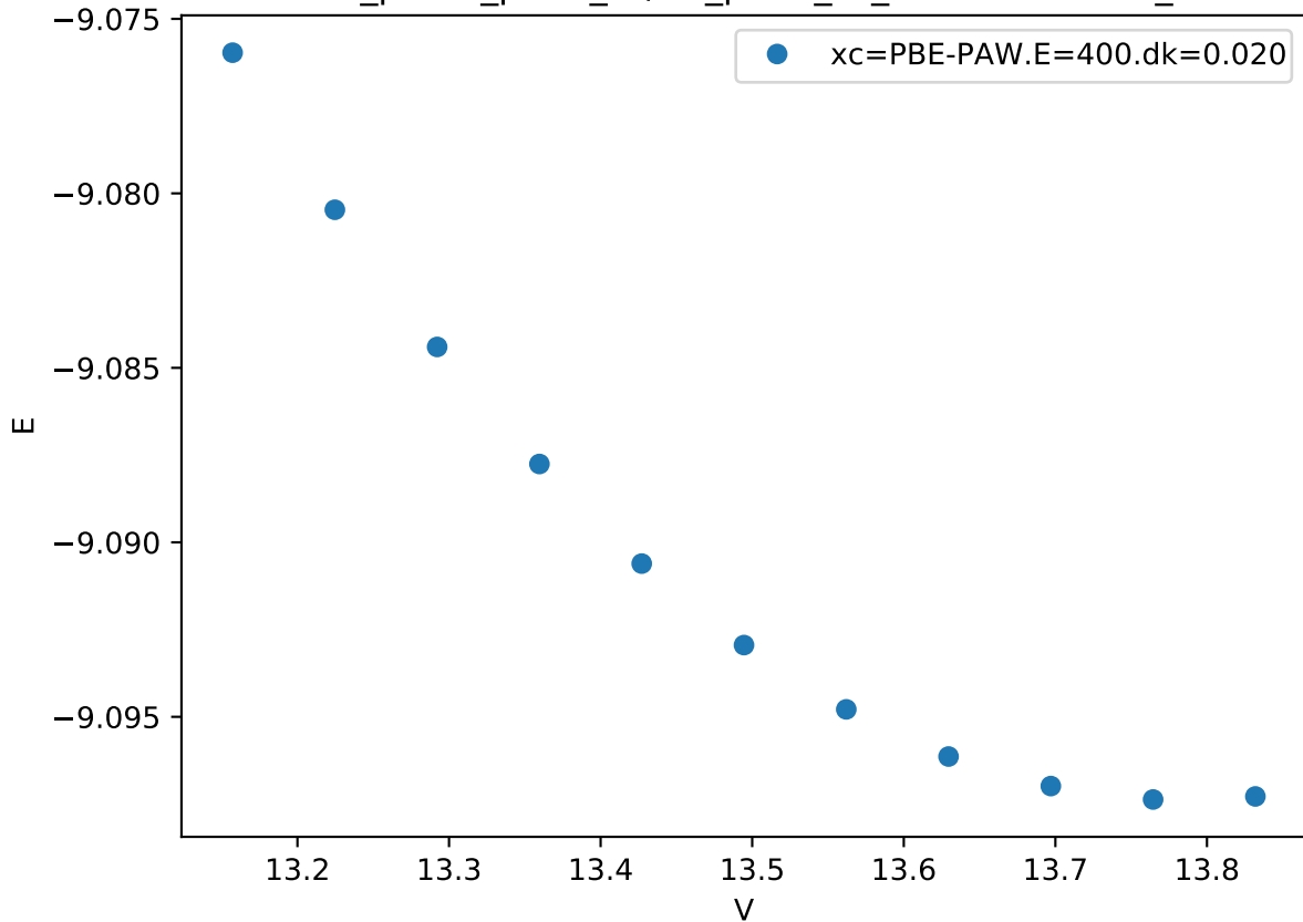
Cr_pv-Co_pv-W_sv/Co_pv-W_sv_C36-ABAAB.FM_
