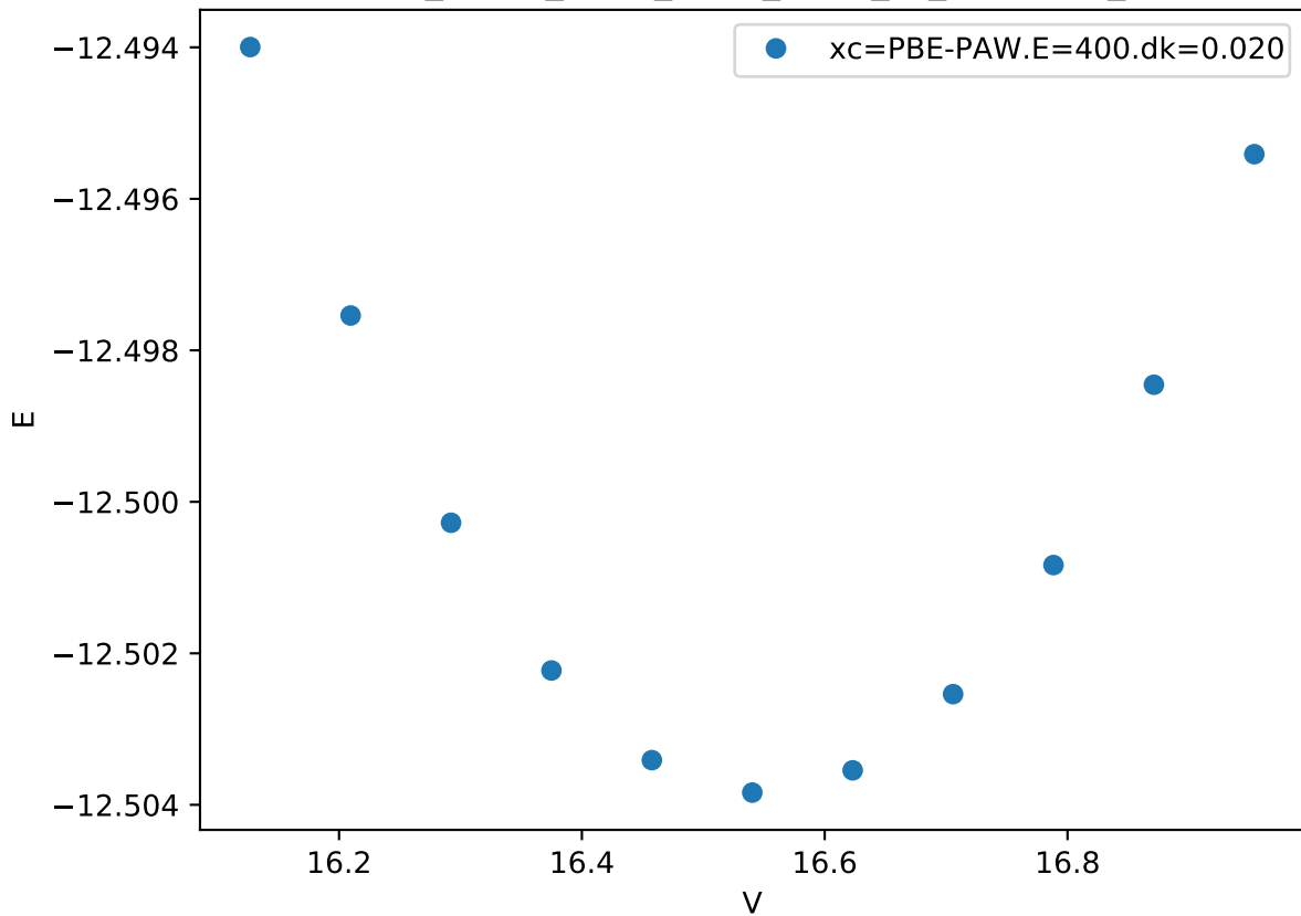
Cr_pv-Co_pv-W_sv/Cr_pv-W_sv_chi-ABBB_
