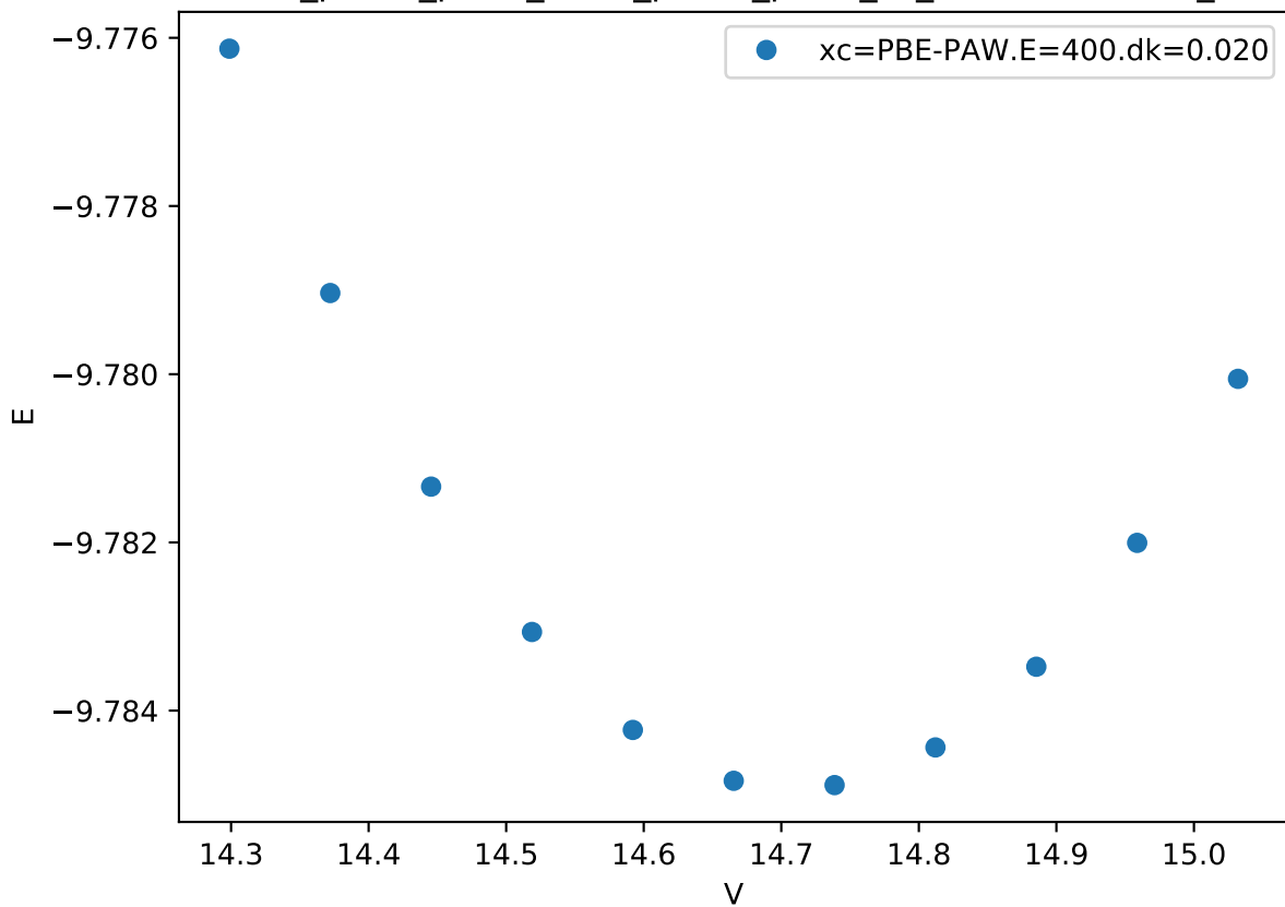
Cr_pv-Co_pv-W_sv/Cr_pv-Co_pv-W_sv_C36-ABBCC.FM_
