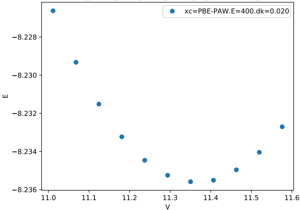
Cr_pv-Co_pv-W_sv/Cr_pv-Co_pv_C36-AABAB_
