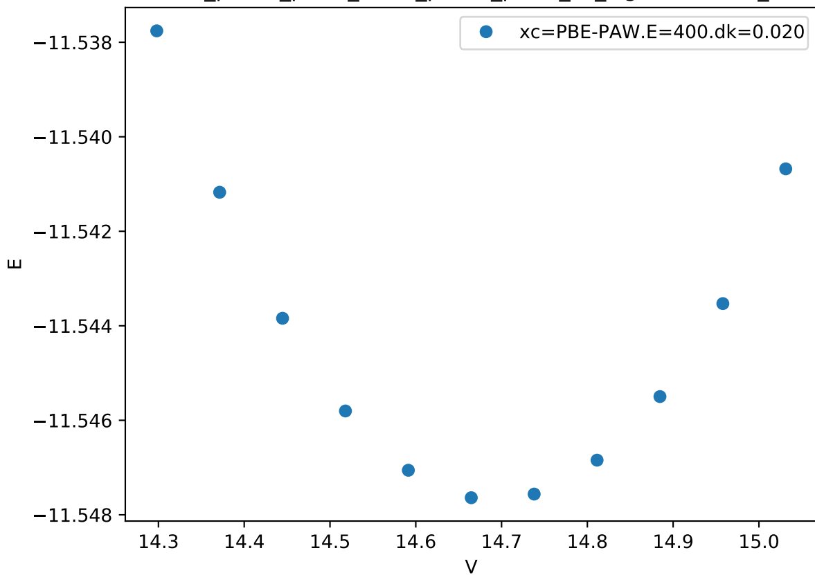
Cr_pv-Co_pv-W_sv/Cr_pv-Co_pv-W_sv_sigma-BCCAC_
