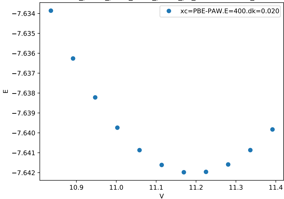
Cr_pv-Co_pv-W_sv/Cr_pv-Co_pv_mu-BBABA.FM_
