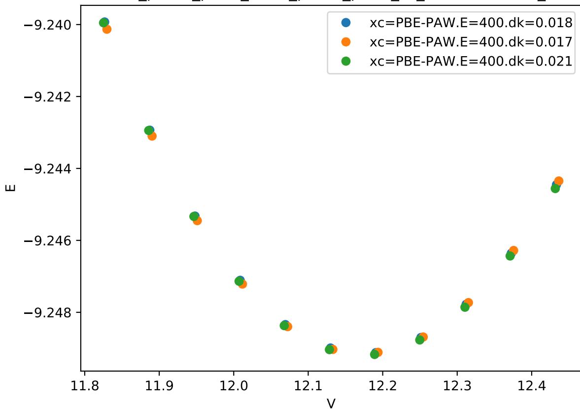
Cr_pv-Co_pv-W_sv/Cr_pv-Co_pv-W_sv_mu-BBCCA.FM_
