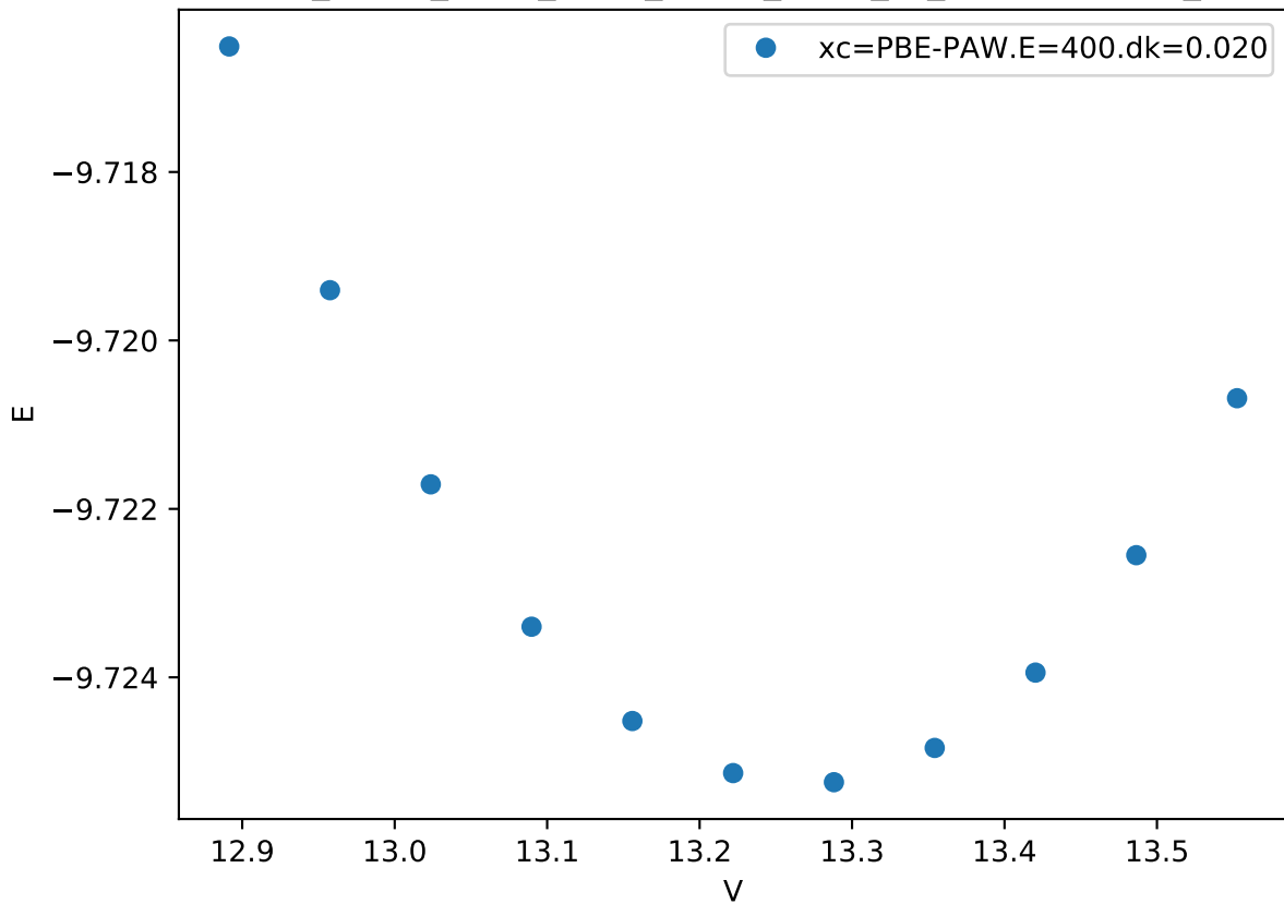
Cr_pv-Co_pv-W_sv/Cr_pv-Co_pv-W_sv_sigma-CABAC_
