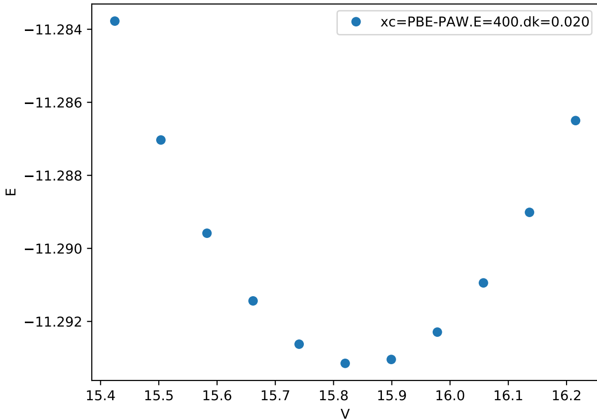
Cr_pv-Co_pv-W_sv/Cr_pv-Co_pv-W_sv_mu-ACCBC.FM_
