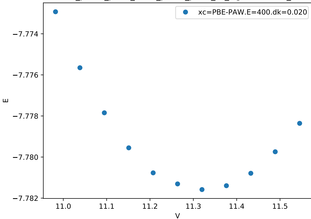
Cr_pv-Co_pv-W_sv/Cr_pv-Co_pv-W_sv_sigma-ACBBB_
