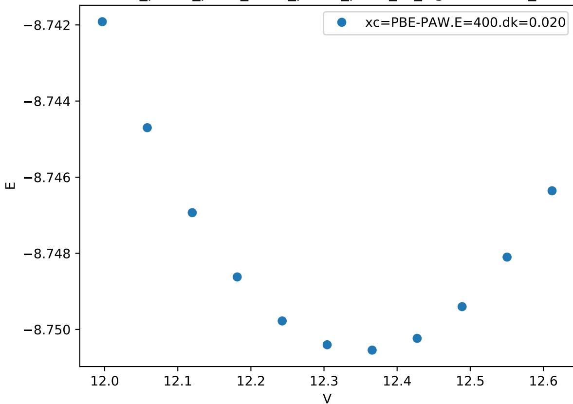
Cr_pv-Co_pv-W_sv/Cr_pv-Co_pv-W_sv_sigma-BABBC_
