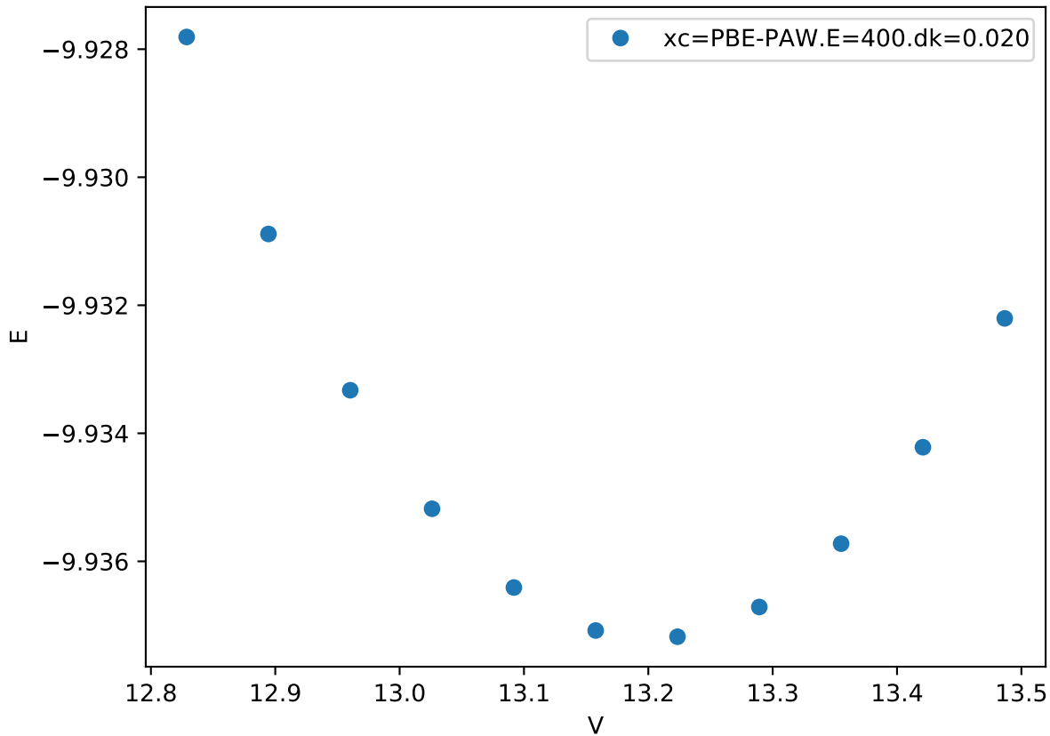
Cr_pv-Co_pv-W_sv/Cr_pv-Co_pv-W_sv_sigma-BCBCA_
