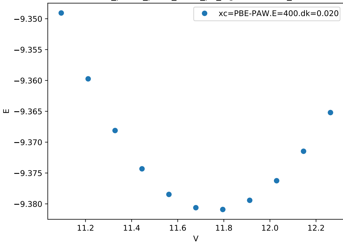
Cr_pv-Co_pv-W_sv/Cr_pv_sigma.DDUUU_
