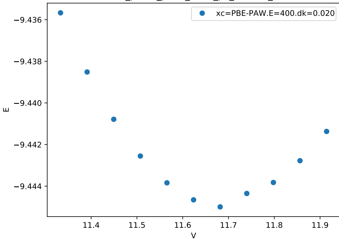
Cr_pv-Co_pv-W_sv/Cr_pv_A15.FM_
