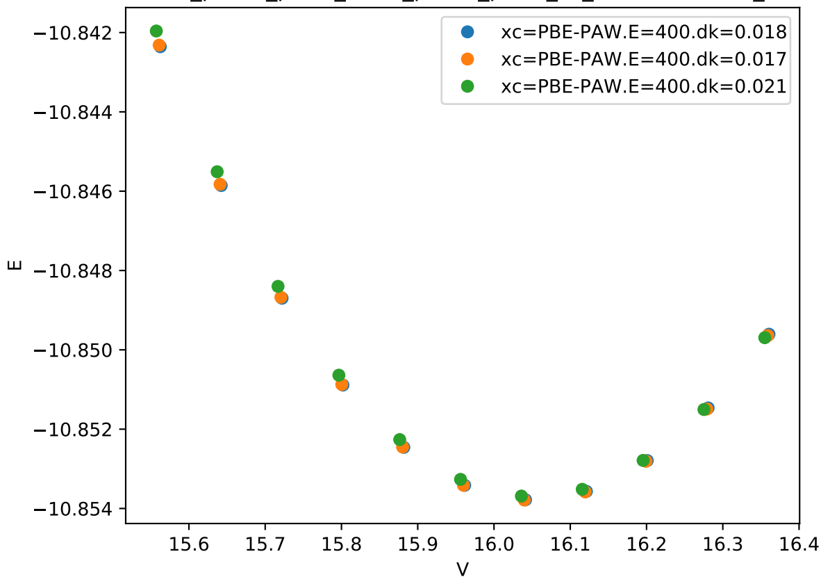
Cr_pv-Co_pv-W_sv/Cr_pv-Co_pv-W_sv_mu-CCBAC.FM_
