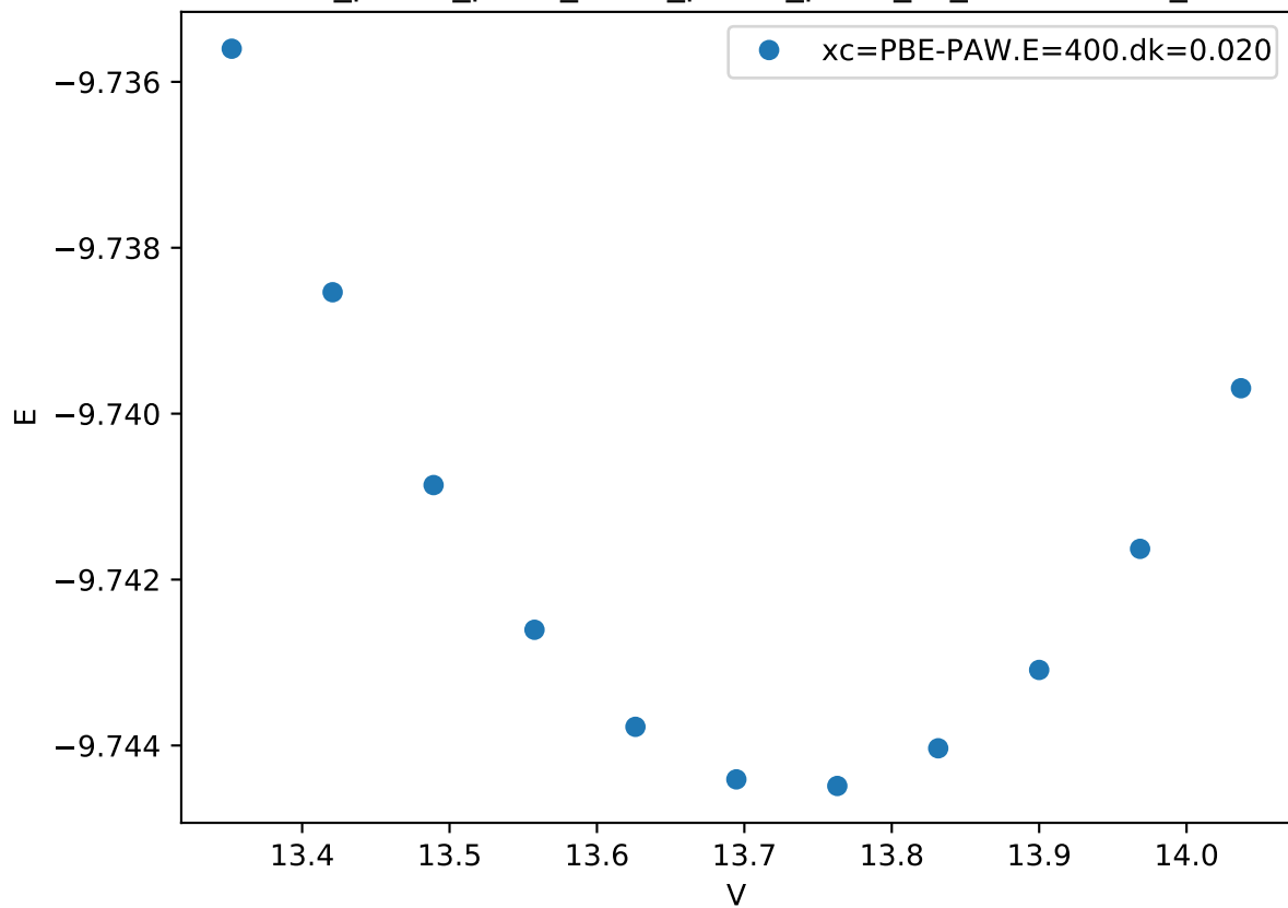
Cr_pv-Co_pv-W_sv/Cr_pv-Co_pv-W_sv_C36-BCBCA_
