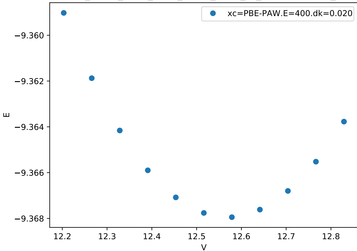
Cr_pv-Co_pv-W_sv/Cr_pv-Co_pv-W_sv_mu-CABCB.FM_
