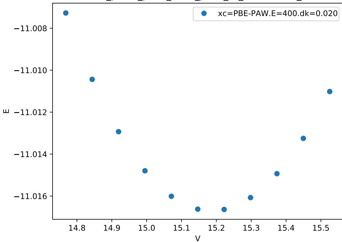
Cr_pv-Co_pv-W_sv/Cr_pv-W_sv_C36-BABAB_
