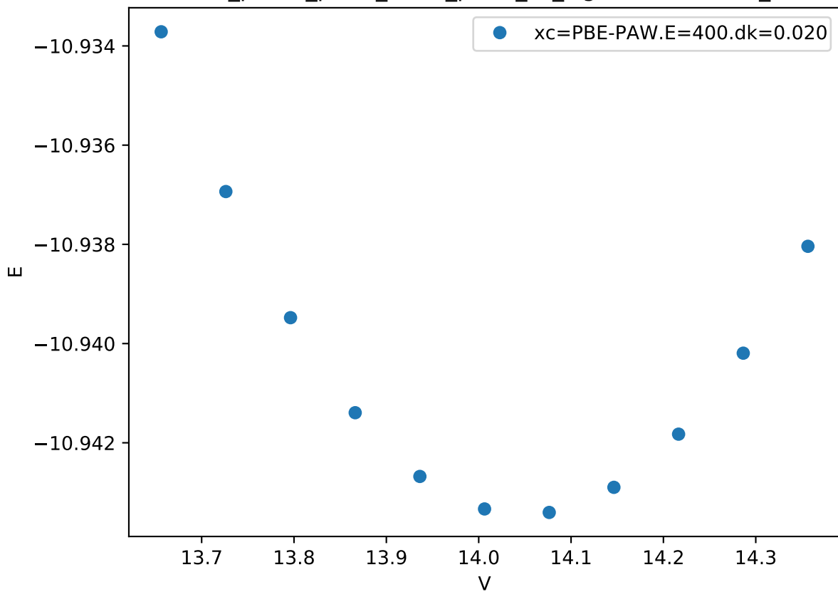
Cr_pv-Co_pv-W_sv/Cr_pv-W_sv_sigma-BBAA.FM_
