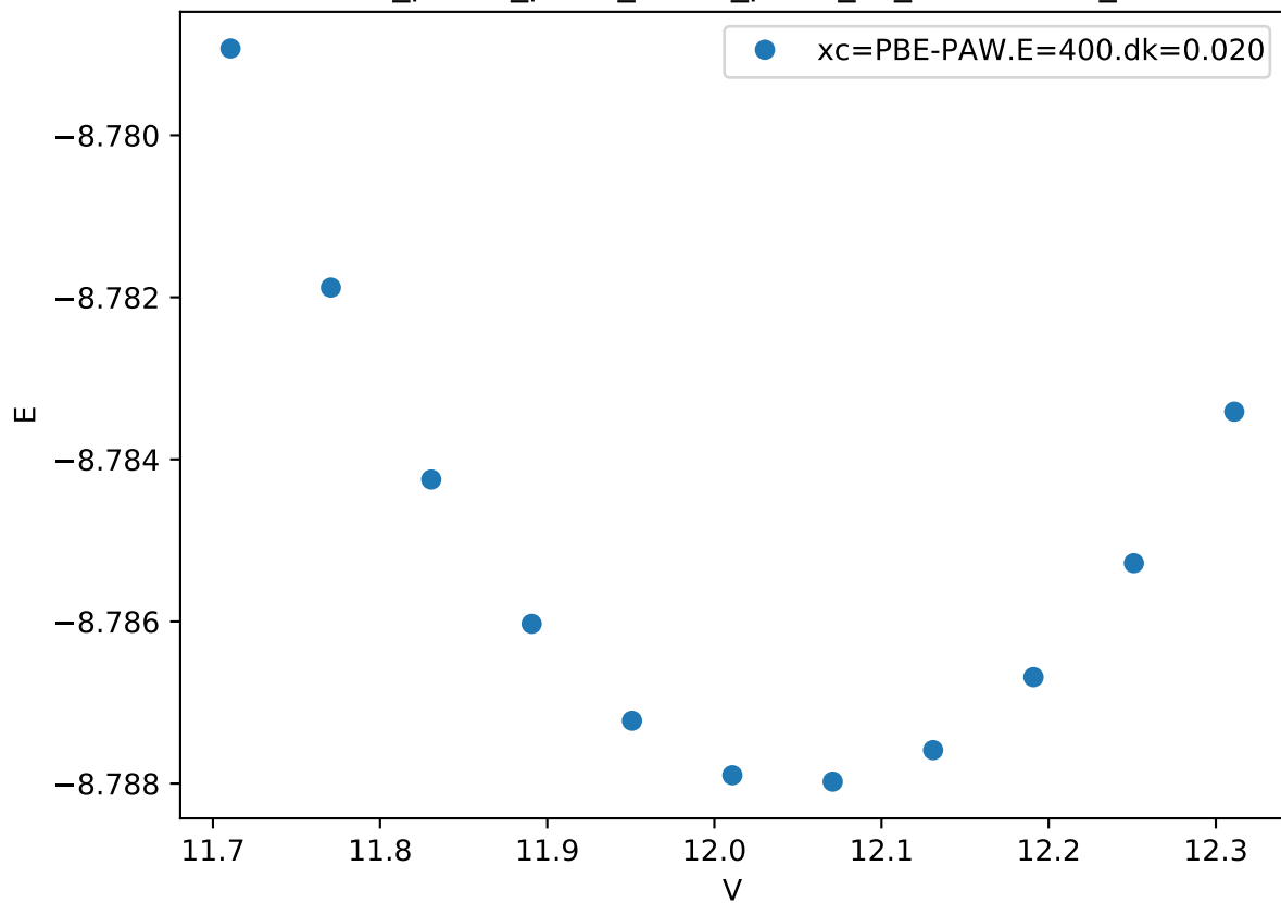
Cr_pv-Co_pv-W_sv/Co_pv-W_sv_mu-AABBA_
