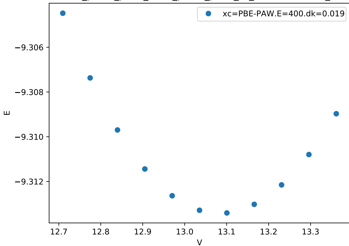
Cr_pv-Co_pv-W_sv/Cr_pv-Co_pv-W_sv_C36-BCCBA.FM_
