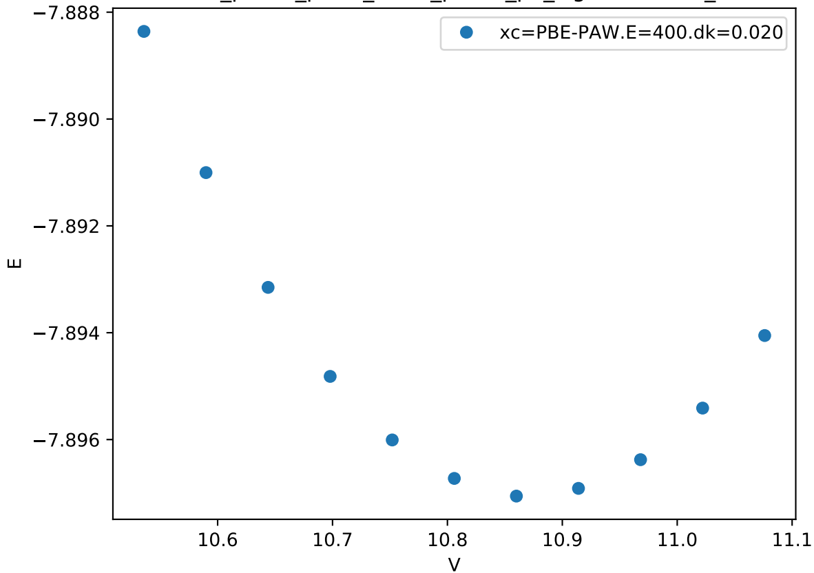
Cr_pv-Co_pv-W_sv/Cr_pv-Co_pv_sigma-BAABB_
