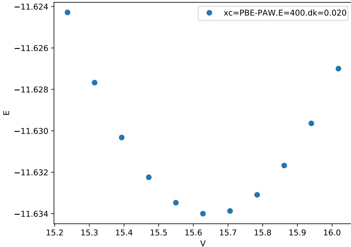
Cr_pv-Co_pv-W_sv/Cr_pv-Co_pv-W_sv_mu-BCCCA.FM_
