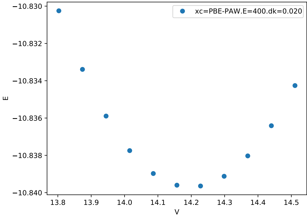
Cr_pv-Co_pv-W_sv/Cr_pv-W_sv_sigma-BBABA_
