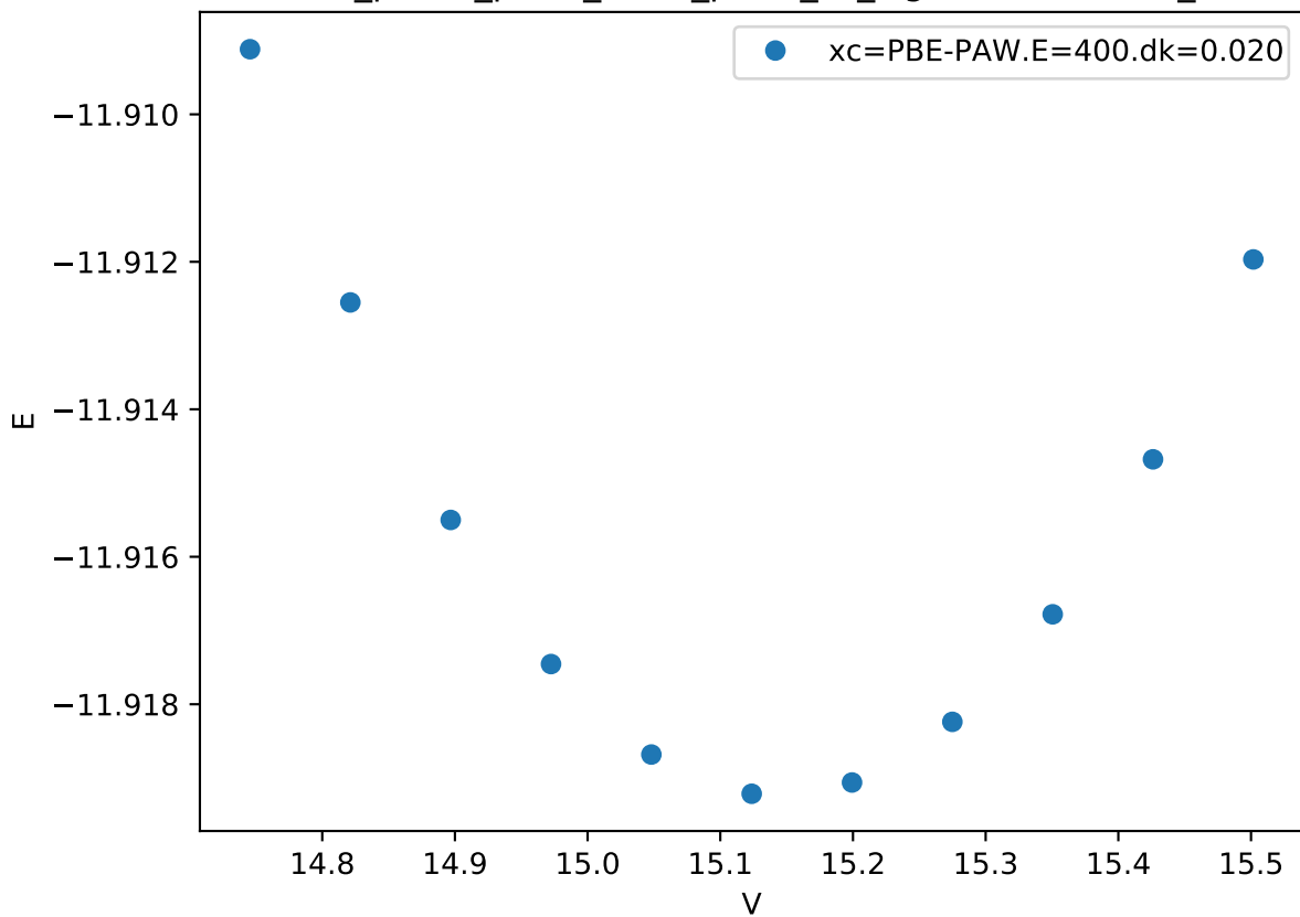
Cr_pv-Co_pv-W_sv/Cr_pv-W_sv_sigma-BBBAB.FM_
