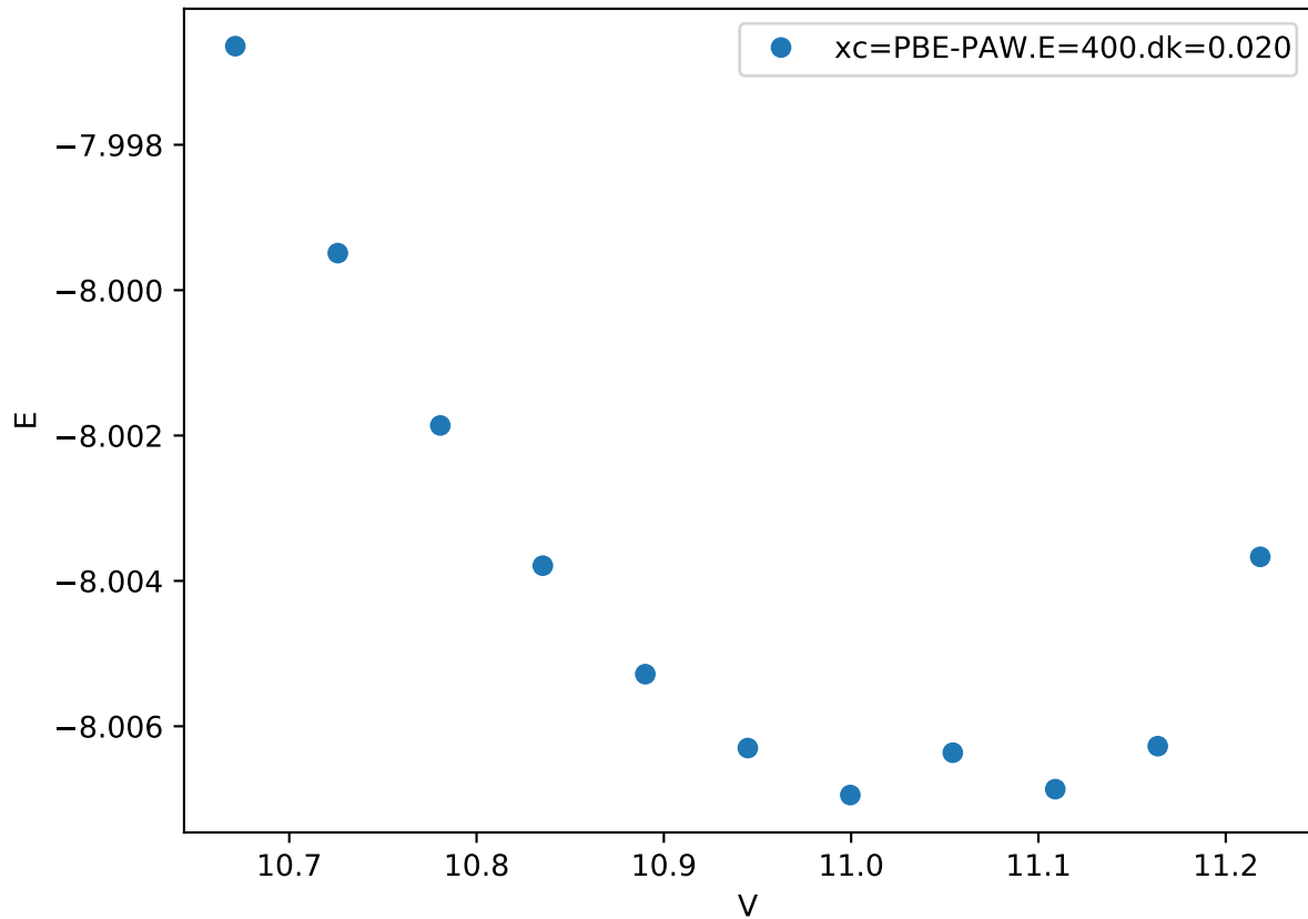
Cr_pv-Co_pv-W_sv/Cr_pv-Co_pv_chi-ABAB.FM_
