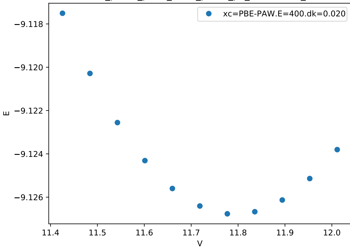
Cr_pv-Co_pv-W_sv/Cr_pv-Co_pv_mu-BAAAA_
