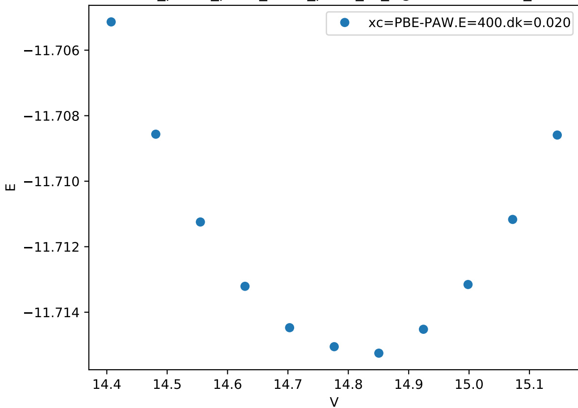
Cr_pv-Co_pv-W_sv/Cr_pv-W_sv_sigma-ABBAB.FM_
