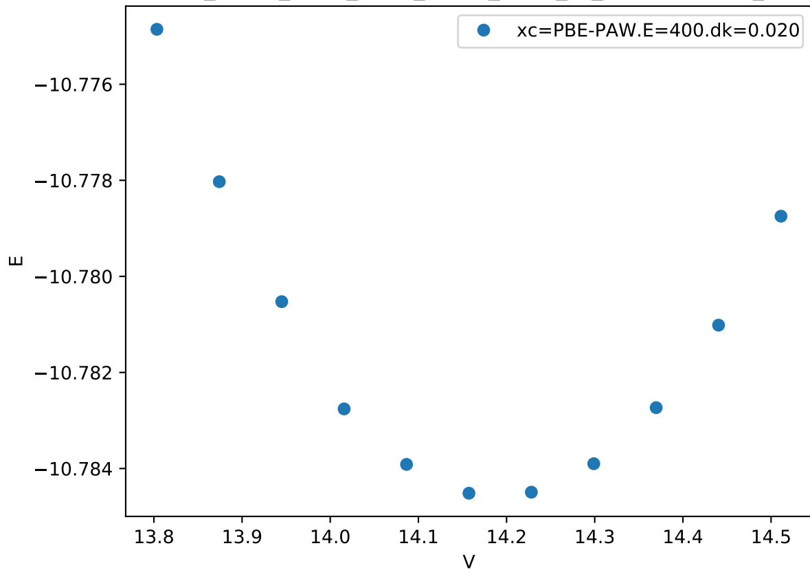
Cr_pv-Co_pv-W_sv/Cr_pv-Co_pv-W_sv_sigma-ABCAC_
