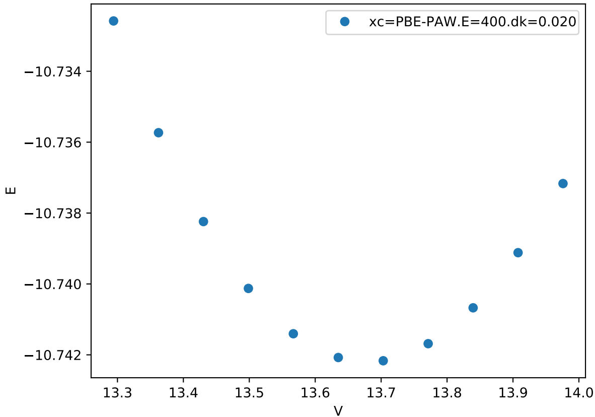
Cr_pv-Co_pv-W_sv/Cr_pv-W_sv_sigma-ABAAB.FM_
