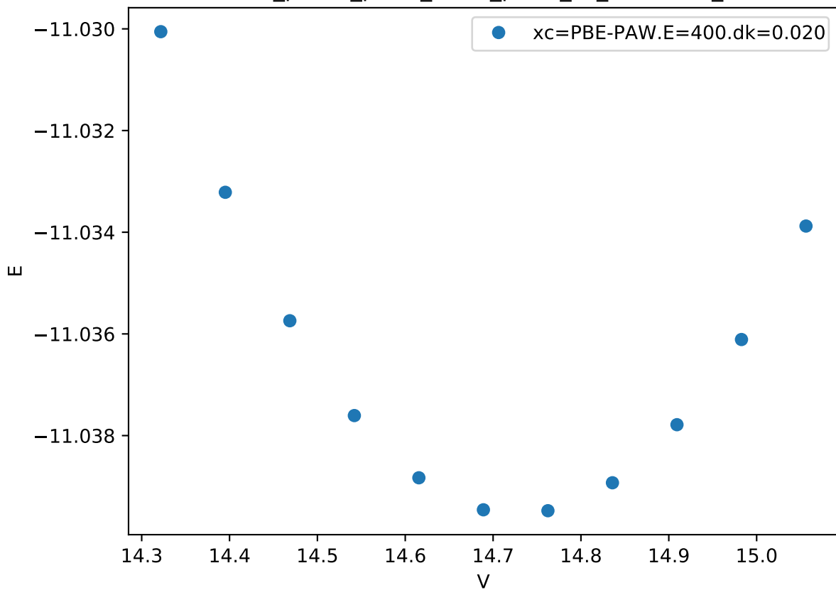
Cr_pv-Co_pv-W_sv/Cr_pv-W_sv_chi-ABAB_
