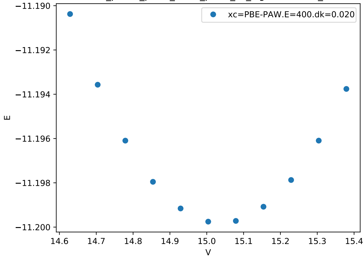
Cr_pv-Co_pv-W_sv/Cr_pv-W_sv_sigma-BAABB_
