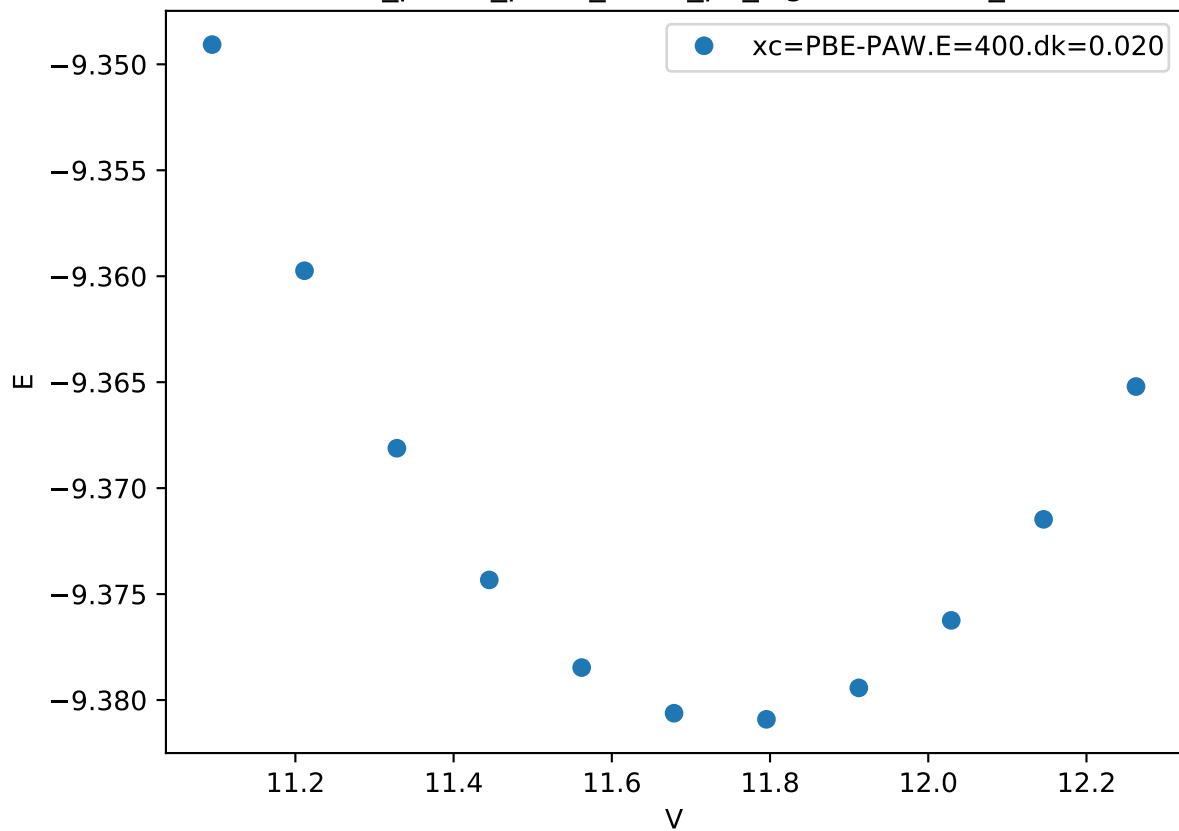
Cr_pv-Co_pv-W_sv/Cr_pv_sigma.DDDDD_
