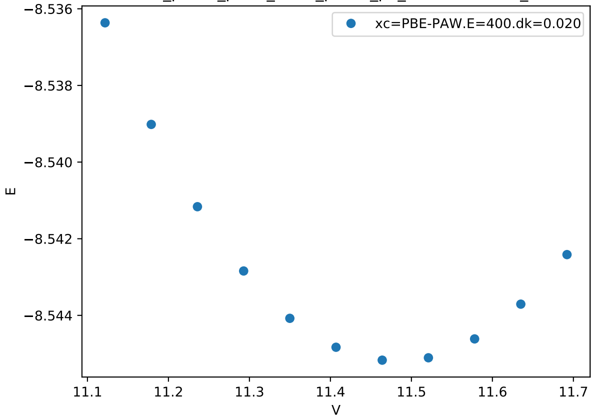
Cr_pv-Co_pv-W_sv/Cr_pv-Co_pv_mu-AAABB.FM_
