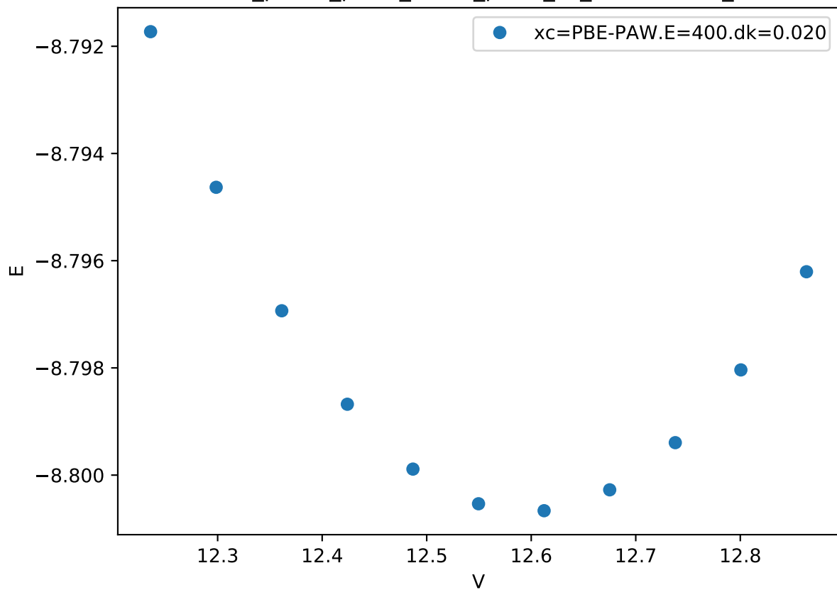
Cr_pv-Co_pv-W_sv/Co_pv-W_sv_C36-ABBAA_
