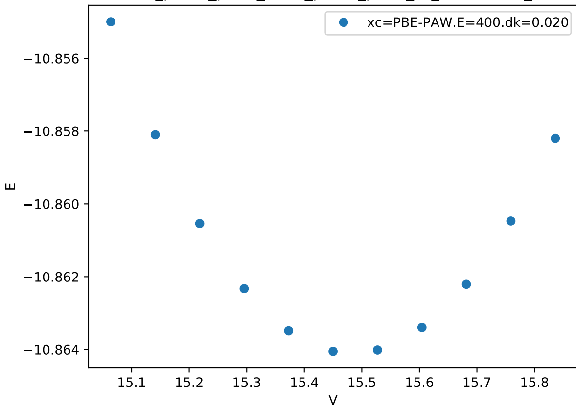
Cr_pv-Co_pv-W_sv/Cr_pv-Co_pv-W_sv_mu-BCAAC_
