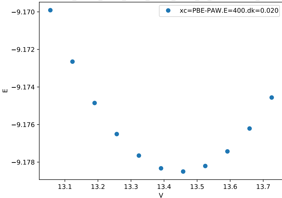
Cr_pv-Co_pv-W_sv/Cr_pv-Co_pv-W_sv_C36-AAABC_
