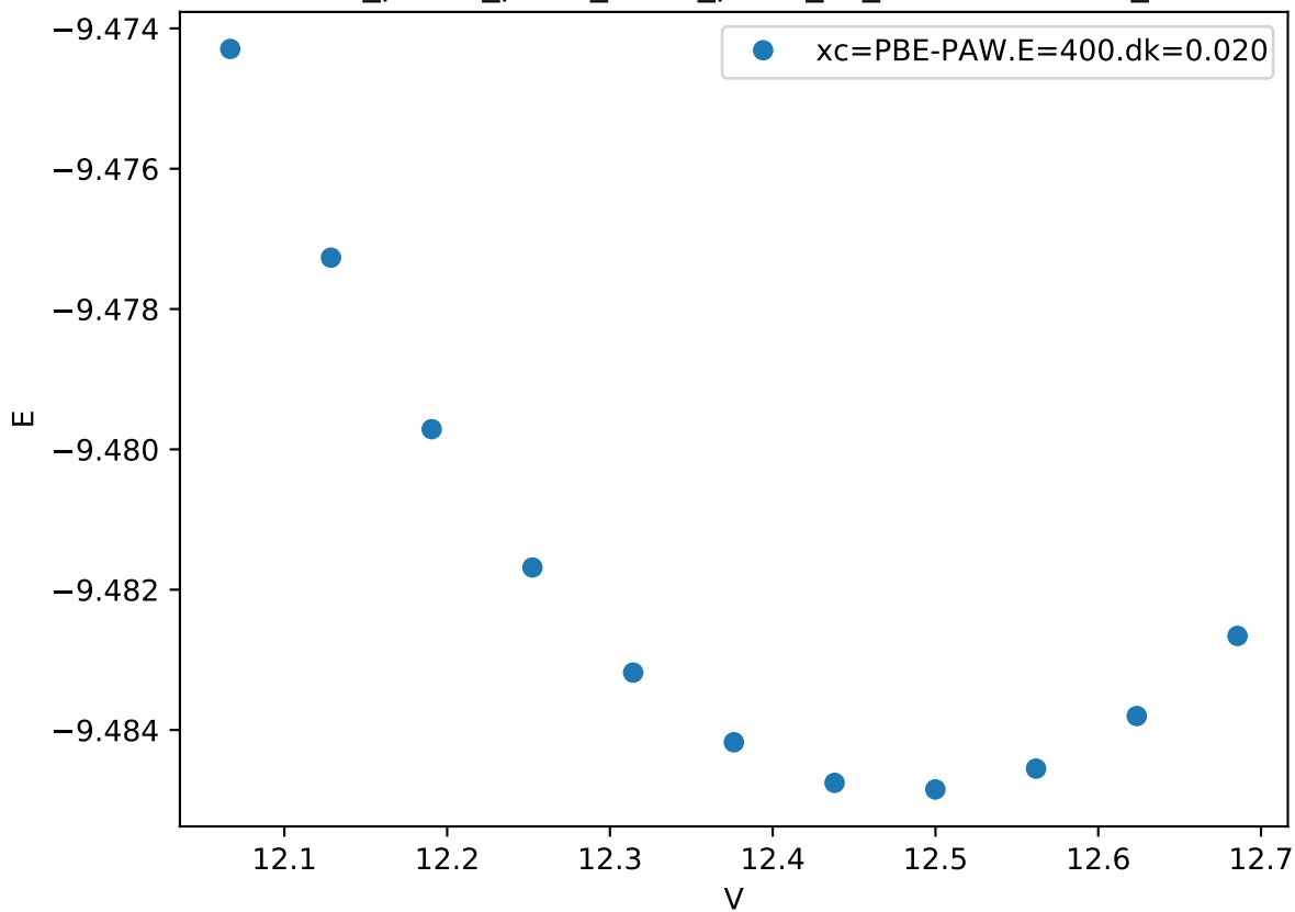
Cr_pv-Co_pv-W_sv/Cr_pv-W_sv_mu-BAAAA.FM_
