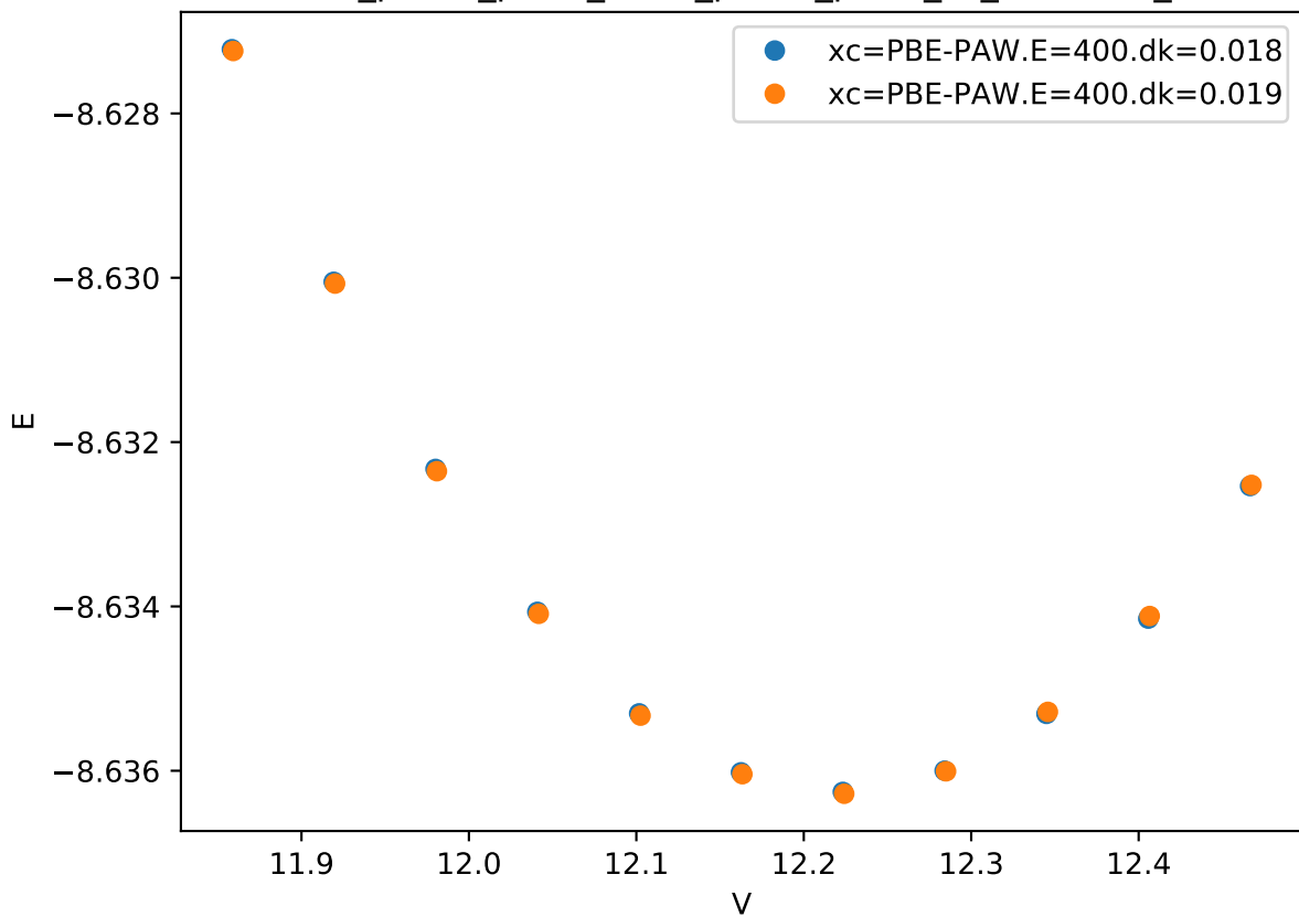
Cr_pv-Co_pv-W_sv/Cr_pv-Co_pv-W_sv_C14-CBA_
