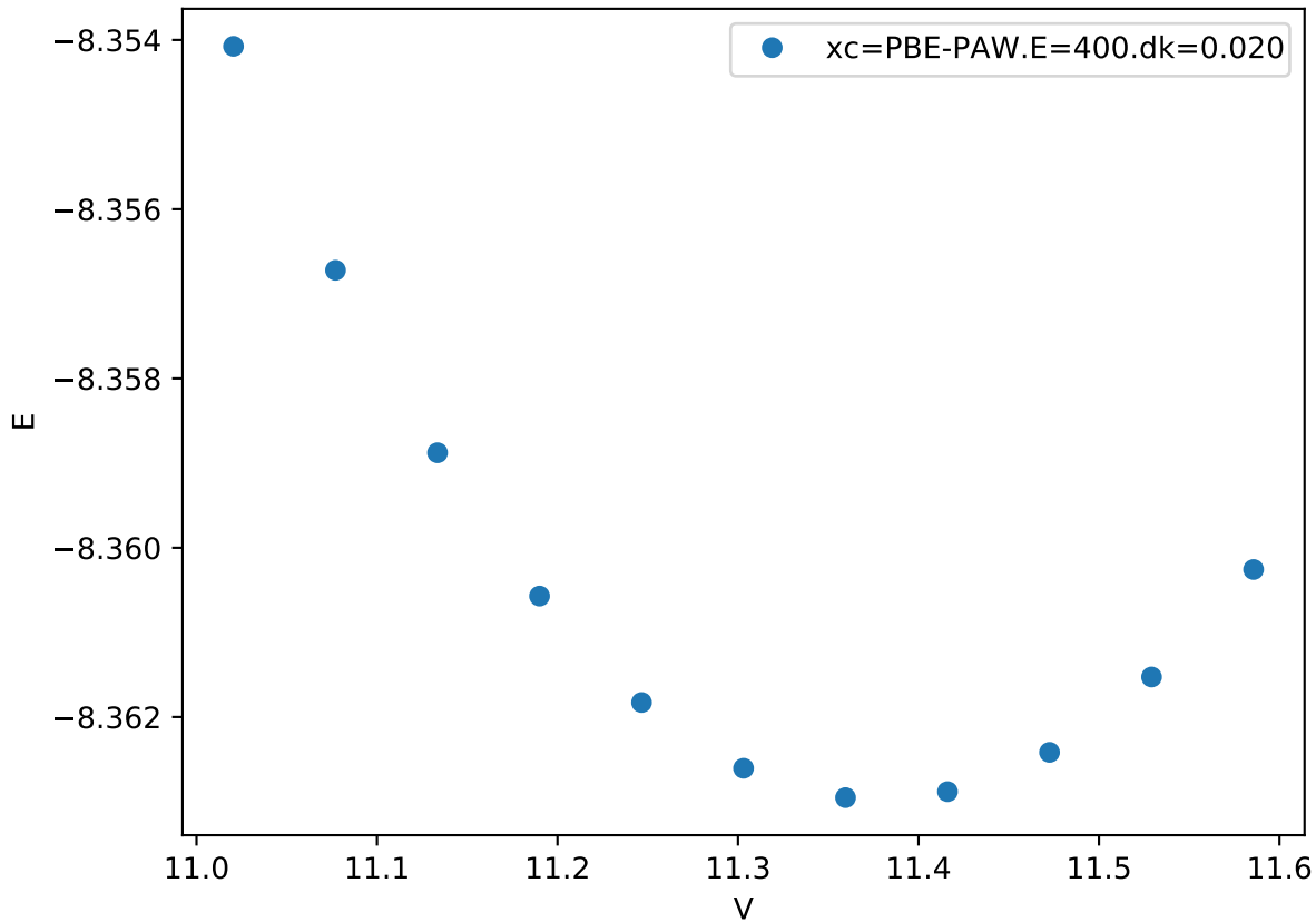
Cr_pv-Co_pv-W_sv/Cr_pv-Co_pv_mu-BAABB_
