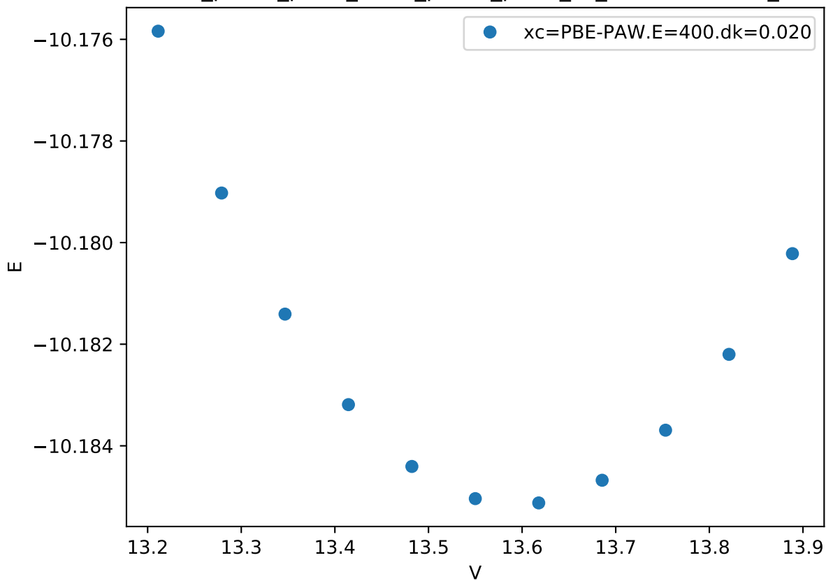
Cr_pv-Co_pv-W_sv/Cr_pv-Co_pv-W_sv_mu-CABCC.FM_
