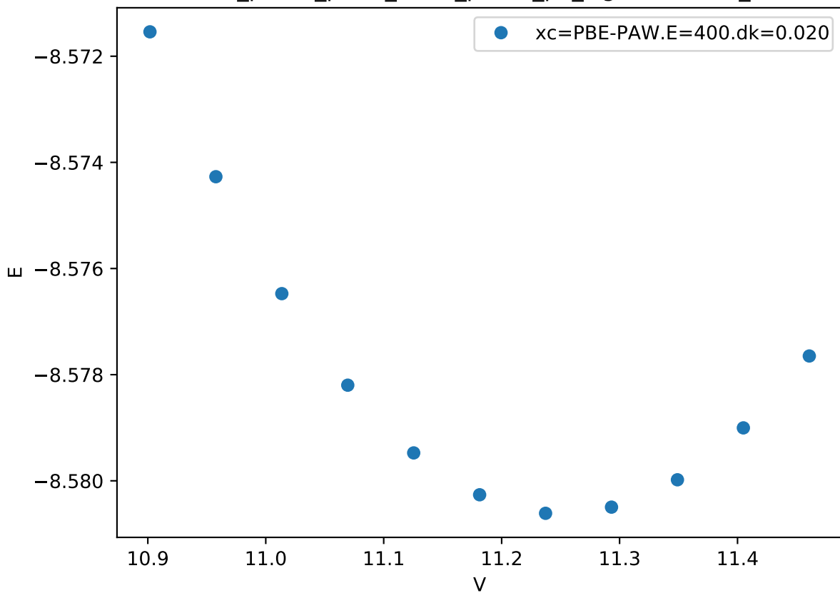
Cr_pv-Co_pv-W_sv/Cr_pv-Co_pv_sigma-BABAA_
