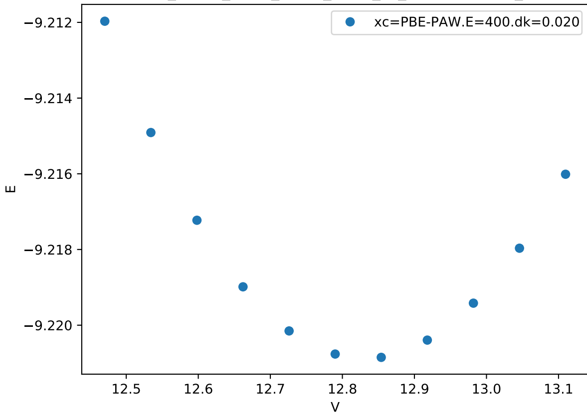
Cr_pv-Co_pv-W_sv/Co_pv-W_sv_sigma-ABBAA_
