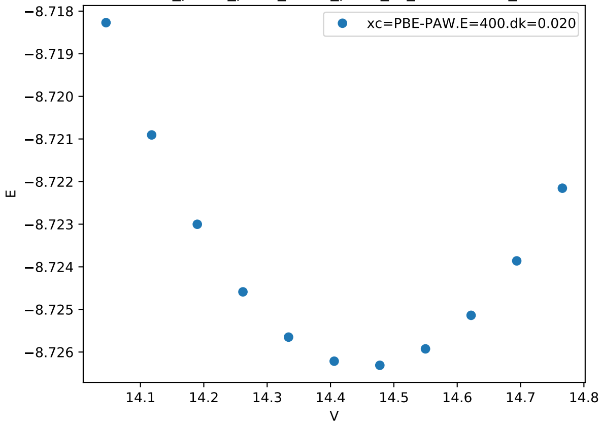
Cr_pv-Co_pv-W_sv/Co_pv-W_sv_C36-AABAB_
