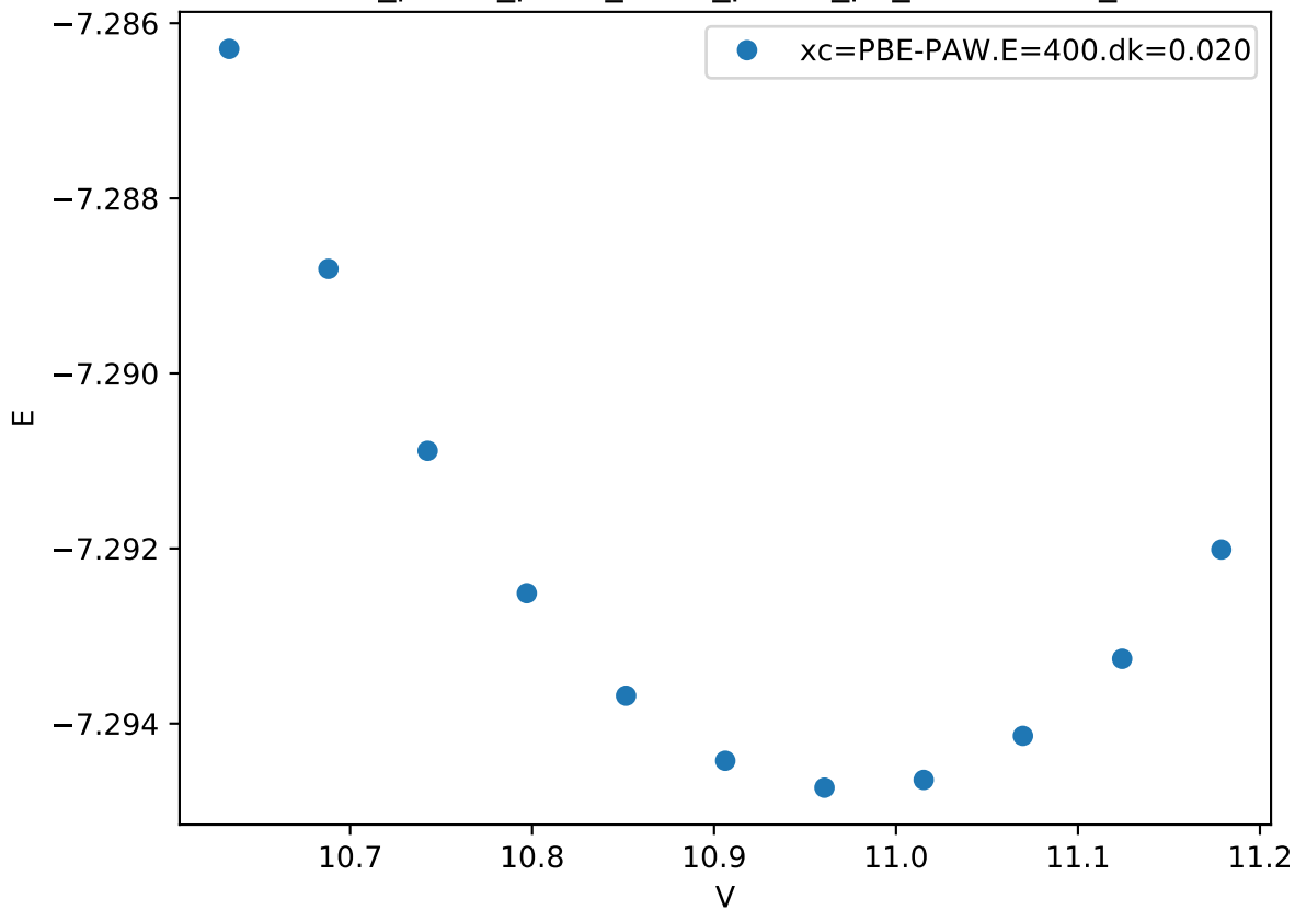
Cr_pv-Co_pv-W_sv/Cr_pv-Co_pv_mu-ABBAB_
