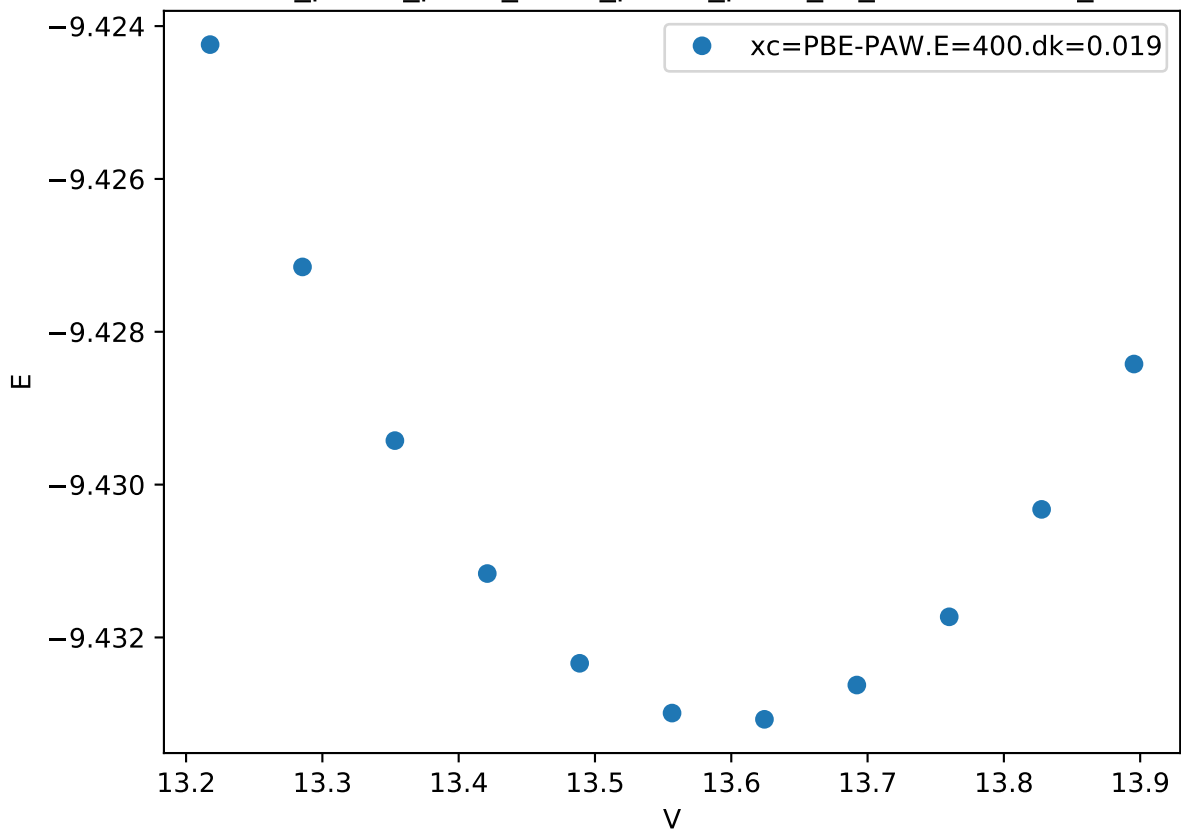
Cr_pv-Co_pv-W_sv/Cr_pv-Co_pv-W_sv_chi-BABC.FM_
