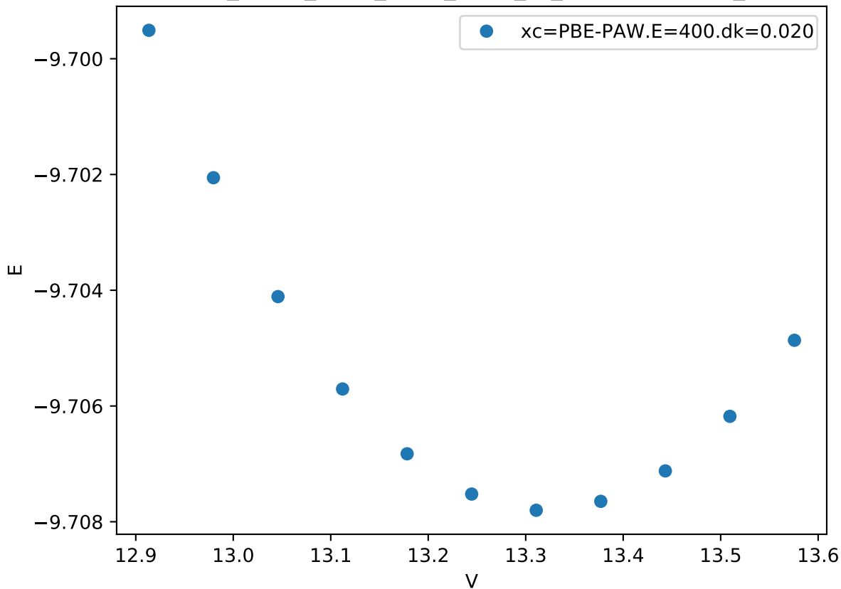
Cr_pv-Co_pv-W_sv/Cr_pv-W_sv_C36-AABAA.FM_
