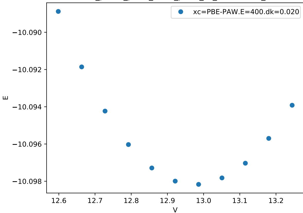
Cr_pv-Co_pv-W_sv/Cr_pv-W_sv_mu-BAABA_
