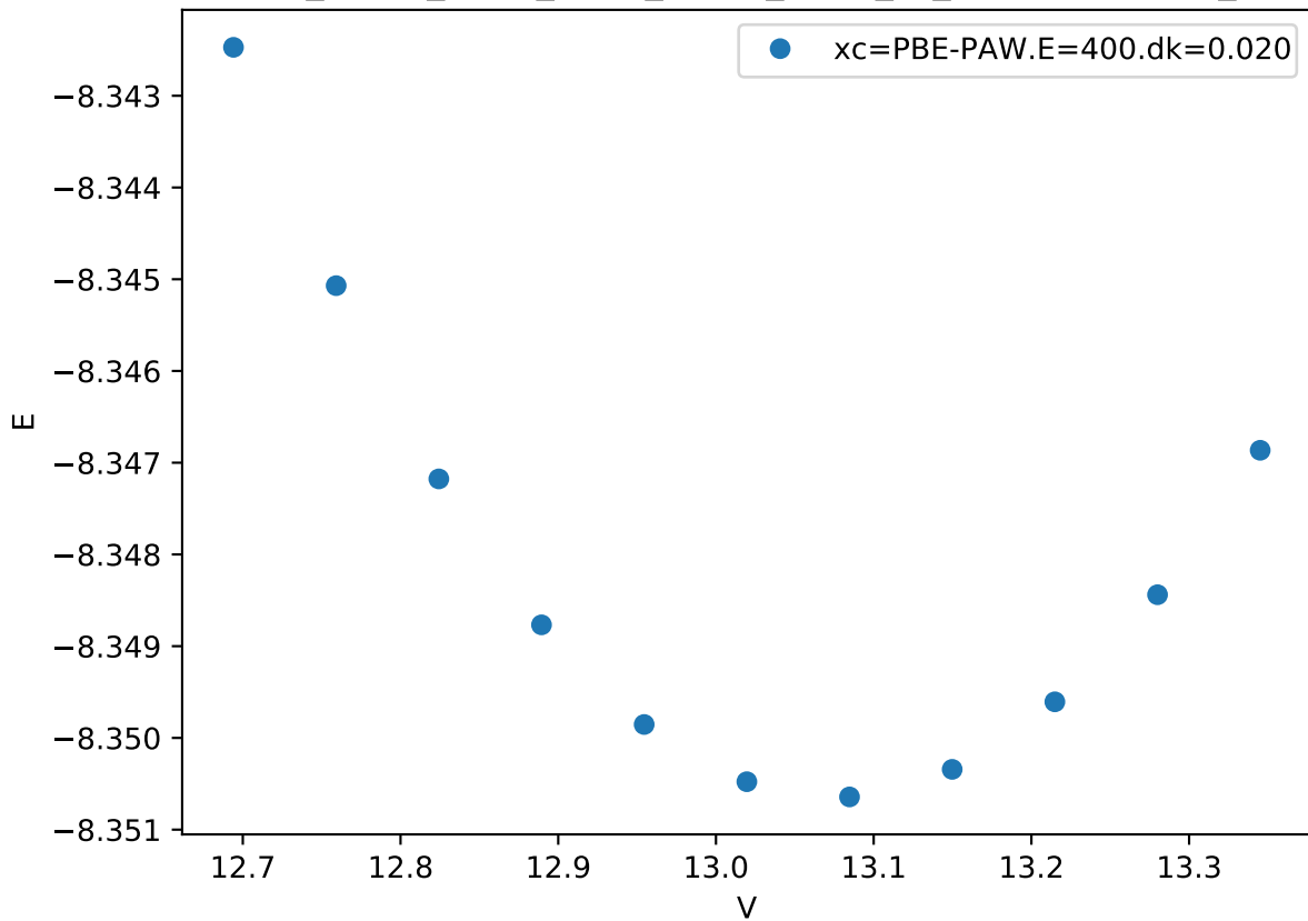
Cr_pv-Co_pv-W_sv/Cr_pv-Co_pv-W_sv_C36-BABCB.FM_
