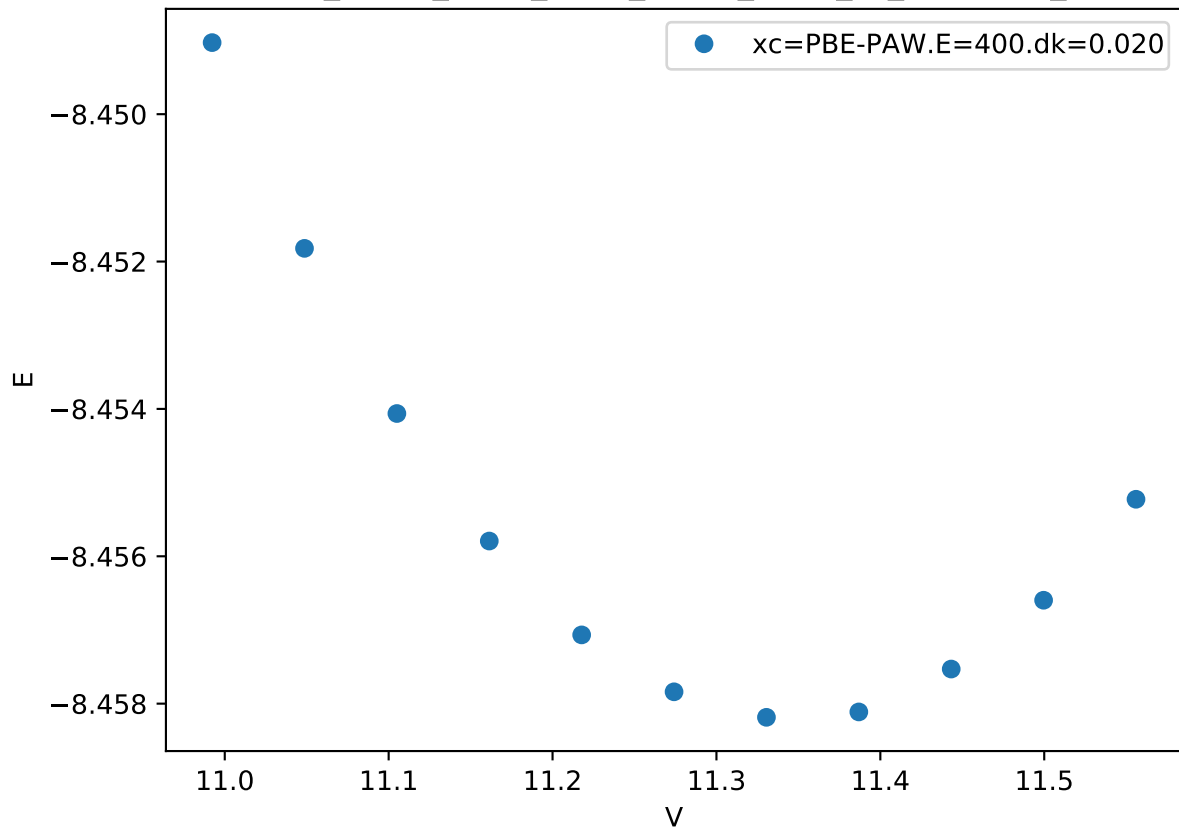
Cr_pv-Co_pv-W_sv/Cr_pv-Co_pv-W_sv_chi-CABA_
