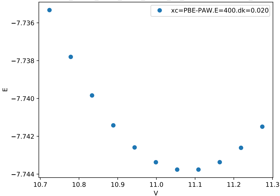
Cr_pv-Co_pv-W_sv/Cr_pv-Co_pv_sigma-ABBBA.FM_
