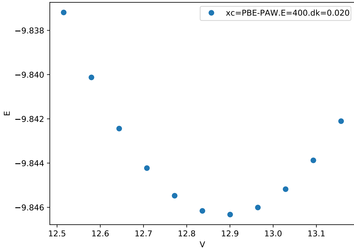
Cr_pv-Co_pv-W_sv/Cr_pv-Co_pv-W_sv_A15-AAAAABCC.FM_
