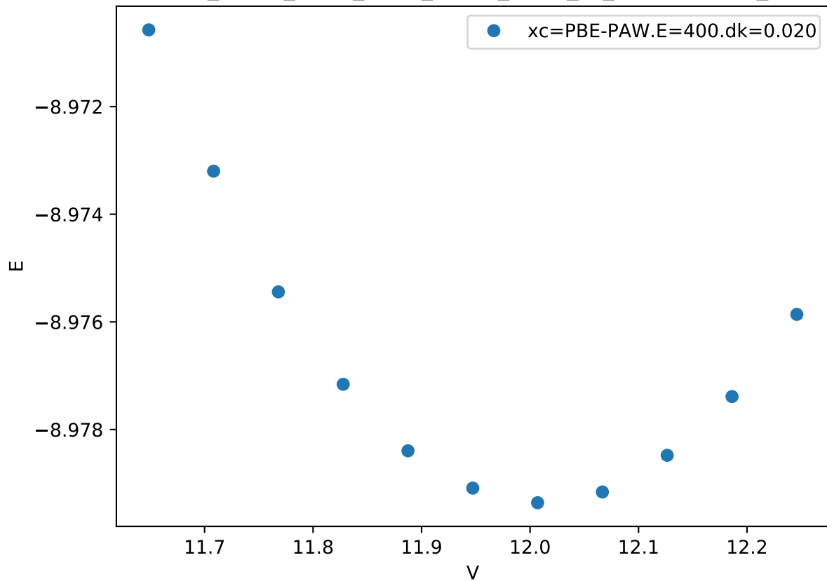
Cr_pv-Co_pv-W_sv/Cr_pv-Co_pv-W_sv_chi-CCBA.FM_
