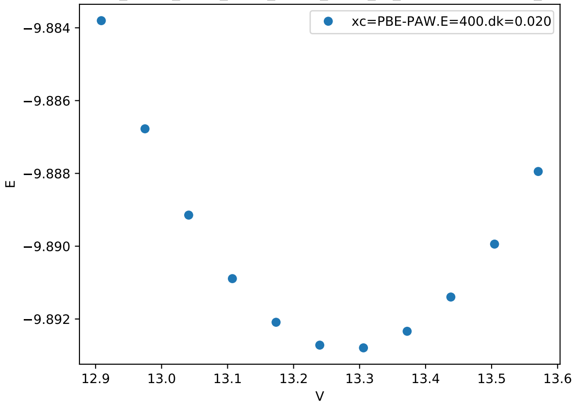
Cr_pv-Co_pv-W_sv/Cr_pv-Co_pv-W_sv_sigma-BCBAC.FM_
