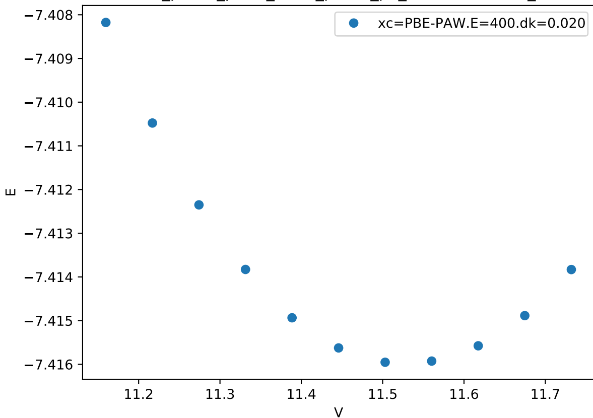
Cr_pv-Co_pv-W_sv/Cr_pv-Co_pv_C36-BBBAB.FM_
