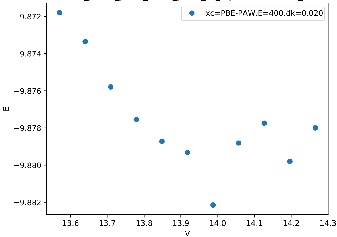
Cr_pv-Co_pv-W_sv/Co_pv-W_sv_sigma-AABBA.FM_
