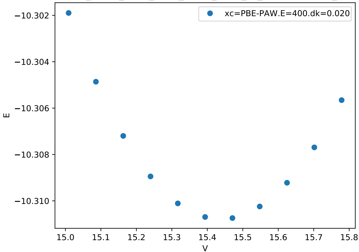
Cr_pv-Co_pv-W_sv/Cr_pv-Co_pv-W_sv_mu-CCBAA.FM_
