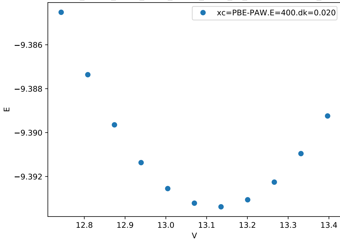
Cr_pv-Co_pv-W_sv/Cr_pv-Co_pv-W_sv_C36-CBCAB.FM_
