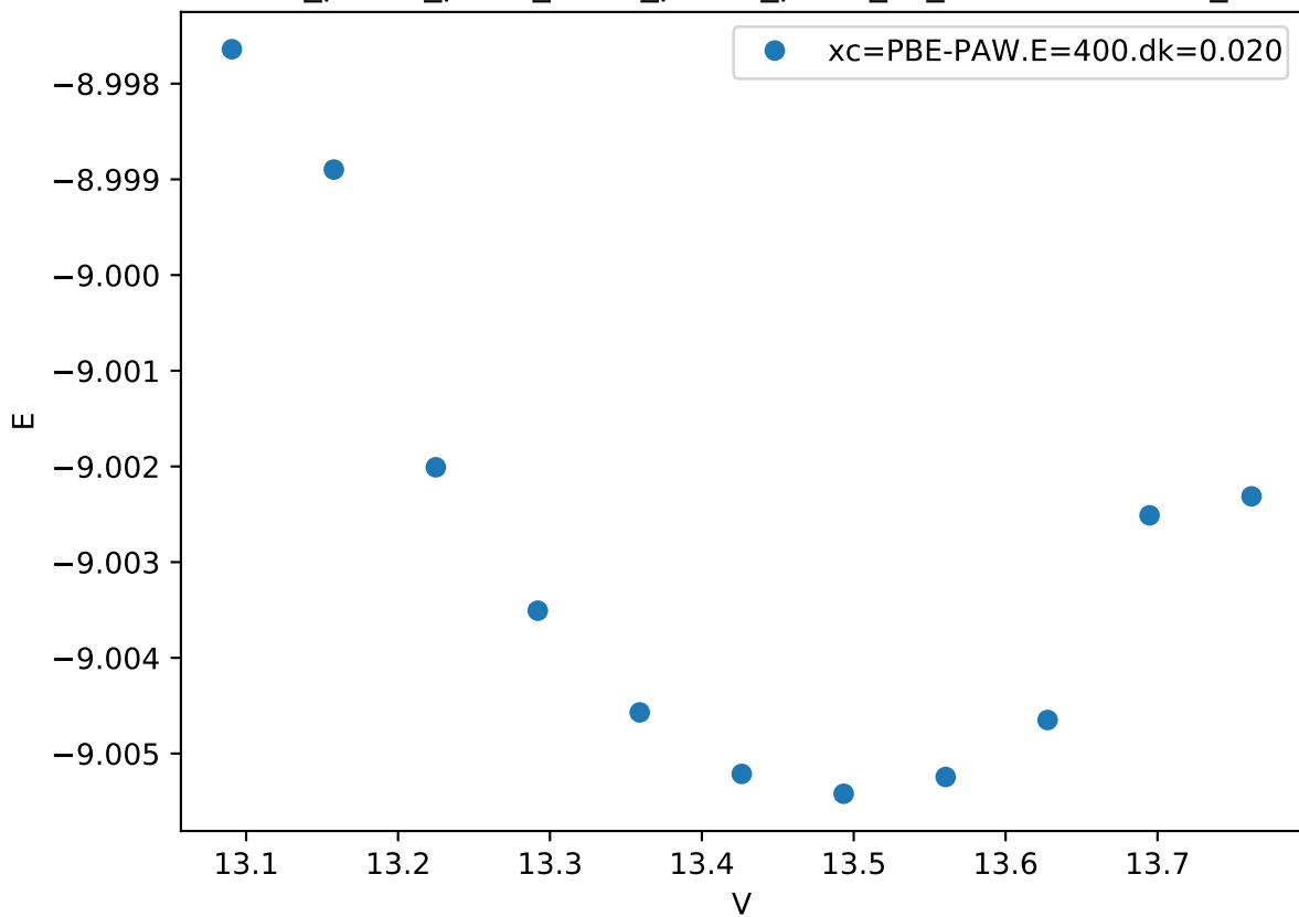
Cr_pv-Co_pv-W_sv/Cr_pv-Co_pv-W_sv_C36-BABAC.FM_
