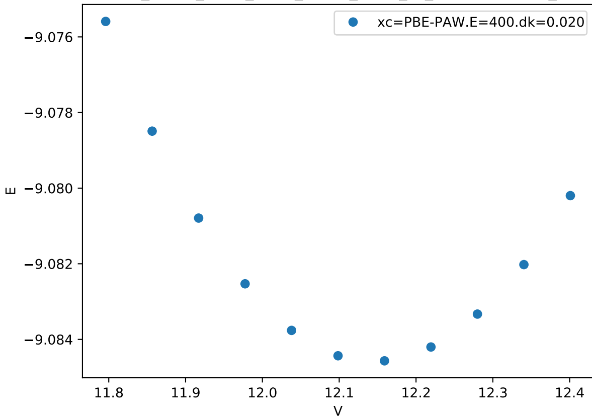
Cr_pv-Co_pv-W_sv/Cr_pv-Co_pv-W_sv_mu-CBACA.FM_
