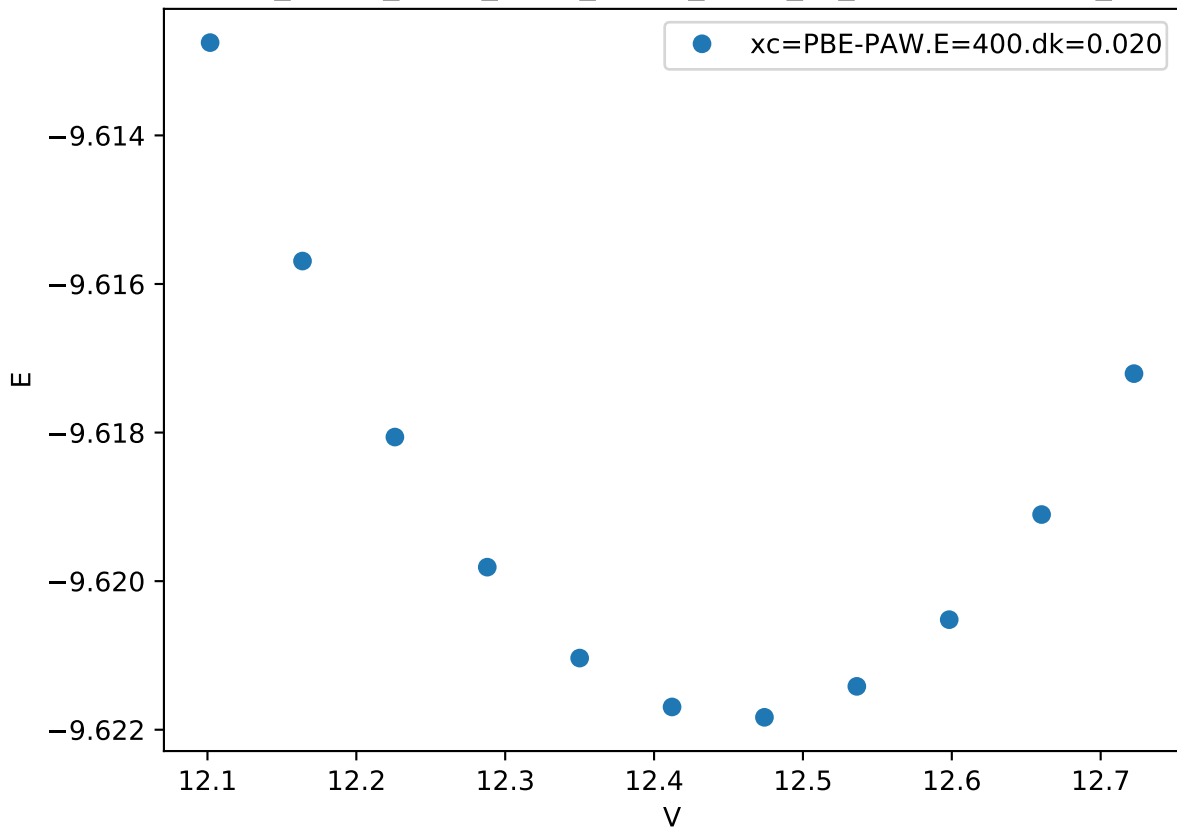
Cr_pv-Co_pv-W_sv/Cr_pv-Co_pv-W_sv_C36-CCBAB.FM_
