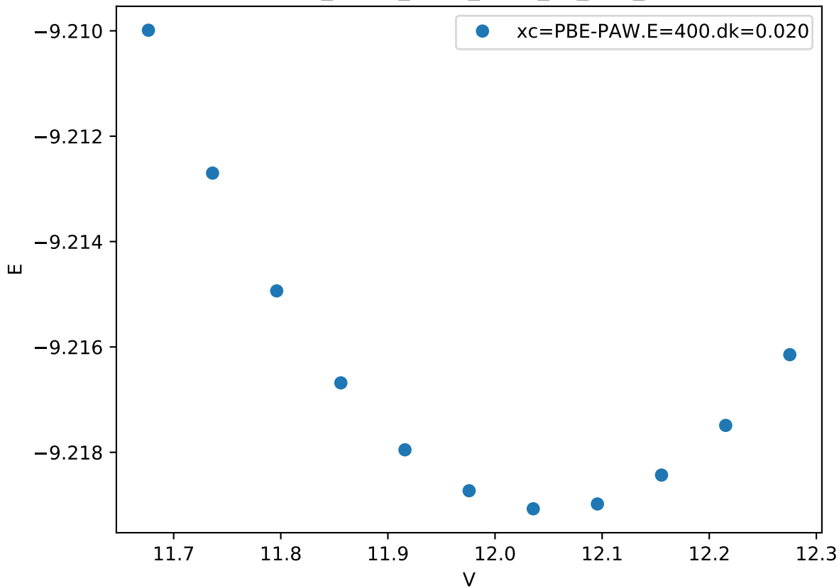
Cr_pv-Co_pv-W_sv/Cr_pv_C14_
