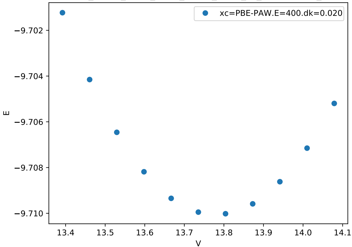
Cr_pv-Co_pv-W_sv/Cr_pv-Co_pv-W_sv_C36-BCBAC_
