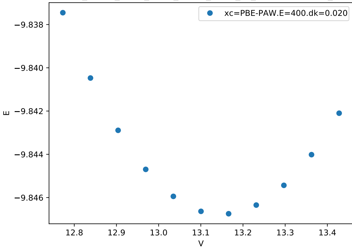
Cr_pv-Co_pv-W_sv/Cr_pv-Co_pv-W_sv_C36-ACCAB.FM_
