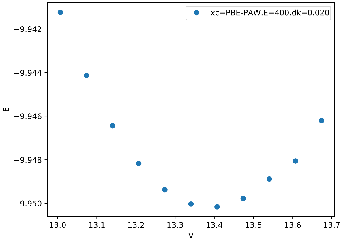
Cr_pv-Co_pv-W_sv/Cr_pv-Co_pv-W_sv_C36-CBCAA_
