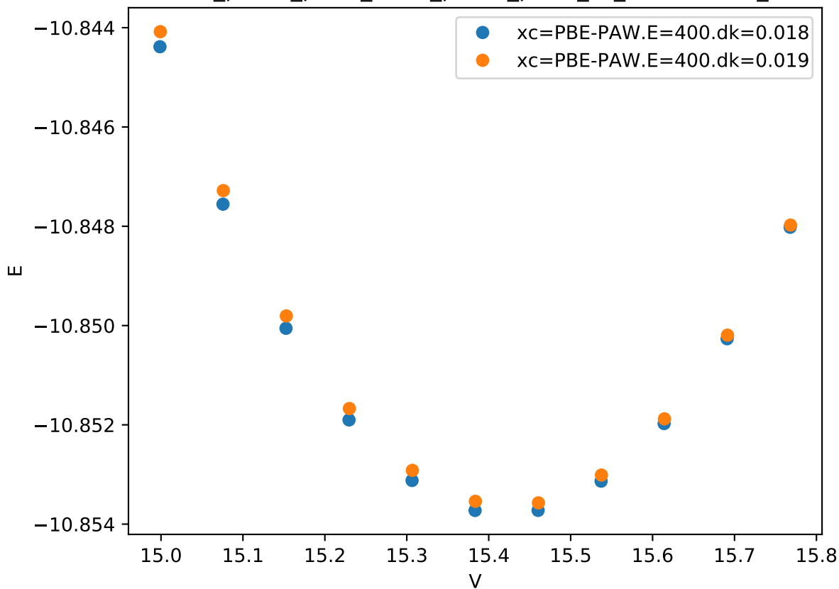
Cr_pv-Co_pv-W_sv/Cr_pv-Co_pv-W_sv_C36-BCACC_
