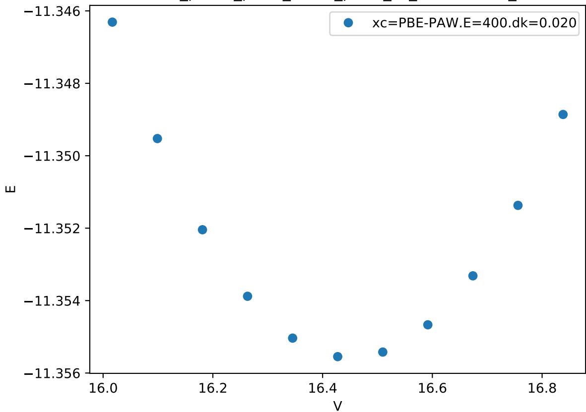
Cr_pv-Co_pv-W_sv/Co_pv-W_sv_C36-BABBB_
