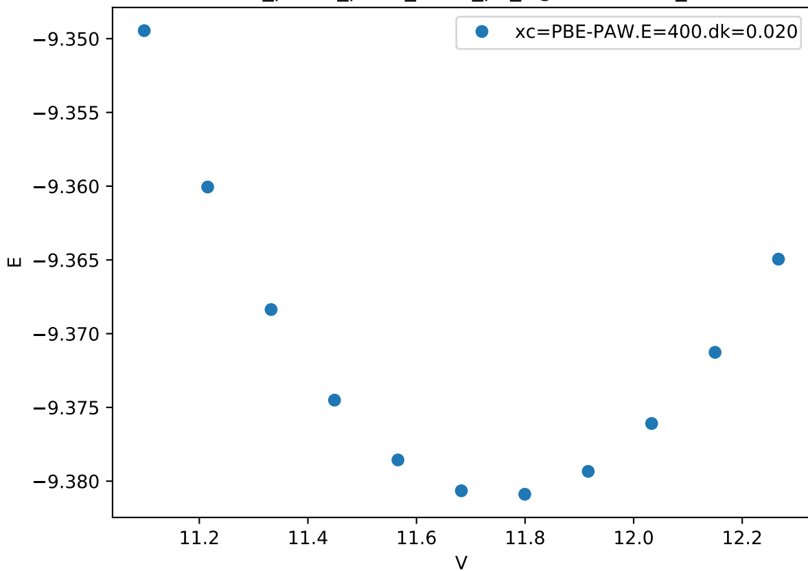
Cr_pv-Co_pv-W_sv/Cr_pv_sigma.UUDUU_
