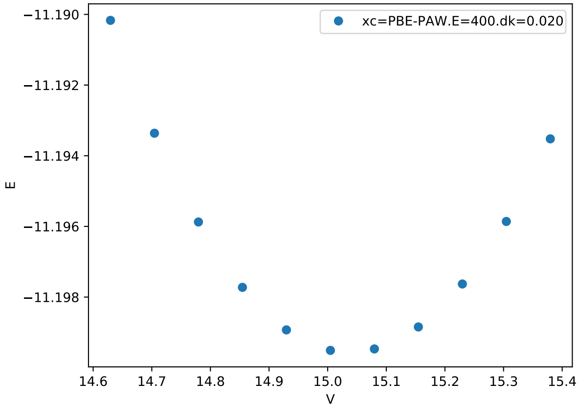
Cr_pv-Co_pv-W_sv/Cr_pv-W_sv_sigma-BAABB.FM_
