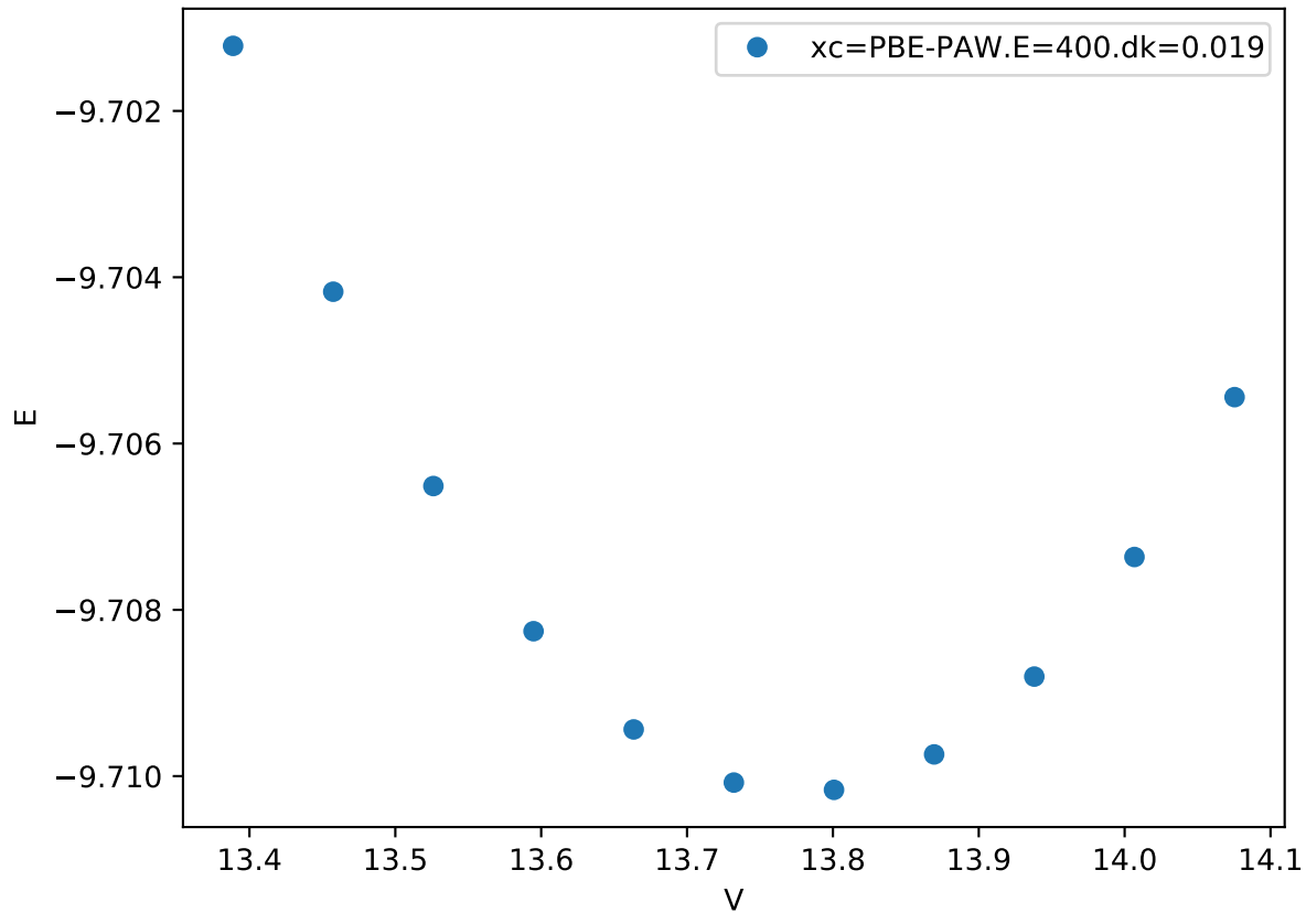
Cr_pv-Co_pv-W_sv/Cr_pv-Co_pv-W_sv_C36-BCBAC.FM_
