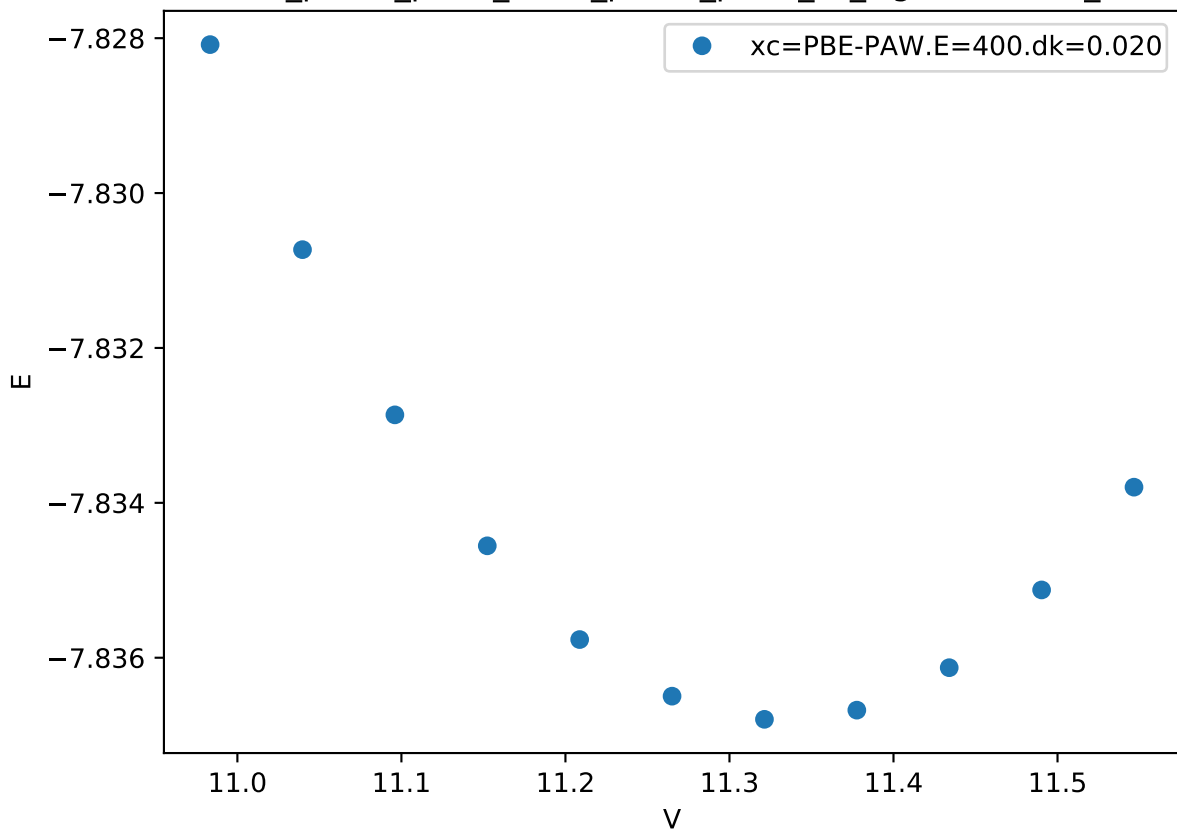
Cr_pv-Co_pv-W_sv/Cr_pv-Co_pv-W_sv_sigma-CBBAB_
