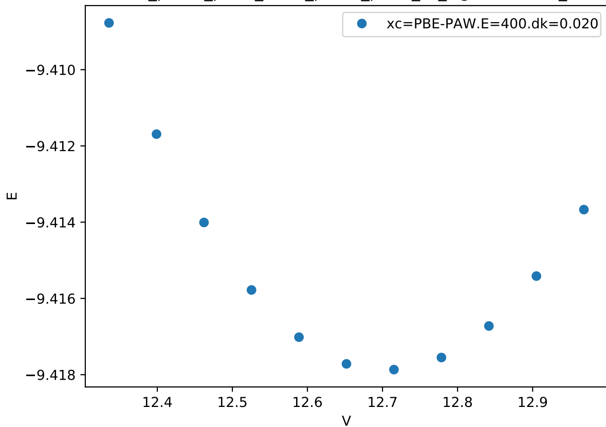
Cr_pv-Co_pv-W_sv/Cr_pv-Co_pv-W_sv_sigma-BABCA_
