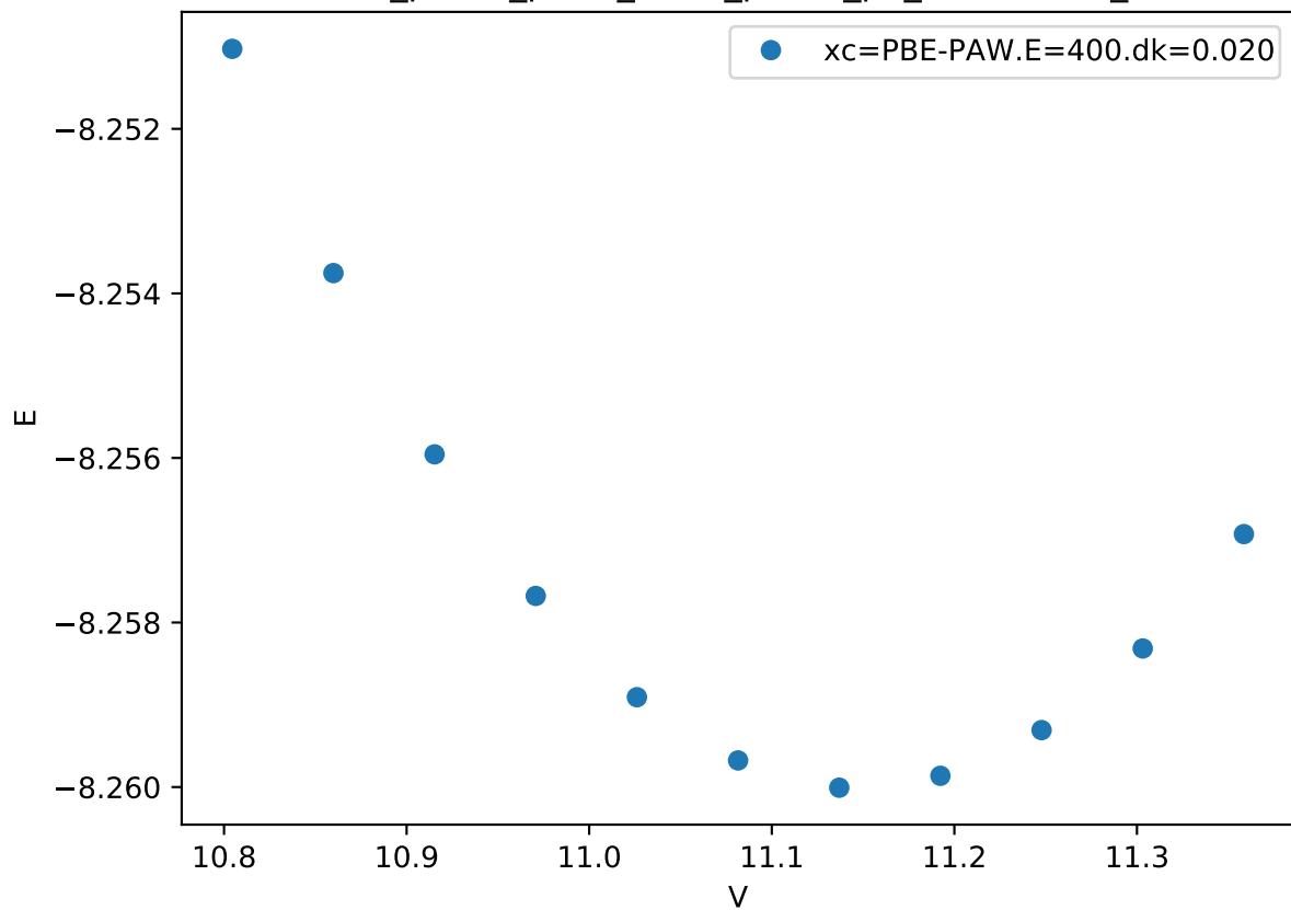
Cr_pv-Co_pv-W_sv/Cr_pv-Co_pv_mu-ABAAA_
