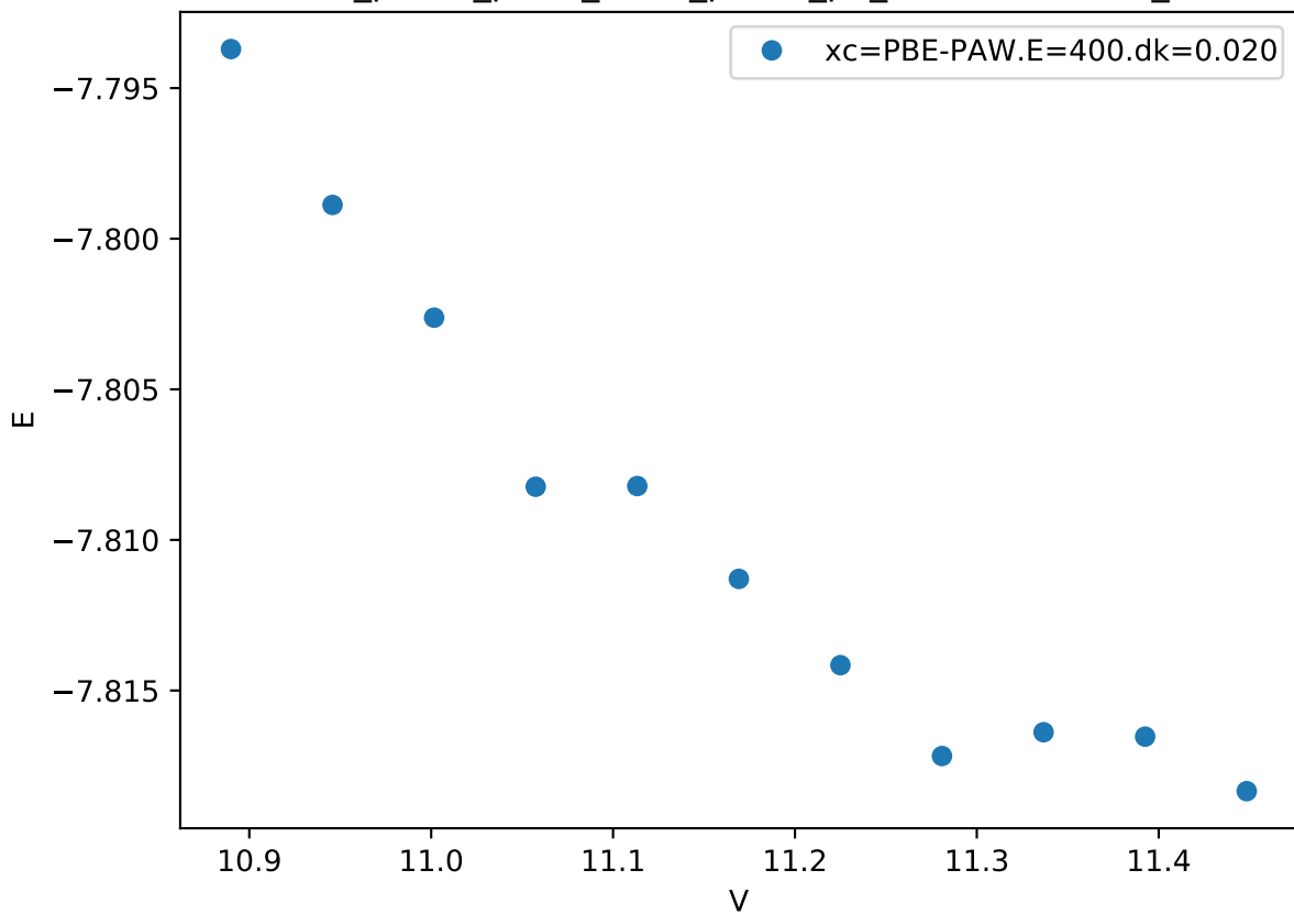
Cr_pv-Co_pv-W_sv/Cr_pv-Co_pv_C36-BABBA.FM_
