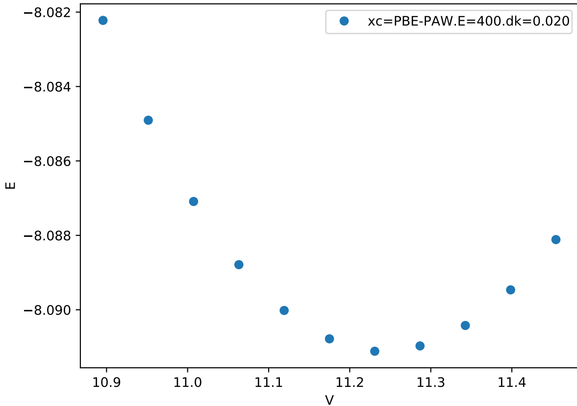
Cr_pv-Co_pv-W_sv/Cr_pv-Co_pv_C36-AAABB_
