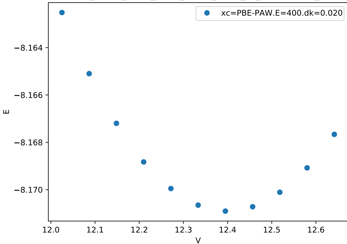
Cr_pv-Co_pv-W_sv/Cr_pv-Co_pv-W_sv_C36-BBCBA_
