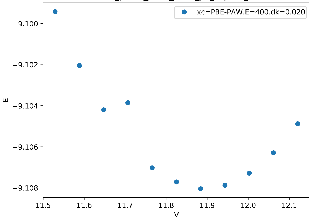
Cr_pv-Co_pv-W_sv/Cr_pv_hcp.FM_
