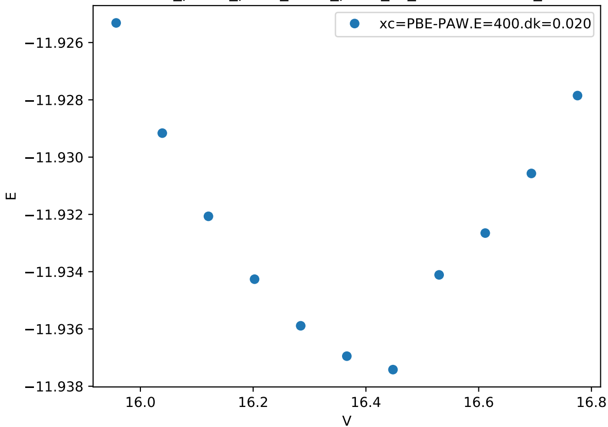
Cr_pv-Co_pv-W_sv/Cr_pv-W_sv_mu-BBABB.FM_
