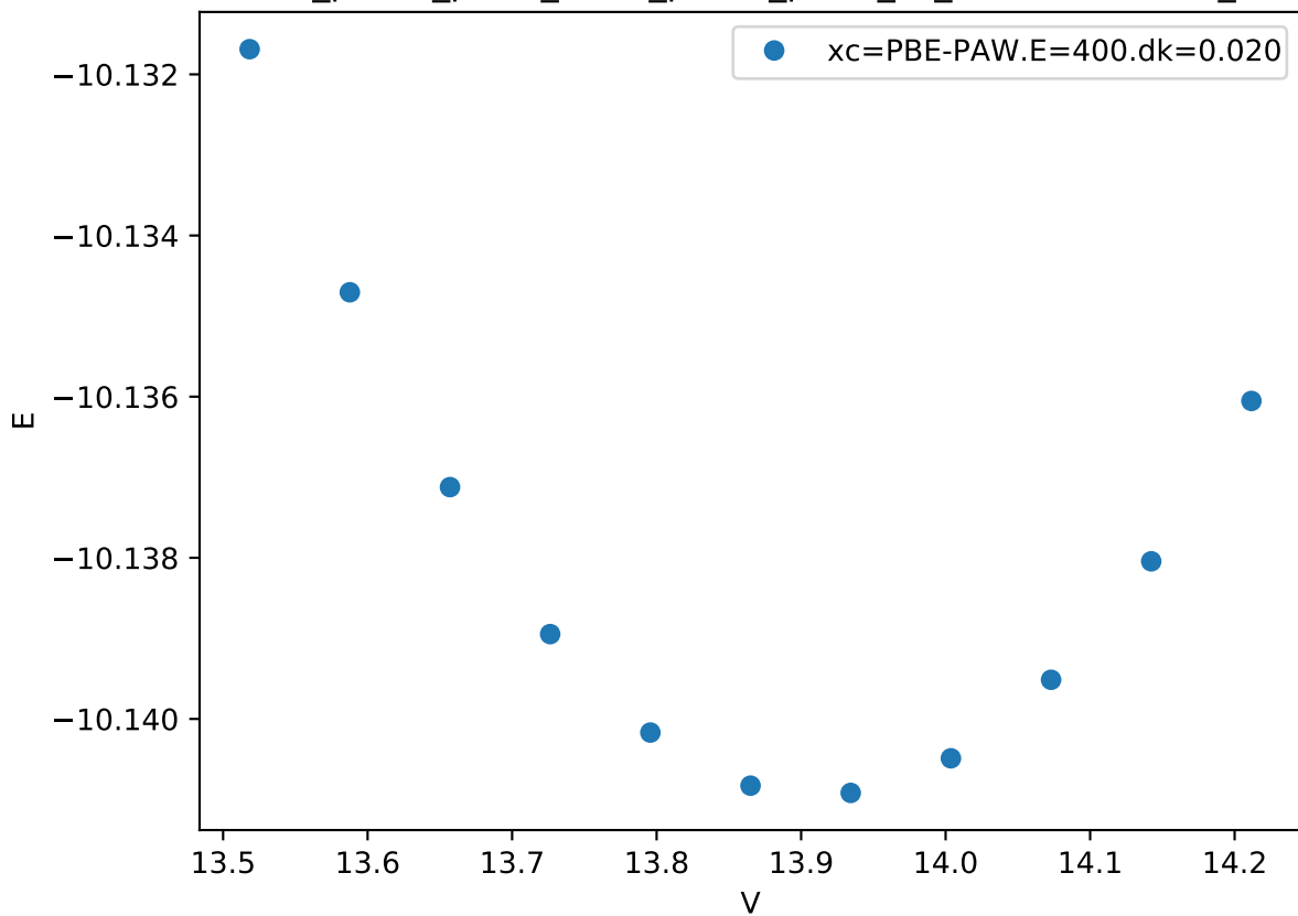
Cr_pv-Co_pv-W_sv/Cr_pv-Co_pv-W_sv_C36-CABAC.FM_
