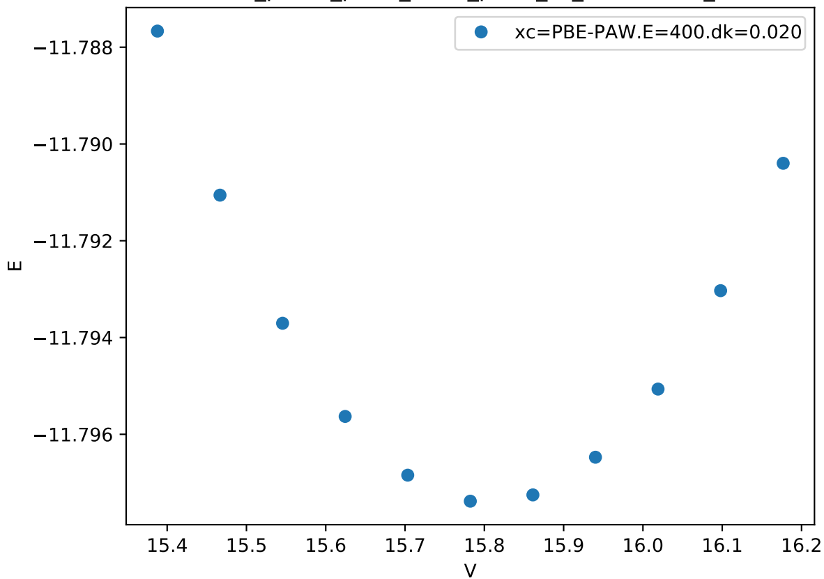
Cr_pv-Co_pv-W_sv/Cr_pv-W_sv_mu-ABBBA_
