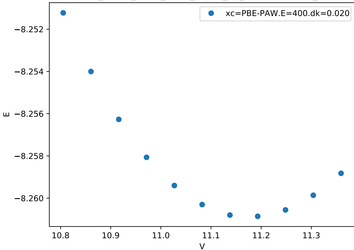
Cr_pv-Co_pv-W_sv/Cr_pv-Co_pv_mu-ABAAA.FM_
