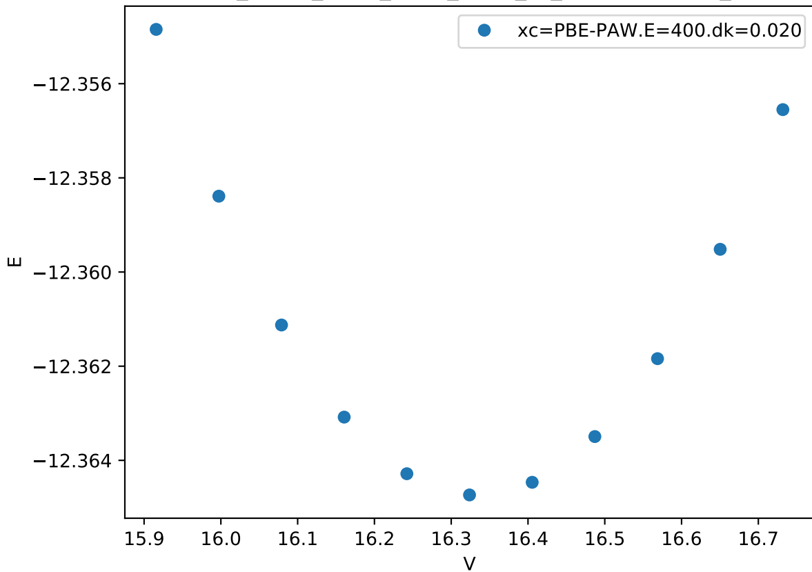
Cr_pv-Co_pv-W_sv/Cr_pv-W_sv_mu-ABBBB.FM_
