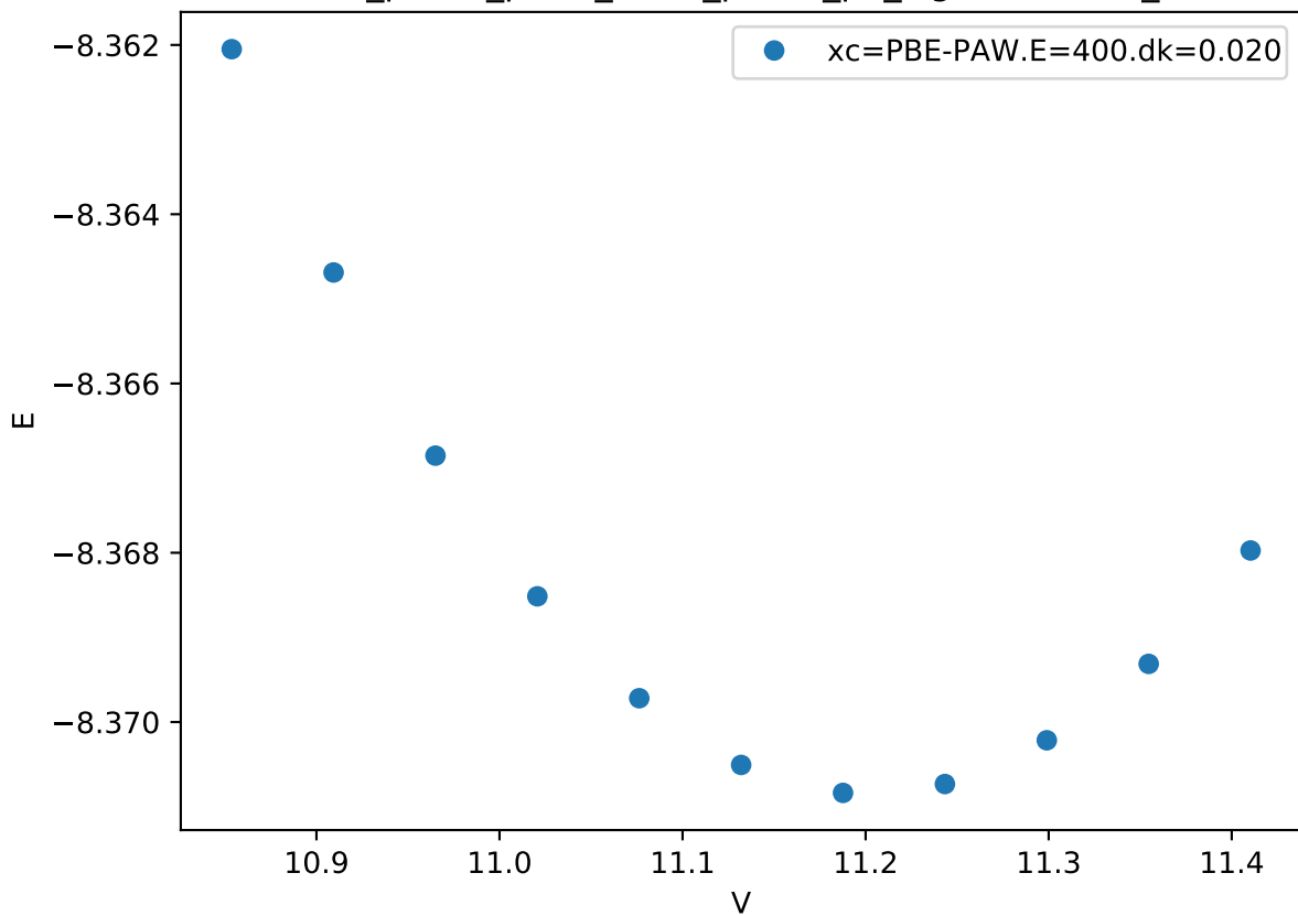
Cr_pv-Co_pv-W_sv/Cr_pv-Co_pv_sigma-ABBAA_
