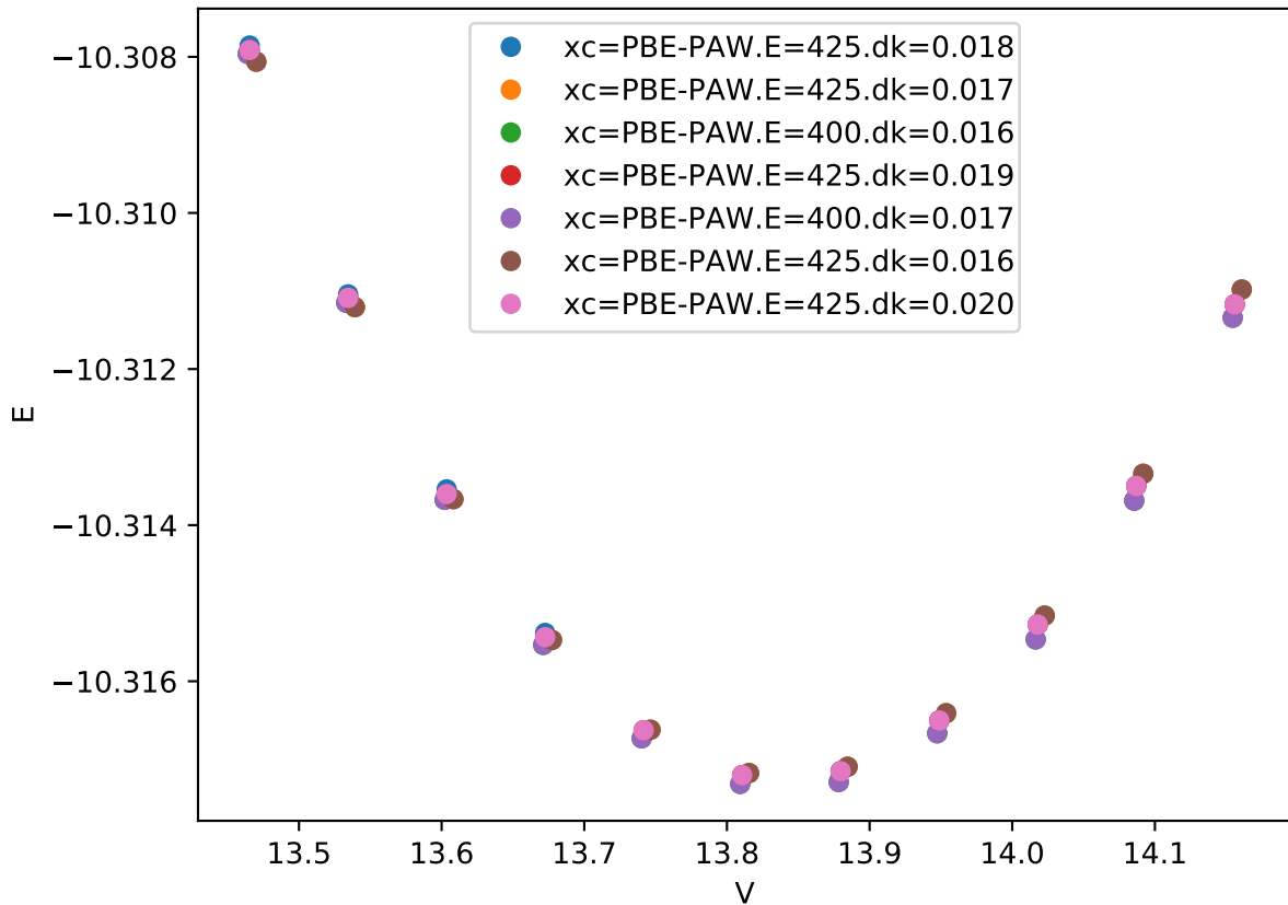
Cr_pv-Co_pv-W_sv/Co_pv-W_sv_chi-BBBA_
