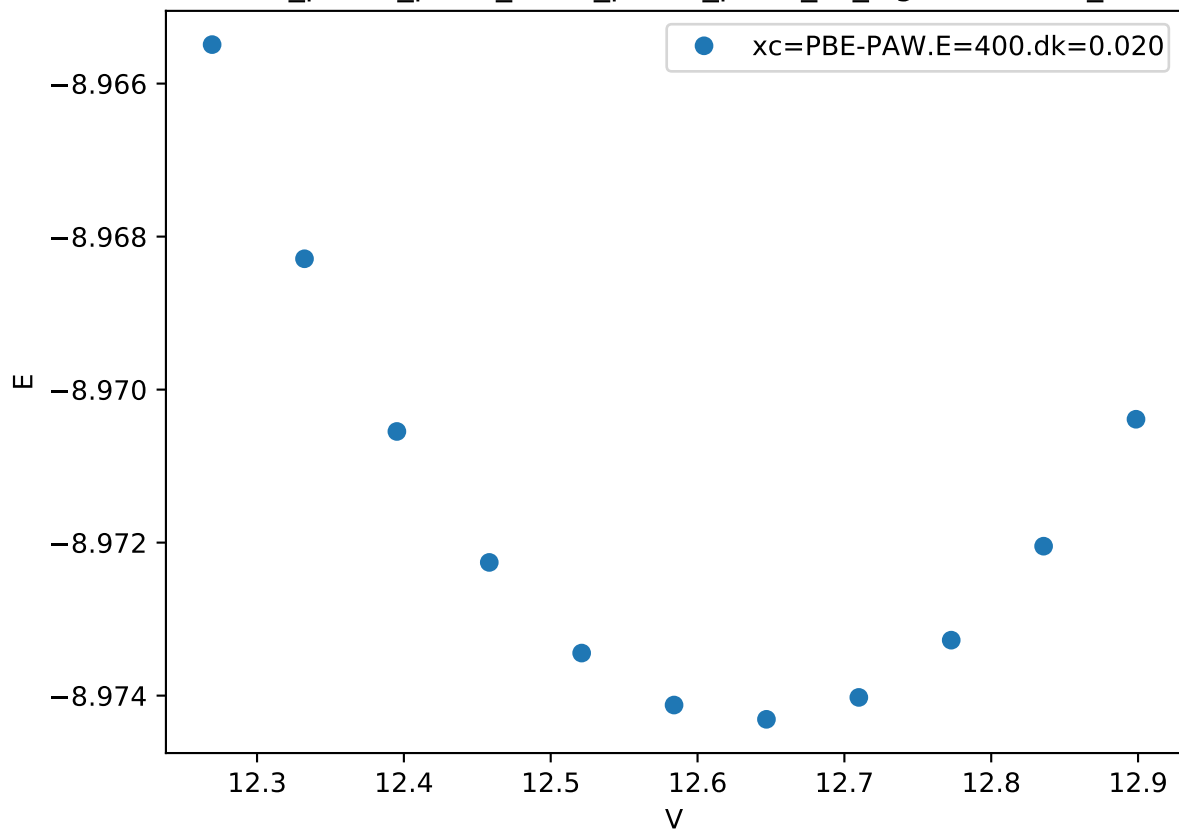
Cr_pv-Co_pv-W_sv/Cr_pv-Co_pv-W_sv_sigma-BBACB_
