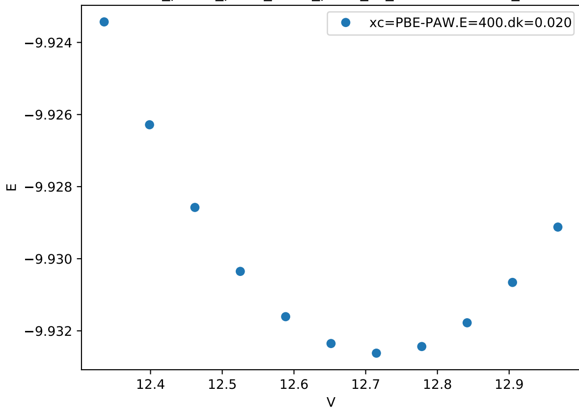
Cr_pv-Co_pv-W_sv/Cr_pv-W_sv_C36-BAAAA.FM_
