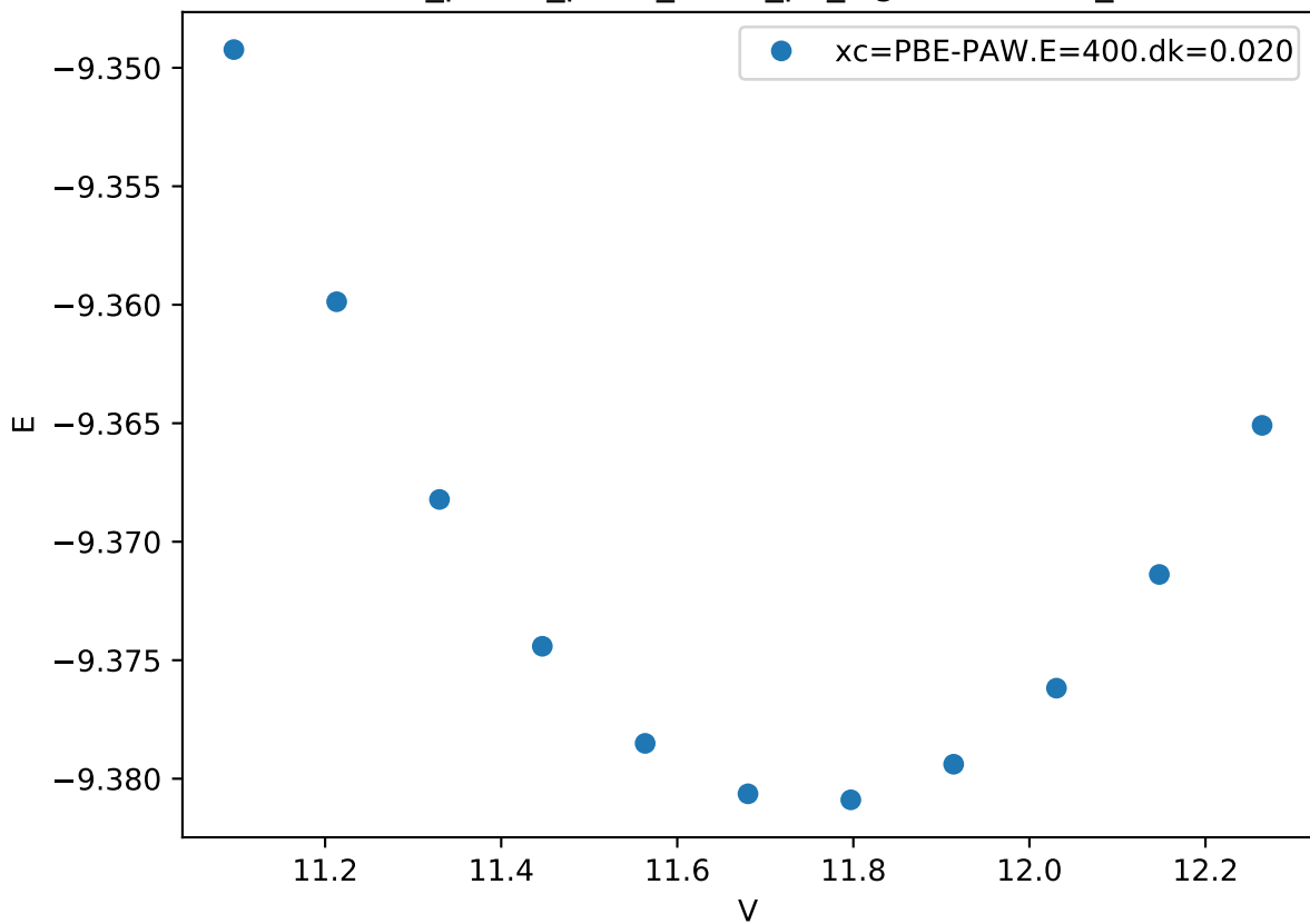
Cr_pv-Co_pv-W_sv/Cr_pv_sigma.DUUUU_
