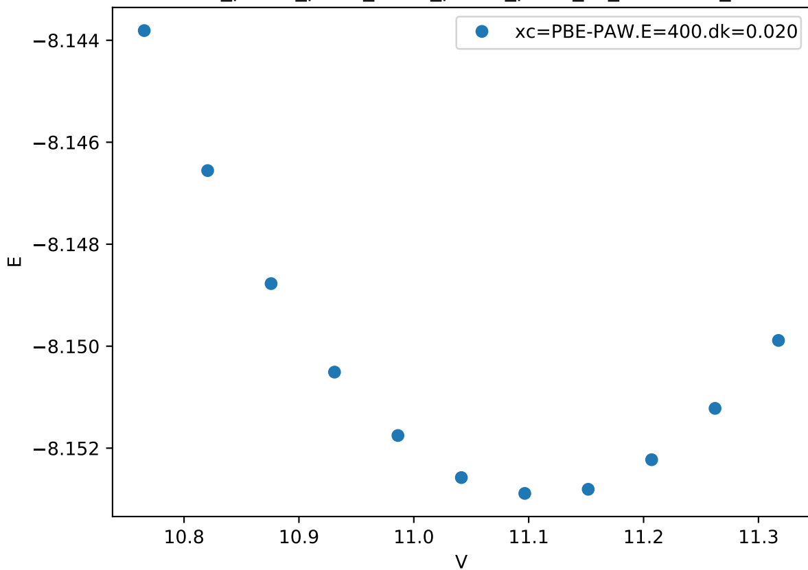
Cr_pv-Co_pv-W_sv/Cr_pv-Co_pv-W_sv_chi-CBAB_
