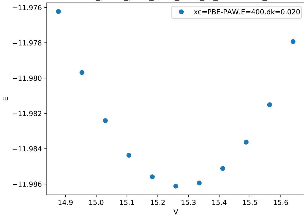
Cr_pv-Co_pv-W_sv/Cr_pv-W_sv_A15-BA.FM_
