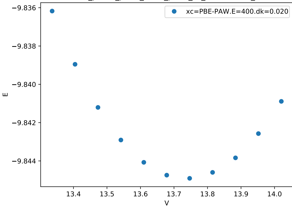
Cr_pv-Co_pv-W_sv/Cr_pv-W_sv_C36-AAABA_
