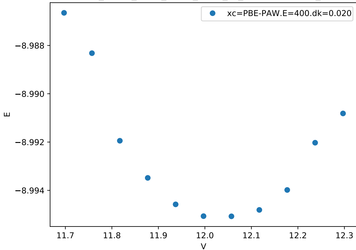
Cr_pv-Co_pv-W_sv/Co_pv-W_sv_C36-BBAAA.FM_
