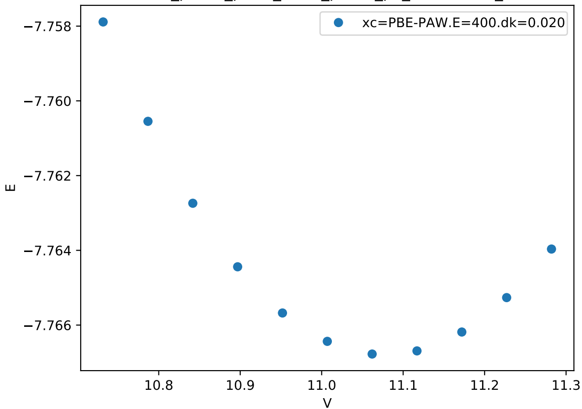
Cr_pv-Co_pv-W_sv/Cr_pv-Co_pv_mu-ABAAB_
