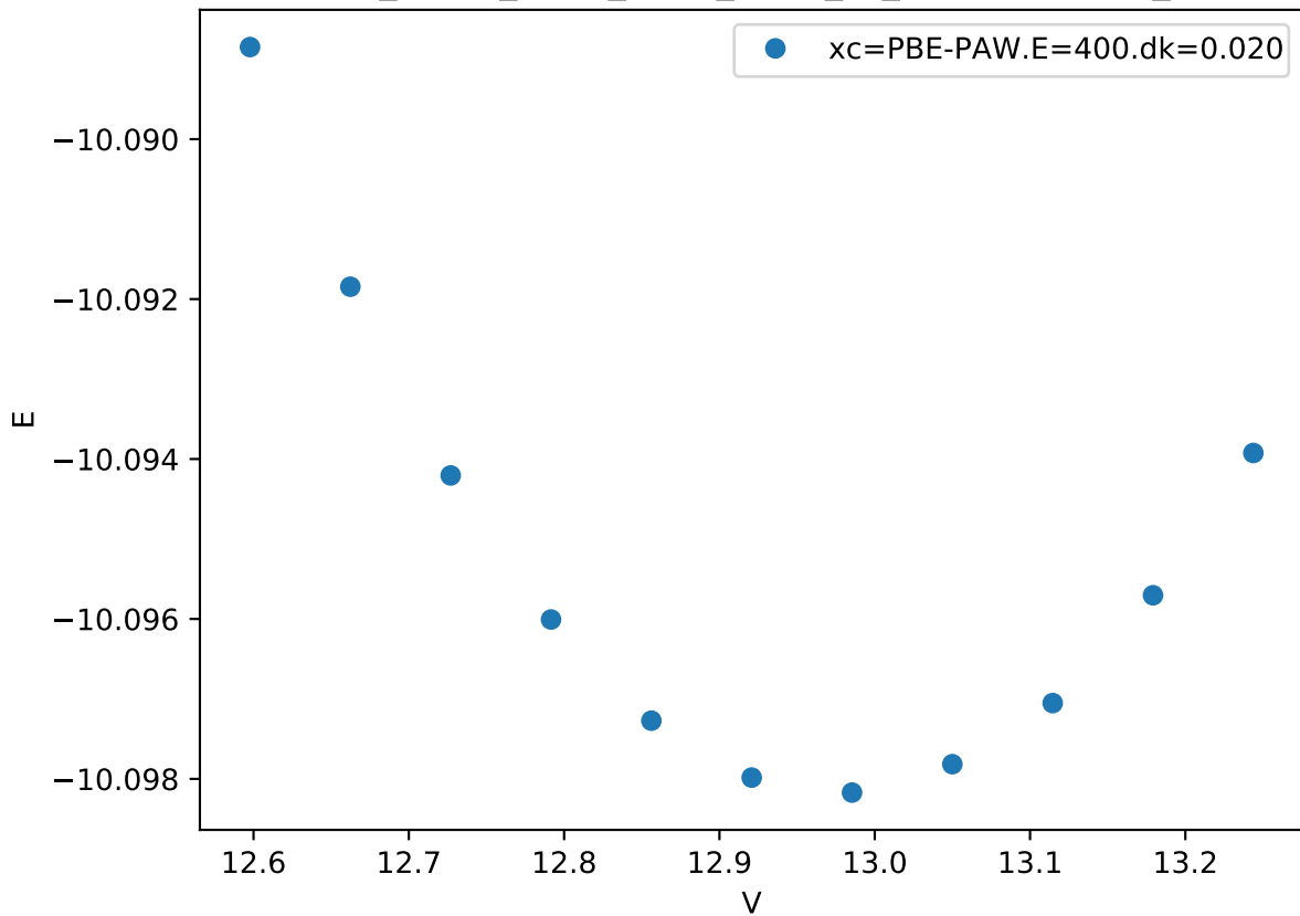
Cr_pv-Co_pv-W_sv/Cr_pv-W_sv_mu-BAABA.FM_
