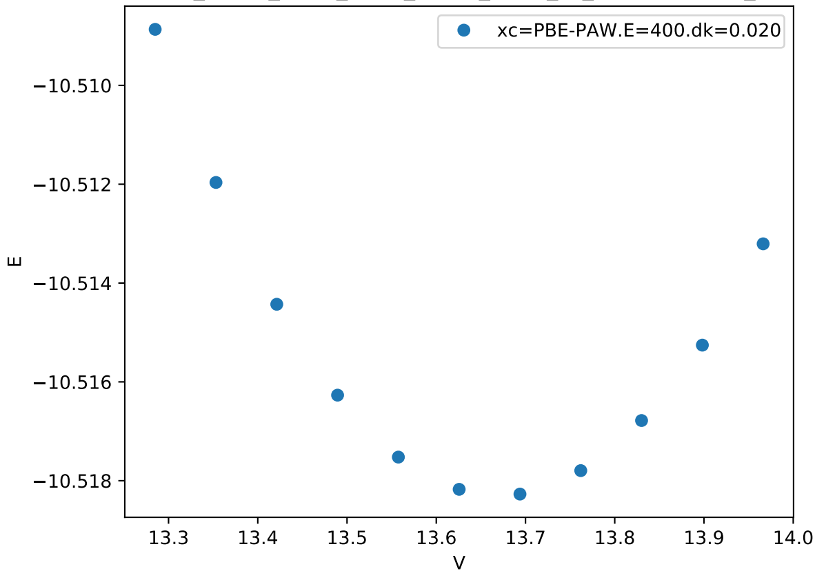
Cr_pv-Co_pv-W_sv/Cr_pv-Co_pv-W_sv_sigma-BCACA_
