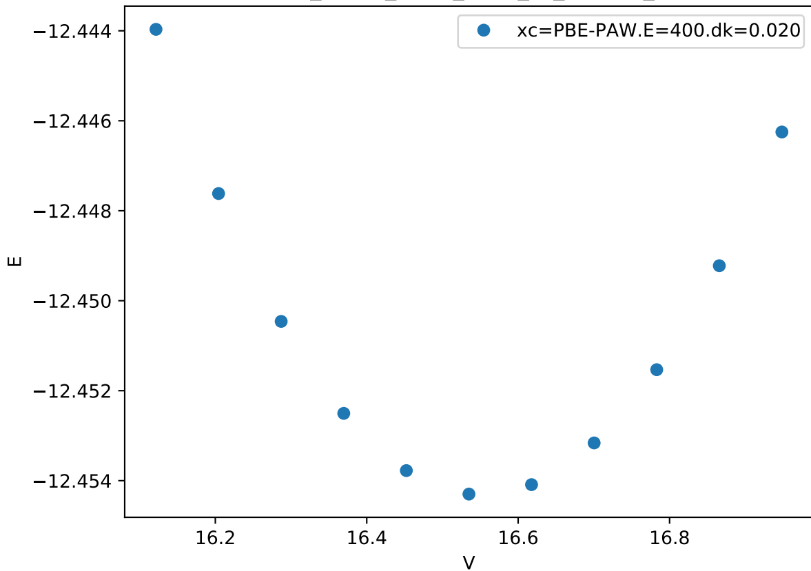
Cr_pv-Co_pv-W_sv/W_sv_hcp.FM_
