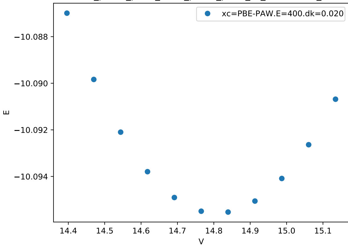
Cr_pv-Co_pv-W_sv/Cr_pv-Co_pv-W_sv_mu-ACABA_
