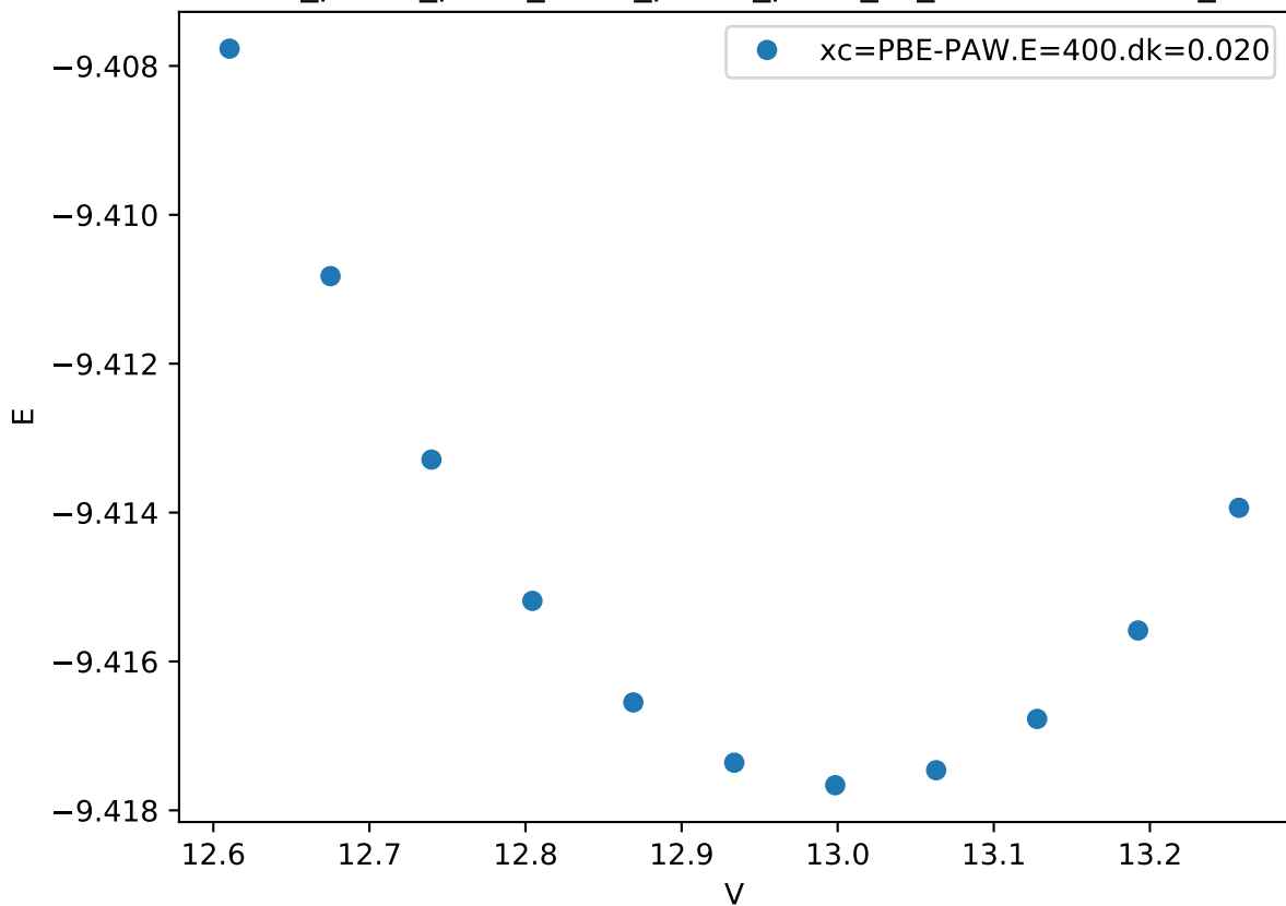
Cr_pv-Co_pv-W_sv/Cr_pv-Co_pv-W_sv_C36-BCCAB.FM_
