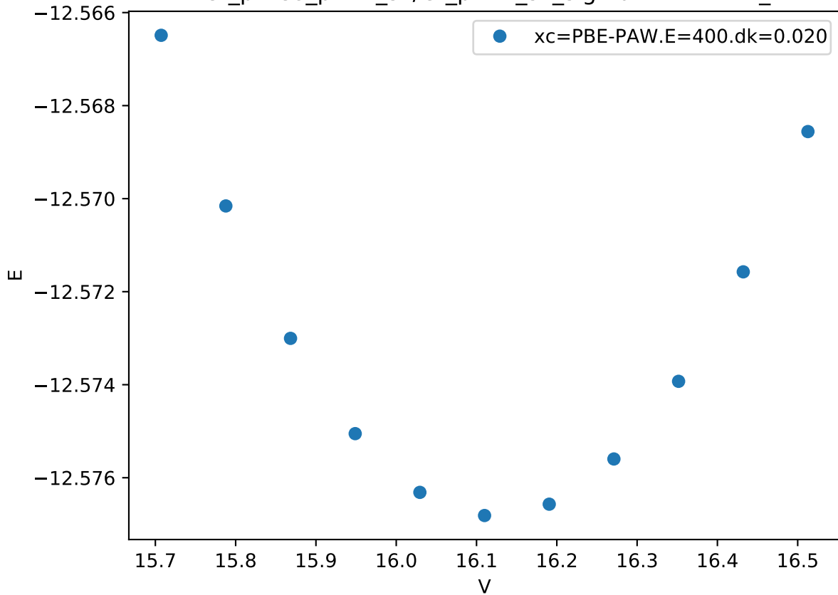
Cr_pv-Co_pv-W_sv/Cr_pv-W_sv_sigma-ABBBB.FM_
