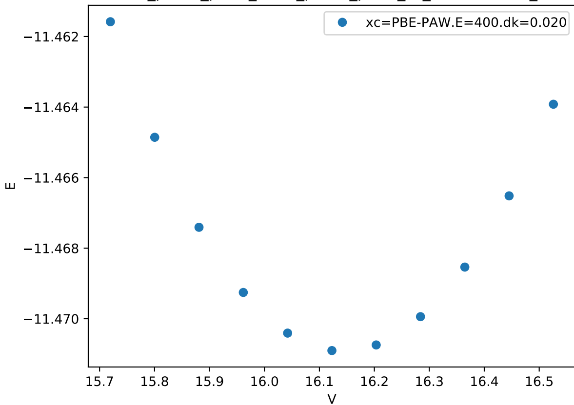
Cr_pv-Co_pv-W_sv/Cr_pv-Co_pv-W_sv_chi-ABCC.FM_
