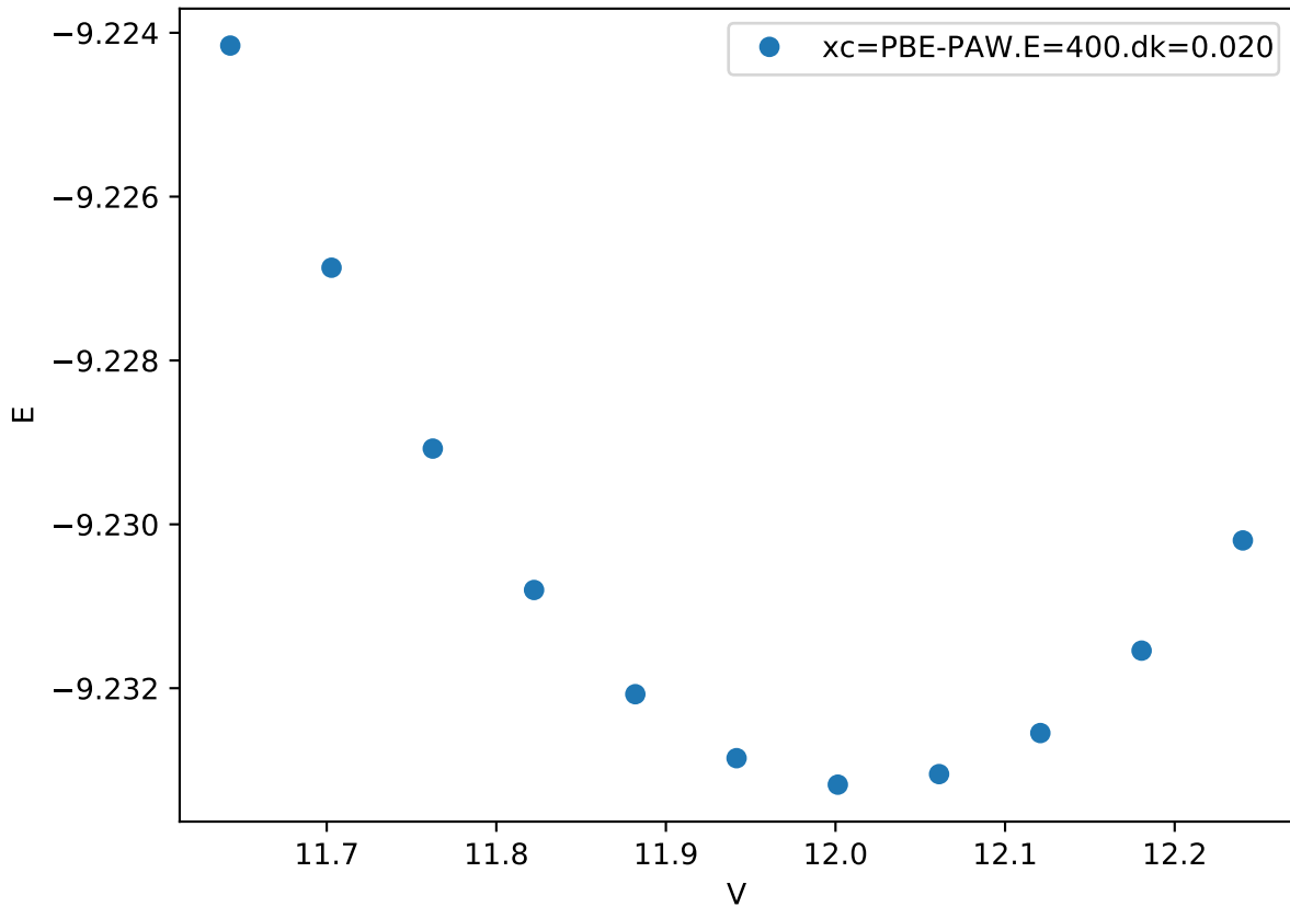
Cr_pv-Co_pv-W_sv/Cr_pv_C15.FM_
