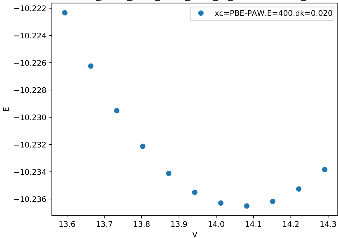
Cr_pv-Co_pv-W_sv/Co_pv-W_sv_C36-BBABA.FM_
