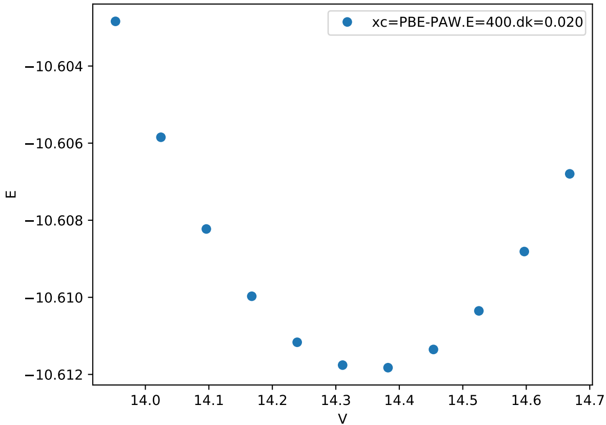
Cr_pv-Co_pv-W_sv/Cr_pv-W_sv_chi-BAAB_
