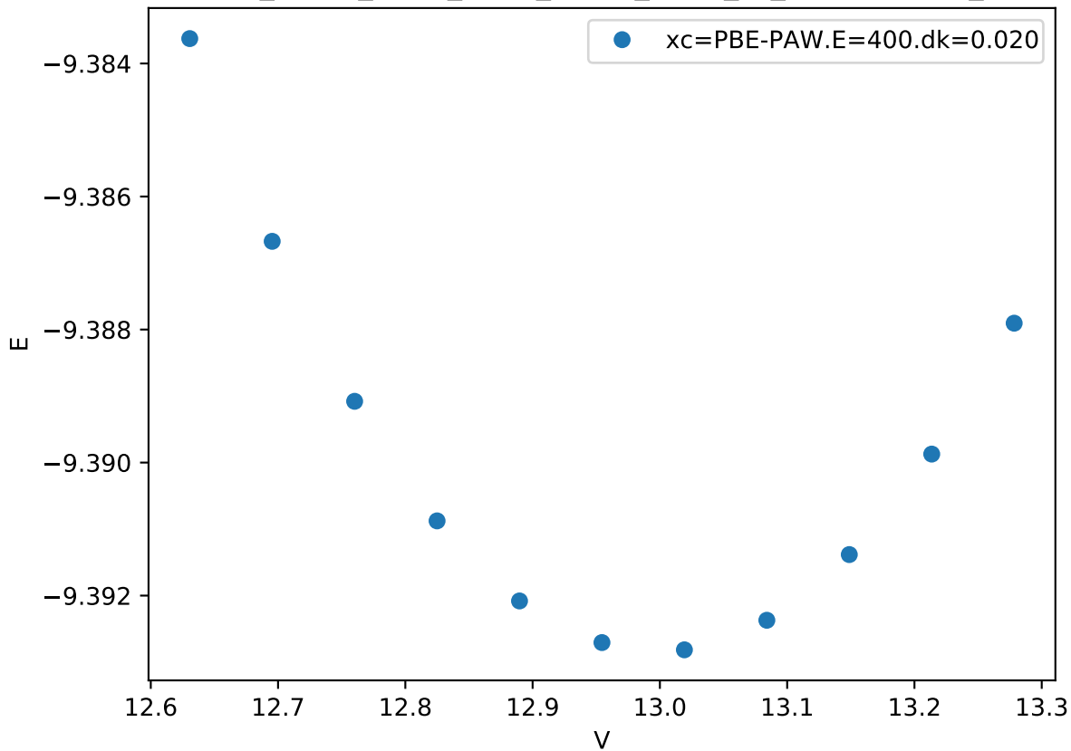
Cr_pv-Co_pv-W_sv/Cr_pv-Co_pv-W_sv_chi-ABCB.FM_
