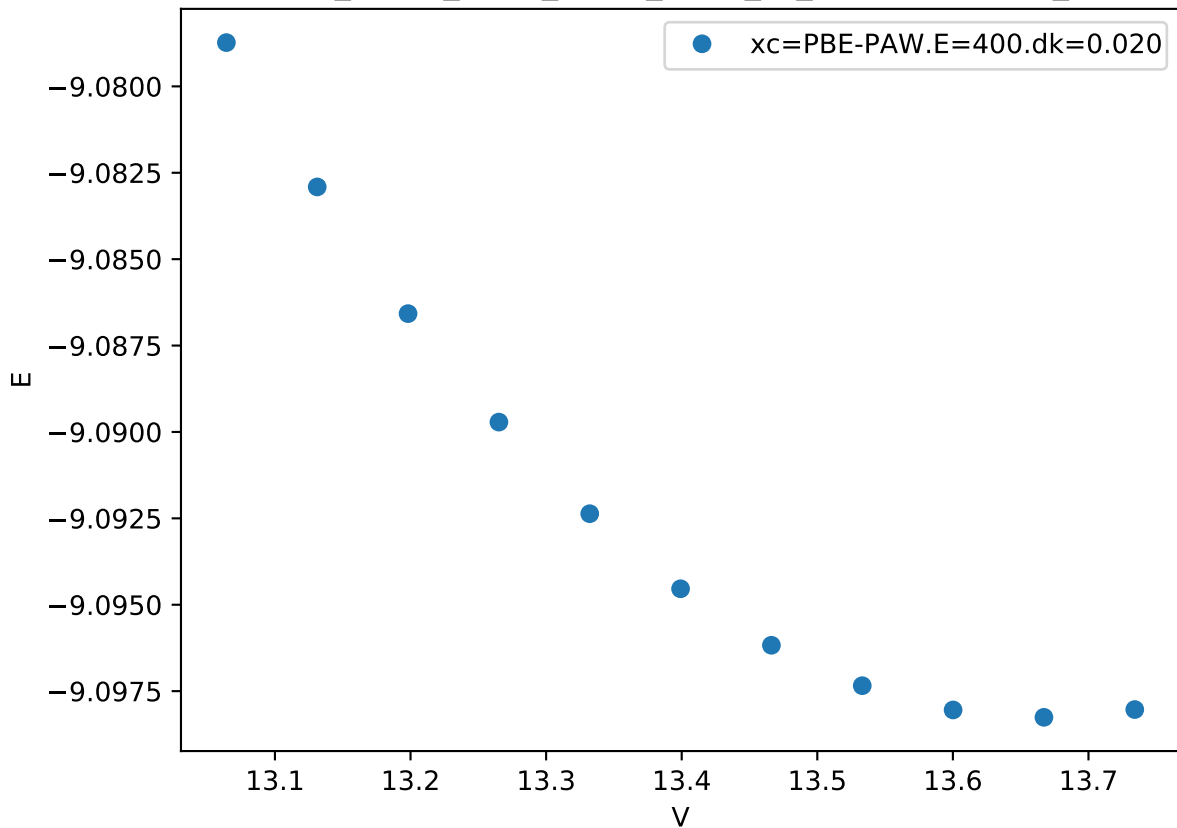
Cr_pv-Co_pv-W_sv/Co_pv-W_sv_C36-ABABA.FM_
