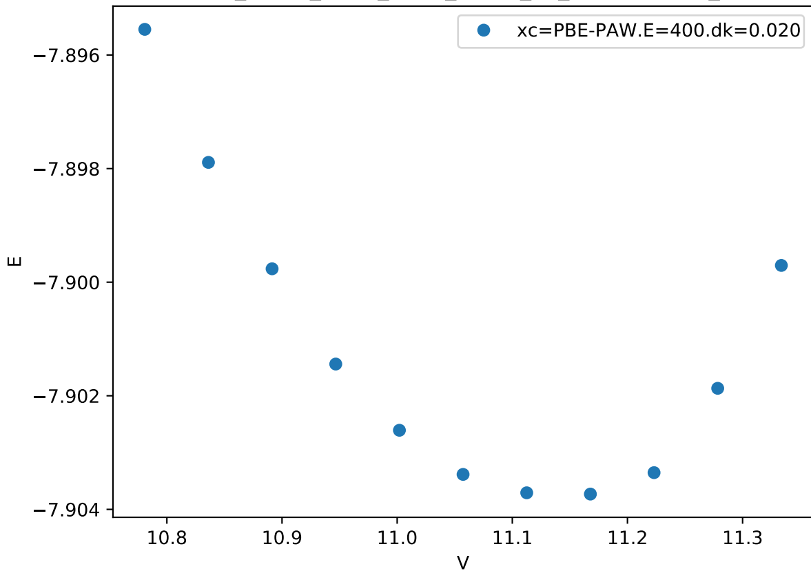
Cr_pv-Co_pv-W_sv/Cr_pv-Co_pv_chi-BBBA.FM_
