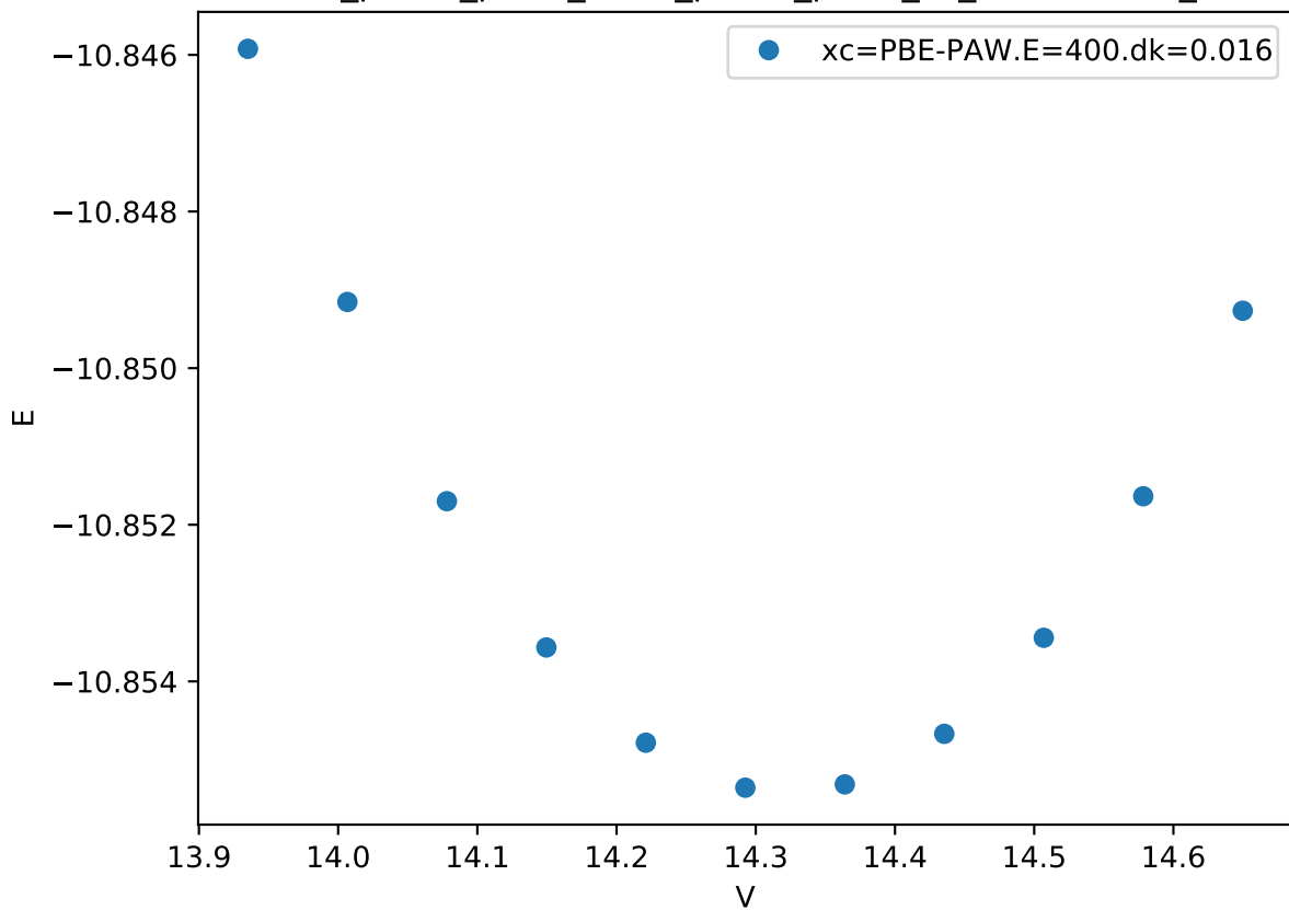
Cr_pv-Co_pv-W_sv/Cr_pv-Co_pv-W_sv_C36-CCBAC_
