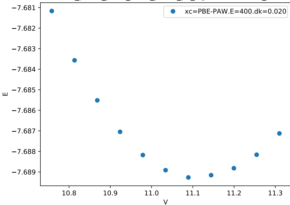
Cr_pv-Co_pv-W_sv/Cr_pv-Co_pv_sigma-ABBAB.FM_
