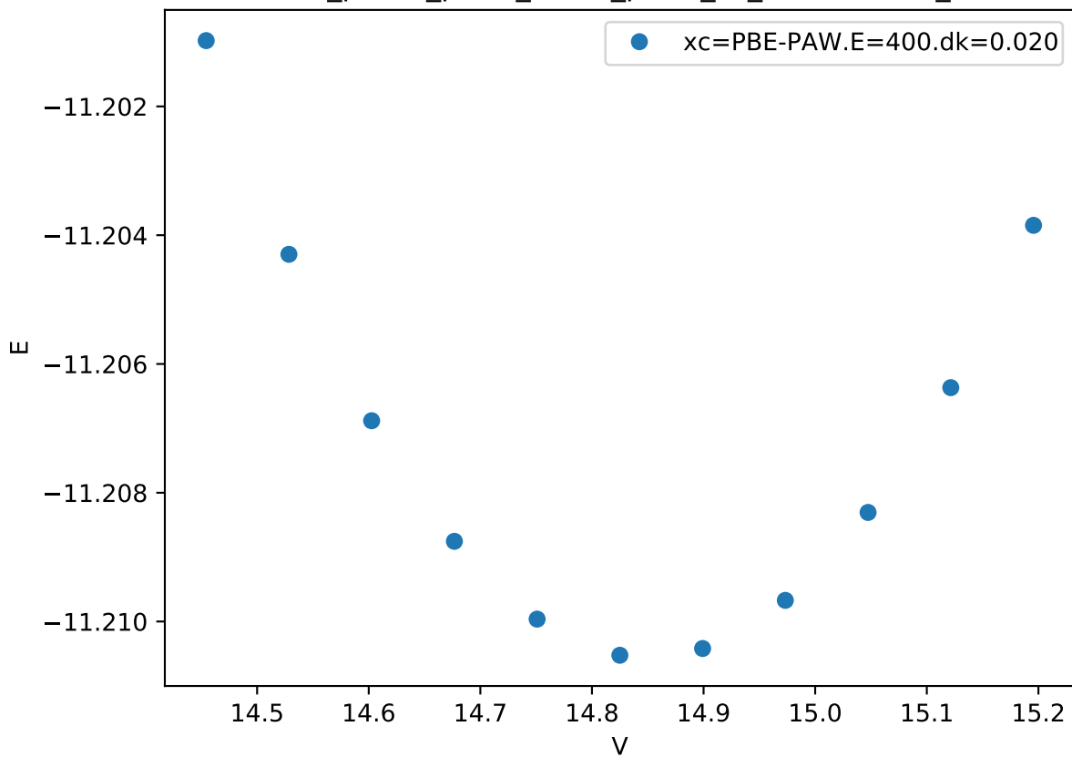
Cr_pv-Co_pv-W_sv/Co_pv-W_sv_L12-AB3.FM_
