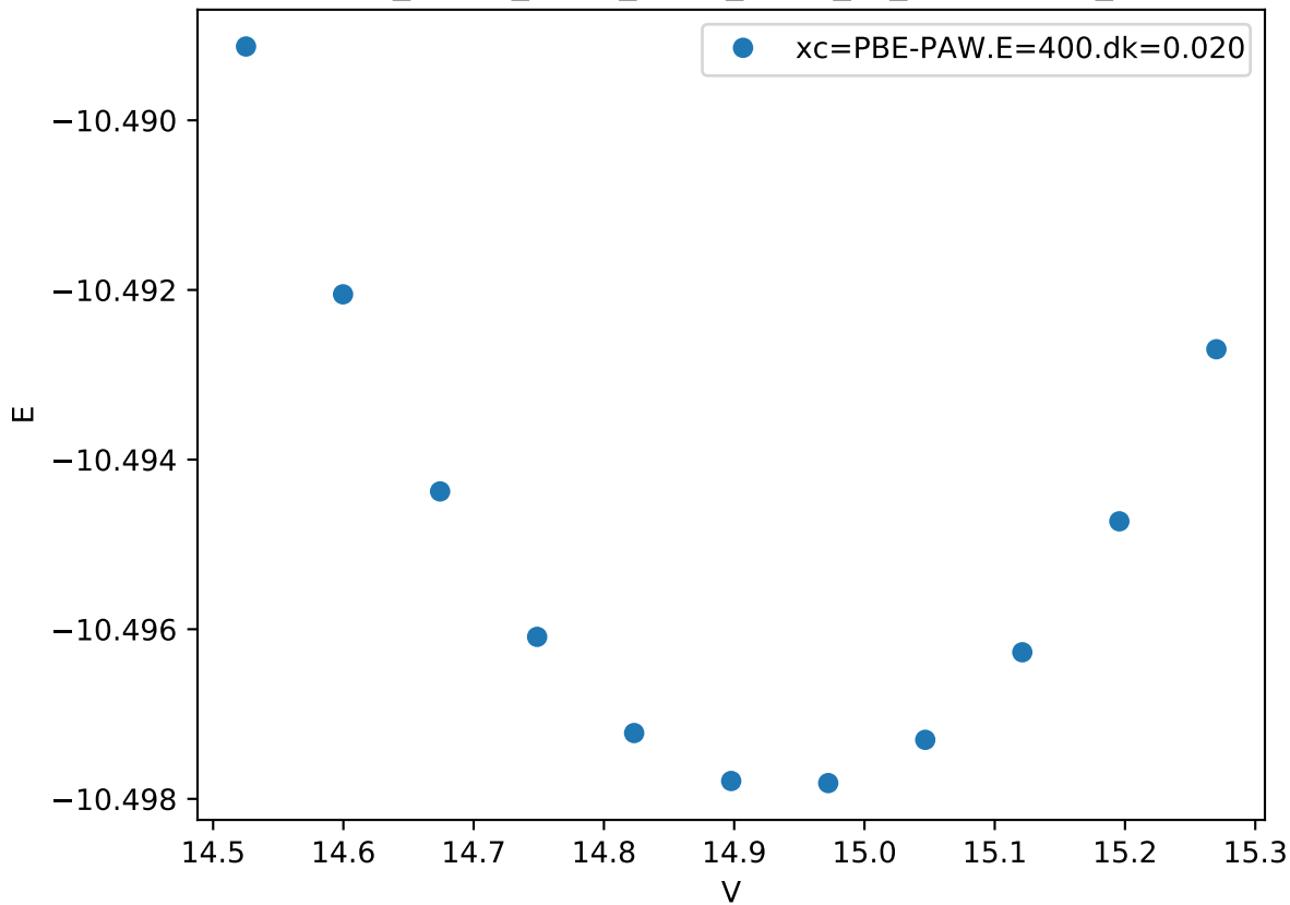
Cr_pv-Co_pv-W_sv/Cr_pv-W_sv_mu-ABAAA_
