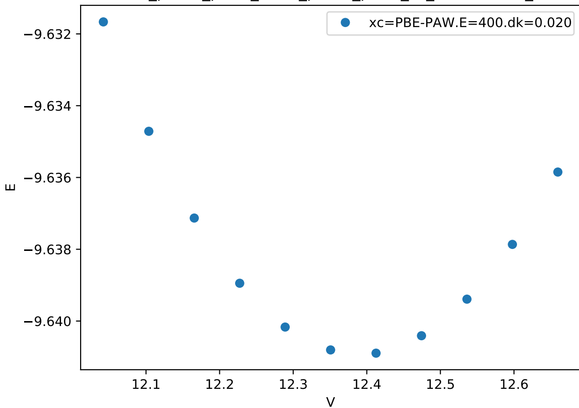
Cr_pv-Co_pv-W_sv/Cr_pv-Co_pv-W_sv_C36-CCBBA_
