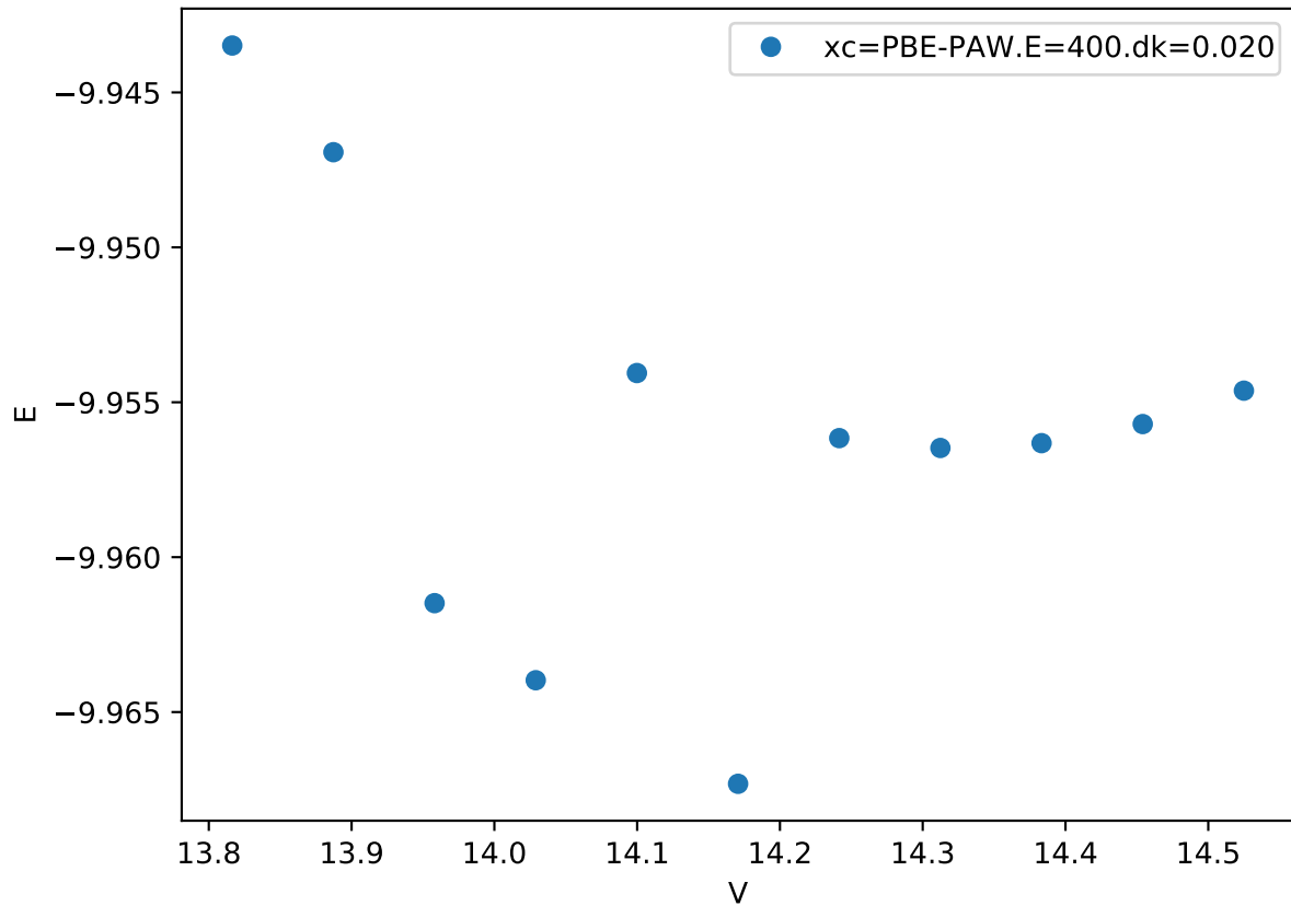
Cr_pv-Co_pv-W_sv/Cr_pv-Co_pv-W_sv_chi-BBAC.FM_
