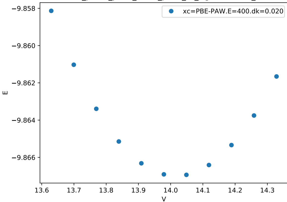
Cr_pv-Co_pv-W_sv/Co_pv-W_sv_sigma-AAABB_
