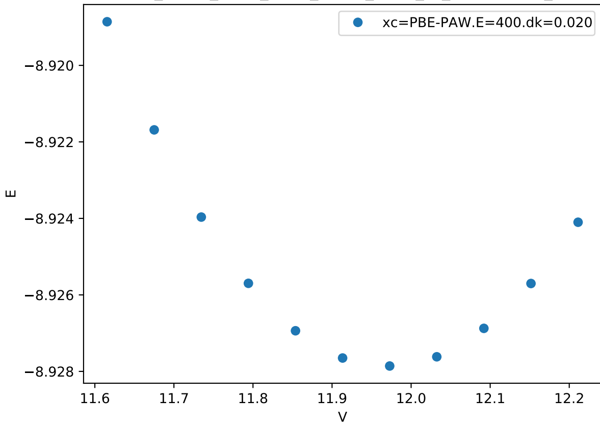
Cr_pv-Co_pv-W_sv/Cr_pv-Co_pv-W_sv_C36-BCAAB_
