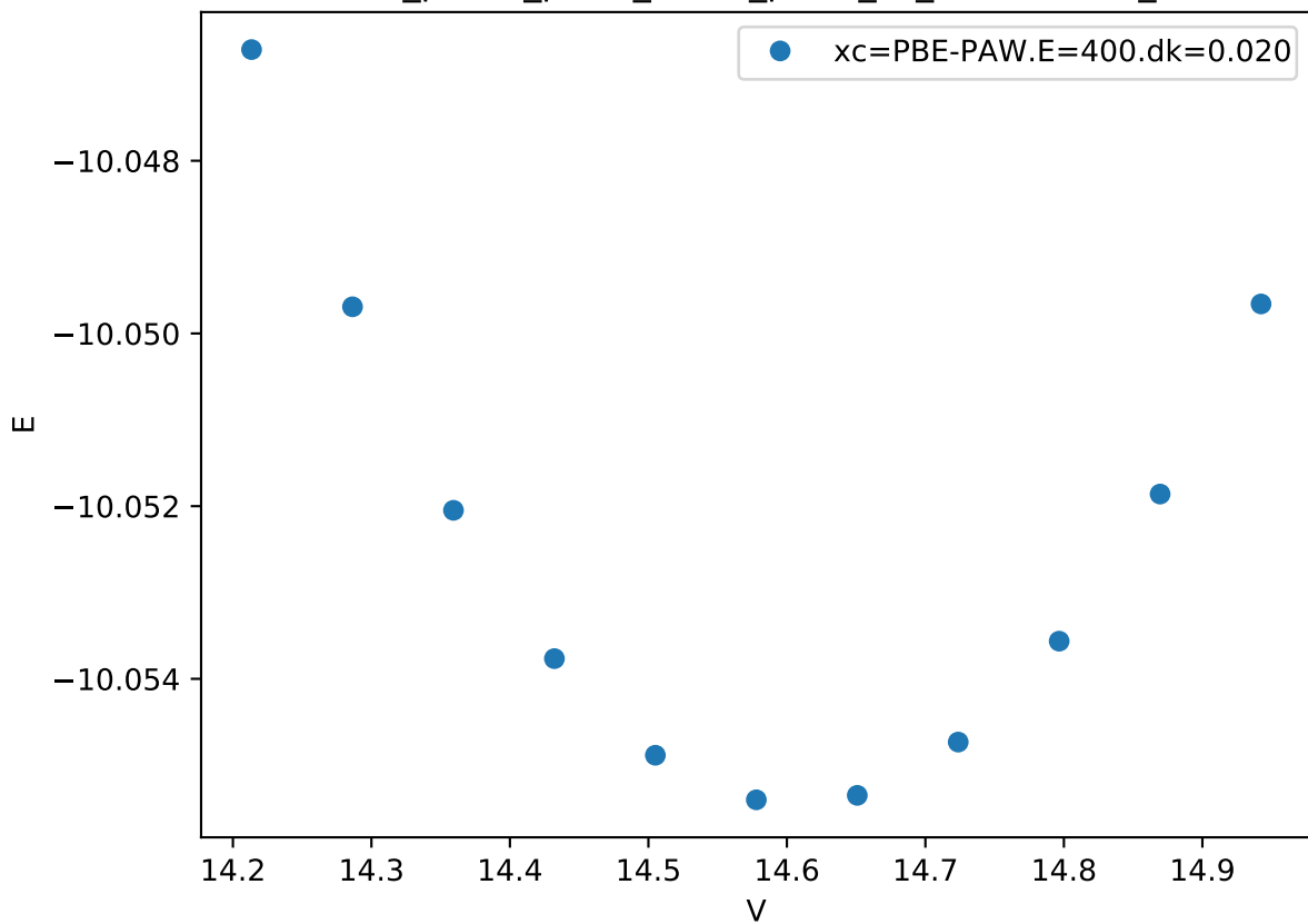
Cr_pv-Co_pv-W_sv/Co_pv-W_sv_C36-ABBBA_
