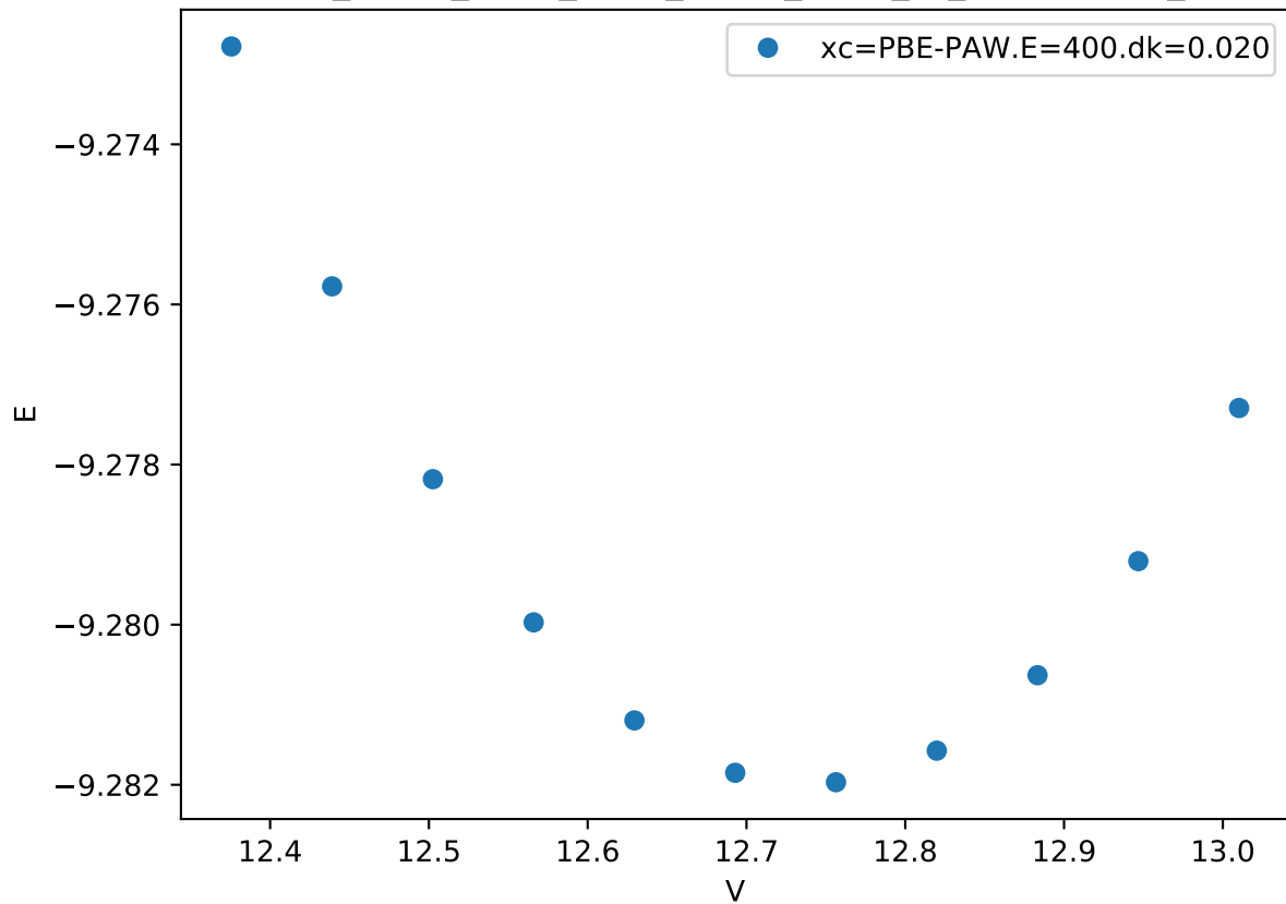
Cr_pv-Co_pv-W_sv/Cr_pv-Co_pv-W_sv_C36-ACCBB_
