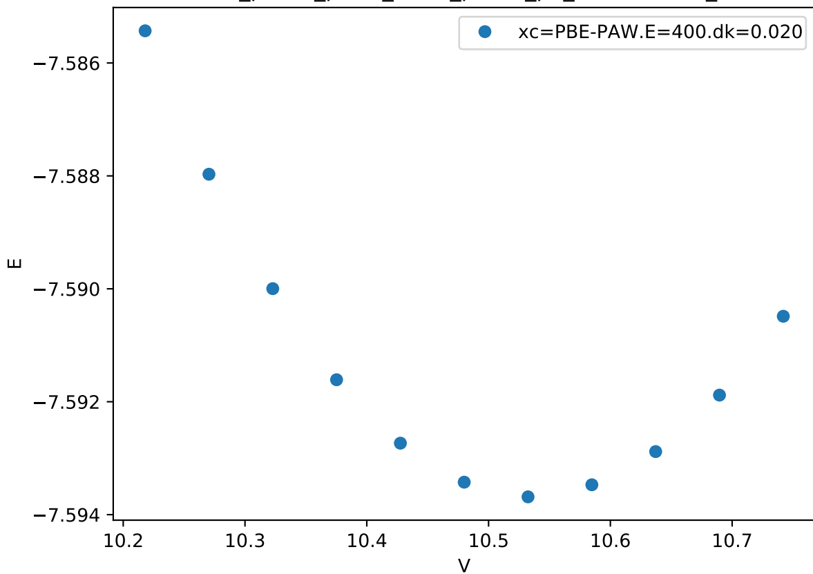
Cr_pv-Co_pv-W_sv/Cr_pv-Co_pv_L12-AB3.FM_
