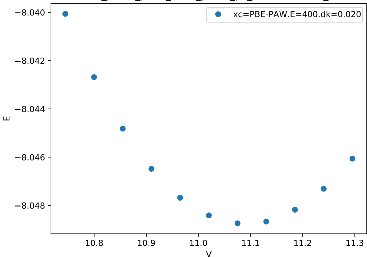
Cr_pv-Co_pv-W_sv/Cr_pv-Co_pv_mu-BBAAA.FM_
