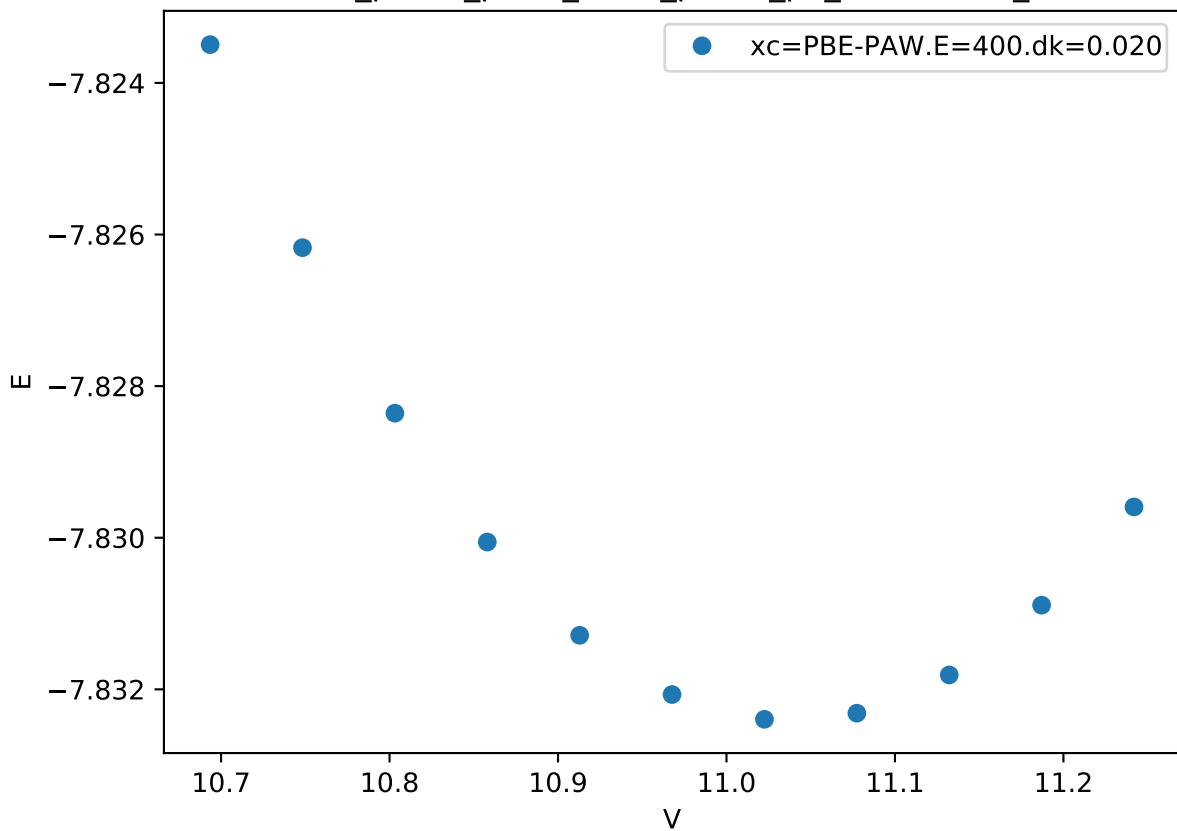
Cr_pv-Co_pv-W_sv/Cr_pv-Co_pv_mu-ABABA_
