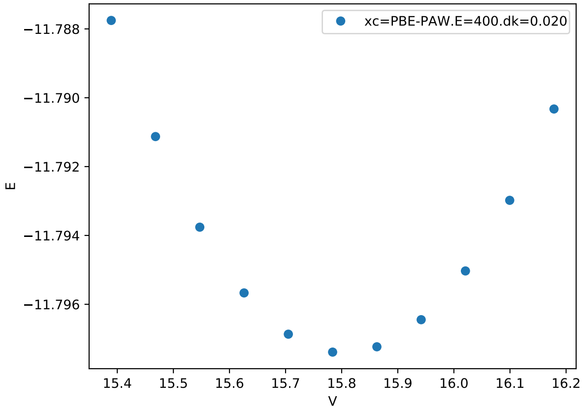
Cr_pv-Co_pv-W_sv/Cr_pv-W_sv_mu-ABBBA.FM_
