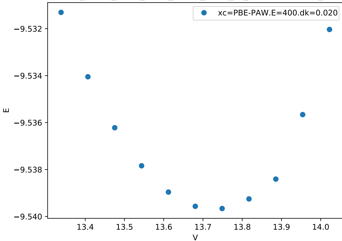
Cr_pv-Co_pv-W_sv/Cr_pv-Co_pv-W_sv_C36-CABBC.FM_
