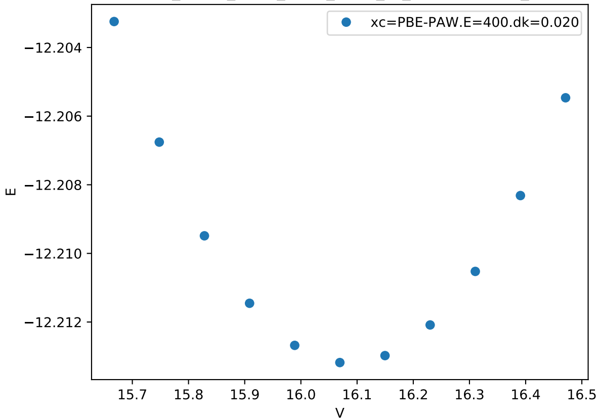
Cr_pv-Co_pv-W_sv/Cr_pv-W_sv_sigma-BABBB_
