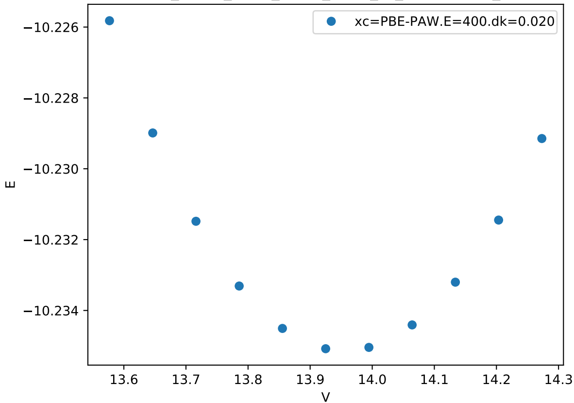
Cr_pv-Co_pv-W_sv/Co_pv-W_sv_C36-BBAAB_
