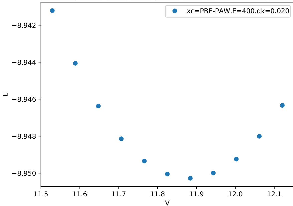
Cr_pv-Co_pv-W_sv/Cr_pv-Co_pv-W_sv_C36-ACBBA_
