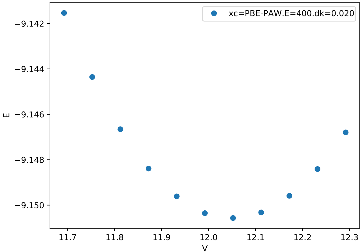
Cr_pv-Co_pv-W_sv/Cr_pv-Co_pv-W_sv_C36-BCBAA.FM_
