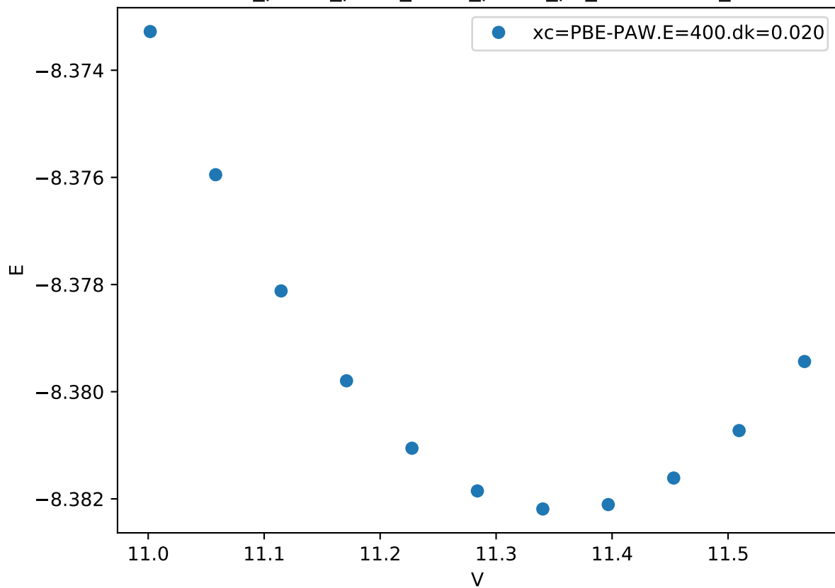
Cr_pv-Co_pv-W_sv/Cr_pv-Co_pv_mu-BABAB_
