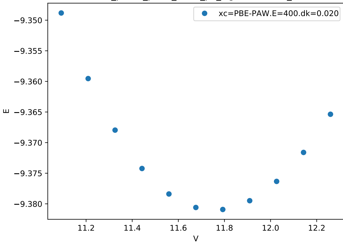
Cr_pv-Co_pv-W_sv/Cr_pv_sigma.UDUDU_
