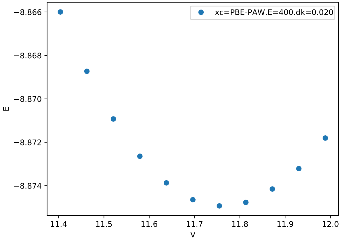
Cr_pv-Co_pv-W_sv/Cr_pv-Co_pv-W_sv_sigma-CAAAB_
