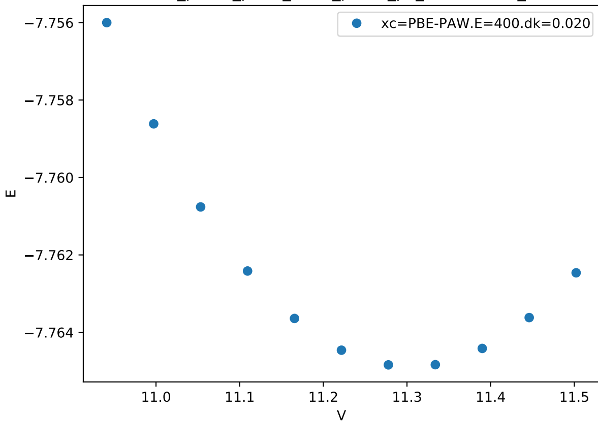
Cr_pv-Co_pv-W_sv/Cr_pv-Co_pv_C36-BBAAB_
