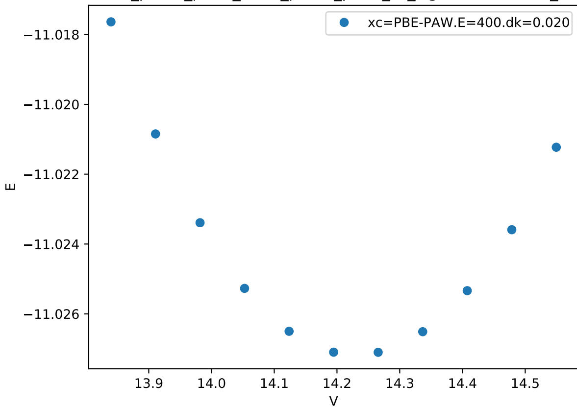
Cr_pv-Co_pv-W_sv/Cr_pv-Co_pv-W_sv_sigma-BACAC.FM_
