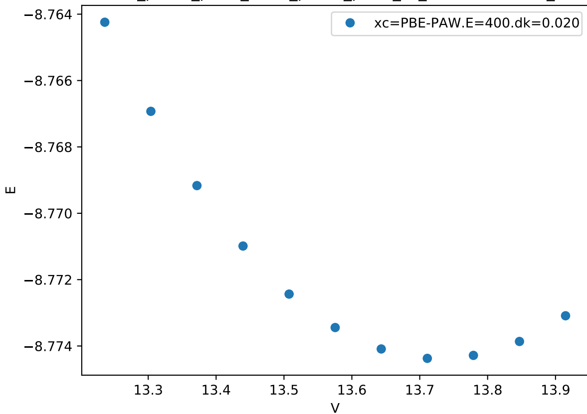
Cr_pv-Co_pv-W_sv/Cr_pv-Co_pv-W_sv_C36-ABABC.FM_
