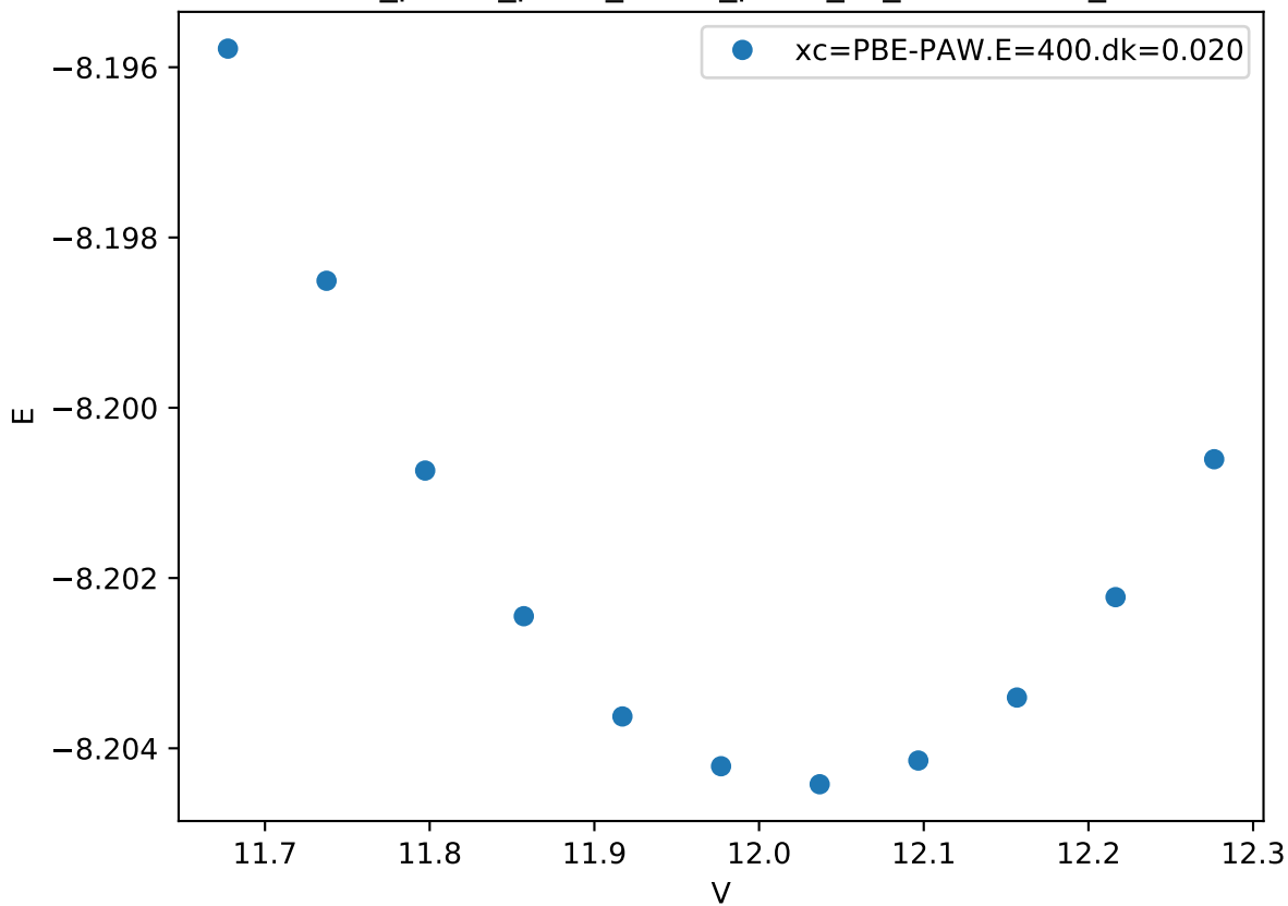
Cr_pv-Co_pv-W_sv/Co_pv-W_sv_mu-BAAAB_
