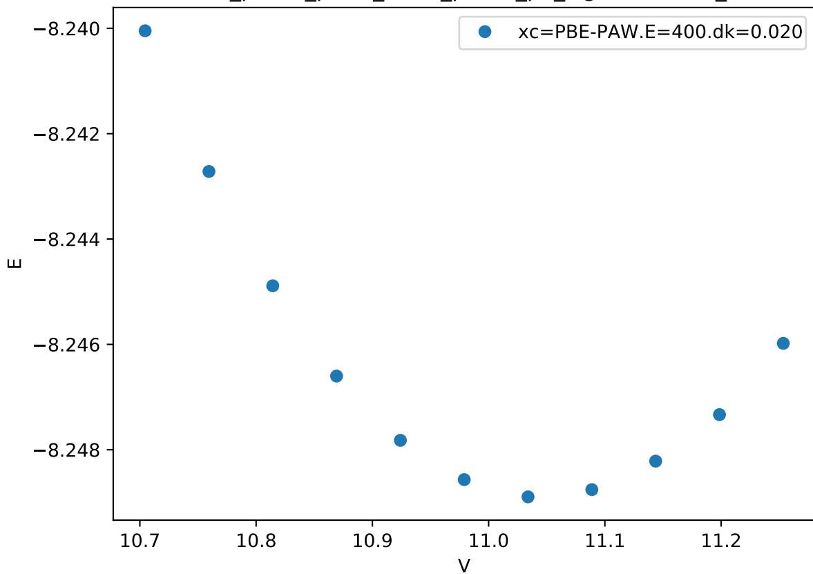
Cr_pv-Co_pv-W_sv/Cr_pv-Co_pv_sigma-BBABA_
