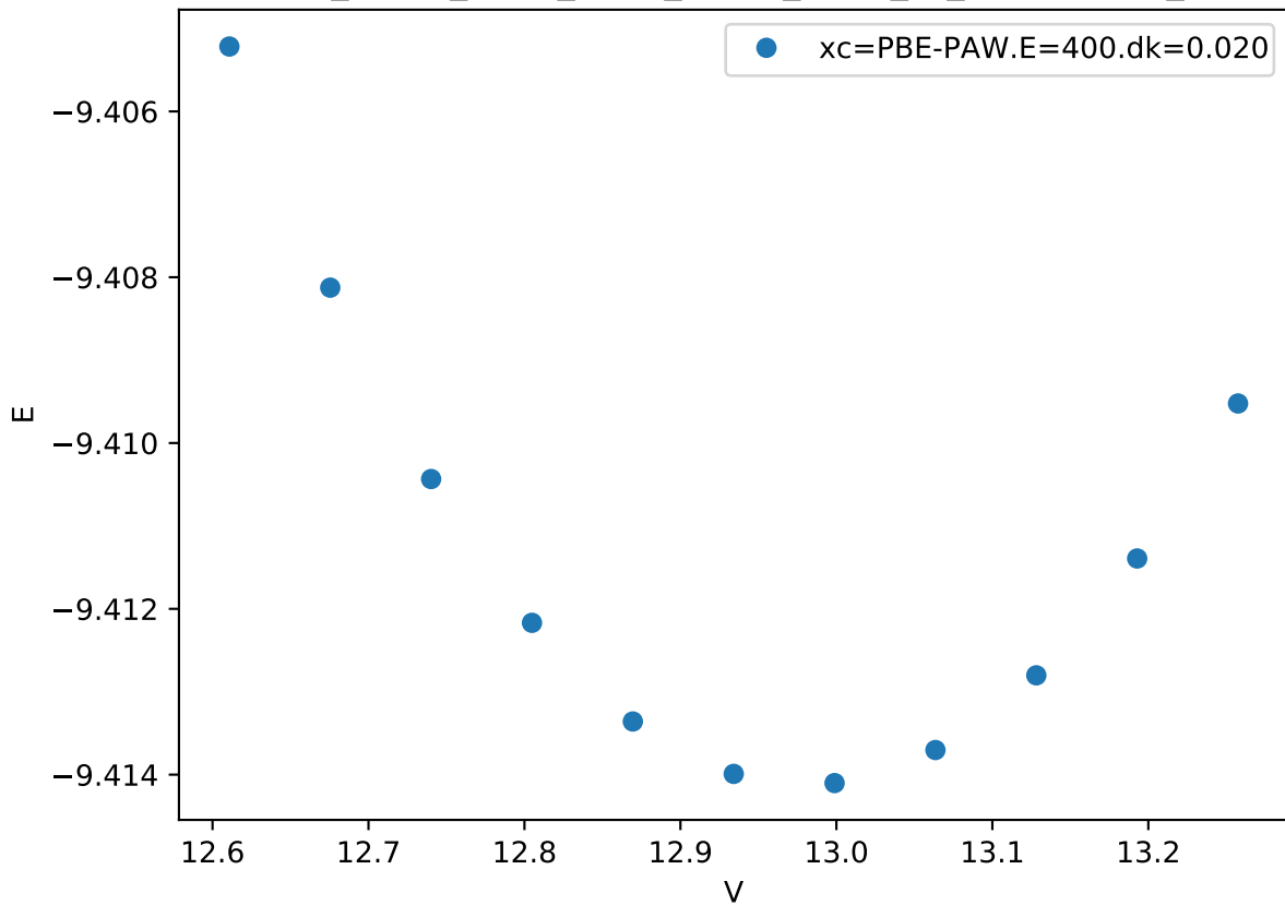
Cr_pv-Co_pv-W_sv/Cr_pv-Co_pv-W_sv_C36-BCCAB_
