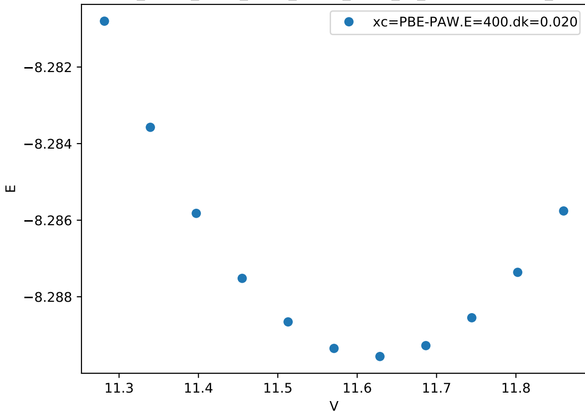
Cr_pv-Co_pv-W_sv/Cr_pv-Co_pv-W_sv_C36-BCABB.FM_
