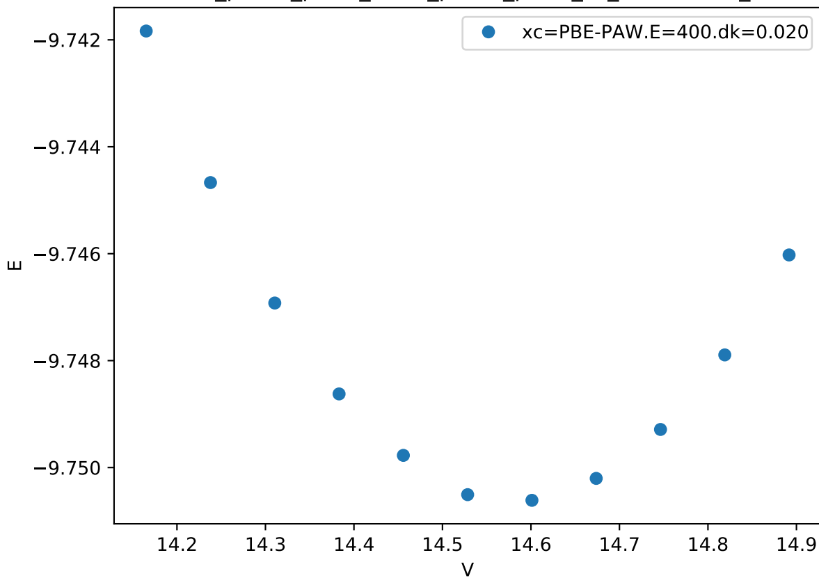
Cr_pv-Co_pv-W_sv/Cr_pv-Co_pv-W_sv_mu-ACABB_
