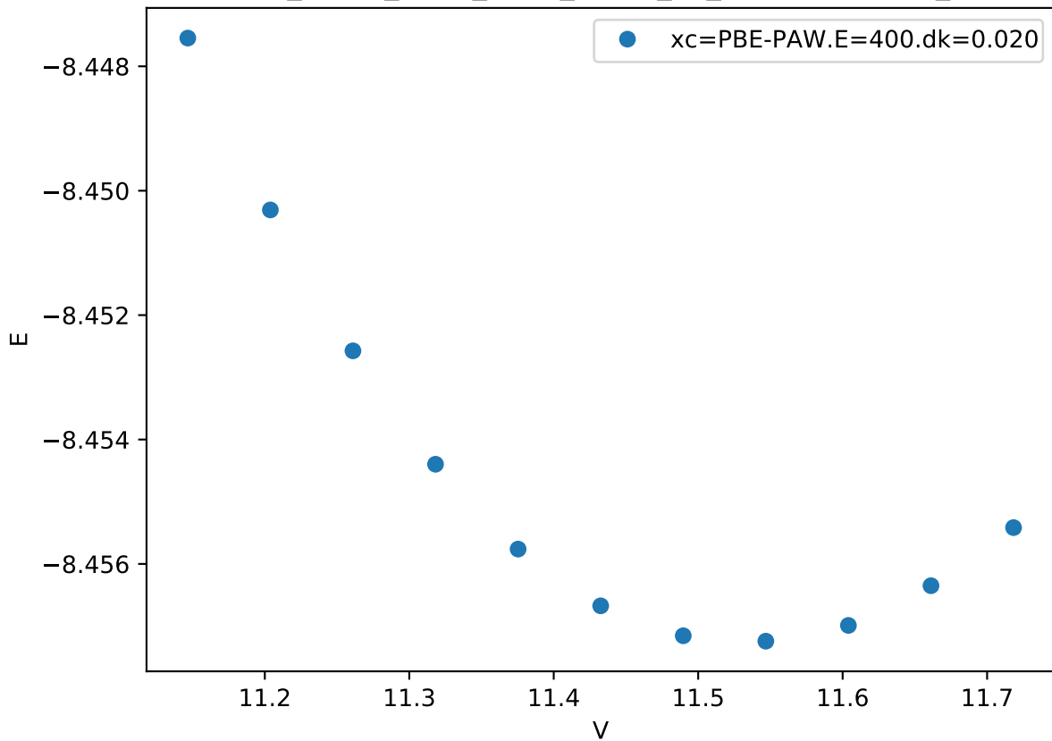
Cr_pv-Co_pv-W_sv/Cr_pv-Co_pv_C36-BABAA.FM_
