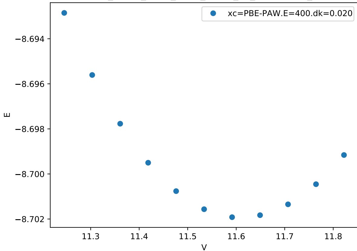
Cr_pv-Co_pv-W_sv/Cr_pv-Co_pv_mu-BABAA_
