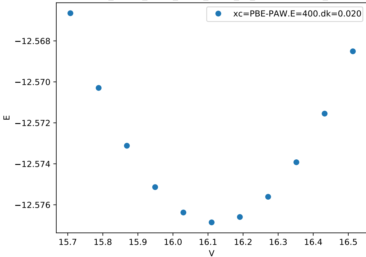
Cr_pv-Co_pv-W_sv/Cr_pv-W_sv_sigma-ABBBB_
