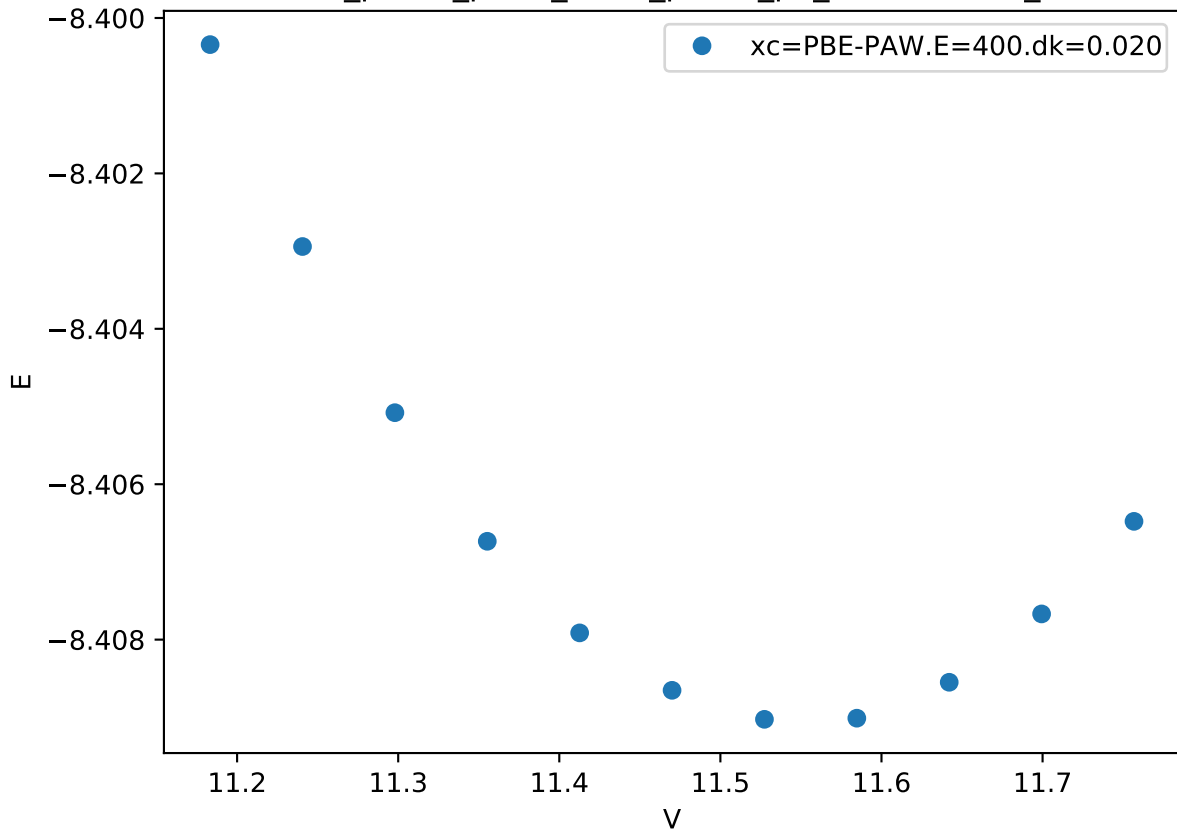
Cr_pv-Co_pv-W_sv/Cr_pv-Co_pv_C15-A2B.FM_
