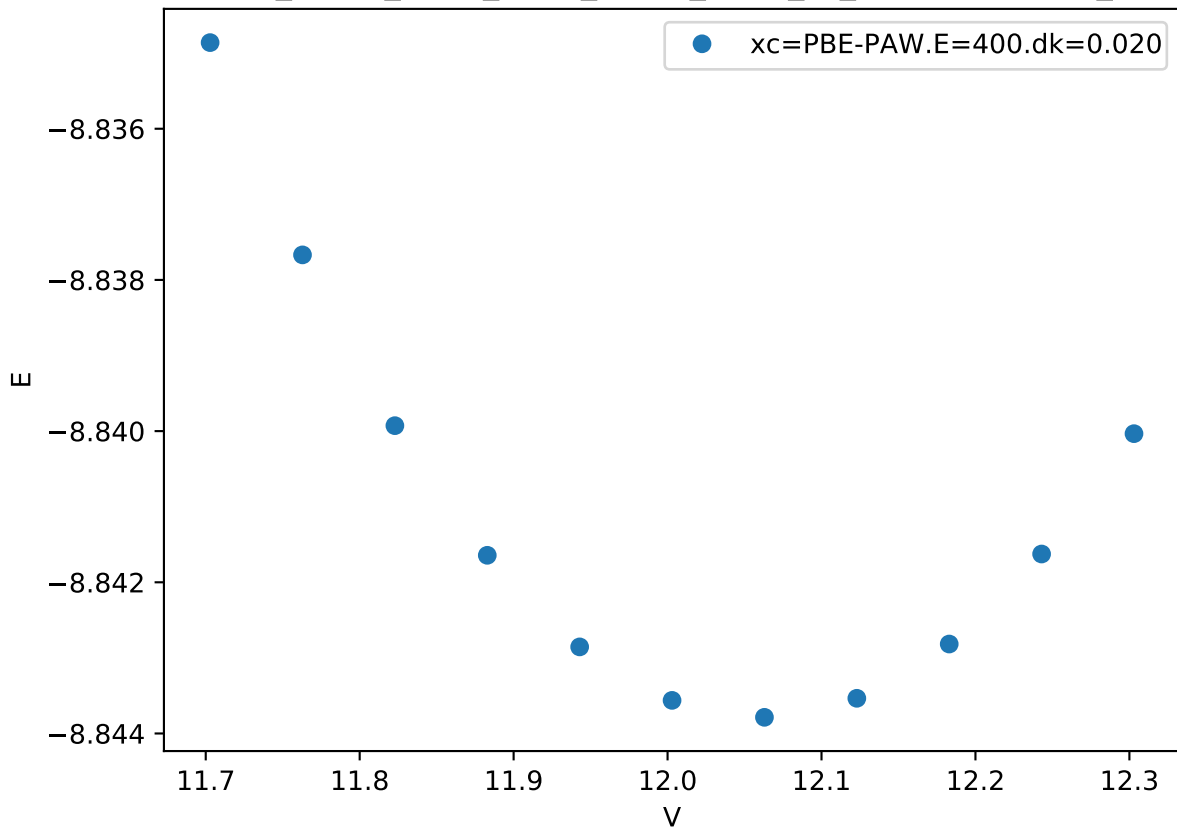
Cr_pv-Co_pv-W_sv/Cr_pv-Co_pv-W_sv_C36-BCABA.FM_
