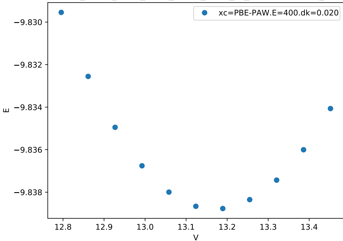
Cr_pv-Co_pv-W_sv/Cr_pv-Co_pv-W_sv_C36-CACAB.FM_
