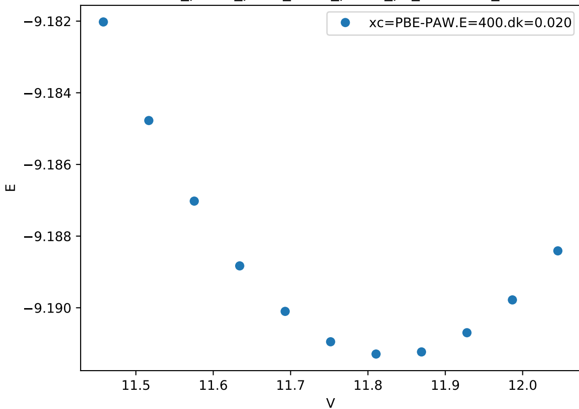
Cr_pv-Co_pv-W_sv/Cr_pv-Co_pv_chi-BAAA_
