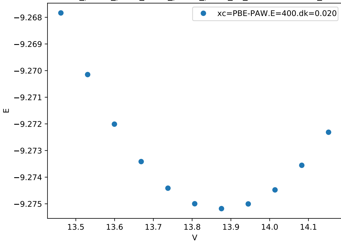
Cr_pv-Co_pv-W_sv/Cr_pv-Co_pv-W_sv_C36-AAACB.FM_
