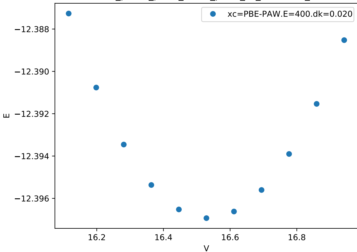
Cr_pv-Co_pv-W_sv/Co_pv-W_sv_chi-ABBB_
