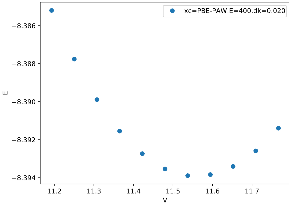
Cr_pv-Co_pv-W_sv/Cr_pv-Co_pv_C36-BBAAA_
