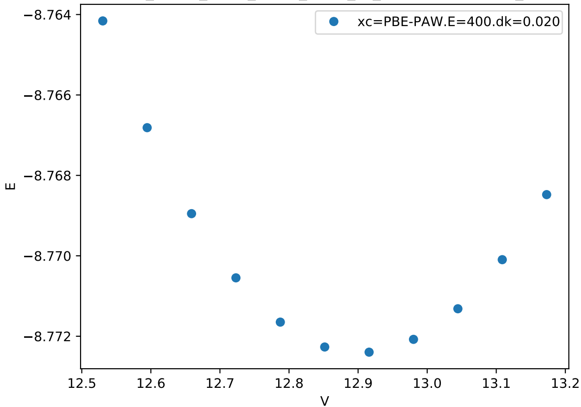
Cr_pv-Co_pv-W_sv/Co_pv-W_sv_sigma-BAAAB.FM_
