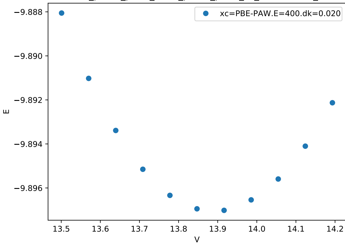
Cr_pv-Co_pv-W_sv/Cr_pv-Co_pv-W_sv_C36-ACABC_
