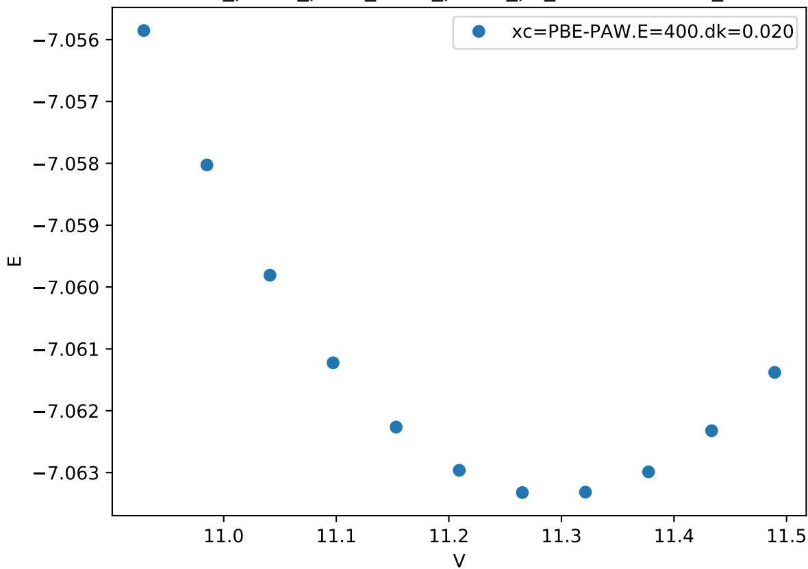
Cr_pv-Co_pv-W_sv/Cr_pv-Co_pv_mu-ABBBB.FM_
