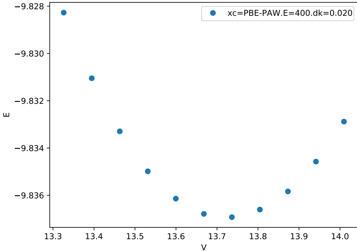
Cr_pv-Co_pv-W_sv/Cr_pv-W_sv_C36-AAAAB_
