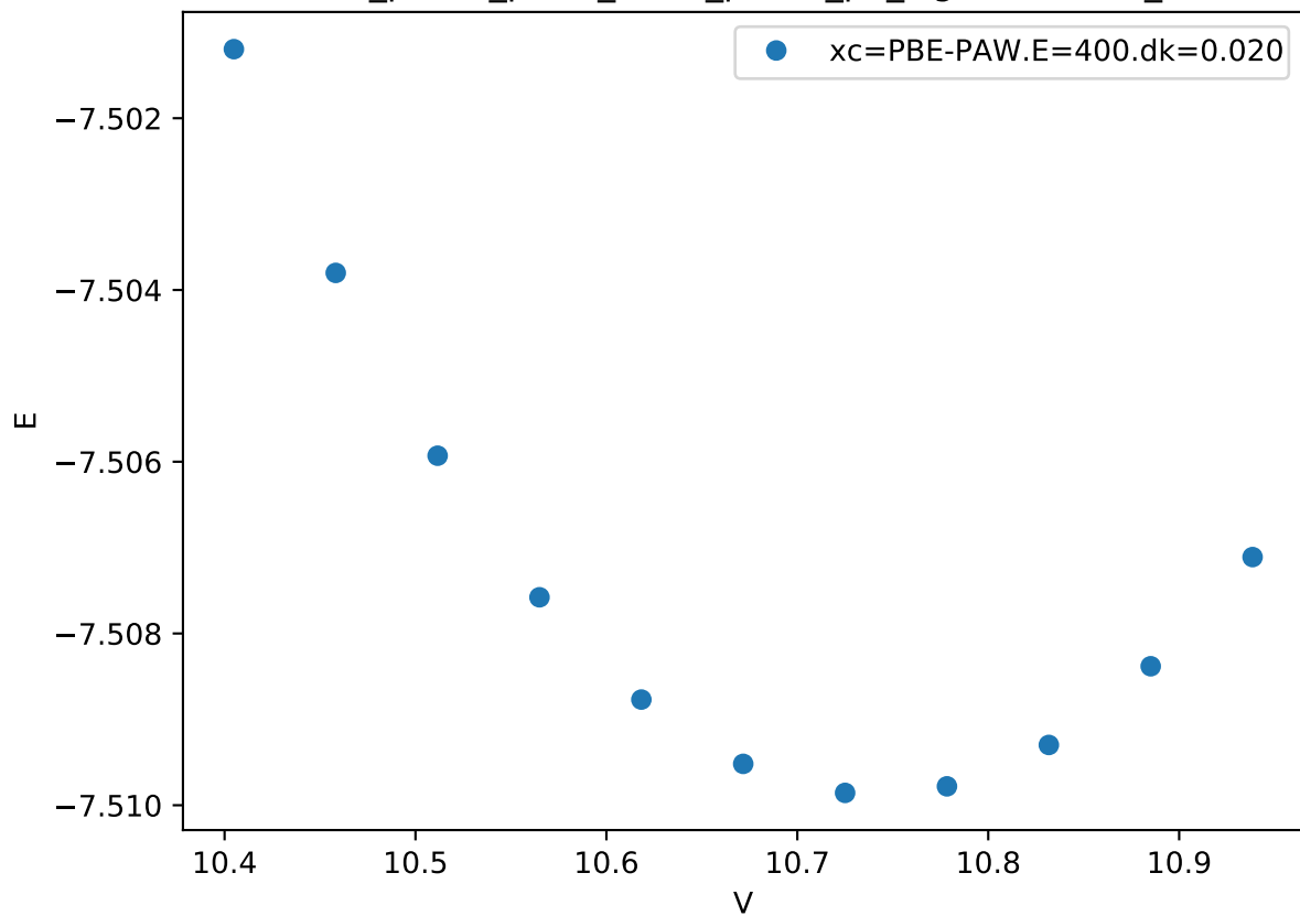
Cr_pv-Co_pv-W_sv/Cr_pv-Co_pv_sigma-BBBBA_
