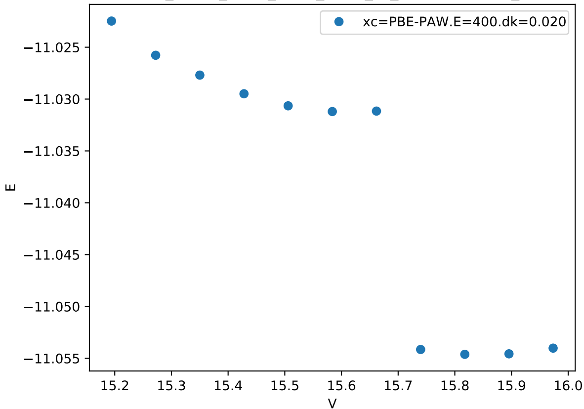
Cr_pv-Co_pv-W_sv/Cr_pv-W_sv_mu-ABAAB.FM_
