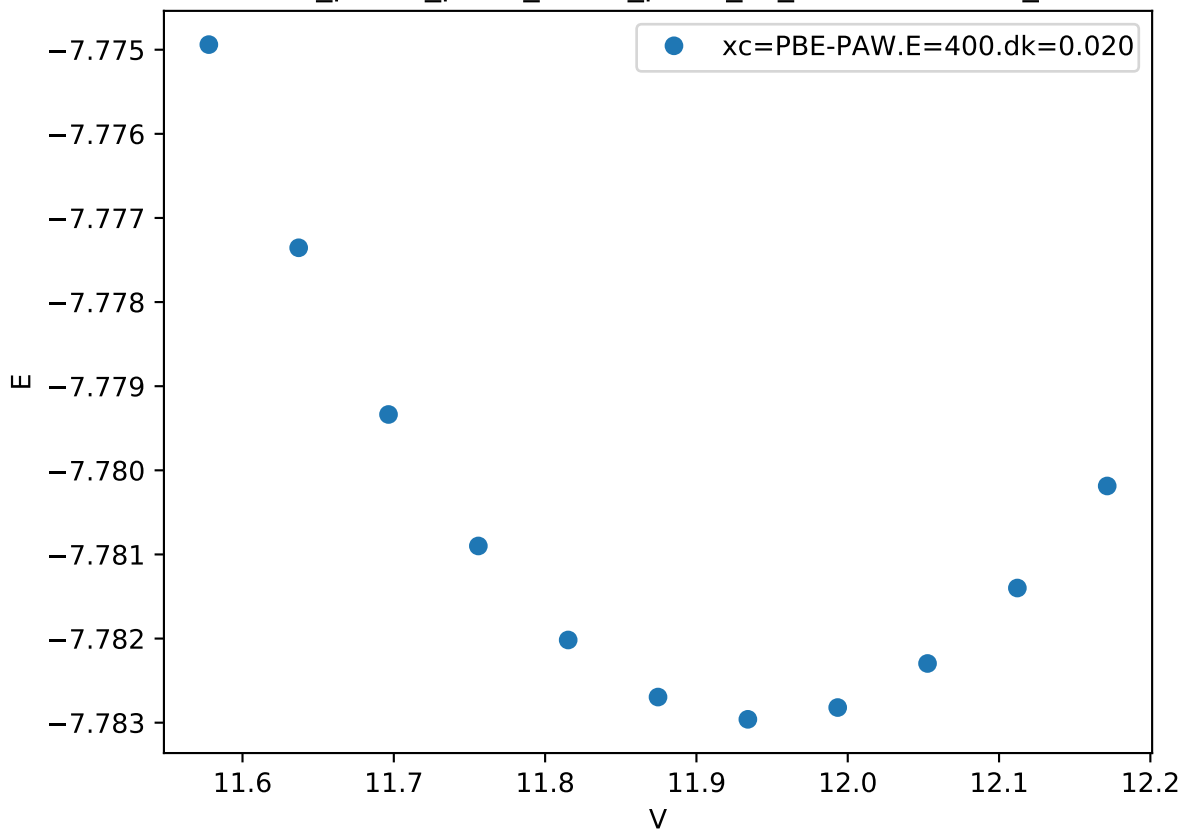
Cr_pv-Co_pv-W_sv/Co_pv-W_sv_mu-AAAAB.FM_
