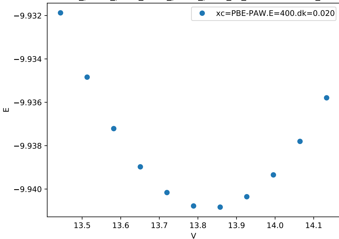
Cr_pv-Co_pv-W_sv/Cr_pv-Co_pv-W_sv_C36-CAACB.FM_
