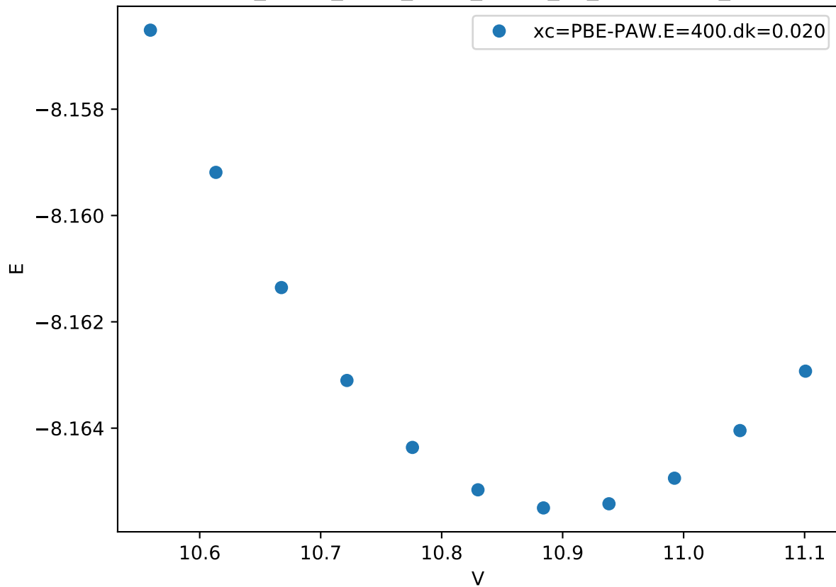
Cr_pv-Co_pv-W_sv/Cr_pv-Co_pv_hcp-AB.FM_
