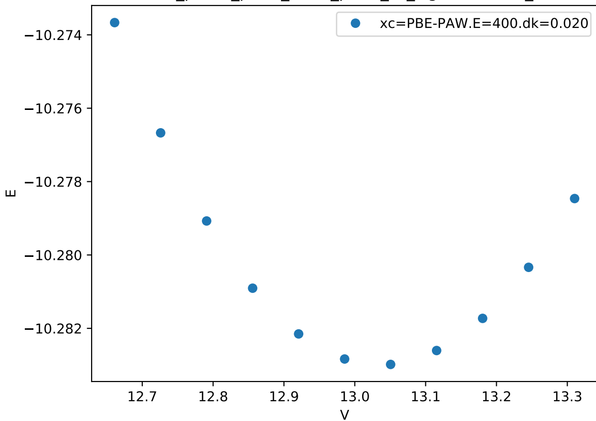
Cr_pv-Co_pv-W_sv/Cr_pv-W_sv_sigma-AABAA_
