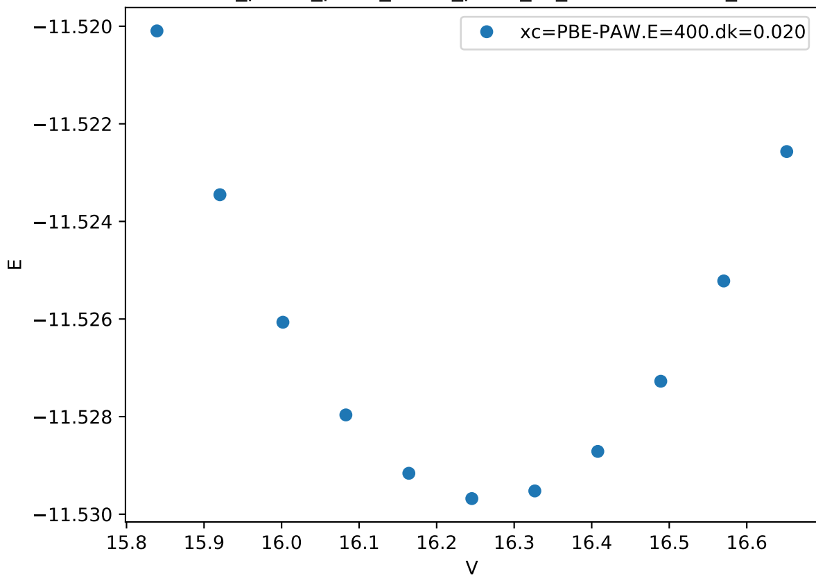
Cr_pv-Co_pv-W_sv/Co_pv-W_sv_mu-BBABB.FM_
