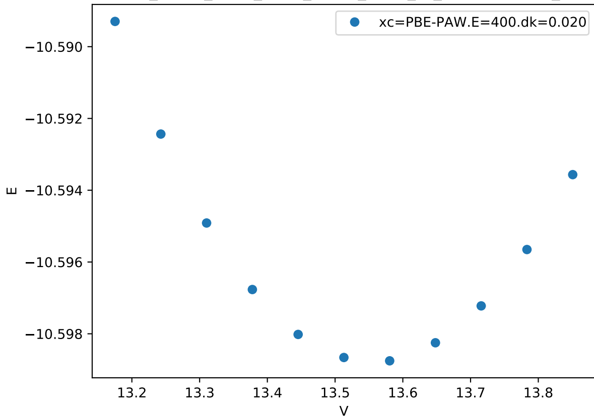
Cr_pv-Co_pv-W_sv/Cr_pv-Co_pv-W_sv_sigma-BCCAA_
