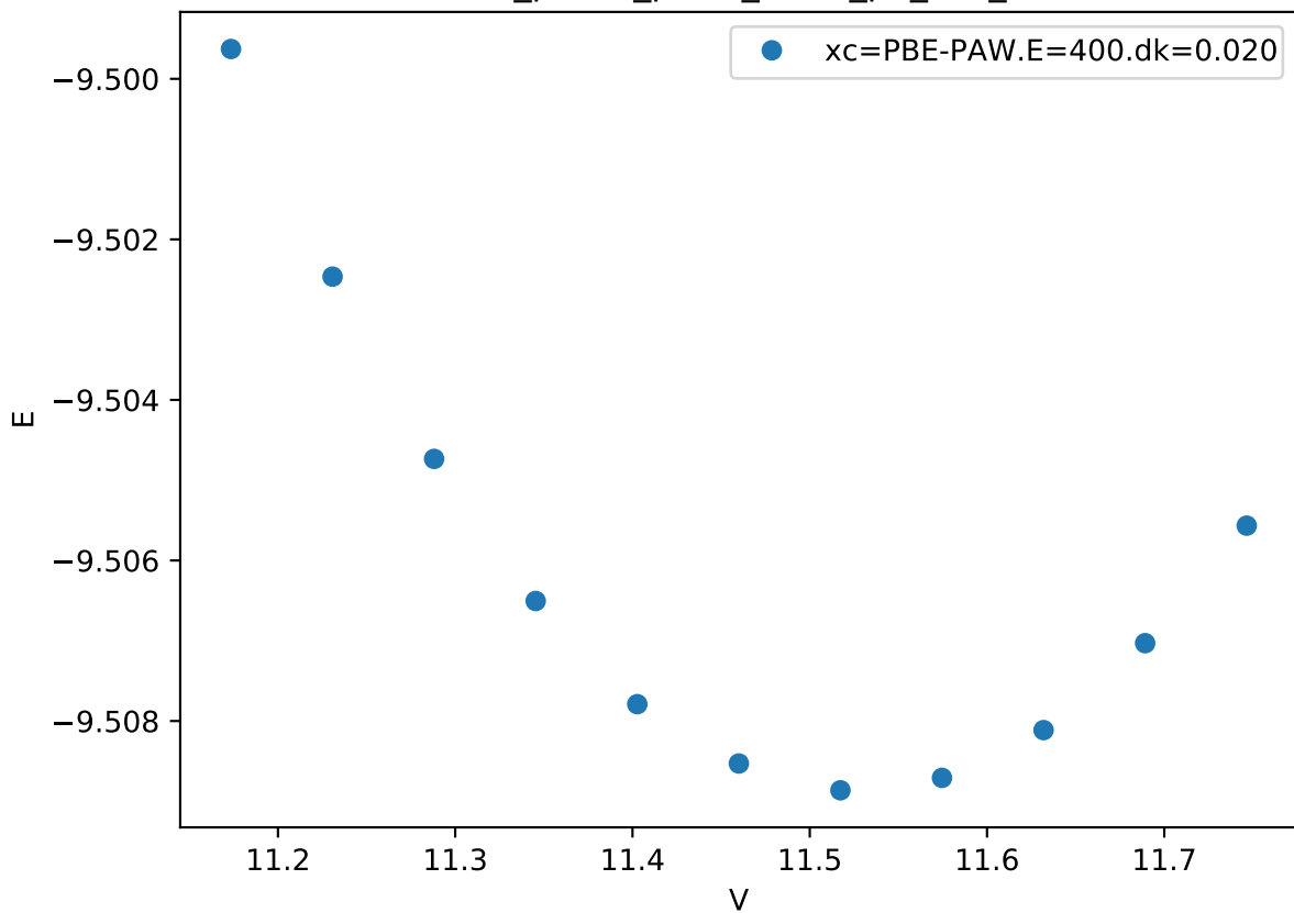
Cr_pv-Co_pv-W_sv/Cr_pv_bcc_
