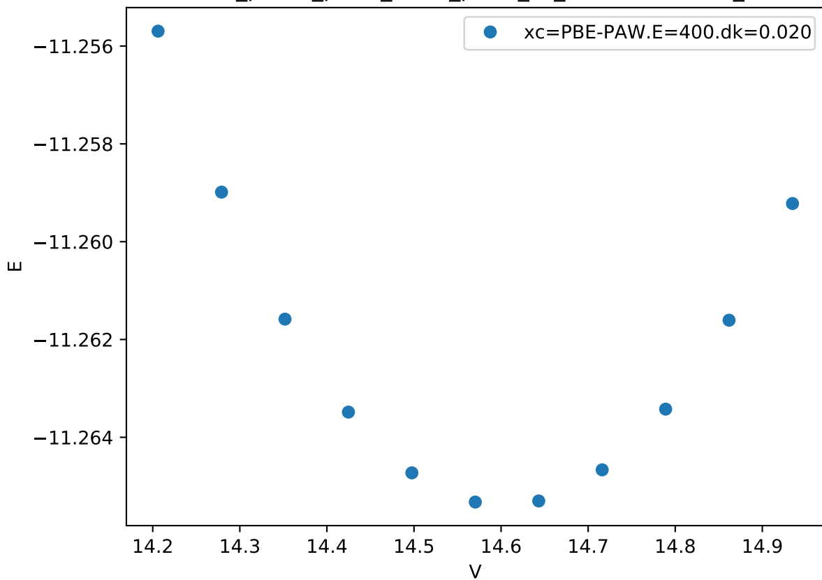
Cr_pv-Co_pv-W_sv/Cr_pv-W_sv_C36-BBABA.FM_
