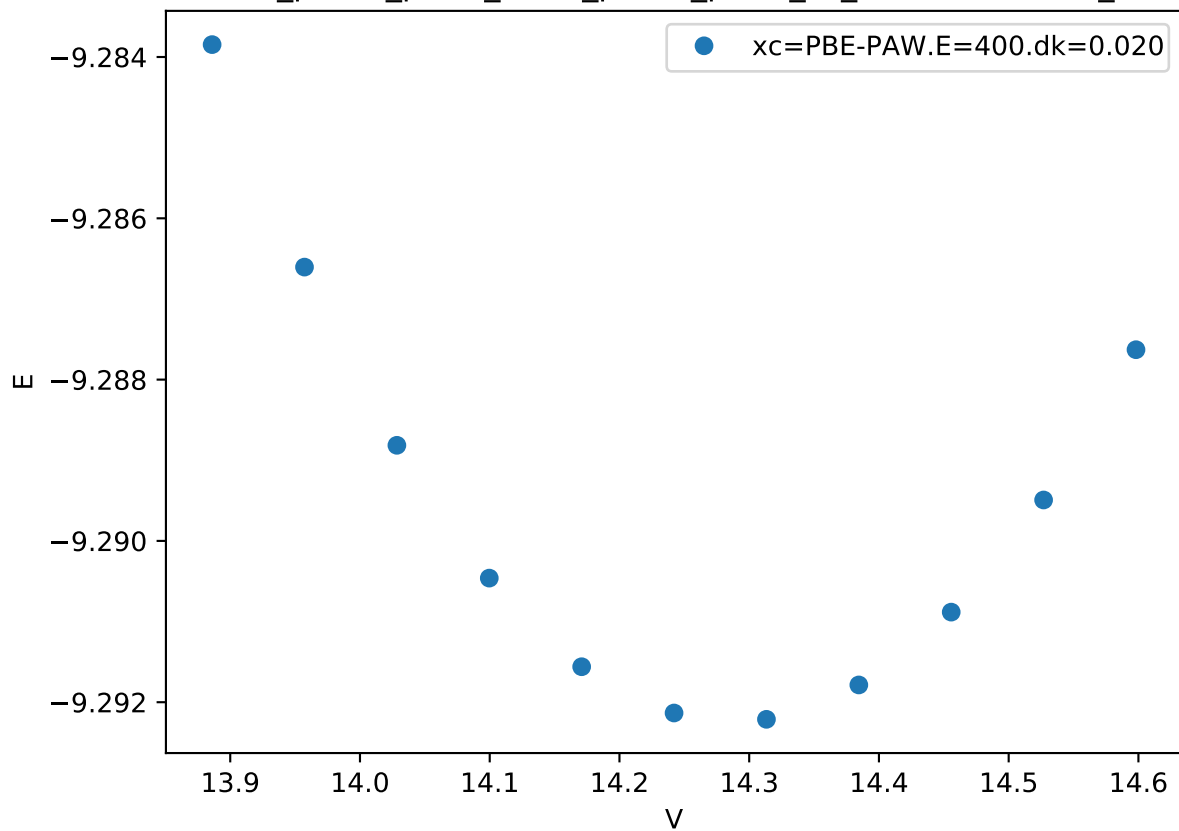
Cr_pv-Co_pv-W_sv/Cr_pv-Co_pv-W_sv_C36-ABCCB.FM_
