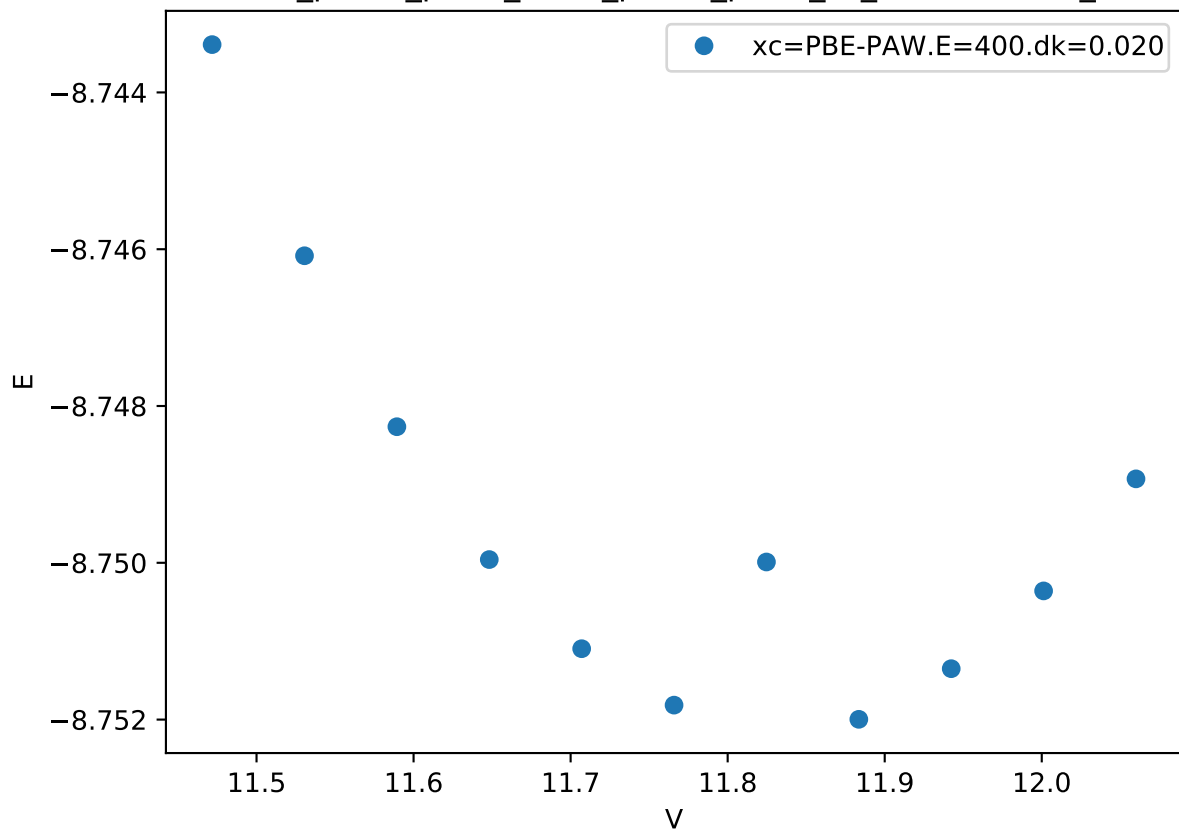
Cr_pv-Co_pv-W_sv/Cr_pv-Co_pv-W_sv_chi-BCBA.FM_
