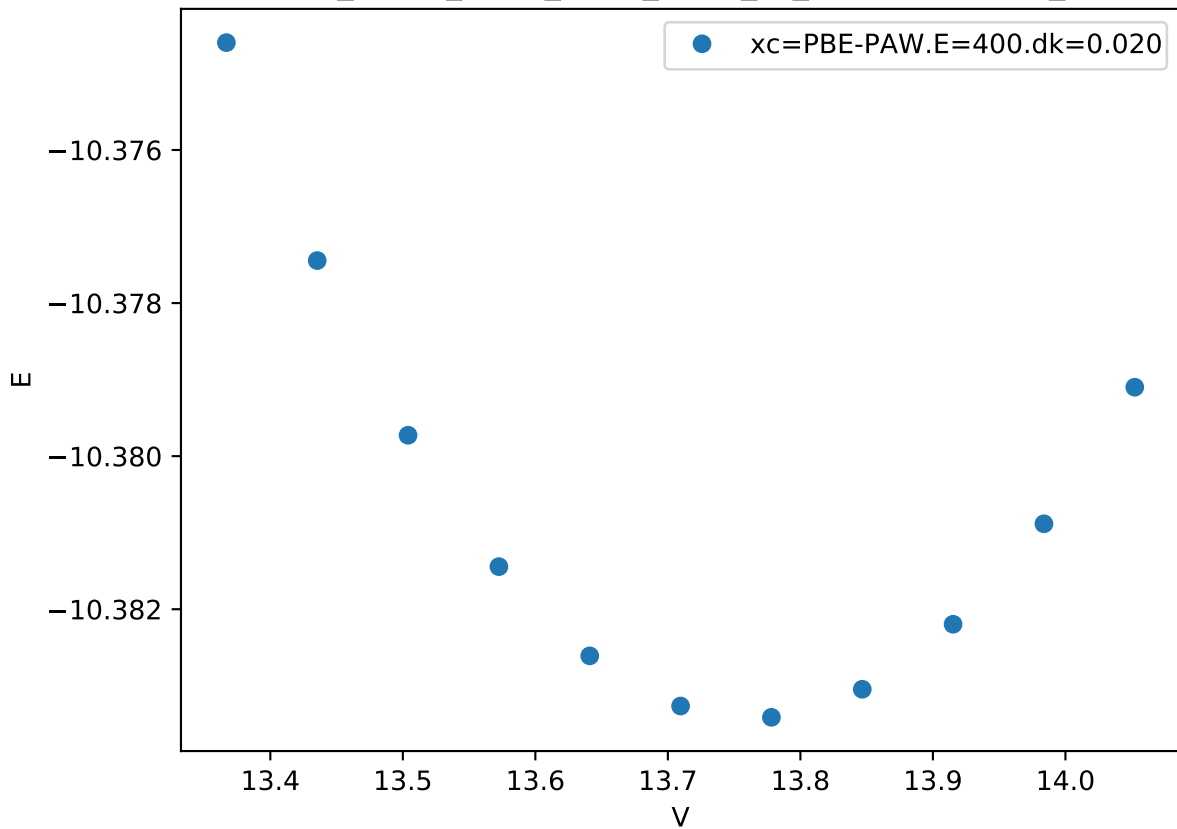
Cr_pv-Co_pv-W_sv/Cr_pv-W_sv_C36-ABBAA.FM_
