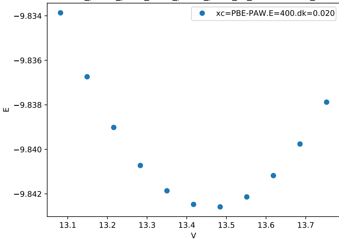
Cr_pv-Co_pv-W_sv/Cr_pv-Co_pv-W_sv_chi-CACB.FM_
