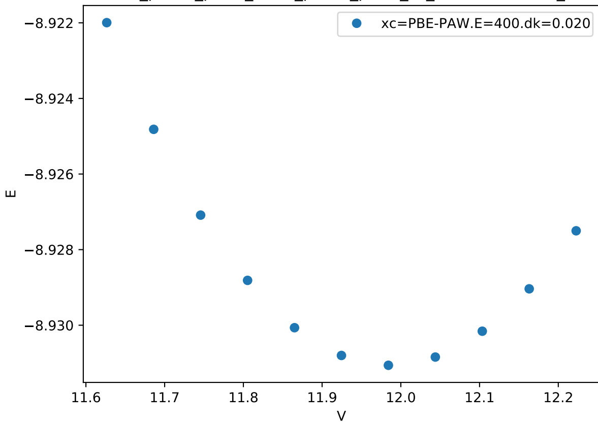
Cr_pv-Co_pv-W_sv/Cr_pv-Co_pv-W_sv_C36-BCAAB.FM_
