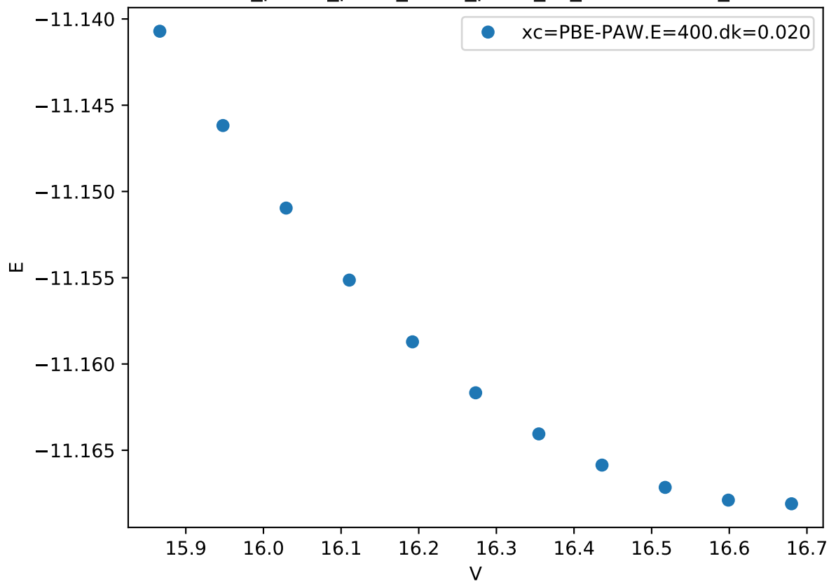
Cr_pv-Co_pv-W_sv/Cr_pv-W_sv_C15-AB2.FM_
