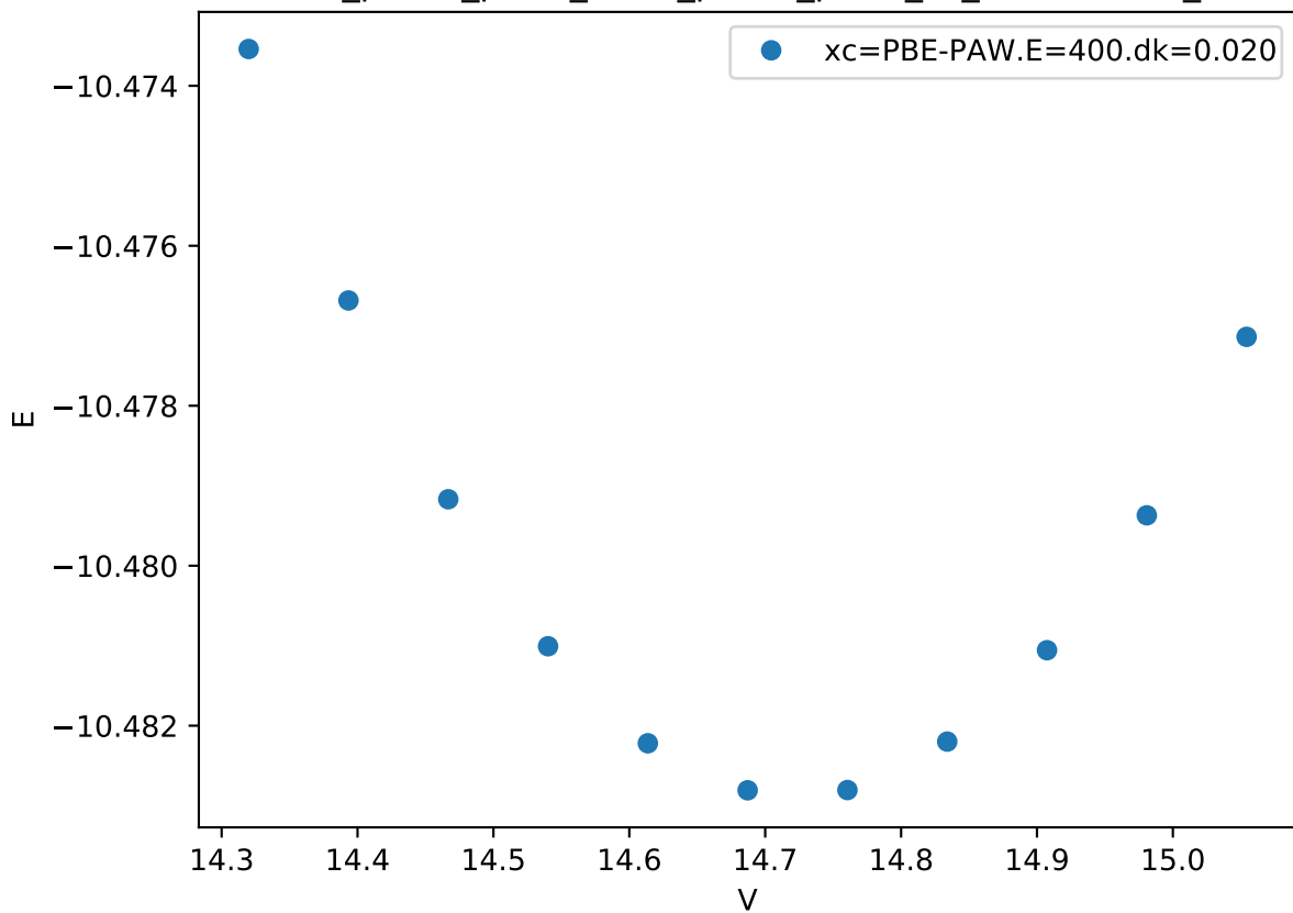
Cr_pv-Co_pv-W_sv/Cr_pv-Co_pv-W_sv_C36-ACCCB_
