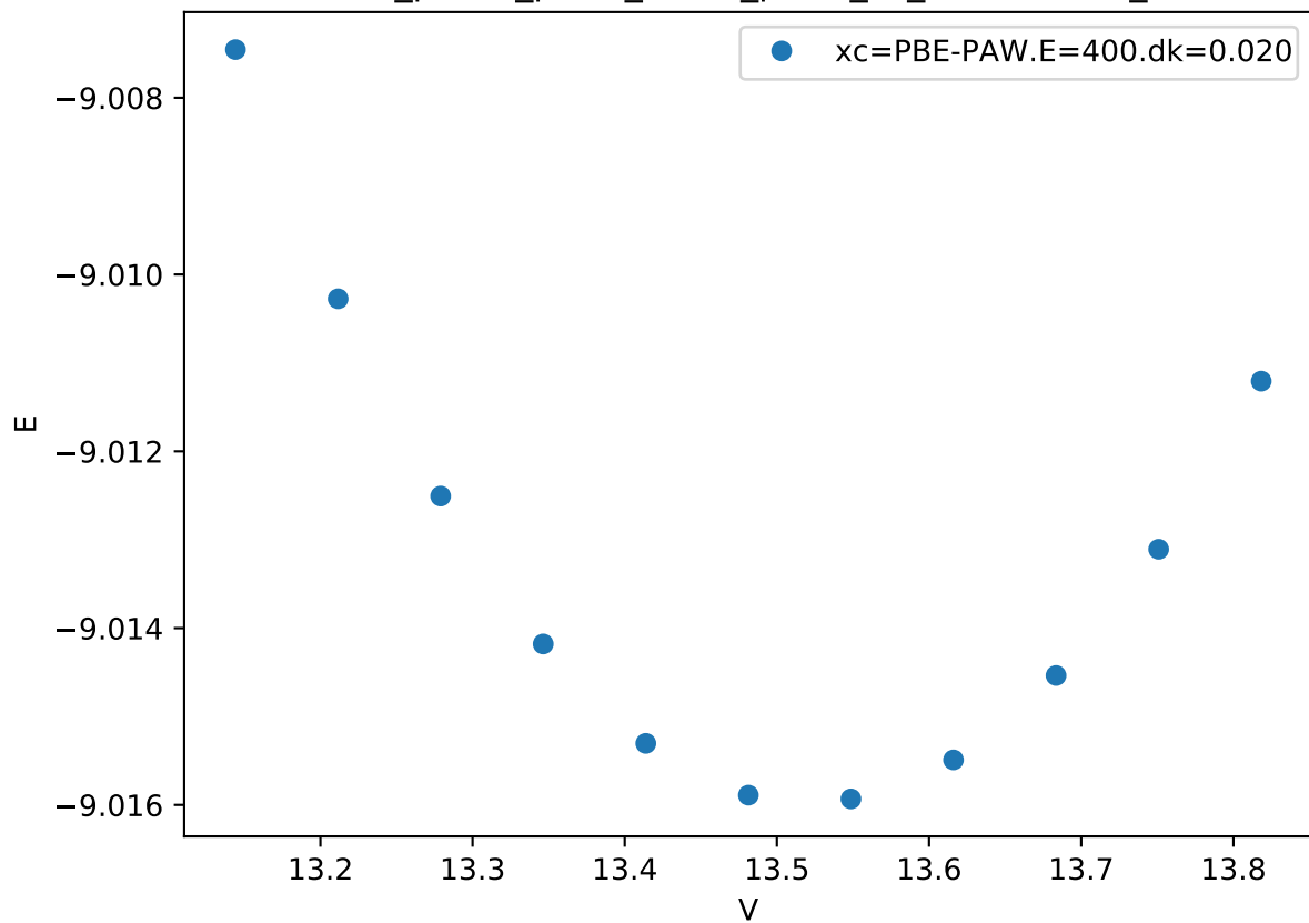
Cr_pv-Co_pv-W_sv/Co_pv-W_sv_C36-ABAAB_
