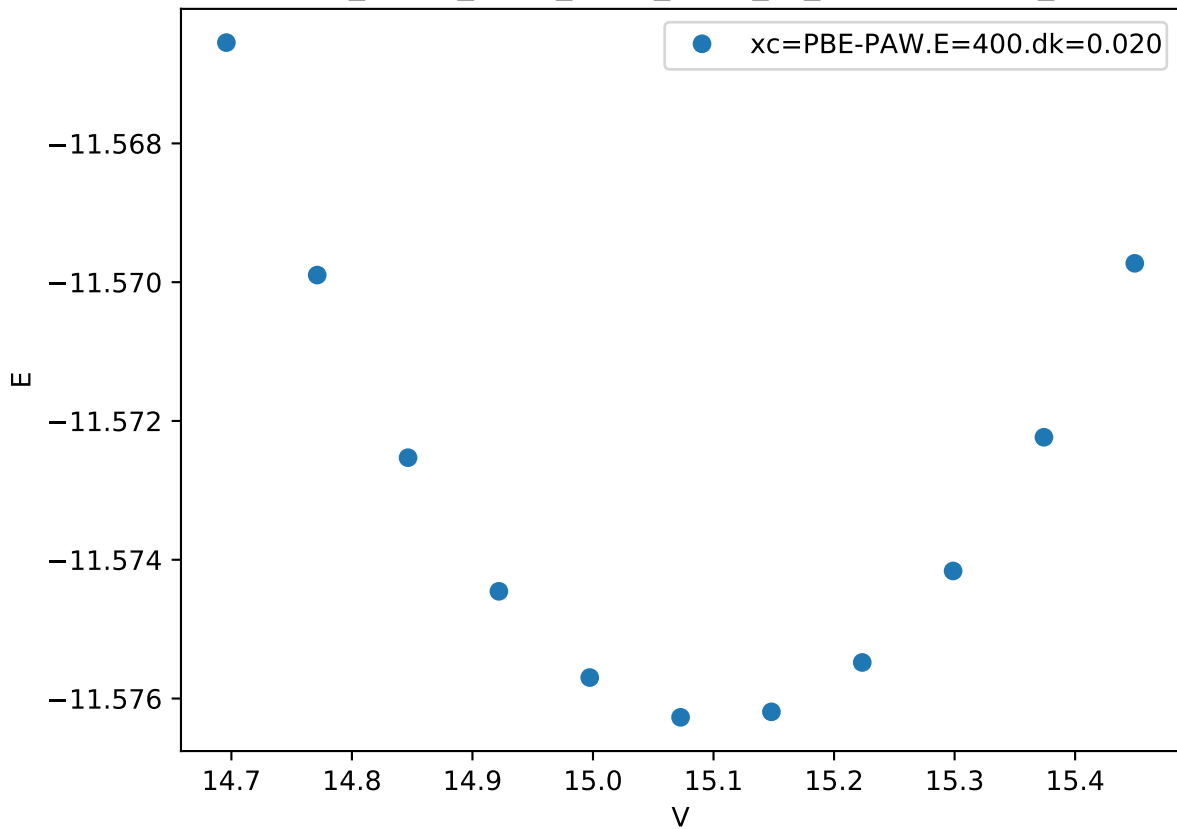
Cr_pv-Co_pv-W_sv/Cr_pv-W_sv_sigma-ABBBA_
