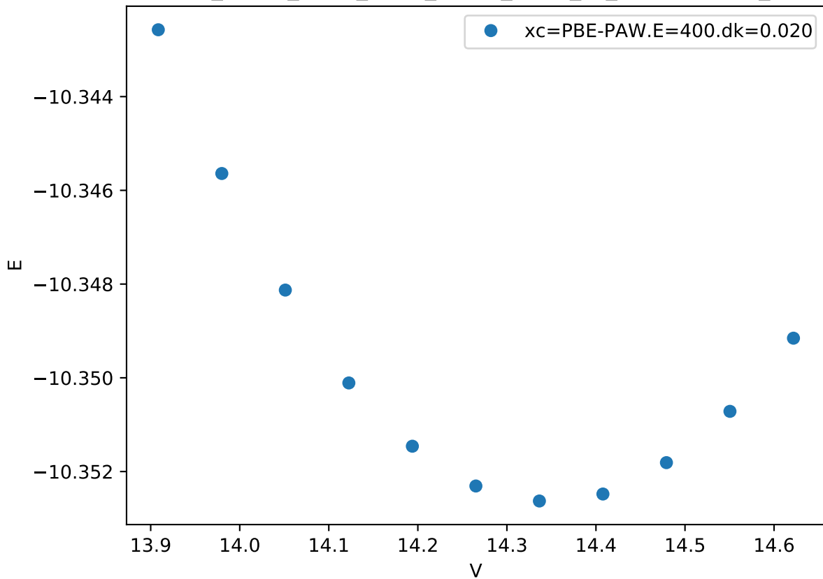
Cr_pv-Co_pv-W_sv/Cr_pv-Co_pv-W_sv_chi-BAAC.FM_
