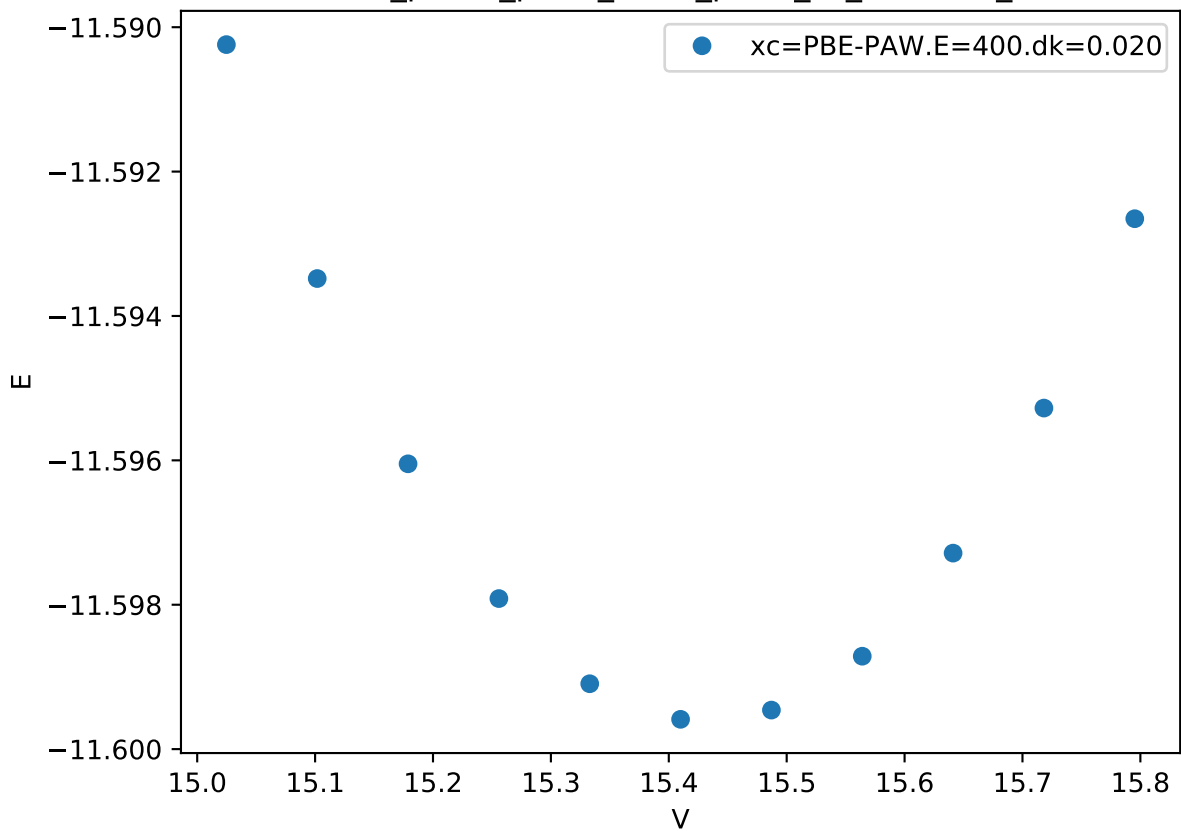
Cr_pv-Co_pv-W_sv/Cr_pv-W_sv_L12-AB3_
