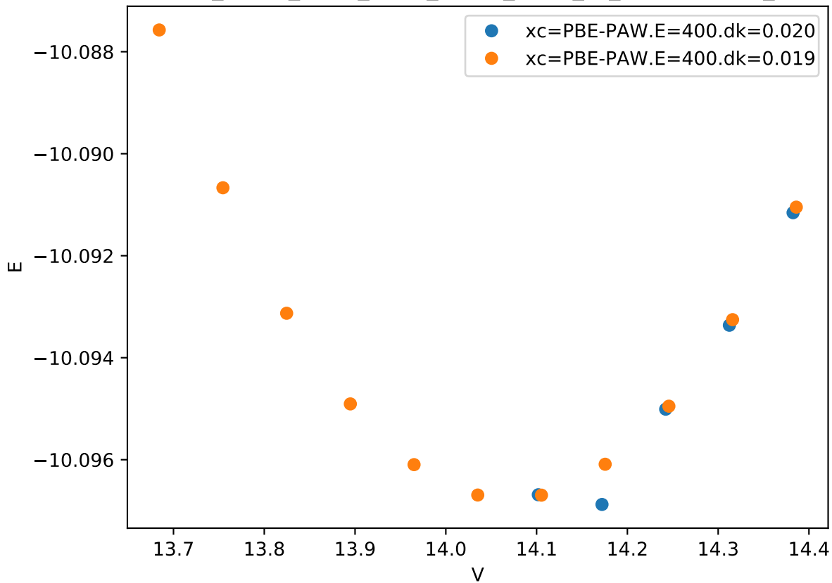
Cr_pv-Co_pv-W_sv/Cr_pv-Co_pv-W_sv_chi-ACBC.FM_
