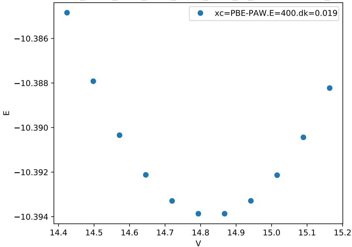
Cr_pv-Co_pv-W_sv/Cr_pv-Co_pv-W_sv_C36-CACBC.FM_
