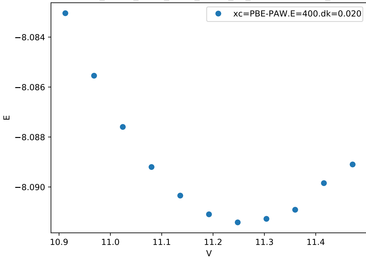
Cr_pv-Co_pv-W_sv/Cr_pv-Co_pv_C36-AAABB.FM_
