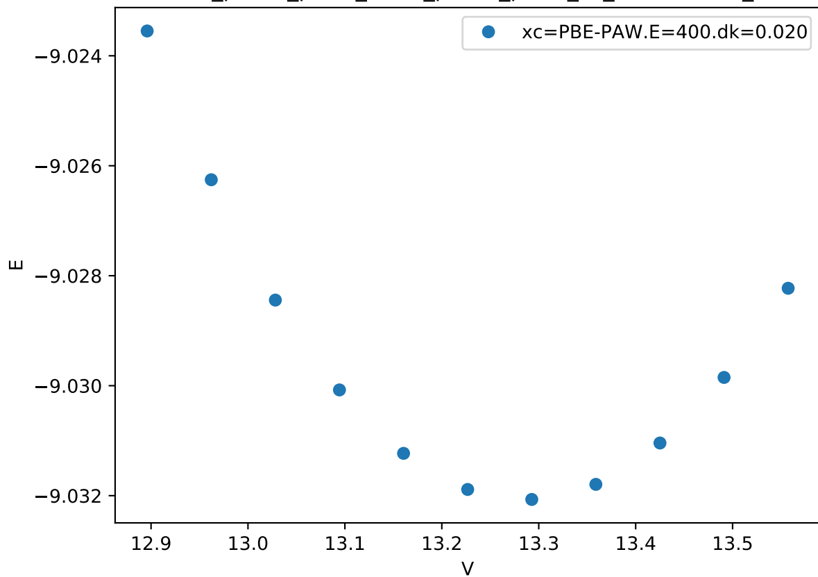
Cr_pv-Co_pv-W_sv/Cr_pv-Co_pv-W_sv_C36-ABBCA_
