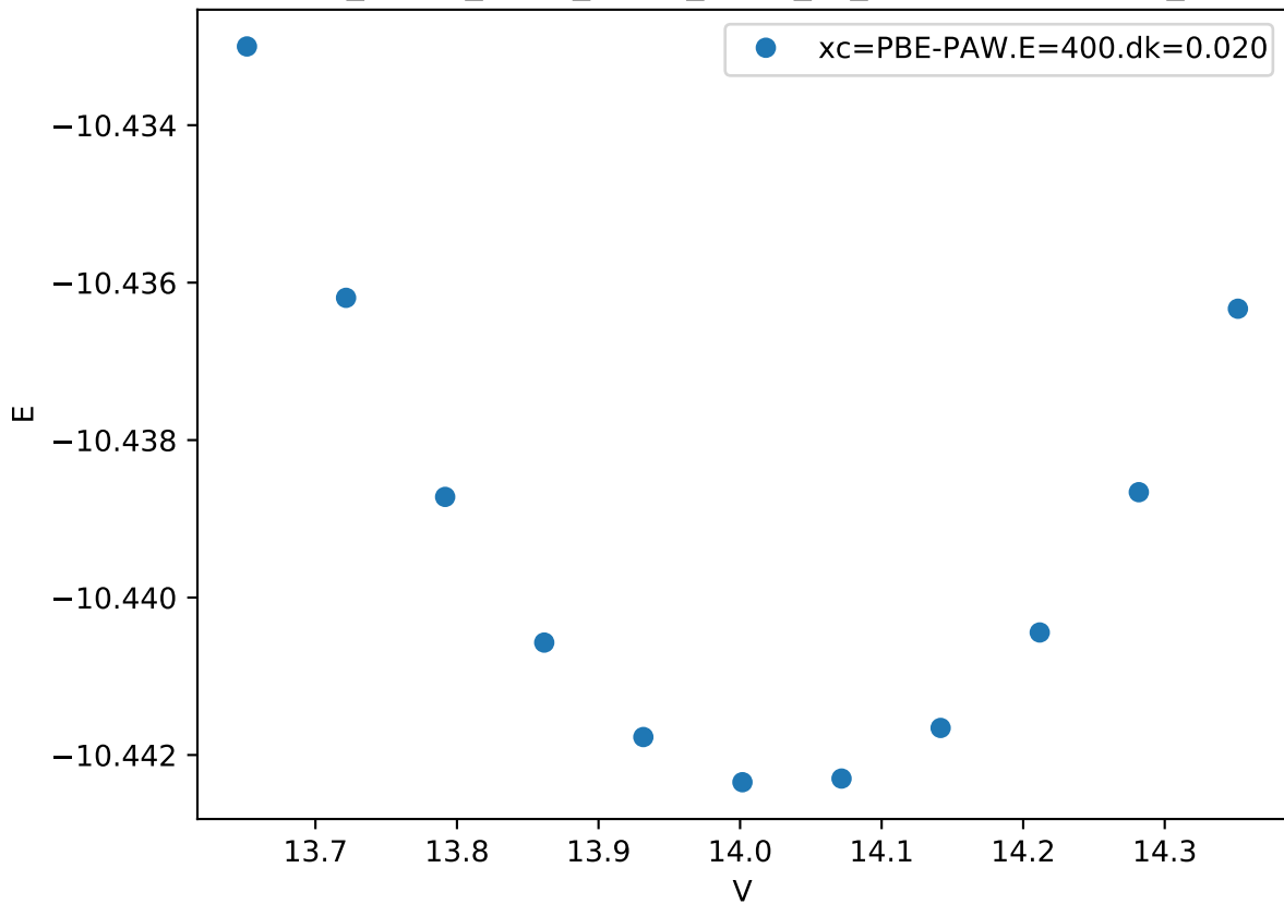
Cr_pv-Co_pv-W_sv/Co_pv-W_sv_sigma-BABAB.FM_
