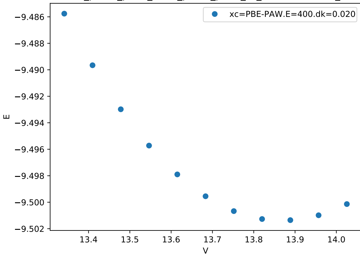
Cr_pv-Co_pv-W_sv/Cr_pv-Co_pv-W_sv_C36-CBACB.FM_
