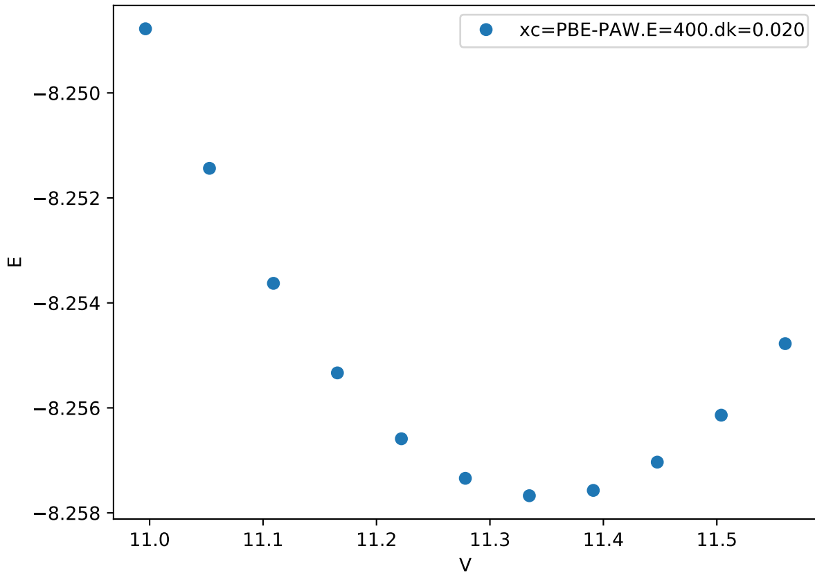
Cr_pv-Co_pv-W_sv/Cr_pv-Co_pv_C36-AABBA_
