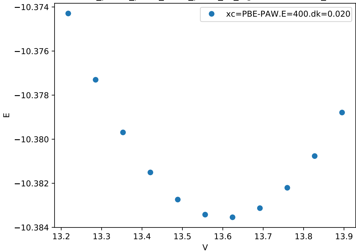
Cr_pv-Co_pv-W_sv/Cr_pv-W_sv_sigma-BAAAB.FM_
