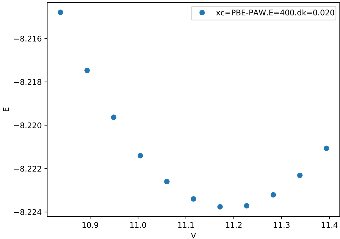
Cr_pv-Co_pv-W_sv/Cr_pv-Co_pv_chi-BABA_
