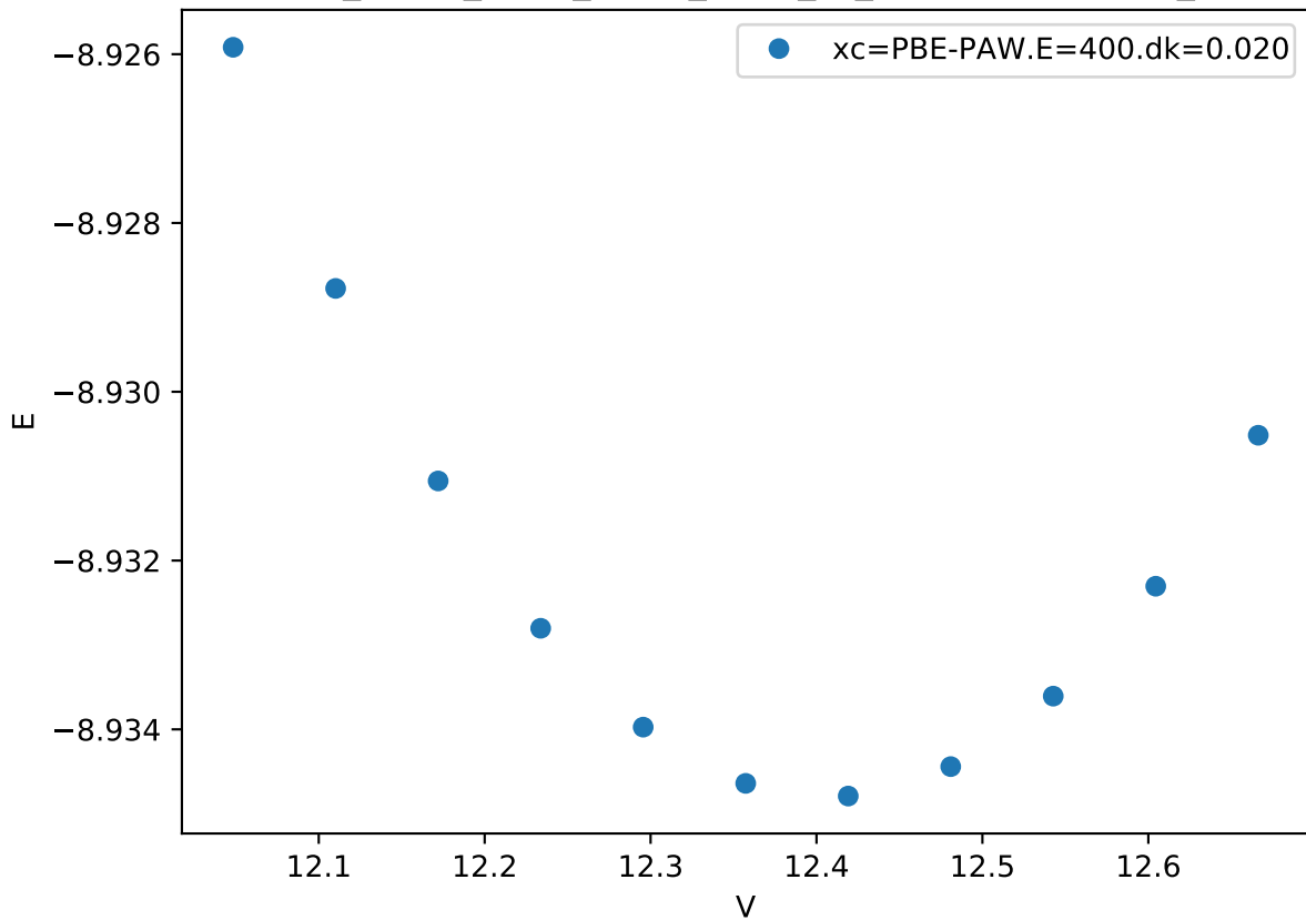
Cr_pv-Co_pv-W_sv/Co_pv-W_sv_sigma-BABAA.FM_
