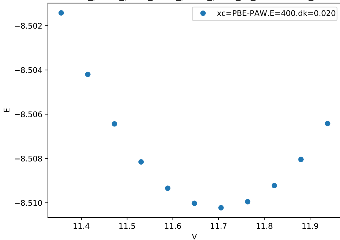
Cr_pv-Co_pv-W_sv/Cr_pv-Co_pv-W_sv_C36-BCBAB_
