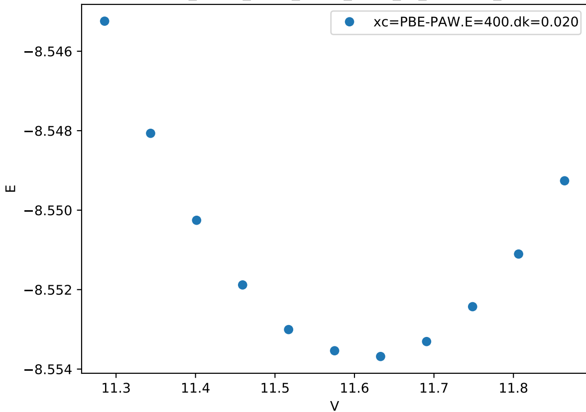
Cr_pv-Co_pv-W_sv/Co_pv-W_sv_L12-A3B_
