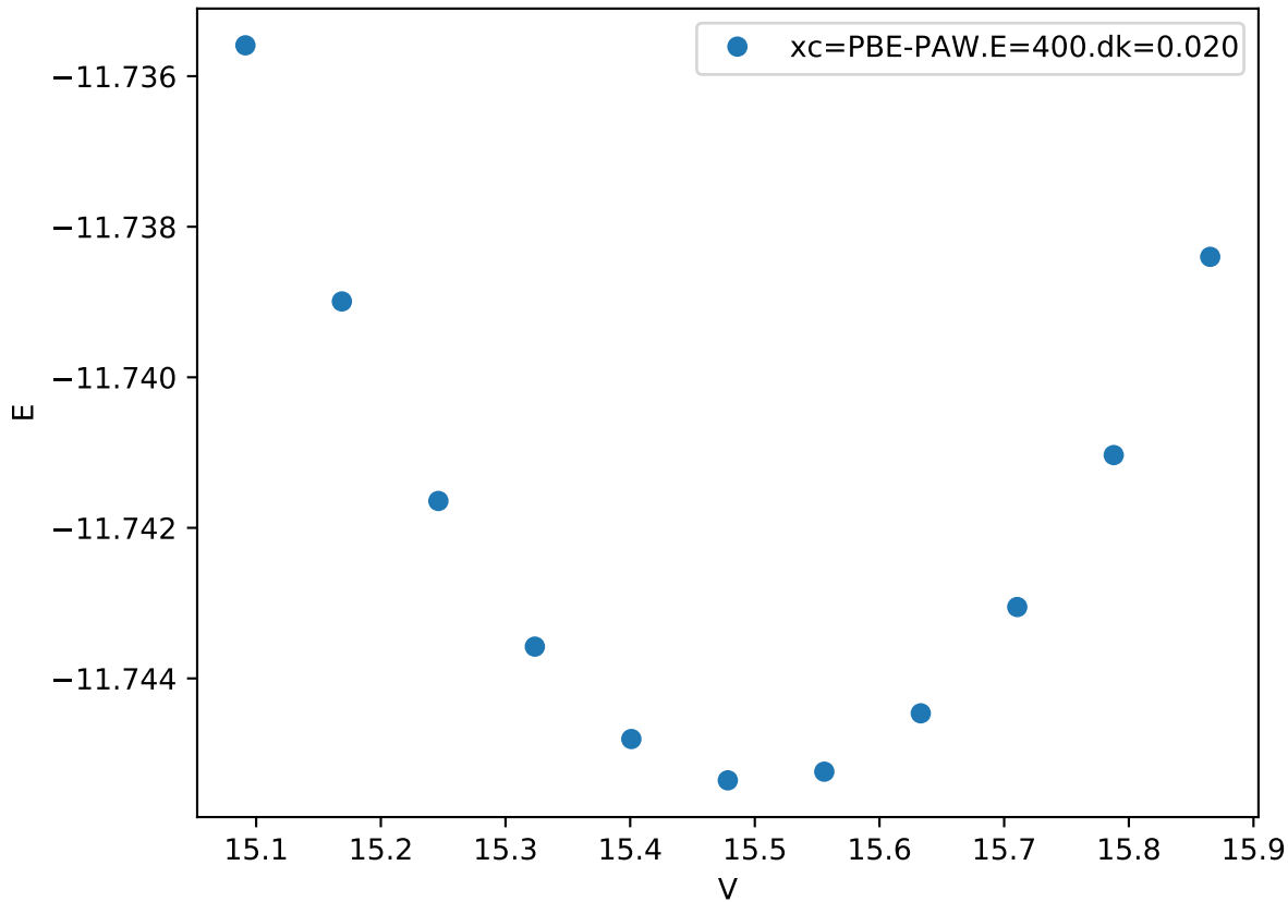
Cr_pv-Co_pv-W_sv/Cr_pv-W_sv_C36-BBBBA_
