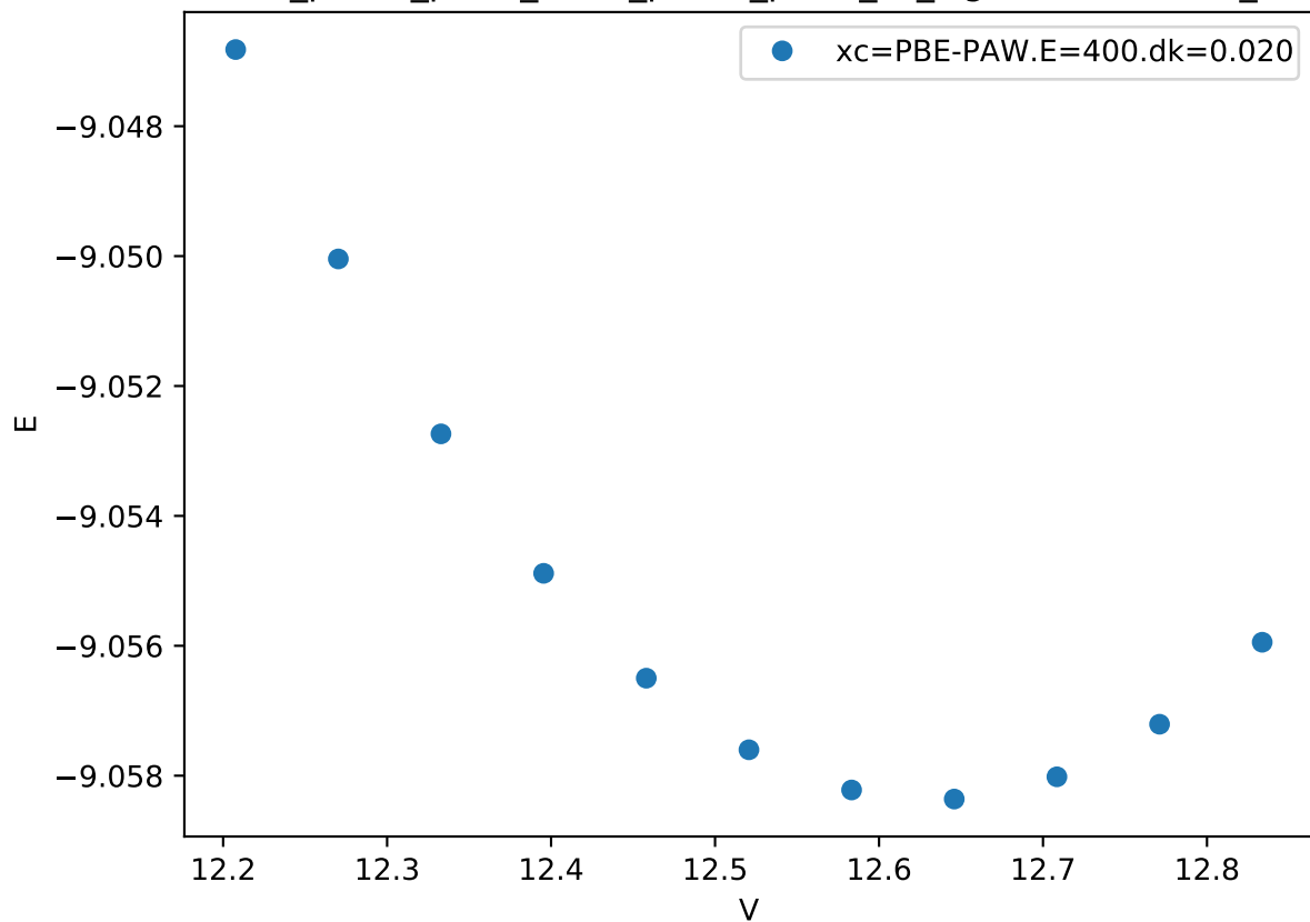
Cr_pv-Co_pv-W_sv/Cr_pv-Co_pv-W_sv_sigma-BBBCA.FM_
