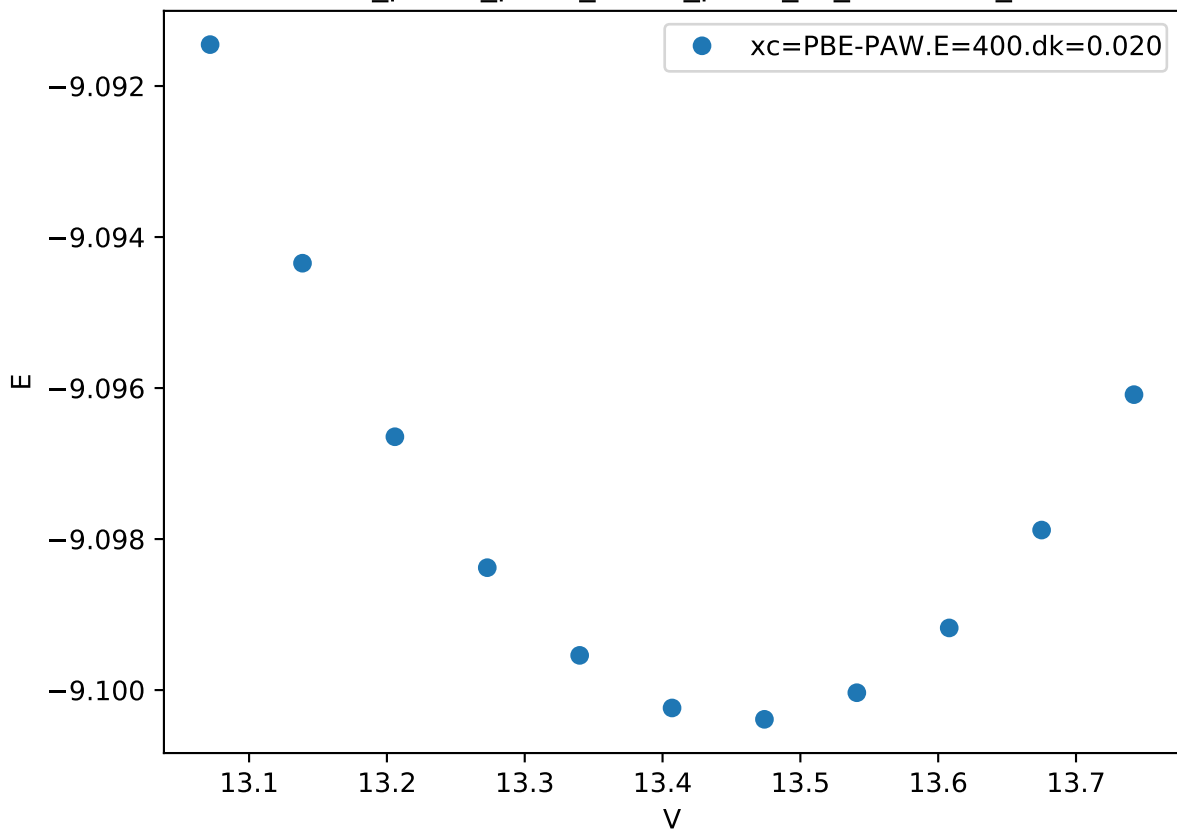
Cr_pv-Co_pv-W_sv/Co_pv-W_sv_chi-AAAB_
