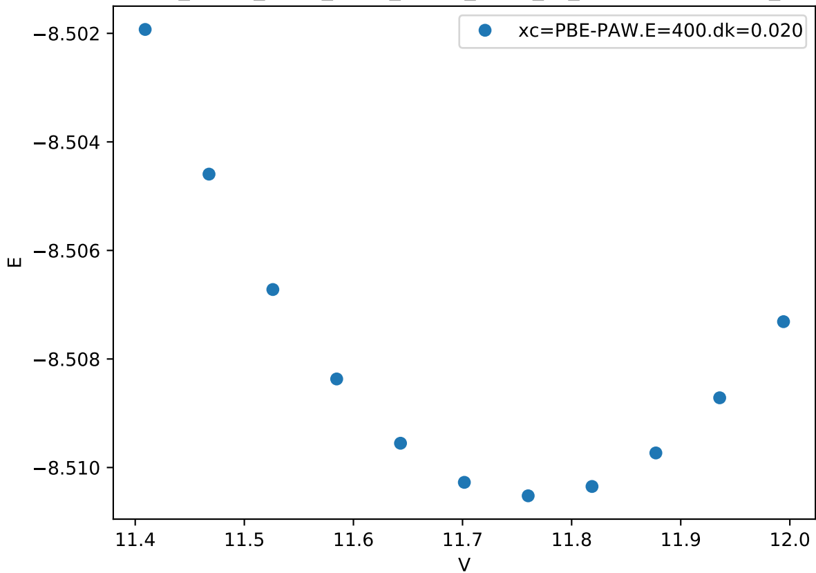
Cr_pv-Co_pv-W_sv/Cr_pv-Co_pv-W_sv_sigma-ACBAB.FM_
