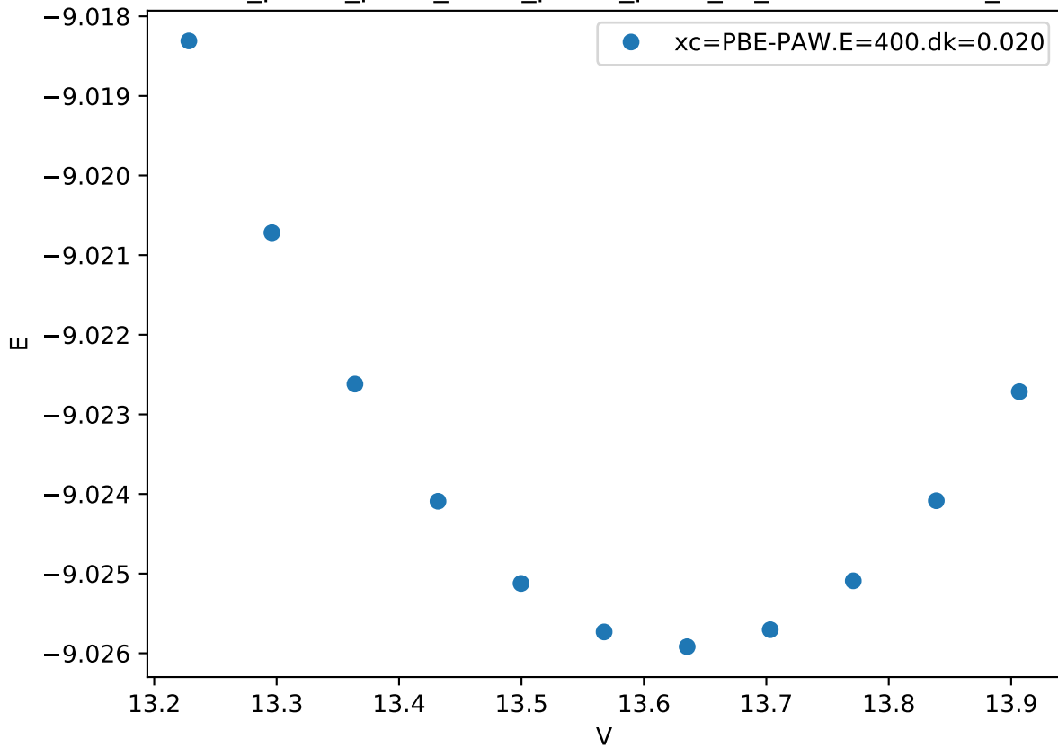
Cr_pv-Co_pv-W_sv/Cr_pv-Co_pv-W_sv_C36-ABBAC.FM_
