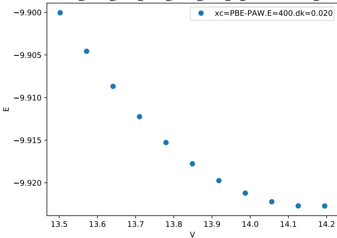
Cr_pv-Co_pv-W_sv/Cr_pv-Co_pv-W_sv_C36-ACABC.FM_
