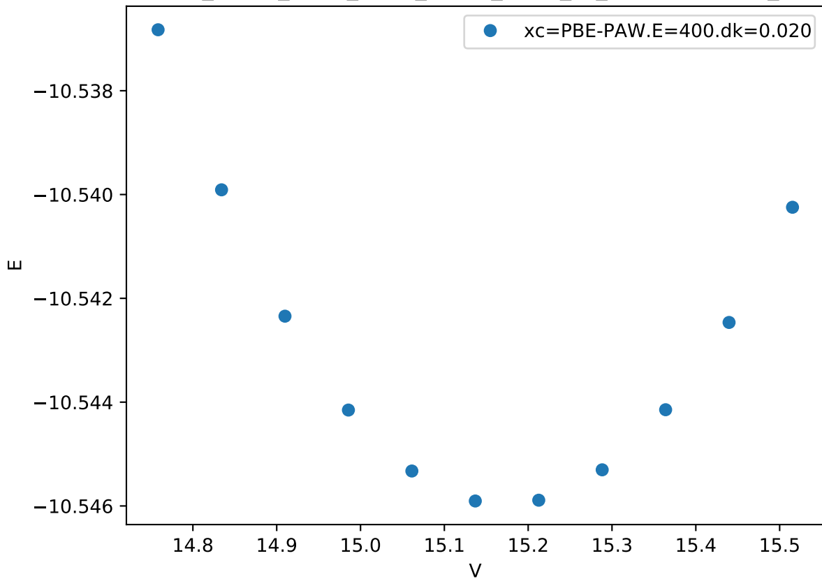
Cr_pv-Co_pv-W_sv/Cr_pv-Co_pv-W_sv_mu-BCCAB.FM_
