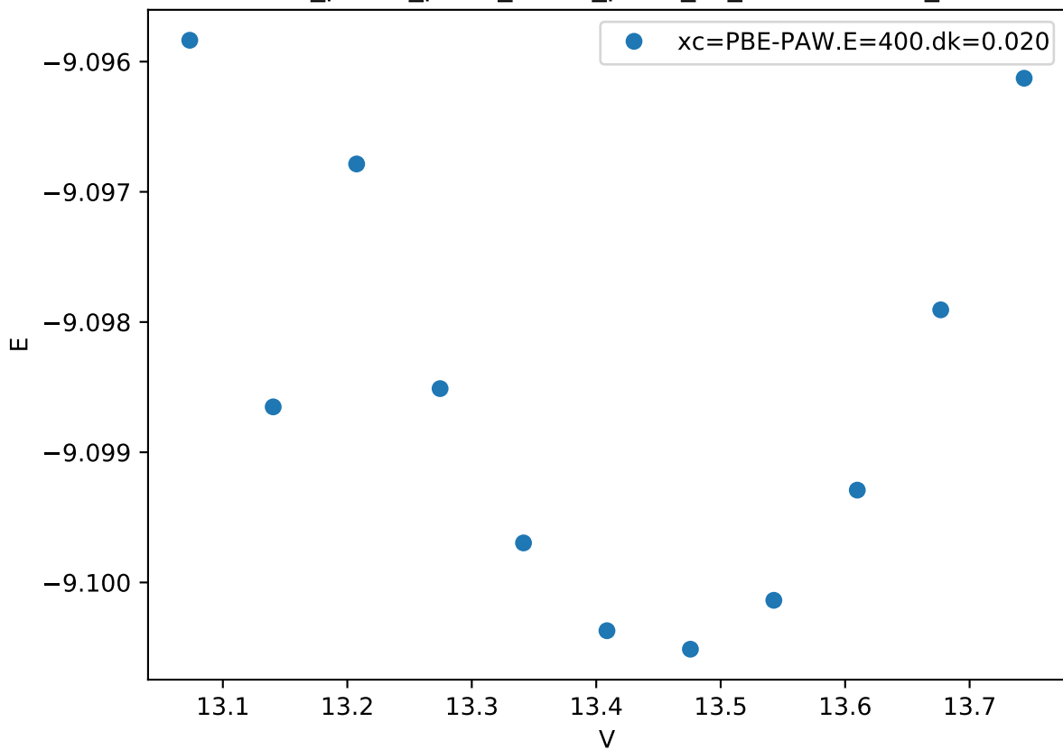
Cr_pv-Co_pv-W_sv/Co_pv-W_sv_chi-AAAB.FM_
