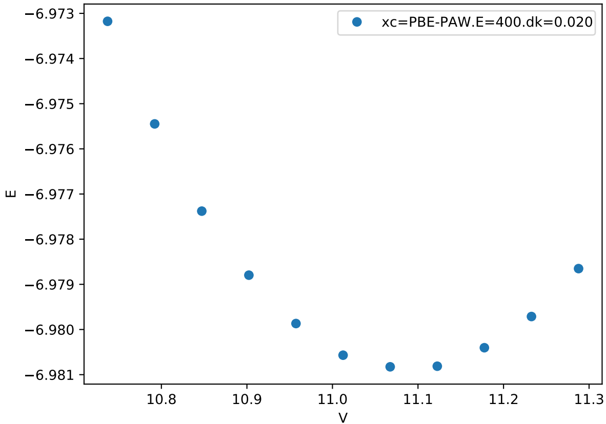
Cr_pv-Co_pv-W_sv/Co_pv_chi.FM_
