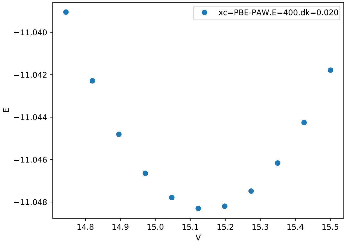
Cr_pv-Co_pv-W_sv/Co_pv-W_sv_sigma-BBBBA_
