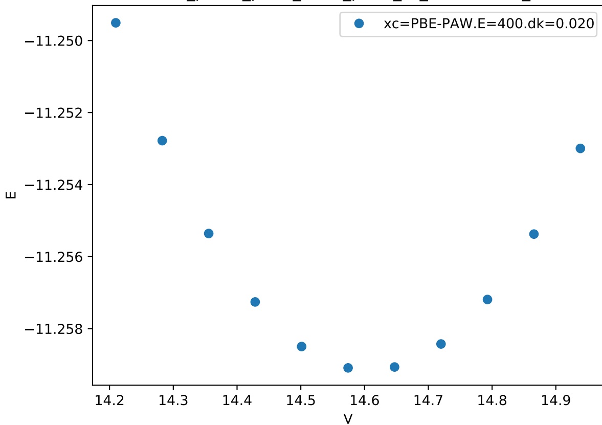
Cr_pv-Co_pv-W_sv/Cr_pv-W_sv_C36-BBAAB_
