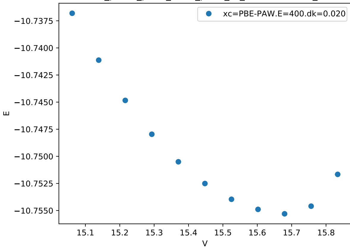
Cr_pv-Co_pv-W_sv/Cr_pv-W_sv_mu-BBAAA.FM_
