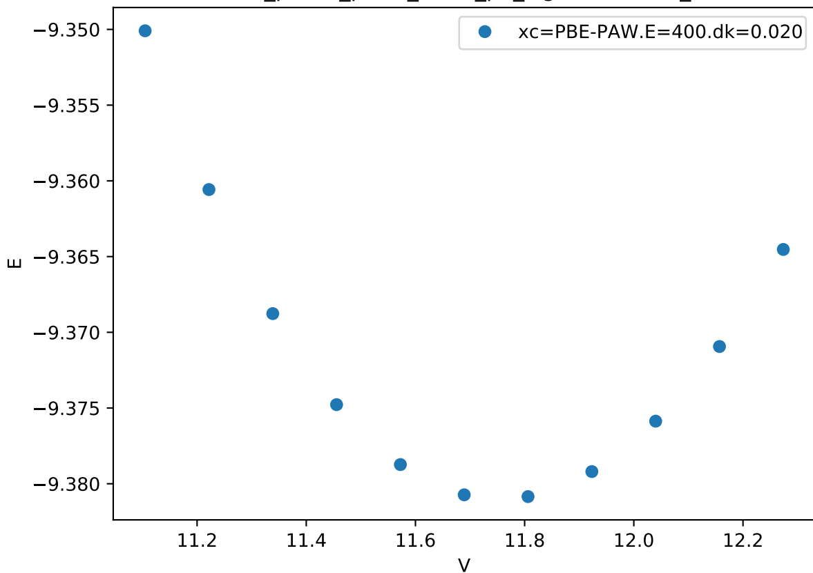
Cr_pv-Co_pv-W_sv/Cr_pv_sigma.UDUUU_
