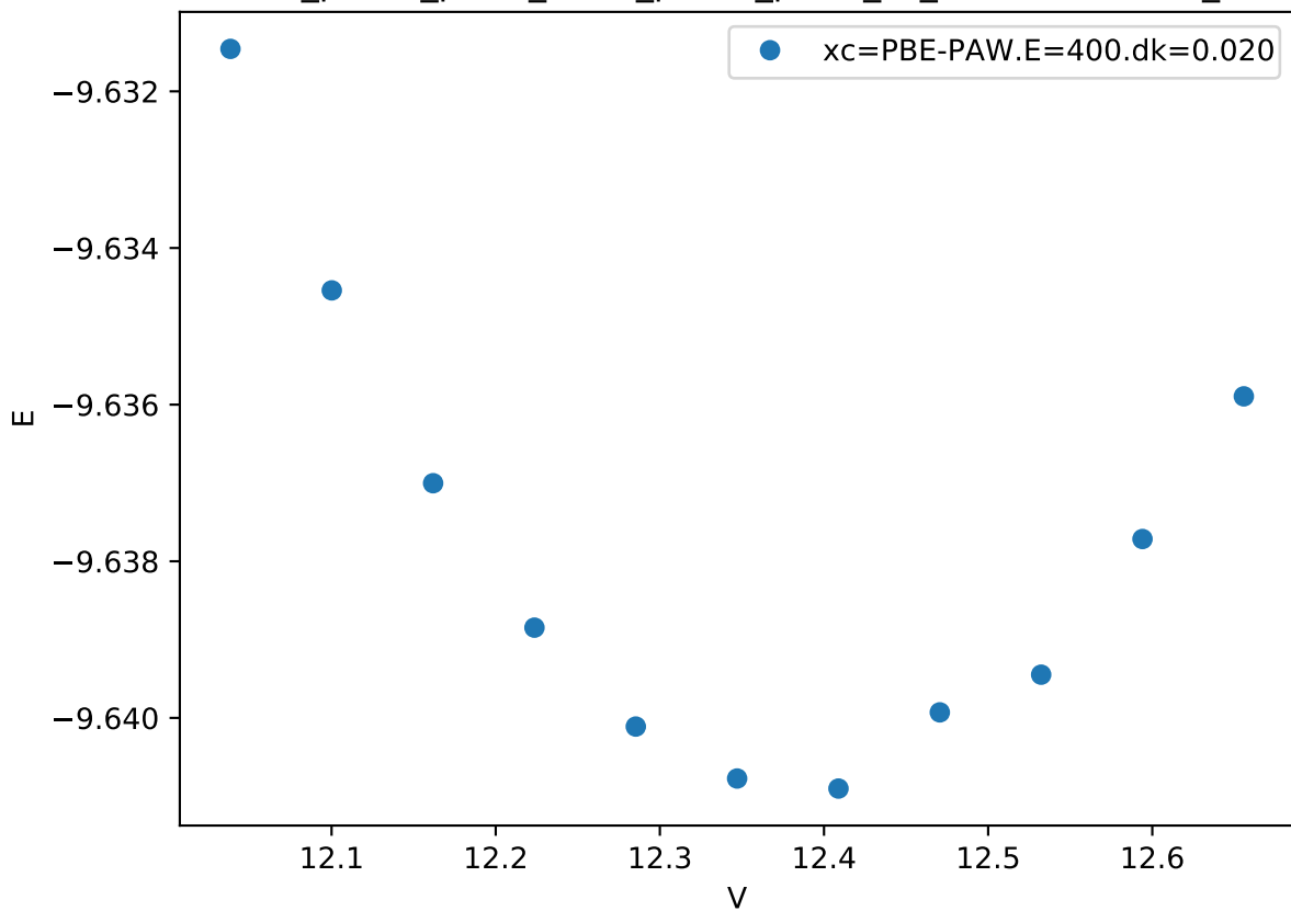
Cr_pv-Co_pv-W_sv/Cr_pv-Co_pv-W_sv_C36-CCBBA.FM_
