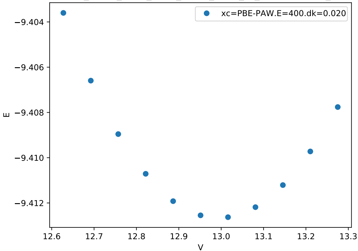
Cr_pv-Co_pv-W_sv/Cr_pv-Co_pv-W_sv_sigma-ACBCB_
