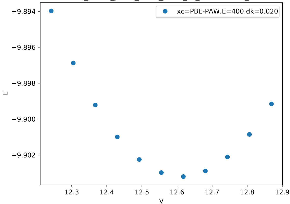
Cr_pv-Co_pv-W_sv/Cr_pv-W_sv_C36-ABAAA_
