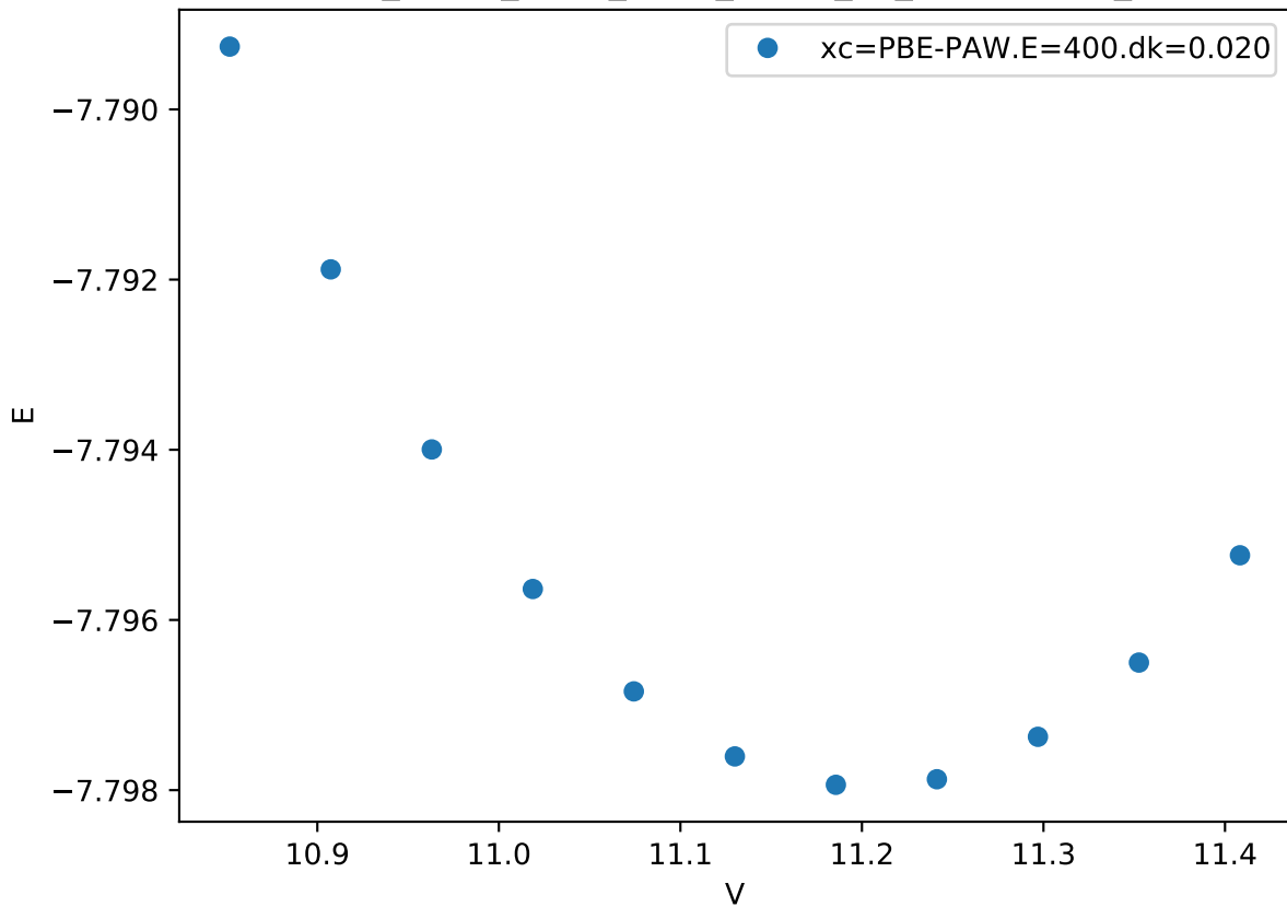
Cr_pv-Co_pv-W_sv/Cr_pv-Co_pv_C36-ABBBA_
