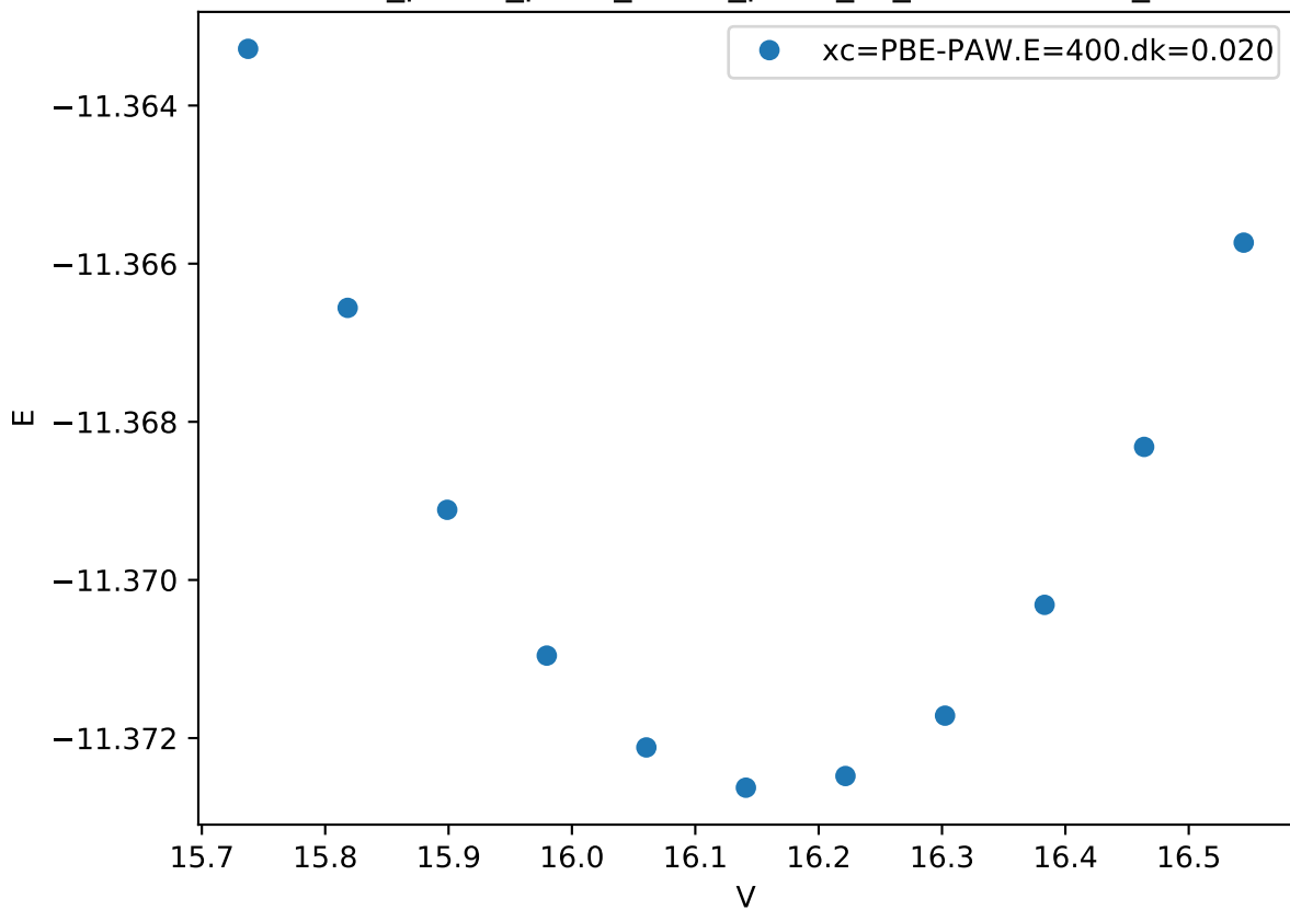
Cr_pv-Co_pv-W_sv/Co_pv-W_sv_chi-AABB.FM_
