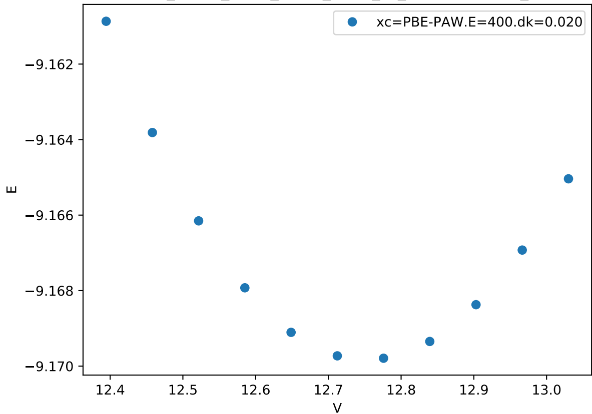
Cr_pv-Co_pv-W_sv/Co_pv-W_sv_mu-BAABB.FM_
