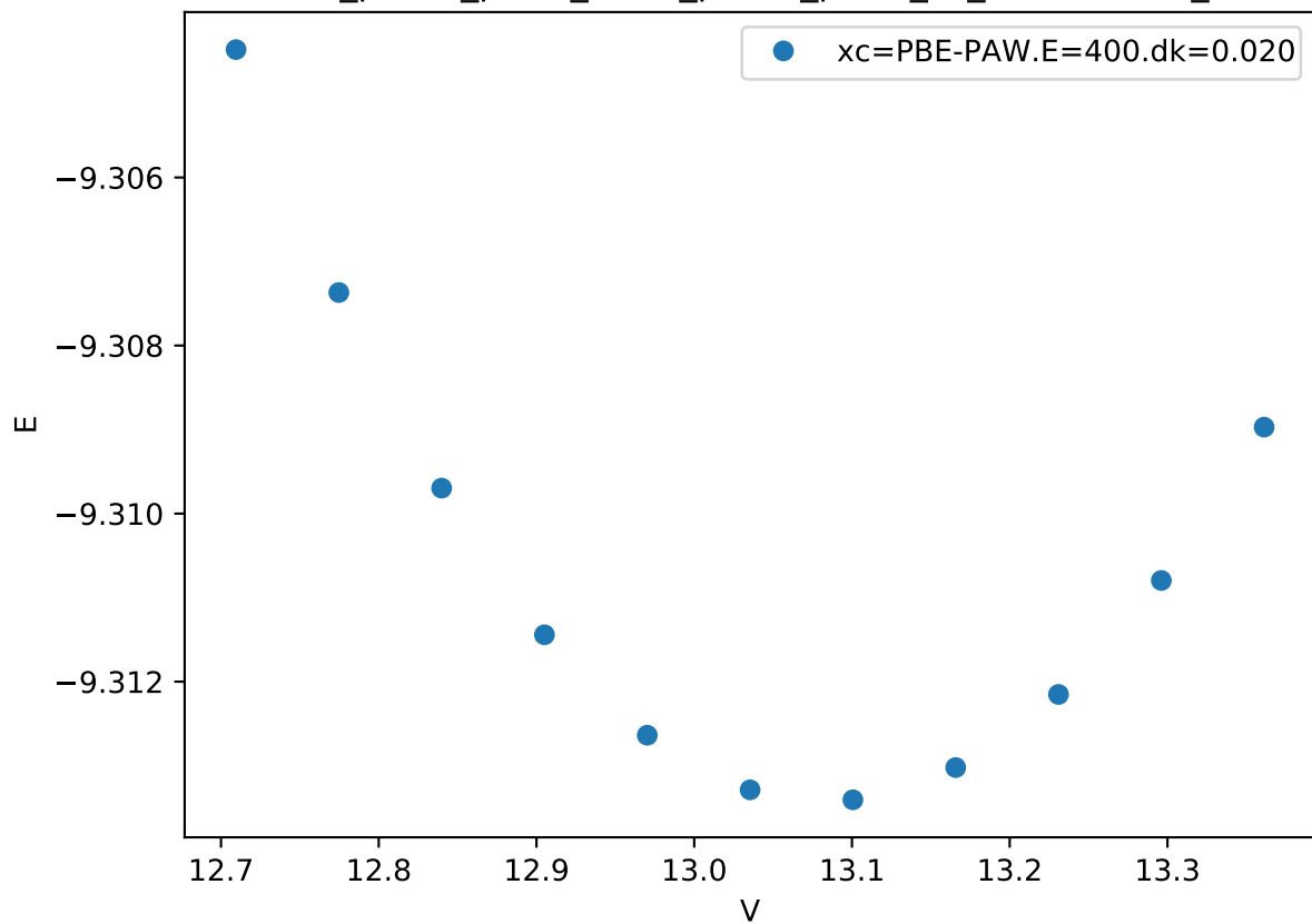
Cr_pv-Co_pv-W_sv/Cr_pv-Co_pv-W_sv_C36-BCCBA_
