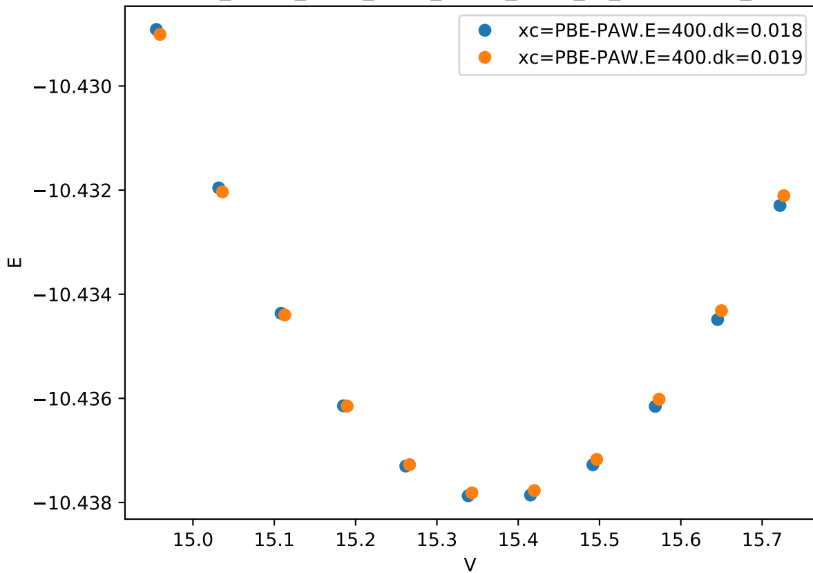
Cr_pv-Co_pv-W_sv/Cr_pv-Co_pv-W_sv_mu-BCBAC_
