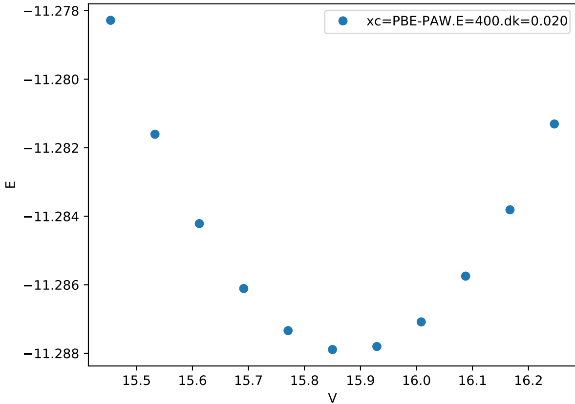
Cr_pv-Co_pv-W_sv/Cr_pv-Co_pv-W_sv_mu-ACBCC.FM_
