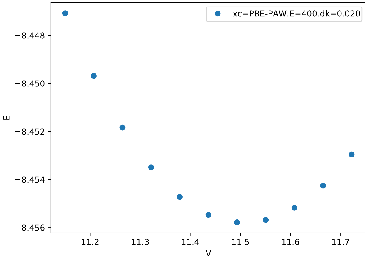
Cr_pv-Co_pv-W_sv/Cr_pv-Co_pv_C36-BABAA_
