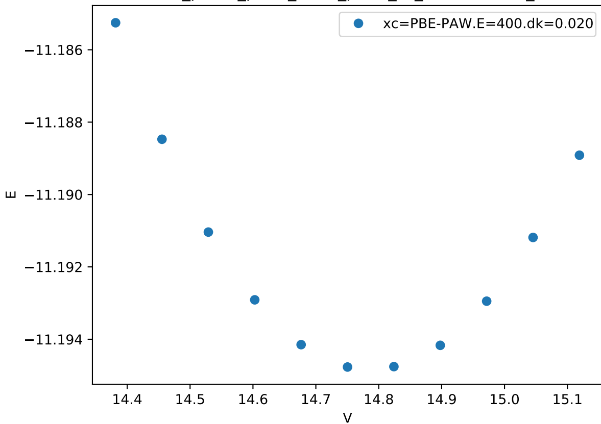
Cr_pv-Co_pv-W_sv/Cr_pv-W_sv_chi-BBAB.FM_
