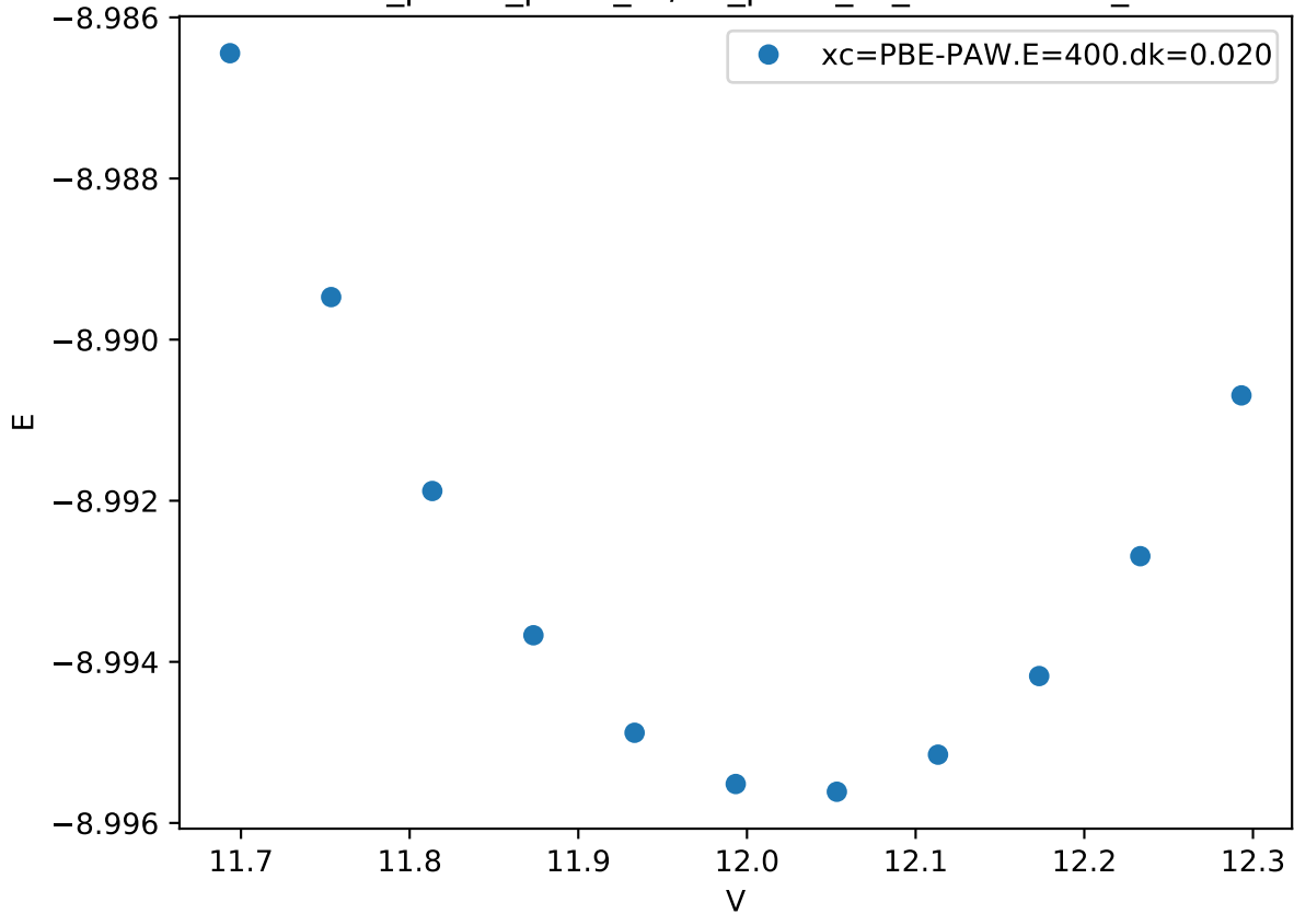
Cr_pv-Co_pv-W_sv/Co_pv-W_sv_C36-BBAAA_
