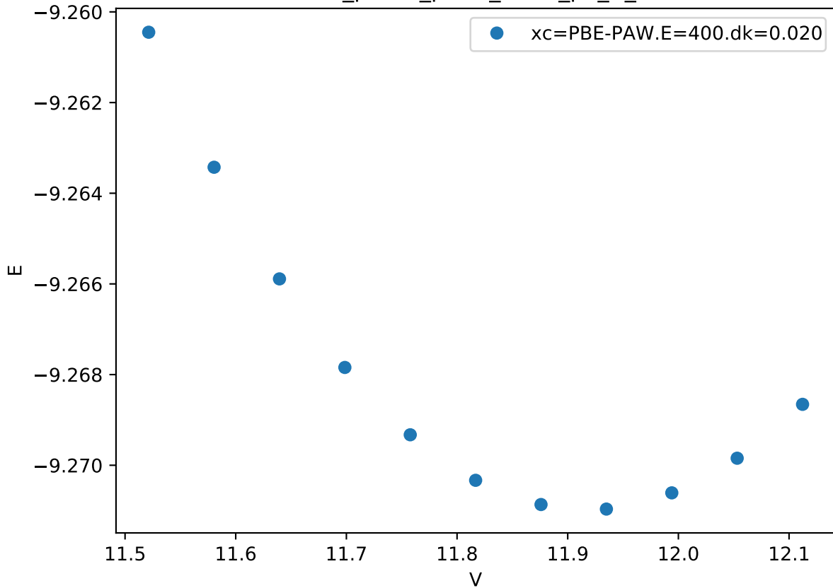
Cr_pv-Co_pv-W_sv/Cr_pv_R_
