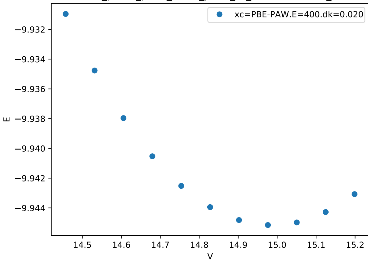
Cr_pv-Co_pv-W_sv/Co_pv-W_sv_C36-ABBAB.FM_
