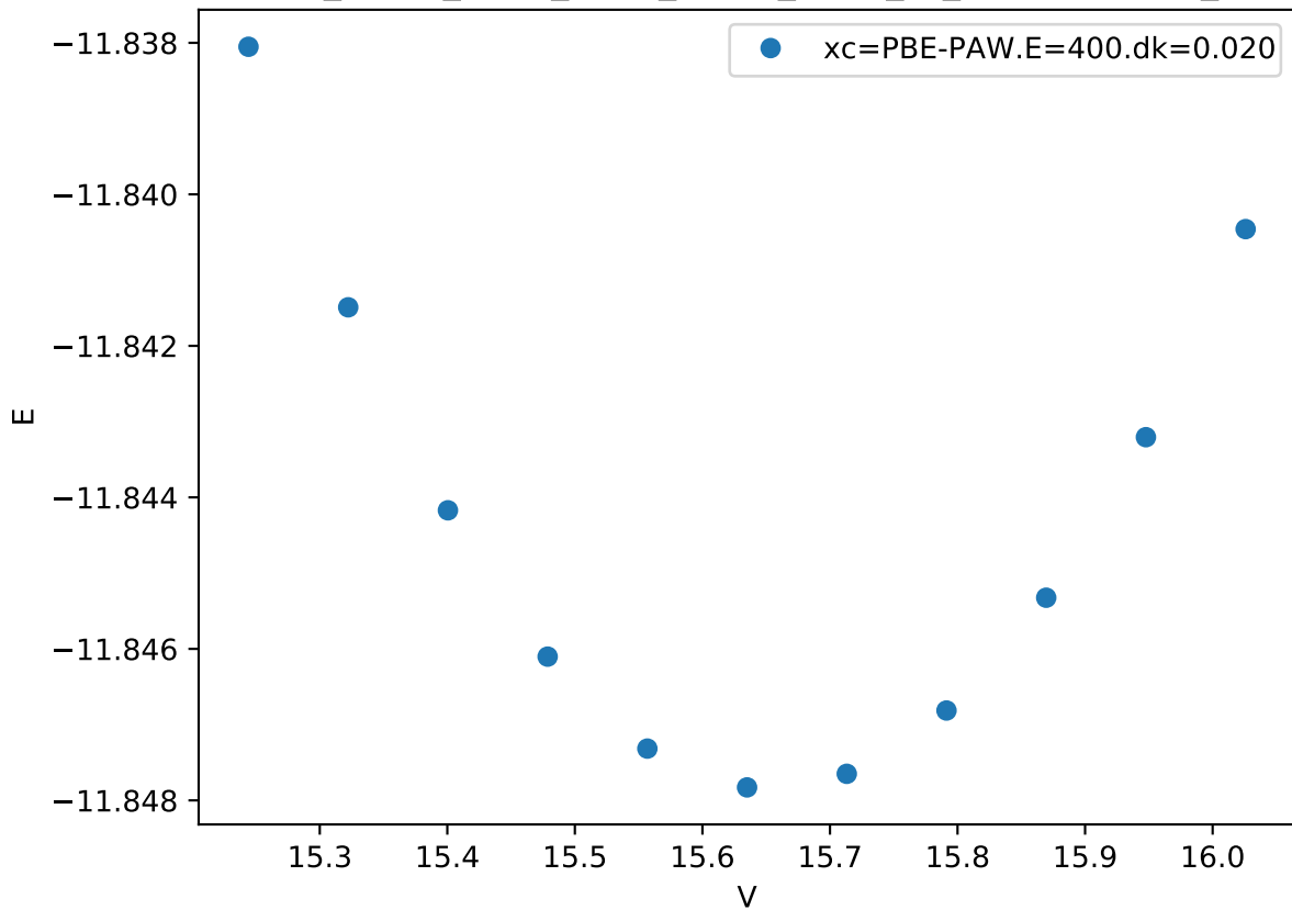
Cr_pv-Co_pv-W_sv/Cr_pv-Co_pv-W_sv_sigma-BACCC_
