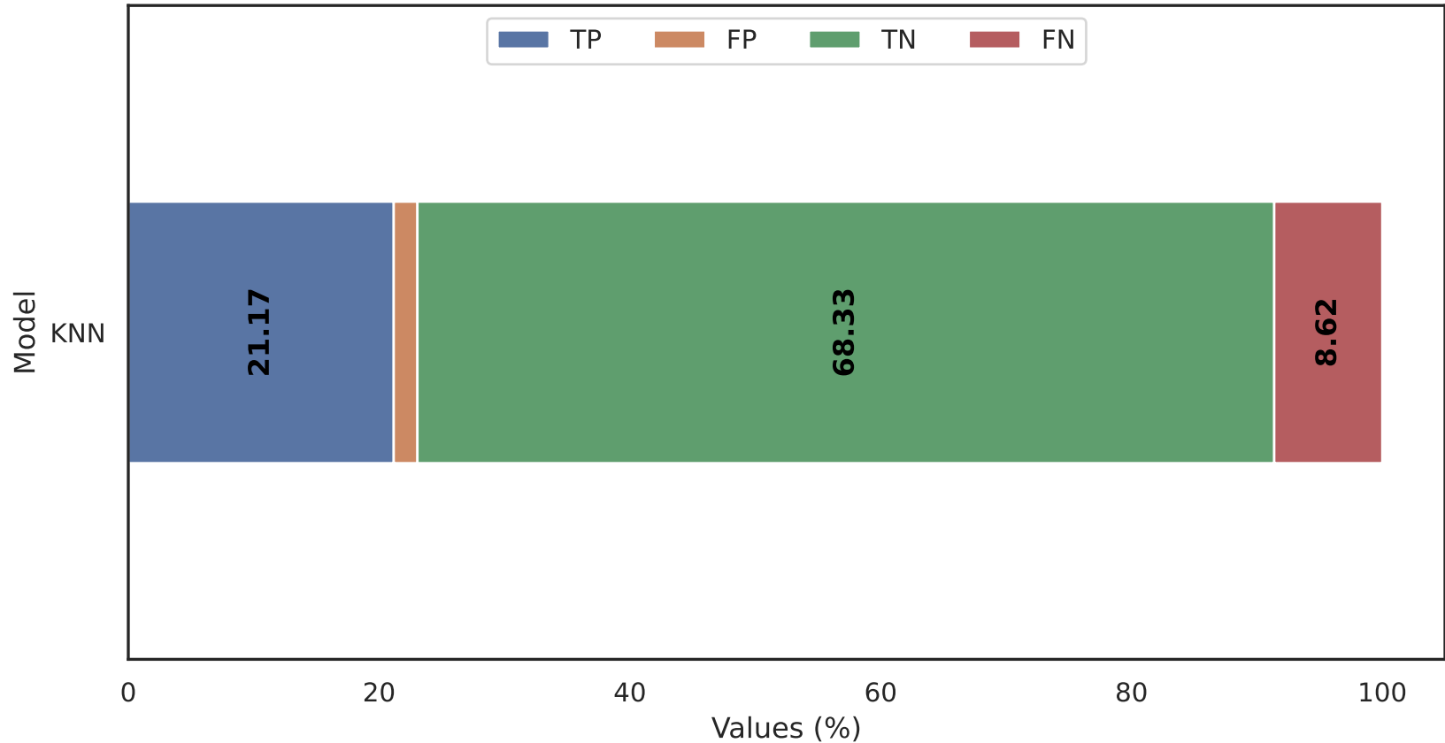
Classification to semidroid With Dataset in adroit.csv
