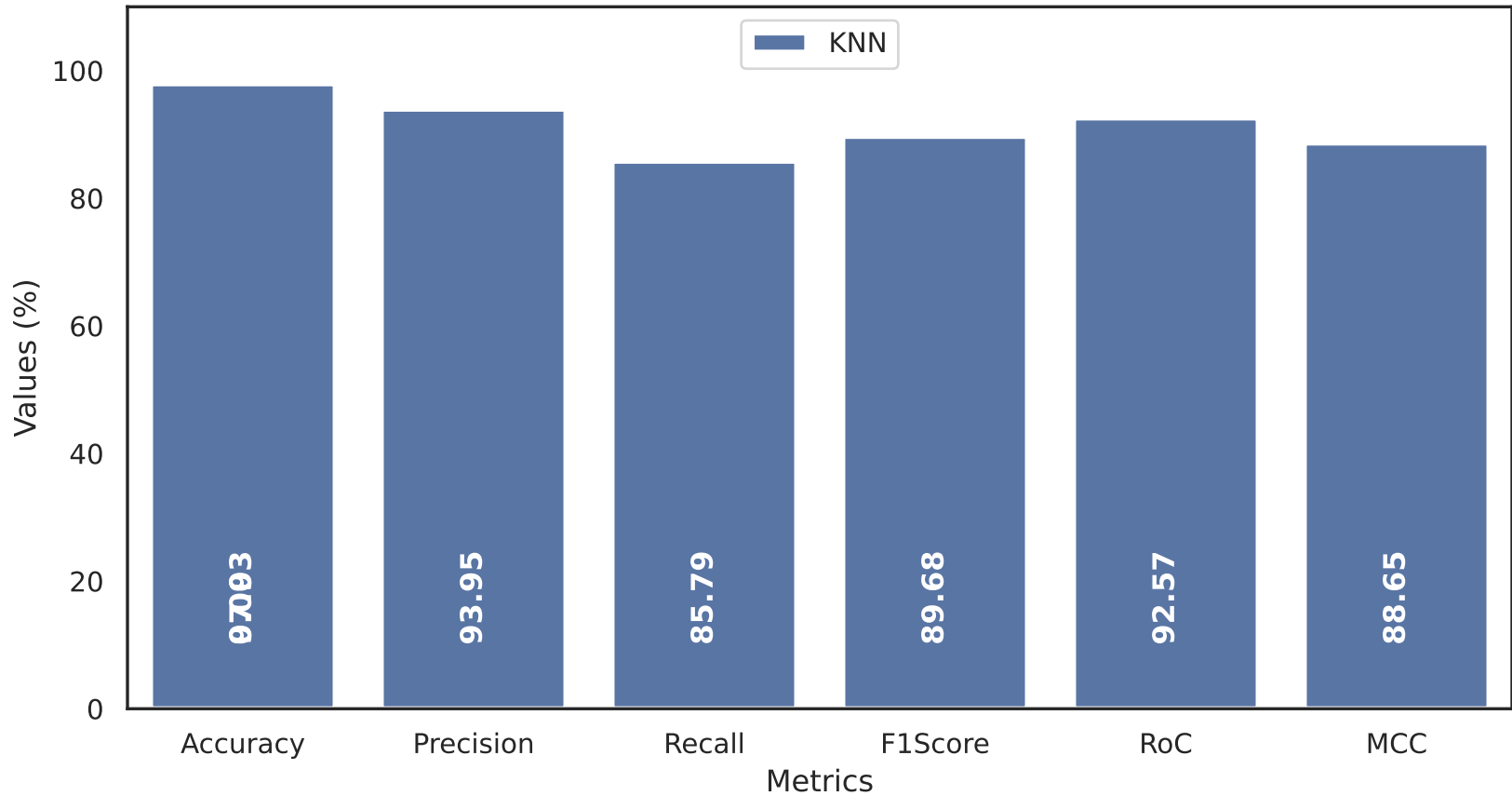
Results for rfe With Dataset in androcrawl.csv
