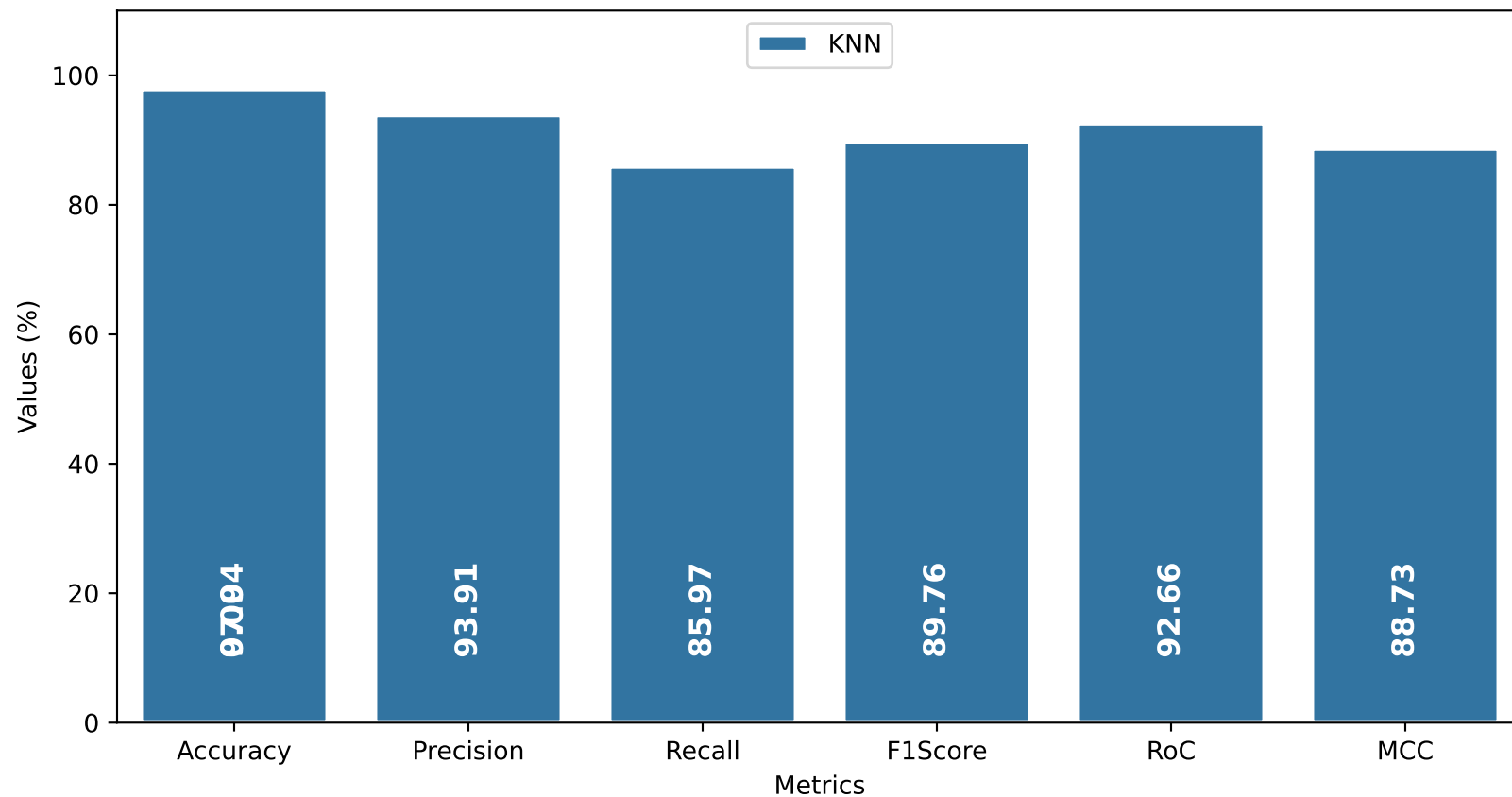
Results for semidroid With Dataset in androcrawl.csv
