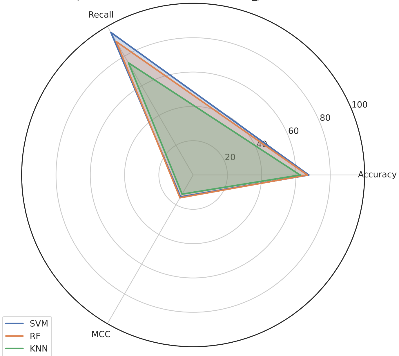
Comparison to rfe With Dataset in android_permissions.csv
