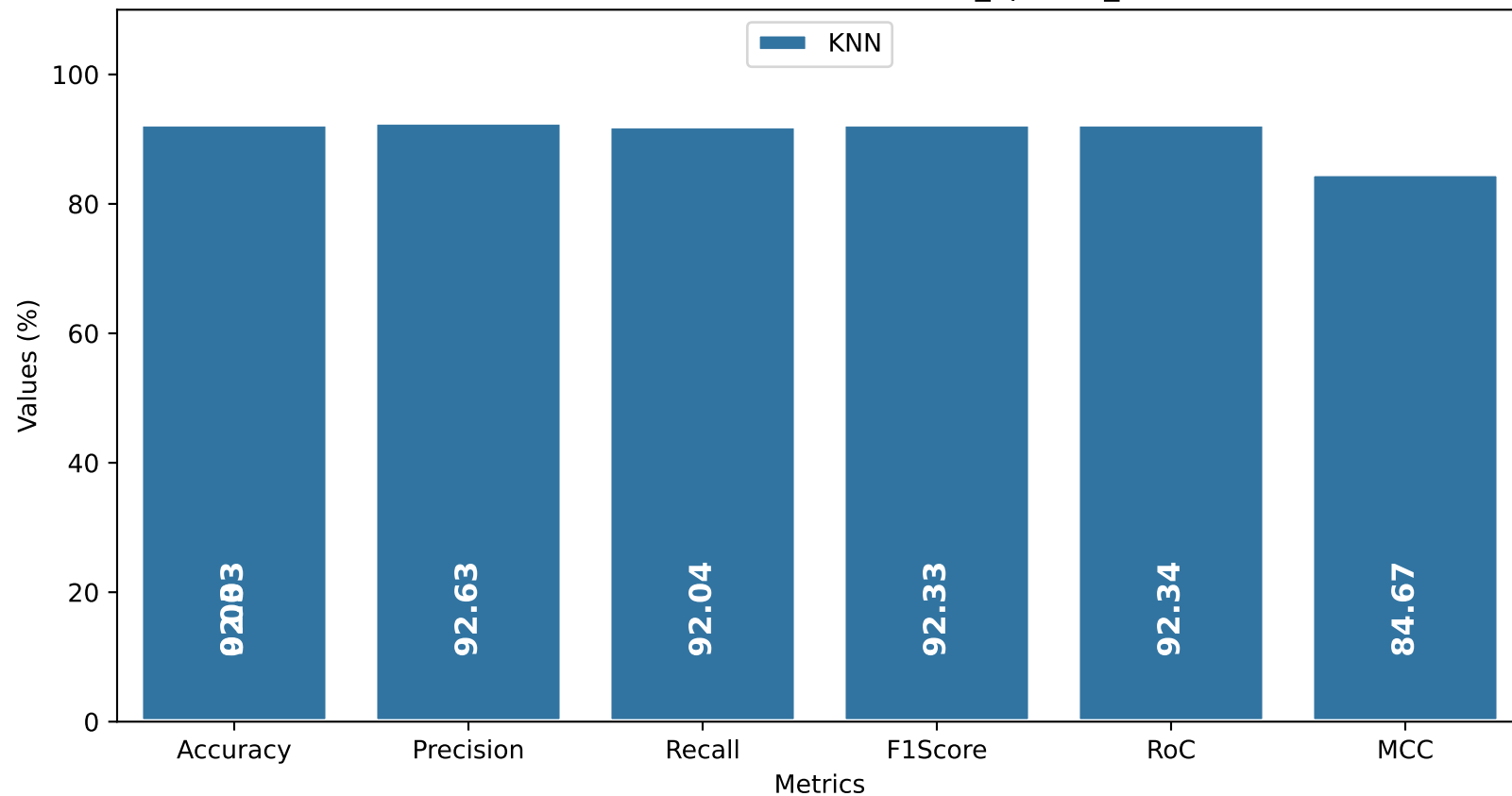
Results for rfe With Dataset in defendedroid_apicalls_closeness.csv
