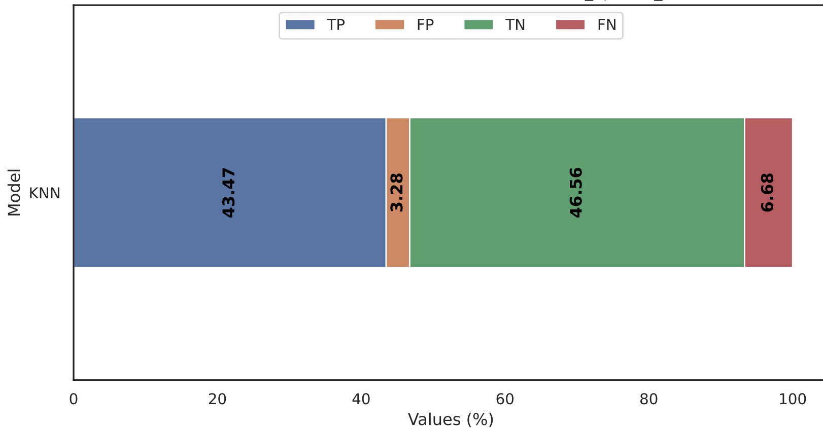
Classification to semidroid With Dataset in defendedroid_apicalls_closeness.csv
