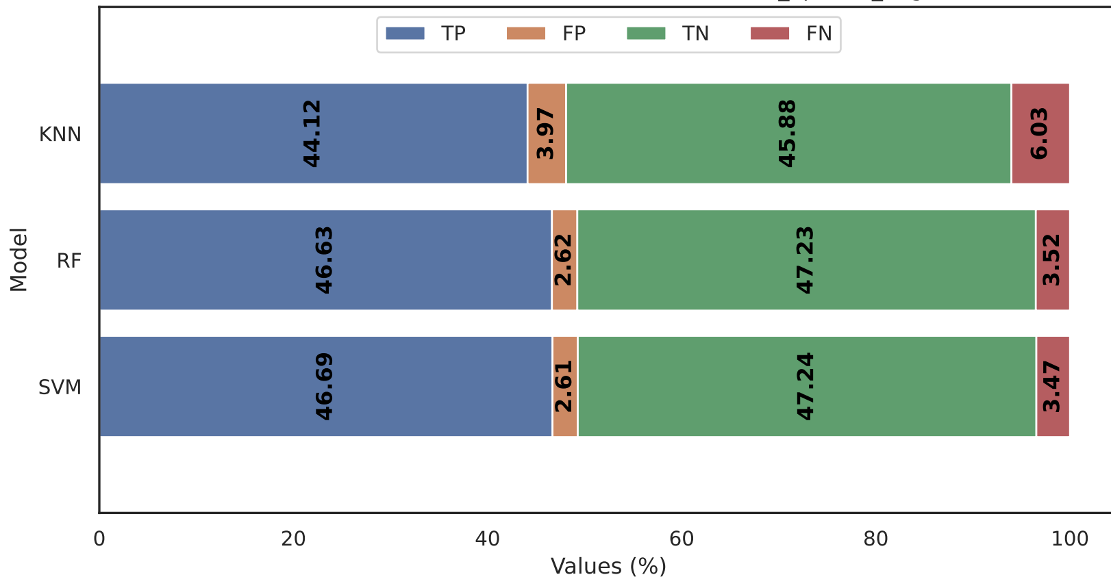
Classification to lasso With Dataset in defensedroid_apicalls_degree.csv
