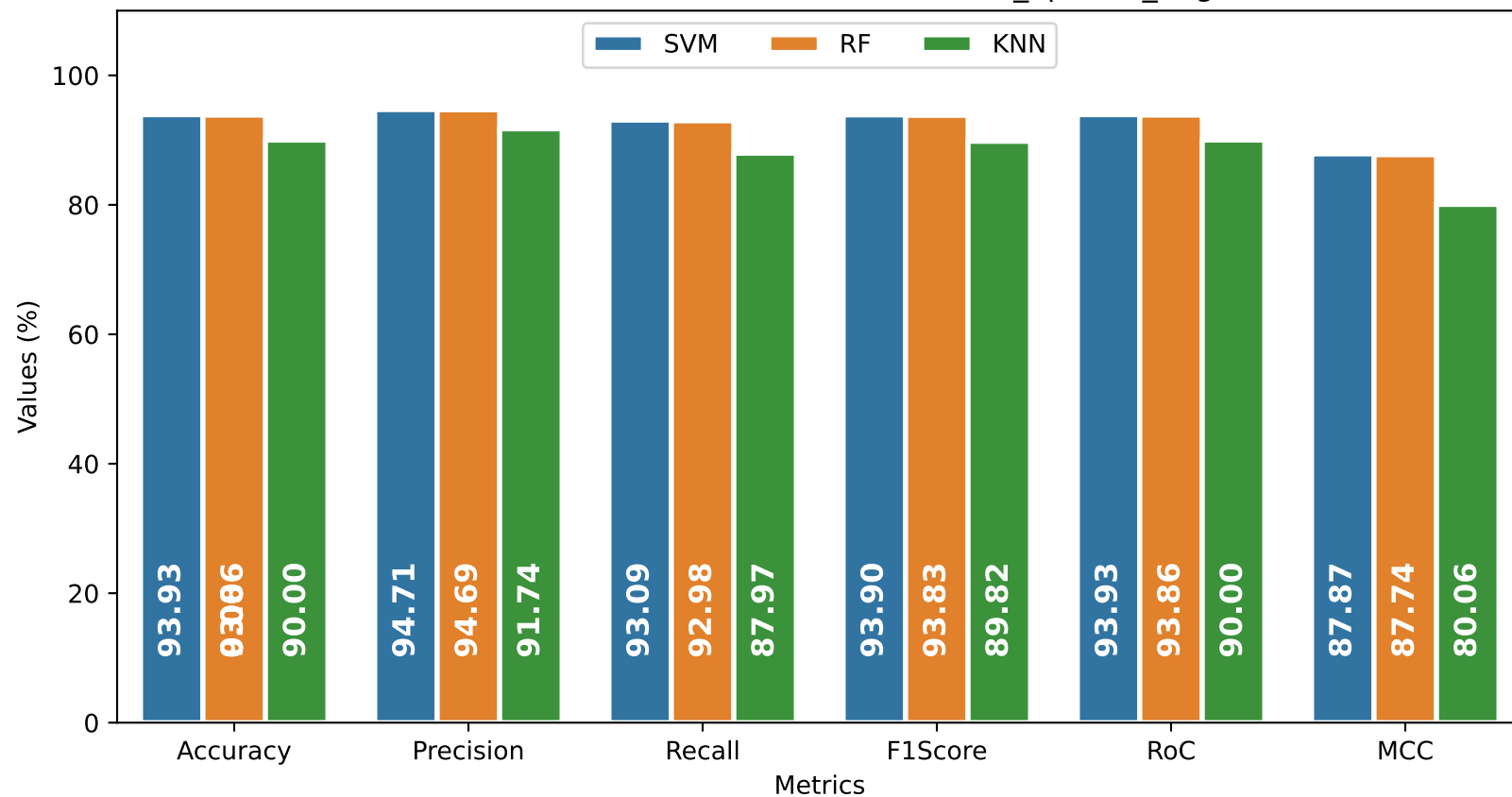
Results for lasso With Dataset in defensedroid_apicalls_degree.csv
