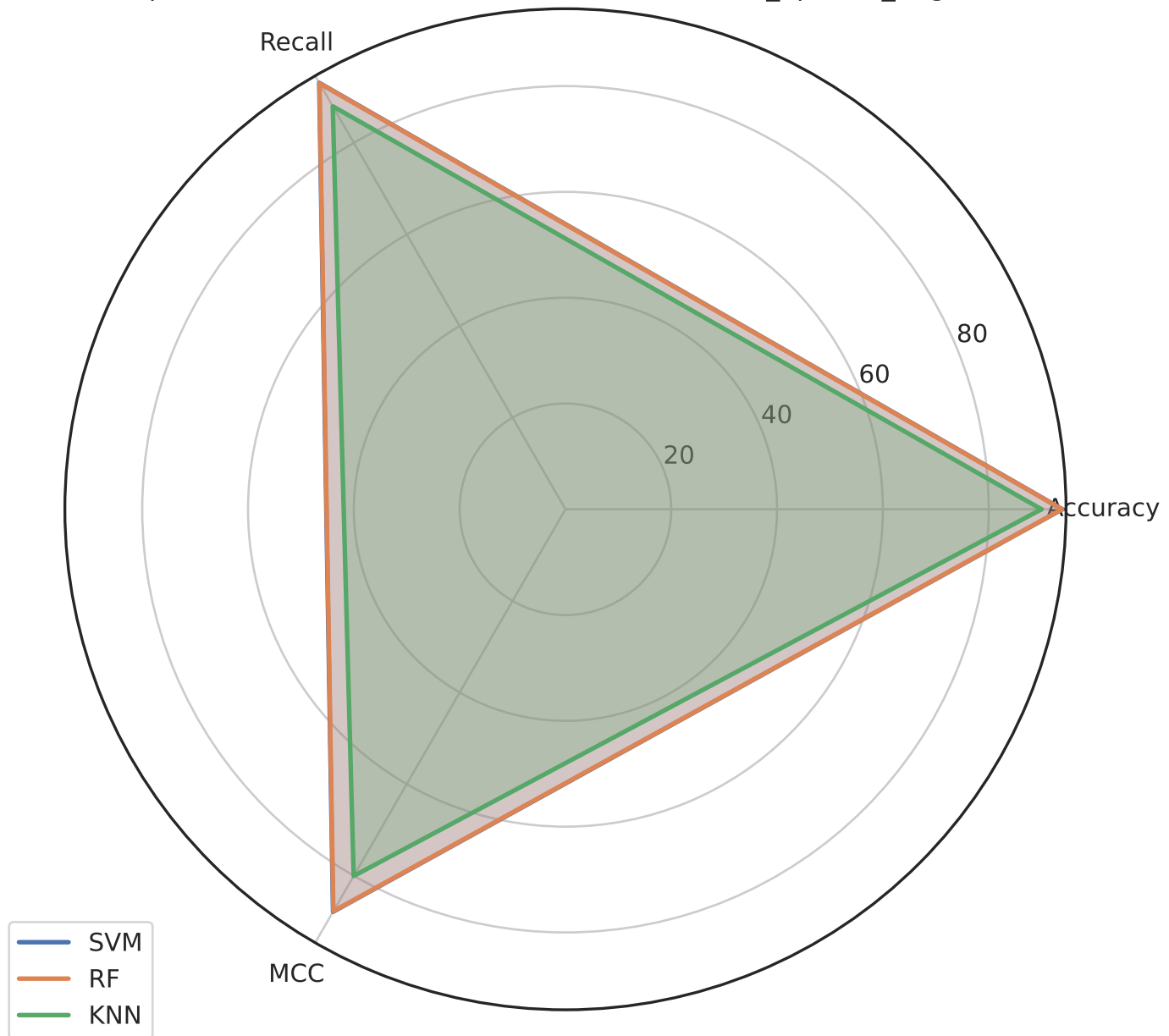
Comparison to lasso With Dataset in defendedroid_apicalls_degree.csv
