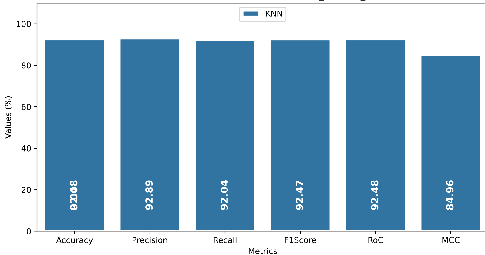
Results for rfe With Dataset in defendedroid_apicalls_degree.csv
