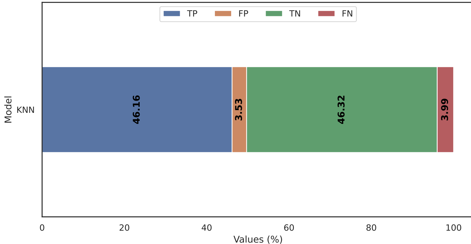
Classification to rfe With Dataset in defendedroid_apicalls_katz.csv
