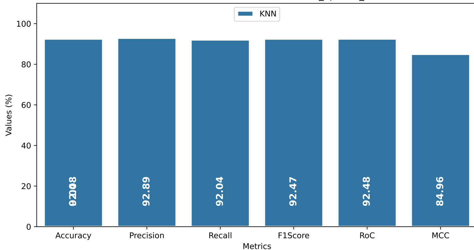
Results for rfe With Dataset in defendedroid_apicalls_katz.csv
