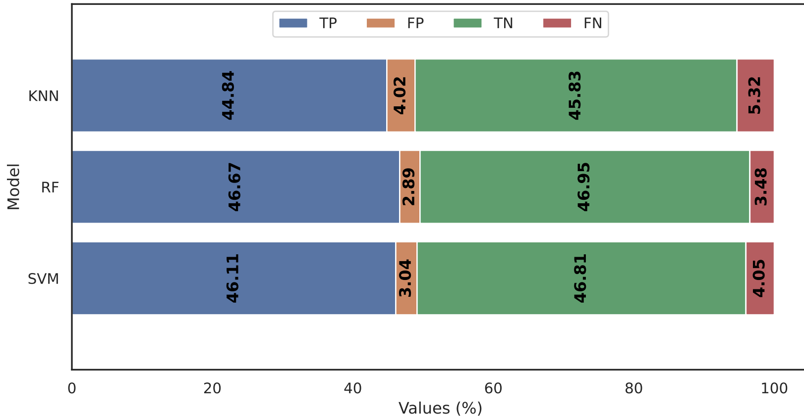
Classification to semidroid With Dataset in defendedroid_apicalls_katz.csv
