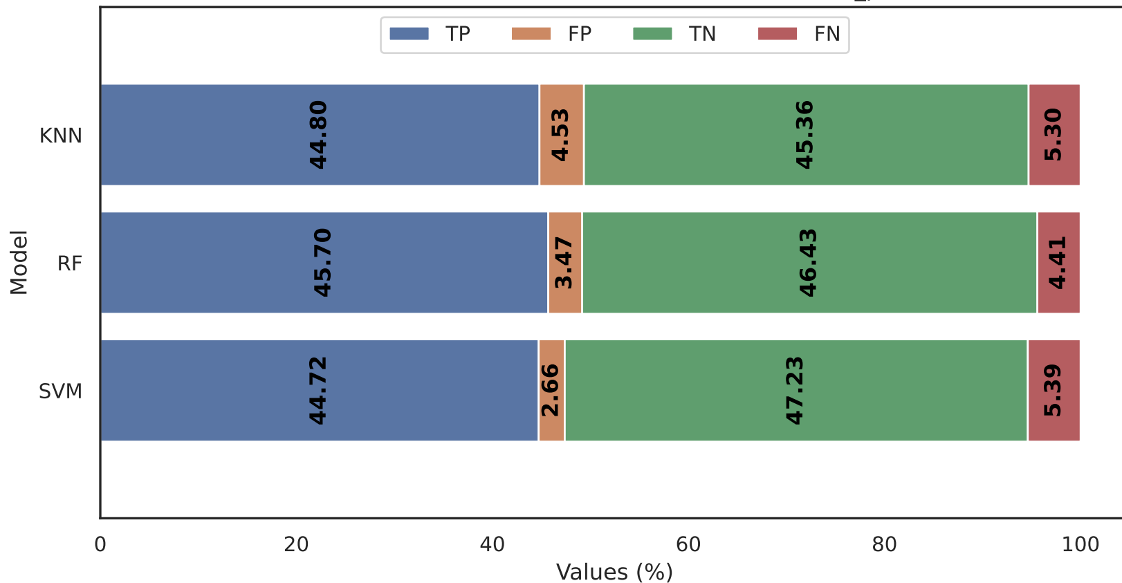
Classification to lasso With Dataset in defendedroid_prs.csv
