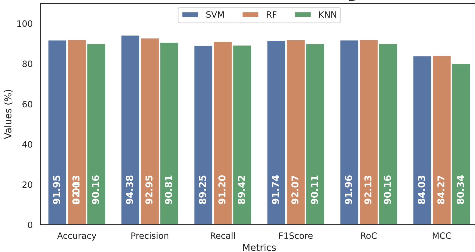
Results for lasso With Dataset in defendedroid_prs.csv
