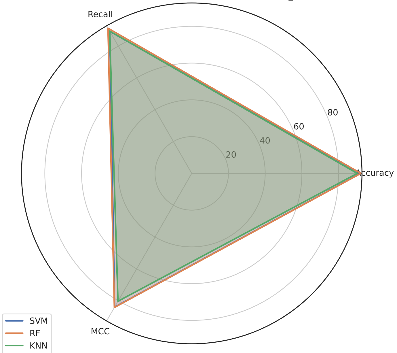
Comparison to lasso With Dataset in defendedroid_prs.csv
