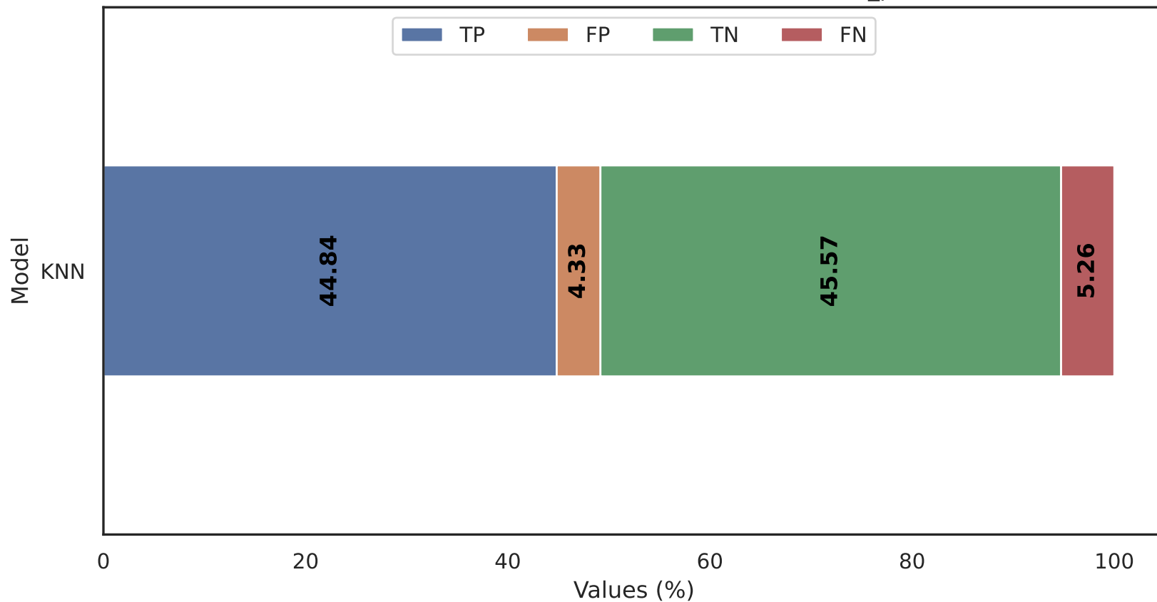
Classification to rfe With Dataset in defendedroid_prs.csv
