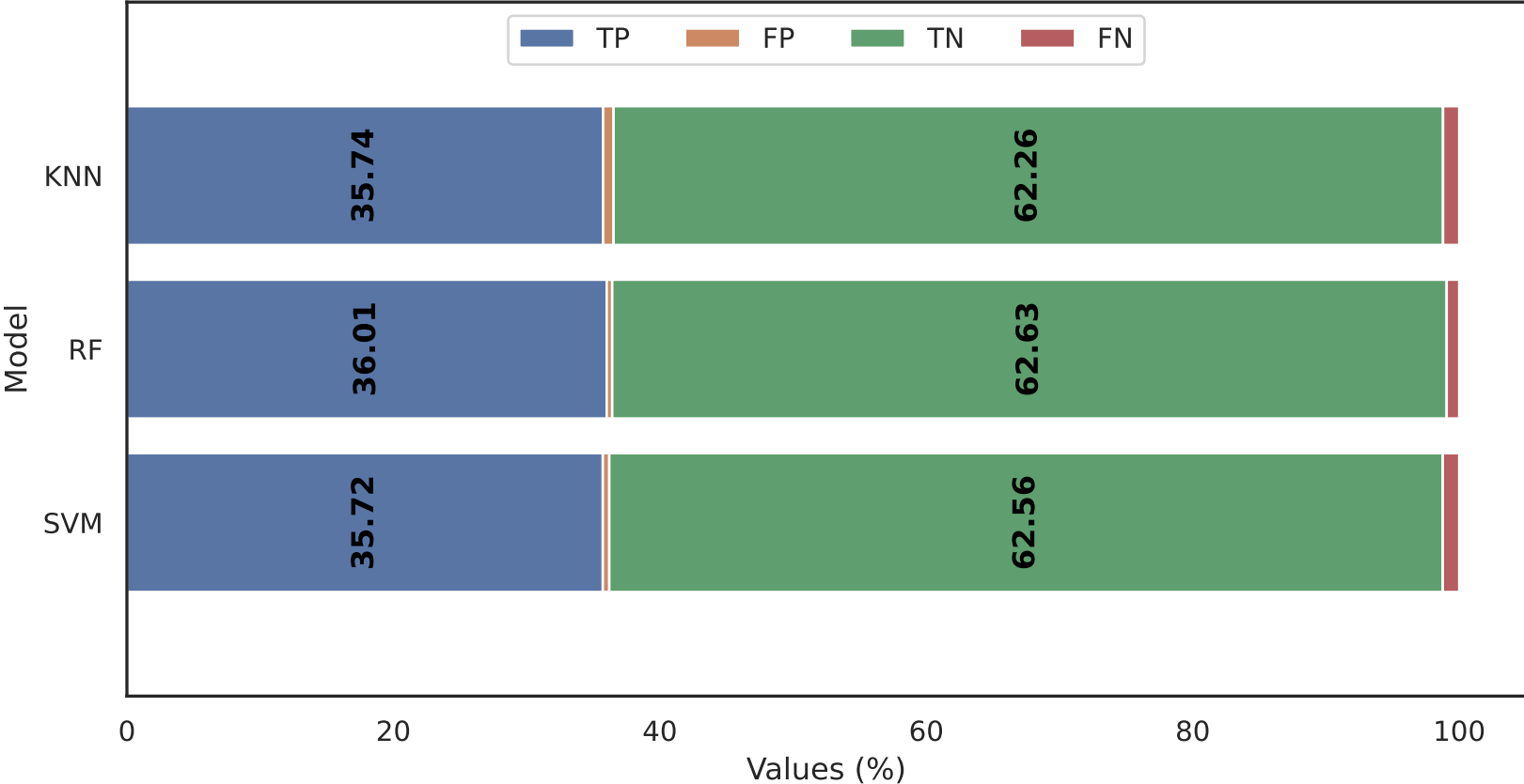
Classification to rfe With Dataset in drebin215.csv
