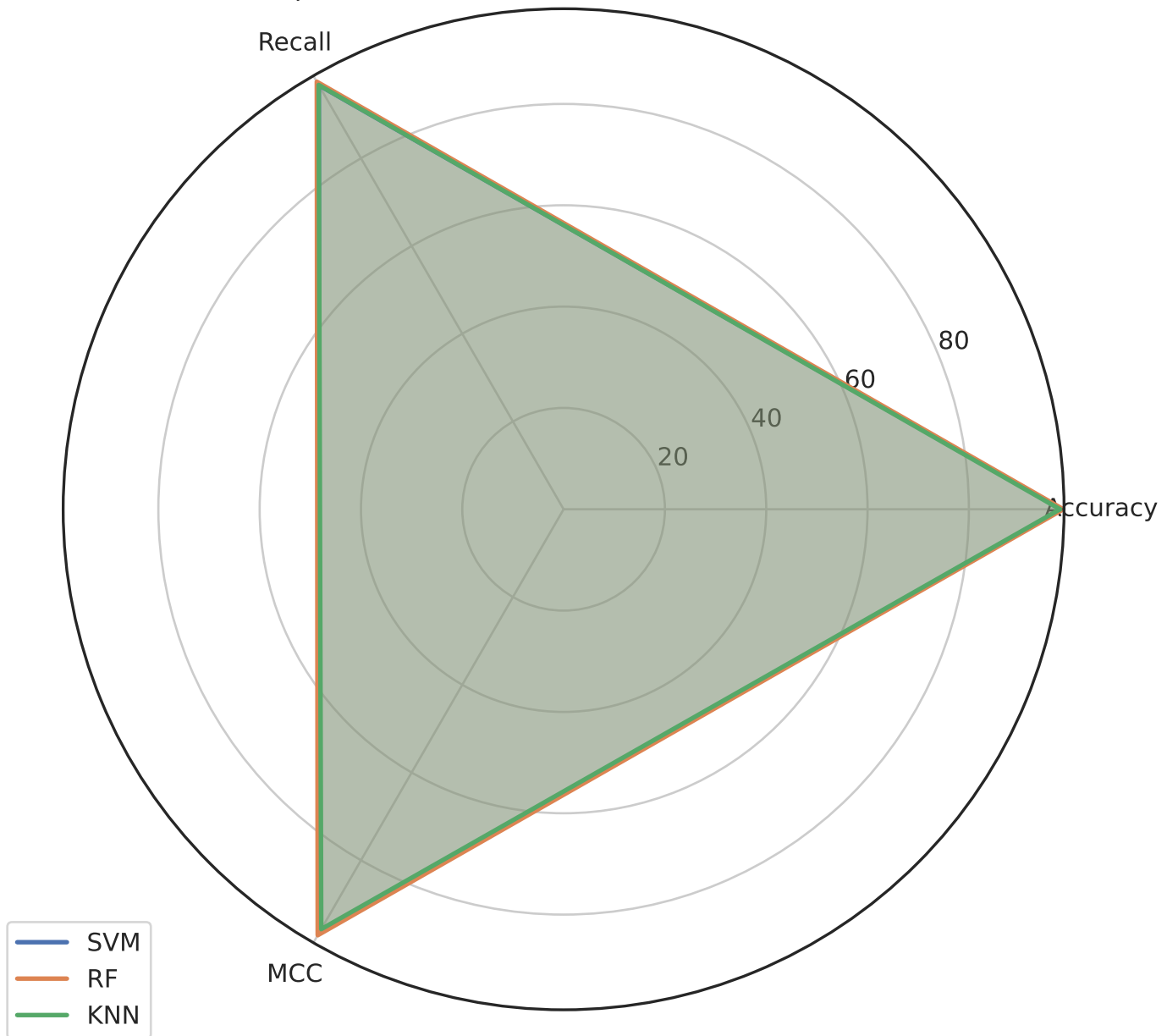
Comparison to rfe With Dataset in drebin215.csv
