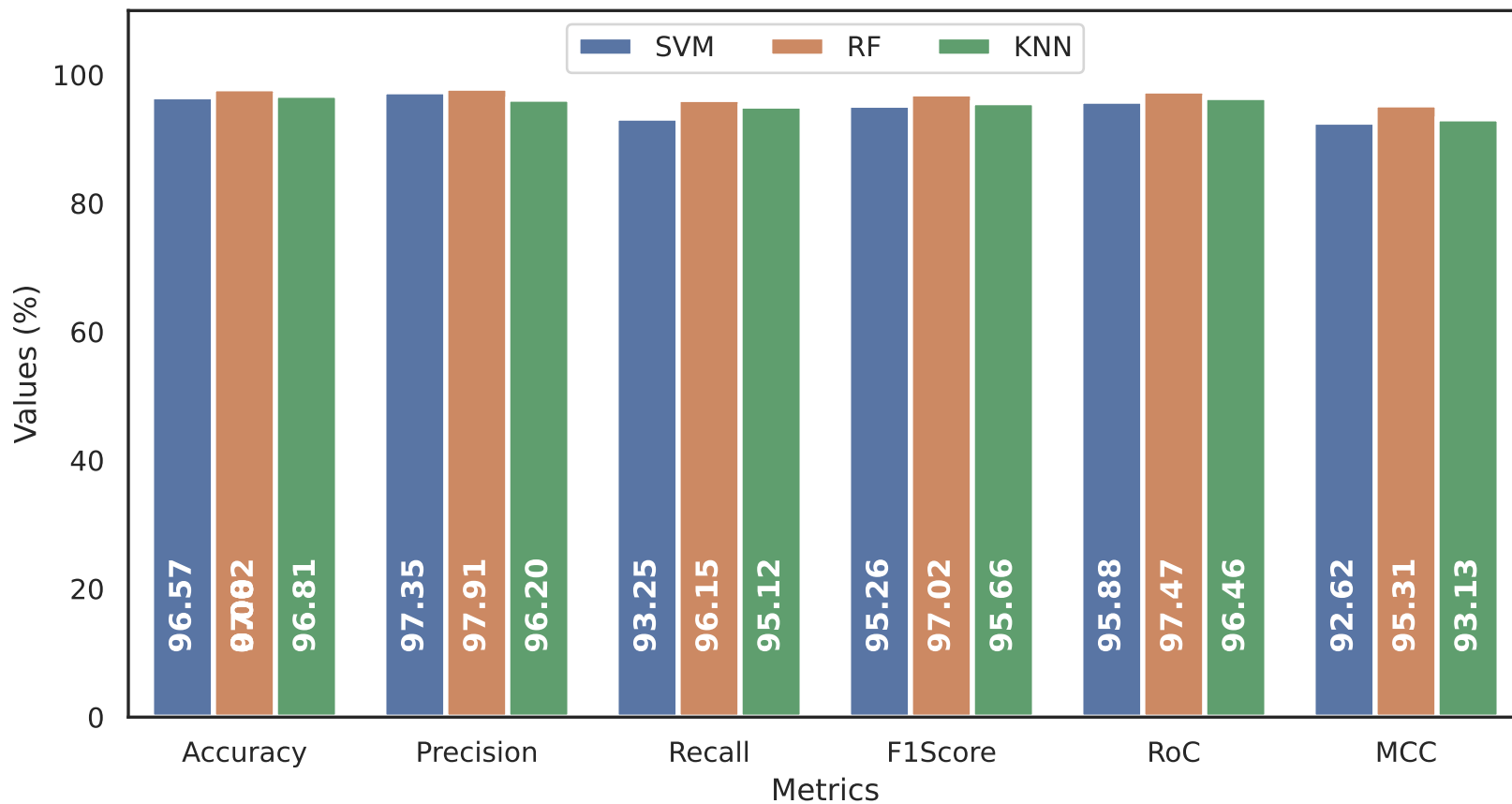
Results for semidroid With Dataset in drebin215.csv
