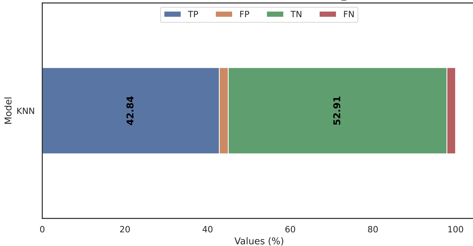
Classification to lasso With Dataset in kronodroid_emulator.csv
