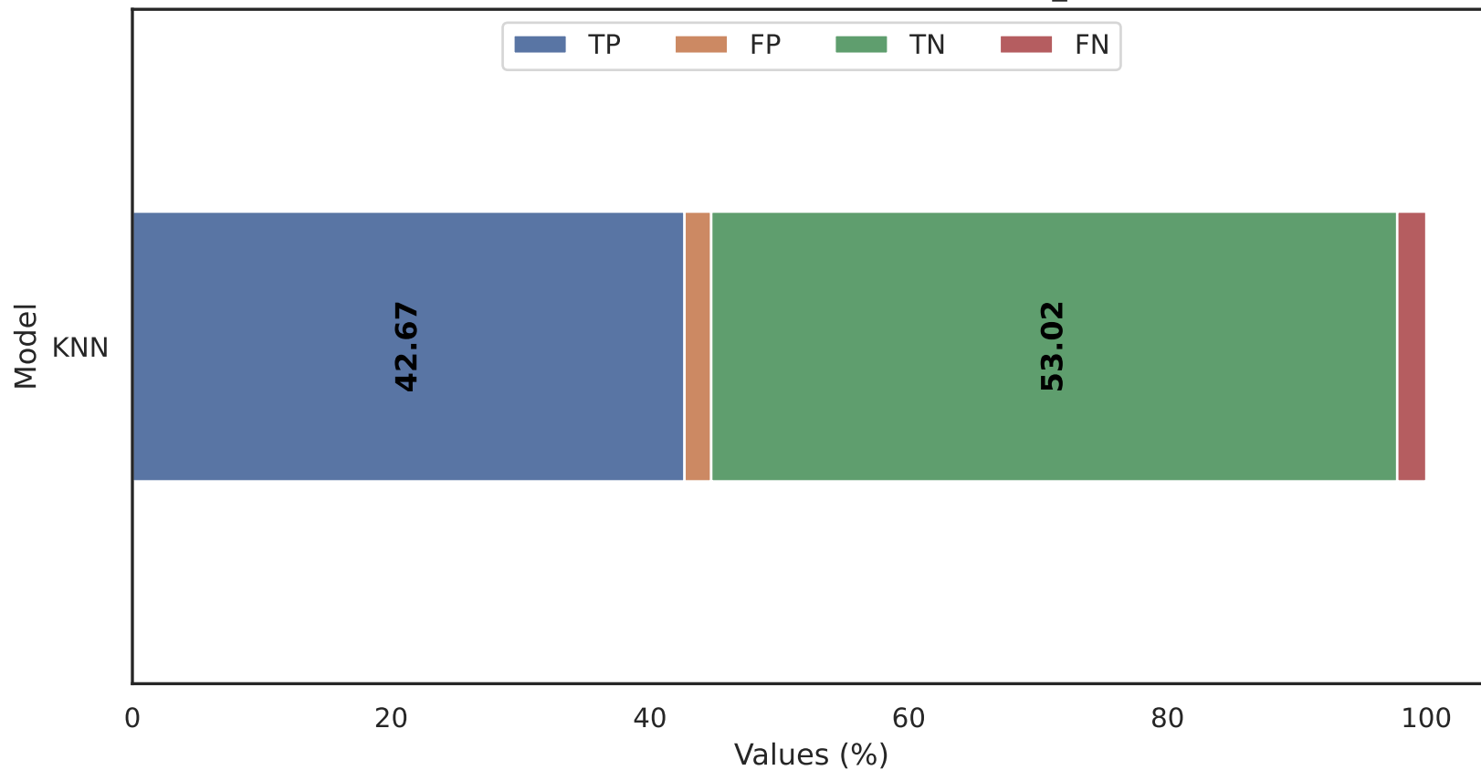
Classification to rfe With Dataset in kronodroid_emulator.csv
