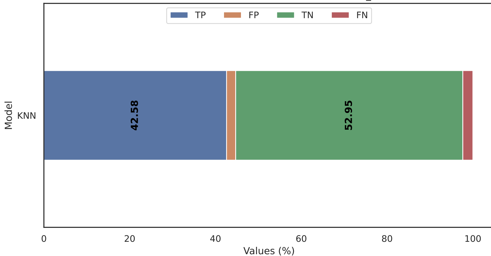
Classification to semidroid With Dataset in kronodroid_emulator.csv
