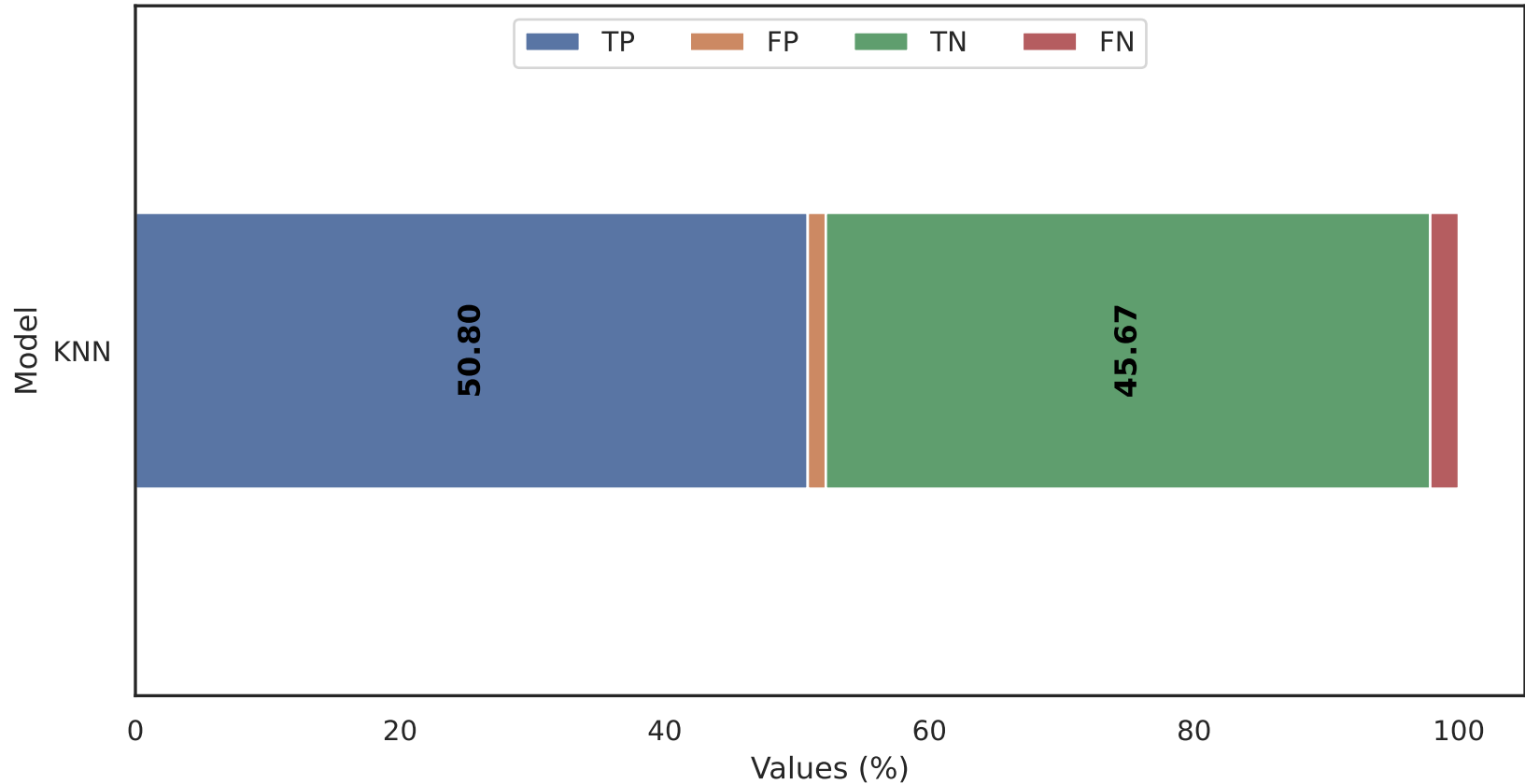
Classification to rfe With Dataset in kronodroid_real_device.csv
