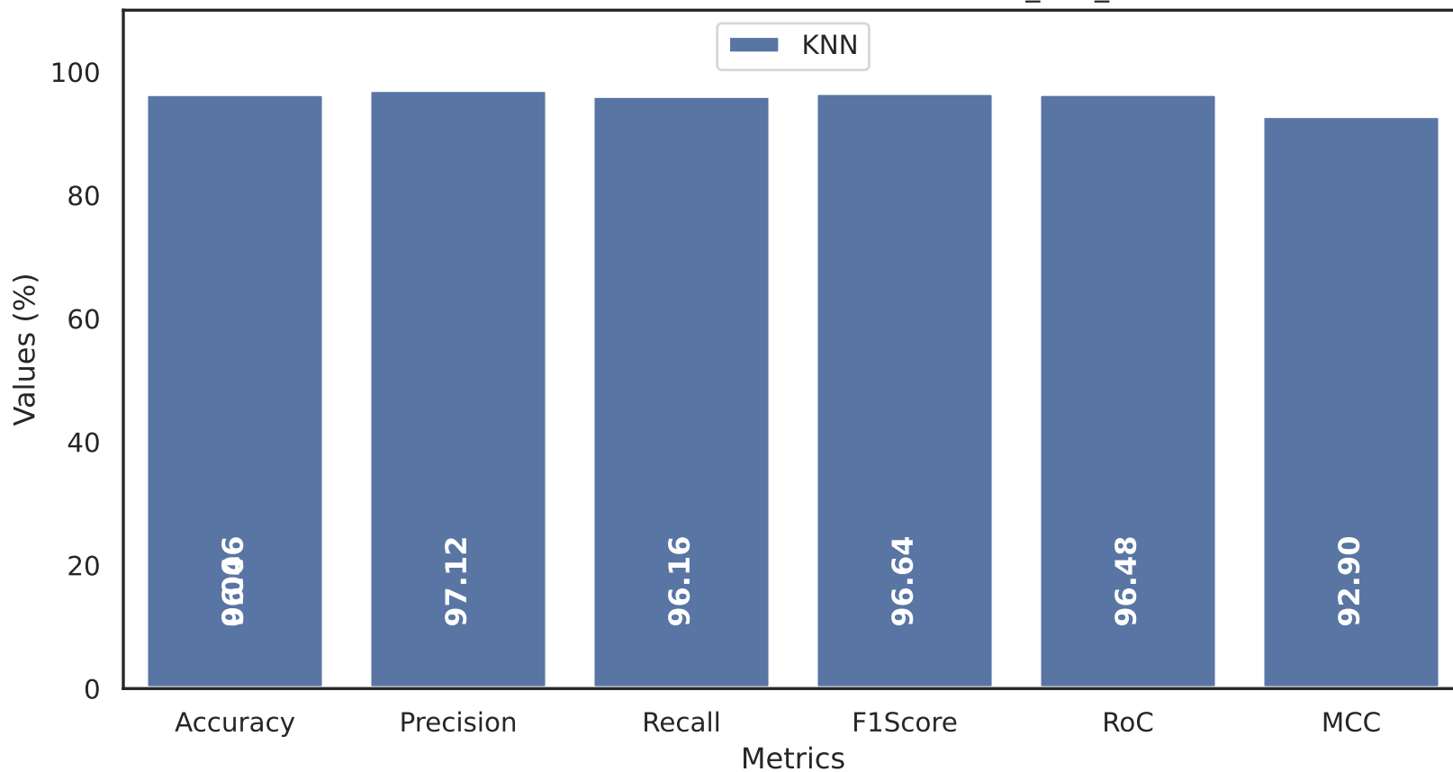
Results for semidroid With Dataset in kronodroid_real_device.csv
