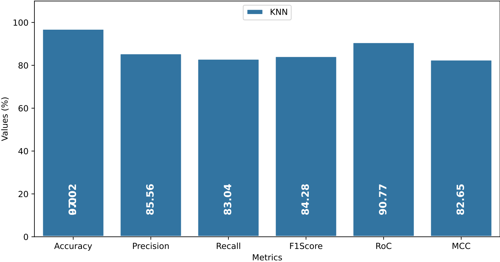
Results for semidroid With Dataset in mh100k.csv
