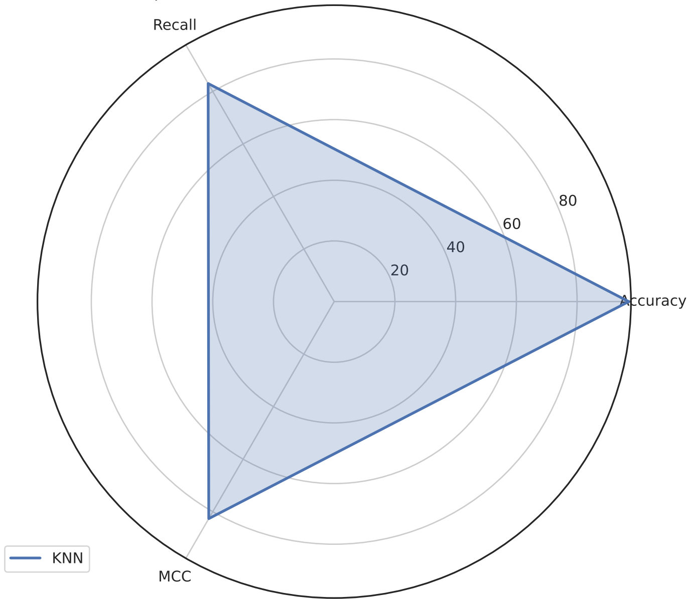
Comparison to semidroid With Dataset in mh100k.csv
