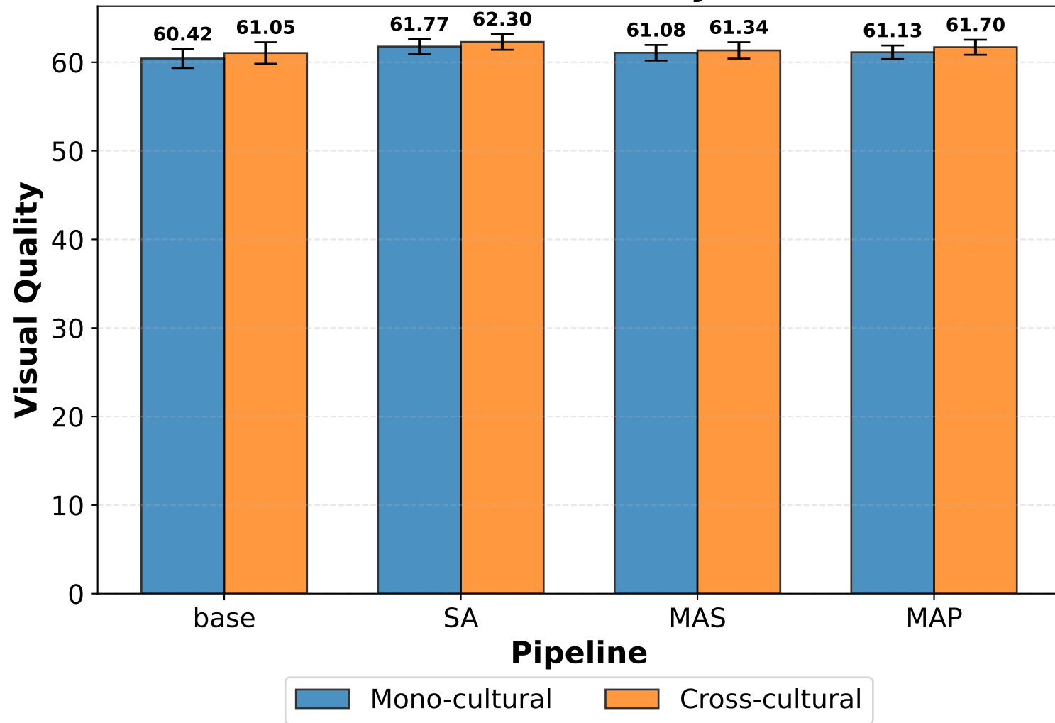
Visual Quality
