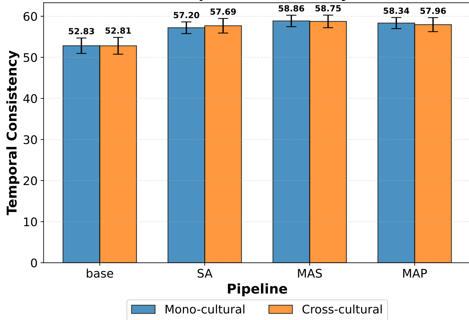
Temporal Consistency
