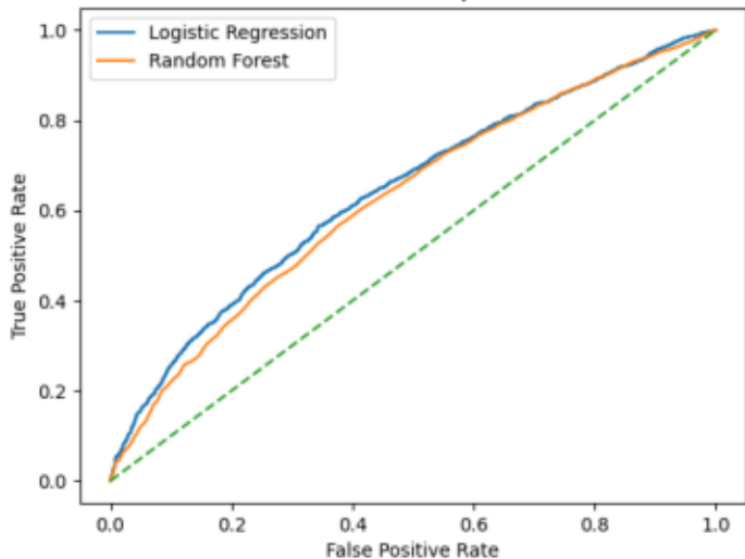
ROC Curve Comparison
