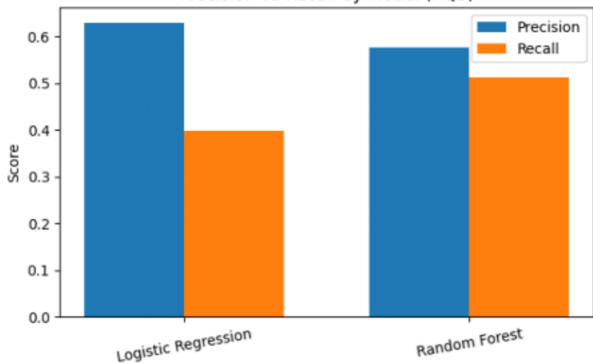
Precision vs Recall by Model (RQ3)
