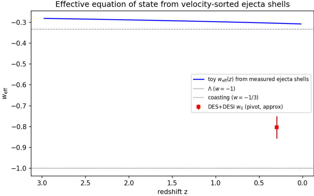
Figure 5: Fig. 5 — Toy effective equation of state from velocity-sorted ejecta shells: a few-percent drift near w = -1/3 , in the opposite direction to the DES+DESI w_0 w_a best fit, and of insufficient magnitude.
