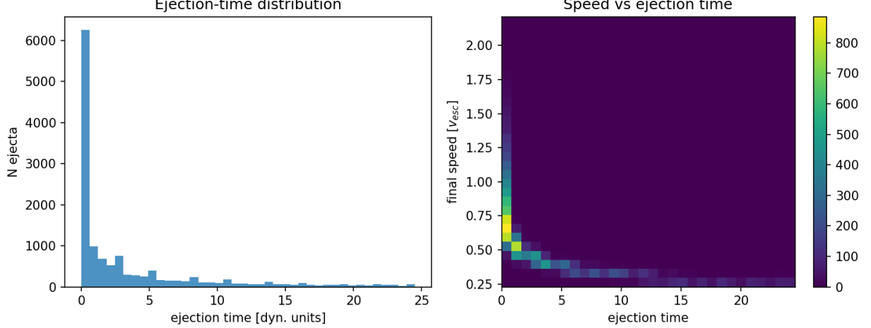
Figure 2: Fig. 2 — Ejecta kinematics over 15 seeds: ejection-time distribution (left) and speed vs ejection time (right), showing the velocity-sorted shell structure.
