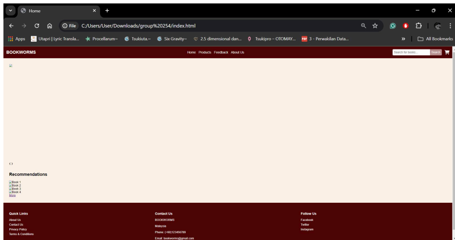
Figure 9: Homepage draft
