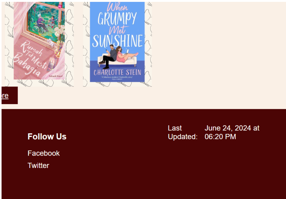
Figure 15: Maintanance update
