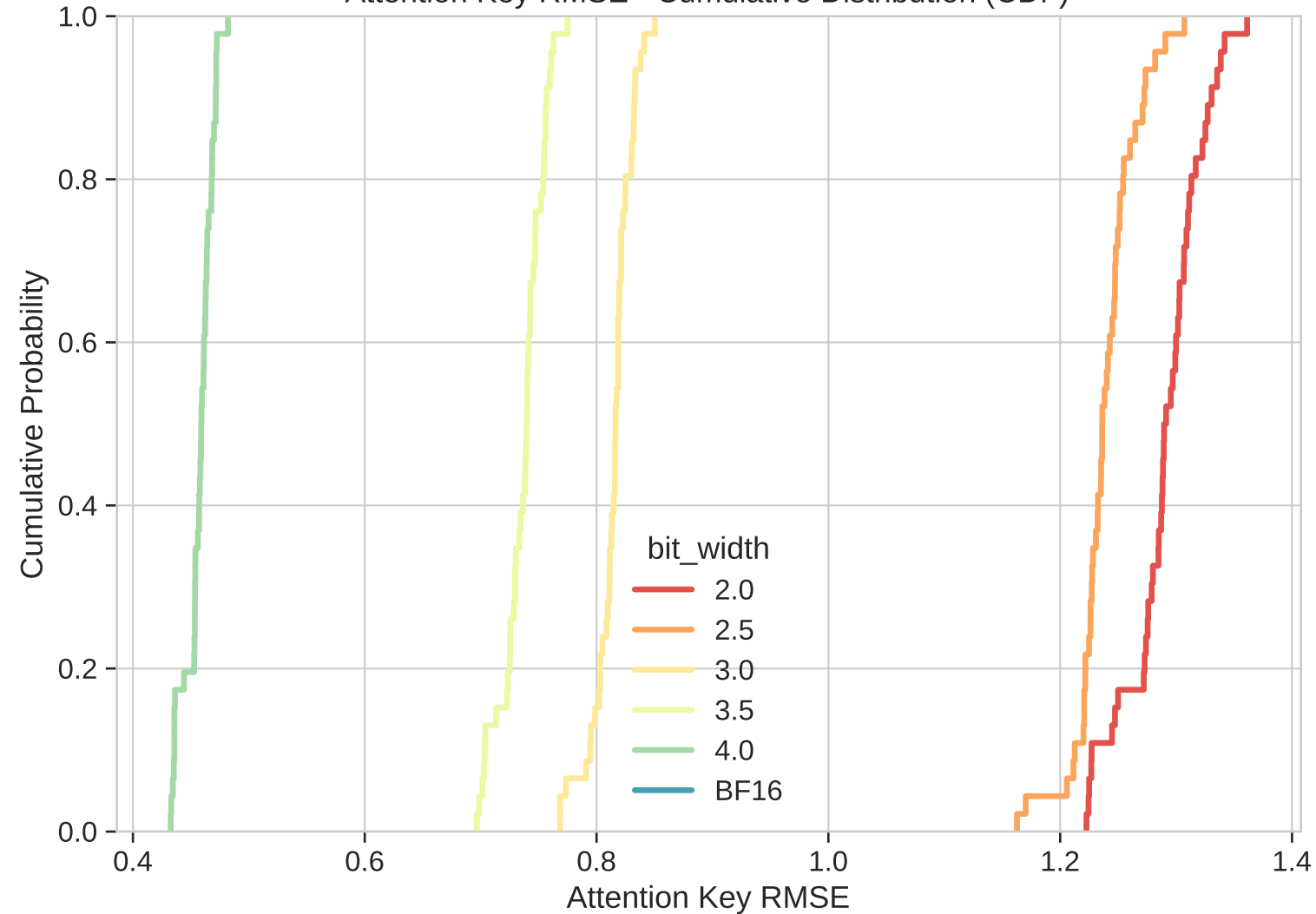
Attention Key RMSE - Cumulative Distribution (CDF)
